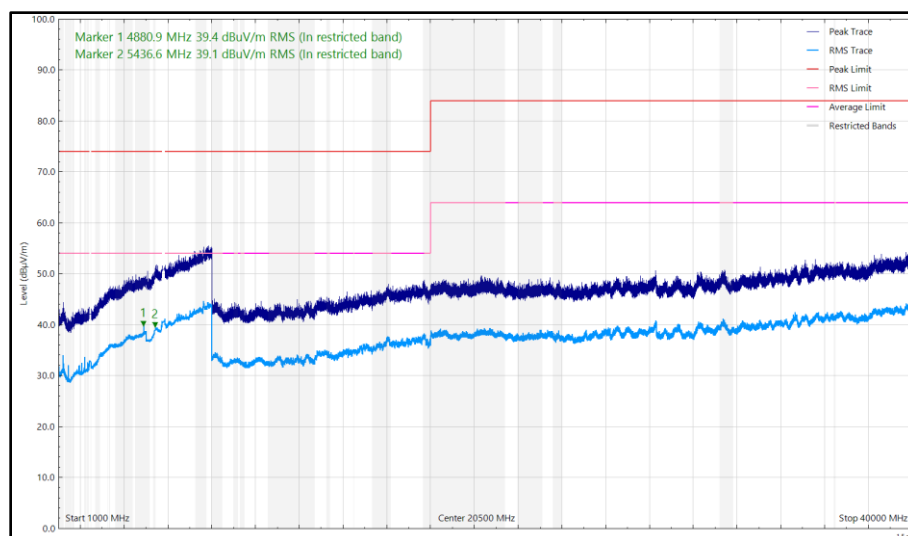
Figure 79 - U-NII-3 - 5785 MHz (CH157), HT20, CDD, Core 0 + Core 1 and 2440 MHz (CH18), ePA, Core 1, 1 GHz to 40 GHz, Horizontal
