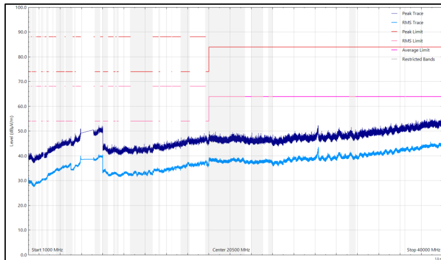
Figure 111 - U-NII-5 - 6175 MHz (CH45), HE20, SU, CDD, Core 0 + Core 1 and 2440 MHz (CH18), iPA, Core 2, 1 GHz to 40 GHz, Horizontal
