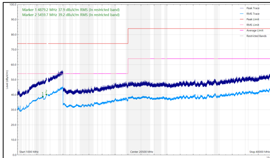
Figure 71 - U-NII-2C - 5640 MHz (CH128), HT20, CDD, Core 0 + Core 1 and 2440 MHz (CH18), ePA, Core 1, 1 GHz to 40 GHz, Horizontal
