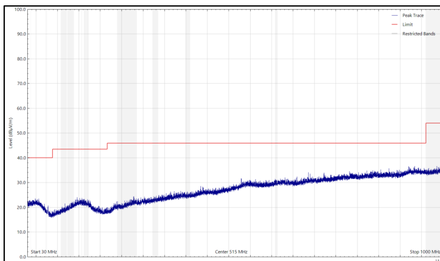
Figure 76 - U-NII-3 - 5785 MHz (CH157), HT20, CDD, Core 0 + Core 1 and 2440 MHz (CH18), ePA, Core 0, 30 MHz to 1 GHz, Vertical (Peak)
