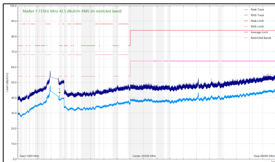
Figure 103 - U-NII-8 - 6995 MHz (CH209), HE20, SU, CDD, Core 0 + Core 1 and 2440 MHz (CH18), ePA, Core 0, 1 GHz to 40 GHz, Horizontal
