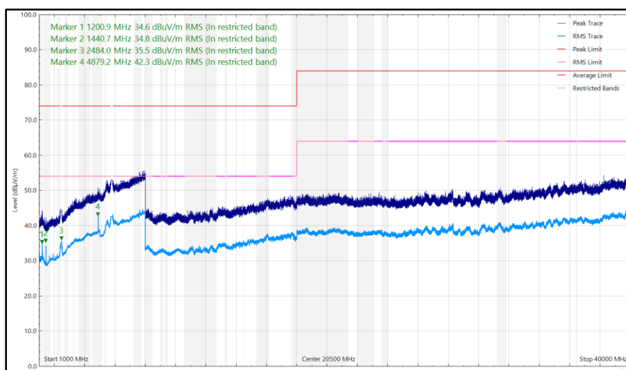
Figure 77 - U-NII-3 - 5785 MHz (CH157), HT20, CDD, Core 0 + Core 1 and 2440 MHz (CH18), ePA, Core 0, 1 GHz to 40 GHz, Vertical
