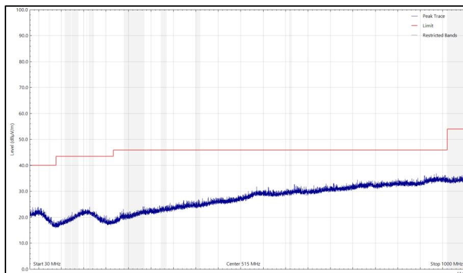
Figure 72 - U-NII-2C - 5640 MHz (CH128), HT20, CDD, Core 0 + Core 1 and 2440 MHz (CH18), ePA, Core 1, 30 MHz to 1 GHz, Vertical (Peak)
