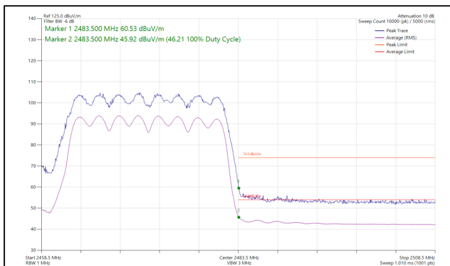
Figure 51 - 802.11ax HE20, SU, CDD, Core 0 - Core 1 - 2472 MHz Band Edge Frequency 2483.5 MHz
