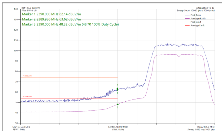
Figure 23 - 802.11n HT20, SISO, Core 1 - 2412 MHz Band Edge Frequency 2390 MHz
