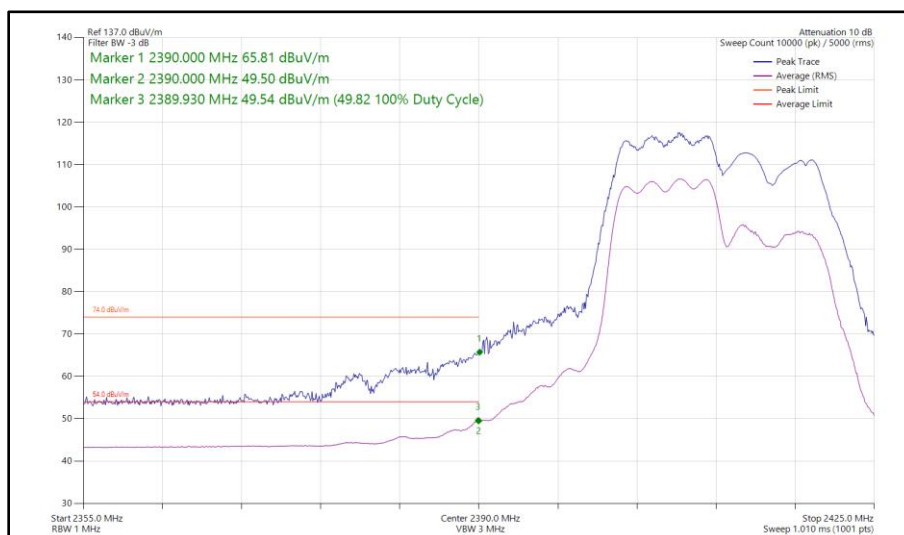
Figure 43 - 802.11ax HE20, RU 106-53, CDD, Core 0 - Core 1 - 2412 MHz Band Edge Frequency 2390 MHz
