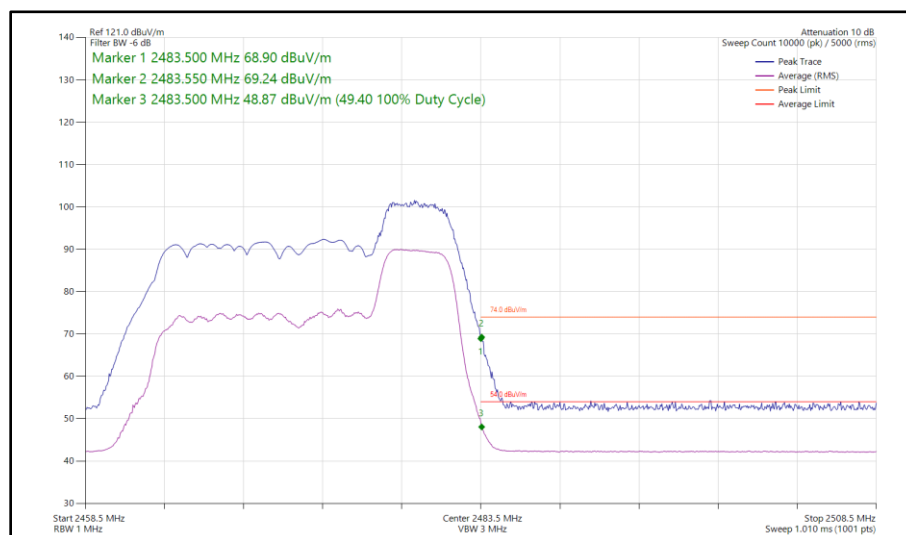
Figure 20 - 802.11ax HE20, RU 52-40, SISO, Core 0 - 2472 MHz Band Edge Frequency 2483.5 MHz
