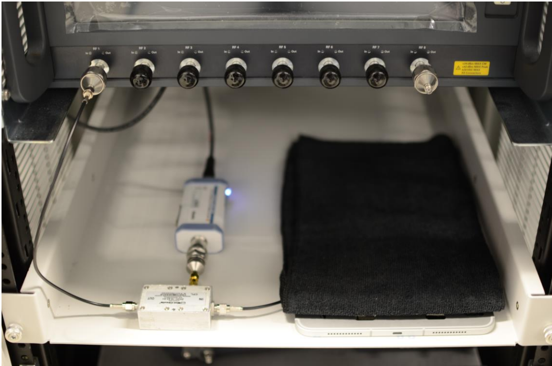
Test Setup Photo 2 – Conducted Test Setup (Figure 5-1a)
