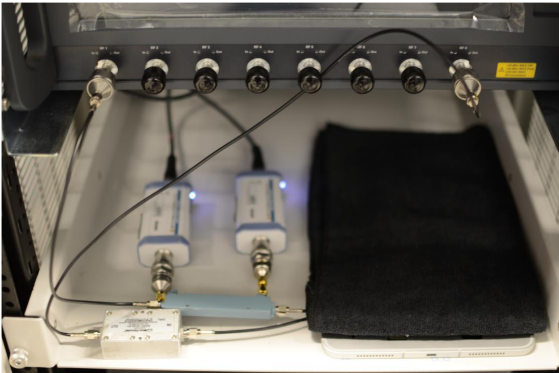
Test Setup Photo 4 – Conducted Test Setup (Figure 5-1c)
