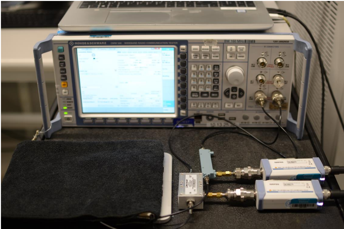
Test Setup Photo 5 – Conducted Test Setup (Figure 5-1d)
