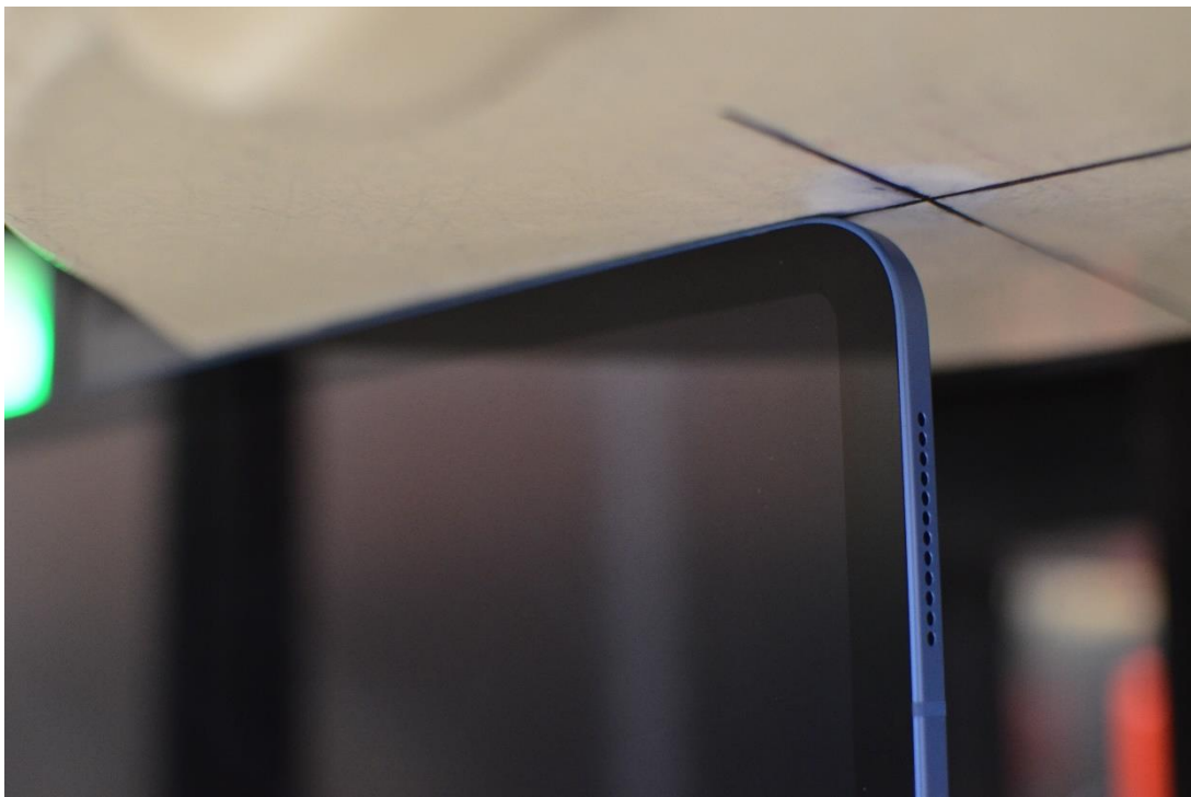
SAR Test Setup Photo 7 – Body, Left Edge at 0mm, Antennas 3a/3b/3c/4
