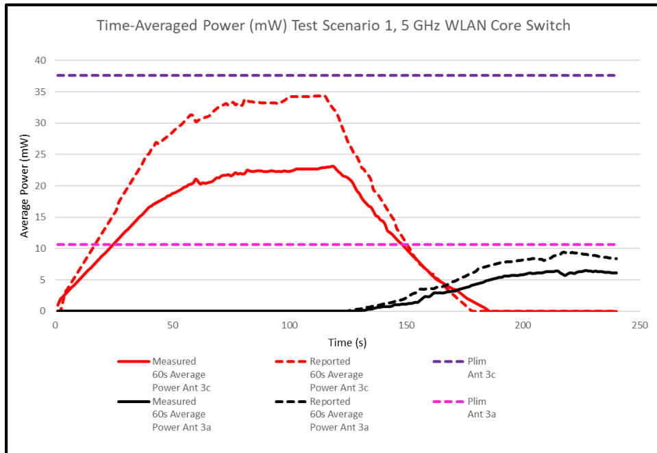
Figure K-4 60s Average Power vs. Time, 5 GHz
