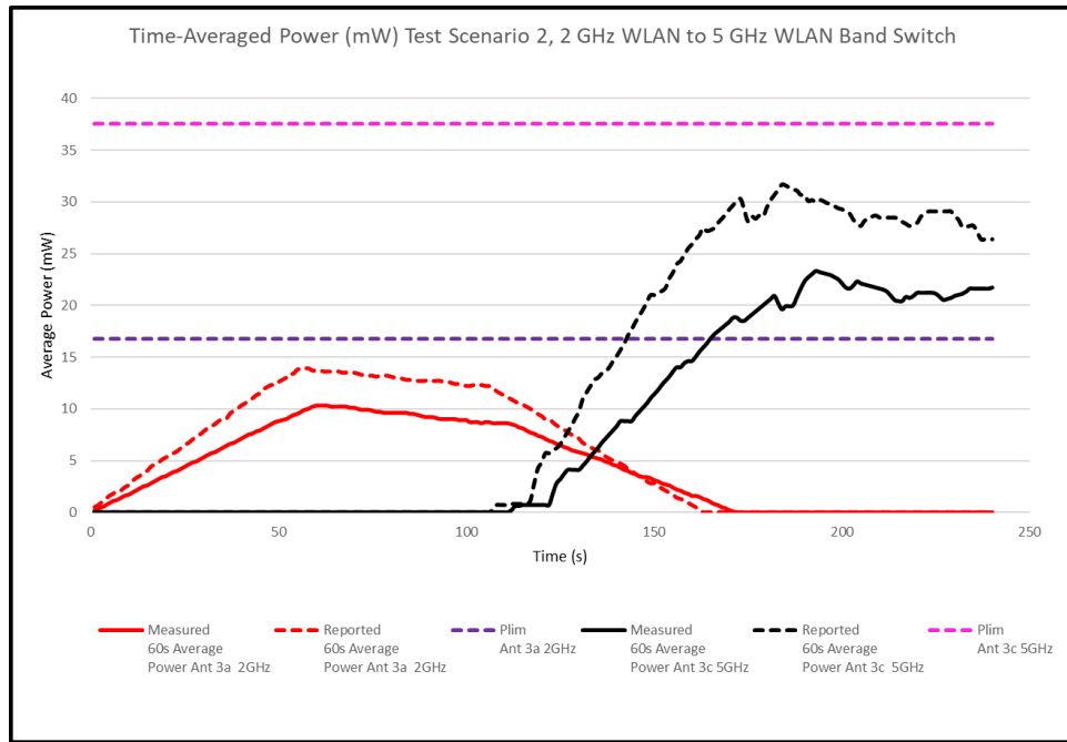
Figure K-6 60s Average Power vs. Time during Band Switch
