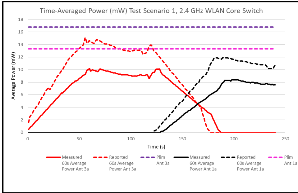
Figure K-2 60s Average Power vs. Time, 2.4 GHz
