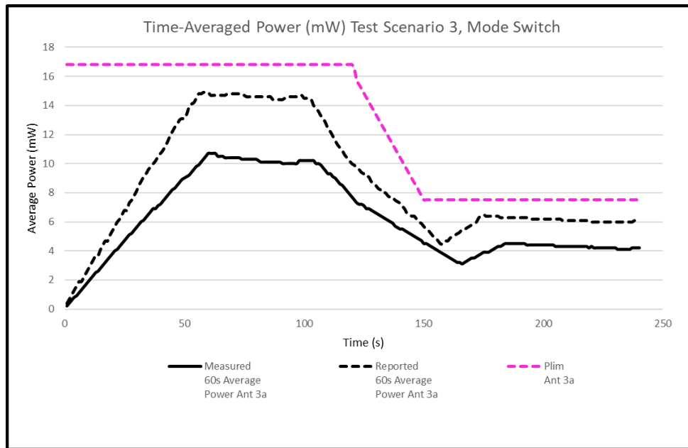
Figure K-8 60s Average Power vs. Time during Mode Switch
