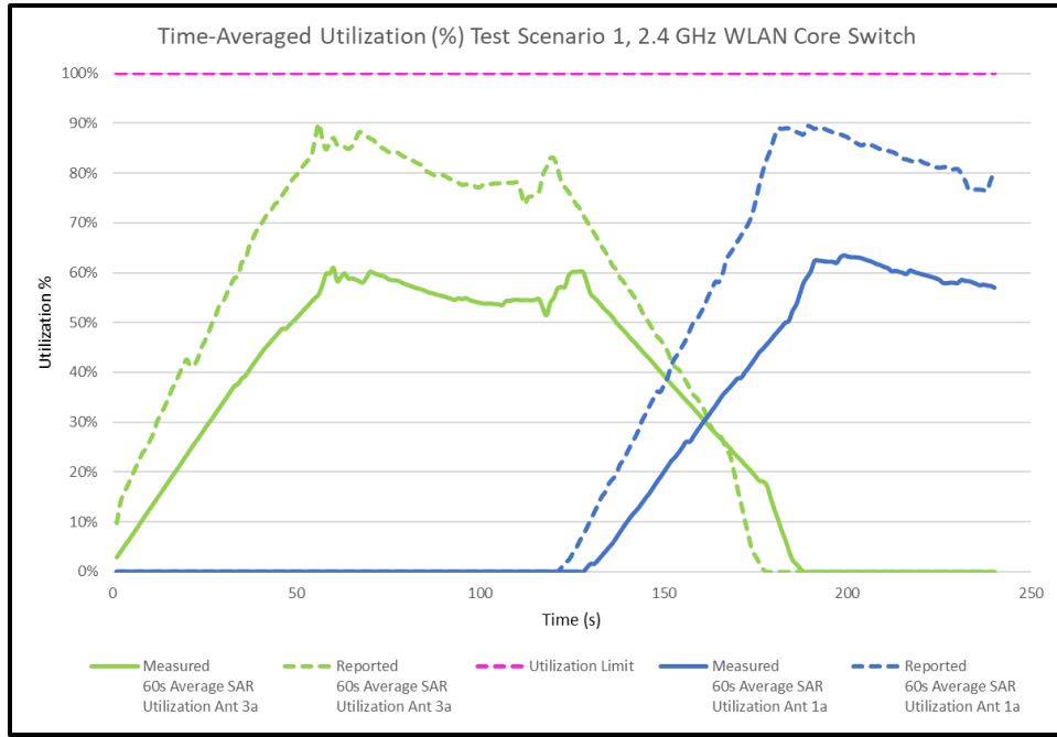
Figure K-1 60s Average SAR Utilization vs. Time, 2.4 GHz
