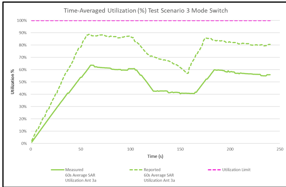
Figure K-7 60s Average Utilization vs. Time during Mode Switch
