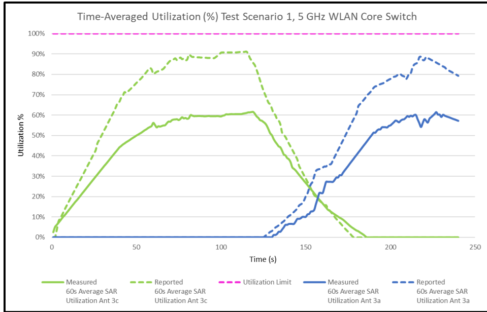
Figure K-3 60s Average SAR Utilization vs. Time, 5 GHz
