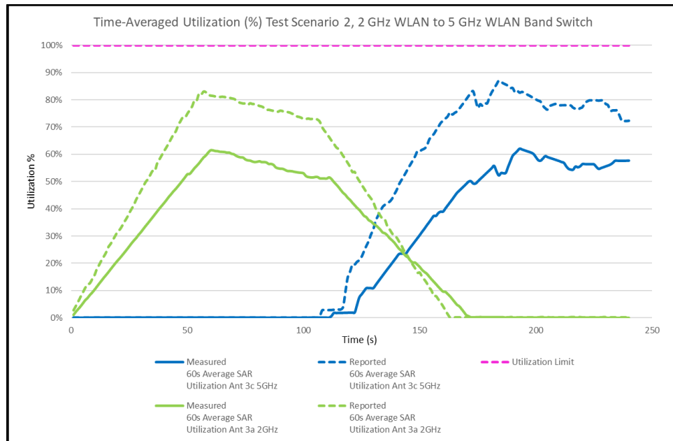
Figure K-5 60s Average Utilization vs. Time during Band Switch
