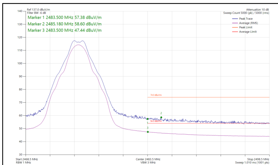
Figure 8 - Thread, SISO, Core 0 - 2475 MHz Band Edge Frequency 2483.5 MHz
