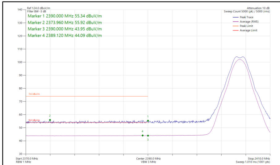
Figure 5 - Thread, SISO, Core 2 - 2405 MHz Band Edge Frequency 2390 MHz
