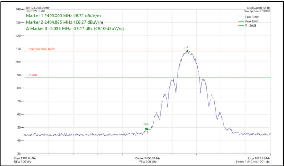
Figure 41 - Thread, SISO, Core 0 - 2405 MHz Band Edge Frequency 2400 MHz
