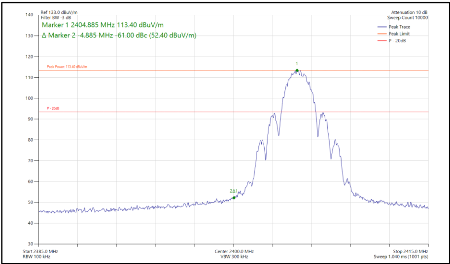
Figure 44 - Thread, SISO, Core 0 - 2405 MHz Band Edge Frequency 2400 MHz
