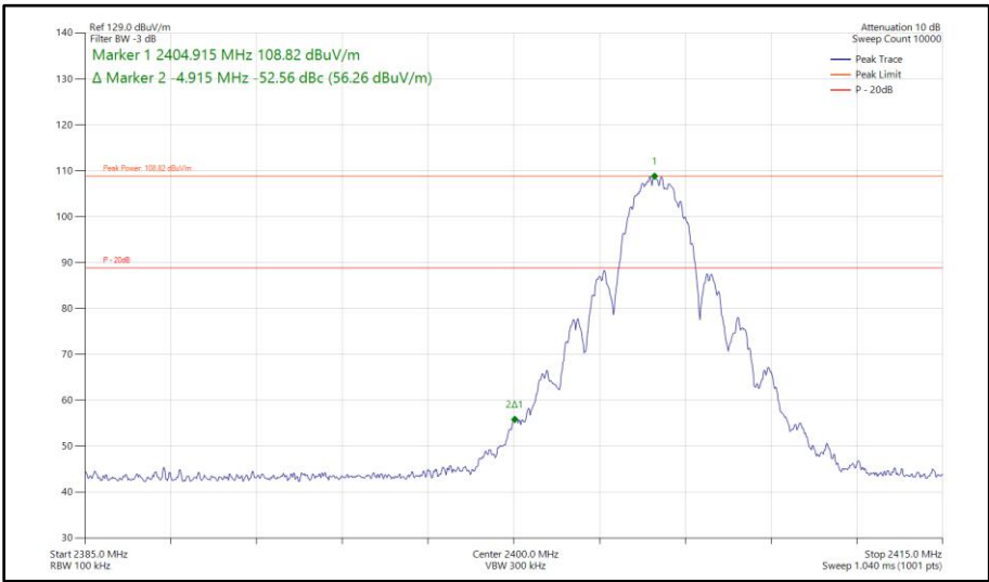
Figure 42 - Thread, SISO, Core 1 - 2405 MHz Band Edge Frequency 2400 MHz
