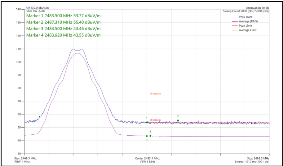
Figure 2 - Thread, SISO, Core 0 - 2475 MHz Band Edge Frequency 2483.5 MHz
