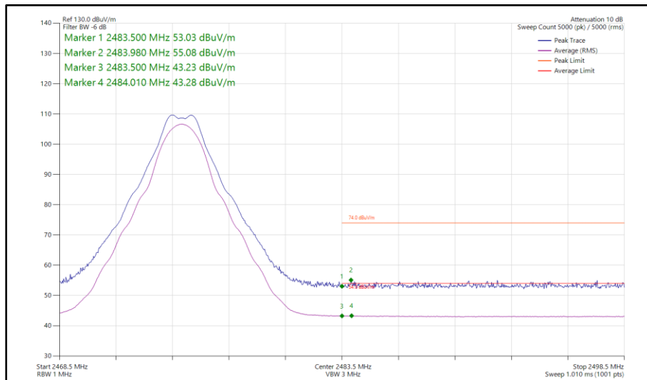
Figure 4 - Thread, SISO, Core 1 - 2475 MHz Band Edge Frequency 2483.5 MHz
