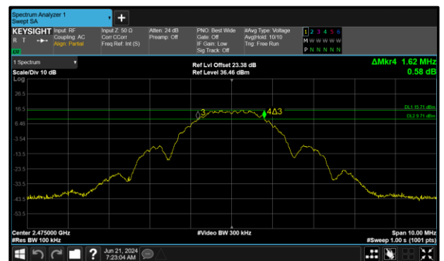
Figure 22 - Core 0 (A) 2475 MHz (CH25) 6 dB Bandwidth
