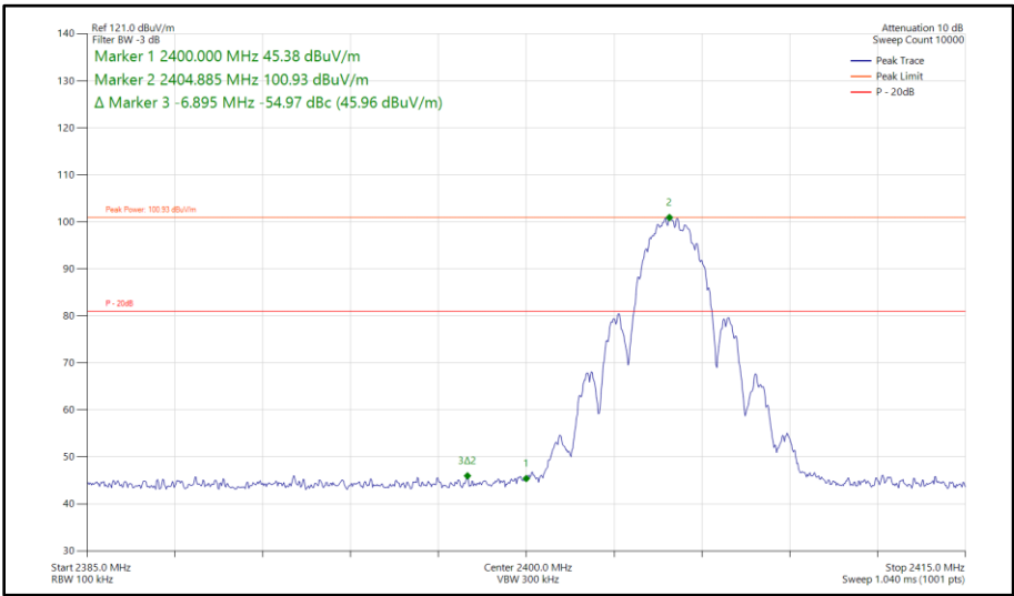
Figure 43 - Thread, SISO, Core 2 - 2405 MHz Band Edge Frequency 2400 MHz
