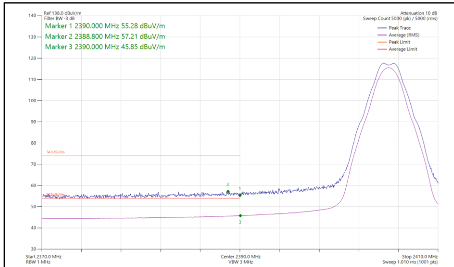
Figure 9 - Thread, SISO, Core 1 - 2405 MHz Band Edge Frequency 2390 MHz
