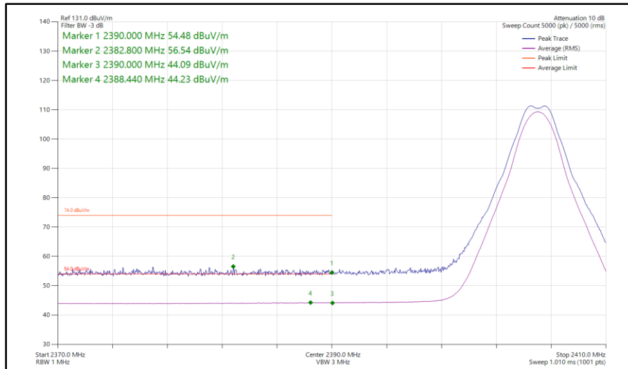
Figure 3 - Thread, SISO, Core 1 - 2405 MHz Band Edge Frequency 2390 MHz
