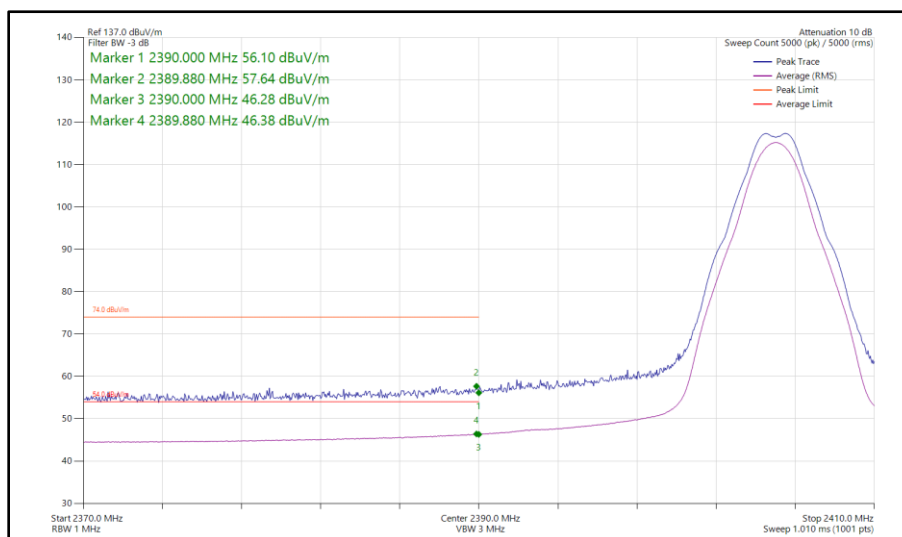
Figure 7 - Thread, SISO, Core 0 - 2405 MHz Band Edge Frequency 2390 MHz
