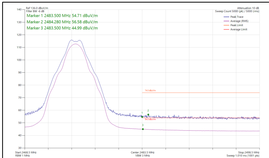
Figure 10 - Thread, SISO, Core 1 - 2475 MHz Band Edge Frequency 2483.5 MHz
