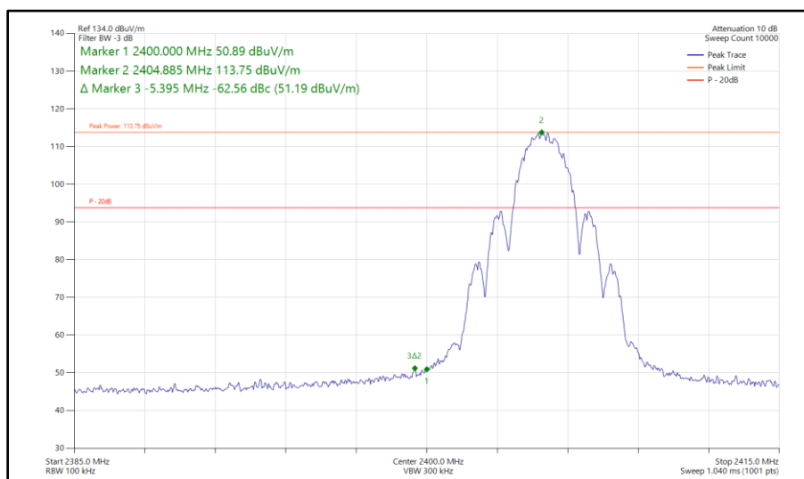
Figure 45 - Thread, SISO, Core 1 - 2405 MHz Band Edge Frequency 2400 MHz
