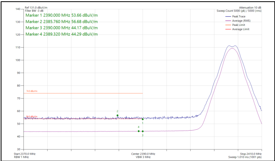
Figure 1 - Thread, SISO, Core 0 - 2405 MHz Band Edge Frequency 2390 MHz
