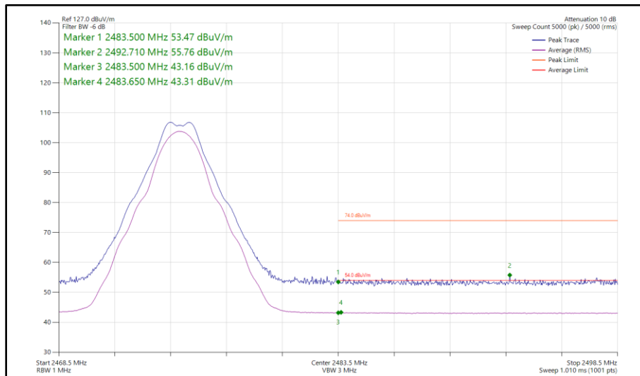
Figure 6 - Thread, SISO, Core 2 - 2475 MHz Band Edge Frequency 2483.5 MHz
