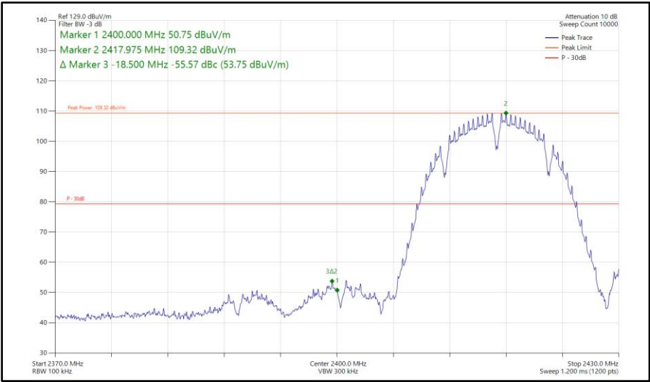
Figure 135 - 802.11b, SISO, Core 0 - 2417 MHz Band Edge Frequency 2400 MHz
