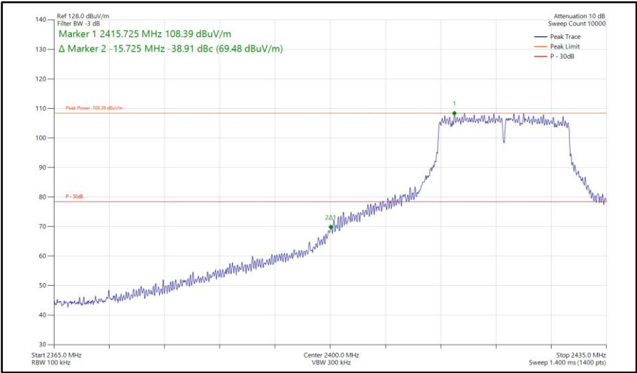
Figure 138 - 802.11g, SISO, Core 0 - 2422 MHz Band Edge Frequency 2400 MHz
