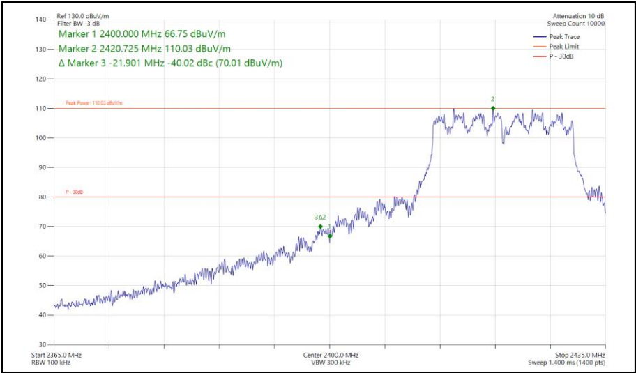
Figure 170 - 802.11n HT20, CDD, Core 0 - Core 1 - 2422 MHz Band Edge Frequency 2400 MHz
