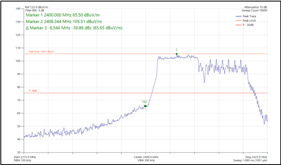
Figure 162 - 802.11ax HE20, RU 106-53, SISO, Core 1 - 2412 MHz Band Edge Frequency 2400 MHz
