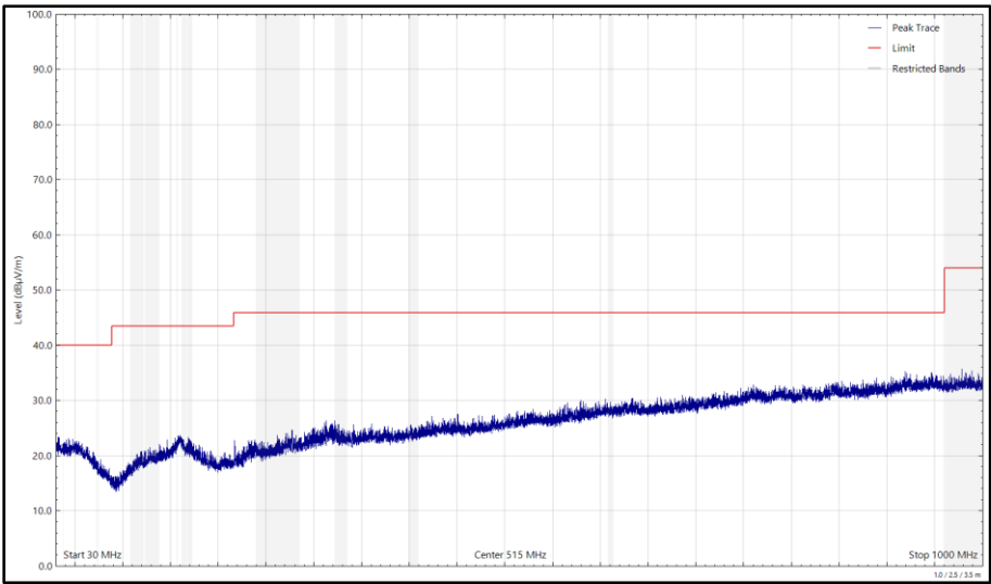
Figure 200 - 2442 MHz (CH7), 802.11g, Core 0, 30 MHz to 1 GHz, Horizontal (Peak)
