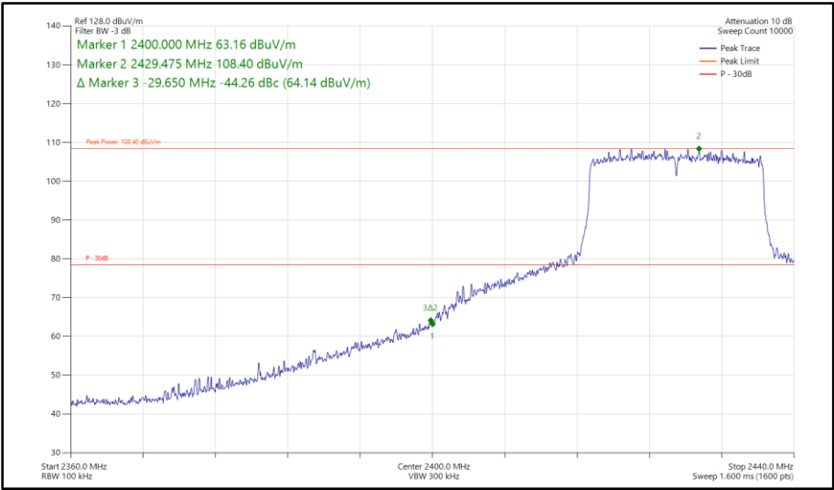
Figure 166 - 802.11ax HE20, SU, SISO, Core 1 - 2427 MHz Band Edge Frequency 2400 MHz
