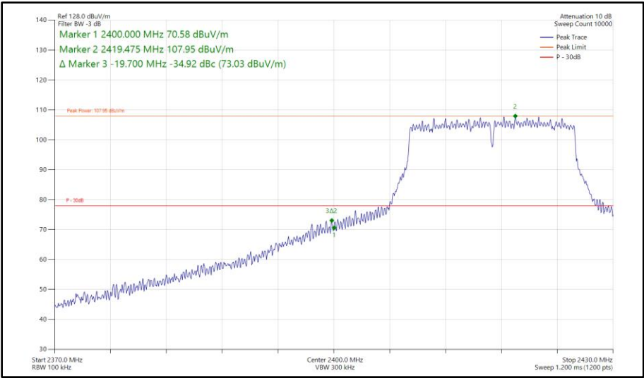
Figure 158 - 802.11n HT20, SISO, Core 1 - 2417 MHz Band Edge Frequency 2400 MHz
