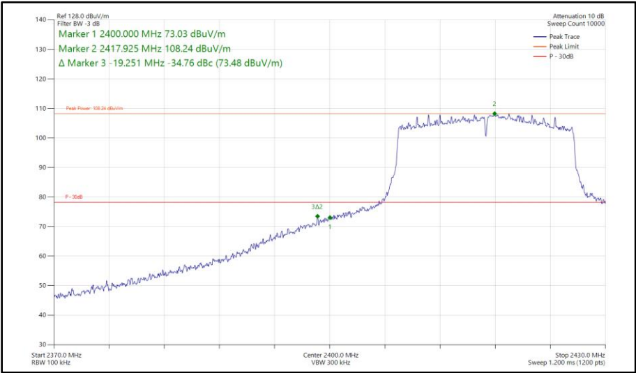
Figure 146 - 802.11ax HE20, SU, SISO, Core 0 - 2417 MHz Band Edge Frequency 2400 MHz
