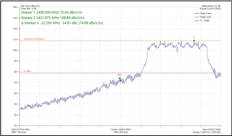
Figure 169 - 802.11n HT20, CDD, Core 0 - Core 1 - 2417 MHz Band Edge Frequency 2400 MHz
