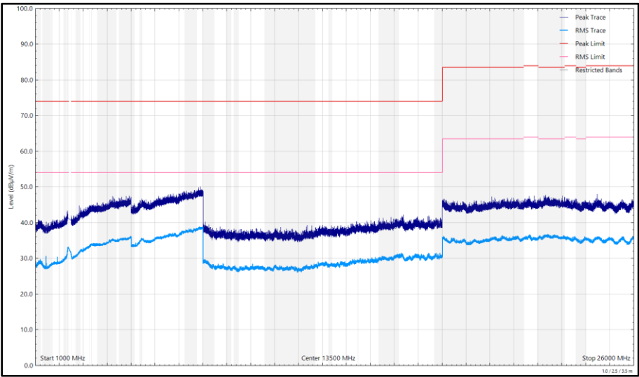
Figure 182 - 2412 MHz (CH1), 802.11b, Core 0, 1 GHz to 26 GHz, Horizontal
