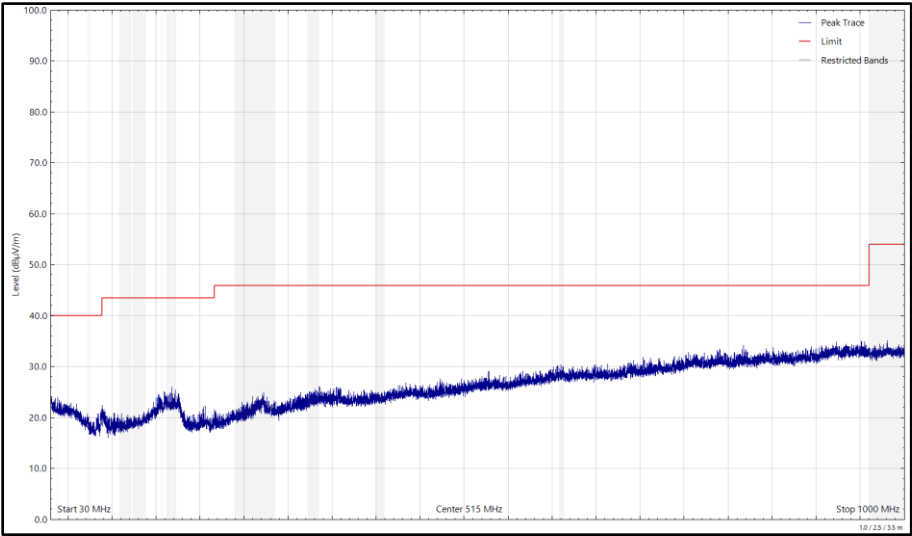
Figure 186 - 2442 MHz (CH7), 802.11b, Core 0, 30 MHz to 1 GHz, Vertical (Peak)
