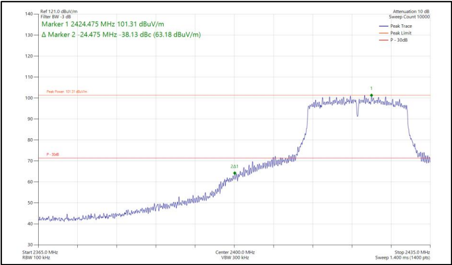
Figure 142 - 802.11n HT20, SISO, Core 0 - 2422 MHz Band Edge Frequency 2400 MHz
