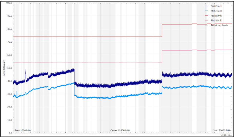
Figure 187 - 2442 MHz (CH7), 802.11b, Core 0, 1 GHz to 26 GHz, Vertical
