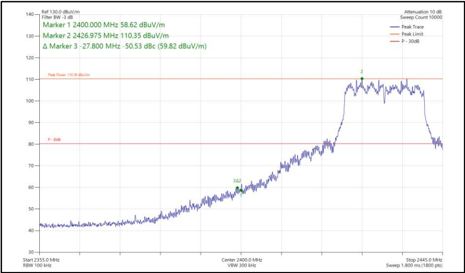
Figure 172 - 802.11n HT20, CDD, Core 0 - Core 1 - 2432 MHz Band Edge Frequency 2400 MHz
