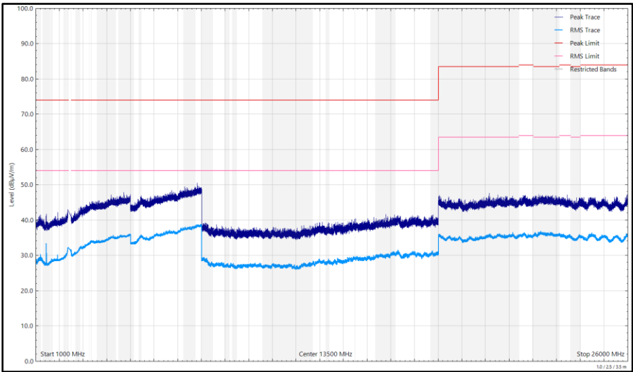
Figure 199 - 2412 MHz (CH1), 802.11g, Core 0, 1 GHz to 26 GHz, Vertical
