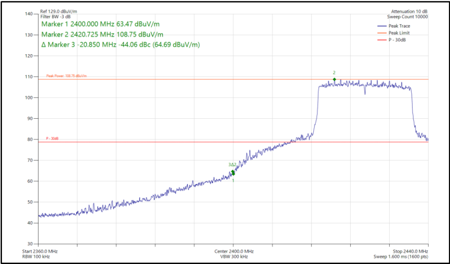
Figure 149 - 802.11ax HE20, SU, SISO, Core 0 - 2427 MHz Band Edge Frequency 2400 MHz
