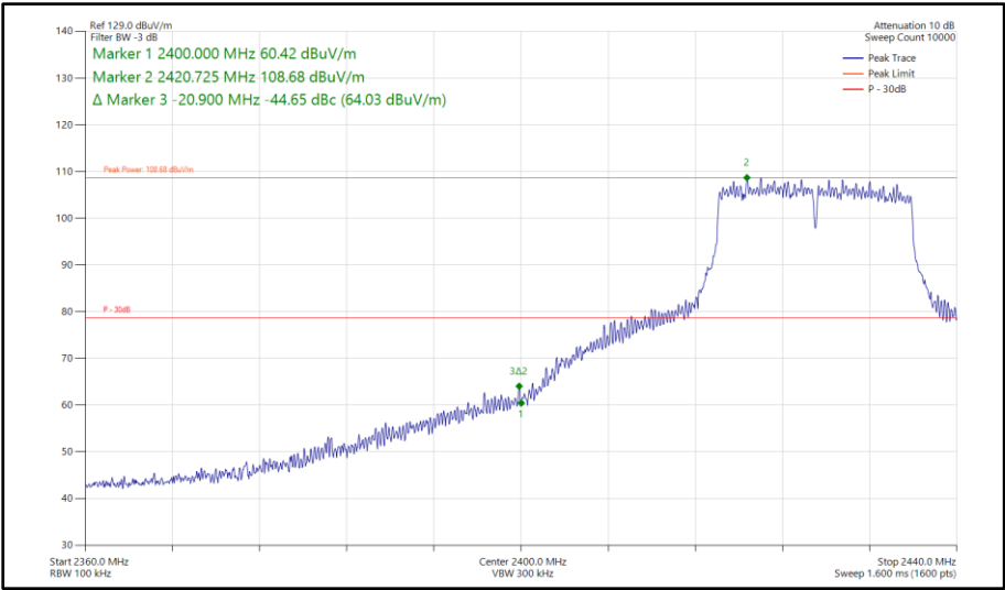
Figure 143 - 802.11n HT20, SISO, Core 0 - 2427 MHz Band Edge Frequency 2400 MHz
