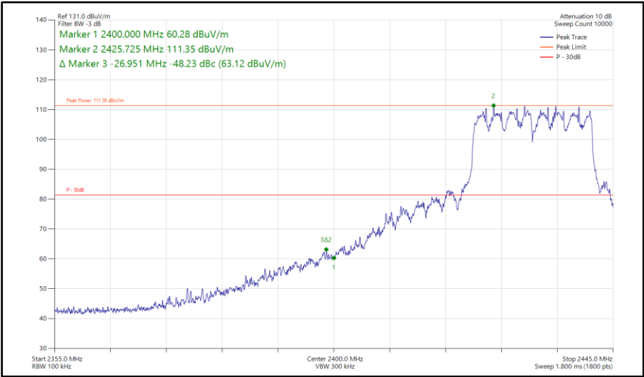
Figure 180 - 802.11ax HE20, SU, CDD, Core 0 - Core 1 - 2432 MHz Band Edge Frequency 2400 MHz
