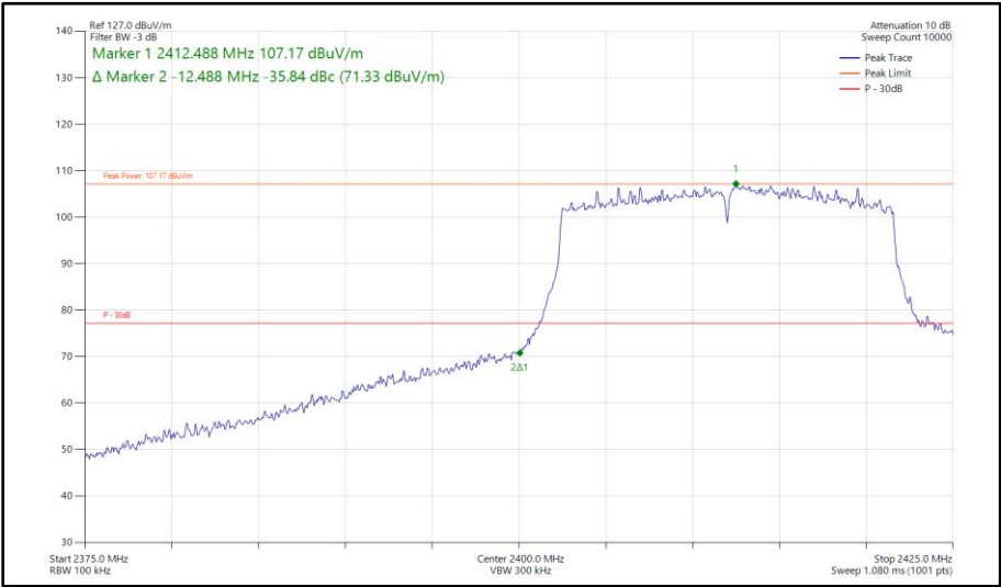
Figure 144 - 802.11ax HE20, SU, SISO, Core 0 - 2412 MHz Band Edge Frequency 2400 MHz
