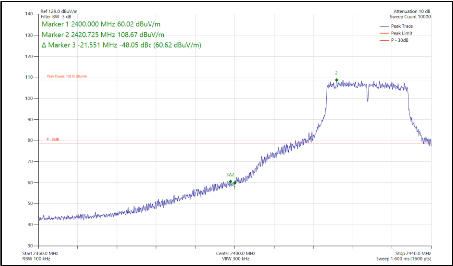
Figure 139 - 802.11g, SISO, Core 0 - 2427 MHz Band Edge Frequency 2400 MHz
