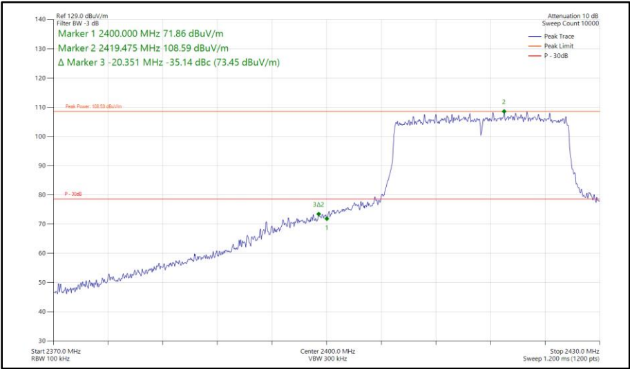
Figure 163 - 802.11ax HE20, SU, SISO, Core 1 - 2417 MHz Band Edge Frequency 2400 MHz
