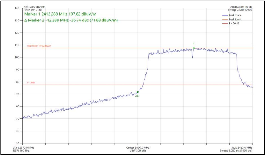
Figure 161 - 802.11ax HE20, SU, SISO, Core 1 - 2412 MHz Band Edge Frequency 2400 MHz
