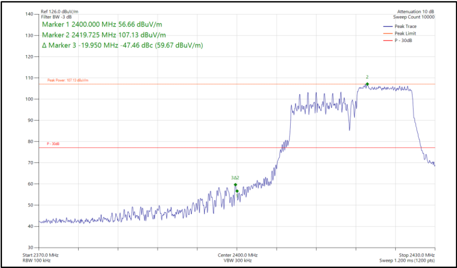
Figure 147 - 802.11ax HE20, RU 106-54, SISO, Core 0 - 2417 MHz Band Edge Frequency 2400 MHz
