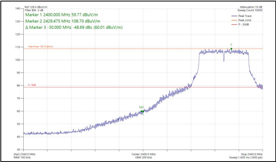
Figure 156 - 802.11g, SISO, Core 1 - 2427 MHz Band Edge Frequency 2400 MHz
