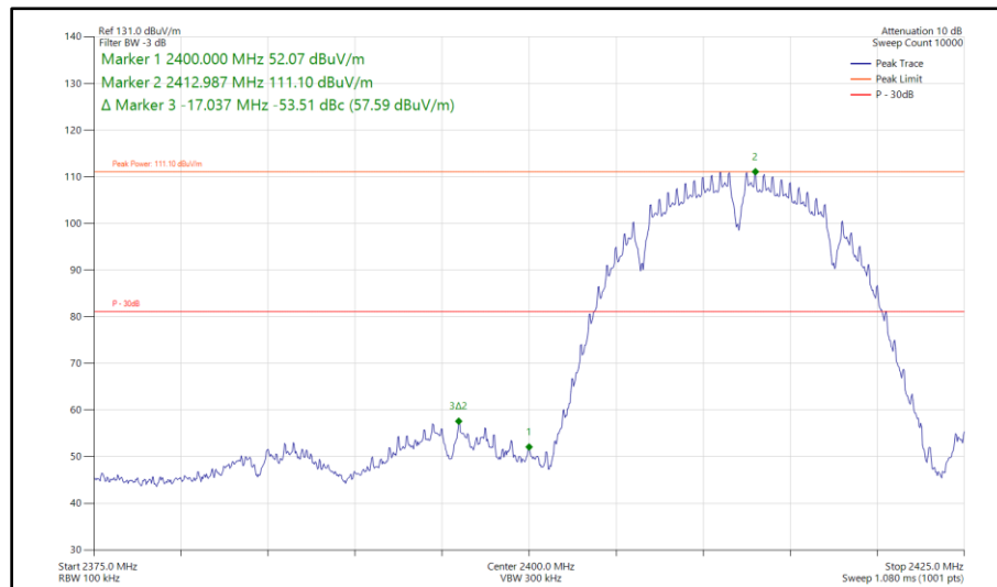
Figure 151 - 802.11b, SISO, Core 1 - 2412 MHz Band Edge Frequency 2400 MHz
