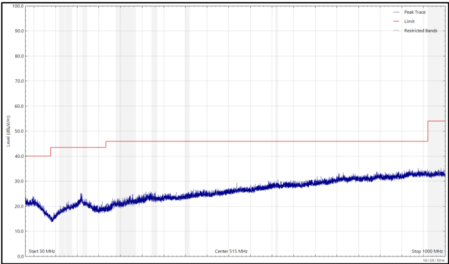
Figure 184 - 2442 MHz (CH7), 802.11b, Core 0, 30 MHz to 1 GHz, Horizontal (Peak)
