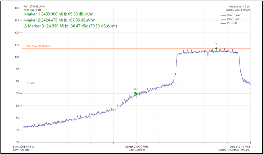
Figure 148 - 802.11ax HE20, SU, SISO, Core 0 - 2422 MHz Band Edge Frequency 2400 MHz
