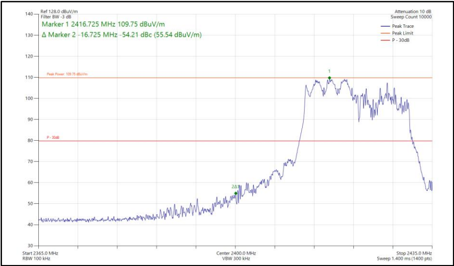
Figure 178 - 802.11ax HE20, RU 106-53, CDD, Core 0 - Core 1 - 2422 MHz Band Edge Frequency 2400 MHz
