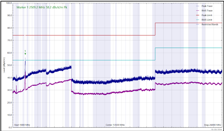
Figure 205 - 2472 MHz (CH13), 802.11g, Core 0, 1 GHz to 26 GHz, Vertical
