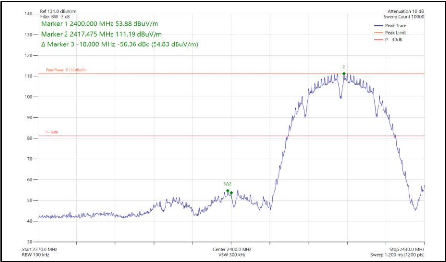
Figure 152 - 802.11b, SISO, Core 1 - 2417 MHz Band Edge Frequency 2400 MHz
