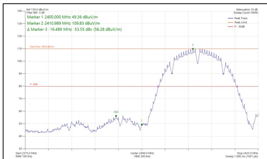
Figure 134 - 802.11b, SISO, Core 0 - 2412 MHz Band Edge Frequency 2400 MHz
