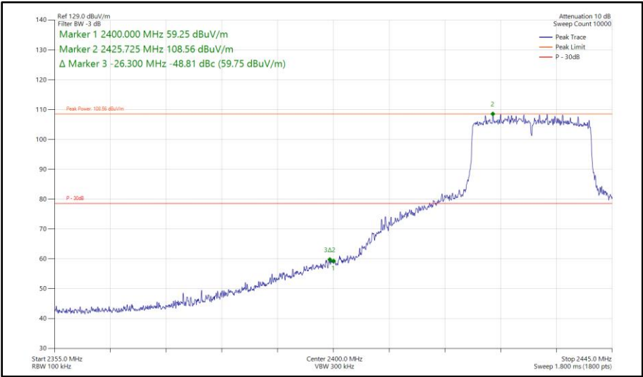
Figure 150 - 802.11ax HE20, SU, SISO, Core 0 - 2432 MHz Band Edge Frequency 2400 MHz
