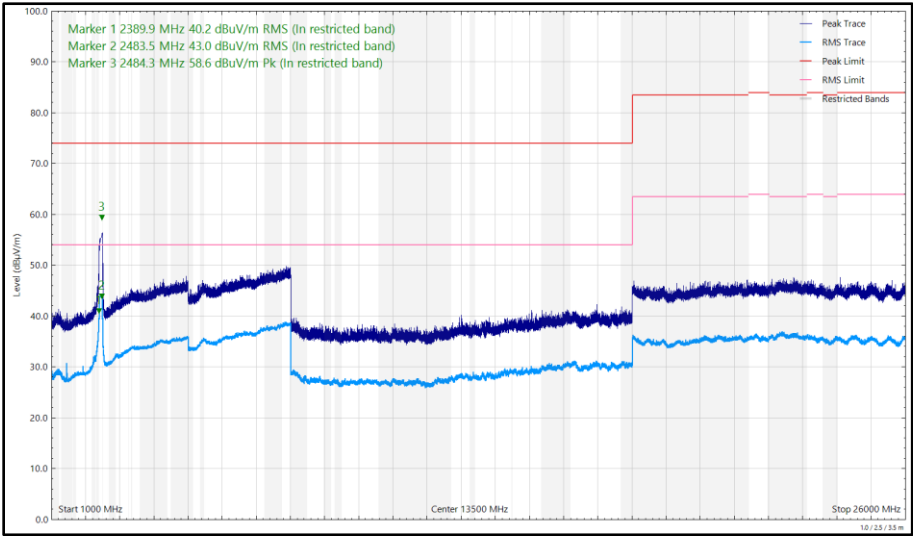
Figure 201 - 2442 MHz (CH7), 802.11g, Core 0, 1 GHz to 26 GHz, Horizontal
