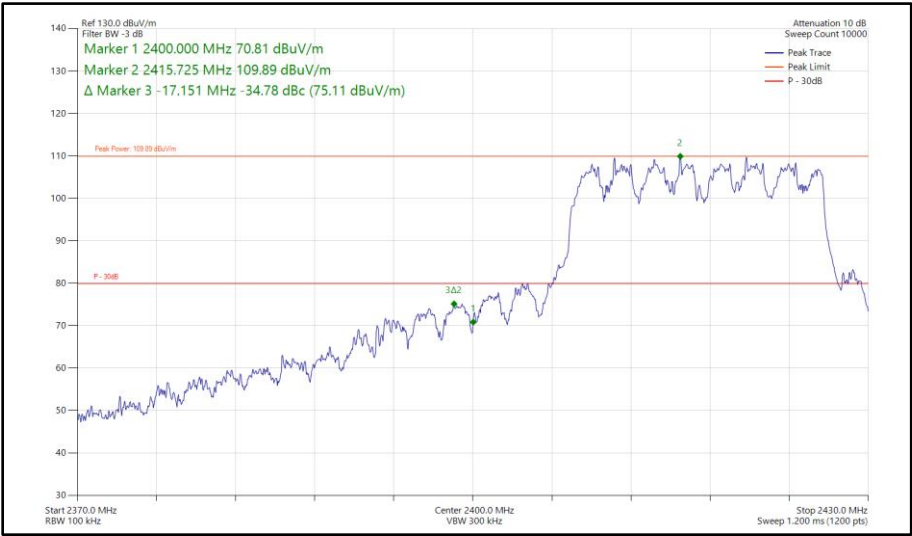
Figure 175 - 802.11ax HE20, SU, CDD, Core 0 - Core 1 - 2417 MHz Band Edge Frequency 2400 MHz
