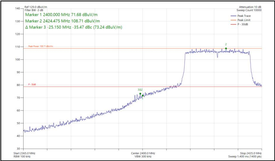
Figure 165 - 802.11ax HE20, SU, SISO, Core 1 - 2422 MHz Band Edge Frequency 2400 MHz
