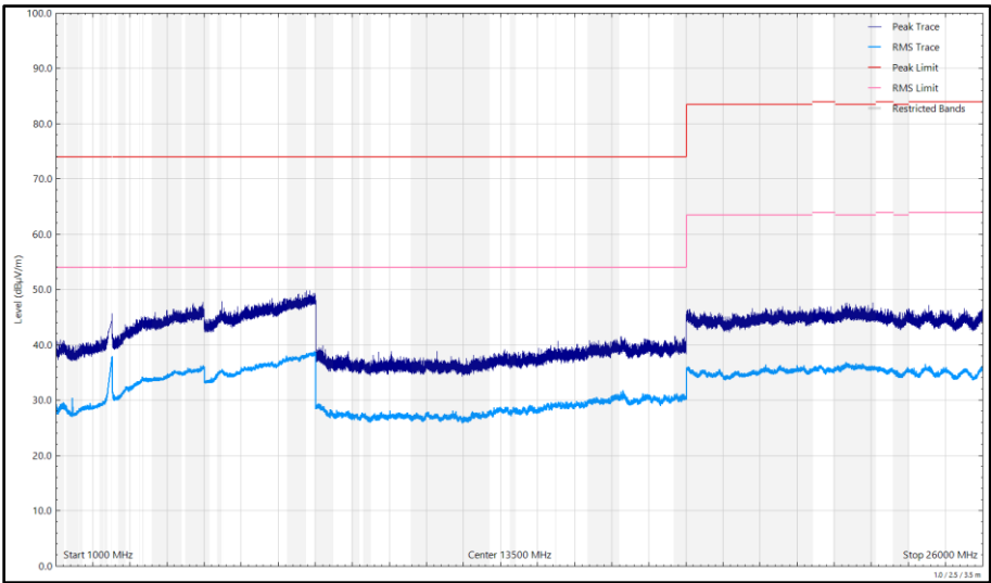
Figure 196 - 2472 MHz (CH13), 802.11b, Core 1, 1 GHz to 26 GHz, Horizontal
