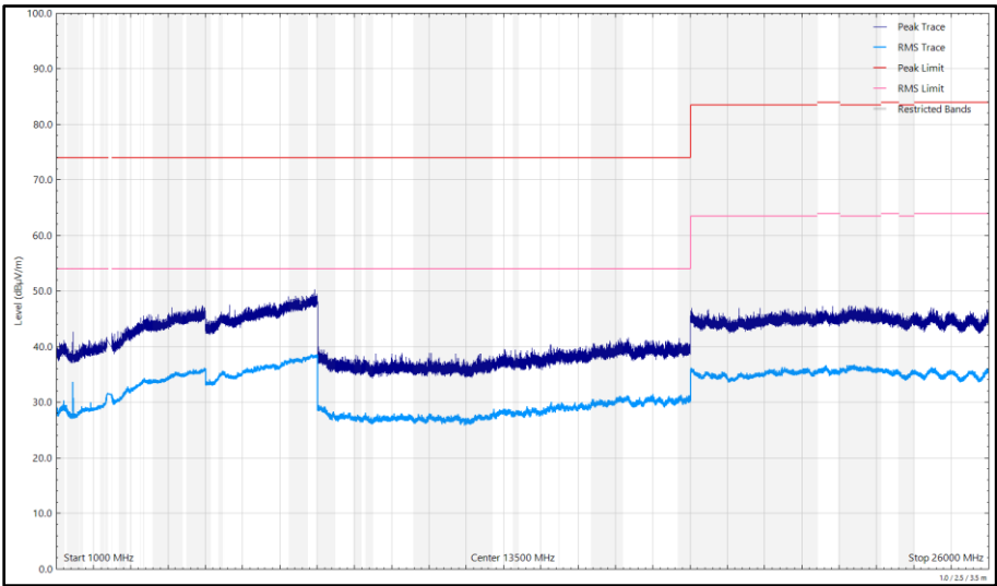
Figure 191 - 2412 MHz (CH1), 802.11b, Core 1, 1 GHz to 26 GHz, Vertical
