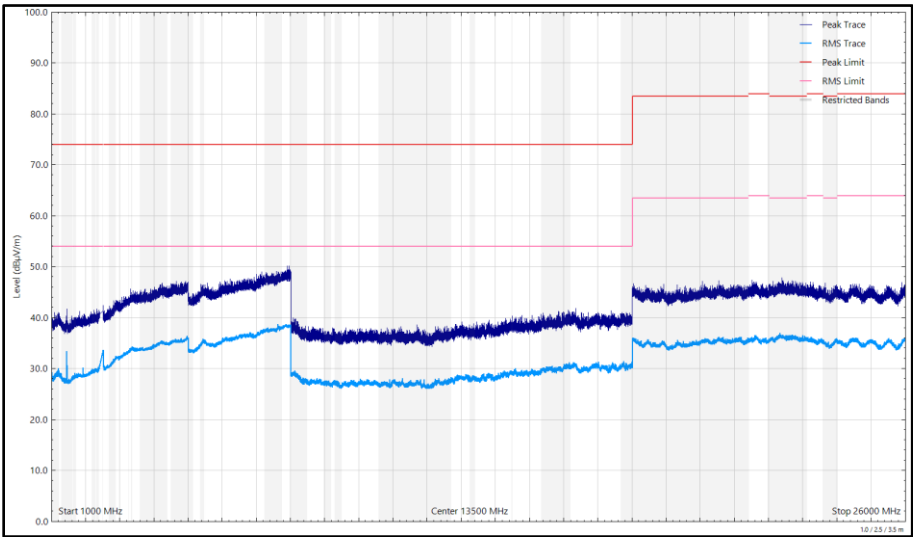
Figure 189 - 2472 MHz (CH13), 802.11b, Core 0, 1 GHz to 26 GHz, Vertical
