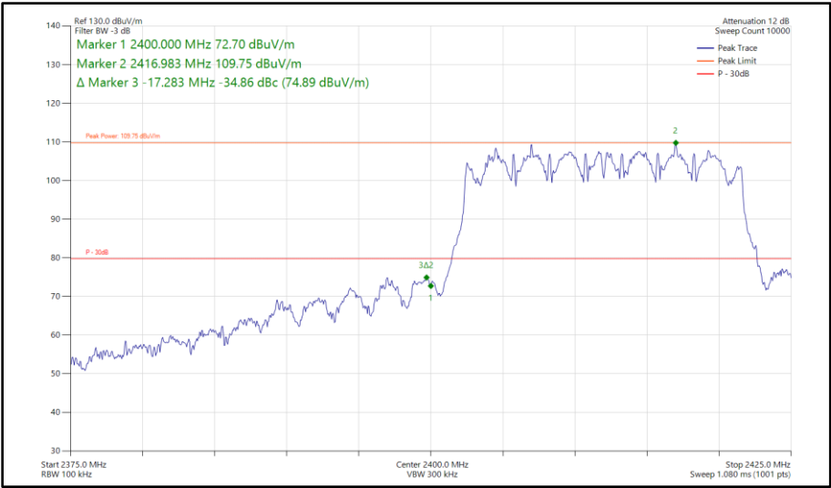
Figure 173 - 802.11ax HE20, SU, CDD, Core 0 - Core 1 - 2412 MHz Band Edge Frequency 2400 MHz
