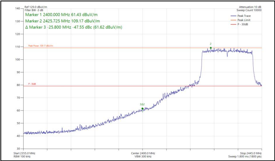
Figure 167 - 802.11ax HE20, SU, SISO, Core 1 - 2432 MHz Band Edge Frequency 2400 MHz
