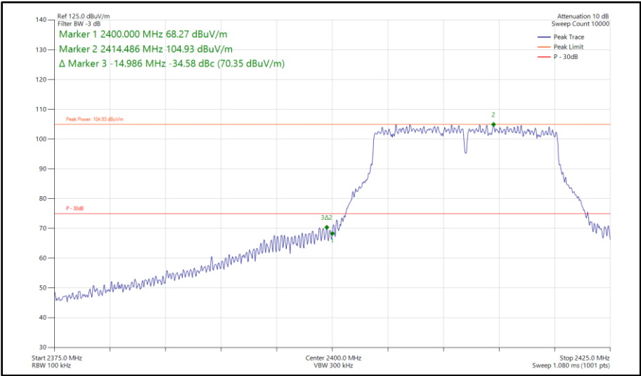
Figure 136 - 802.11g, SISO, Core 0 - 2412 MHz Band Edge Frequency 2400 MHz
