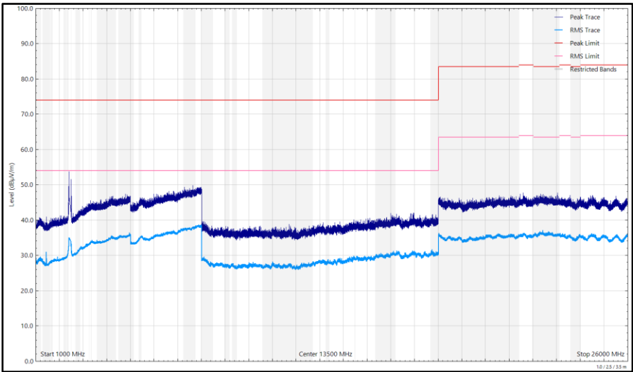
Figure 193 - 2442 MHz (CH7), 802.11b, Core 1, 1 GHz to 26 GHz, Horizontal
