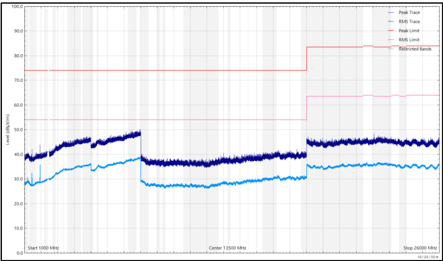
Figure 183 - 2412 MHz (CH1), 802.11b, Core 0, 1 GHz to 26 GHz, Vertical
