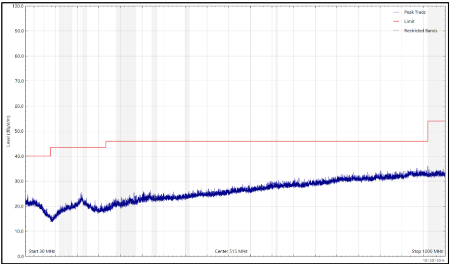
Figure 192 - 2442 MHz (CH7), 802.11b, Core 1, 30 MHz to 1 GHz, Horizontal (Peak)
