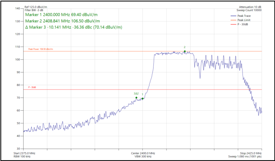
Figure 145 - 802.11ax HE20, RU 106-53, SISO, Core 0 - 2412 MHz Band Edge Frequency 2400 MHz
