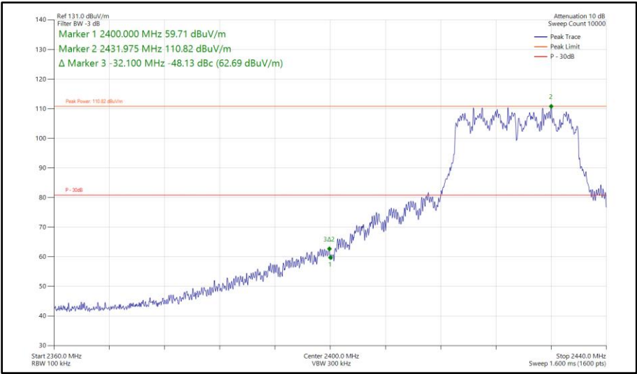
Figure 171 - 802.11n HT20, CDD, Core 0 - Core 1 - 2427 MHz Band Edge Frequency 2400 MHz
