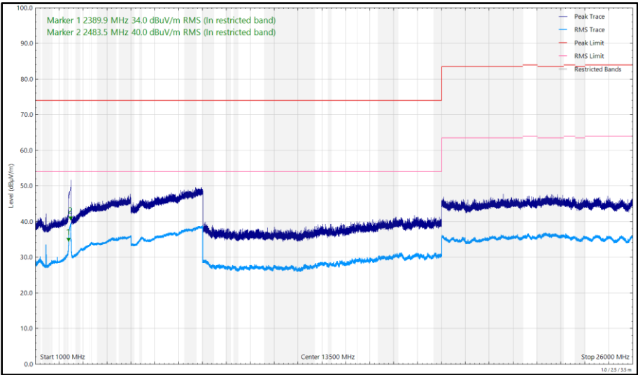
Figure 203 - 2442 MHz (CH7), 802.11g, Core 0, 1 GHz to 26 GHz, Vertical
