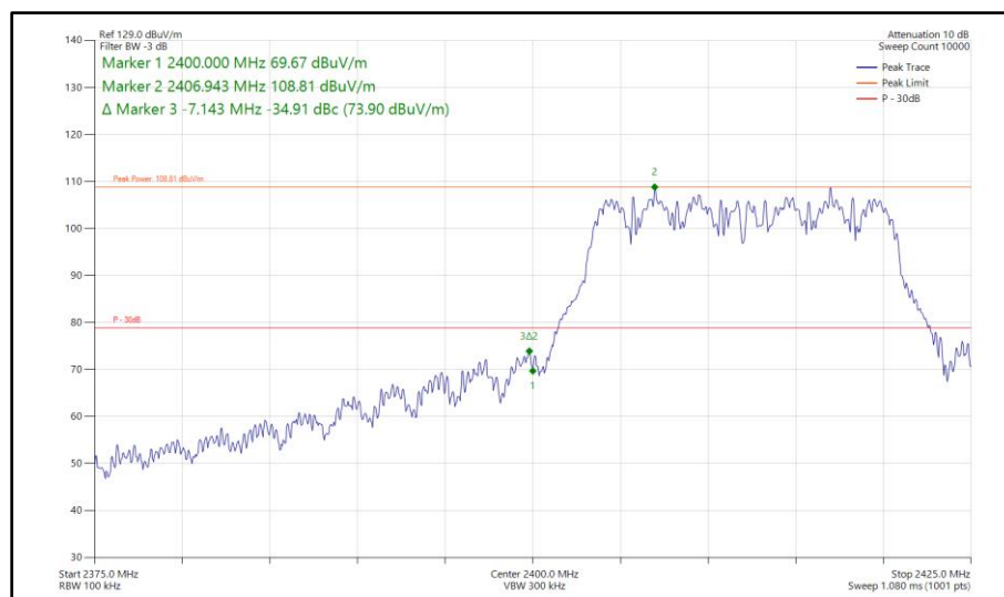
Figure 168 - 802.11n HT20, CDD, Core 0 - Core 1 - 2412 MHz Band Edge Frequency 2400 MHz
