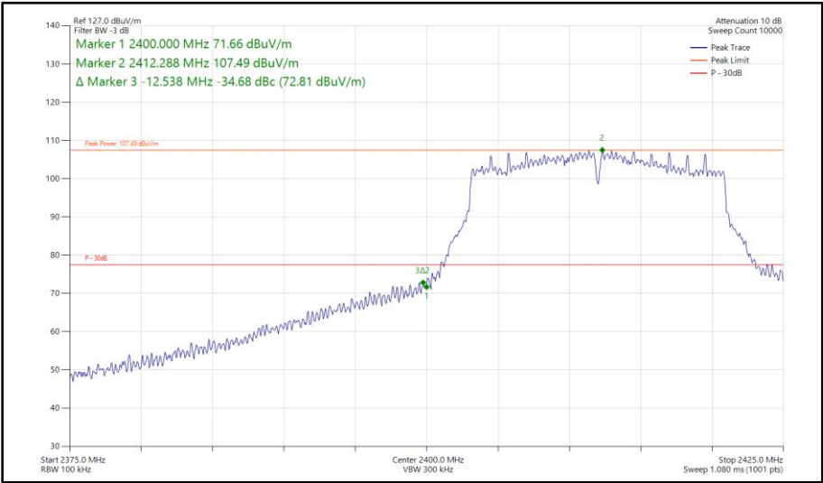
Figure 140 - 802.11n HT20, SISO, Core 0 - 2412 MHz Band Edge Frequency 2400 MHz
