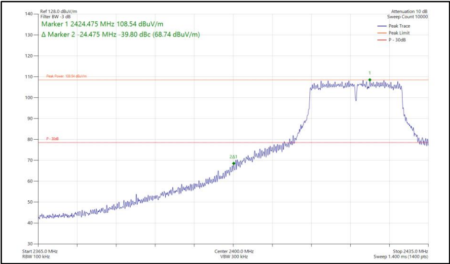
Figure 155 - 802.11g, SISO, Core 1 - 2422 MHz Band Edge Frequency 2400 MHz
