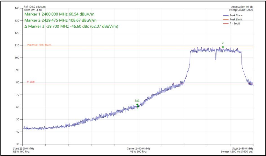
Figure 160 - 802.11n HT20, SISO, Core 1 - 2427 MHz Band Edge Frequency 2400 MHz
