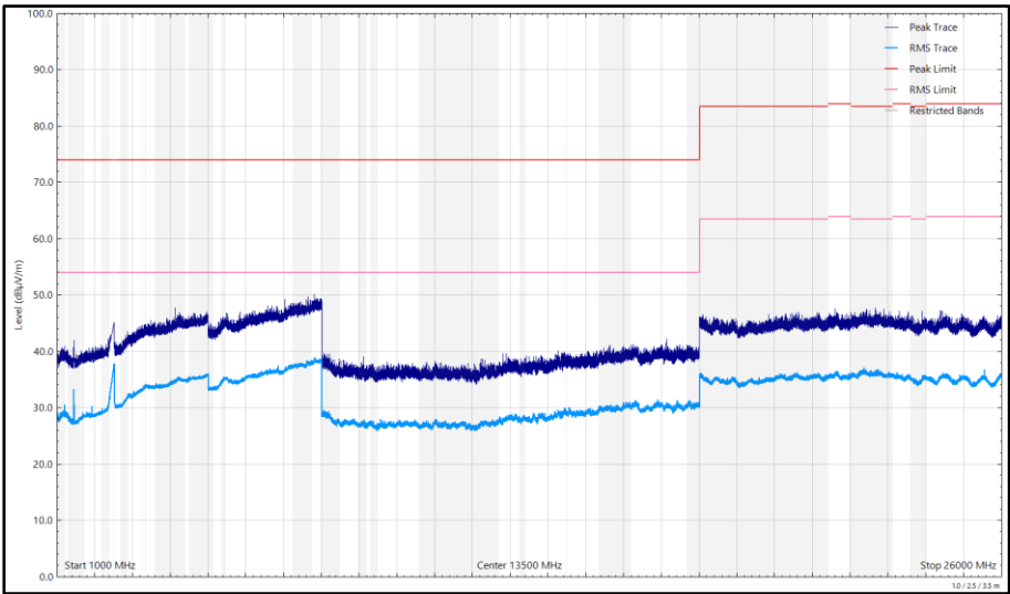
Figure 197 - 2472 MHz (CH13), 802.11b, Core 1, 1 GHz to 26 GHz, Vertical
