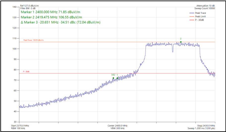
Figure 137 - 802.11g, SISO, Core 0 - 2417 MHz Band Edge Frequency 2400 MHz
