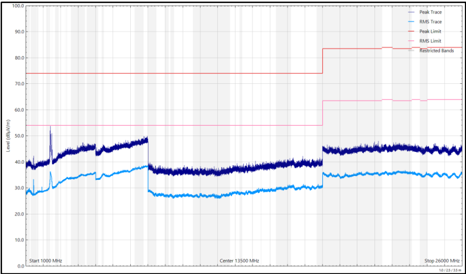
Figure 195 - 2442 MHz (CH7), 802.11b, Core 1, 1 GHz to 26 GHz, Vertical
