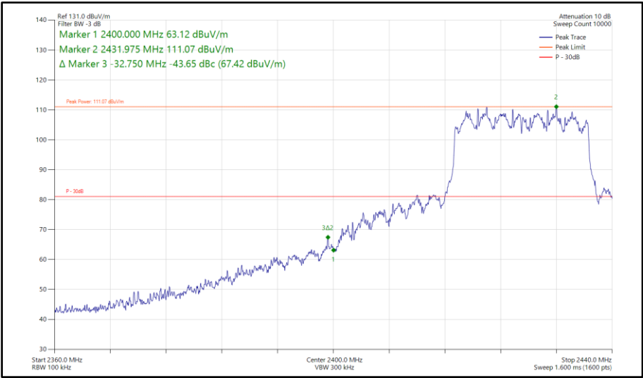
Figure 179 - 802.11ax HE20, SU, CDD, Core 0 - Core 1 - 2427 MHz Band Edge Frequency 2400 MHz
