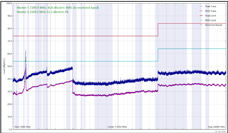
Figure 204 - 2472 MHz (CH13), 802.11g, Core 0, 1 GHz to 26 GHz, Horizontal
