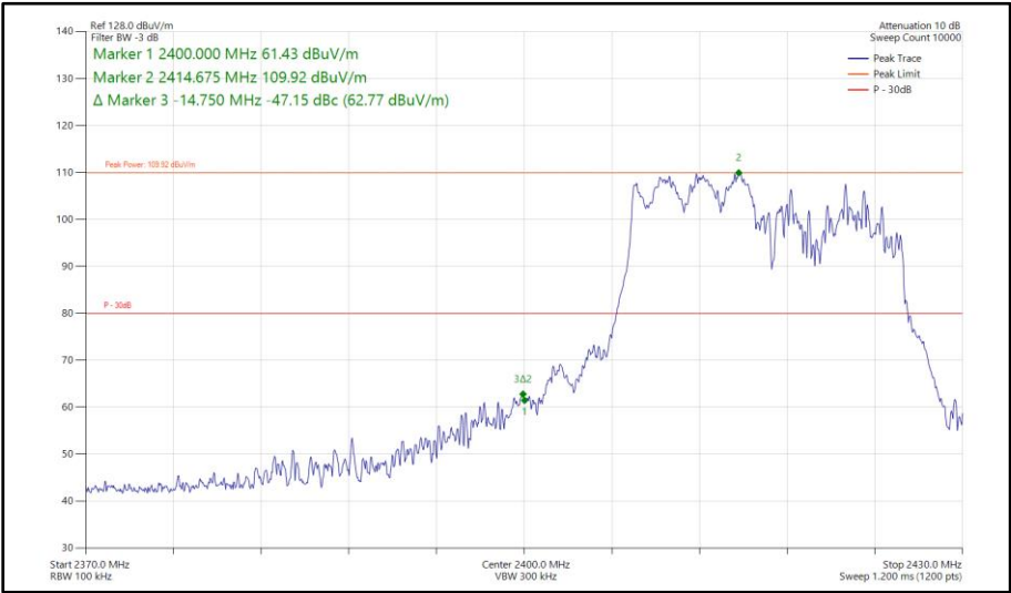
Figure 176 - 802.11ax HE20, RU 106-53, CDD, Core 0 - Core 1 - 2417 MHz Band Edge Frequency 2400 MHz
