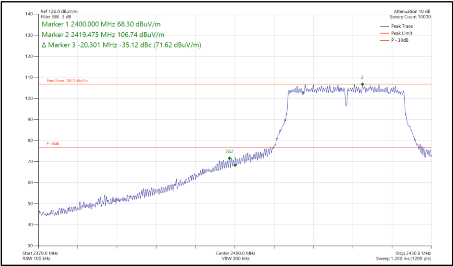
Figure 141 - 802.11n HT20, SISO, Core 0 - 2417 MHz Band Edge Frequency 2400 MHz
