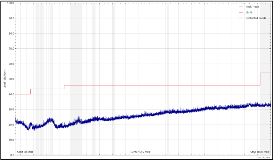
Figure 194 - 2442 MHz (CH7), 802.11b, Core 1, 30 MHz to 1 GHz, Vertical (Peak)
