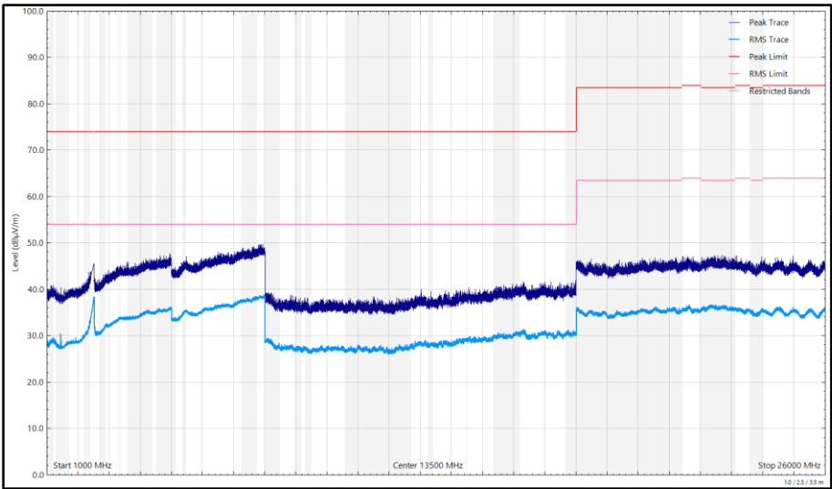
Figure 188 - 2472 MHz (CH13), 802.11b, Core 0, 1 GHz to 26 GHz, Horizontal
