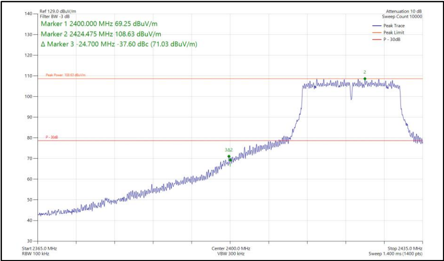
Figure 159 - 802.11n HT20, SISO, Core 1 - 2422 MHz Band Edge Frequency 2400 MHz
