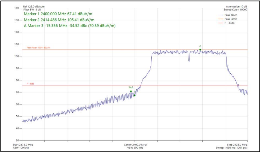
Figure 153 - 802.11g, SISO, Core 1 - 2412 MHz Band Edge Frequency 2400 MHz
