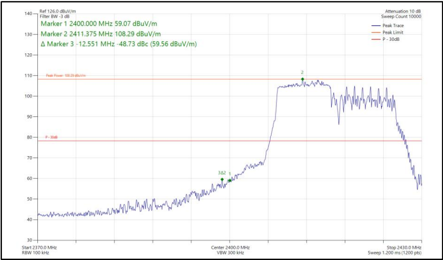
Figure 164 - 802.11ax HE20, RU 106-53, SISO, Core 1 - 2417 MHz Band Edge Frequency 2400 MHz
