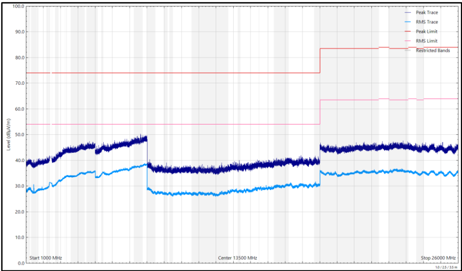
Figure 190 - 2412 MHz (CH1), 802.11b, Core 1, 1 GHz to 26 GHz, Horizontal
