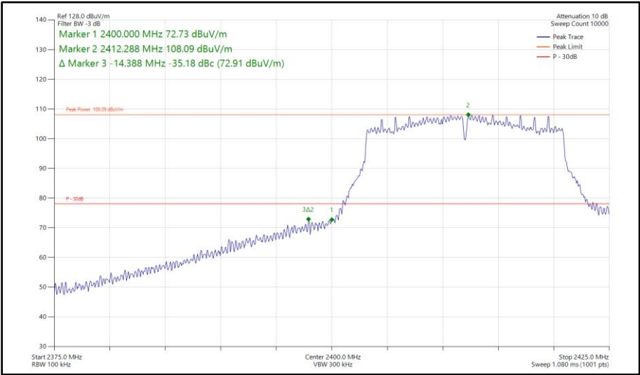
Figure 157 - 802.11n HT20, SISO, Core 1 - 2412 MHz Band Edge Frequency 2400 MHz
