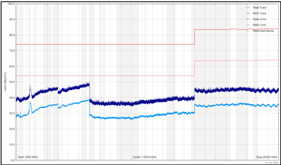
Figure 198 - 2412 MHz (CH1), 802.11g, Core 0, 1 GHz to 26 GHz, Horizontal
