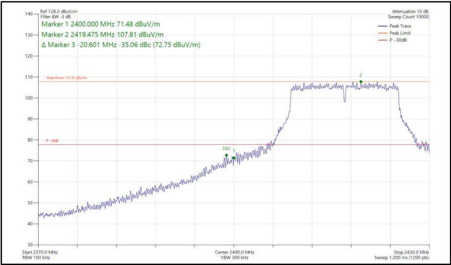
Figure 154 - 802.11g, SISO, Core 1 - 2417 MHz Band Edge Frequency 2400 MHz
