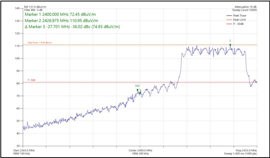
Figure 177 - 802.11ax HE20, SU, CDD, Core 0 - Core 1 - 2422 MHz Band Edge Frequency 2400 MHz
