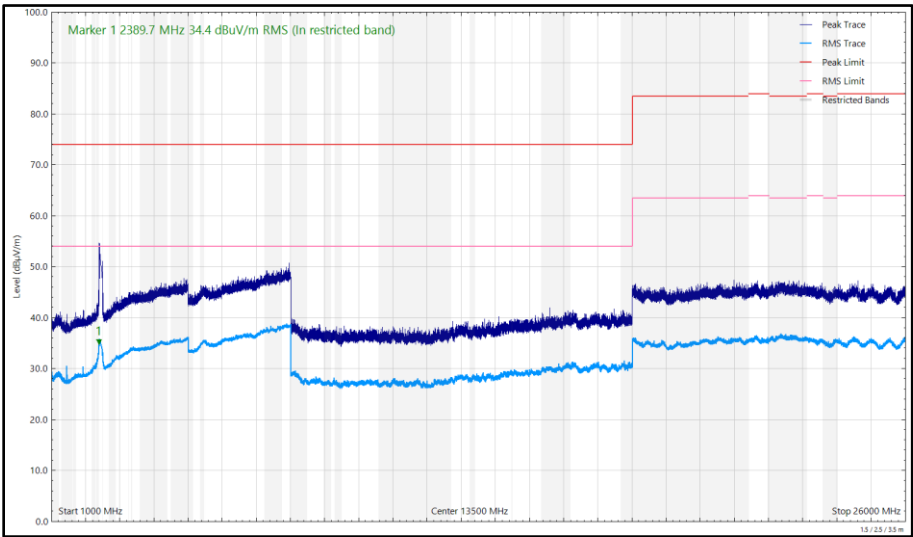
Figure 185 - 2442 MHz (CH7), 802.11b, Core 0, 1 GHz to 26 GHz, Horizontal
