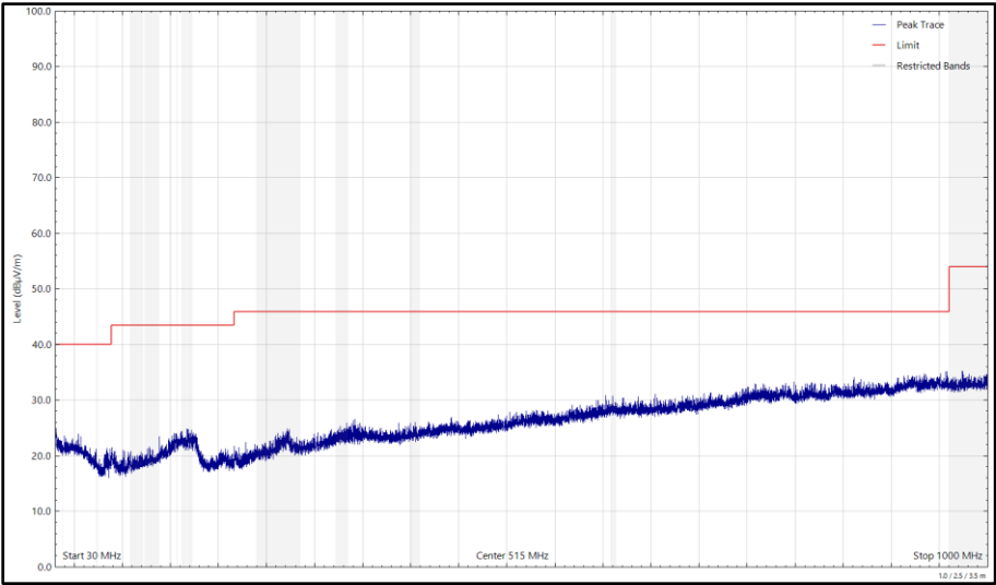
Figure 202 - 2442 MHz (CH7), 802.11g, Core 0, 30 MHz to 1 GHz, Vertical (Peak)
