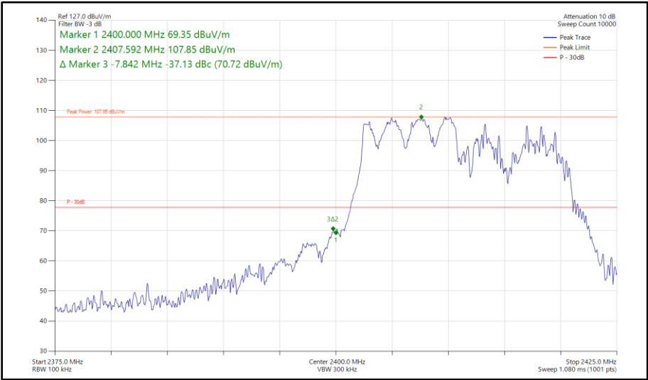
Figure 174 - 802.11ax HE20, RU 106-53, CDD, Core 0 - Core 1 - 2412 MHz Band Edge Frequency 2400 MHz
