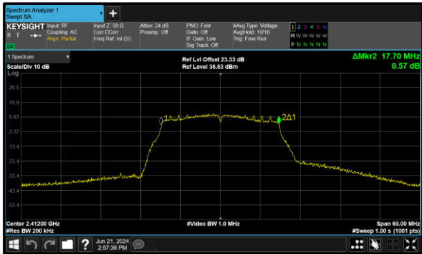
Figure 122 - 802.11n HT20 Minimum 99% OBW
