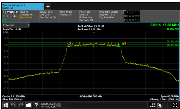
Figure 128 - 802.11ax HE20 SU Minimum 6 dB EBW
