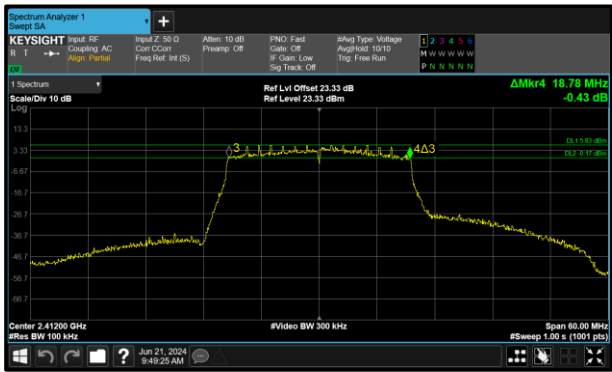
Figure 116 - 802.11ax HE20 SU Minimum 6 dB EBW
