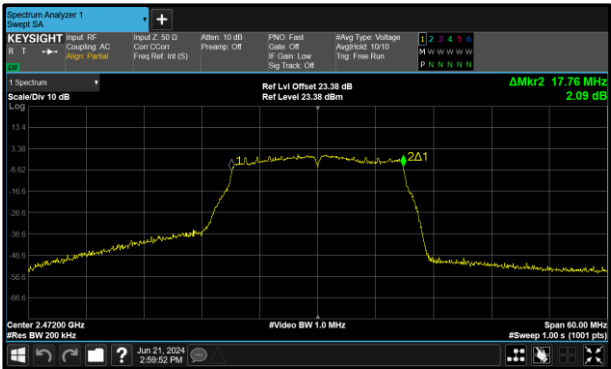
Figure 123 - 802.11n HT20 Maximum 99% OBW
