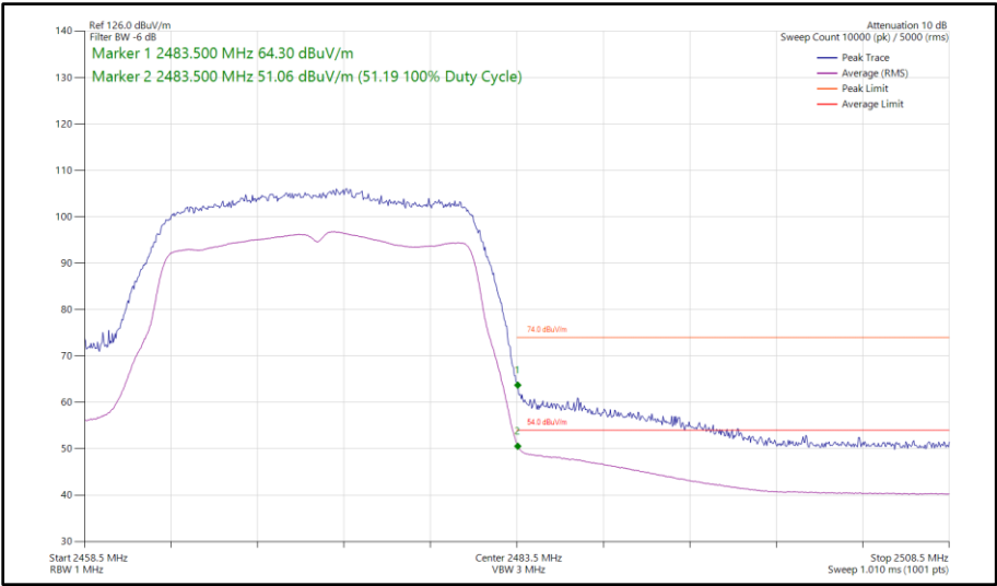
Figure 31 - 802.11n HT20, SISO, Core 0 - 2472 MHz Band Edge Frequency 2483.5 MHz
