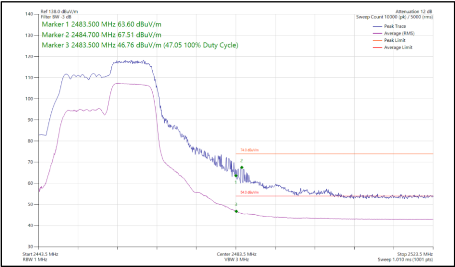
Figure 35 - 802.11ax HE20, RU 106-54, SISO, Core 0 - 2457 MHz Band Edge Frequency 2483.5 MHz
