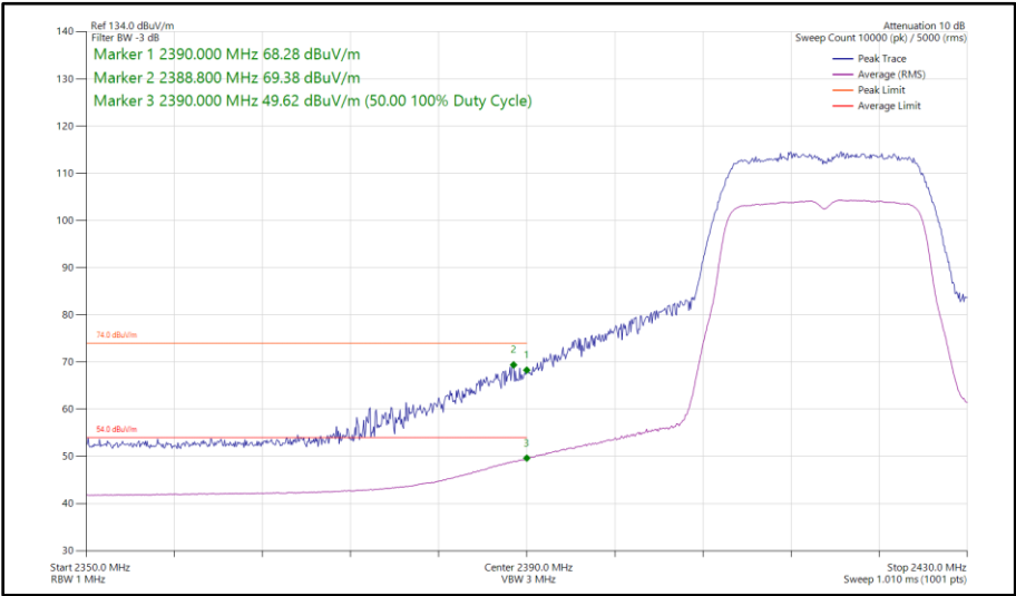
Figure 49 - 802.11n HT20, SISO, Core 1 - 2417 MHz Band Edge Frequency 2390 MHz
