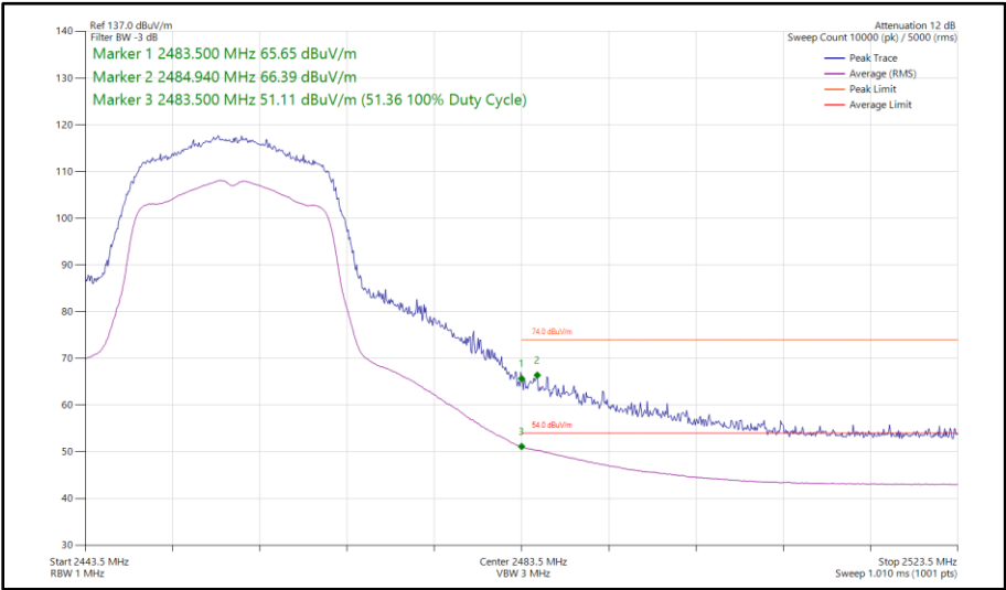
Figure 28 - 802.11n HT20, SISO, Core 0 - 2457 MHz Band Edge Frequency 2483.5 MHz
