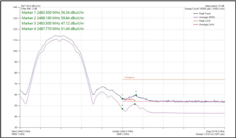
Figure 18 - 802.11b, SISO, Core 0 - 2462 MHz Band Edge Frequency 2483.5 MHz
