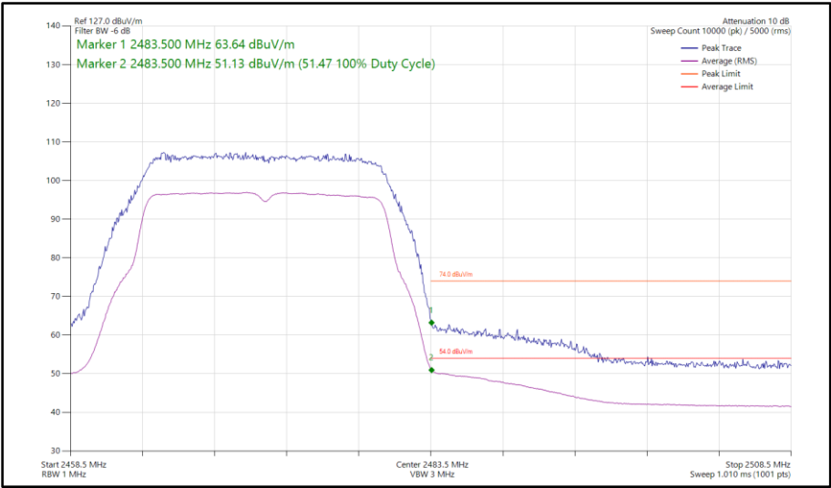
Figure 25 - 802.11g, SISO, Core 0 - 2472 MHz Band Edge Frequency 2483.5 MHz
