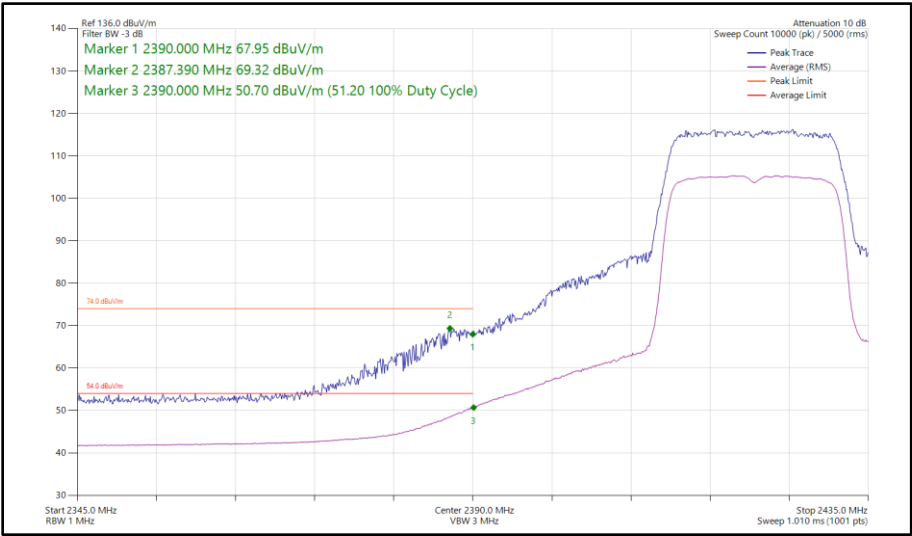
Figure 56 - 802.11ax HE20, SU, SISO, Core 1 - 2422 MHz Band Edge Frequency 2390 MHz
