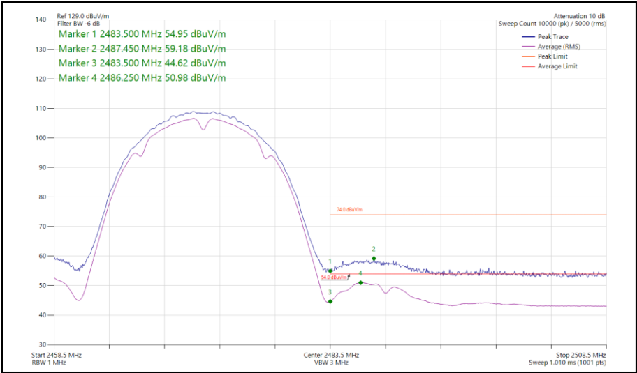
Figure 20 - 802.11b, SISO, Core 0 - 2472 MHz Band Edge Frequency 2483.5 MHz
