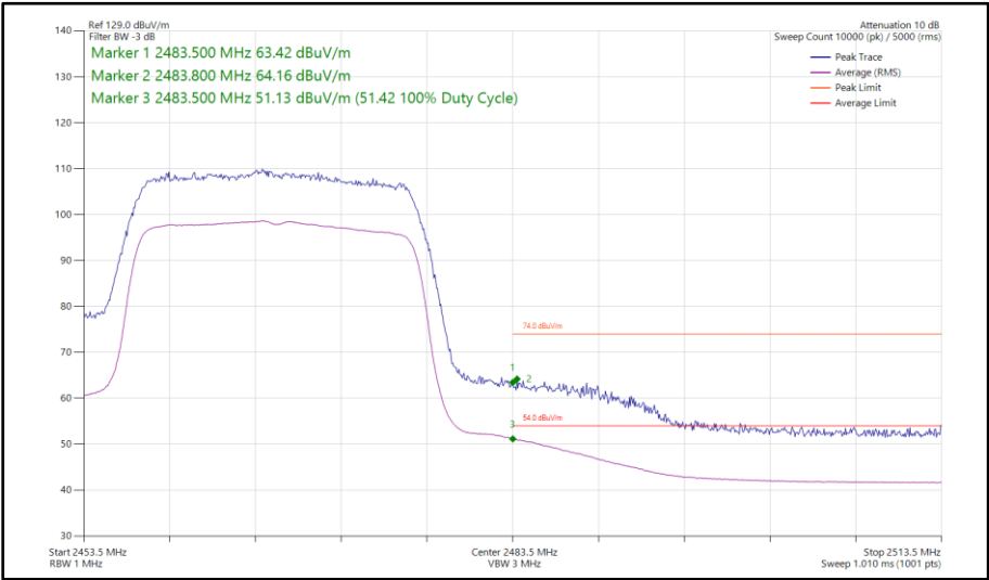
Figure 38 - 802.11ax HE20, SU, SISO, Core 0 - 2467 MHz Band Edge Frequency 2483.5 MHz
