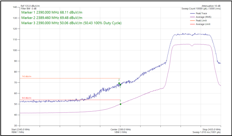
Figure 50 - 802.11n HT20, SISO, Core 1 - 2422 MHz Band Edge Frequency 2390 MHz
