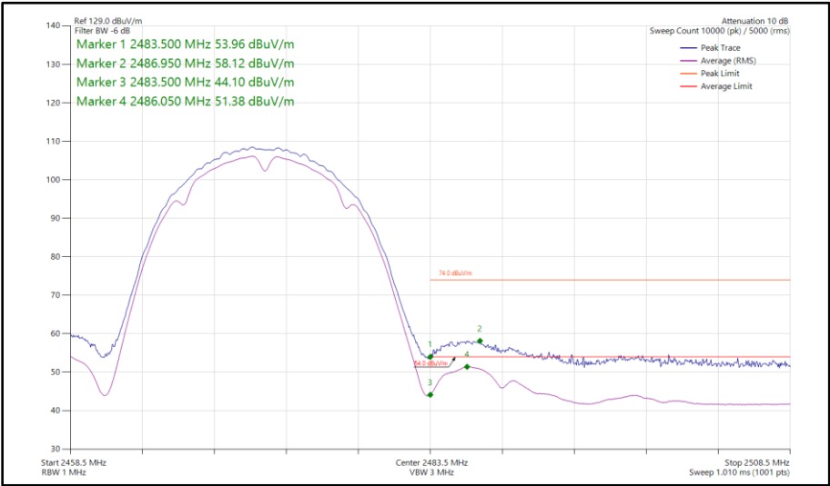
Figure 61 - 802.11b, SISO, Core 1 - 2472 MHz Band Edge Frequency 2483.5 MHz
