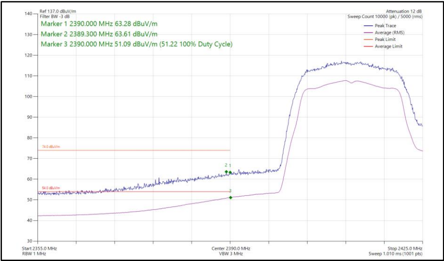
Figure 48 - 802.11n HT20, SISO, Core 1 - 2412 MHz Band Edge Frequency 2390 MHz
