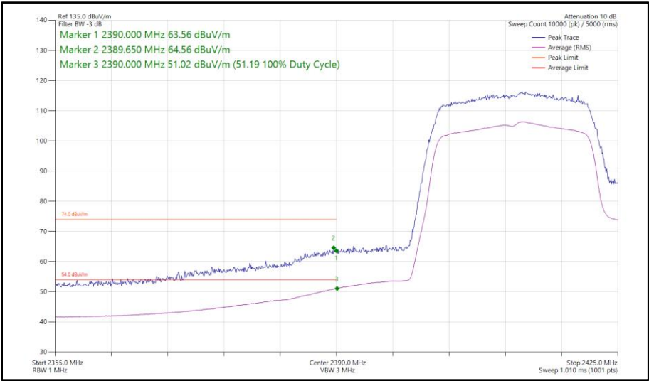
Figure 52 - 802.11ax HE20, SU, SISO, Core 1 - 2412 MHz Band Edge Frequency 2390 MHz
