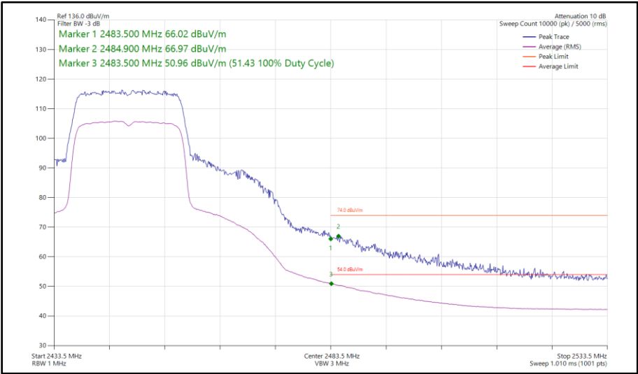
Figure 32 - 802.11ax HE20, SU, SISO, Core 0 - 2447 MHz Band Edge Frequency 2483.5 MHz
