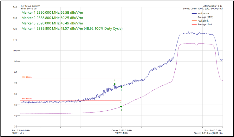
Figure 51 - 802.11n HT20, SISO, Core 1 - 2427 MHz Band Edge Frequency 2390 MHz
