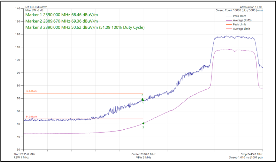
Figure 58 - 802.11ax HE20, SU, SISO, Core 1 - 2432 MHz Band Edge Frequency 2390 MHz
