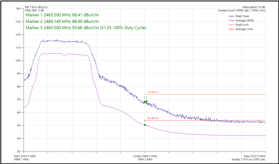
Figure 63 - 802.11g, SISO, Core 1 - 2457 MHz Band Edge Frequency 2483.5 MHz
