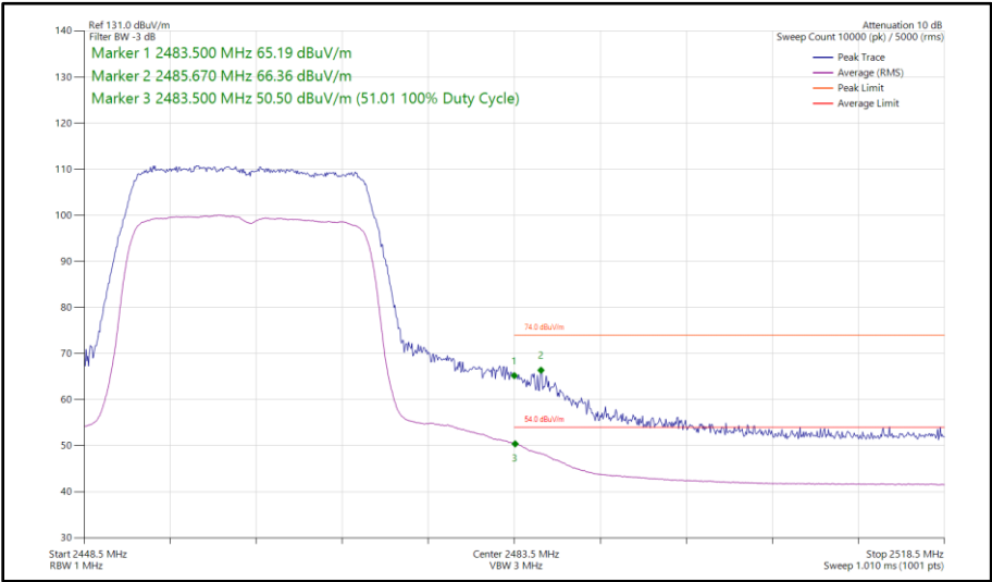
Figure 36 - 802.11ax HE20, SU, SISO, Core 0 - 2462 MHz Band Edge Frequency 2483.5 MHz
