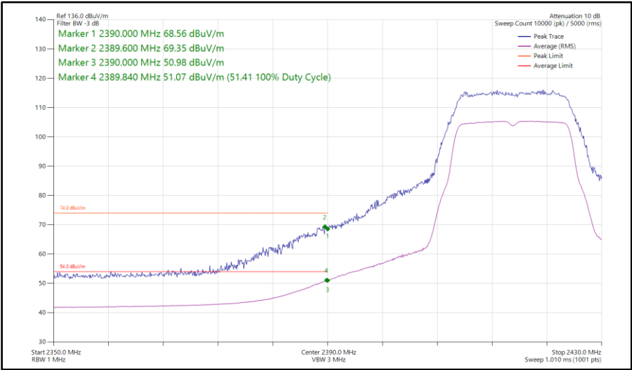
Figure 45 - 802.11g, SISO, Core 1 - 2417 MHz Band Edge Frequency 2390 MHz
