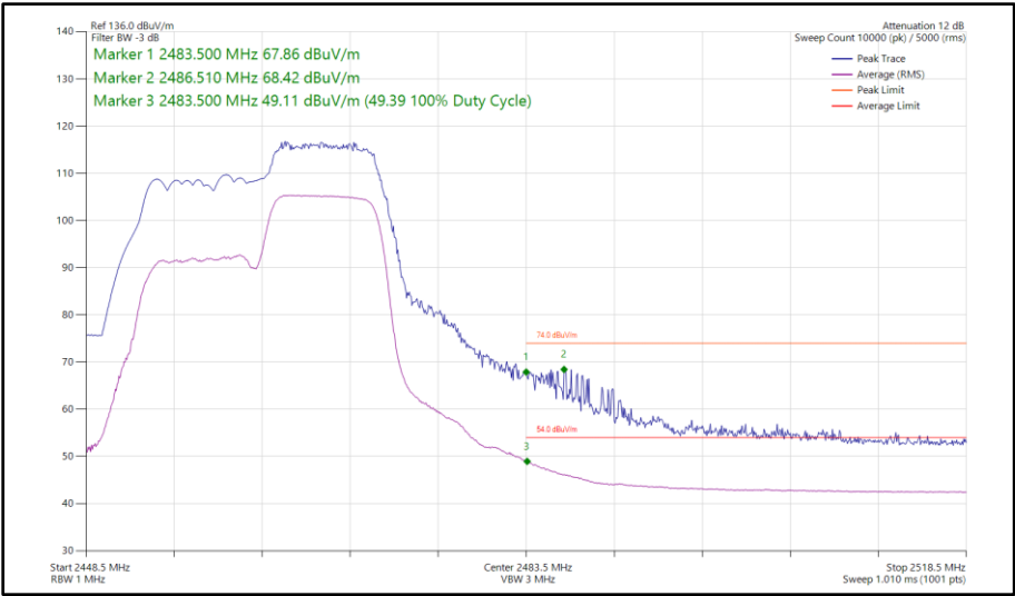
Figure 37 - 802.11ax HE20, RU 106-54, SISO, Core 0 - 2462 MHz Band Edge Frequency 2483.5 MHz
