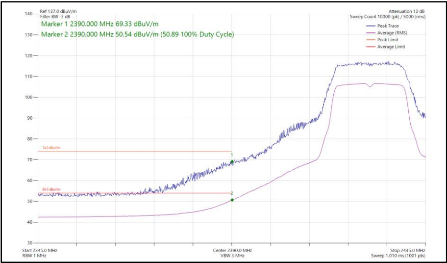
Figure 46 - 802.11g, SISO, Core 1 - 2422 MHz Band Edge Frequency 2390 MHz
