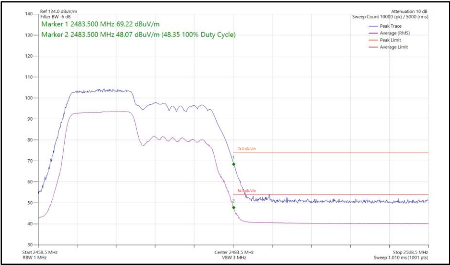
Figure 41 - 802.11ax HE20, RU 106-53, SISO, Core 0 - 2472 MHz Band Edge Frequency 2483.5 MHz
