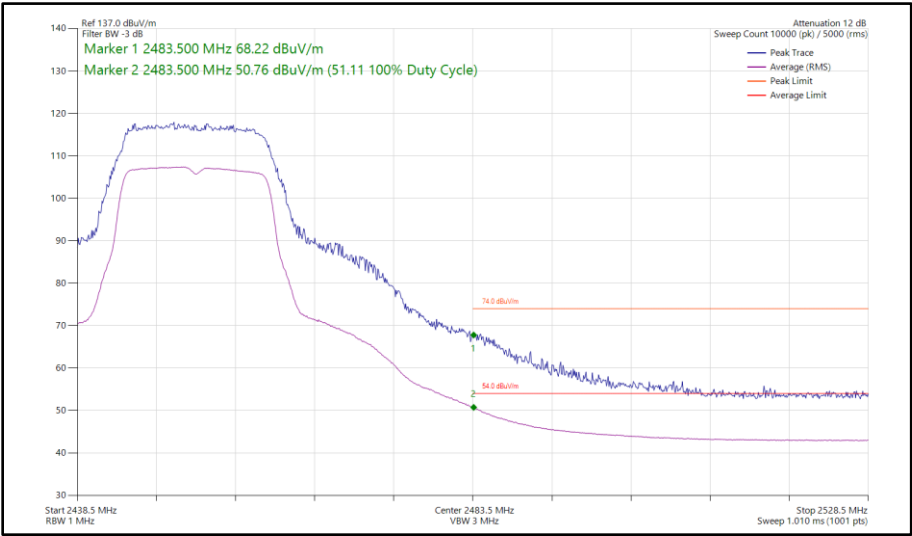
Figure 62 - 802.11g, SISO, Core 1 - 2452 MHz Band Edge Frequency 2483.5 MHz
