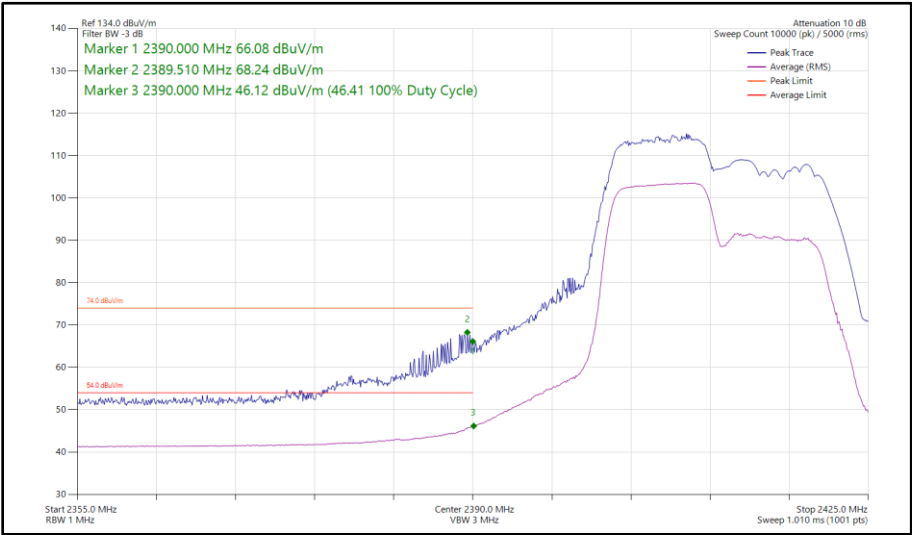
Figure 53 - 802.11ax HE20, RU 106-53, SISO, Core 1 - 2412 MHz Band Edge Frequency 2390 MHz
