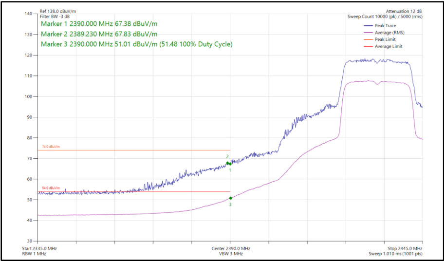
Figure 17 - 802.11ax HE20, SU, SISO, Core 0 - 2432 MHz Band Edge Frequency 2390 MHz
