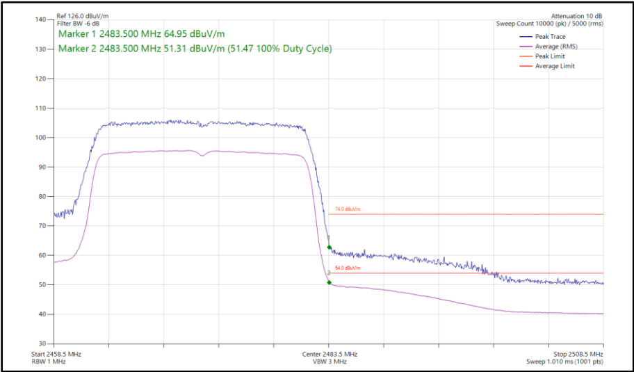
Figure 40 - 802.11ax HE20, SU, SISO, Core 0 - 2472 MHz Band Edge Frequency 2483.5 MHz
