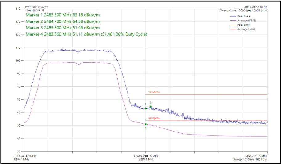
Figure 30 - 802.11n HT20, SISO, Core 0 - 2467 MHz Band Edge Frequency 2483.5 MHz
