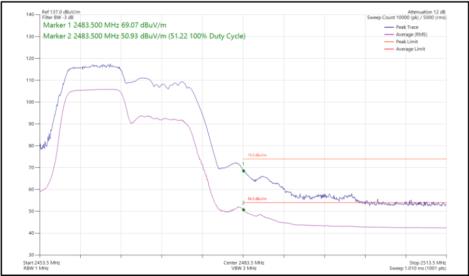
Figure 39 - 802.11ax HE20, RU 106-53, SISO, Core 0 - 2467 MHz Band Edge Frequency 2483.5 MHz
