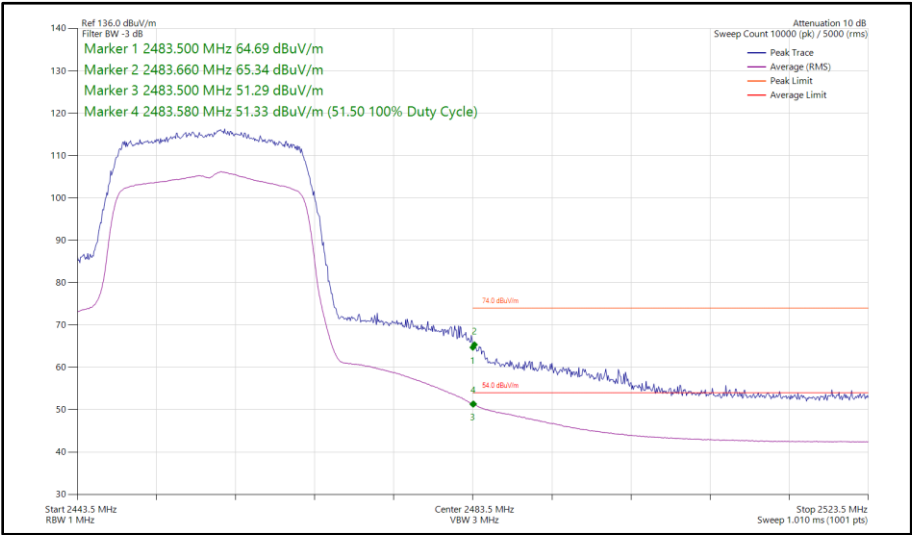
Figure 34 - 802.11ax HE20, SU, SISO, Core 0 - 2457 MHz Band Edge Frequency 2483.5 MHz
