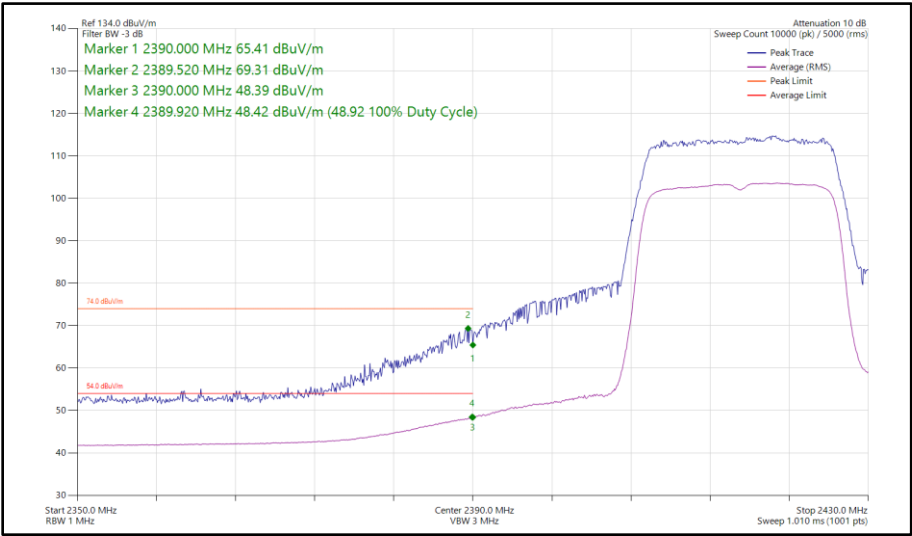
Figure 54 - 802.11ax HE20, SU, SISO, Core 1 - 2417 MHz Band Edge Frequency 2390 MHz
