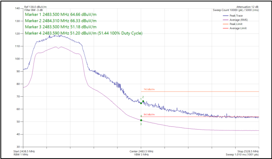
Figure 27 - 802.11n HT20, SISO, Core 0 - 2452 MHz Band Edge Frequency 2483.5 MHz
