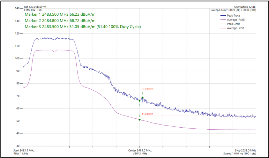
Figure 26 - 802.11n HT20, SISO, Core 0 - 2447 MHz Band Edge Frequency 2483.5 MHz
