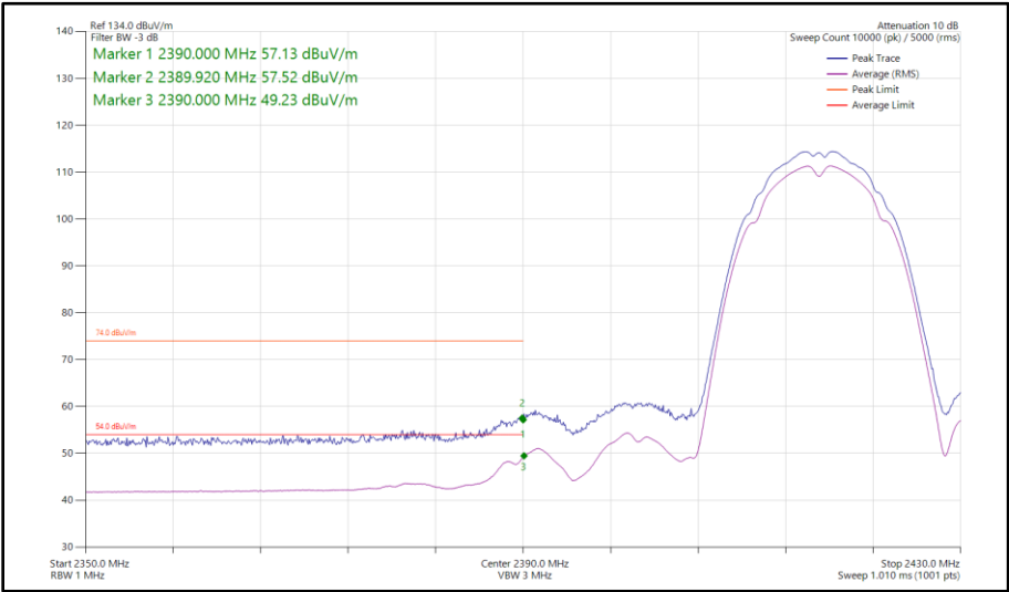
Figure 43 - 802.11b, SISO, Core 1 - 2417 MHz Band Edge Frequency 2390 MHz
