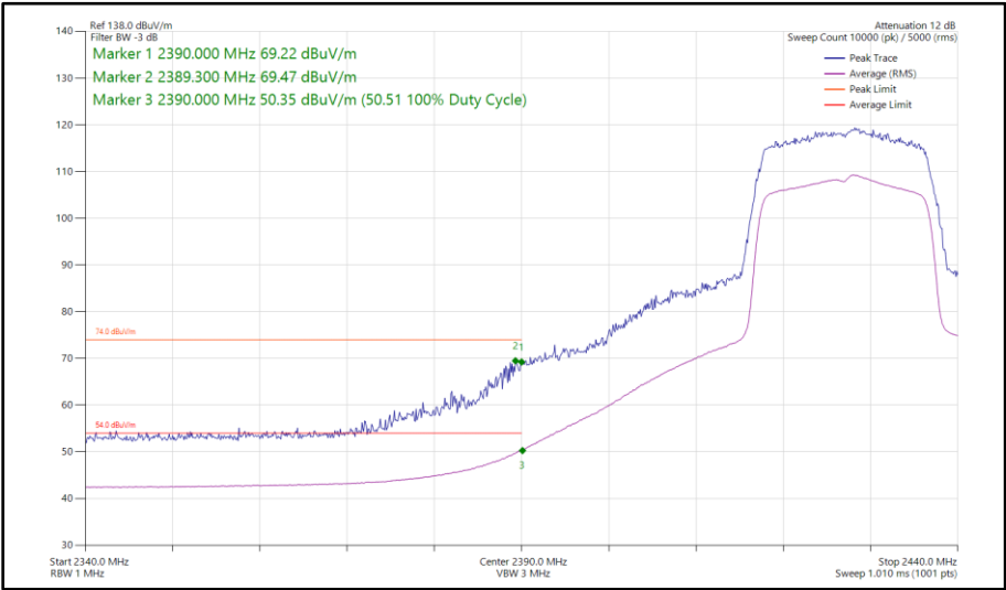
Figure 57 - 802.11ax HE20, SU, SISO, Core 1 - 2427 MHz Band Edge Frequency 2390 MHz
