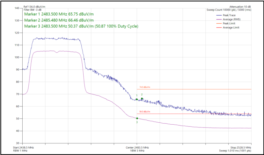
Figure 33 - 802.11ax HE20, SU, SISO, Core 0 - 2452 MHz Band Edge Frequency 2483.5 MHz
