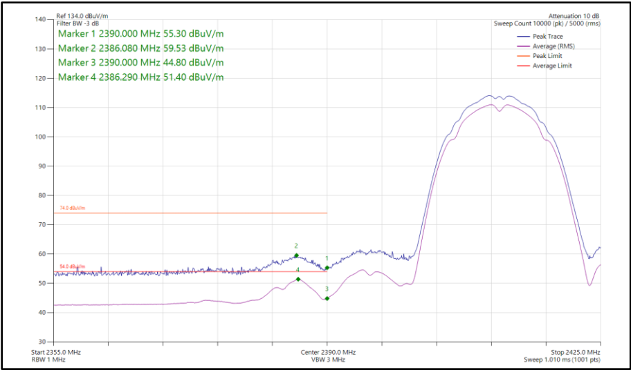
Figure 42 - 802.11b, SISO, Core 1 - 2412 MHz Band Edge Frequency 2390 MHz
