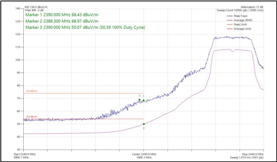
Figure 47 - 802.11g, SISO, Core 1 - 2427 MHz Band Edge Frequency 2390 MHz
