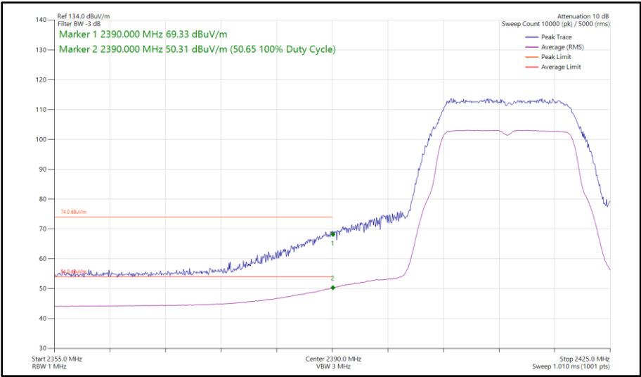
Figure 44 - 802.11g, SISO, Core 1 - 2412 MHz Band Edge Frequency 2390 MHz
