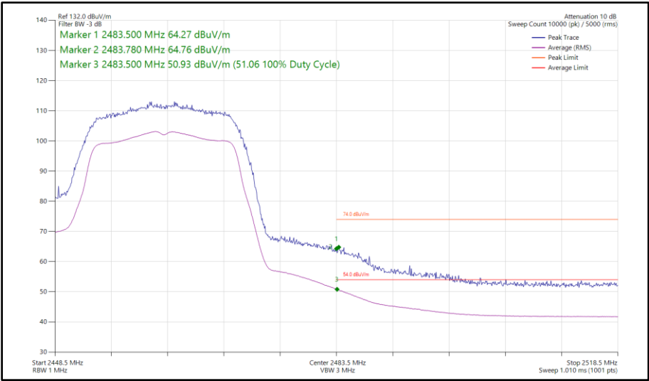
Figure 29 - 802.11n HT20, SISO, Core 0 - 2462 MHz Band Edge Frequency 2483.5 MHz
