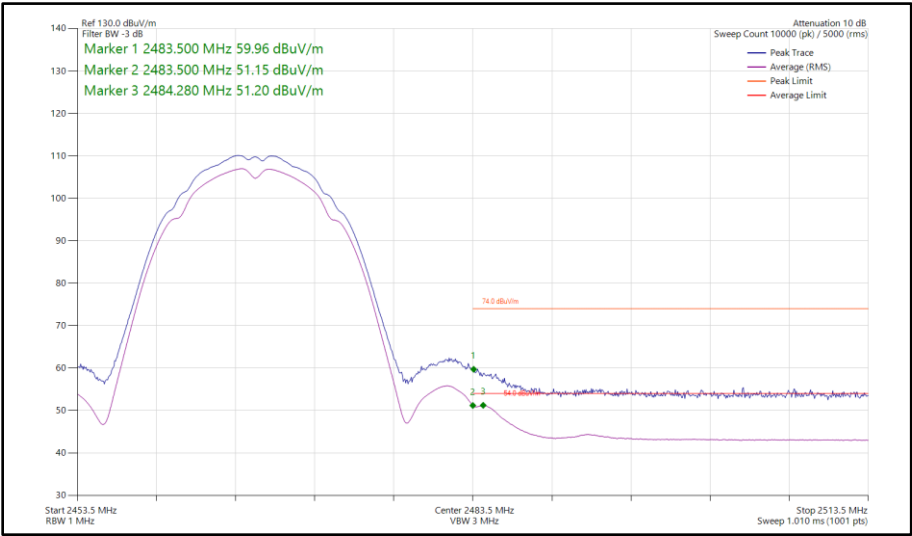
Figure 19 - 802.11b, SISO, Core 0 - 2467 MHz Band Edge Frequency 2483.5 MHz
