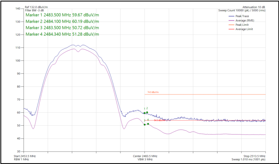
Figure 60 - 802.11b, SISO, Core 1 - 2467 MHz Band Edge Frequency 2483.5 MHz
