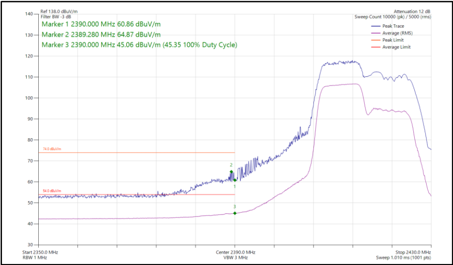
Figure 55 - 802.11ax HE20, RU 106-53, SISO, Core 1 - 2417 MHz Band Edge Frequency 2390 MHz
