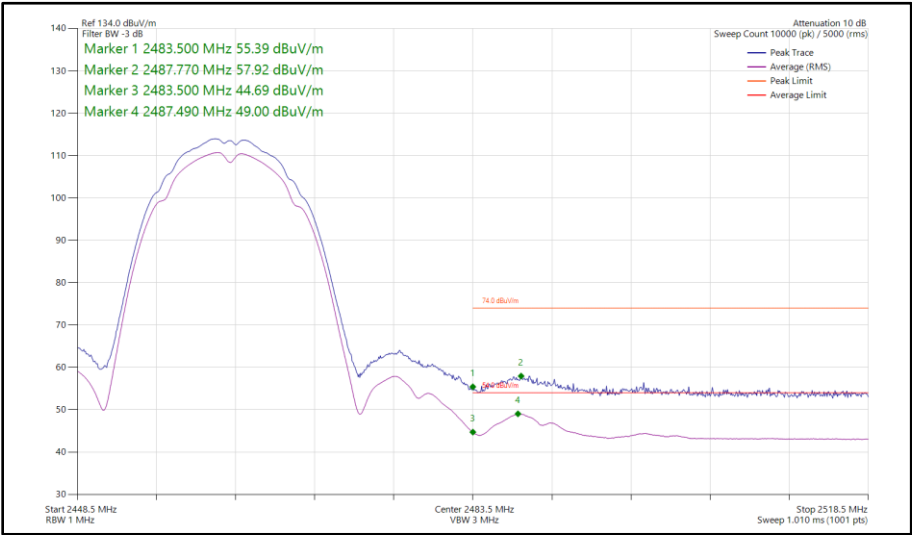
Figure 59 - 802.11b, SISO, Core 1 - 2462 MHz Band Edge Frequency 2483.5 MHz
