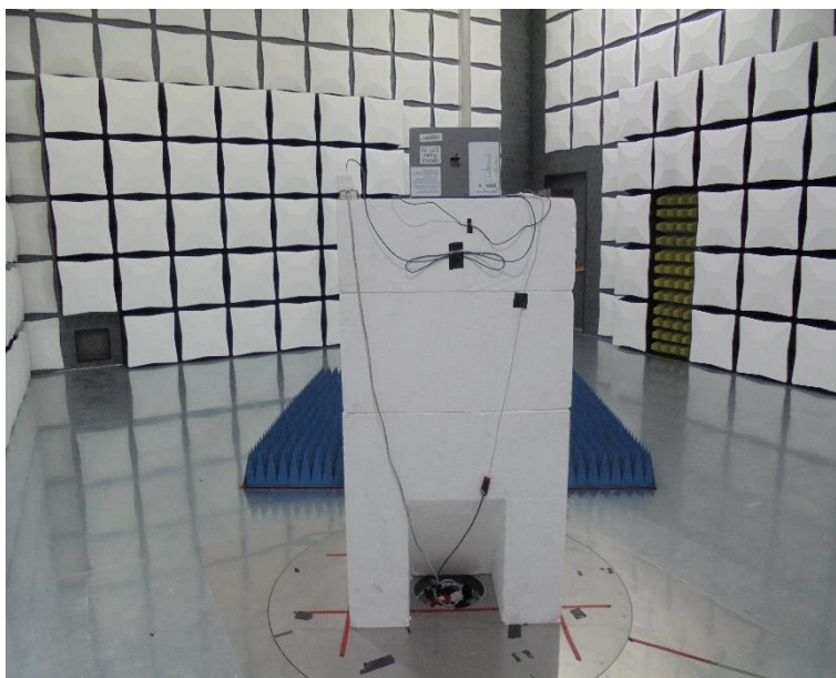
Figure 3 - Radiated Disturbance - Above 1 GHz
