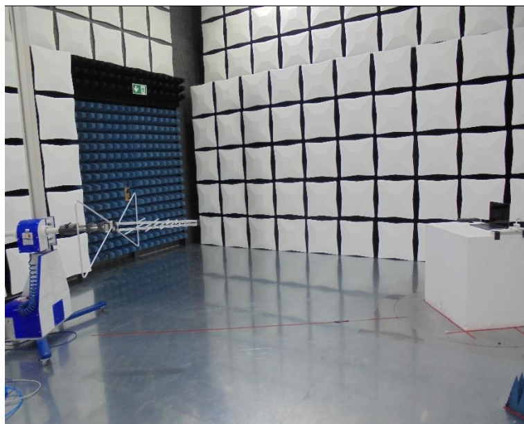
Figure 2 - Radiated Disturbance - Below 1 GHz
