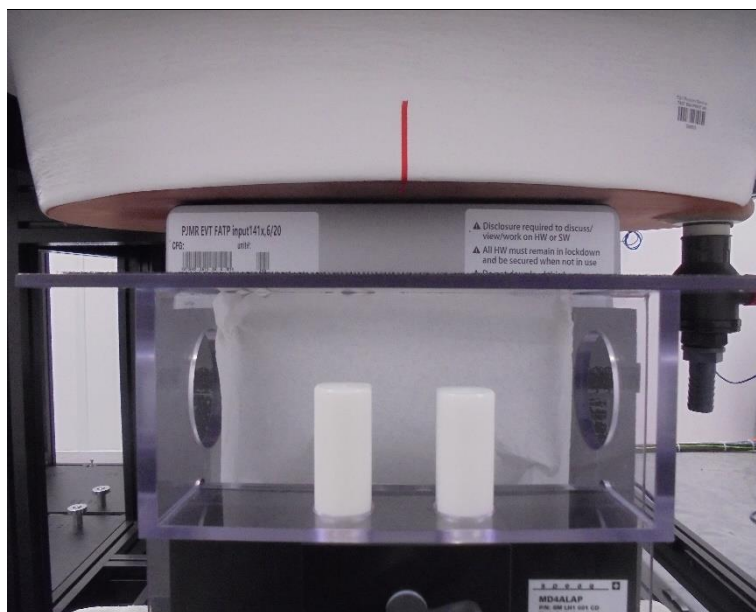
Figure 6 - SAR Bottom Position
