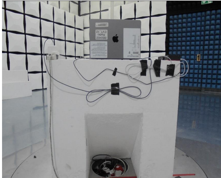
Figure 1 - Radiated Disturbance - Below 1 GHz
