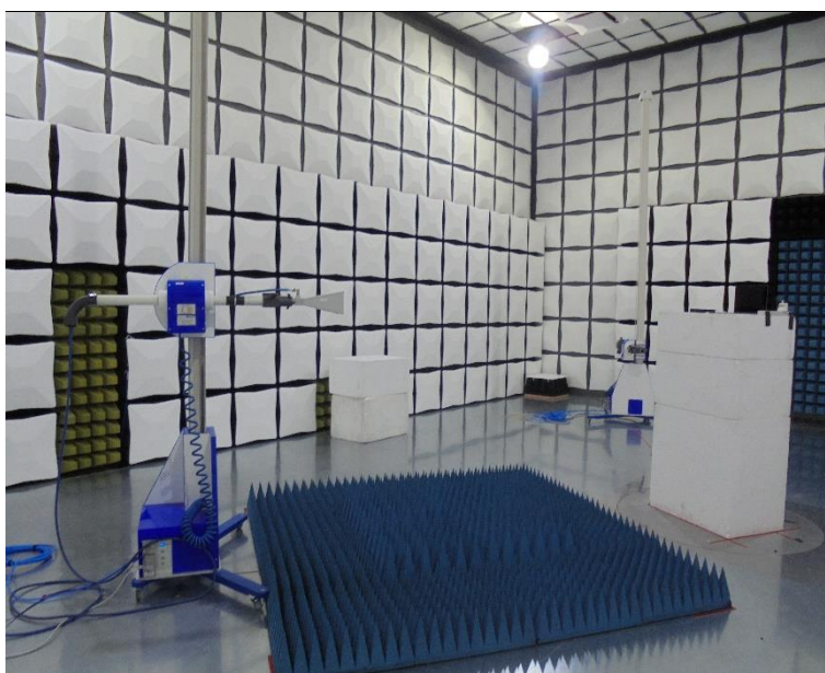
Figure 4 - Radiated Disturbance - Above 1 GHz
