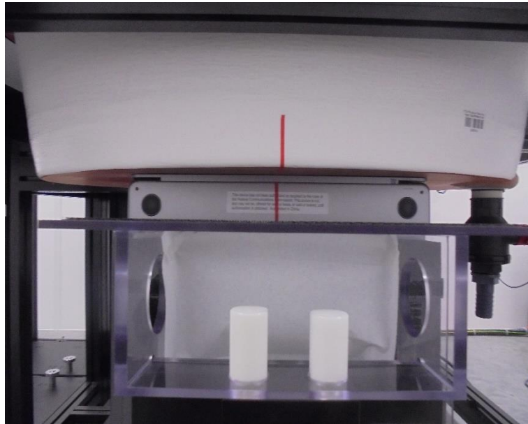
Figure 5 - SAR - Rear of Display Position
