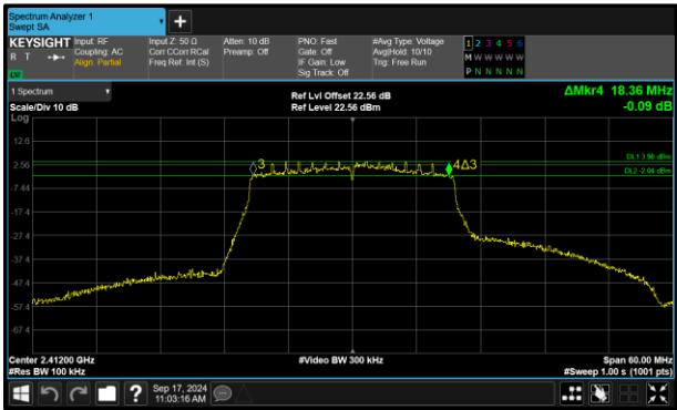
Figure 85 - 802.11ax HE20 SU Minimum 6 dB EBW
