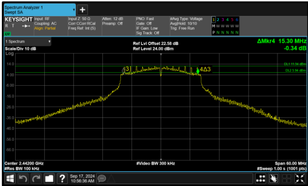
Figure 81 - 802.11g Minimum 6 dB EBW
