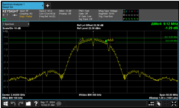
Figure 80 - 802.11b Maximum 6 dB EBW
