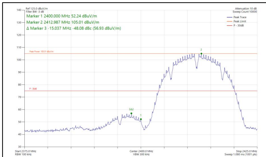
Figure 118 - 802.11b, SISO, Core 1 - 2412 MHz Band Edge Frequency 2400 MHz
