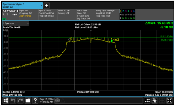
Figure 83 - 802.11n HT20 Minimum 6 dB EBW
