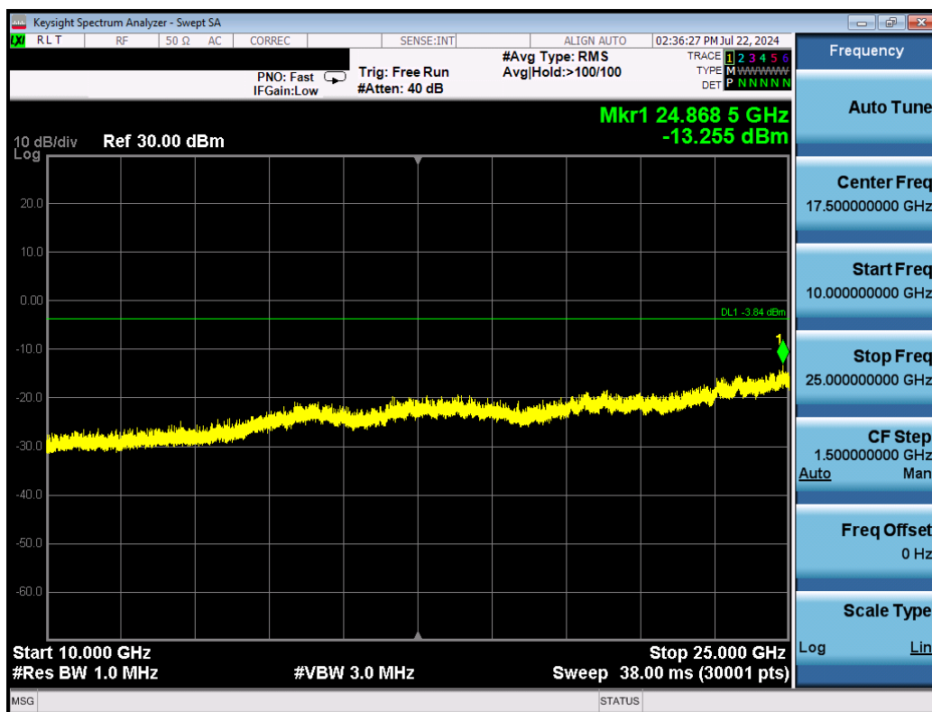
Plot 7-34. Conducted Spurious Plot (Bluetooth (HDR4), 4 Mbps, – Ch. 1)
