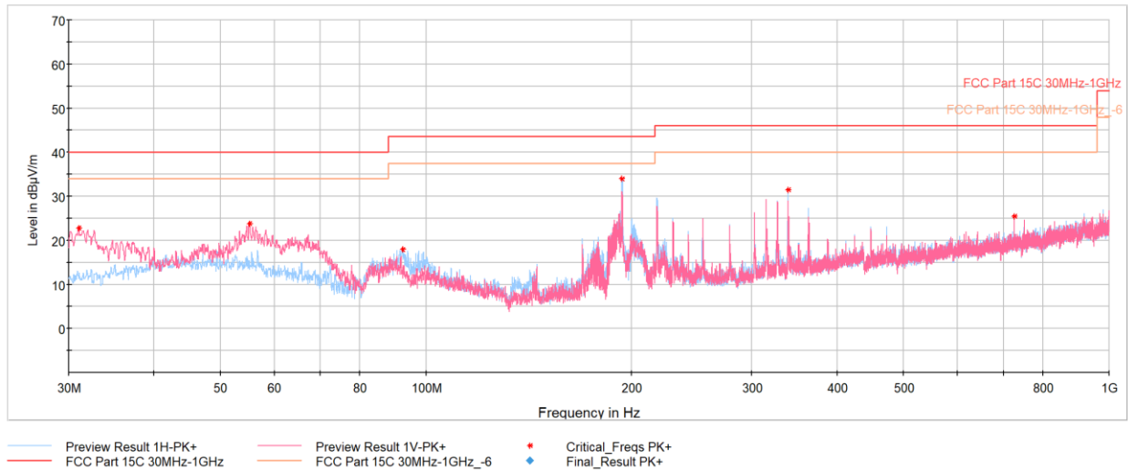
Plot 7-53. Radiated Spurious Emissions Below 1GHz (4Mbps, – Ch.73 with AC/DC Adapter and USB-C cable)
