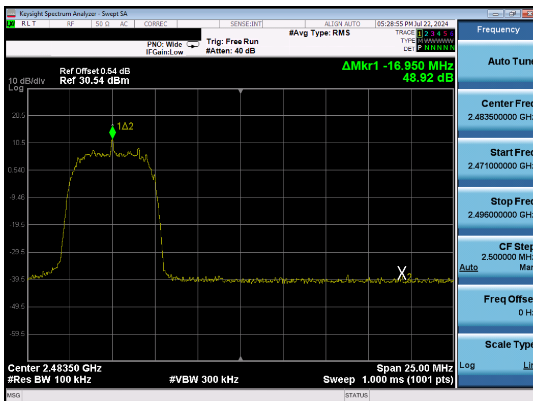
Plot 7-32. Band Edge Plot (Bluetooth (HDRp8), – Ch. 73)
