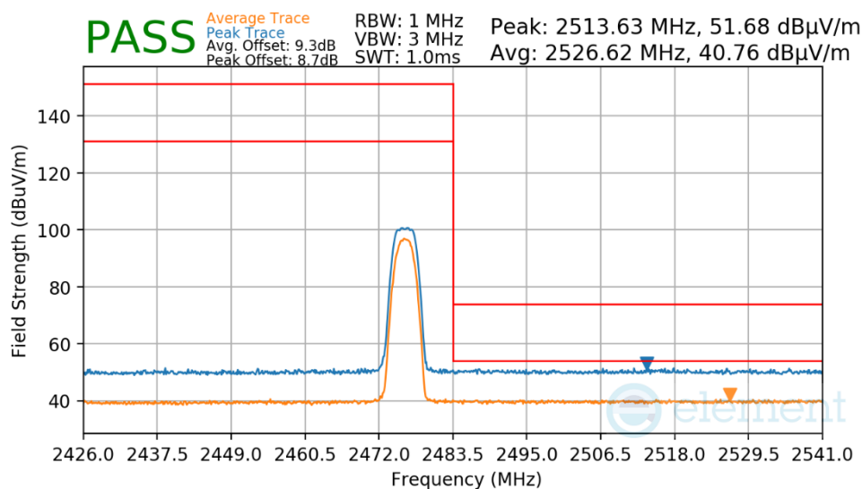
Plot 7-51. Radiated Restricted Upper Band Edge Measurement
