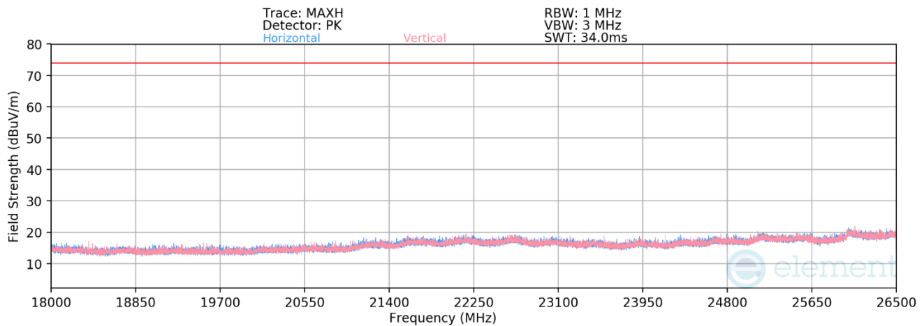
Plot 7-41. Radiated Spurious Emissions Above 18GHz (4Mbps, HDR4, - Ch. 73)
