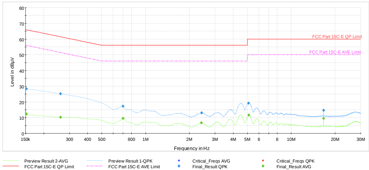
Plot 7-54. AC Line Conducted Plot with Bluetooth HDR (L1, 4Mbps - Ch.73 with host PC and USB-C cable)
