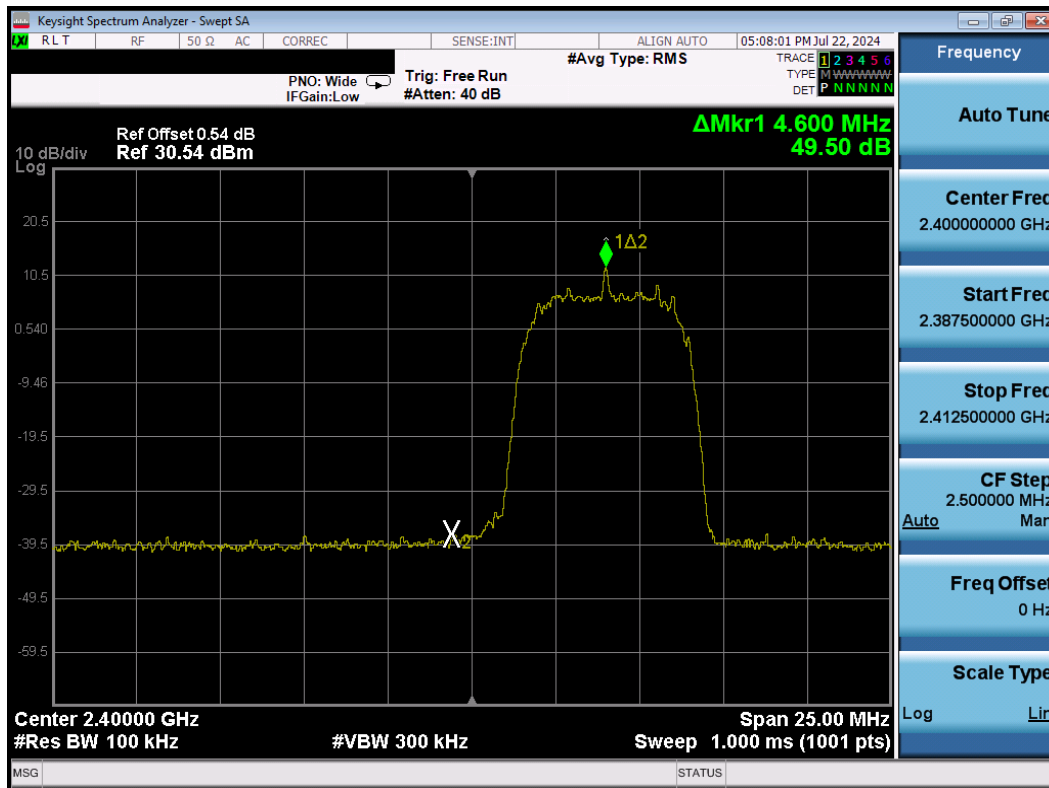
Plot 7-27. Band Edge Plot (Bluetooth (HDR8), – Ch. 1)
