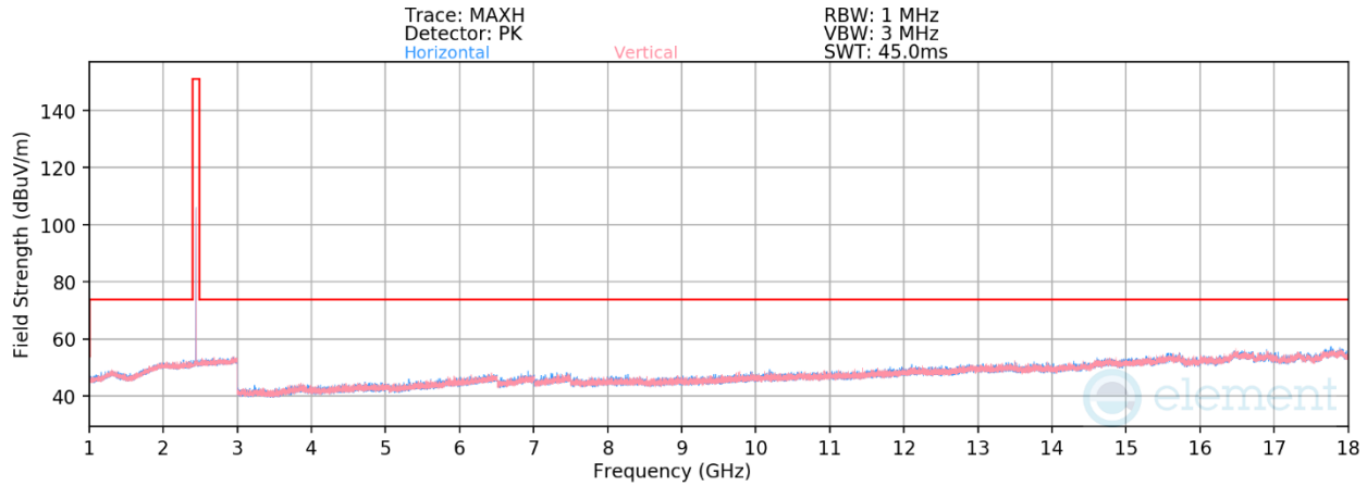
Plot 7-43. Radiated Spurious Emissions 1-18GHz (4Mbps, HDRp4, - Ch. 37)
