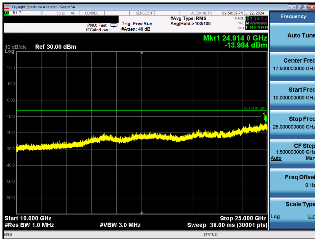
Plot 7-38. Conducted Spurious Plot (Bluetooth (HDR4), 4 Mbps, – Ch. 73)
