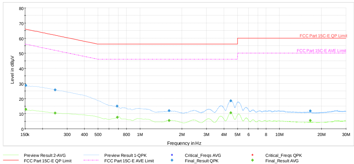
Plot 7-55. AC Line Conducted Plot with Bluetooth HDR (N, 4Mbps - Ch.73 with host PC and USB-C cable)
