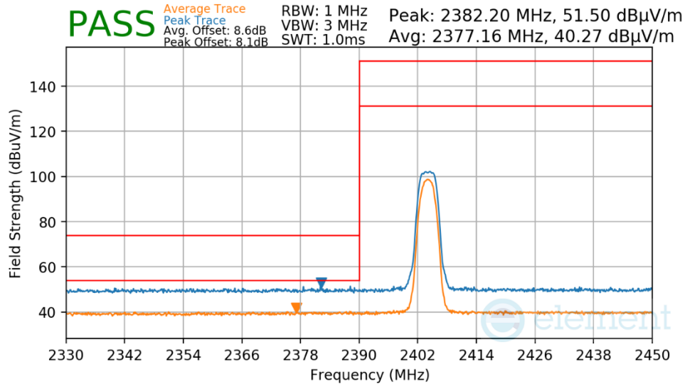
Plot 7-47. Radiated Restricted Lower Band Edge Measurement
