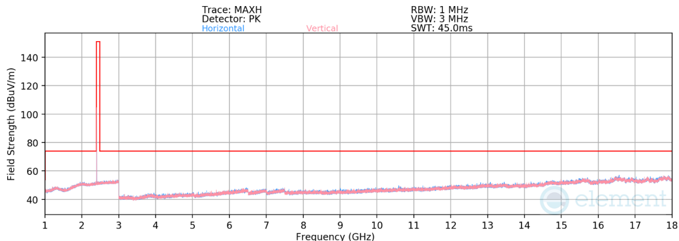
Plot 7-42. Radiated Spurious Emissions 1-18GHz (4Mbps, HDRp4, - Ch. 1)
