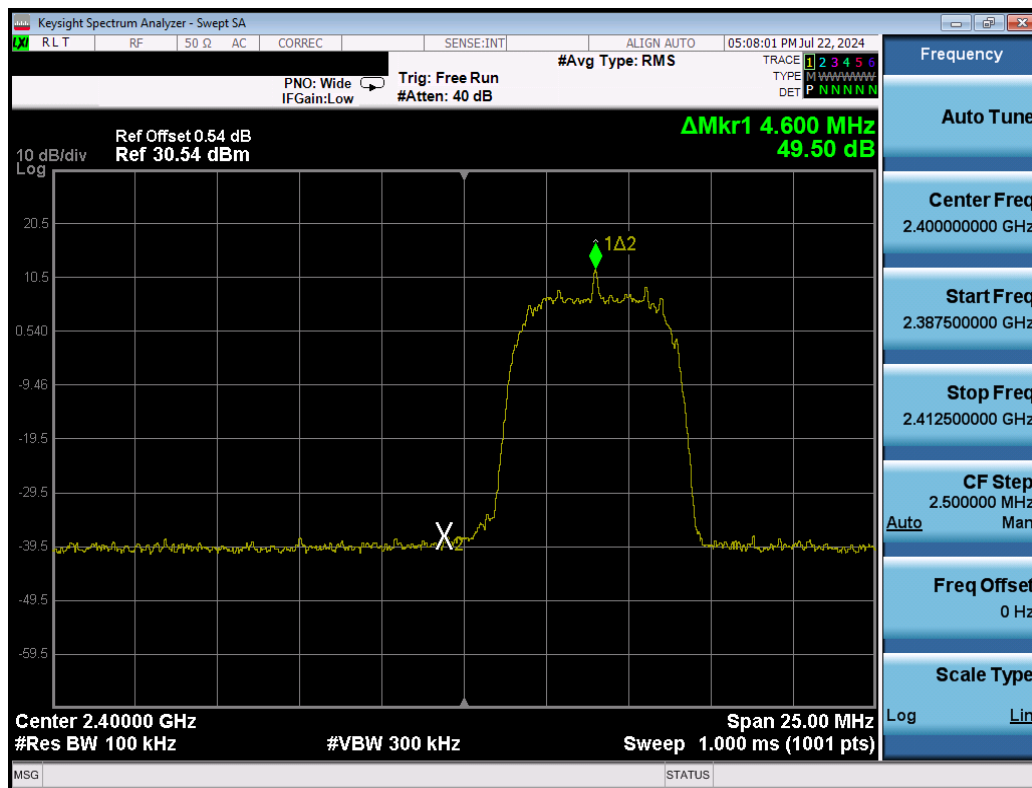
Plot 7-31. Band Edge Plot (Bluetooth (HDRp8), – Ch. 1)
