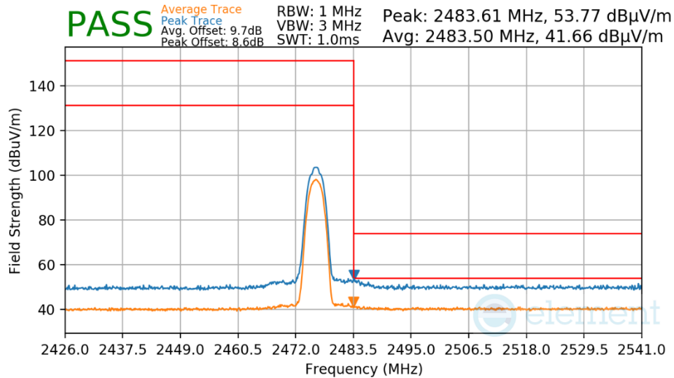
Plot 7-49. Radiated Restricted Upper Band Edge Measurement
