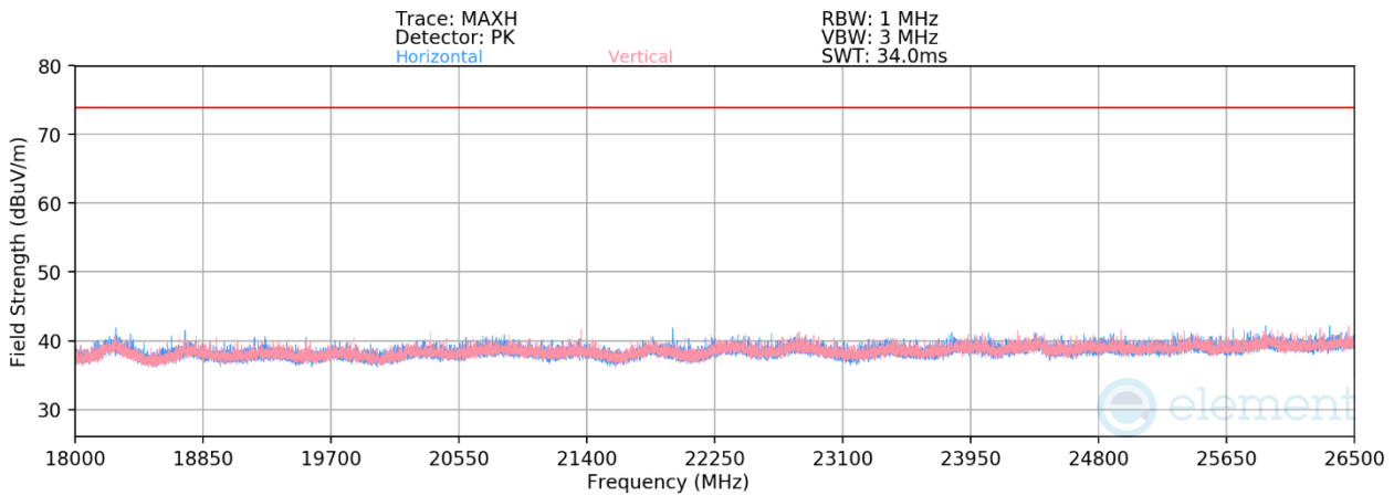
Plot 7-41. Radiated Spurious Emissions Above 18GHz (4Mbps, HDRp4, - Ch. 37)
