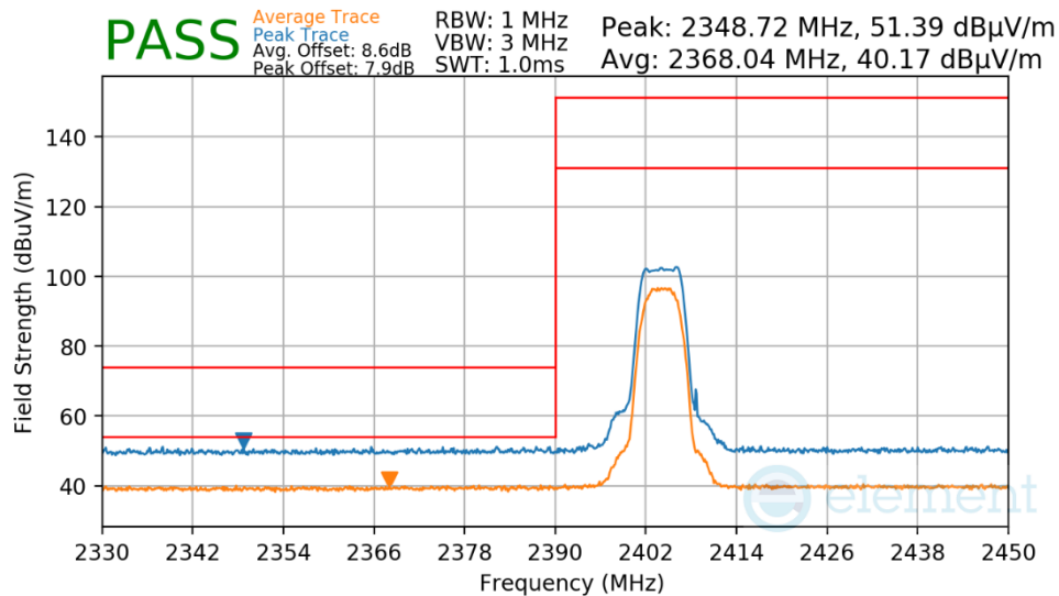
Plot 7-48. Radiated Restricted Lower Band Edge Measurement
