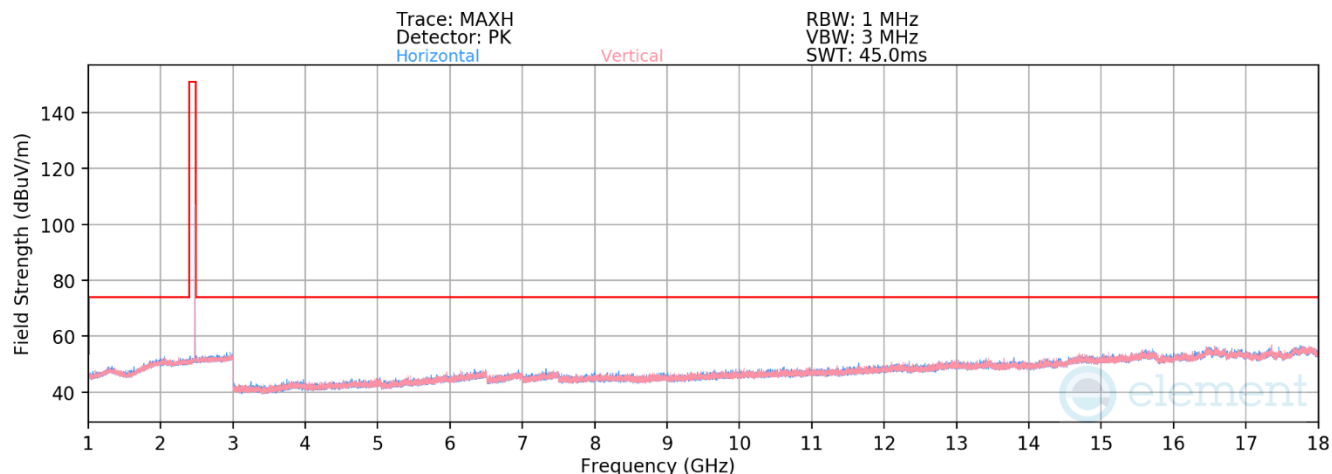
Plot 7-44. Radiated Spurious Emissions 1-18GHz (4Mbps, HDRp4, – Ch. 73)
