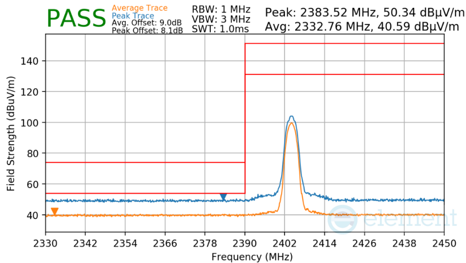
Plot 7-45. Radiated Restricted Lower Band Edge Measurement
