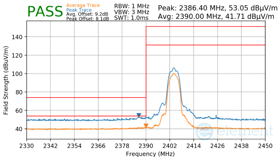
Plot 7-46. Radiated Restricted Lower Band Edge Measurement
