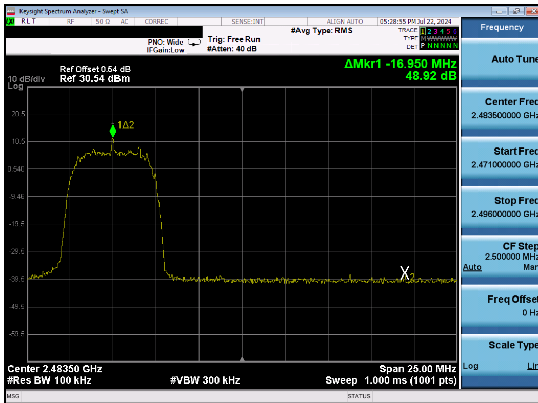
Plot 7-28. Band Edge Plot (Bluetooth (HDR8), – Ch. 73)
