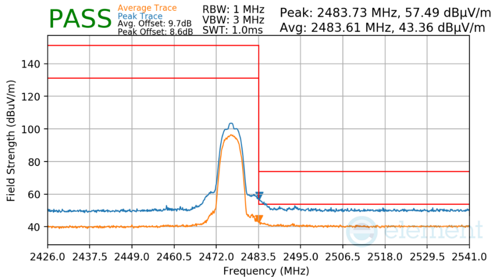
Plot 7-50. Radiated Restricted Upper Band Edge Measurement
