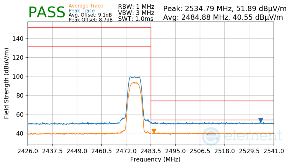
Plot 7-52. Radiated Restricted Upper Band Edge Measurement
