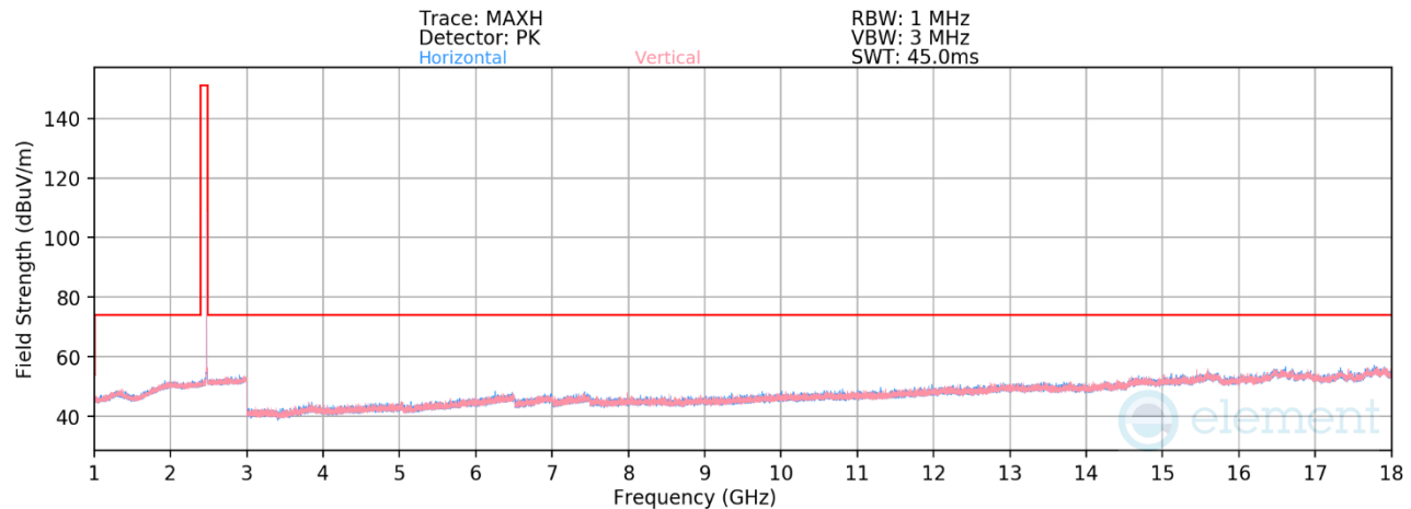
Plot 7-41. Radiated Spurious Emissions 1-18GHz (4Mbps, HDR4, - Ch. 73)
