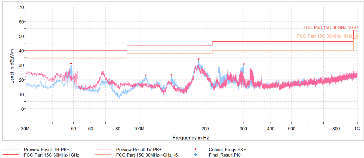
Plot 7-31. Radiated Spurious Emissions Below 1GHz (1Mbps, Ch.39, Pol. H & V, with host PC with USB-C cable)
