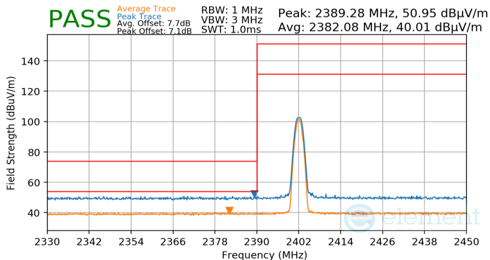
Plot 7-27. Radiated Restricted Lower Band Edge Measurement (Average & Peak)
