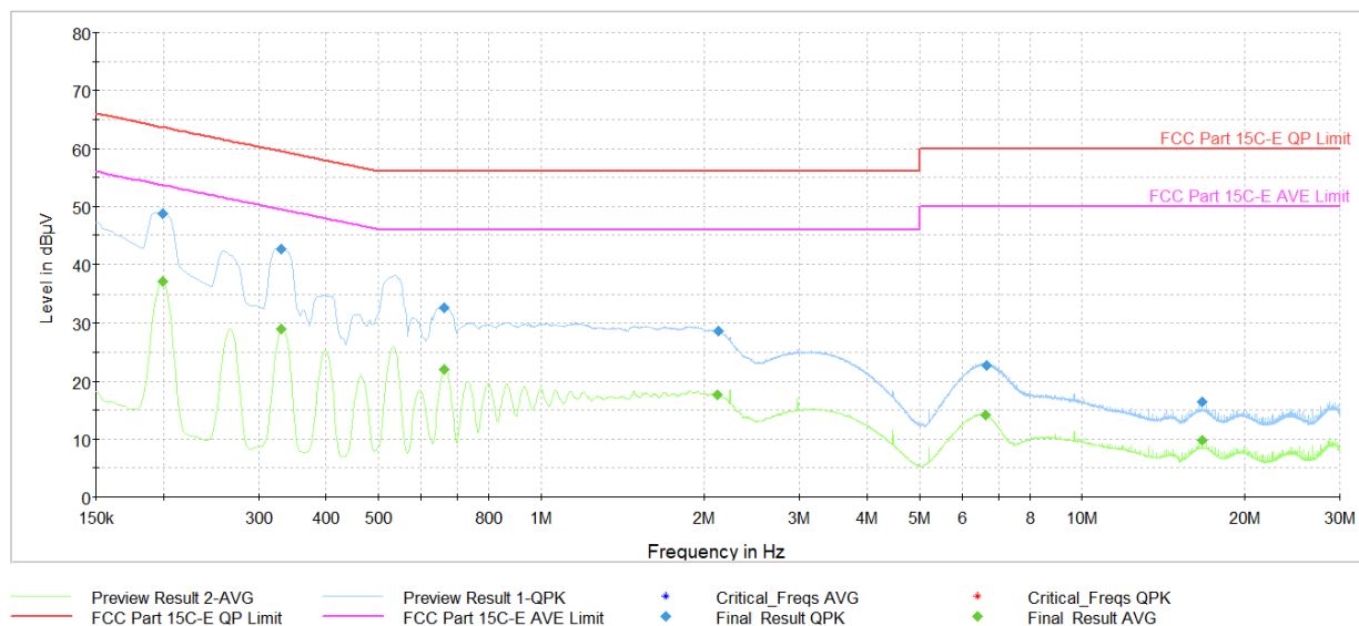
Plot 7-33. AC Line Conducted Plot with Bluetooth LE (N, 1Mbps, Ch.39, with host PC with USB-C cable)
