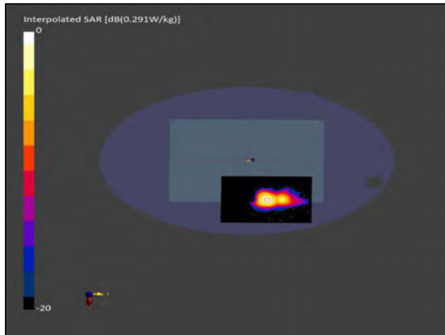
Figure C.9: SAR Testing Results for the A3113 at 5850 MHz Core 1
