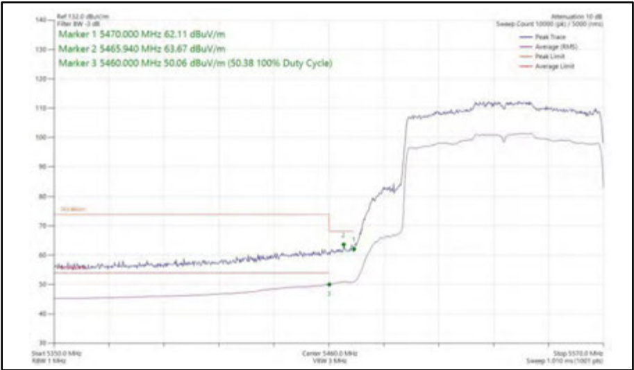
Figure 630 - 802.11ax HE80, SU, SISO, Core 1 - 5530 MHz Band Edge Frequency 5470 MHz
