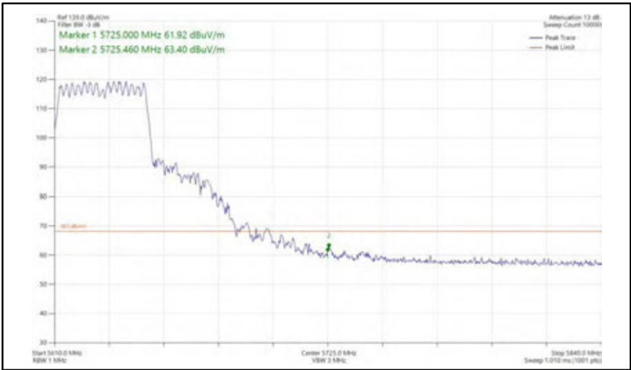
Figure 573 - 802.11ax HE40, SU, CDD, Core 0 + Core 1 - 5630 MHz Band Edge Frequency 5725 MHz
