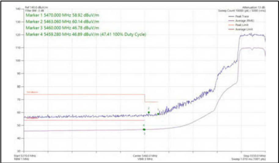
Figure 416 - 802.11ax HE20, SU, SISO, Core 1 - 5540 MHz Band Edge Frequency 5470 MHz
