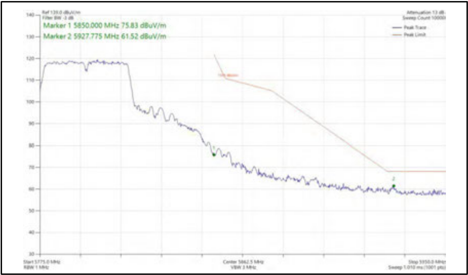
Figure 601 - 802.11n HT40, SDM, Core 0 + Core 1 - 5795 MHz Band Edge Frequency 5850 MHz
