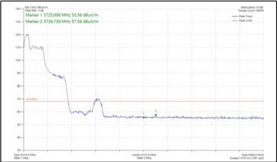
Figure 528 - 802.11ax HE40, RU 52-37, SISO, Core 0 - 5630 MHz Band Edge Frequency 5725 MHz
