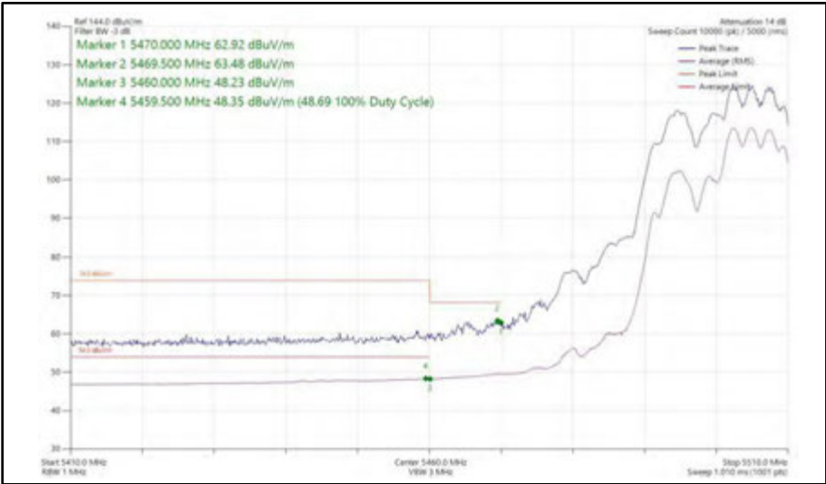
Figure 478 - 802.11ax HE20, RU 106-54, SDM, Core 0 + Core 1 - 5500 MHz Band Edge Frequency 5470 MHz
