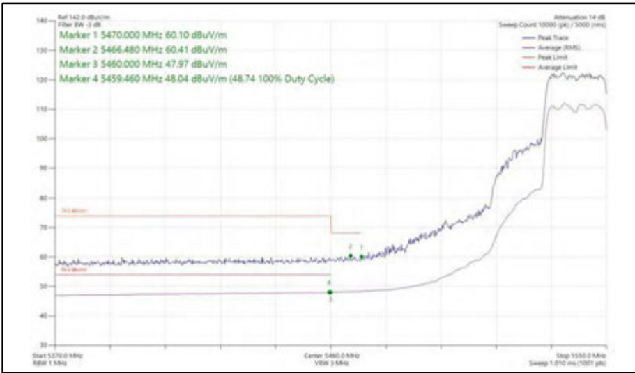
Figure 481 - 802.11ax HE20, SU, SDM, Core 0 + Core 1 - 5540 MHz Band Edge Frequency 5470 MHz
