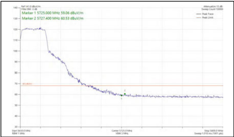
Figure 487 - 802.11n HT20, SDM, Core 0 + Core 1 - 5660 MHz Band Edge Frequency 5725 MHz
