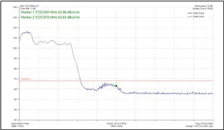
Figure 433 - 802.11ax HE20, RU 52-37, SISO, Core 1 - 5700 MHz Band Edge Frequency 5725 MHz
