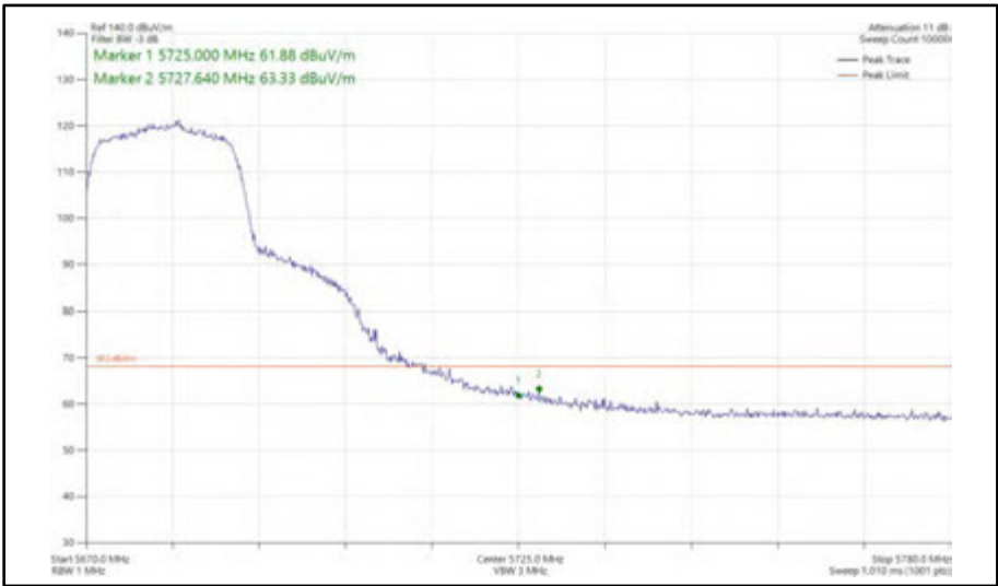
Figure 390 - 802.11n HT20, SISO, Core 0 - 5680 MHz Band Edge Frequency 5725 MHz
