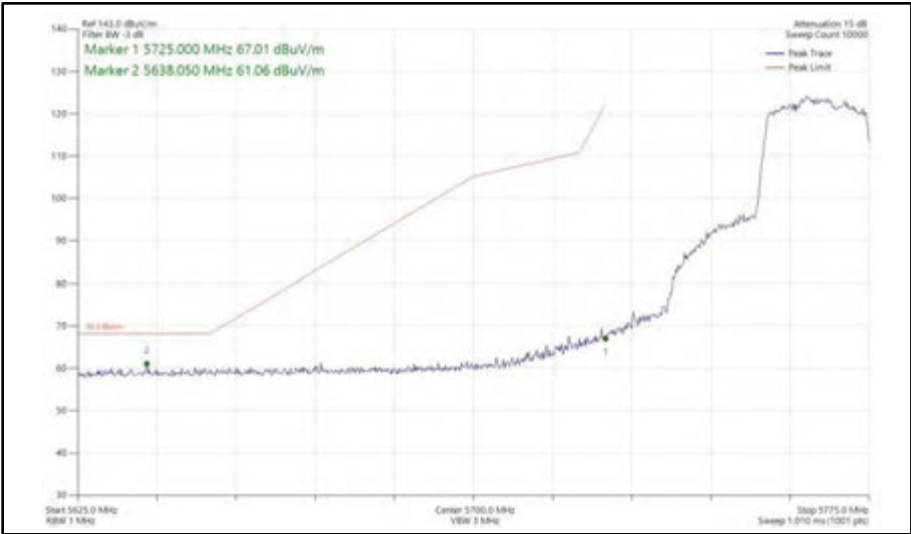
Figure 486 - 802.11ax HE20, SU, SDM, Core 0 + Core 1 - 5765 MHz Band Edge Frequency 5725 MHz
