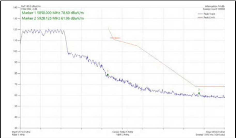
Figure 578 - 802.11n HT40, CDD, Core 0 + Core 1 - 5795 MHz Band Edge Frequency 5850 MHz
