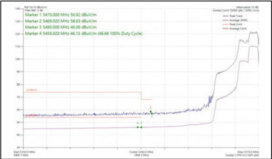
Figure 543 - 802.11ax HE40, RU 106-56, SISO, Core 1 - 5550 MHz Band Edge Frequency 5470 MHz
