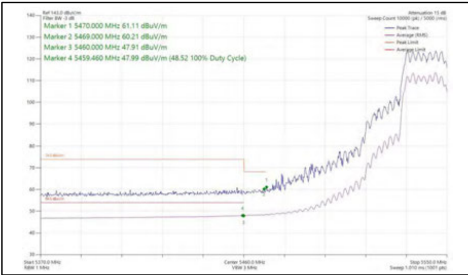
Figure 452 - 802.11ax HE20, SU, CDD, Core 0 + Core 1 - 5540 MHz Band Edge Frequency 5470 MHz
