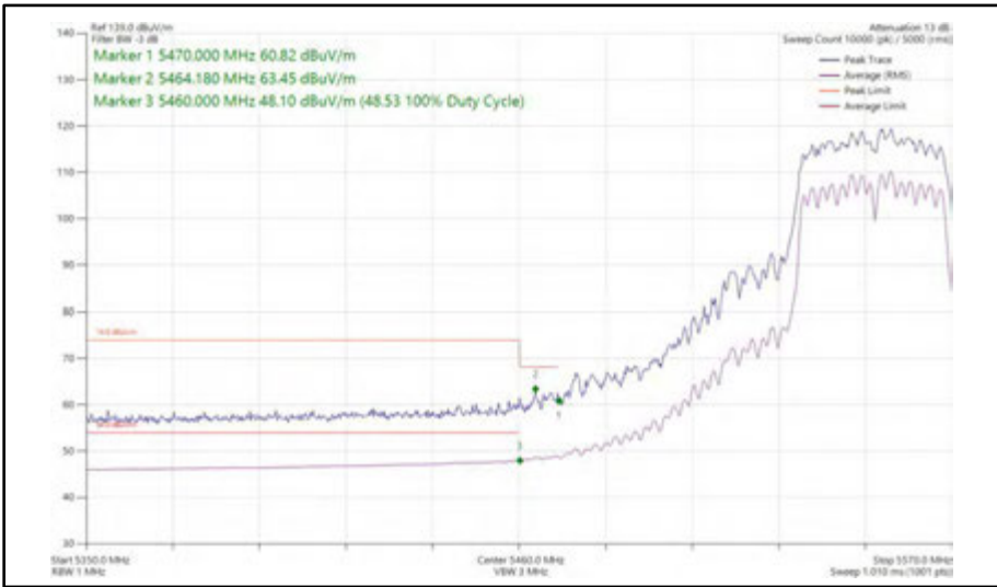
Figure 561 - 802.11n HT40, CDD, Core 0 + Core 1 - 5550 MHz Band Edge Frequency 5470 MHz
