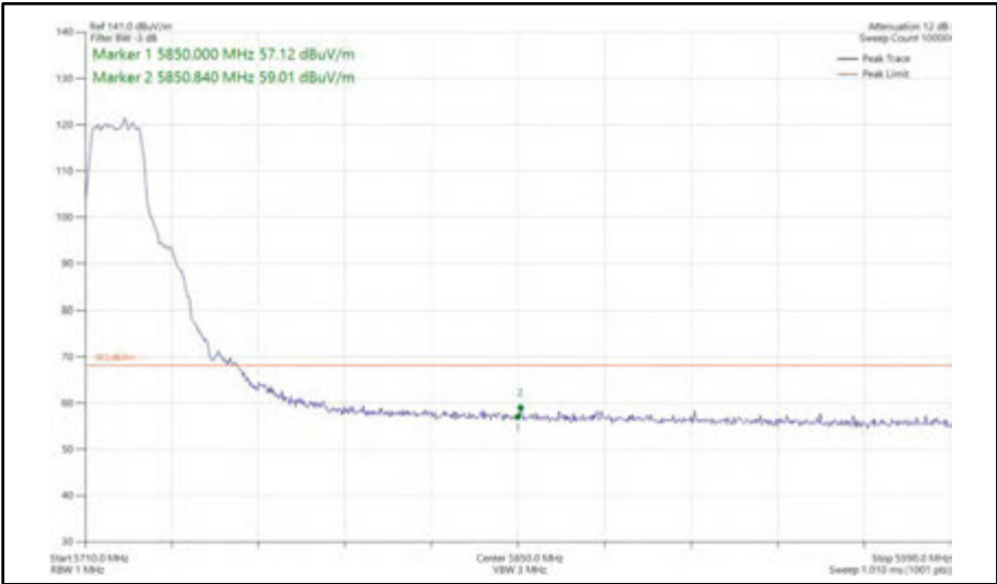
Figure 397 - 802.11a, SISO, Core 0 - 5720 MHz Band Edge Frequency 5850 MHz
