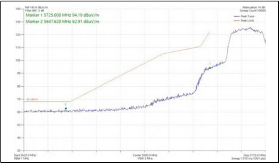
Figure 506 - 802.11ac VHT20, TxBF, Core 0 + Core 1 - 5745 MHz Band Edge Frequency 5725 MHz
