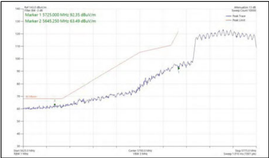
Figure 569 - 802.11ax HE40, SU, CDD, Core 0 + Core 1 - 5755 MHz Band Edge Frequency 5725 MHz
