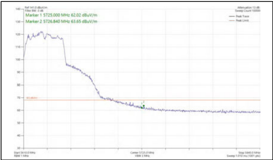
Figure 610 - 802.11ac VHT40, TxBF, Core 0 + Core 1 - 5630 MHz Band Edge Frequency 5725 MHz
