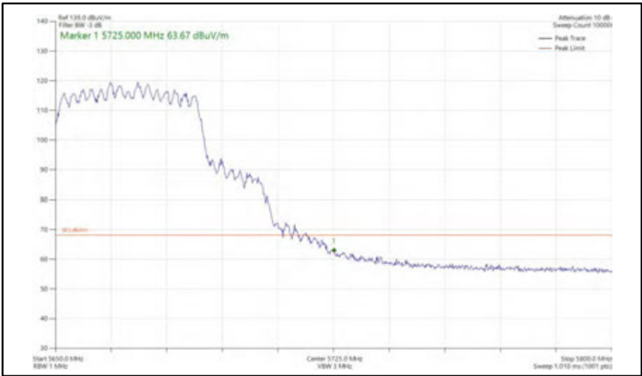
Figure 575 - 802.11ax HE40, SU, CDD, Core 0 + Core 1 - 5670 MHz Band Edge Frequency 5725 MHz
