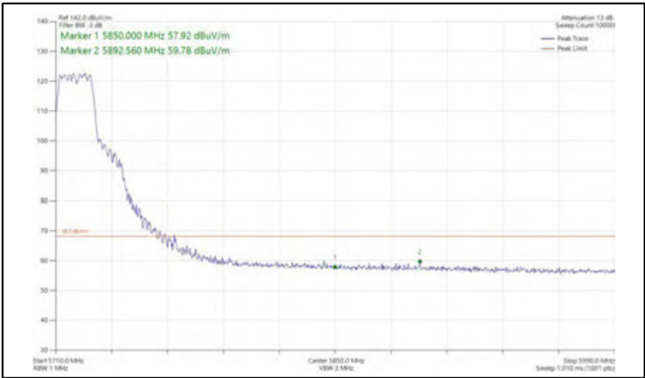
Figure 466 - 802.11n HT20, CDD, Core 0 + Core 1 - 5720 MHz Band Edge Frequency 5850 MHz
