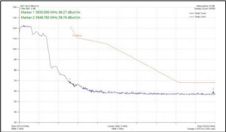
Figure 444 - 802.11ax HE20, RU 106-53, SISO, Core 1 - 5825 MHz Band Edge Frequency 5850 MHz
