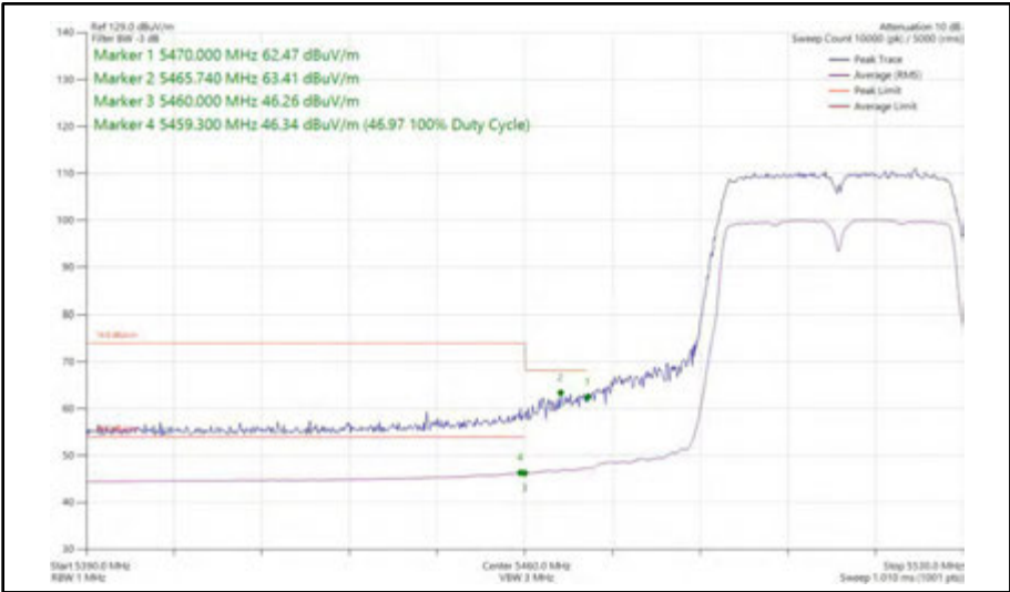
Figure 537 - 802.11n HT40, SISO, Core 1 - 5510 MHz Band Edge Frequency 5470 MHz
