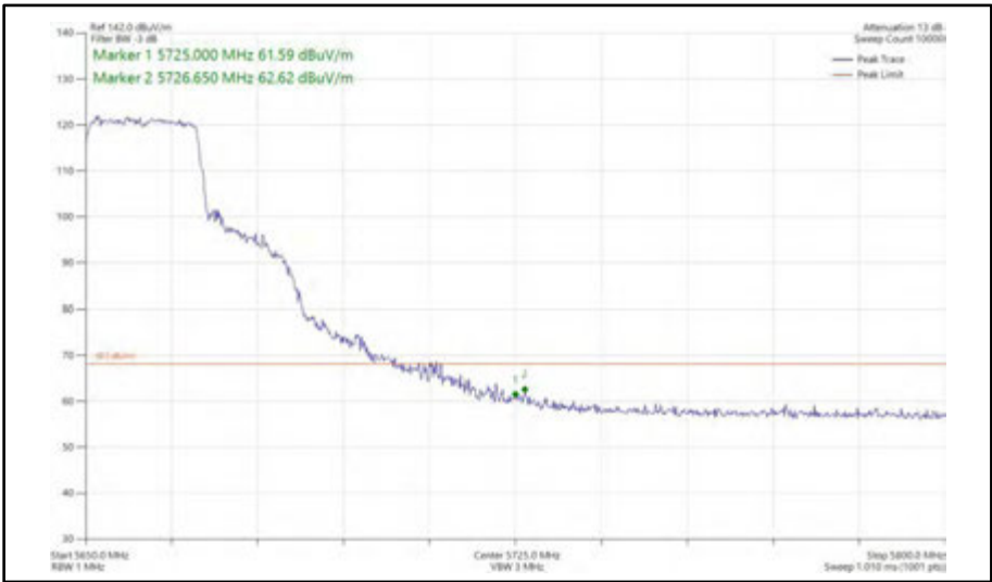
Figure 392 - 802.11ax HE20, SU, SISO, Core 0 - 5660 MHz Band Edge Frequency 5725 MHz
