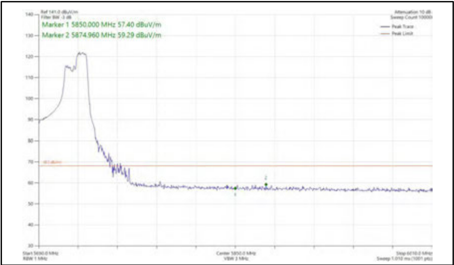
Figure 557 - 802.11ax HE40, RU 106-56, SISO, Core 1 - 5710 MHz Band Edge Frequency 5850 MHz
