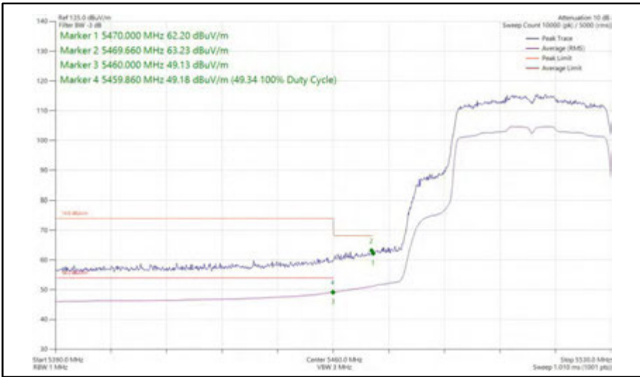
Figure 517 - 802.11ax HE40, SU, SISO, Core 0 - 5510 MHz Band Edge Frequency 5470 MHz
