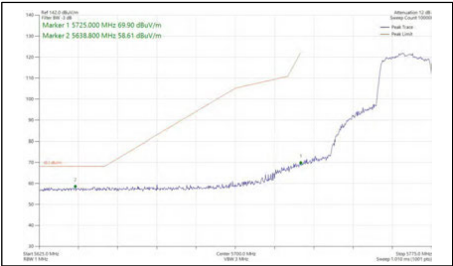
Figure 386 - 802.11ax HE20, SU, SISO, Core 0 - 5765 MHz Band Edge Frequency 5725 MHz
