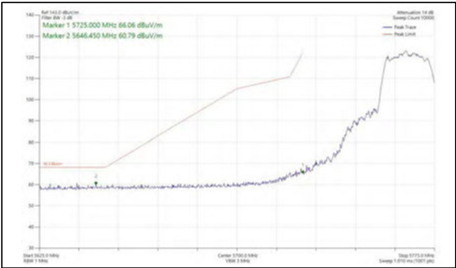
Figure 454 - 802.11n HT20, CDD, Core 0 + Core 1 - 5765 MHz Band Edge Frequency 5725 MHz
