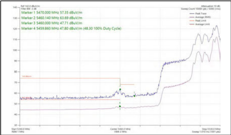
Figure 564 - 802.11ax HE40, RU 52-44, CDD, Core 0 + Core 1 - 5510 MHz Band Edge Frequency 5470 MHz
