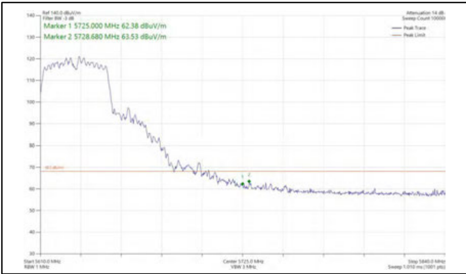
Figure 571 - 802.11n HT40, CDD, Core 0 + Core 1 - 5630 MHz Band Edge Frequency 5725 MHz
