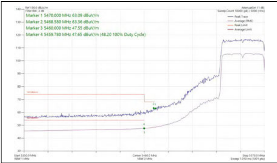
Figure 519 - 802.11ax HE40, SU, SISO, Core 0 - 5550 MHz Band Edge Frequency 5470 MHz
