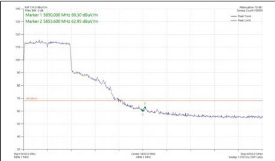
Figure 623 - 802.11ac VHT80, SISO, Core 0 - 5690 MHz Band Edge Frequency 5850 MHz
