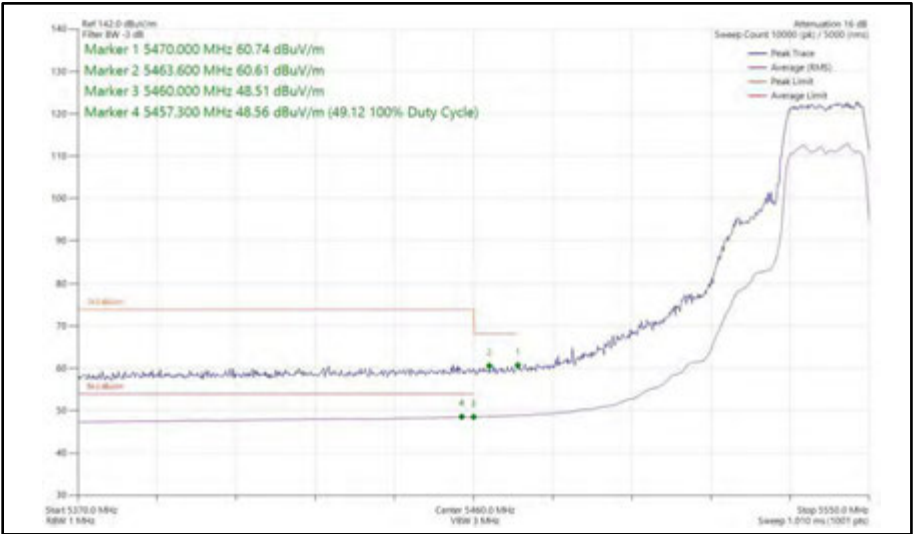
Figure 476 - 802.11n HT20, SDM, Core 0 + Core 1 - 5540 MHz Band Edge Frequency 5470 MHz
