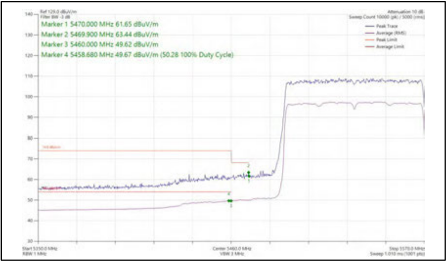
Figure 615 - 802.11ax HE80, SU, SISO, Core 0 - 5530 MHz Band Edge Frequency 5470 MHz
