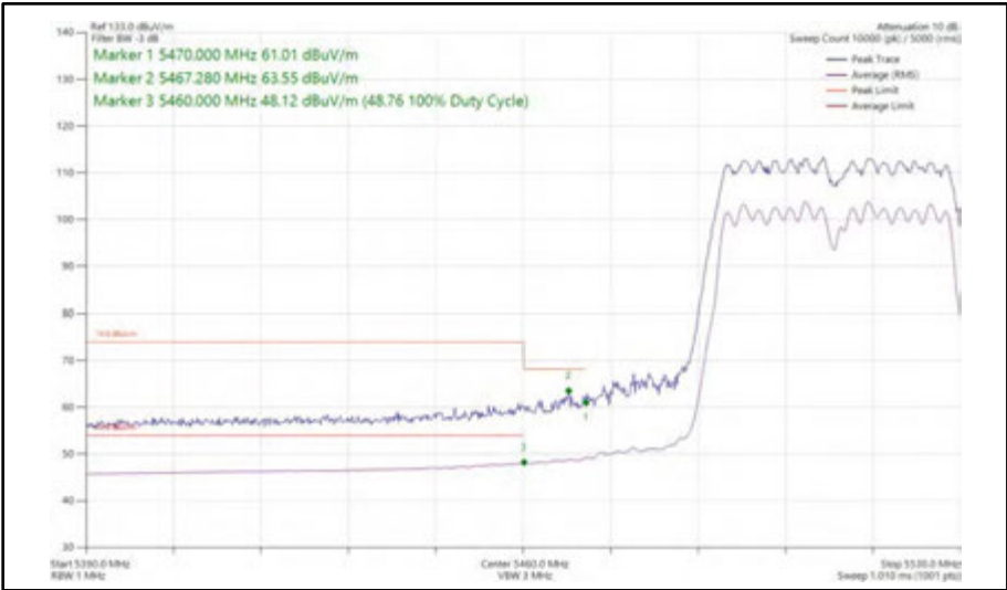
Figure 560 - 802.11n HT40, CDD, Core 0 + Core 1 - 5510 MHz Band Edge Frequency 5470 MHz
