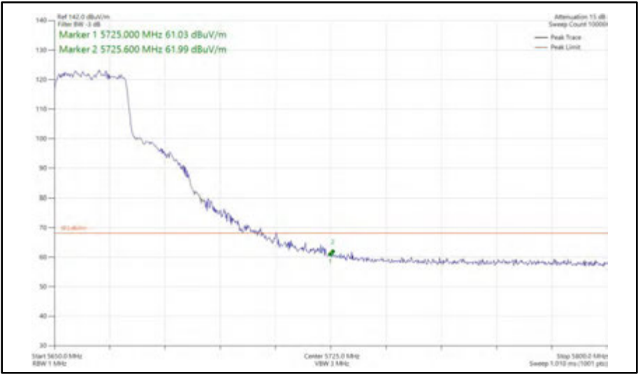
Figure 490 - 802.11ax HE20, SU, SDM, Core 0 + Core 1 - 5660 MHz Band Edge Frequency 5725 MHz
