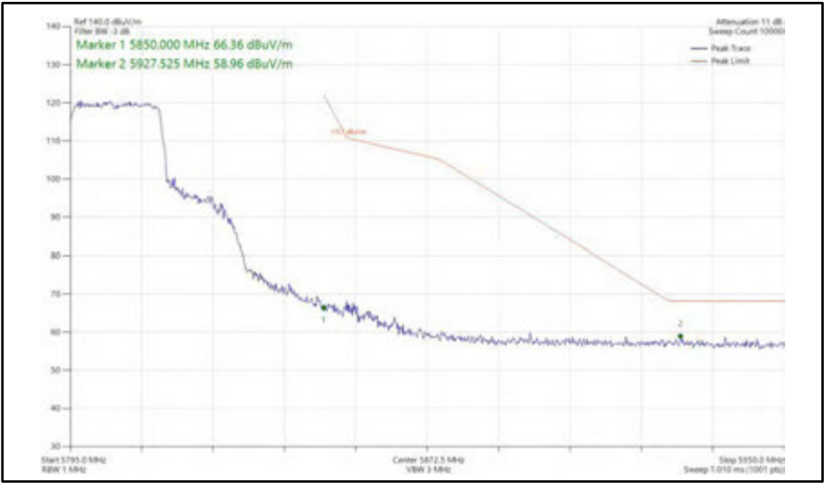
Figure 442 - 802.11ax HE20, SU, SISO, Core 1 - 5805 MHz Band Edge Frequency 5850 MHz
