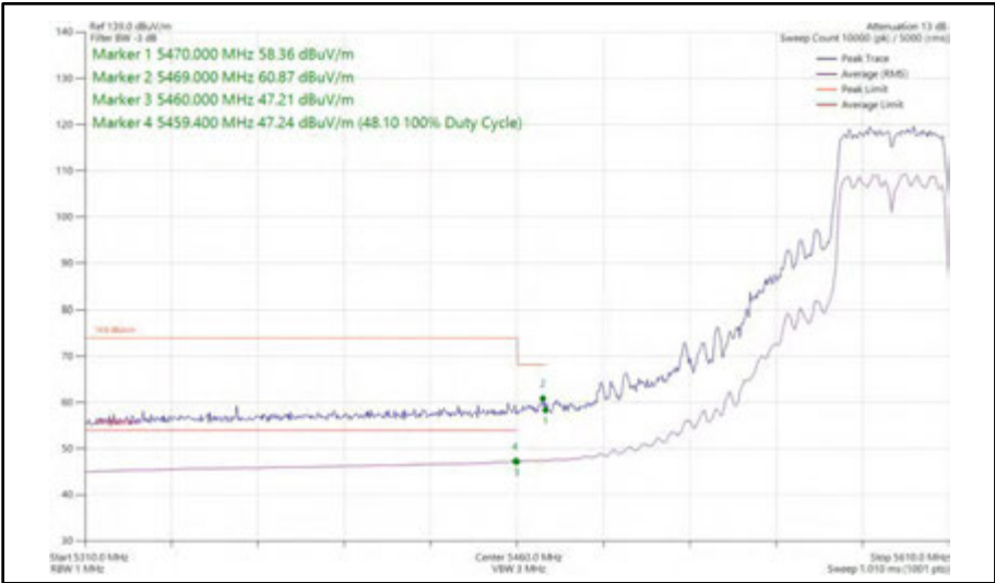
Figure 585 - 802.11n HT40, SDM, Core 0 + Core 1 - 5590 MHz Band Edge Frequency 5470 MHz
