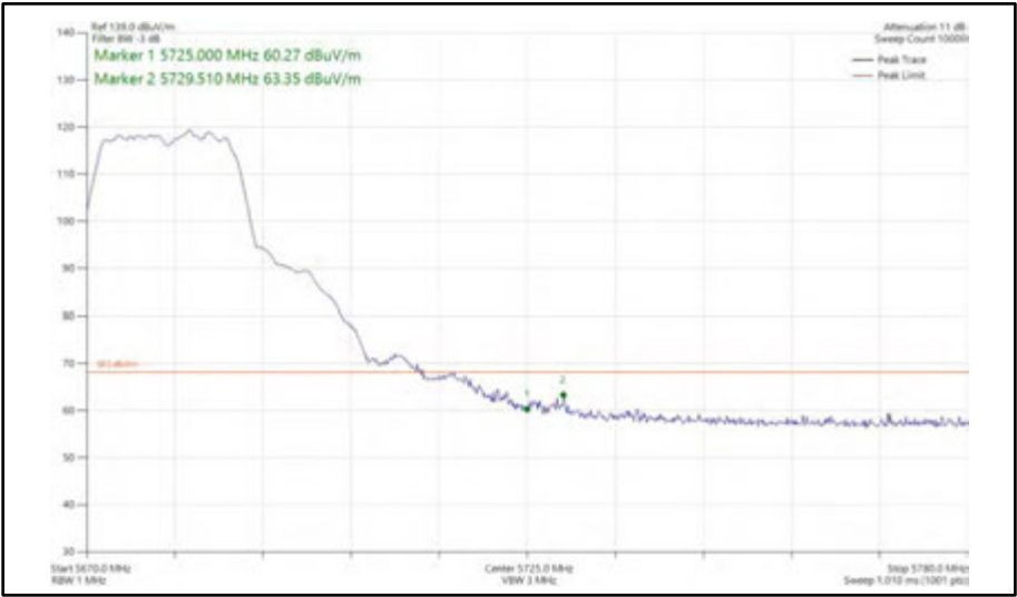
Figure 424 - 802.11a, SISO, Core 1 - 5680 MHz Band Edge Frequency 5725 MHz
