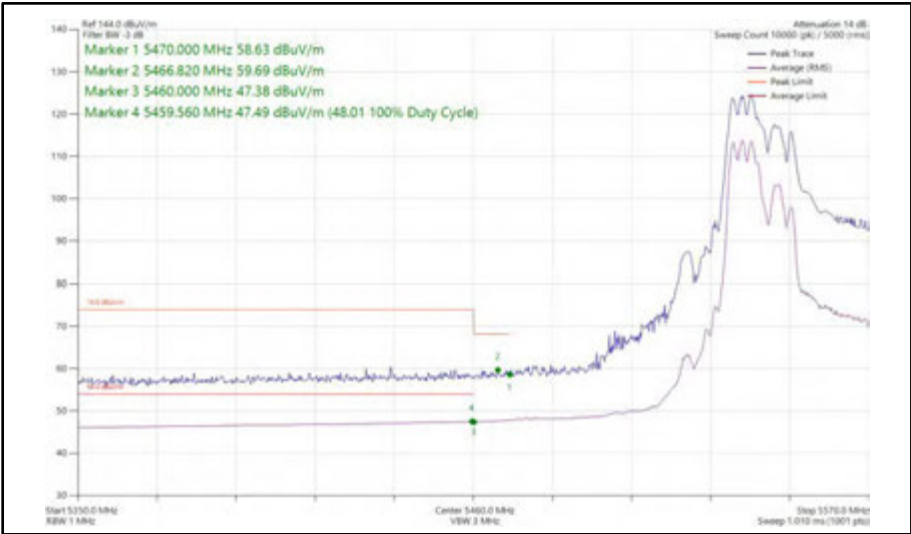
Figure 566 - 802.11ax HE40, RU 106-53, CDD, Core 0 + Core 1 - 5550 MHz Band Edge Frequency 5470 MHz
