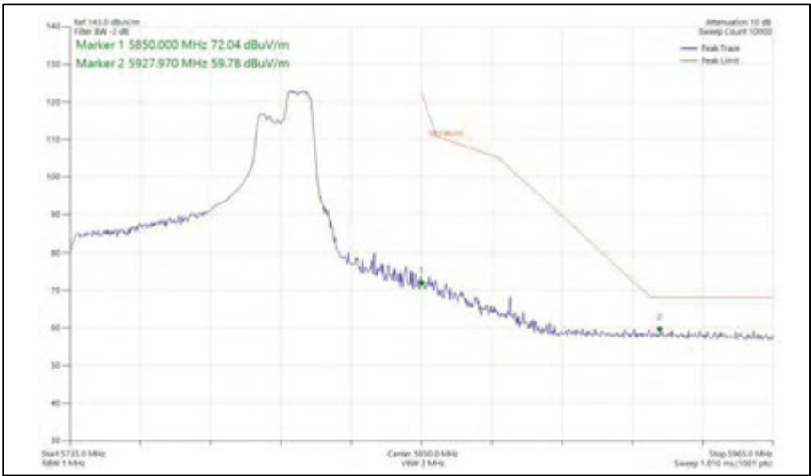
Figure 628 - 802.11ax HE80, RU 106-60, SISO, Core 0 - 5775 MHz Band Edge Frequency 5850 MHz
