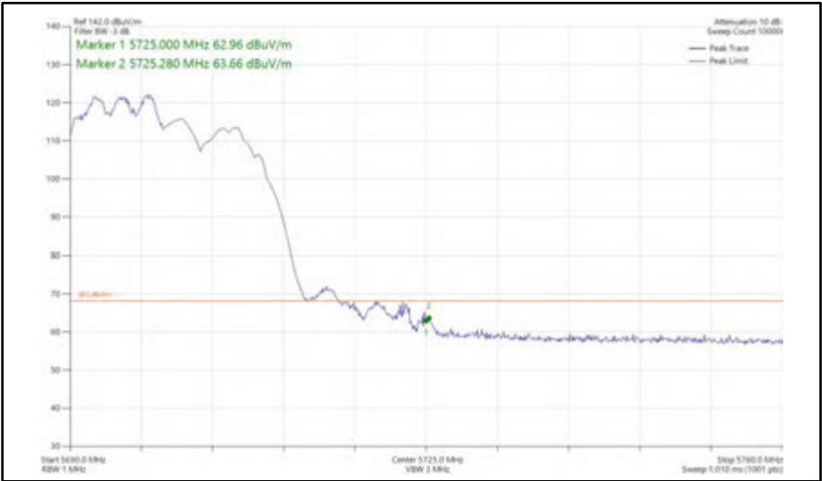
Figure 494 - 802.11ax HE20, RU 106-53, SDM, Core 0 + Core 1 - 5700 MHz Band Edge Frequency 5725 MHz
