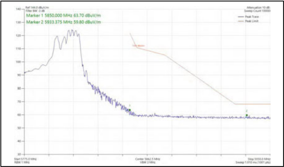
Figure 605 - 802.11ax HE40, RU 106-56, SDM, Core 0 + Core 1 - 5795 MHz Band Edge Frequency 5850 MHz
