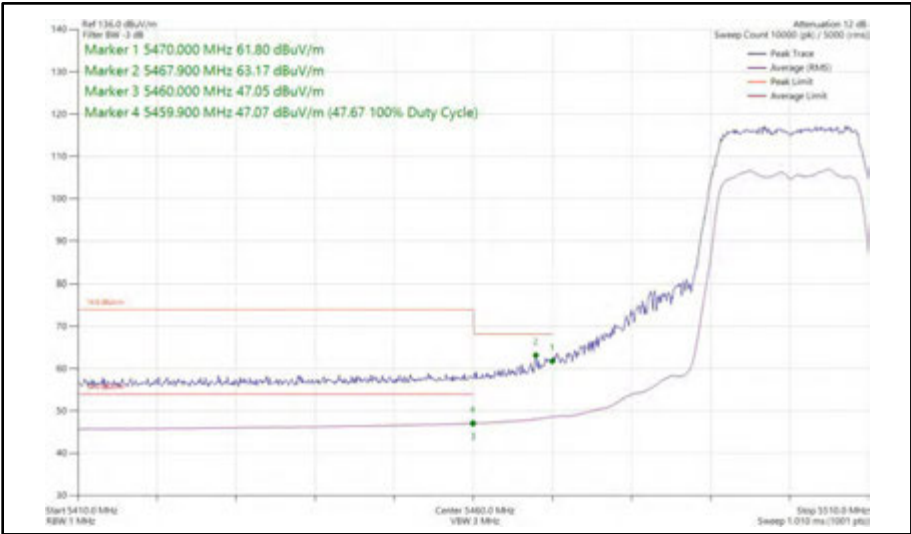
Figure 474 - 802.11n HT20, SDM, Core 0 + Core 1 - 5500 MHz Band Edge Frequency 5470 MHz
