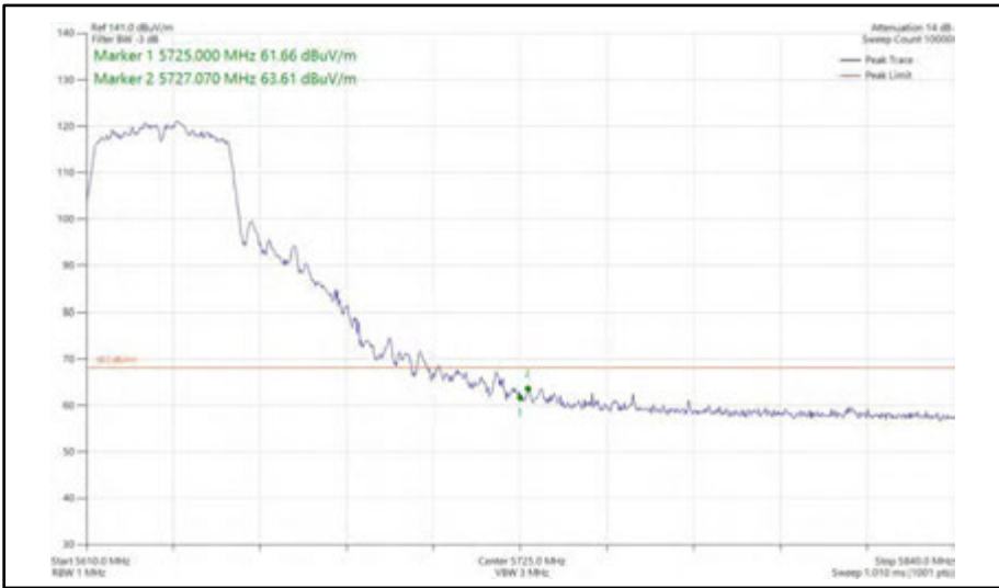
Figure 594 - 802.11n HT40, SDM, Core 0 + Core 1 - 5630 MHz Band Edge Frequency 5725 MHz
