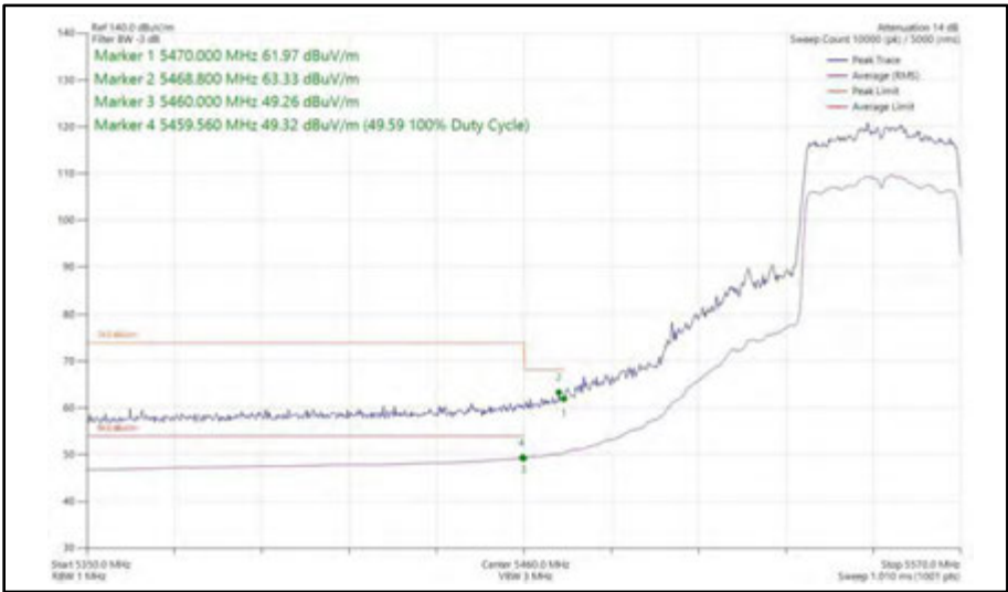
Figure 588 - 802.11ax HE40, SU, SDM, Core 0 + Core 1 - 5550 MHz Band Edge Frequency 5470 MHz
