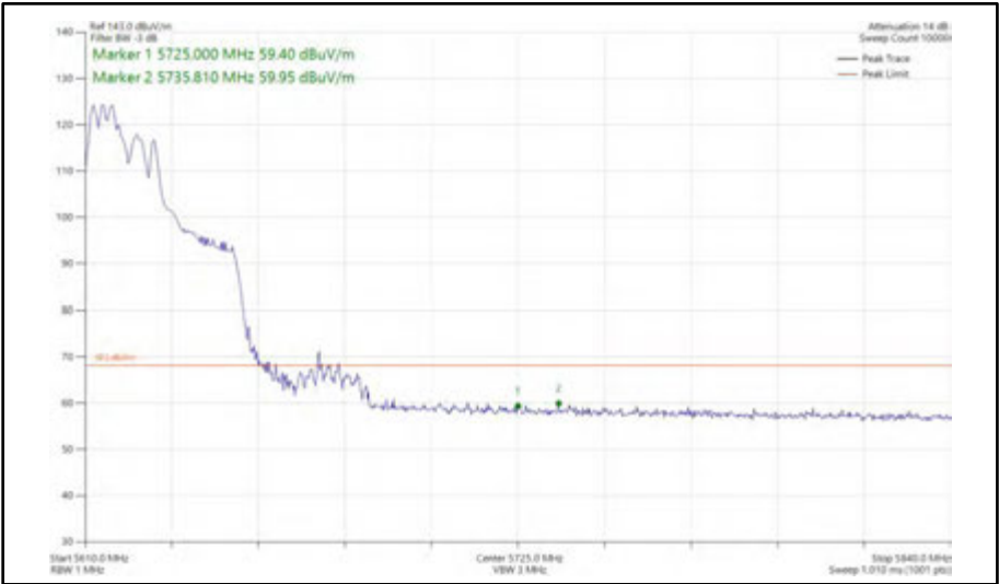
Figure 574 - 802.11ax HE40, RU 106-53, CDD, Core 0 + Core 1 - 5630 MHz Band Edge Frequency 5725 MHz
