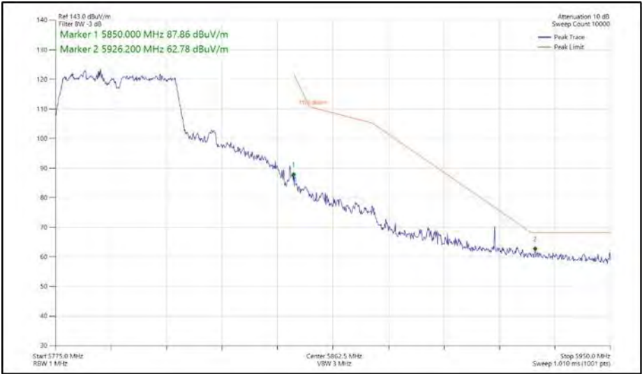
Figure 613 - 802.11ac VHT40, TxBF, Core 0 + Core 1 - 5795 MHz Band Edge Frequency 5850 MHz
