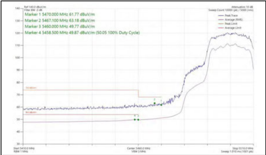
Figure 503 - 802.11ac VHT20, TxBF, Core 0 + Core 1 - 5500 MHz Band Edge Frequency 5470 MHz
