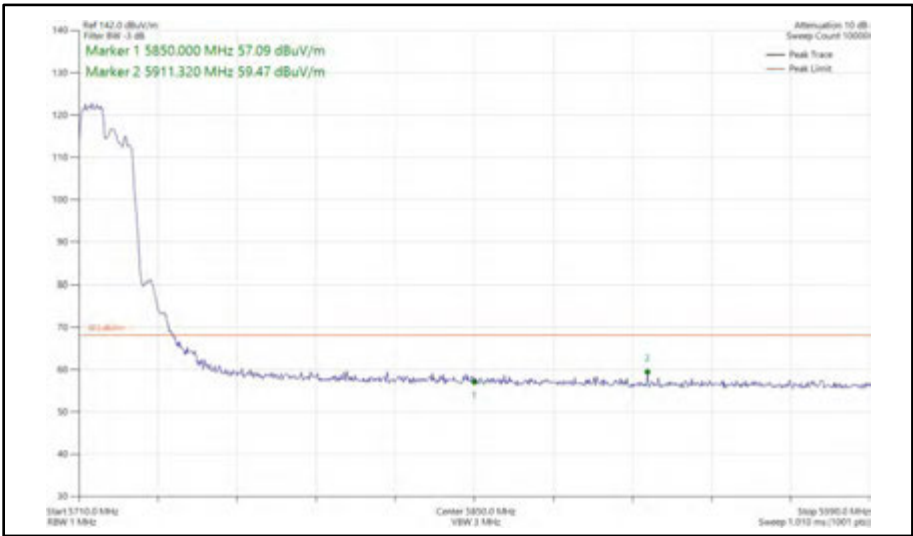
Figure 404 - 802.11ax HE20, RU 106-53, SISO, Core 0 - 5720 MHz Band Edge Frequency 5850 MHz
