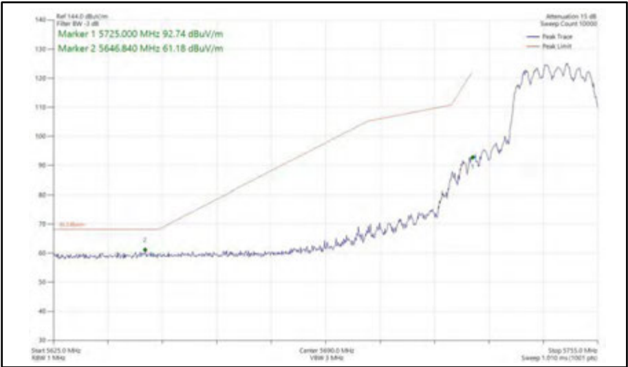
Figure 455 - 802.11ax HE20, SU, CDD, Core 0 + Core 1 - 5745 MHz Band Edge Frequency 5725 MHz
