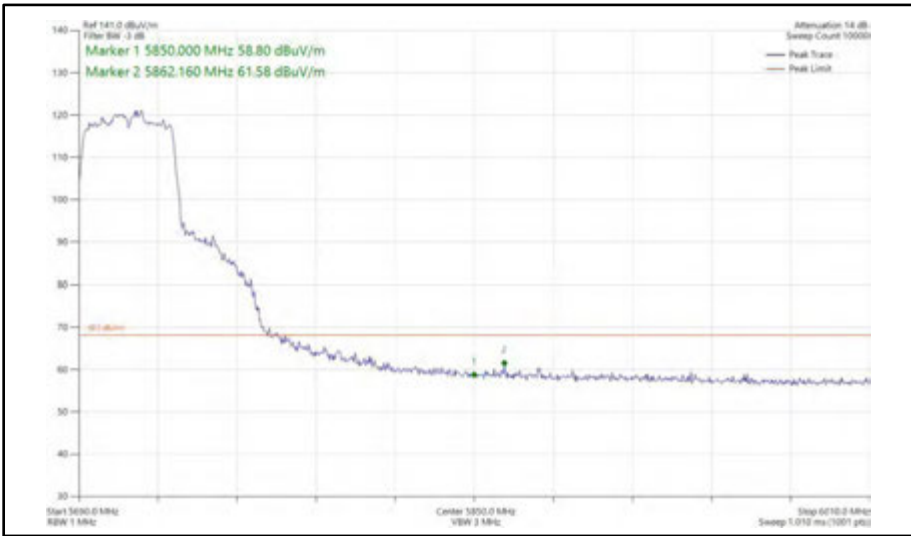
Figure 600 - 802.11n HT40, SDM, Core 0 + Core 1 - 5710 MHz Band Edge Frequency 5850 MHz
