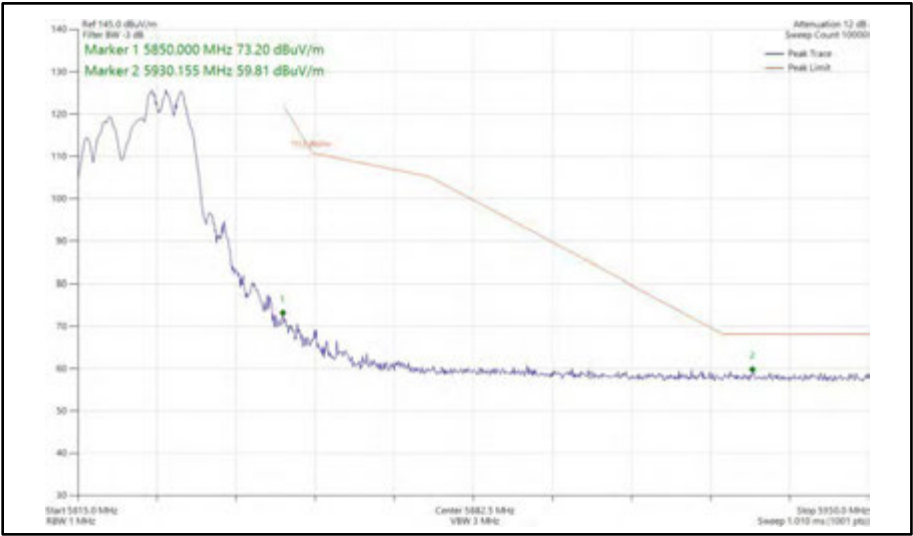
Figure 502 - 802.11ax HE20, RU 106-54, SDM, Core 0 + Core 1 - 5825 MHz Band Edge Frequency 5850 MHz
