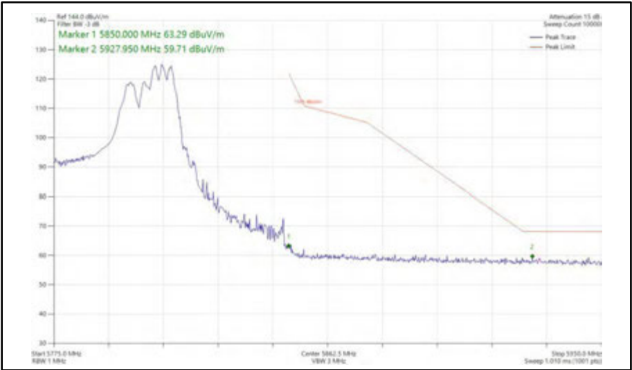
Figure 582 - 802.11ax HE40, RU 106-56, CDD, Core 0 + Core 1 - 5795 MHz Band Edge Frequency 5850 MHz
