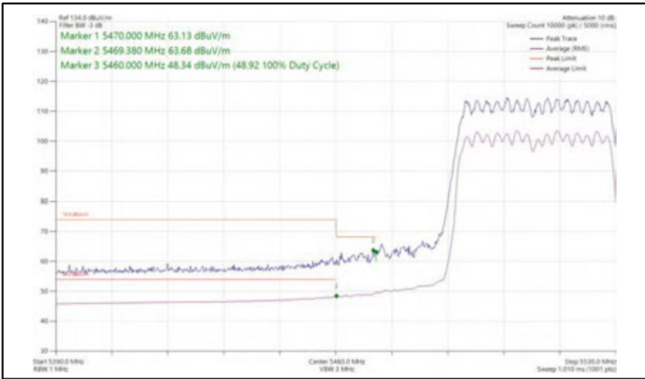
Figure 563 - 802.11ax HE40, SU, CDD, Core 0 + Core 1 - 5510 MHz Band Edge Frequency 5470 MHz
