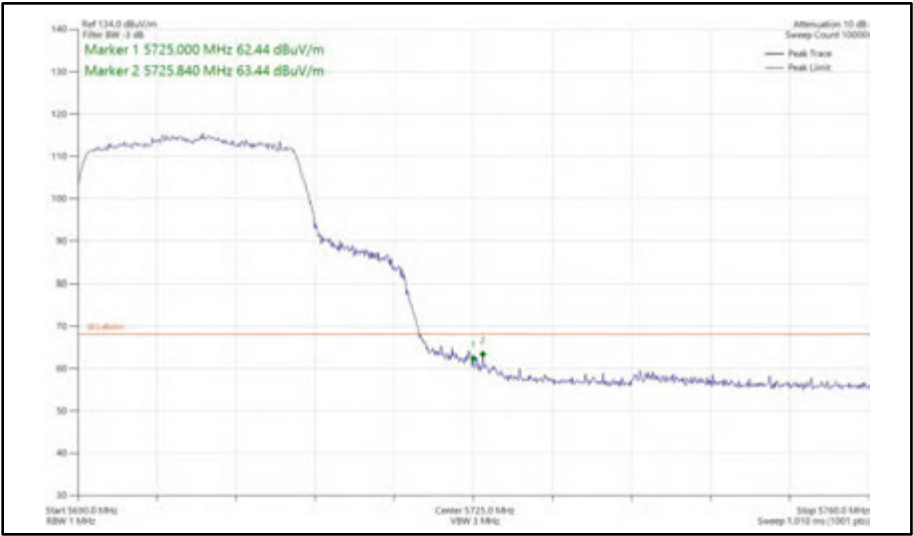
Figure 432 - 802.11ax HE20, SU, SISO, Core 1 - 5700 MHz Band Edge Frequency 5725 MHz
