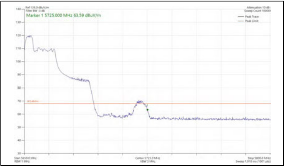
Figure 553 - 802.11ax HE40, RU 52-37, SISO, Core 1 - 5670 MHz Band Edge Frequency 5725 MHz
