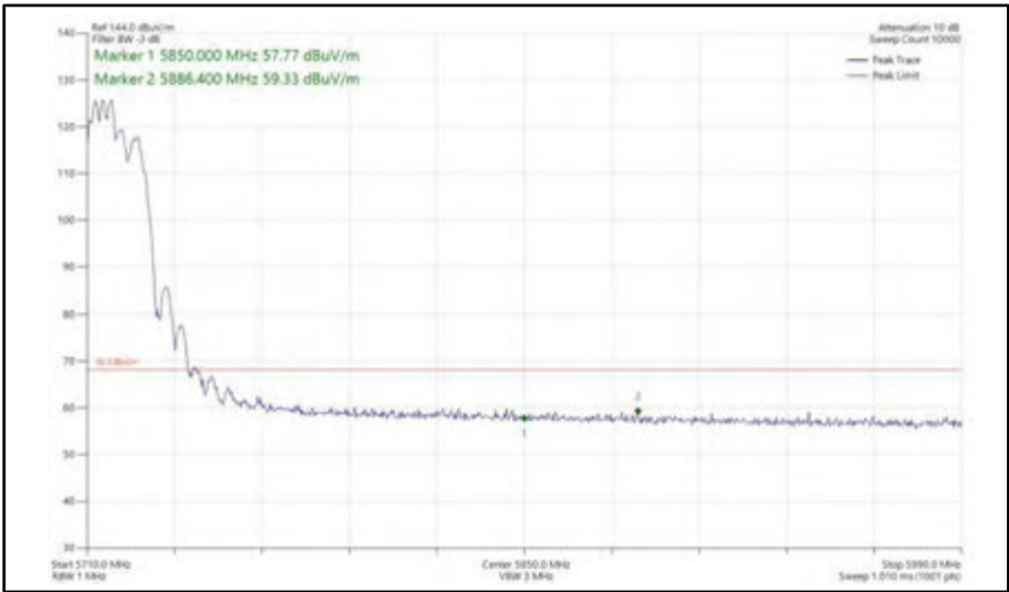
Figure 499 - 802.11ax HE20, RU 106-53, SDM, Core 0 + Core 1 - 5720 MHz Band Edge Frequency 5850 MHz
