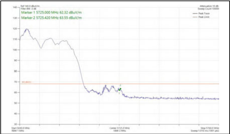
Figure 465 - 802.11ax HE20, RU 52-37, CDD, Core 0 + Core 1 - 5700 MHz Band Edge Frequency 5725 MHz
