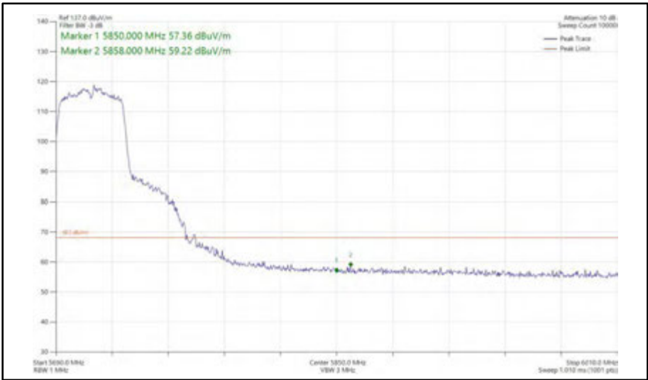
Figure 554 - 802.11n HT40, SISO, Core 1 - 5710 MHz Band Edge Frequency 5850 MHz
