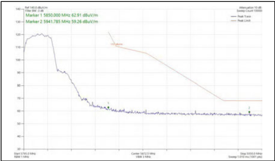
Figure 435 - 802.11a, SISO, Core 1 - 5805 MHz Band Edge Frequency 5850 MHz
