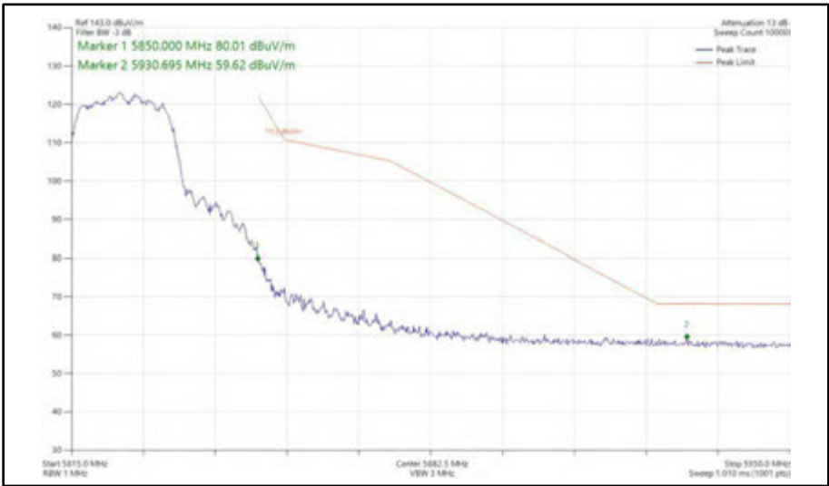
Figure 468 - 802.11n HT20, CDD, Core 0 + Core 1 - 5825 MHz Band Edge Frequency 5850 MHz
