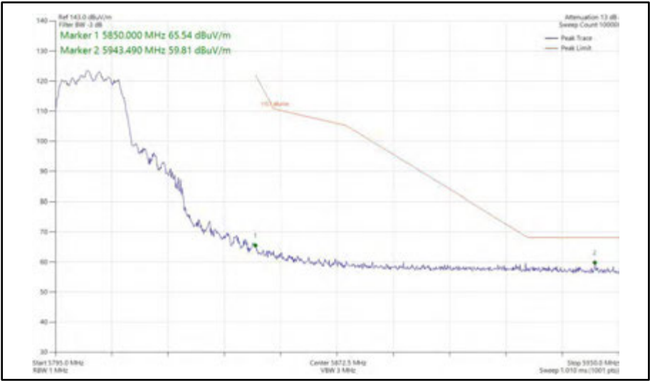
Figure 467 - 802.11n HT20, CDD, Core 0 + Core 1 - 5805 MHz Band Edge Frequency 5850 MHz
