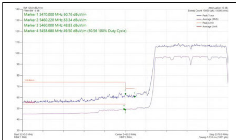
Figure 614 - 802.11ac VHT80, SISO, Core 0 - 5530 MHz Band Edge Frequency 5470 MHz
