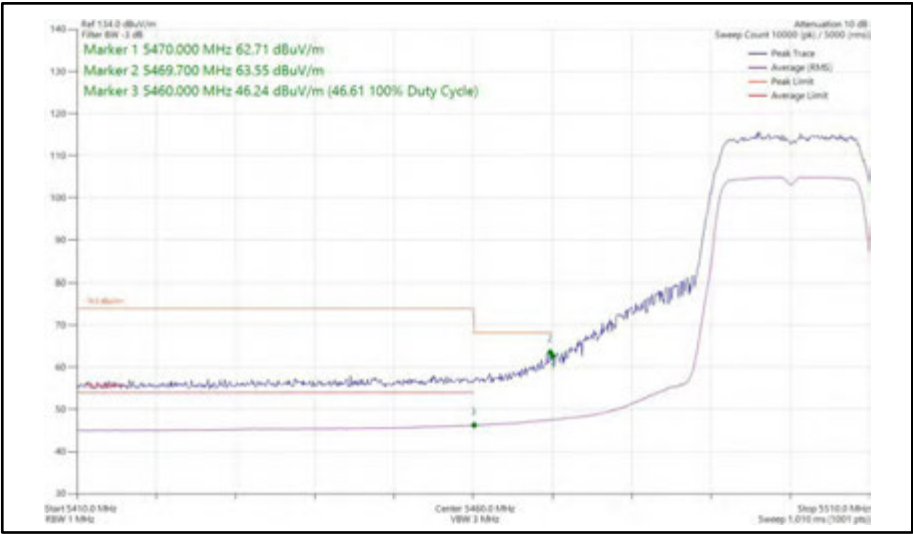
Figure 410 - 802.11n HT20, SISO, Core 1 - 5500 MHz Band Edge Frequency 5470 MHz
