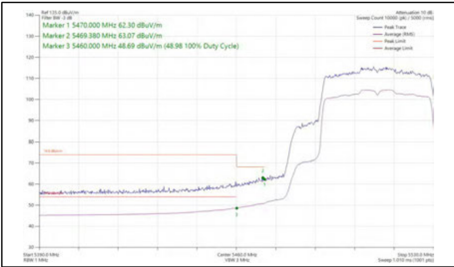
Figure 540 - 802.11ax HE40, SU, SISO, Core 1 - 5510 MHz Band Edge Frequency 5470 MHz
