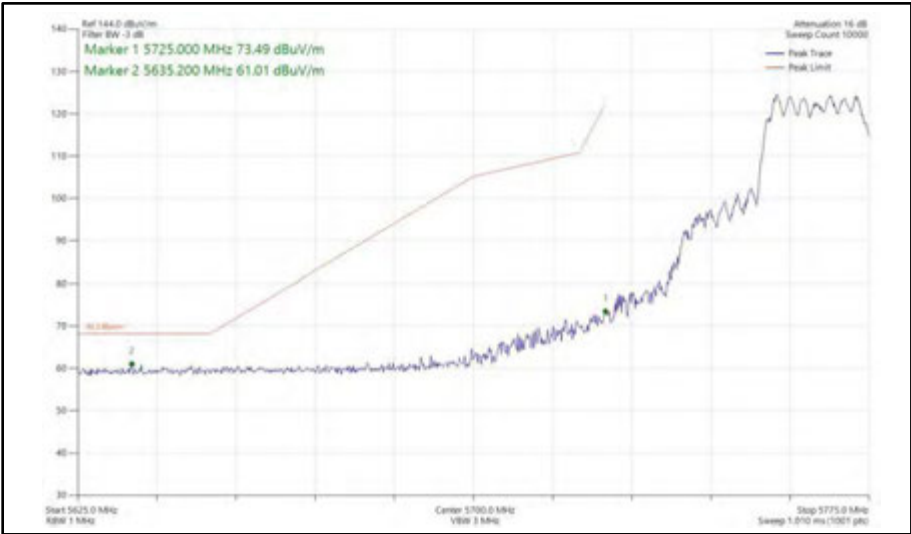
Figure 457 - 802.11ax HE20, SU, CDD, Core 0 + Core 1 - 5765 MHz Band Edge Frequency 5725 MHz
