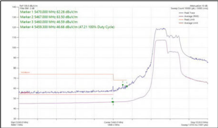
Figure 541 - 802.11ax HE40, RU 106-53, SISO, Core 1 - 5510 MHz Band Edge Frequency 5470 MHz
