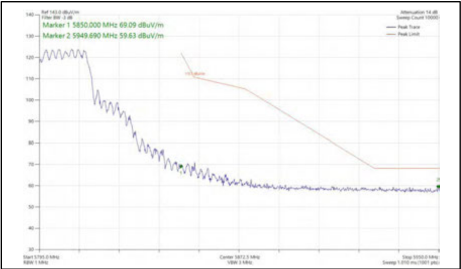
Figure 471 - 802.11ax HE20, SU, CDD, Core 0 + Core 1 - 5805 MHz Band Edge Frequency 5850 MHz
