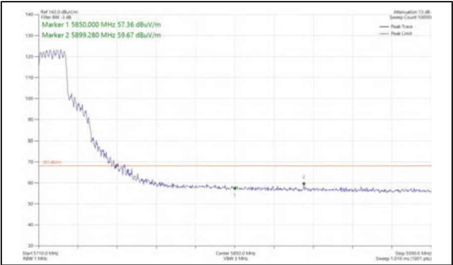
Figure 469 - 802.11ax HE20, SU, CDD, Core 0 + Core 1 - 5720 MHz Band Edge Frequency 5850 MHz
