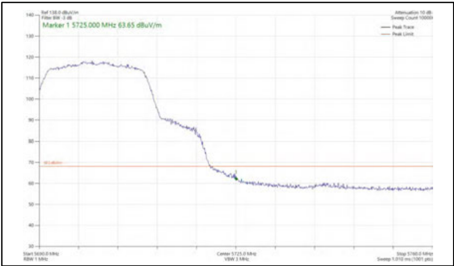
Figure 489 - 802.11n HT20, SDM, Core 0 + Core 1 - 5700 MHz Band Edge Frequency 5725 MHz
