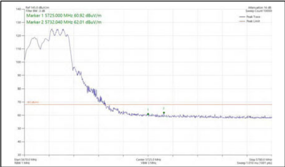
Figure 492 - 802.11ax HE20, RU 106-54, SDM, Core 0 + Core 1 - 5680 MHz Band Edge Frequency 5725 MHz
