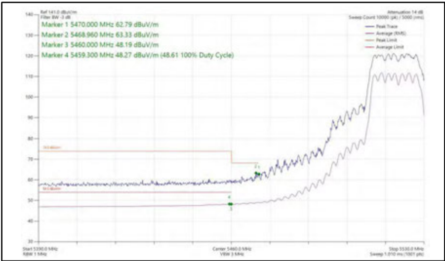
Figure 446 - 802.11n HT20, CDD, Core 0 + Core 1 - 5520 MHz Band Edge Frequency 5470 MHz
