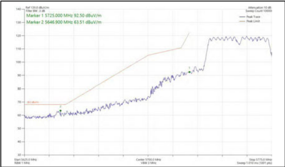
Figure 568 - 802.11n HT40, CDD, Core 0 + Core 1 - 5755 MHz Band Edge Frequency 5725 MHz
