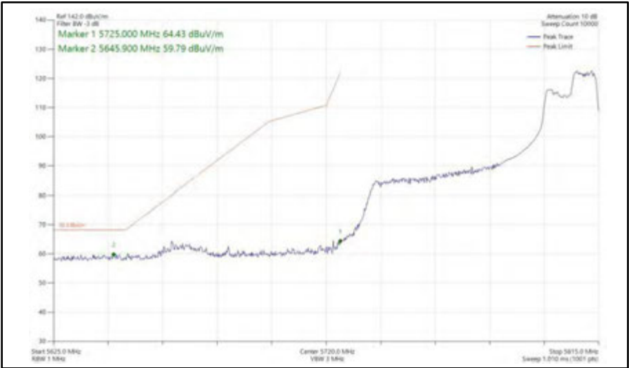
Figure 619 - 802.11ax HE80, RU 106-60, SISO, Core 0 - 5775 MHz Band Edge Frequency 5725 MHz
