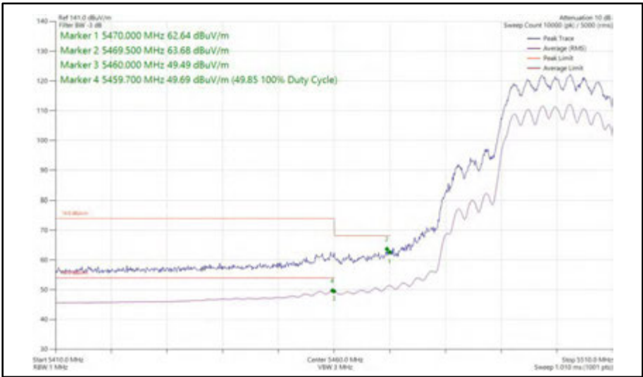
Figure 448 - 802.11ax HE20, SU, CDD, Core 0 + Core 1 - 5500 MHz Band Edge Frequency 5470 MHz
