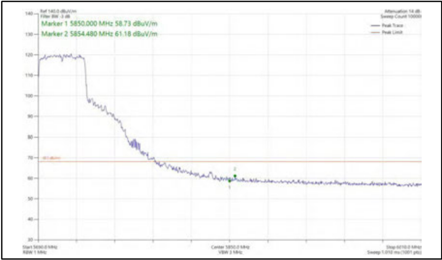
Figure 602 - 802.11ax HE40, SU, SDM, Core 0 + Core 1 - 5710 MHz Band Edge Frequency 5850 MHz
