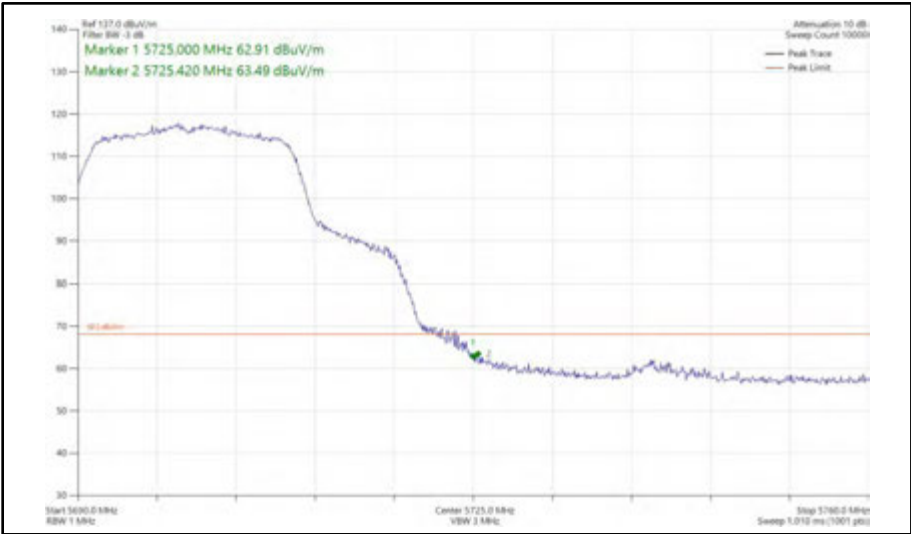
Figure 428 - 802.11n HT20, SISO, Core 1 - 5700 MHz Band Edge Frequency 5725 MHz
