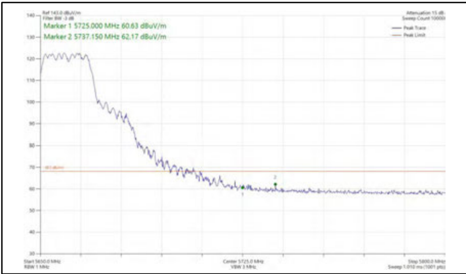
Figure 458 - 802.11n HT20, CDD, Core 0 + Core 1 - 5660 MHz Band Edge Frequency 5725 MHz
