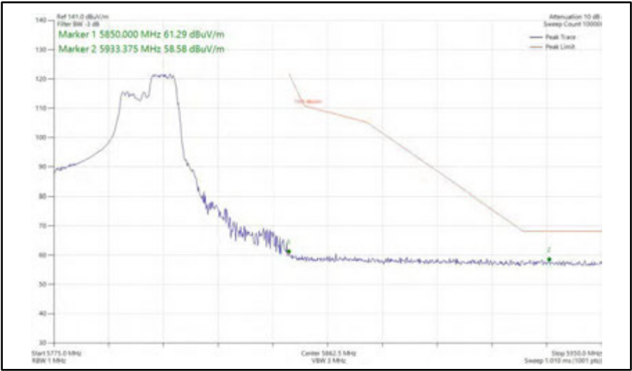
Figure 559 - 802.11ax HE40, RU 106-56, SISO, Core 1 - 5795 MHz Band Edge Frequency 5850 MHz
