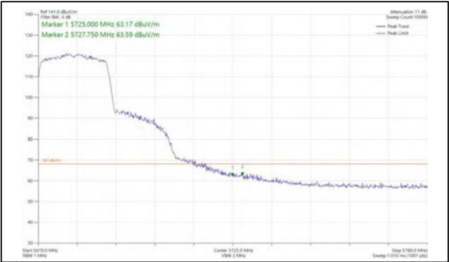
Figure 393 - 802.11ax HE20, SU, SISO, Core 0 - 5680 MHz Band Edge Frequency 5725 MHz
