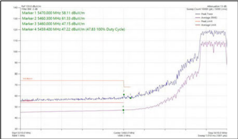
Figure 562 - 802.11n HT40, CDD, Core 0 + Core 1 - 5590 MHz Band Edge Frequency 5470 MHz
