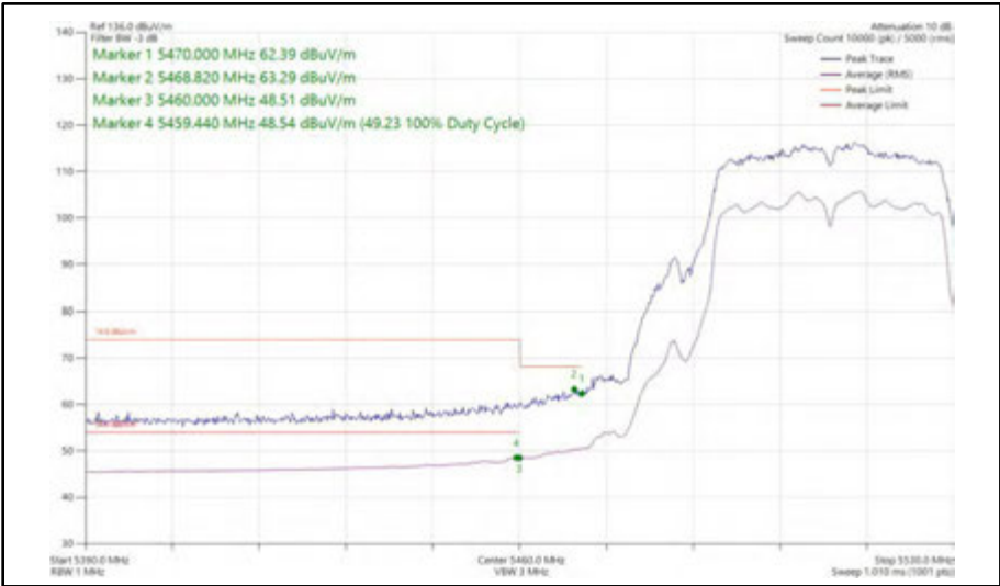
Figure 583 - 802.11n HT40, SDM, Core 0 + Core 1 - 5510 MHz Band Edge Frequency 5470 MHz
