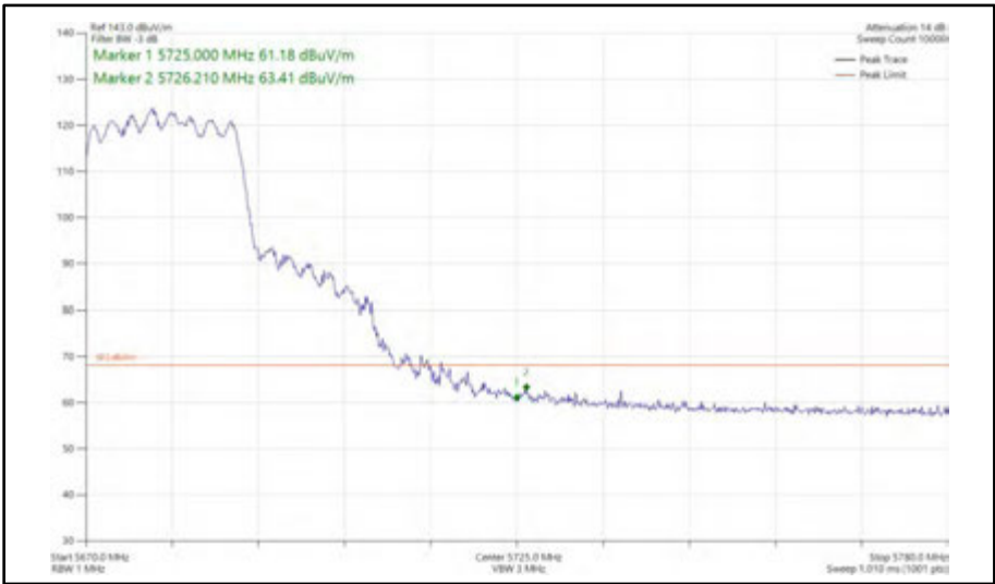
Figure 462 - 802.11ax HE20, SU, CDD, Core 0 + Core 1 - 5680 MHz Band Edge Frequency 5725 MHz
