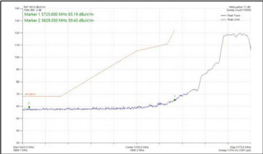
Figure 418 - 802.11a, SISO, Core 1 - 5765 MHz Band Edge Frequency 5725 MHz
