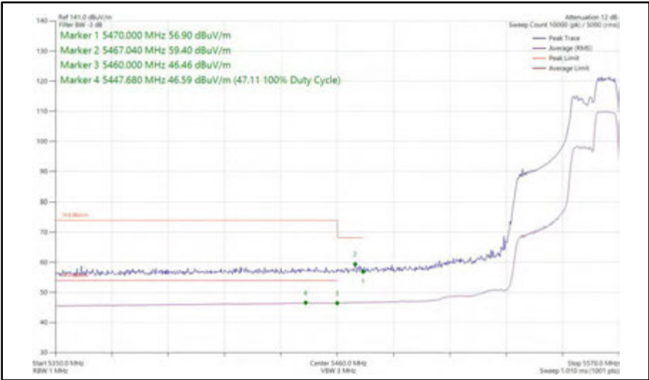
Figure 520 - 802.11ax HE40, RU 106-56, SISO, Core 0 - 5550 MHz Band Edge Frequency 5470 MHz
