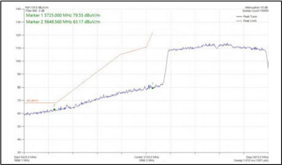
Figure 632 - 802.11ac VHT80, SISO, Core 1 - 5775 MHz Band Edge Frequency 5725 MHz
