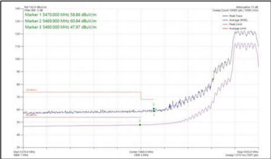
Figure 447 - 802.11n HT20, CDD, Core 0 + Core 1 - 5540 MHz Band Edge Frequency 5470 MHz
