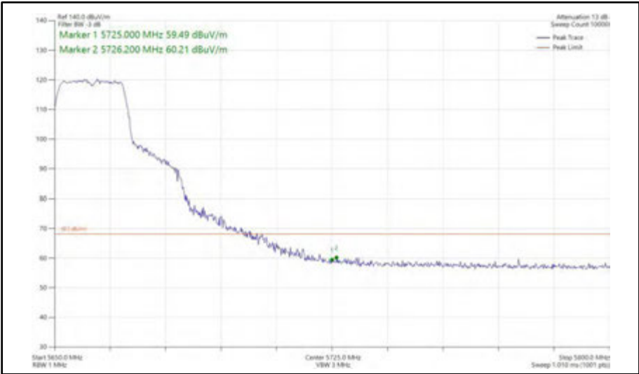
Figure 426 - 802.11n HT20, SISO, Core 1 - 5660 MHz Band Edge Frequency 5725 MHz
