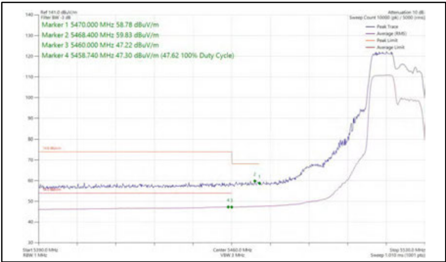
Figure 415 - 802.11ax HE20, RU 106-53, SISO, Core 1 - 5520 MHz Band Edge Frequency 5470 MHz
