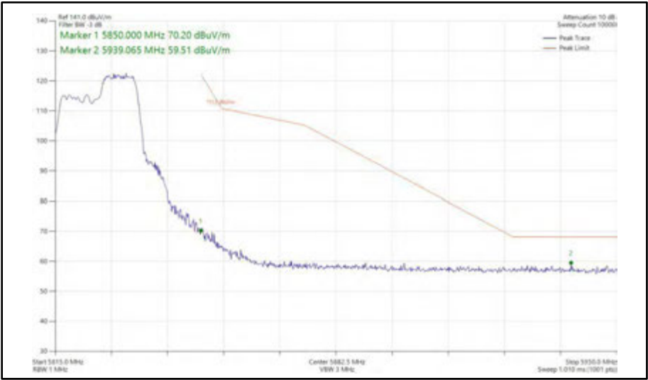
Figure 407 - 802.11ax HE20, RU 106-54, SISO, Core 0 - 5825 MHz Band Edge Frequency 5850 MHz
