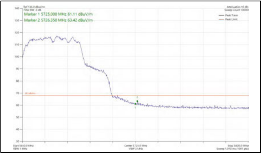
Figure 611 - 802.11ac VHT40, TxBF, Core 0 + Core 1 - 5670 MHz Band Edge Frequency 5725 MHz
