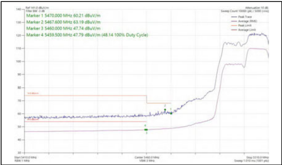
Figure 413 - 802.11ax HE20, RU 106-54, SISO, Core 1 - 5500 MHz Band Edge Frequency 5470 MHz
