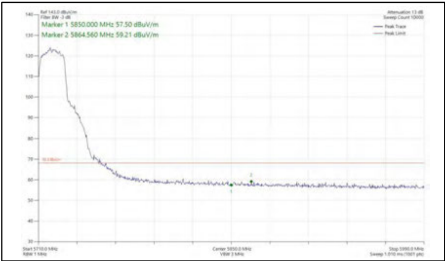
Figure 495 - 802.11n HT20, SDM, Core 0 + Core 1 - 5720 MHz Band Edge Frequency 5850 MHz
