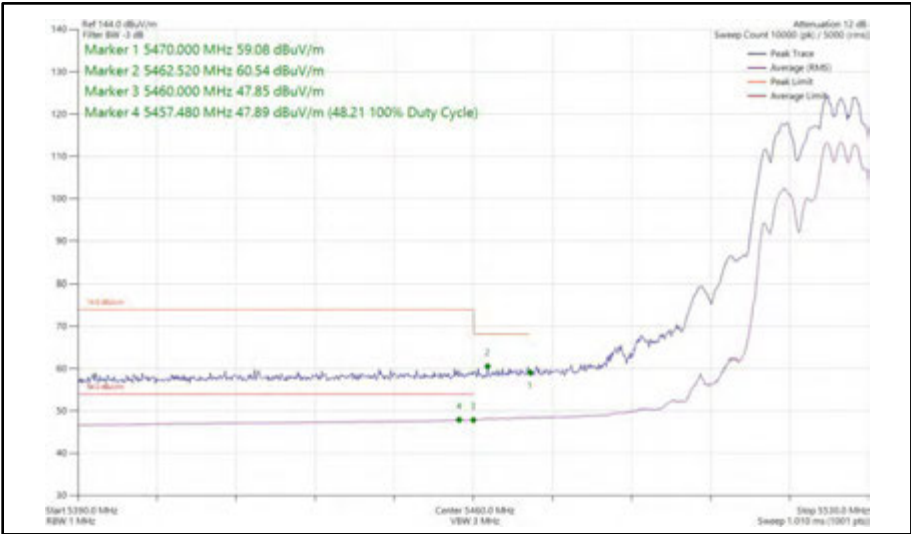
Figure 451 - 802.11ax HE20, RU 106-54, CDD, Core 0 + Core 1 - 5520 MHz Band Edge Frequency 5470 MHz
