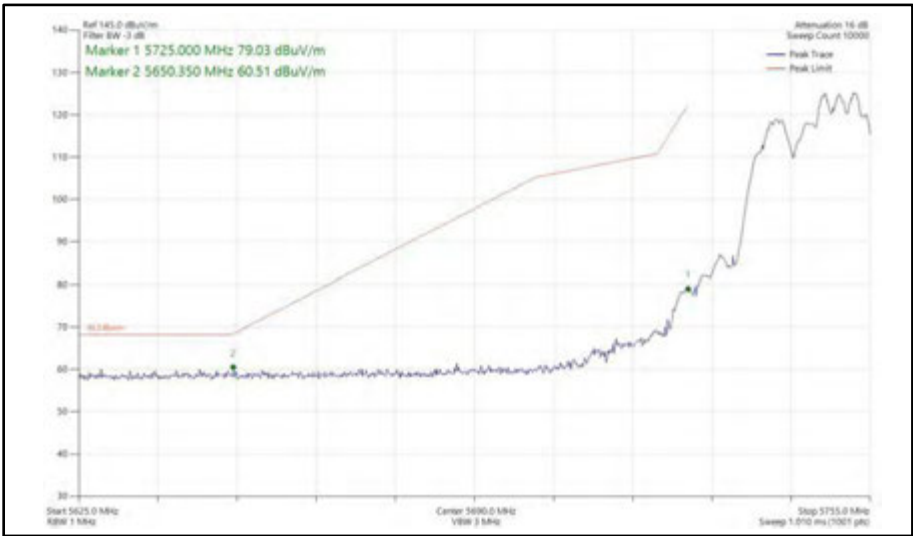
Figure 485 - 802.11ax HE20, RU 106-54, SDM, Core 0 + Core 1 - 5745 MHz Band Edge Frequency 5725 MHz
