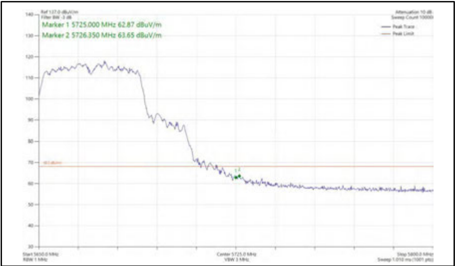
Figure 572 - 802.11n HT40, CDD, Core 0 + Core 1 - 5670 MHz Band Edge Frequency 5725 MHz
