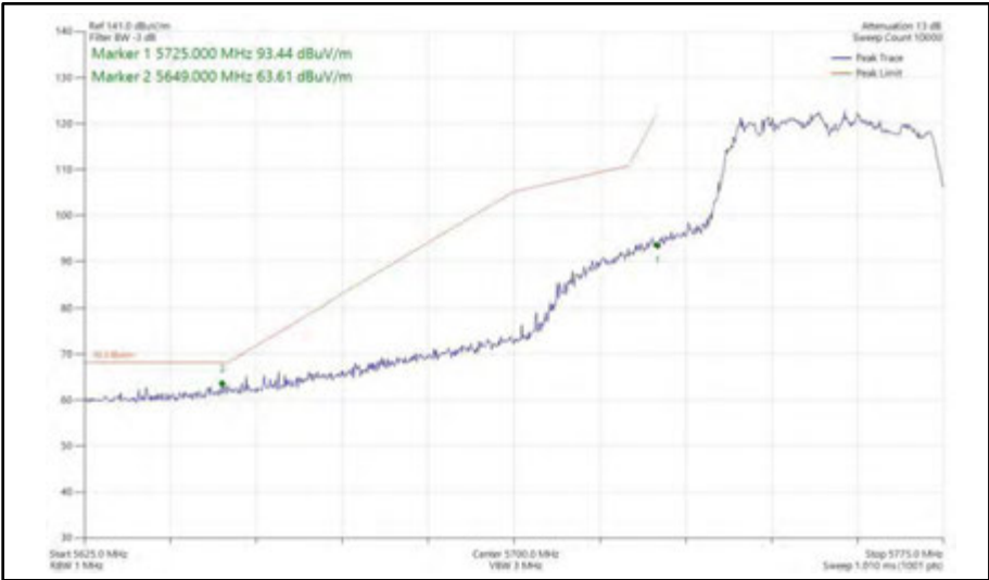
Figure 609 - 802.11ac VHT40, TxBF, Core 0 + Core 1 - 5755 MHz Band Edge Frequency 5725 MHz
