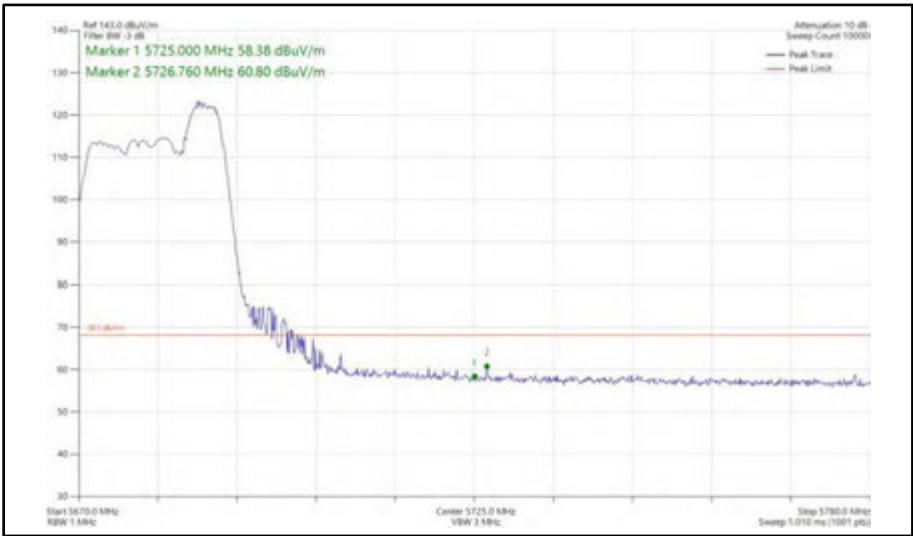
Figure 394 - 802.11ax HE20, RU 52-40, SISO, Core 0 - 5680 MHz Band Edge Frequency 5725 MHz
