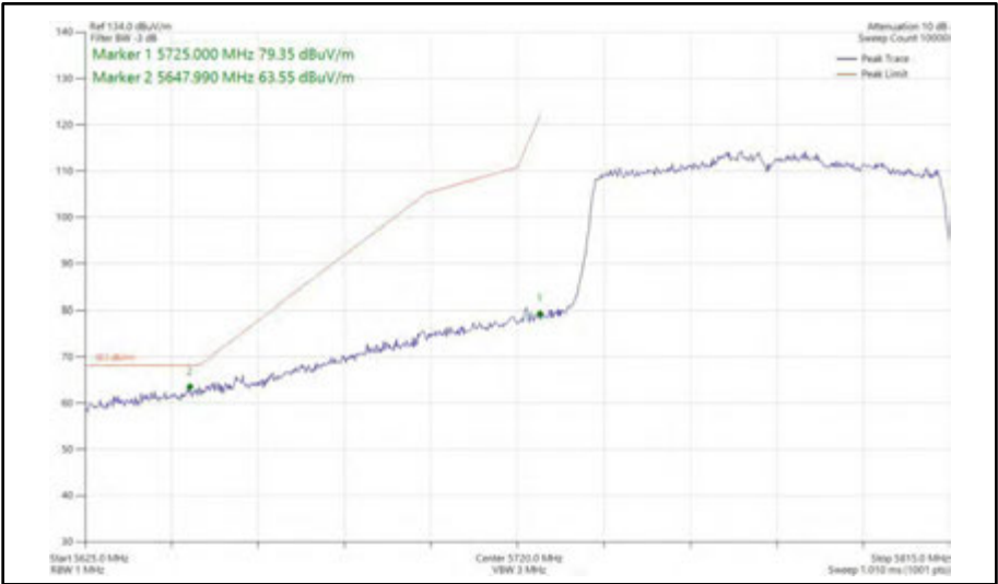
Figure 617 - 802.11ac VHT80, SISO, Core 0 - 5775 MHz Band Edge Frequency 5725 MHz
