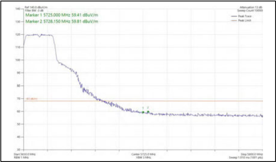
Figure 389 - 802.11n HT20, SISO, Core 0 - 5660 MHz Band Edge Frequency 5725 MHz
