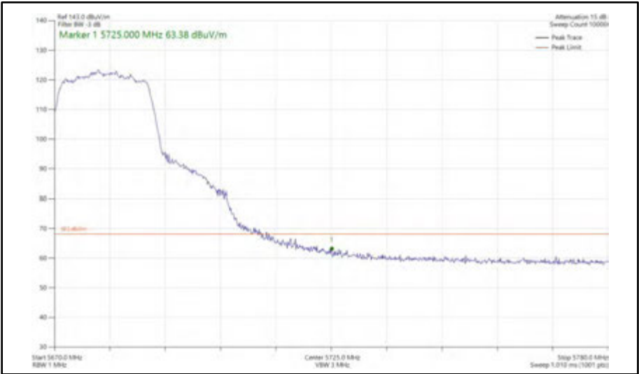
Figure 488 - 802.11n HT20, SDM, Core 0 + Core 1 - 5680 MHz Band Edge Frequency 5725 MHz
