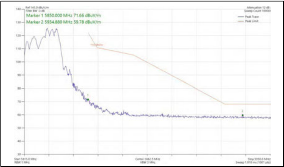
Figure 473 - 802.11ax HE20, RU 106-54, CDD, Core 0 + Core 1 - 5825 MHz Band Edge Frequency 5850 MHz
