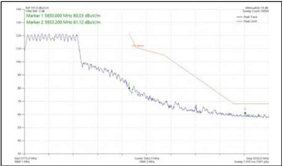
Figure 581 - 802.11ax HE40, SU, CDD, Core 0 + Core 1 - 5795 MHz Band Edge Frequency 5850 MHz
