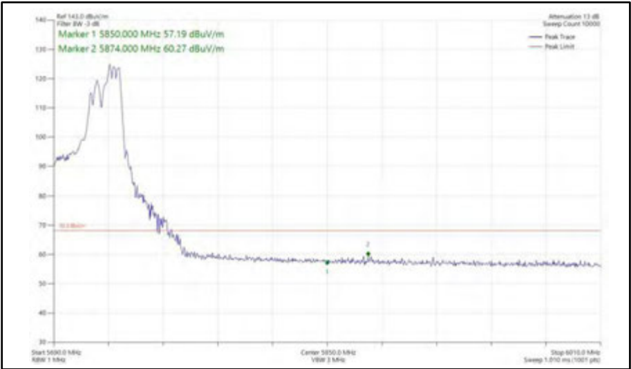
Figure 580 - 802.11ax HE40, RU 106-56, CDD, Core 0 + Core 1 - 5710 MHz Band Edge Frequency 5850 MHz
