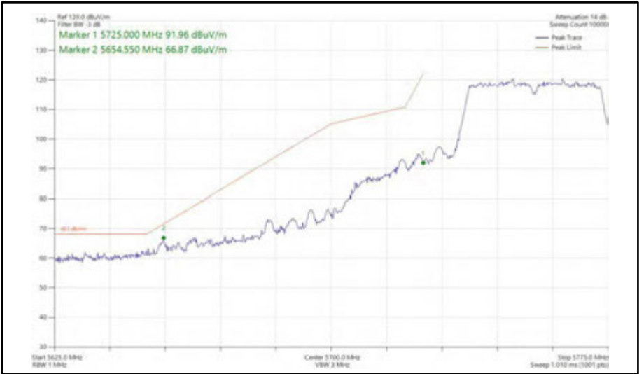
Figure 591 - 802.11n HT40, SDM, Core 0 + Core 1 - 5755 MHz Band Edge Frequency 5725 MHz
