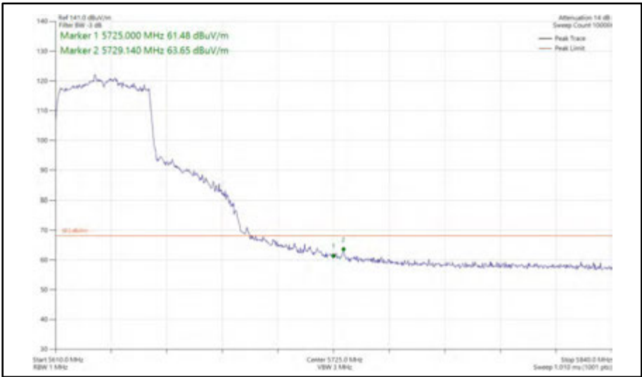
Figure 596 - 802.11ax HE40, SU, SDM, Core 0 + Core 1 - 5630 MHz Band Edge Frequency 5725 MHz
