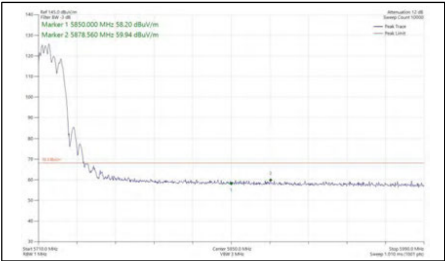
Figure 470 - 802.11ax HE20, RU 106-53, CDD, Core 0 + Core 1 - 5720 MHz Band Edge Frequency 5850 MHz
