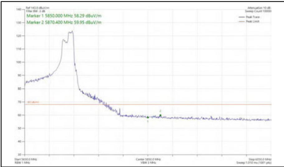
Figure 626 - 802.11ax HE80, RU 106-60, SISO, Core 0 - 5690 MHz Band Edge Frequency 5850 MHz
