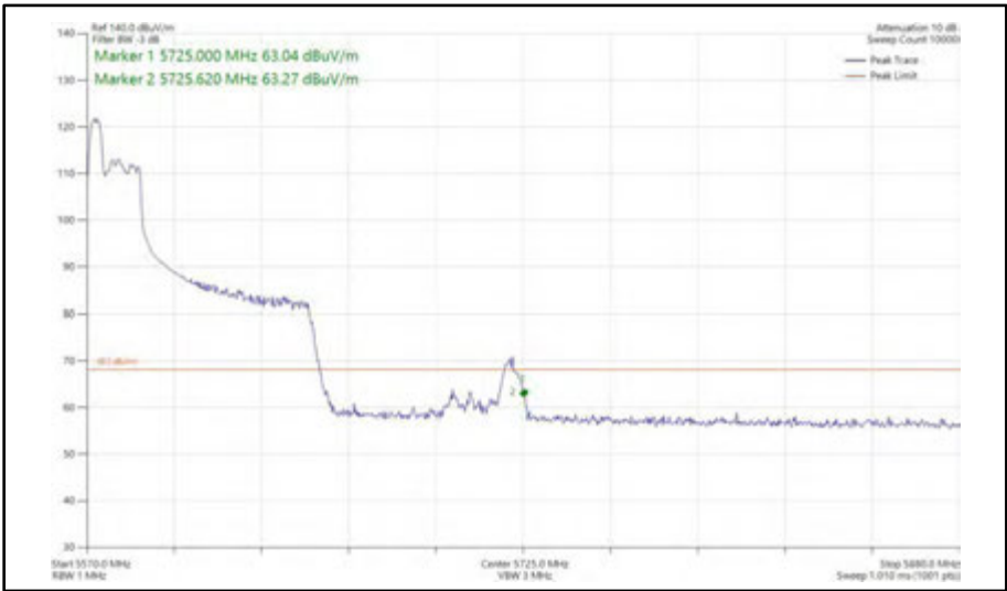
Figure 622 - 802.11ax HE80, RU 52-37, SISO, Core 0 - 5610 MHz Band Edge Frequency 5725 MHz
