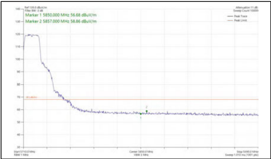
Figure 437 - 802.11n HT20, SISO, Core 1 - 5720 MHz Band Edge Frequency 5850 MHz
