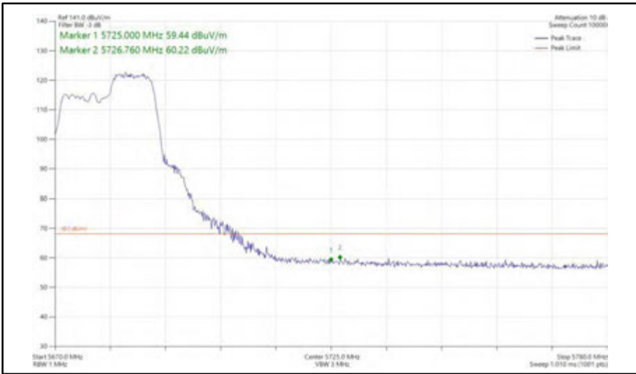
Figure 431 - 802.11ax HE20, RU 106-54, SISO, Core 1 - 5680 MHz Band Edge Frequency 5725 MHz
