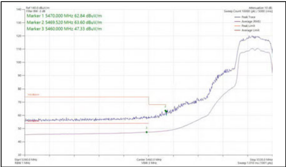
Figure 411 - 802.11n HT20, SISO, Core 1 - 5520 MHz Band Edge Frequency 5470 MHz
