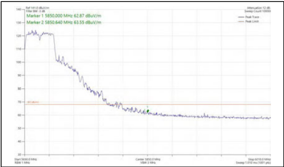
Figure 612 - 802.11ac VHT40, TxBF, Core 0 + Core 1 - 5710 MHz Band Edge Frequency 5850 MHz
