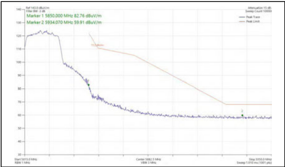
Figure 497 - 802.11n HT20, SDM, Core 0 + Core 1 - 5825 MHz Band Edge Frequency 5850 MHz
