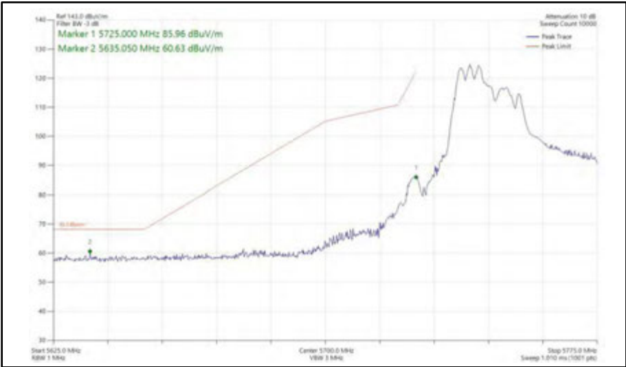
Figure 570 - 802.11ax HE40, RU 106-53, CDD, Core 0 + Core 1 - 5755 MHz Band Edge Frequency 5725 MHz
