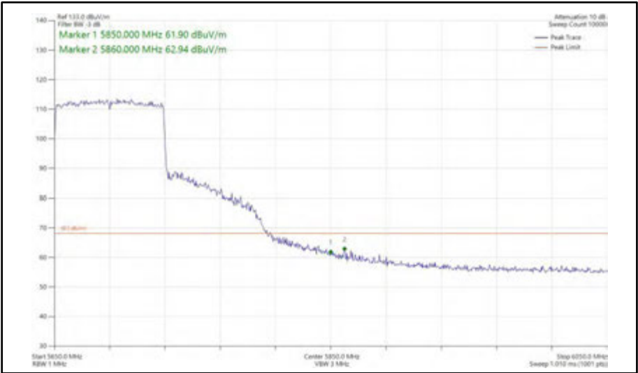
Figure 640 - 802.11ax HE80, SU, SISO, Core 1 - 5690 MHz Band Edge Frequency 5850 MHz
