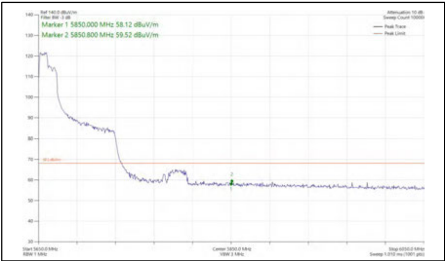
Figure 641 - 802.11ax HE80, RU 106-53, SISO, Core 1 - 5690 MHz Band Edge Frequency 5850 MHz
