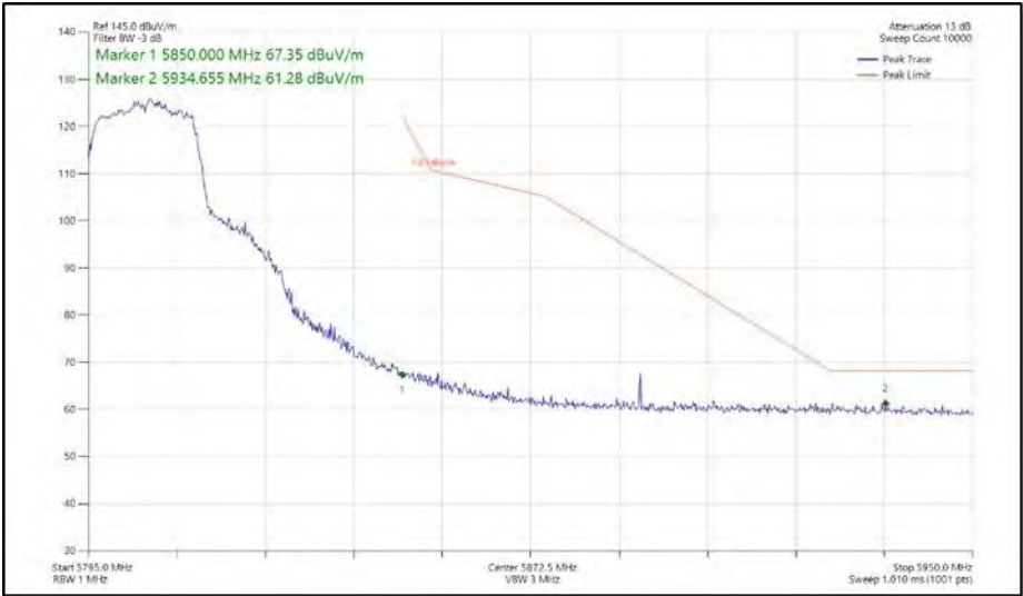
Figure 512 - 802.11ac VHT20, TxBF, Core 0 + Core 1 - 5805 MHz Band Edge Frequency 5850 MHz
