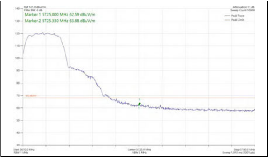
Figure 387 - 802.11a, SISO, Core 0 - 5680 MHz Band Edge Frequency 5725 MHz
