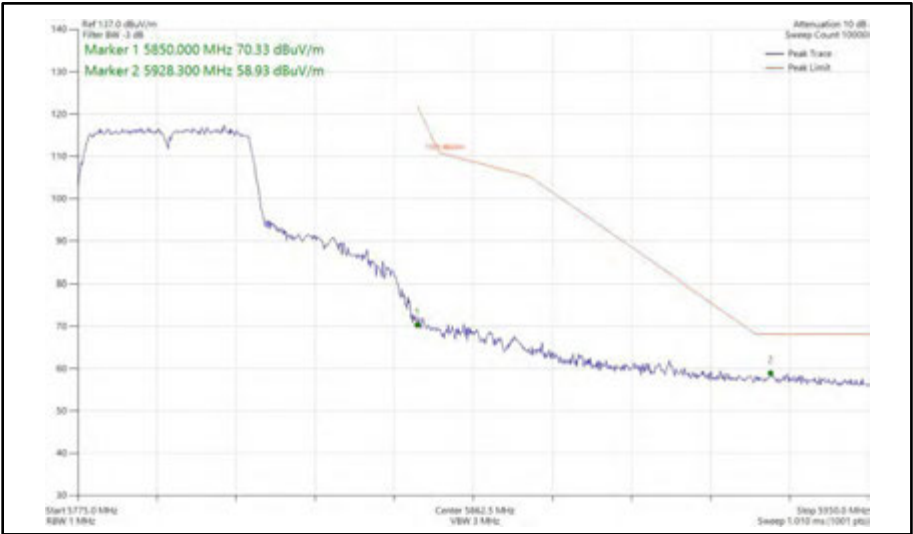
Figure 555 - 802.11n HT40, SISO, Core 1 - 5795 MHz Band Edge Frequency 5850 MHz
