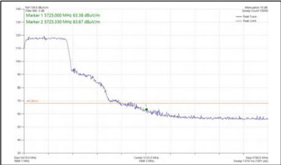
Figure 430 - 802.11ax HE20, SU, SISO, Core 1 - 5680 MHz Band Edge Frequency 5725 MHz
