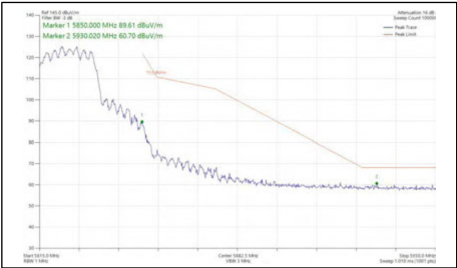
Figure 472 - 802.11ax HE20, SU, CDD, Core 0 + Core 1 - 5825 MHz Band Edge Frequency 5850 MHz
