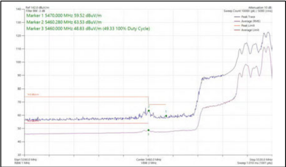
Figure 587 - 802.11ax HE40, RU 52-44, SDM, Core 0 + Core 1 - 5510 MHz Band Edge Frequency 5470 MHz
