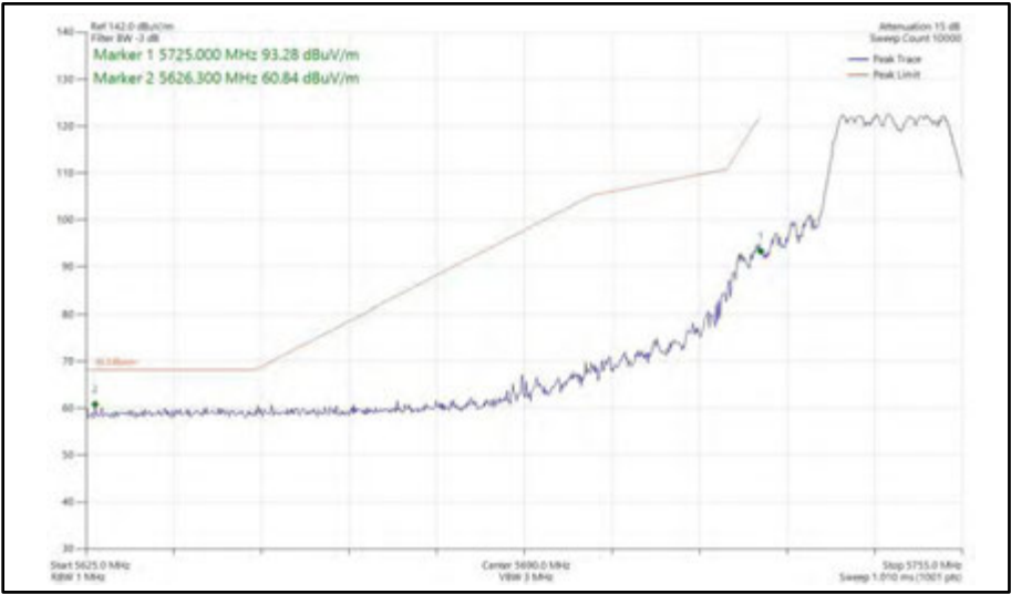
Figure 453 - 802.11n HT20, CDD, Core 0 + Core 1 - 5745 MHz Band Edge Frequency 5725 MHz
