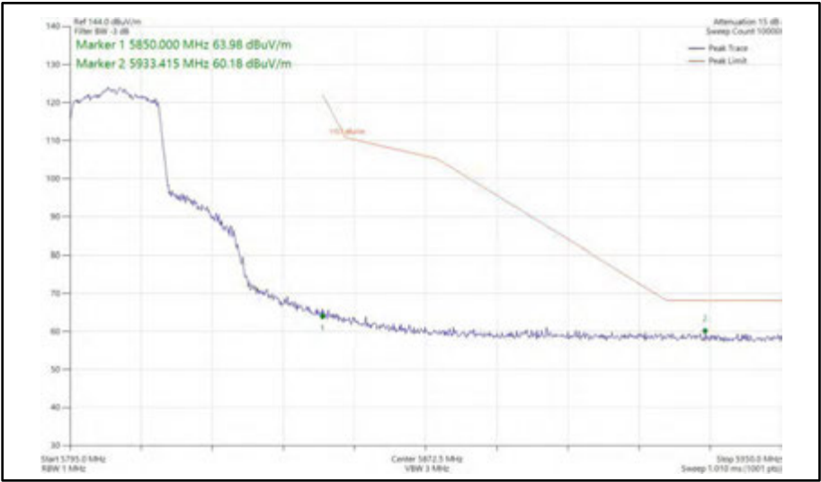
Figure 500 - 802.11ax HE20, SU, SDM, Core 0 + Core 1 - 5805 MHz Band Edge Frequency 5850 MHz
