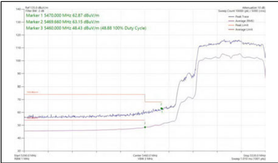
Figure 586 - 802.11ax HE40, SU, SDM, Core 0 + Core 1 - 5510 MHz Band Edge Frequency 5470 MHz
