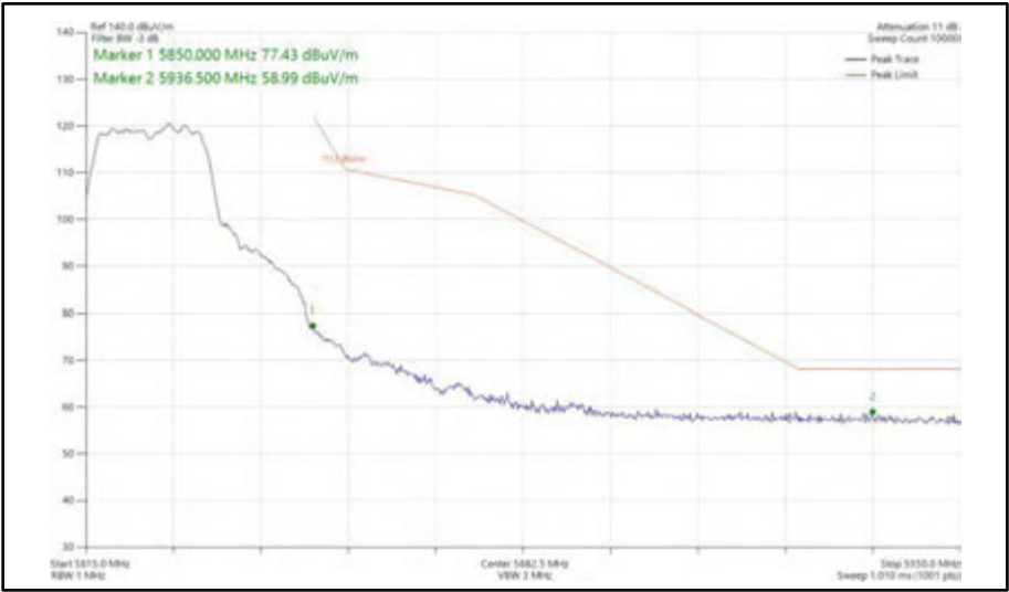
Figure 436 - 802.11a, SISO, Core 1 - 5825 MHz Band Edge Frequency 5850 MHz
