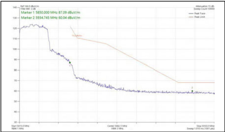
Figure 501 - 802.11ax HE20, SU, SDM, Core 0 + Core 1 - 5825 MHz Band Edge Frequency 5850 MHz
