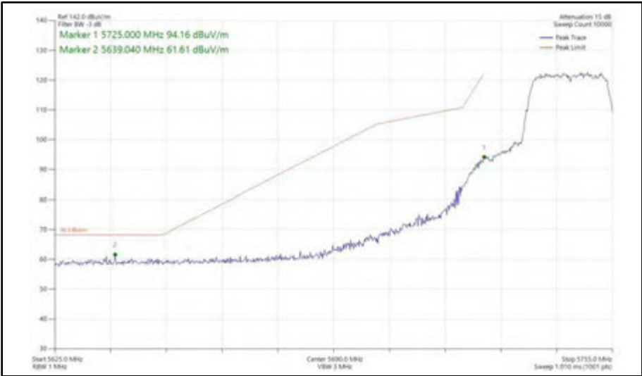
Figure 482 - 802.11n HT20, SDM, Core 0 + Core 1 - 5745 MHz Band Edge Frequency 5725 MHz
