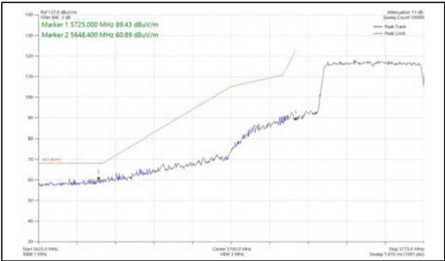
Figure 546 - 802.11ax HE40, SU, SISO, Core 1 - 5755 MHz Band Edge Frequency 5725 MHz
