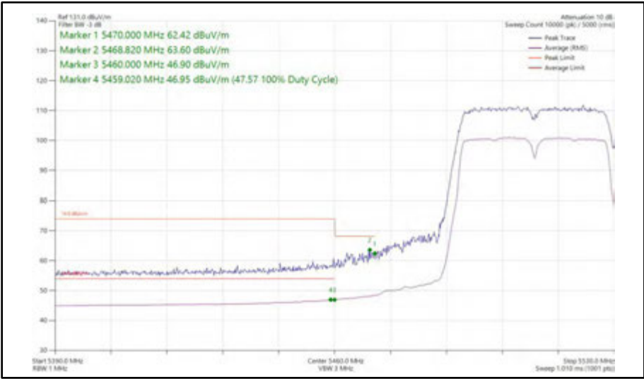
Figure 514 - 802.11n HT40, SISO, Core 0 - 5510 MHz Band Edge Frequency 5470 MHz
