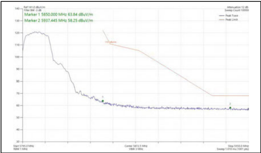
Figure 398 - 802.11a, SISO, Core 0 - 5805 MHz Band Edge Frequency 5850 MHz
