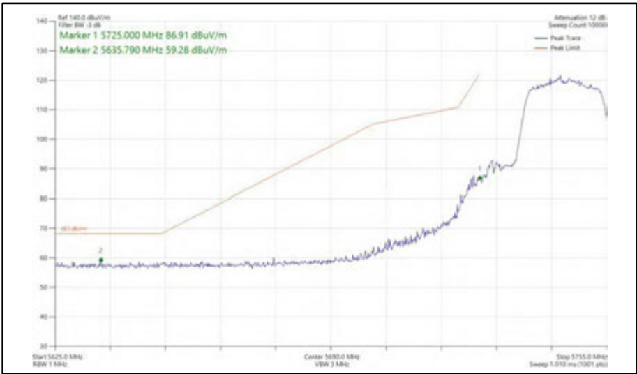
Figure 419 - 802.11n HT20, SISO, Core 1 - 5745 MHz Band Edge Frequency 5725 MHz
