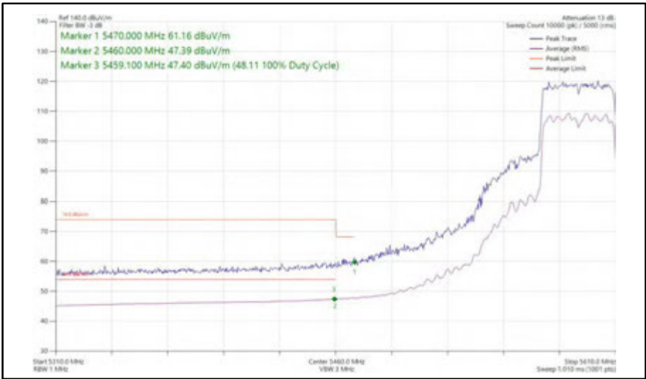
Figure 590 - 802.11ax HE40, SU, SDM, Core 0 + Core 1 - 5590 MHz Band Edge Frequency 5470 MHz
