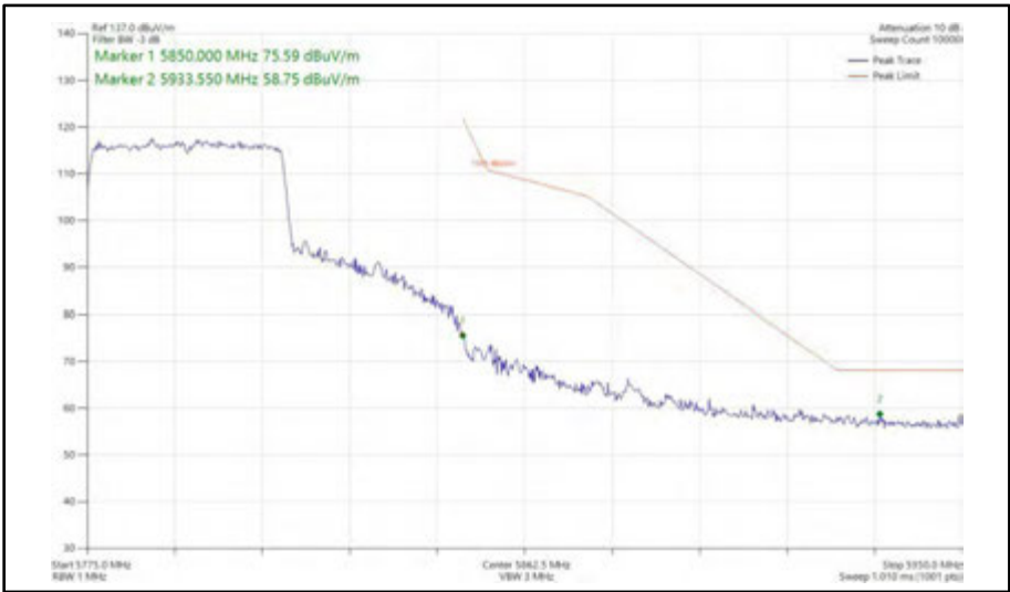
Figure 558 - 802.11ax HE40, SU, SISO, Core 1 - 5795 MHz Band Edge Frequency 5850 MHz
