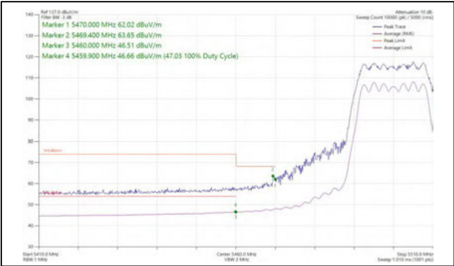
Figure 445 - 802.11n HT20, CDD, Core 0 + Core 1 - 5500 MHz Band Edge Frequency 5470 MHz
