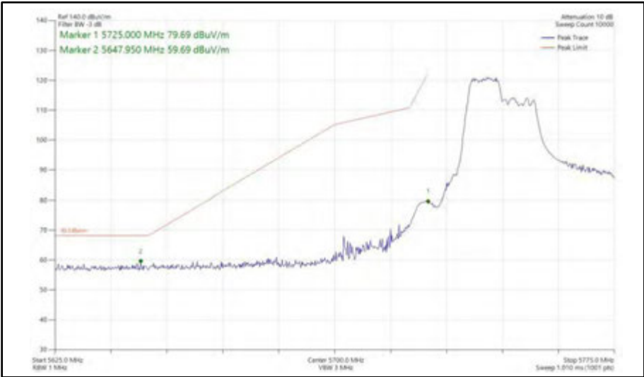
Figure 547 - 802.11ax HE40, RU 106-53, SISO, Core 1 - 5755 MHz Band Edge Frequency 5725 MHz
