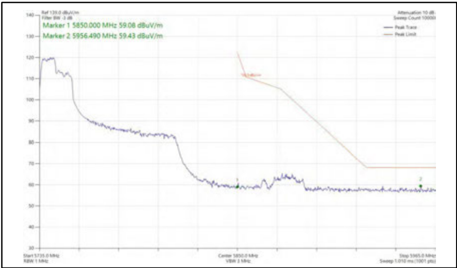
Figure 643 - 802.11ax HE80, RU 106-53, SISO, Core 1 - 5775 MHz Band Edge Frequency 5850 MHz
