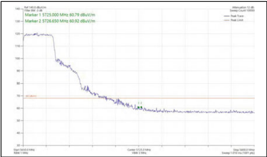
Figure 429 - 802.11ax HE20, SU, SISO, Core 1 - 5660 MHz Band Edge Frequency 5725 MHz
