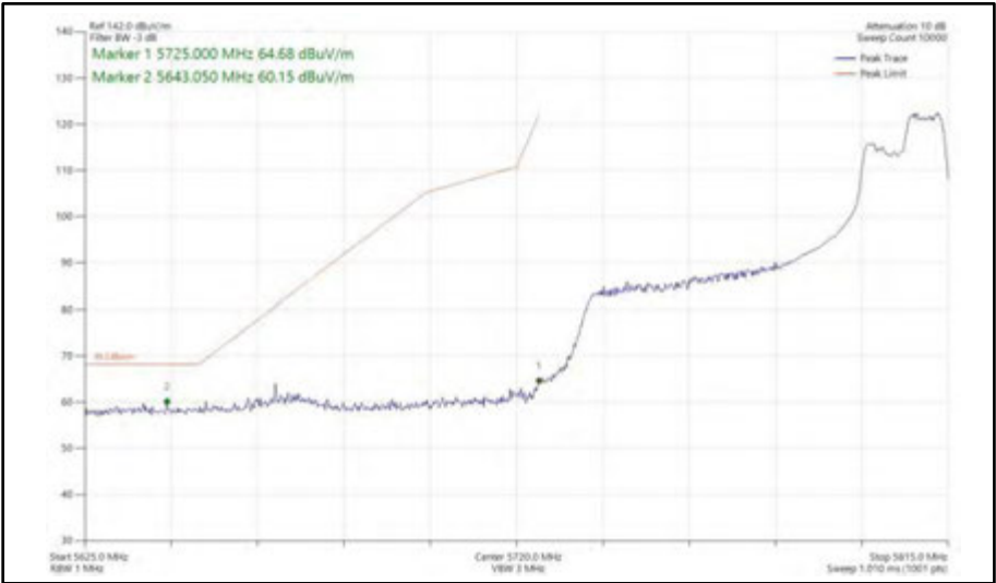
Figure 634 - 802.11ax HE80, RU 106-60, SISO, Core 1 - 5775 MHz Band Edge Frequency 5725 MHz
