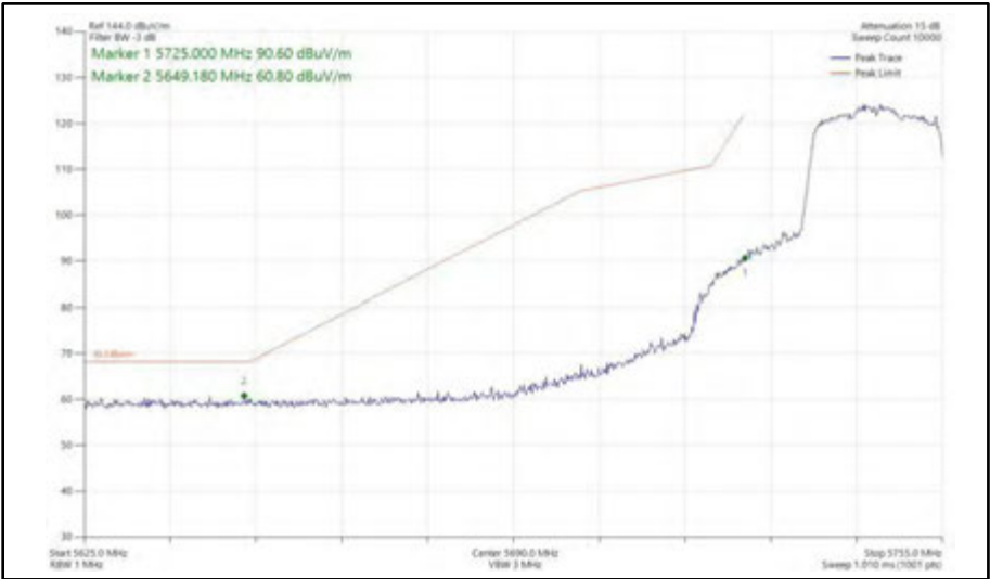
Figure 484 - 802.11ax HE20, SU, SDM, Core 0 + Core 1 - 5745 MHz Band Edge Frequency 5725 MHz
