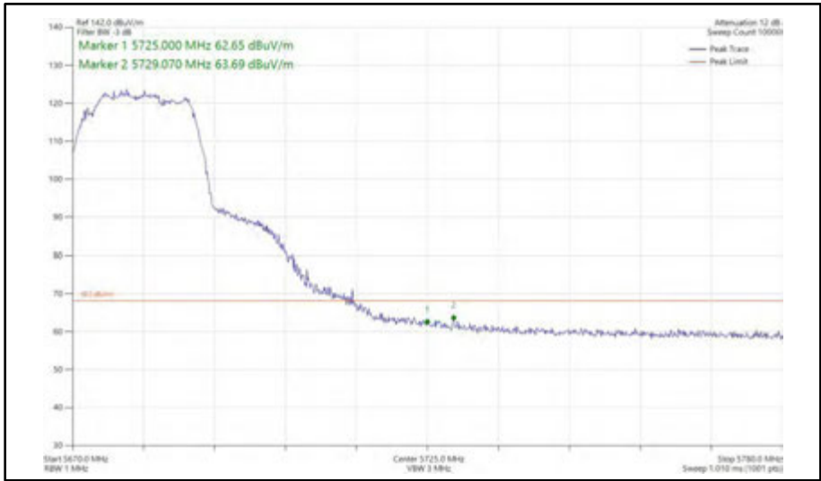
Figure 509 - 802.11ac VHT20, TxBF, Core 0 + Core 1 - 5680 MHz Band Edge Frequency 5725 MHz
