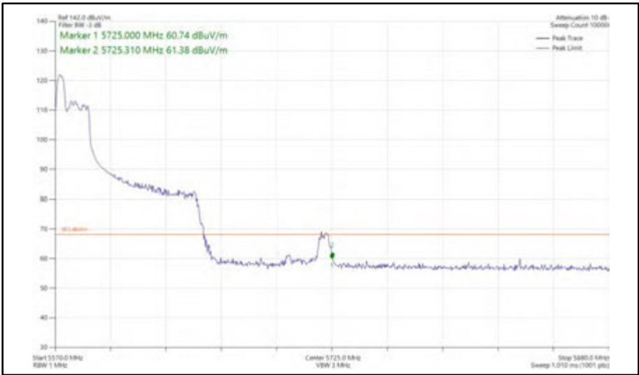
Figure 637 - 802.11ax HE80, RU 52-37, SISO, Core 1 - 5610 MHz Band Edge Frequency 5725 MHz
