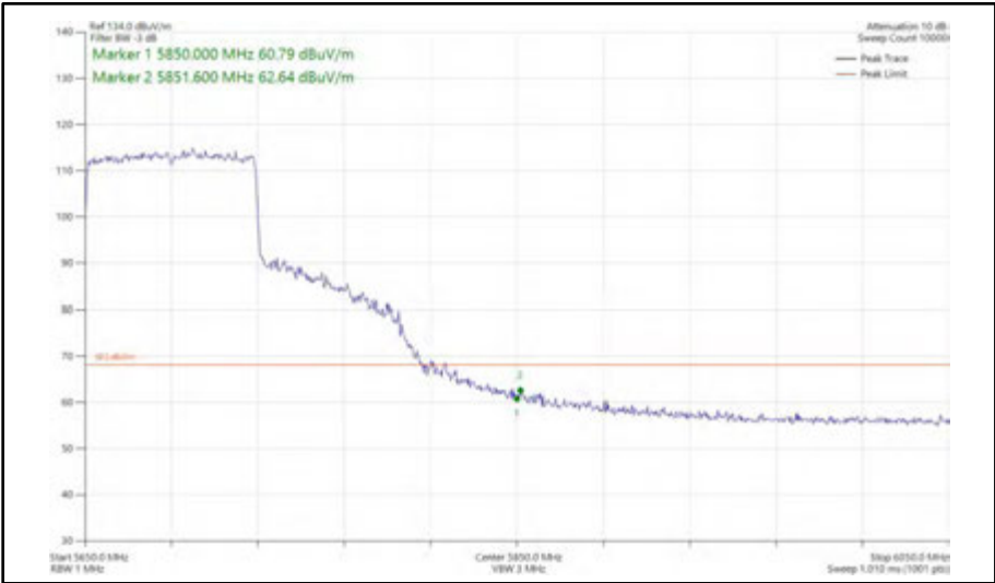
Figure 625 - 802.11ax HE80, SU, SISO, Core 0 - 5690 MHz Band Edge Frequency 5850 MHz
