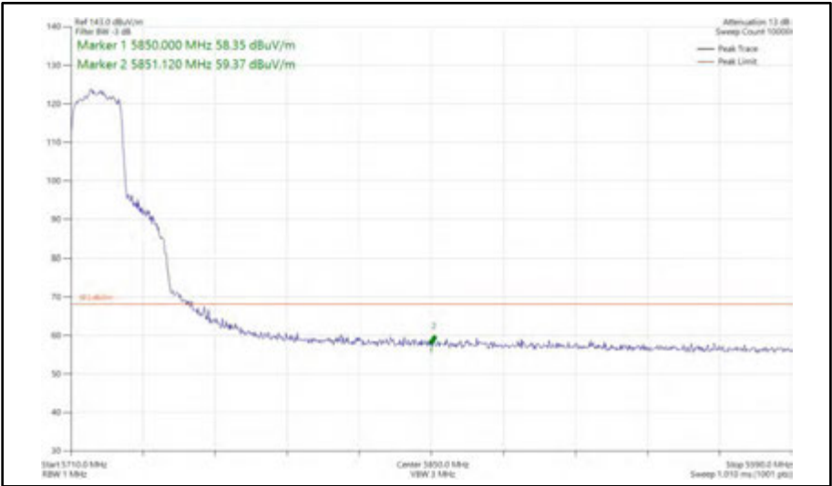
Figure 498 - 802.11ax HE20, SU, SDM, Core 0 + Core 1 - 5720 MHz Band Edge Frequency 5850 MHz
