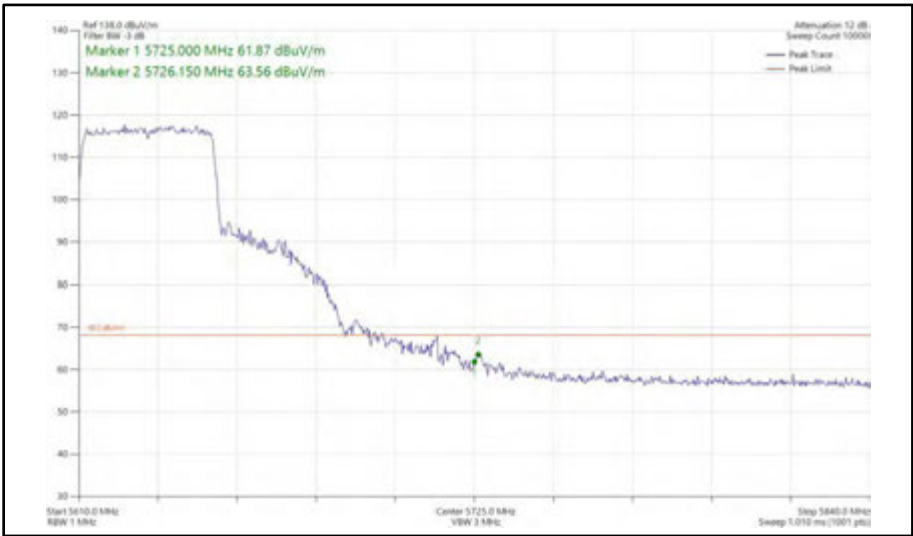
Figure 550 - 802.11ax HE40, SU, SISO, Core 1 - 5630 MHz Band Edge Frequency 5725 MHz
