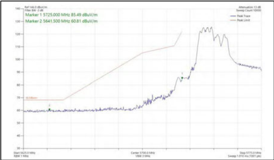
Figure 593 - 802.11ax HE40, RU 106-53, SDM, Core 0 + Core 1 - 5755 MHz Band Edge Frequency 5725 MHz
