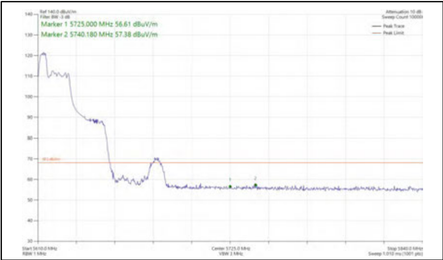
Figure 551 - 802.11ax HE40, RU 52-37, SISO, Core 1 - 5630 MHz Band Edge Frequency 5725 MHz
