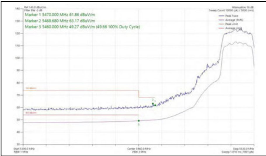
Figure 475 - 802.11n HT20, SDM, Core 0 + Core 1 - 5520 MHz Band Edge Frequency 5470 MHz
