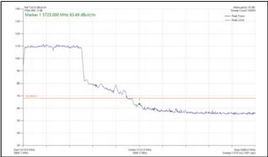
Figure 635 - 802.11ac VHT80, SISO, Core 1 - 5610 MHz Band Edge Frequency 5725 MHz
