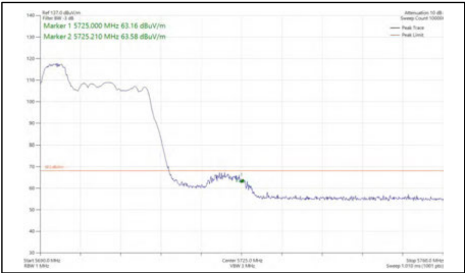
Figure 396 - 802.11ax HE20, RU 52-37, SISO, Core 0 - 5700 MHz Band Edge Frequency 5725 MHz
