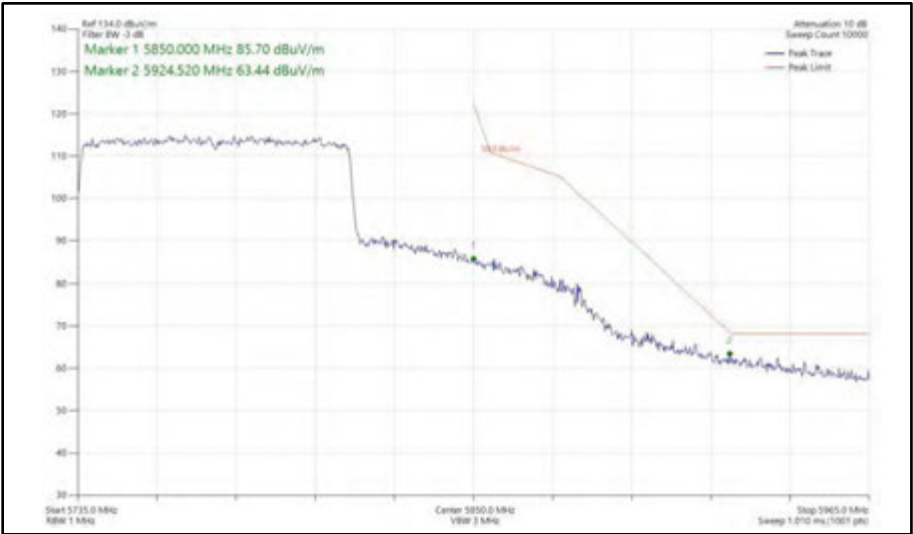
Figure 627 - 802.11ax HE80, SU, SISO, Core 0 - 5775 MHz Band Edge Frequency 5850 MHz
