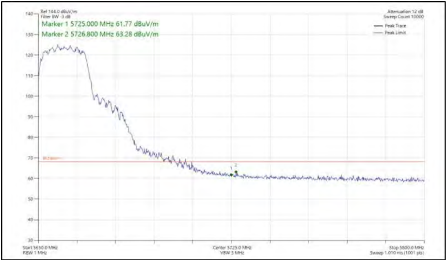
Figure 508 - 802.11ac VHT20, TxBF, Core 0 + Core 1 - 5660 MHz Band Edge Frequency 5725 MHz
