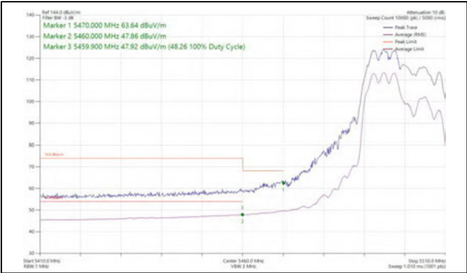
Figure 449 - 802.11ax HE20, RU 106-53, CDD, Core 0 + Core 1 - 5500 MHz Band Edge Frequency 5470 MHz
