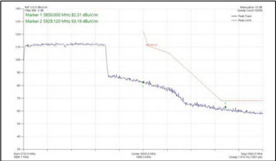
Figure 642 - 802.11ax HE80, SU, SISO, Core 1 - 5775 MHz Band Edge Frequency 5850 MHz
