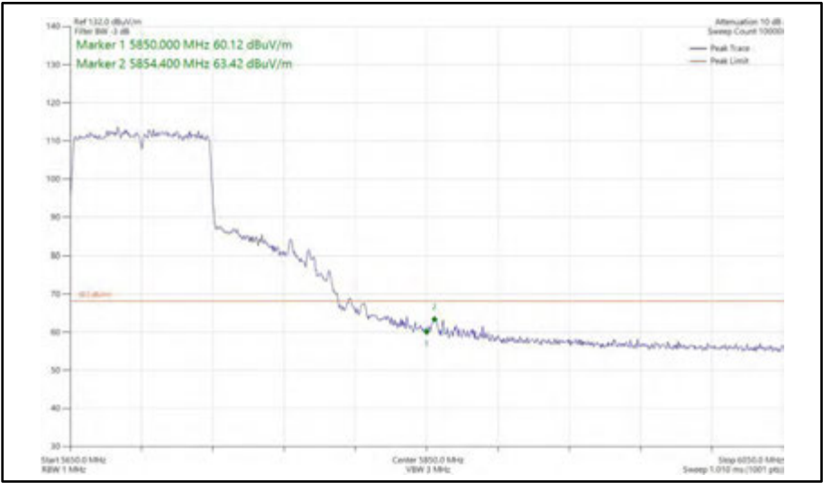
Figure 638 - 802.11ac VHT80, SISO, Core 1 - 5690 MHz Band Edge Frequency 5850 MHz
