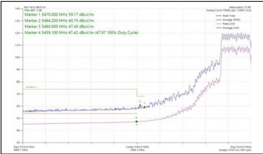
Figure 567 - 802.11ax HE40, SU, CDD, Core 0 + Core 1 - 5590 MHz Band Edge Frequency 5470 MHz
