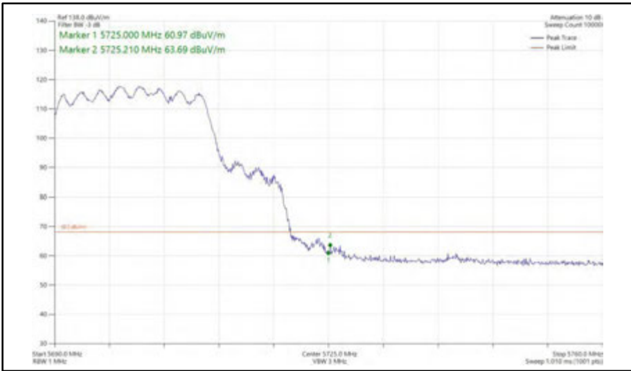
Figure 464 - 802.11ax HE20, SU, CDD, Core 0 + Core 1 - 5700 MHz Band Edge Frequency 5725 MHz
