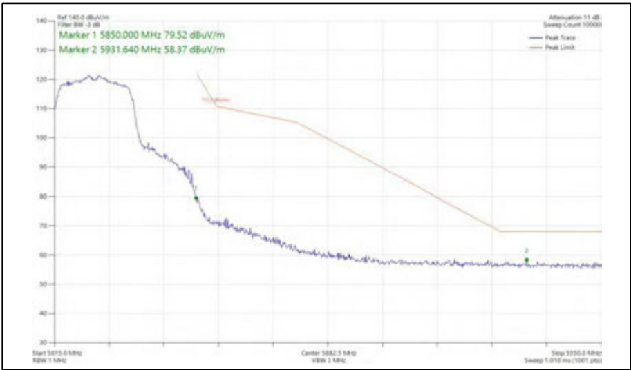
Figure 402 - 802.11n HT20, SISO, Core 0 - 5825 MHz Band Edge Frequency 5850 MHz
