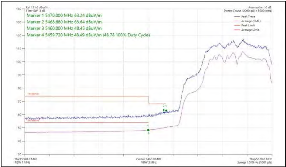
Figure 606 - 802.11ac VHT40, TxBF, Core 0 + Core 1 - 5510 MHz Band Edge Frequency 5470 MHz
