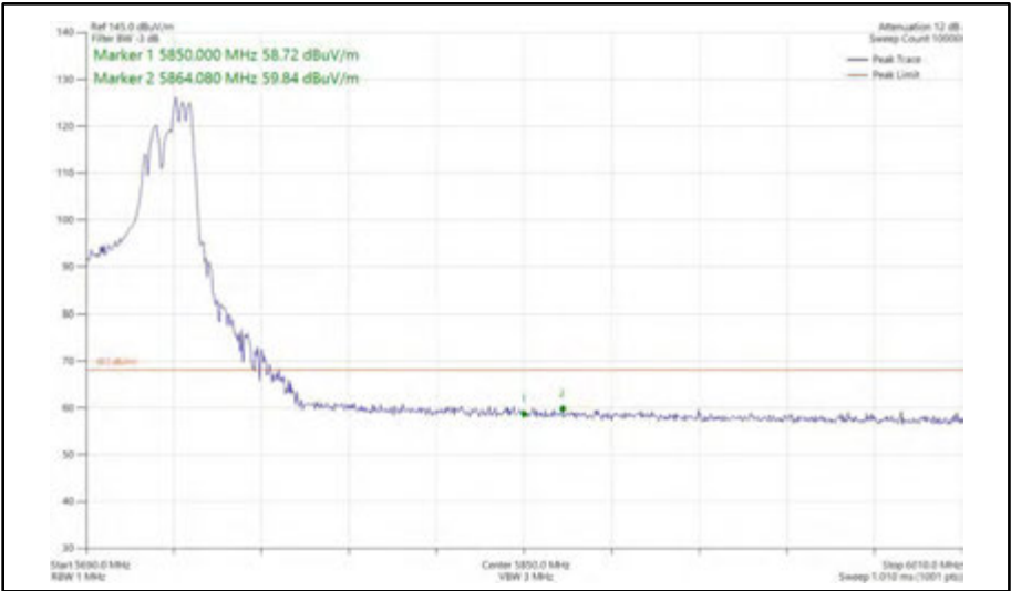
Figure 603 - 802.11ax HE40, RU 106-56, SDM, Core 0 + Core 1 - 5710 MHz Band Edge Frequency 5850 MHz
