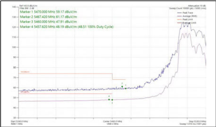
Figure 480 - 802.11ax HE20, RU 106-53, SDM, Core 0 + Core 1 - 5520 MHz Band Edge Frequency 5470 MHz
