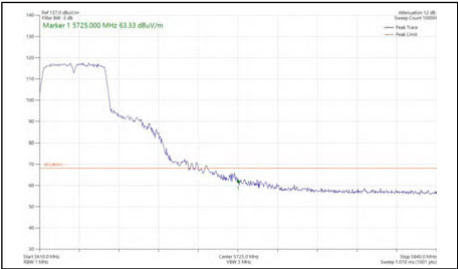
Figure 548 - 802.11n HT40, SISO, Core 1 - 5630 MHz Band Edge Frequency 5725 MHz
