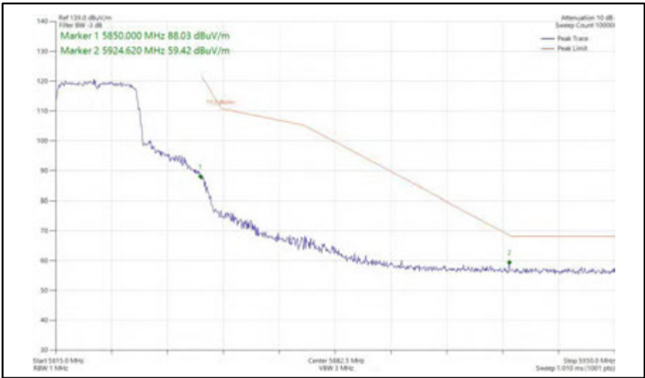
Figure 443 - 802.11ax HE20, SU, SISO, Core 1 - 5825 MHz Band Edge Frequency 5850 MHz
