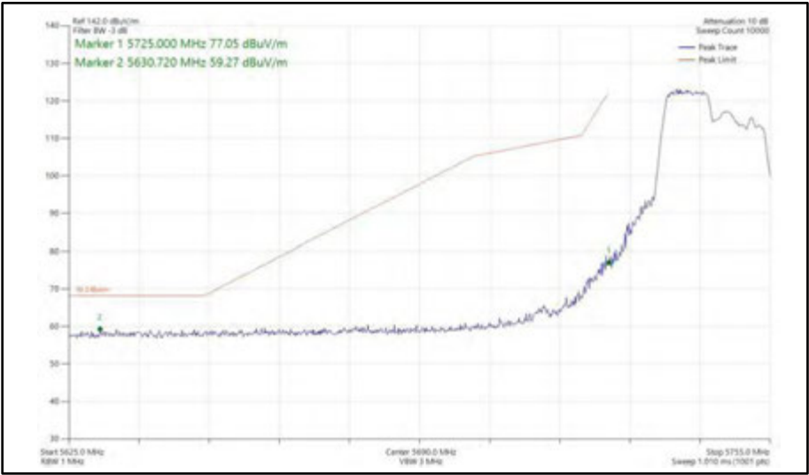
Figure 385 - 802.11ax HE20, RU 106-53, SISO, Core 0 - 5745 MHz Band Edge Frequency 5725 MHz
