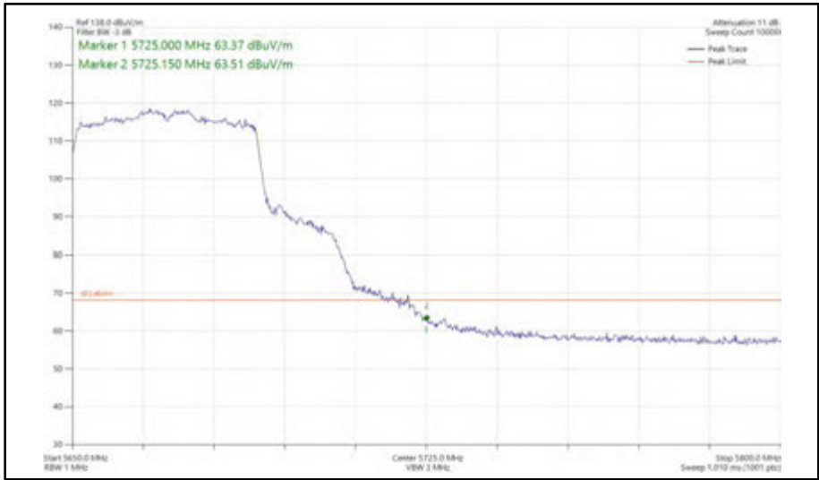
Figure 598 - 802.11ax HE40, SU, SDM, Core 0 + Core 1 - 5670 MHz Band Edge Frequency 5725 MHz
