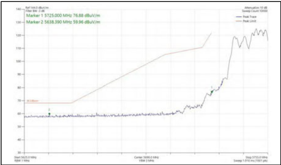
Figure 456 - 802.11ax HE20, RU 106-54, CDD, Core 0 + Core 1 - 5745 MHz Band Edge Frequency 5725 MHz
