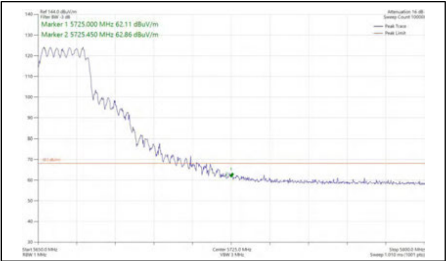
Figure 461 - 802.11ax HE20, SU, CDD, Core 0 + Core 1 - 5660 MHz Band Edge Frequency 5725 MHz
