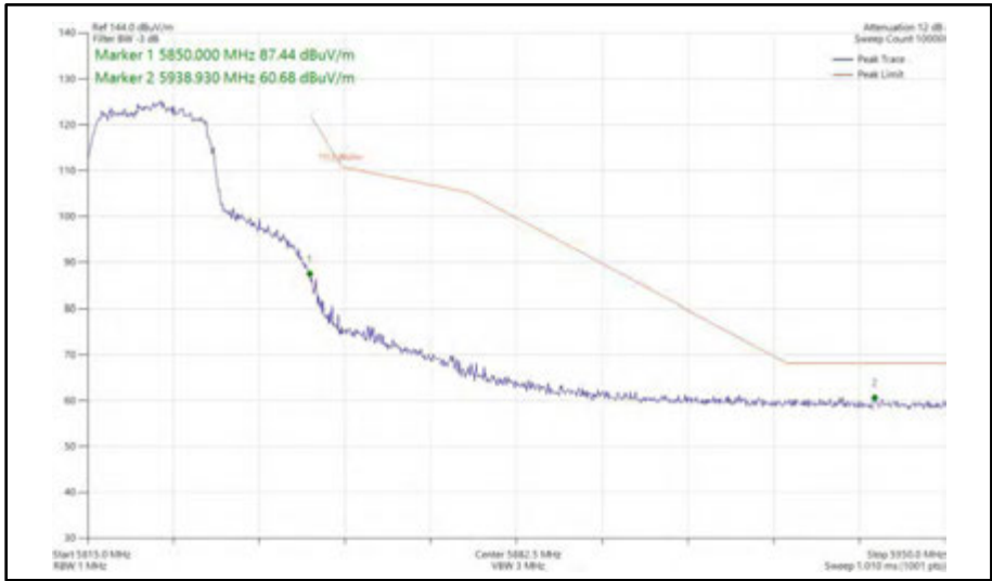
Figure 513 - 802.11ac VHT20, TxBF, Core 0 + Core 1 - 5825 MHz Band Edge Frequency 5850 MHz
