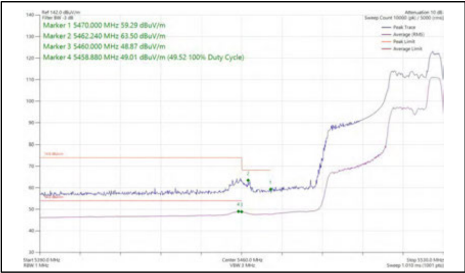
Figure 518 - 802.11ax HE40, RU 52-44, SISO, Core 0 - 5510 MHz Band Edge Frequency 5470 MHz
