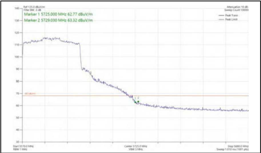
Figure 621 - 802.11ax HE80, SU, SISO, Core 0 - 5610 MHz Band Edge Frequency 5725 MHz
