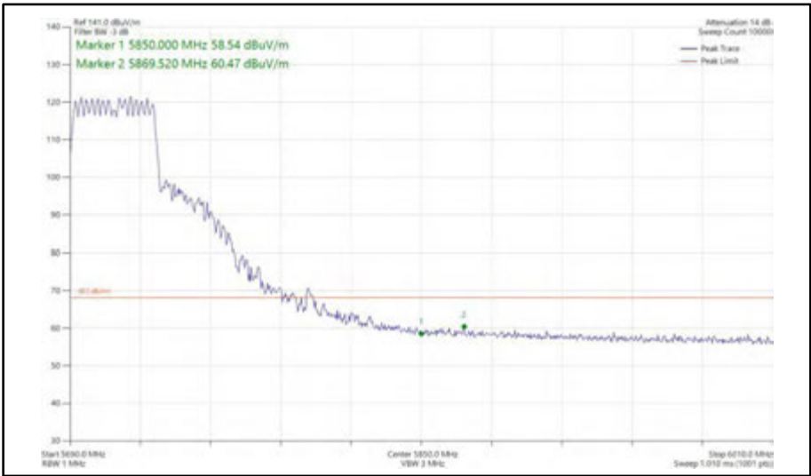
Figure 579 - 802.11ax HE40, SU, CDD, Core 0 + Core 1 - 5710 MHz Band Edge Frequency 5850 MHz
