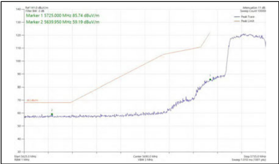
Figure 421 - 802.11ax HE20, SU, SISO, Core 1 - 5745 MHz Band Edge Frequency 5725 MHz
