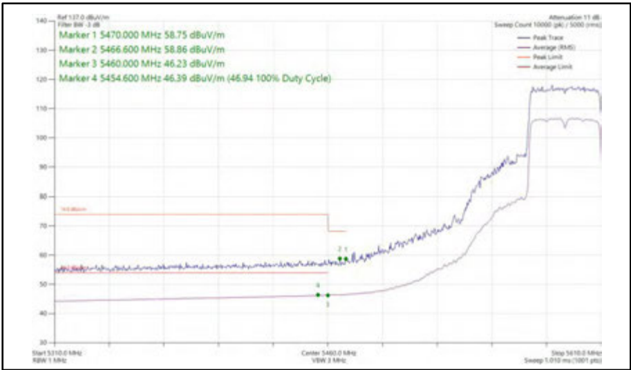
Figure 544 - 802.11ax HE40, SU, SISO, Core 1 - 5590 MHz Band Edge Frequency 5470 MHz
