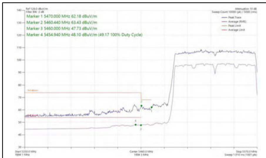
Figure 629 - 802.11ac VHT80, SISO, Core 1 - 5530 MHz Band Edge Frequency 5470 MHz
