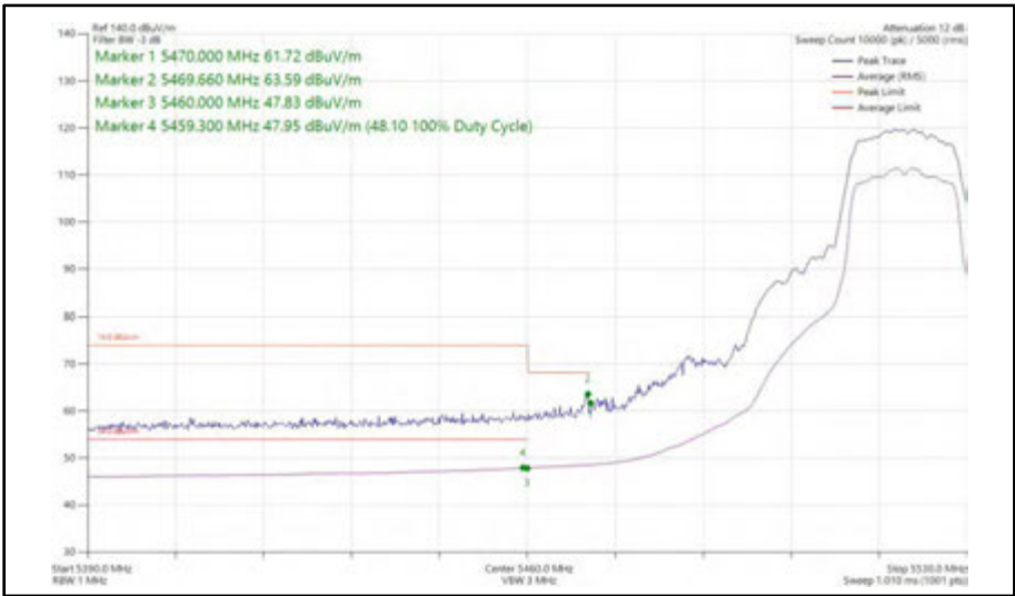
Figure 409 - 802.11a, SISO, Core 1 - 5520 MHz Band Edge Frequency 5470 MHz
