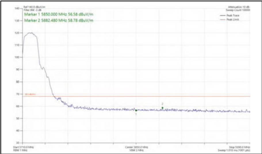
Figure 434 - 802.11a, SISO, Core 1 - 5720 MHz Band Edge Frequency 5850 MHz
