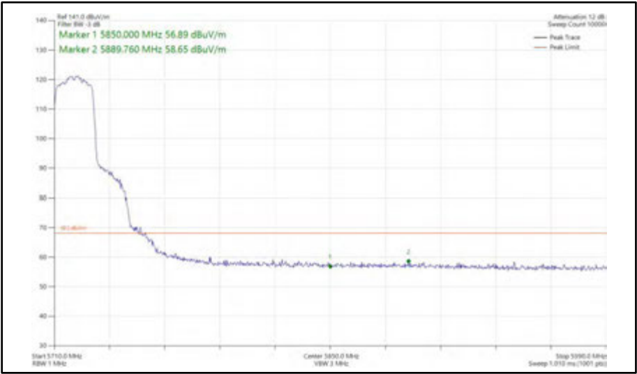
Figure 440 - 802.11ax HE20, SU, SISO, Core 1 - 5720 MHz Band Edge Frequency 5850 MHz
