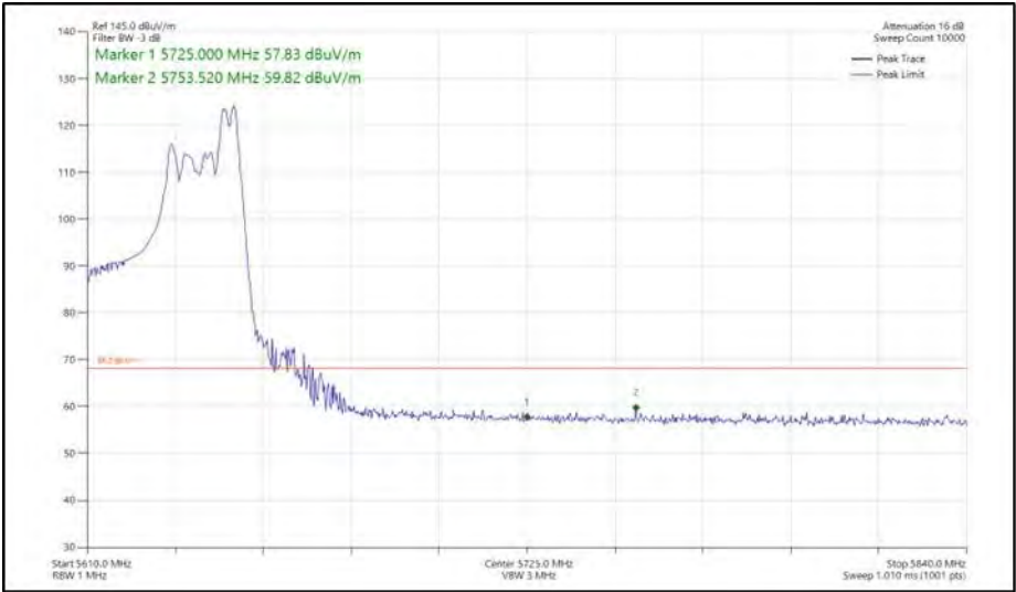
Figure 597 - 802.11ax HE40, RU 52-44, SDM, Core 0 + Core 1 - 5630 MHz Band Edge Frequency 5725 MHz
