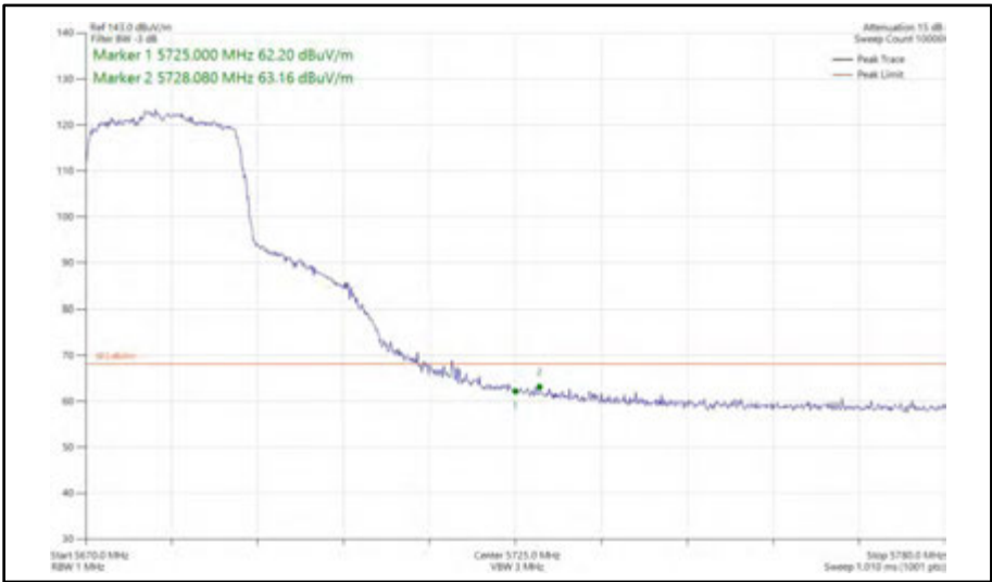
Figure 491 - 802.11ax HE20, SU, SDM, Core 0 + Core 1 - 5680 MHz Band Edge Frequency 5725 MHz
