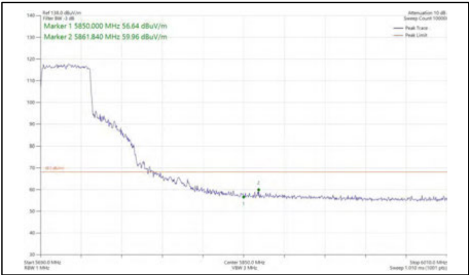
Figure 556 - 802.11ax HE40, SU, SISO, Core 1 - 5710 MHz Band Edge Frequency 5850 MHz
