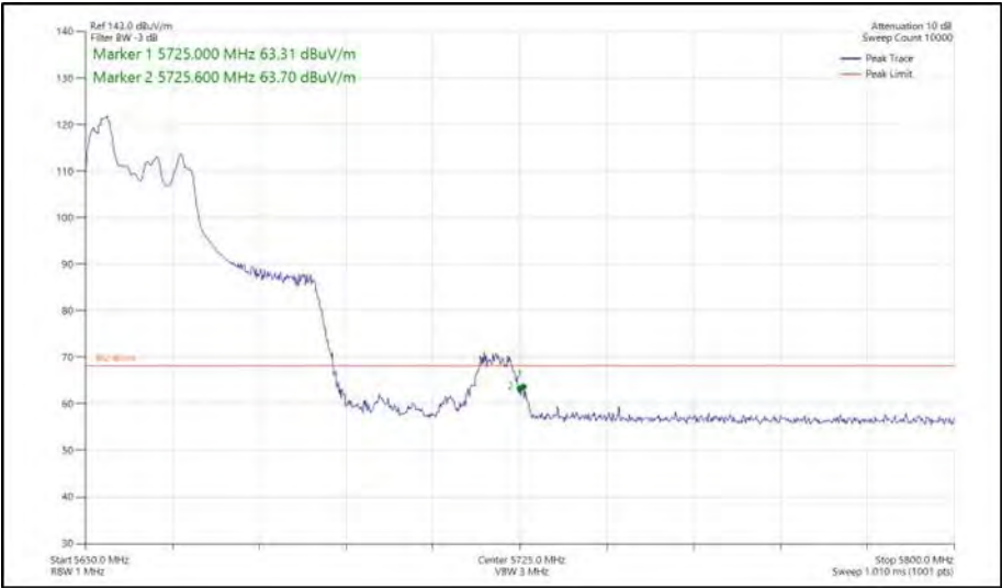
Figure 576 - 802.11ax HE40, RU 52-37, CDD, Core 0 + Core 1 - 5670 MHz Band Edge Frequency 5725 MHz
