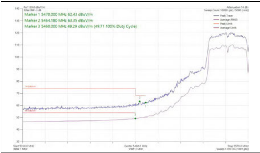
Figure 584 - 802.11n HT40, SDM, Core 0 + Core 1 - 5550 MHz Band Edge Frequency 5470 MHz
