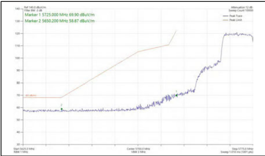
Figure 423 - 802.11ax HE20, SU, SISO, Core 1 - 5765 MHz Band Edge Frequency 5725 MHz
