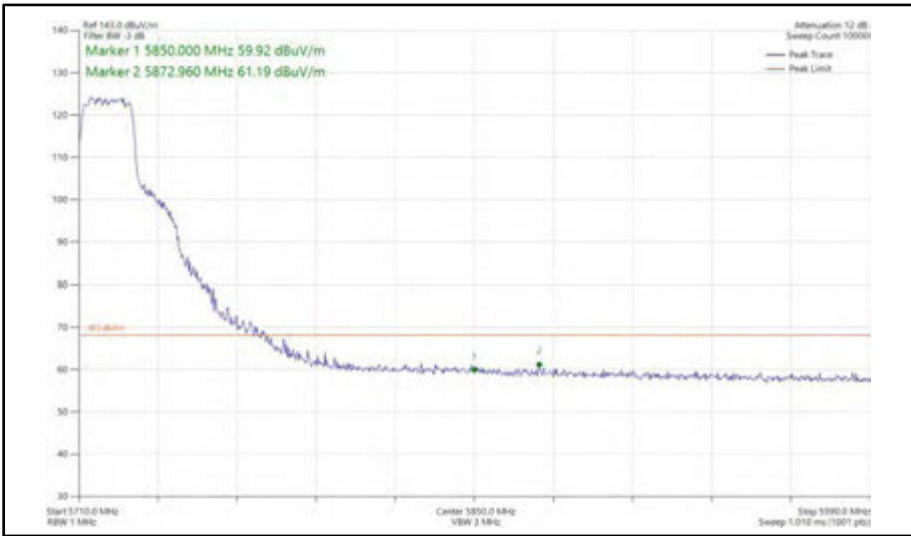
Figure 511 - 802.11ac VHT20, TxBF, Core 0 + Core 1 - 5720 MHz Band Edge Frequency 5850 MHz
