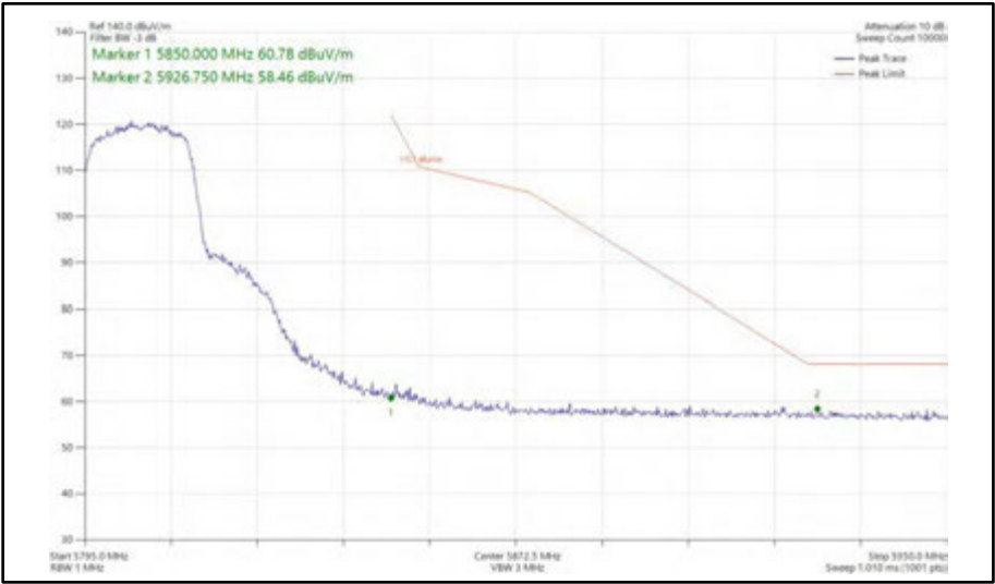
Figure 438 - 802.11n HT20, SISO, Core 1 - 5805 MHz Band Edge Frequency 5850 MHz
