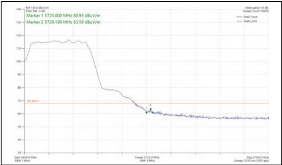
Figure 388 - 802.11a, SISO, Core 0 - 5700 MHz Band Edge Frequency 5725 MHz
