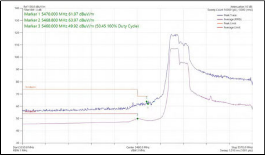
Figure 631 - 802.11ax HE80, RU 106-53, SISO, Core 1 - 5530 MHz Band Edge Frequency 5470 MHz
