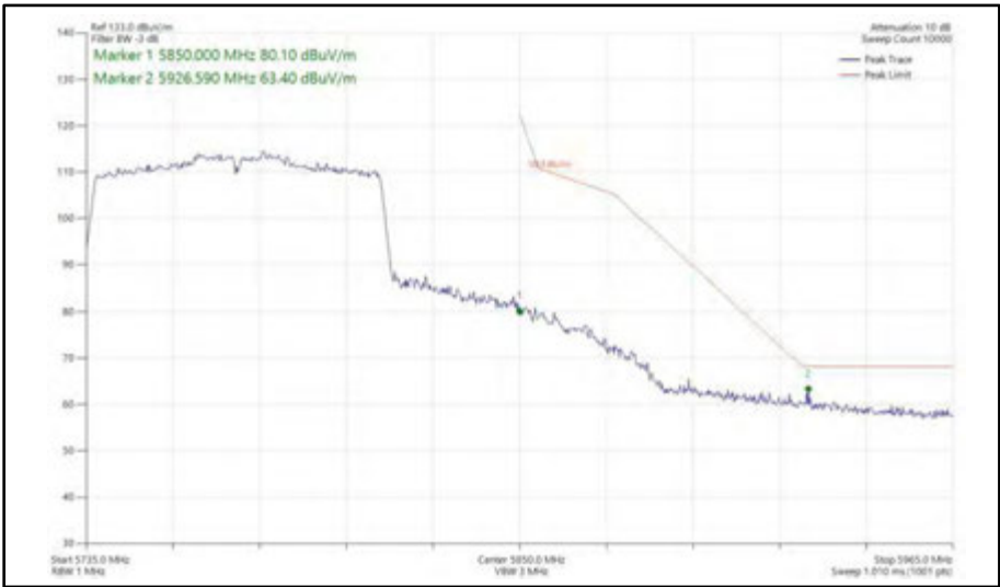
Figure 639 - 802.11ac VHT80, SISO, Core 1 - 5775 MHz Band Edge Frequency 5850 MHz
