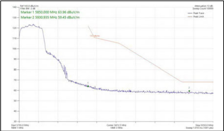
Figure 496 - 802.11n HT20, SDM, Core 0 + Core 1 - 5805 MHz Band Edge Frequency 5850 MHz
