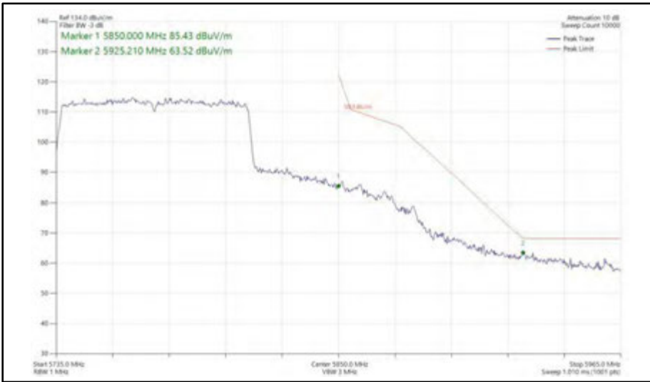
Figure 624 - 802.11ac VHT80, SISO, Core 0 - 5775 MHz Band Edge Frequency 5850 MHz
