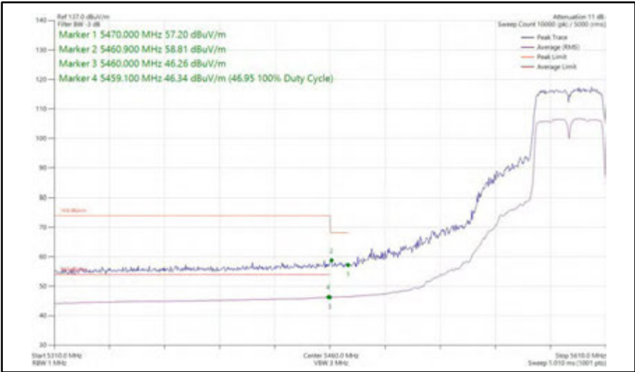
Figure 539 - 802.11n HT40, SISO, Core 1 - 5590 MHz Band Edge Frequency 5470 MHz
