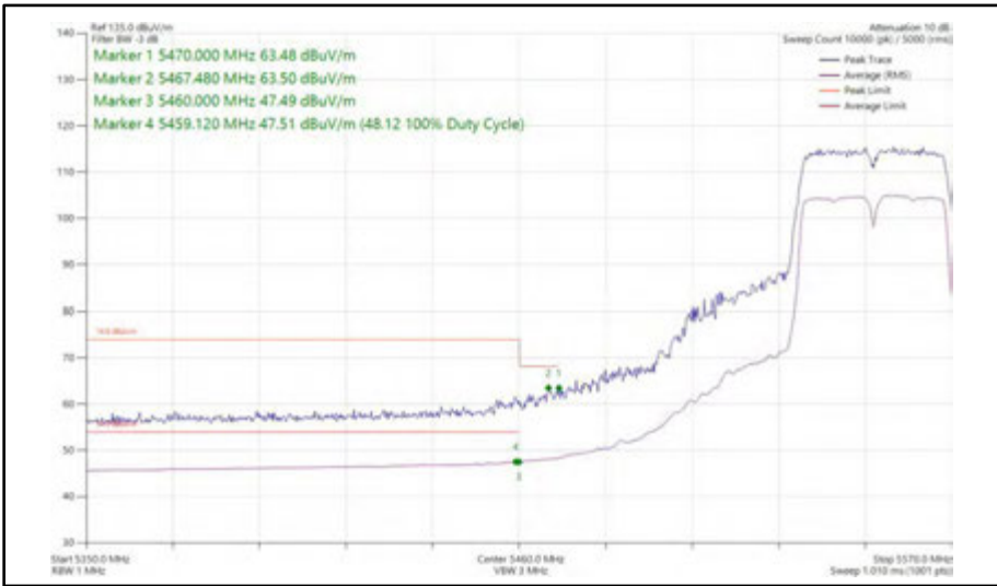
Figure 515 - 802.11n HT40, SISO, Core 0 - 5550 MHz Band Edge Frequency 5470 MHz
