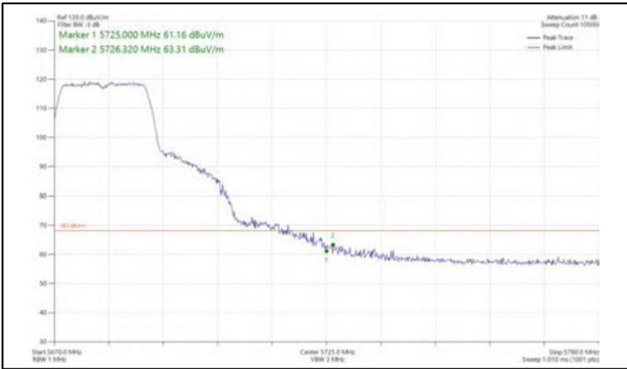
Figure 427 - 802.11n HT20, SISO, Core 1 - 5680 MHz Band Edge Frequency 5725 MHz
