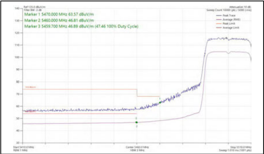
Figure 412 - 802.11ax HE20, SU, SISO, Core 1 - 5500 MHz Band Edge Frequency 5470 MHz
