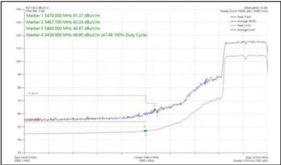
Figure 542 - 802.11ax HE40, SU, SISO, Core 1 - 5550 MHz Band Edge Frequency 5470 MHz
