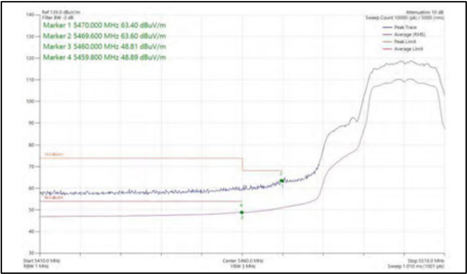
Figure 408 - 802.11a, SISO, Core 1 - 5500 MHz Band Edge Frequency 5470 MHz
