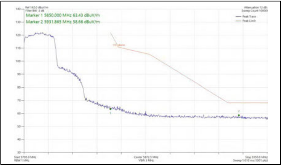
Figure 405 - 802.11ax HE20, SU, SISO, Core 0 - 5805 MHz Band Edge Frequency 5850 MHz
