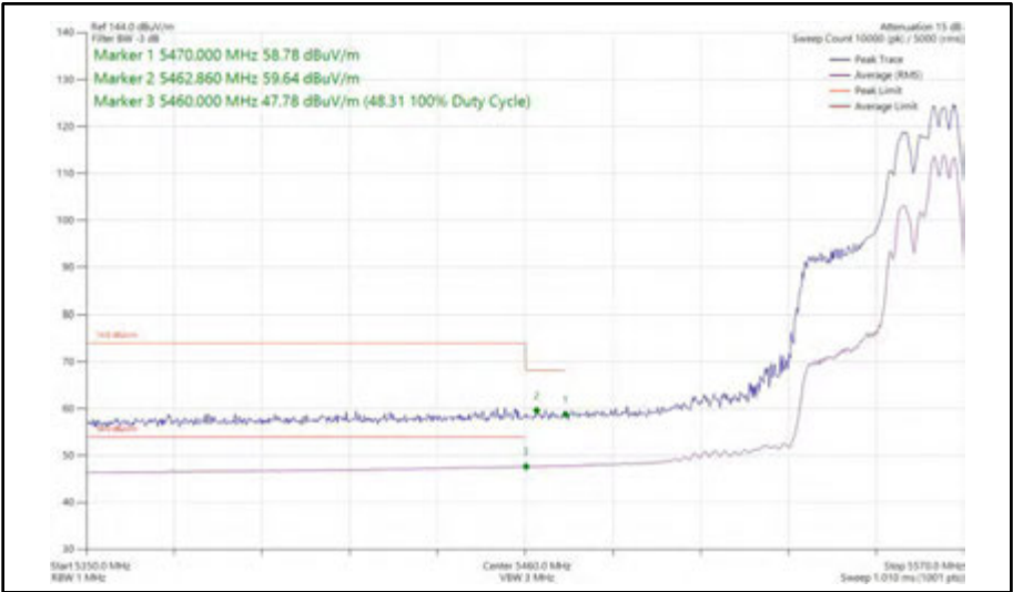
Figure 589 - 802.11ax HE40, RU 106-56, SDM, Core 0 + Core 1 - 5550 MHz Band Edge Frequency 5470 MHz
