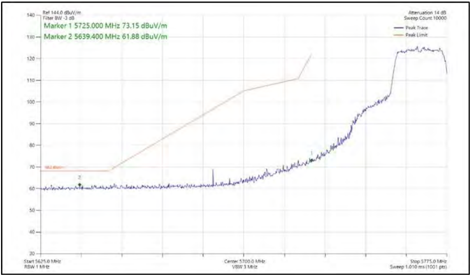
Figure 507 - 802.11ac VHT20, TxBF, Core 0 + Core 1 - 5765 MHz Band Edge Frequency 5725 MHz
