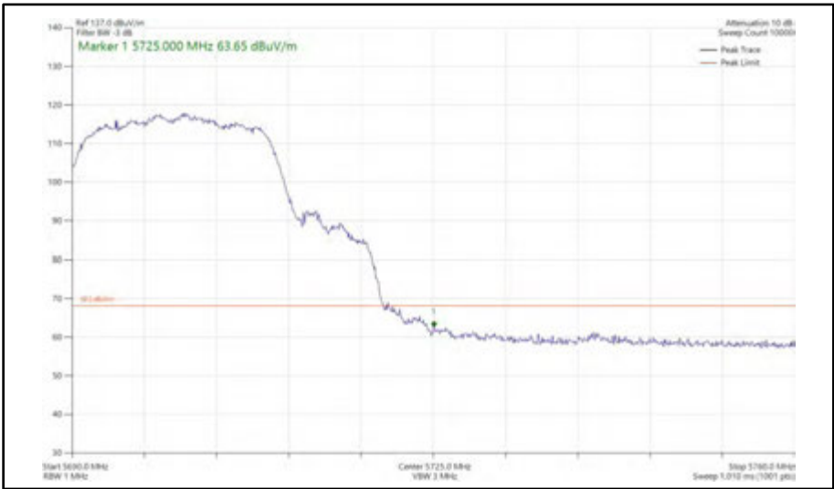
Figure 460 - 802.11n HT20, CDD, Core 0 + Core 1 - 5700 MHz Band Edge Frequency 5725 MHz
