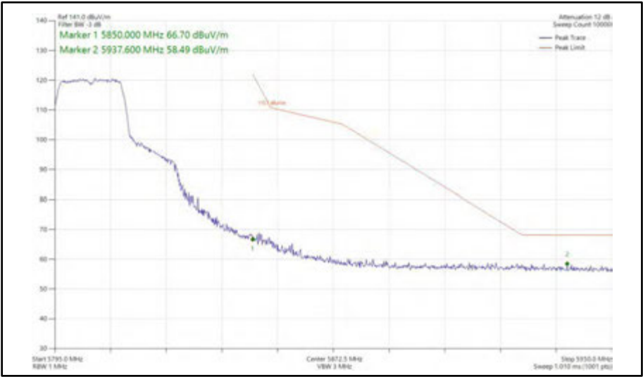
Figure 401 - 802.11n HT20, SISO, Core 0 - 5805 MHz Band Edge Frequency 5850 MHz
