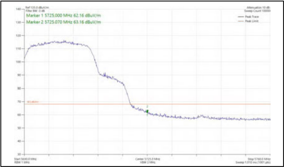
Figure 391 - 802.11n HT20, SISO, Core 0 - 5700 MHz Band Edge Frequency 5725 MHz
