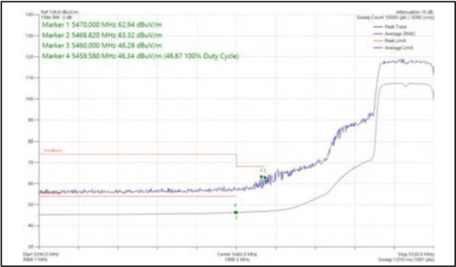
Figure 414 - 802.11ax HE20, SU, SISO, Core 1 - 5520 MHz Band Edge Frequency 5470 MHz
