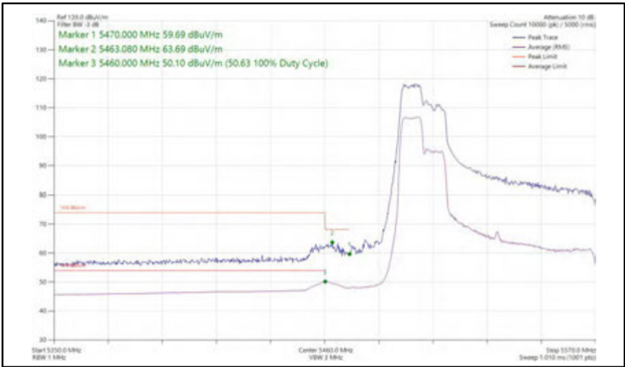
Figure 616 - 802.11ax HE80, RU 106-53, SISO, Core 0 - 5530 MHz Band Edge Frequency 5470 MHz
