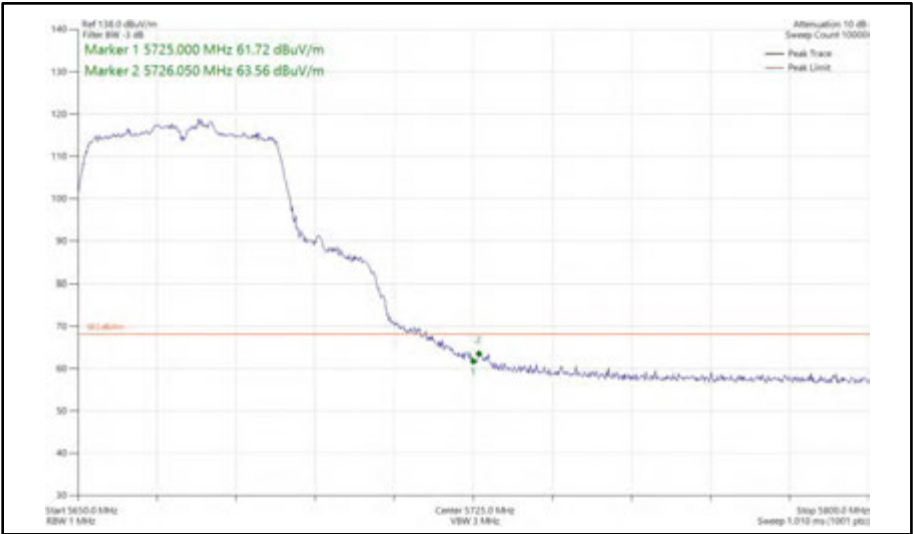
Figure 595 - 802.11n HT40, SDM, Core 0 + Core 1 - 5670 MHz Band Edge Frequency 5725 MHz
