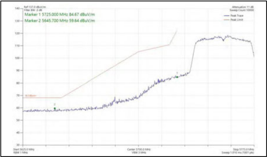
Figure 545 - 802.11n HT40, SISO, Core 1 - 5755 MHz Band Edge Frequency 5725 MHz
