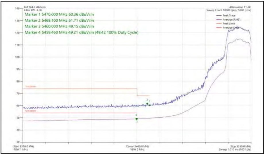
Figure 505 - 802.11ac VHT20, TxBF, Core 0 + Core 1 - 5540 MHz Band Edge Frequency 5470 MHz
