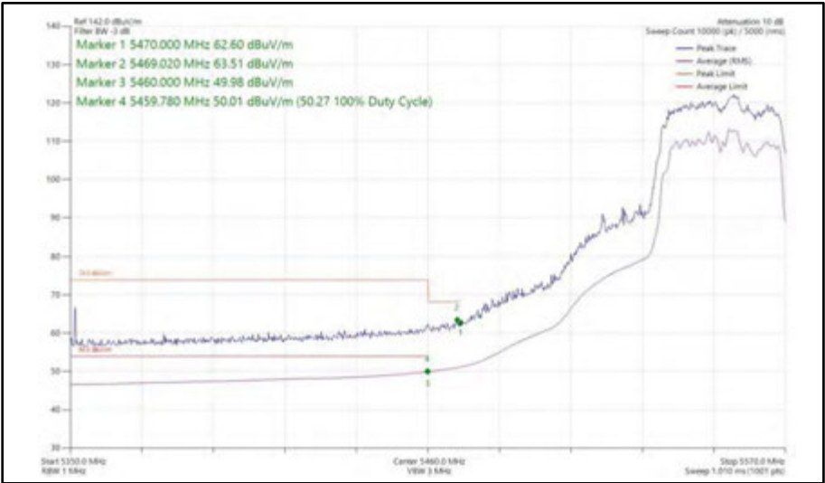
Figure 607 - 802.11ac VHT40, TxBF, Core 0 + Core 1 - 5550 MHz Band Edge Frequency 5470 MHz
