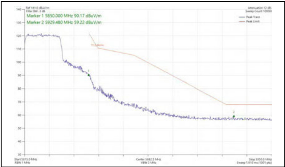
Figure 406 - 802.11ax HE20, SU, SISO, Core 0 - 5825 MHz Band Edge Frequency 5850 MHz
