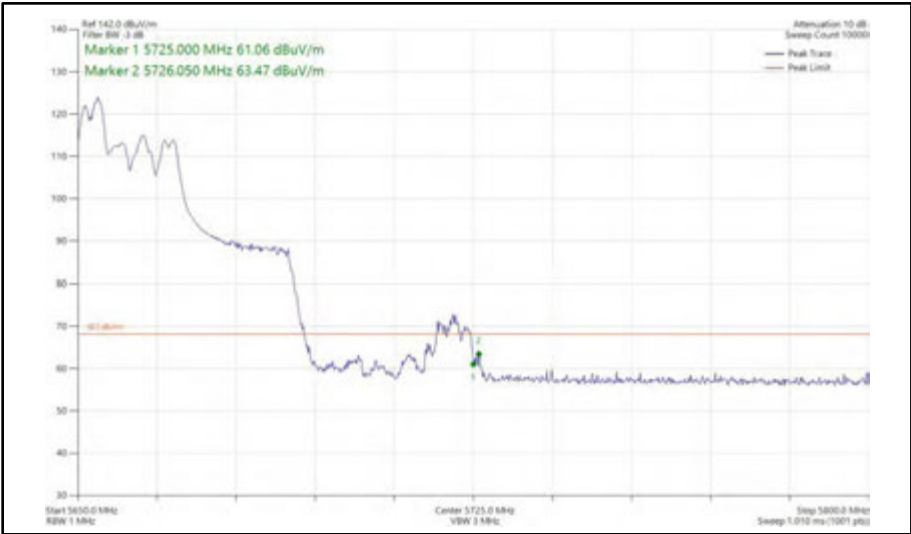
Figure 599 - 802.11ax HE40, RU 52-37, SDM, Core 0 + Core 1 - 5670 MHz Band Edge Frequency 5725 MHz
