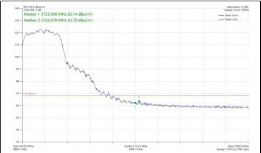
Figure 459 - 802.11n HT20, CDD, Core 0 + Core 1 - 5680 MHz Band Edge Frequency 5725 MHz
