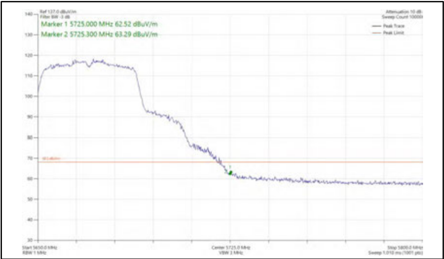
Figure 549 - 802.11n HT40, SISO, Core 1 - 5670 MHz Band Edge Frequency 5725 MHz
