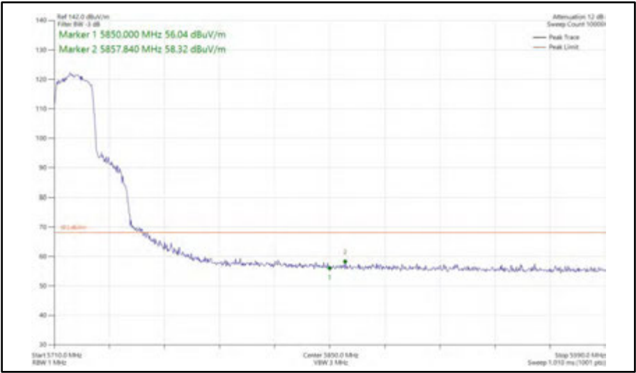
Figure 403 - 802.11ax HE20, SU, SISO, Core 0 - 5720 MHz Band Edge Frequency 5850 MHz
