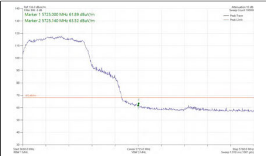
Figure 510 - 802.11ac VHT20, TxBF, Core 0 + Core 1 - 5700 MHz Band Edge Frequency 5725 MHz
