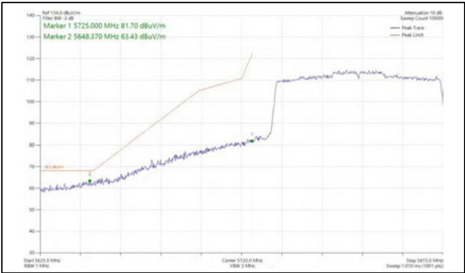
Figure 633 - 802.11ax HE80, SU, SISO, Core 1 - 5775 MHz Band Edge Frequency 5725 MHz
