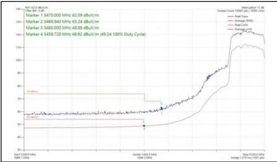
Figure 479 - 802.11ax HE20, SU, SDM, Core 0 + Core 1 - 5520 MHz Band Edge Frequency 5470 MHz
