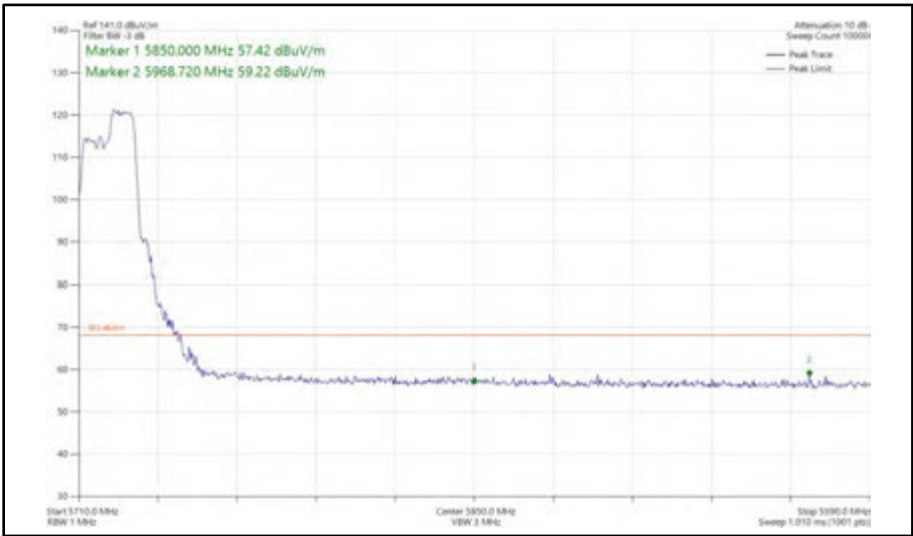
Figure 441 - 802.11ax HE20, RU 106-54, SISO, Core 1 - 5720 MHz Band Edge Frequency 5850 MHz
