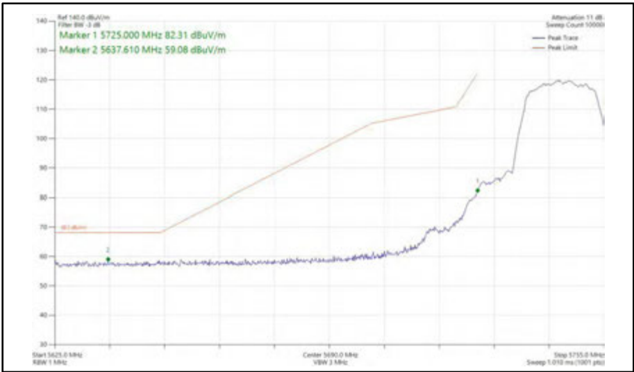
Figure 417 - 802.11a, SISO, Core 1 - 5745 MHz Band Edge Frequency 5725 MHz
