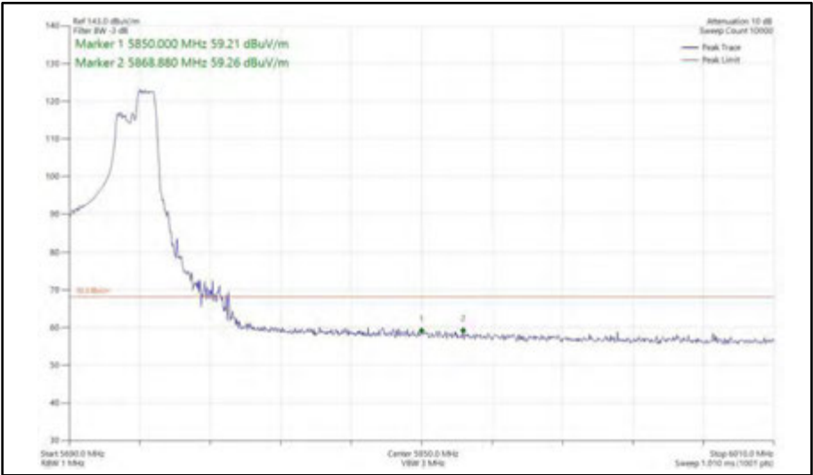
Figure 534 - 802.11ax HE40, RU 106-56, SISO, Core 0 - 5710 MHz Band Edge Frequency 5850 MHz
