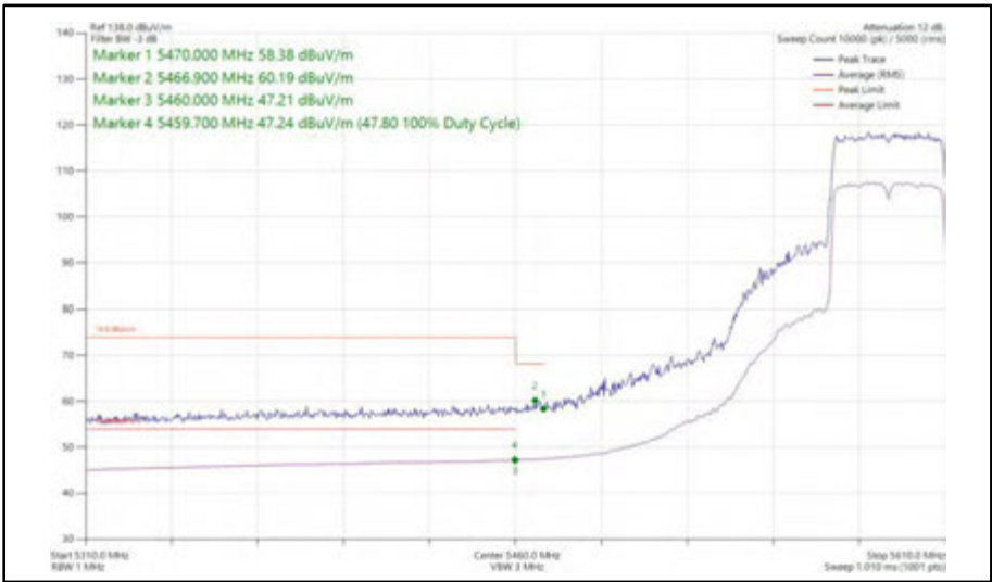
Figure 521 - 802.11ax HE40, SU, SISO, Core 0 - 5590 MHz Band Edge Frequency 5470 MHz
