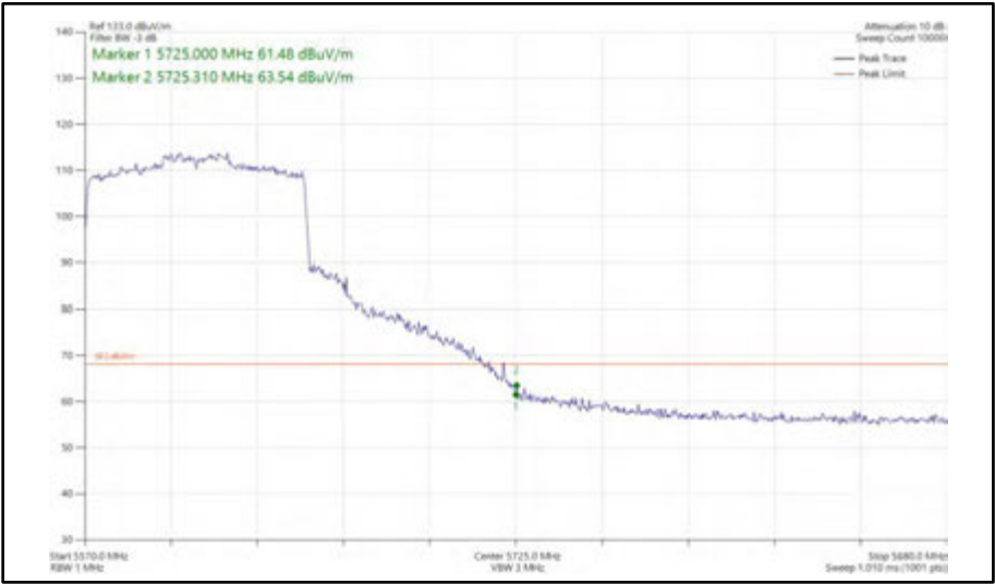
Figure 636 - 802.11ax HE80, SU, SISO, Core 1 - 5610 MHz Band Edge Frequency 5725 MHz
