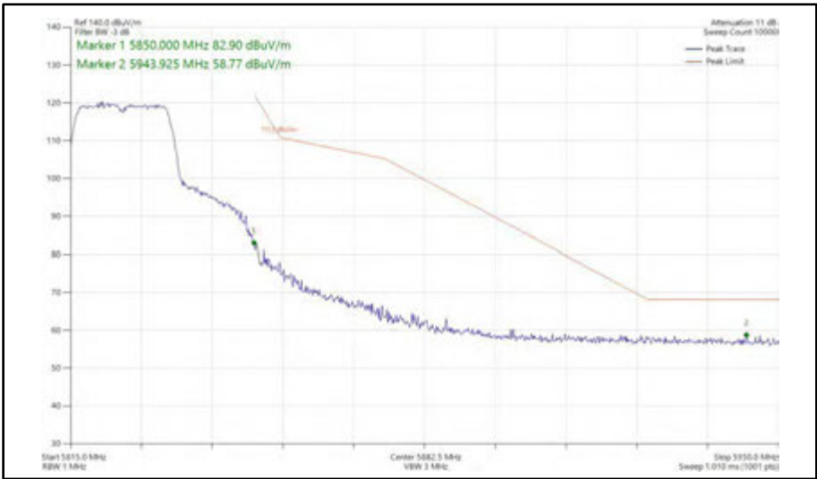
Figure 439 - 802.11n HT20, SISO, Core 1 - 5825 MHz Band Edge Frequency 5850 MHz
