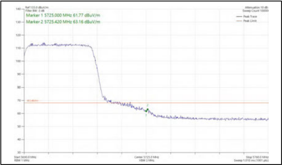
Figure 395 - 802.11ax HE20, SU, SISO, Core 0 - 5700 MHz Band Edge Frequency 5725 MHz
