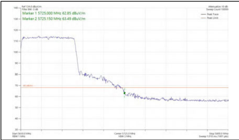
Figure 552 - 802.11ax HE40, SU, SISO, Core 1 - 5670 MHz Band Edge Frequency 5725 MHz
