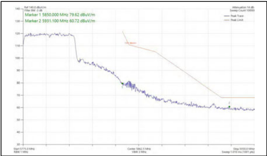
Figure 604 - 802.11ax HE40, SU, SDM, Core 0 + Core 1 - 5795 MHz Band Edge Frequency 5850 MHz
