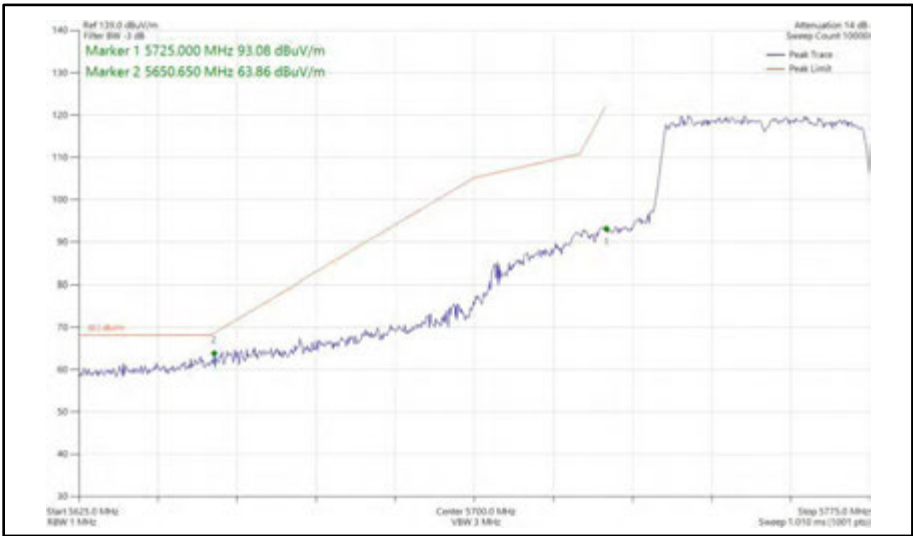
Figure 592 - 802.11ax HE40, SU, SDM, Core 0 + Core 1 - 5755 MHz Band Edge Frequency 5725 MHz
