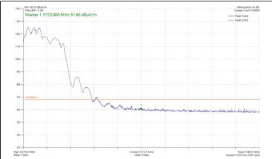
Figure 463 - 802.11ax HE20, RU 106-53, CDD, Core 0 + Core 1 - 5680 MHz Band Edge Frequency 5725 MHz
