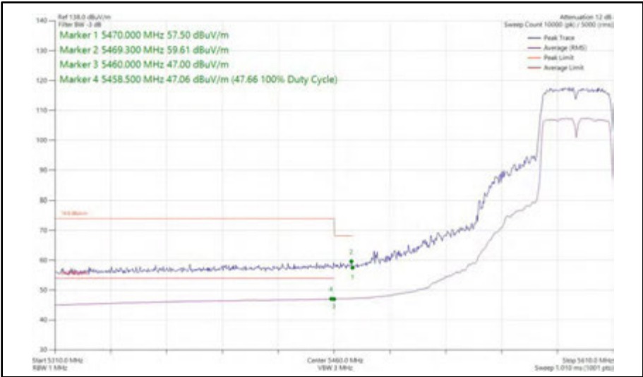
Figure 516 - 802.11n HT40, SISO, Core 0 - 5590 MHz Band Edge Frequency 5470 MHz
