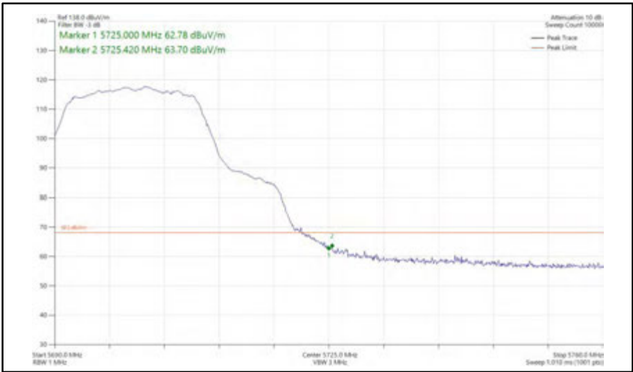
Figure 425 - 802.11a, SISO, Core 1 - 5700 MHz Band Edge Frequency 5725 MHz
