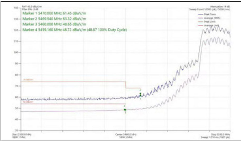
Figure 450 - 802.11ax HE20, SU, CDD, Core 0 + Core 1 - 5520 MHz Band Edge Frequency 5470 MHz
