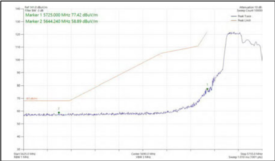
Figure 422 - 802.11ax HE20, RU 106-53, SISO, Core 1 - 5745 MHz Band Edge Frequency 5725 MHz
