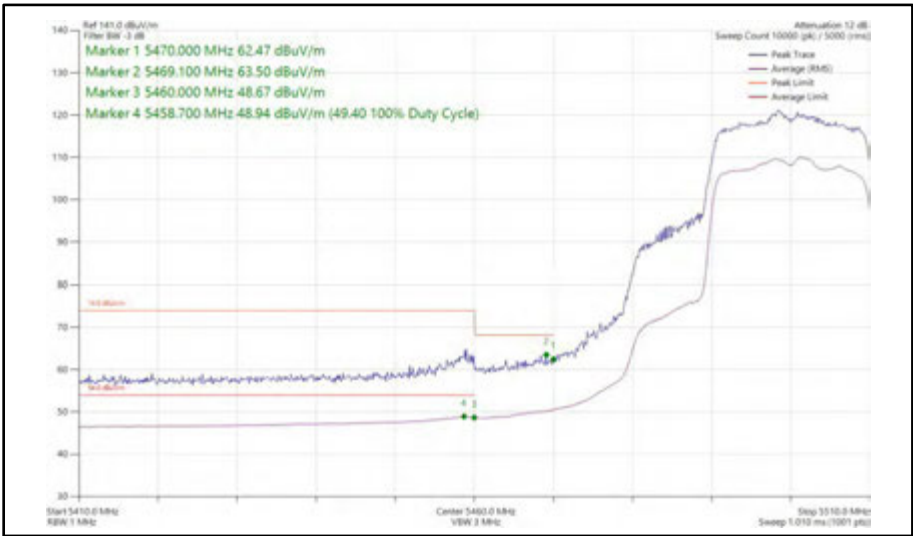
Figure 477 - 802.11ax HE20, SU, SDM, Core 0 + Core 1 - 5500 MHz Band Edge Frequency 5470 MHz
