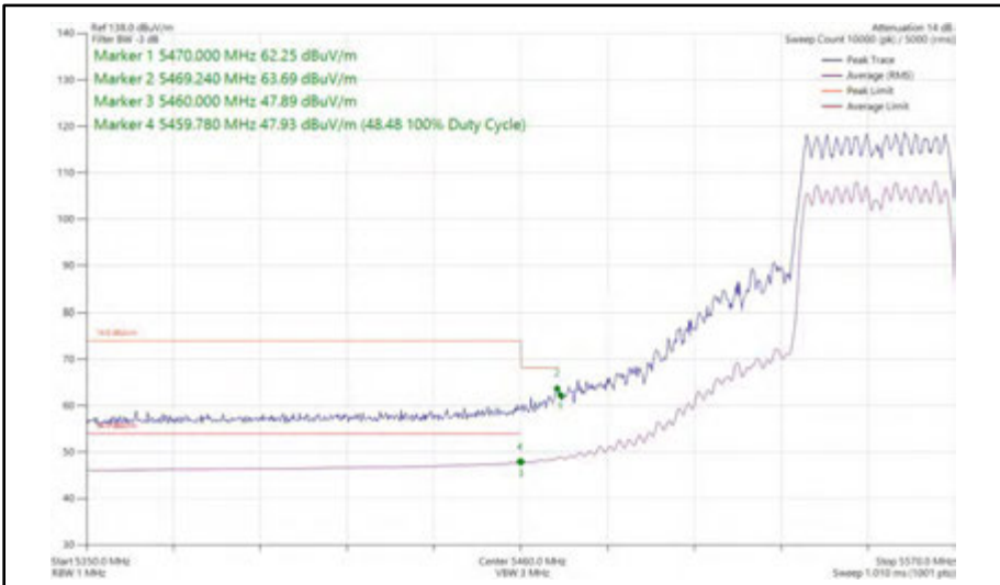
Figure 565 - 802.11ax HE40, SU, CDD, Core 0 + Core 1 - 5550 MHz Band Edge Frequency 5470 MHz
