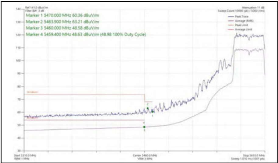
Figure 608 - 802.11ac VHT40, TxBF, Core 0 + Core 1 - 5590 MHz Band Edge Frequency 5470 MHz
