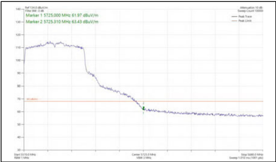
Figure 620 - 802.11ac VHT80, SISO, Core 0 - 5610 MHz Band Edge Frequency 5725 MHz
