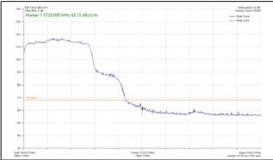
Figure 493 - 802.11ax HE20, SU, SDM, Core 0 + Core 1 - 5700 MHz Band Edge Frequency 5725 MHz
