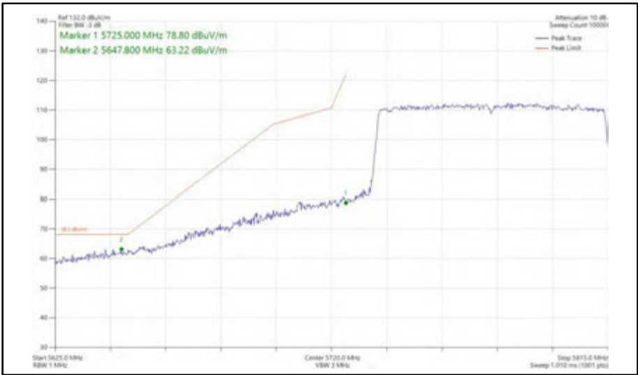
Figure 618 - 802.11ax HE80, SU, SISO, Core 0 - 5775 MHz Band Edge Frequency 5725 MHz
