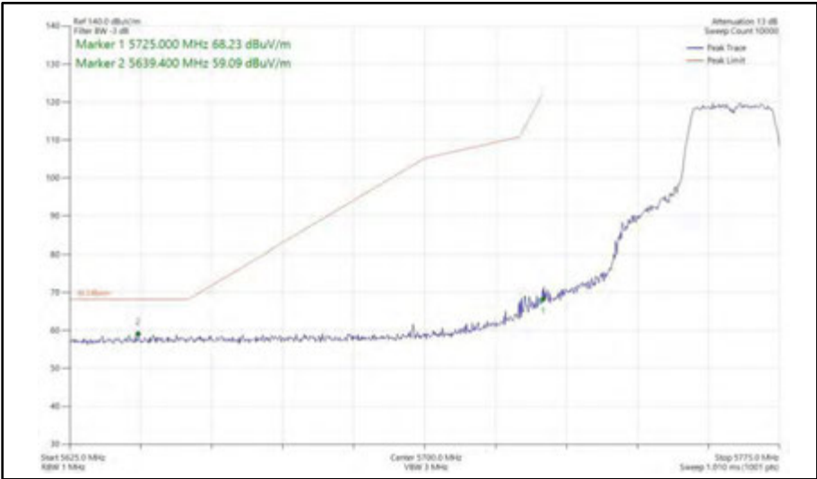
Figure 420 - 802.11n HT20, SISO, Core 1 - 5765 MHz Band Edge Frequency 5725 MHz
