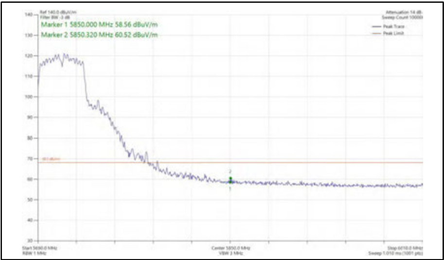
Figure 577 - 802.11n HT40, CDD, Core 0 + Core 1 - 5710 MHz Band Edge Frequency 5850 MHz
