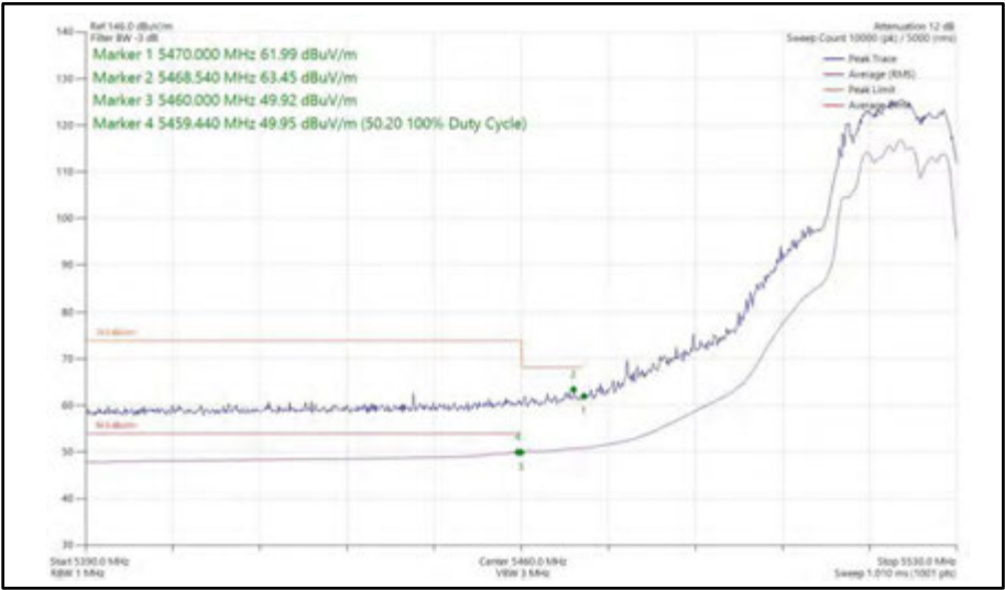
Figure 504 - 802.11ac VHT20, TxBF, Core 0 + Core 1 - 5520 MHz Band Edge Frequency 5470 MHz
