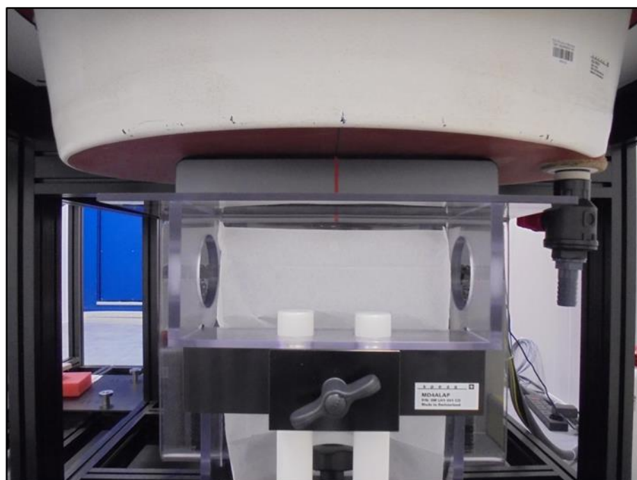
Figure 6 - SAR - Bottom Position
