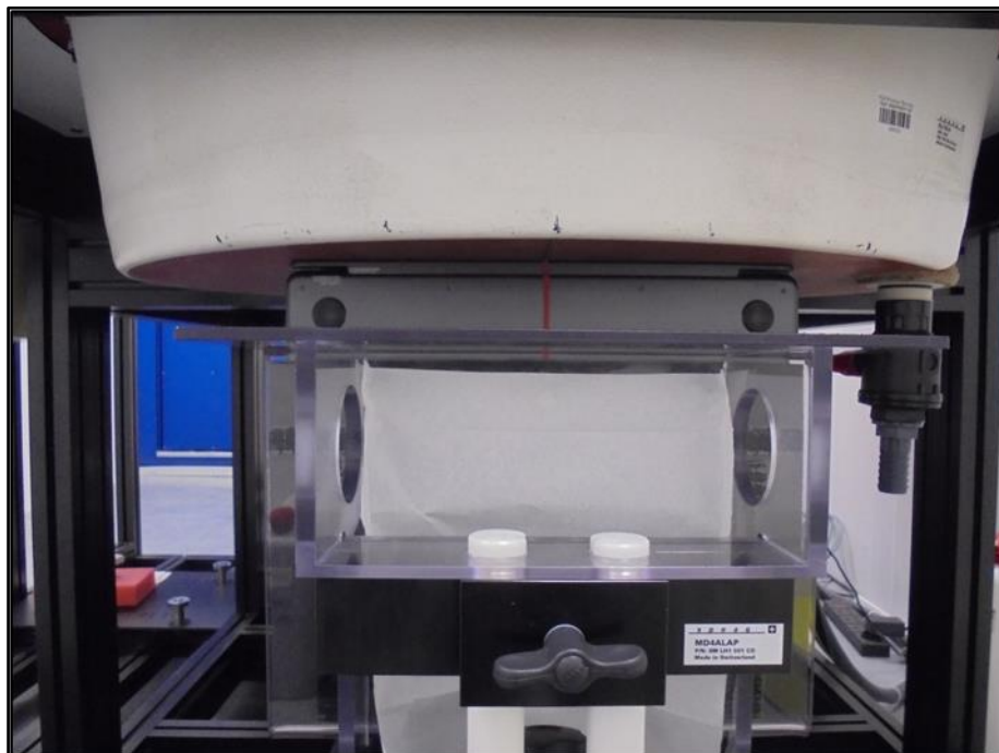
Figure 5 - SAR – Rear of Display Position
