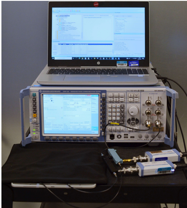
Test Setup Photo 5 – Conducted Test Setup (Figure 5-1d)
