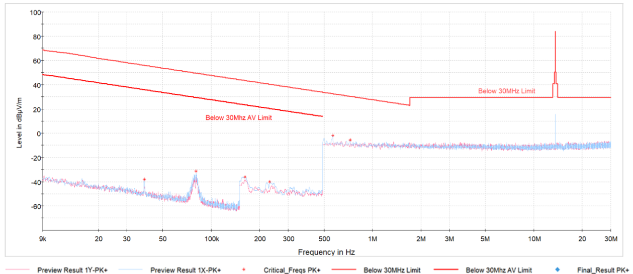
Plot 7-2. Radiated Spurious Plot 9kHz – 30MHz (Charging Rate 2.6C, with AC/DC Adapter)
