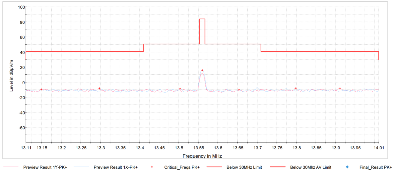
Plot 7-1. In Band Radiated Spurious Emissions (Charging Rate 2.6C, with AC/DC Adapter)
