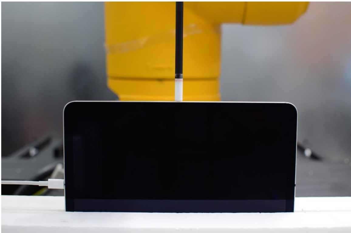
Near Field Power Density Test Setup 19: Left Edge at 2mm – Antenna 1b/3a/3c
