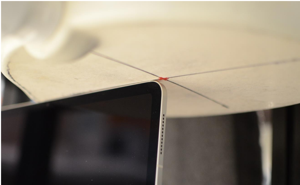
SAR Test Setup Photo 6: Body, Right Edge at 0.0 cm – Antenna 1a/1b/2a/2b
