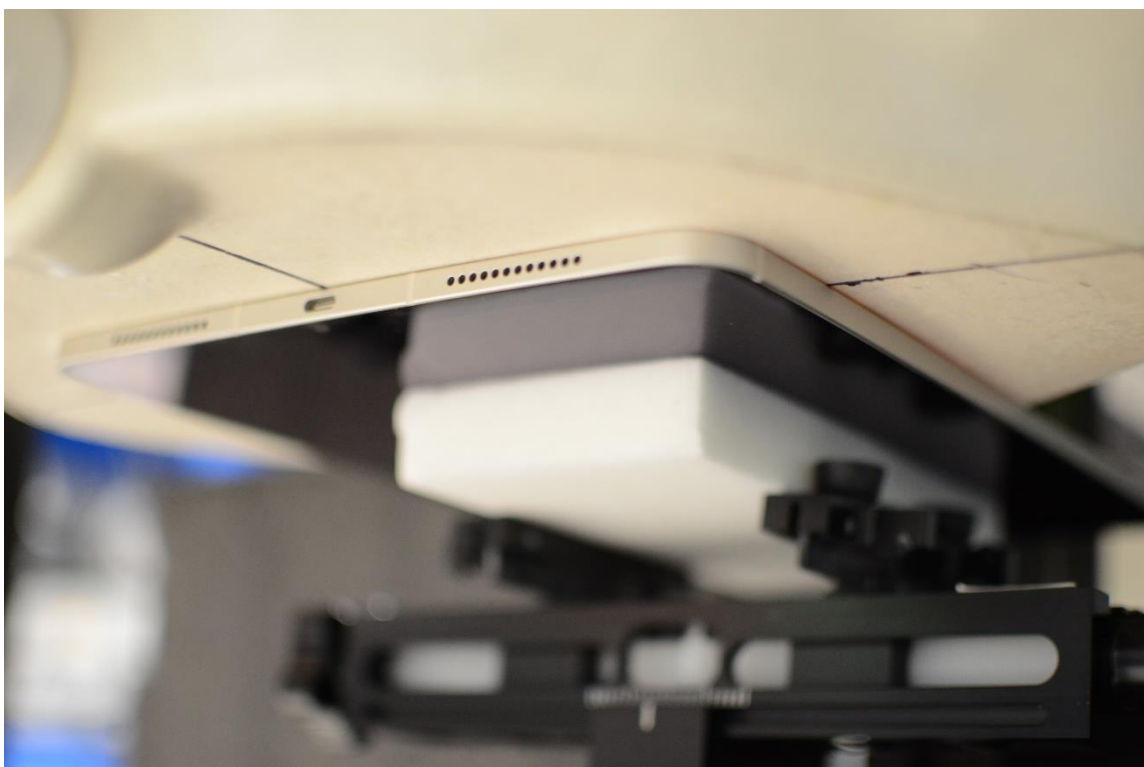
SAR Test Setup Photo 2: Body, Back Side at 0.0 cm – Antenna 1a/1b/2a/2b
