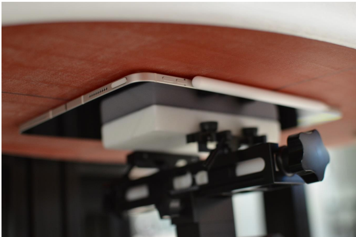
Wireless Power Transfer (wPT) Test Setup Photo 9: Body, Back Side at 0.0 cm
