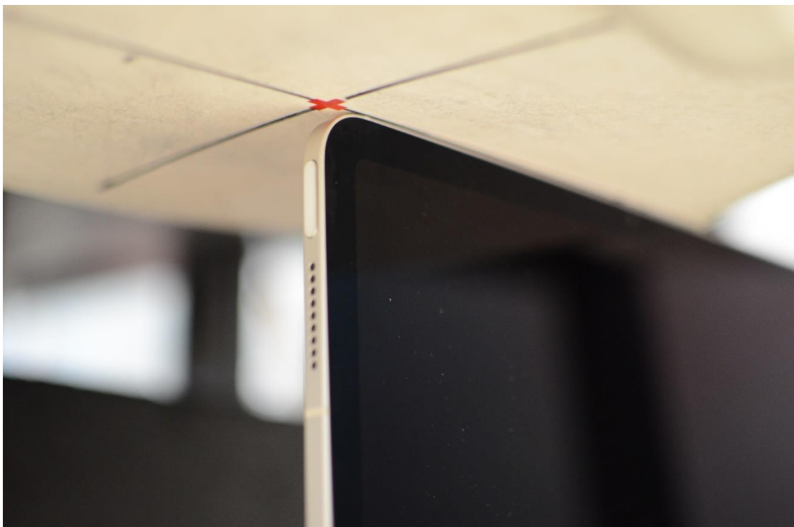
SAR Test Setup Photo 5: Body, Right Edge at 0.0 cm – Antenna 3a/3b/3c/4
