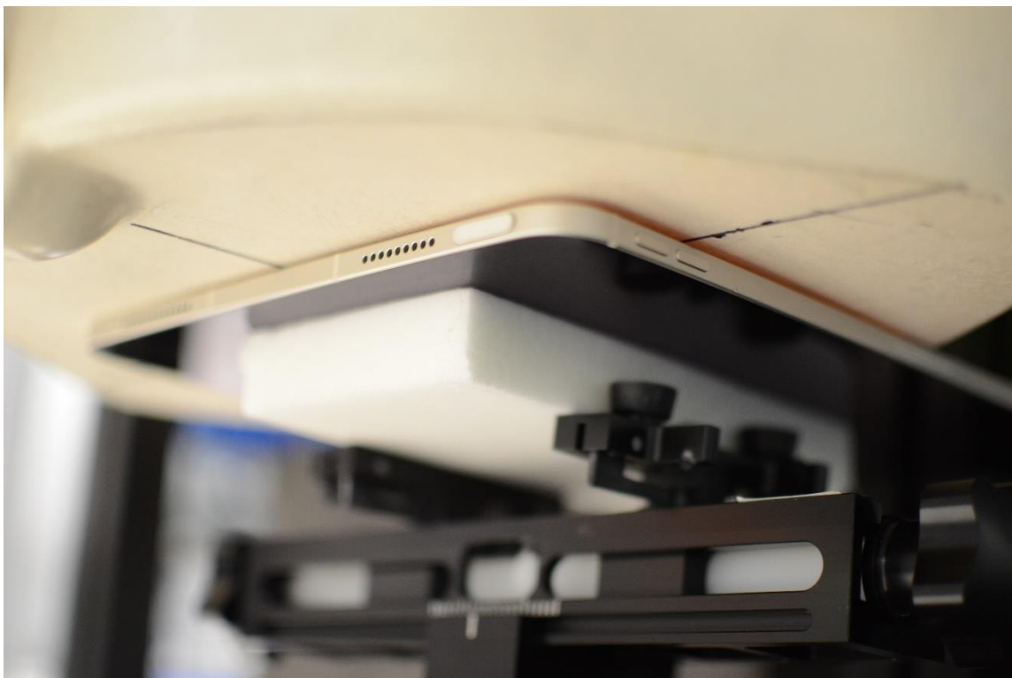
SAR Test Setup Photo 1: Body, Back Side at 0.0 cm – Antenna 3a/3b/3c/4
