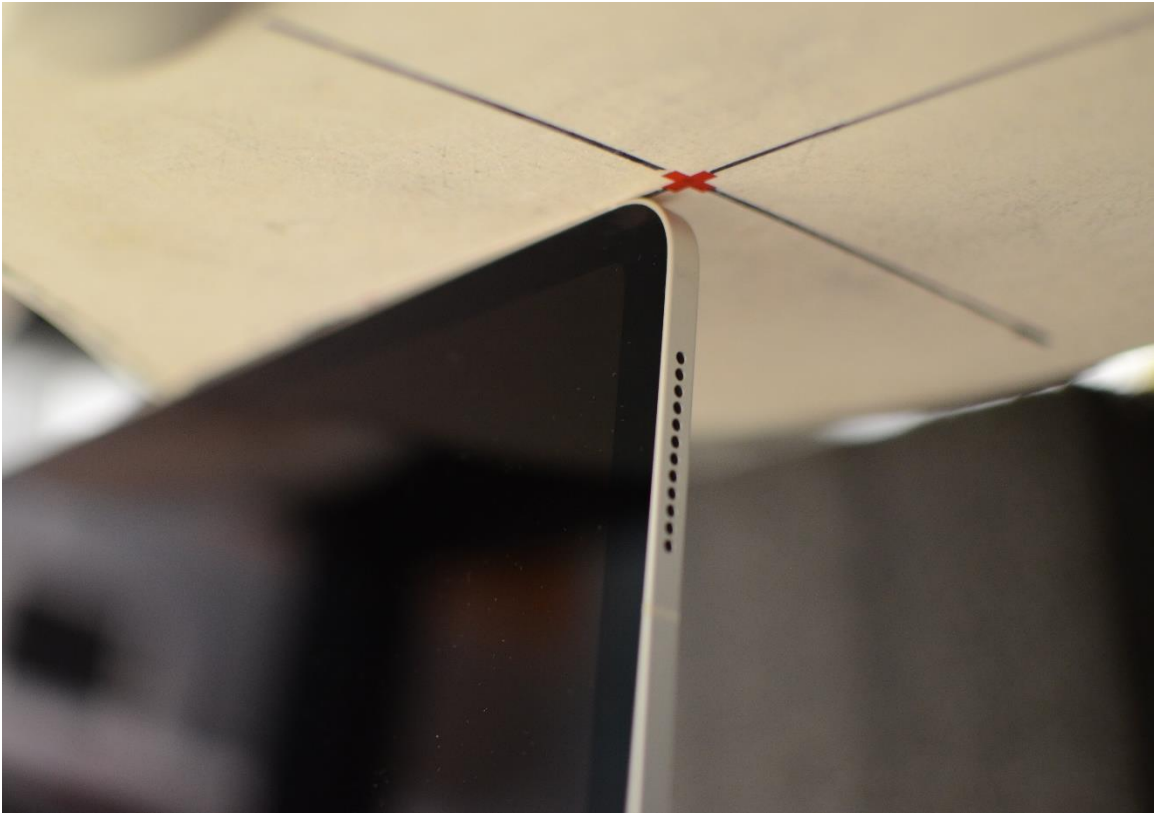
SAR Test Setup Photo 7: Body, Left Edge at 0.0 cm – Antenna 3a/3b/3c/4
