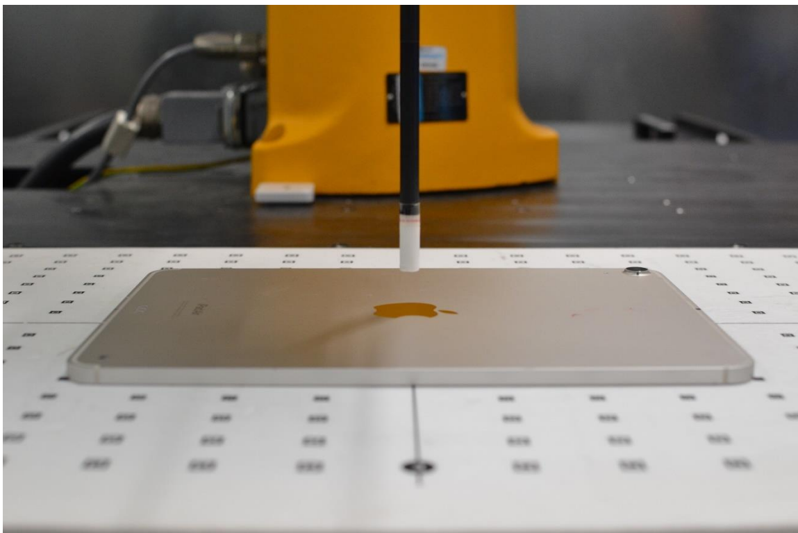
Near Field Power Density Test Setup 15: Back Side at 9mm – Antenna 3a
