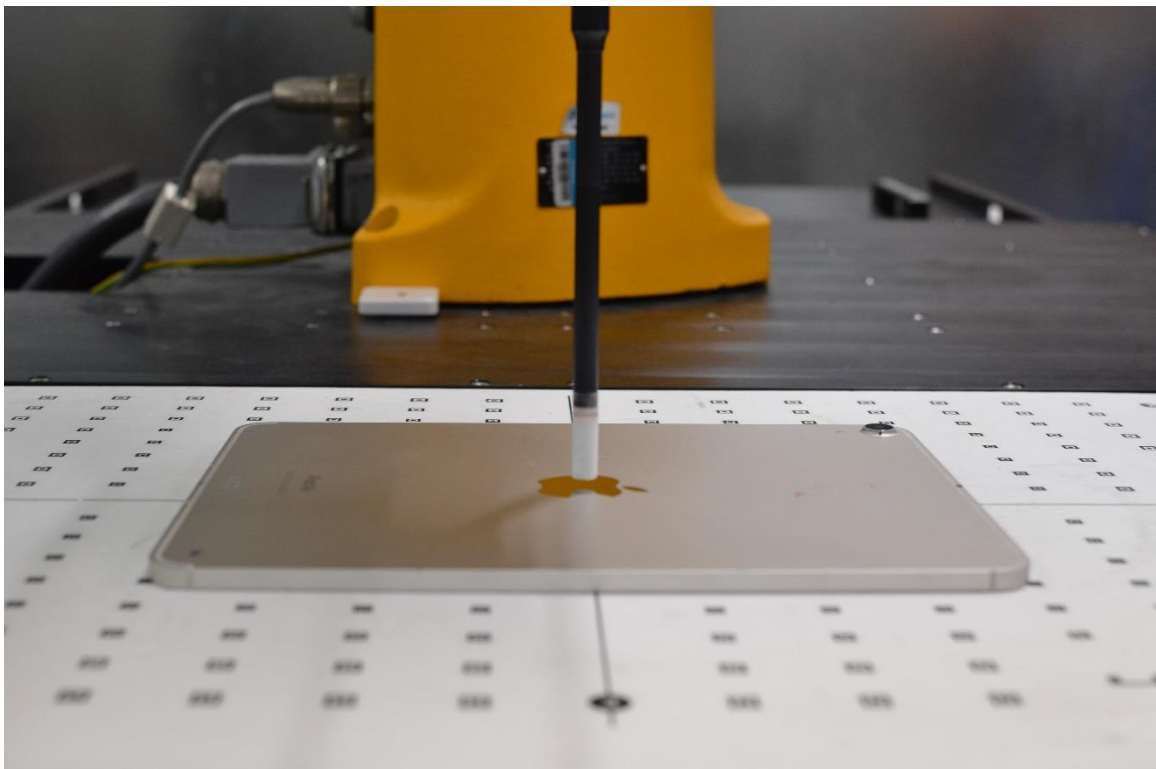
Near Field Power Density Test Setup 14: Back Side at 2mm – Antenna 1b/3a/3c
