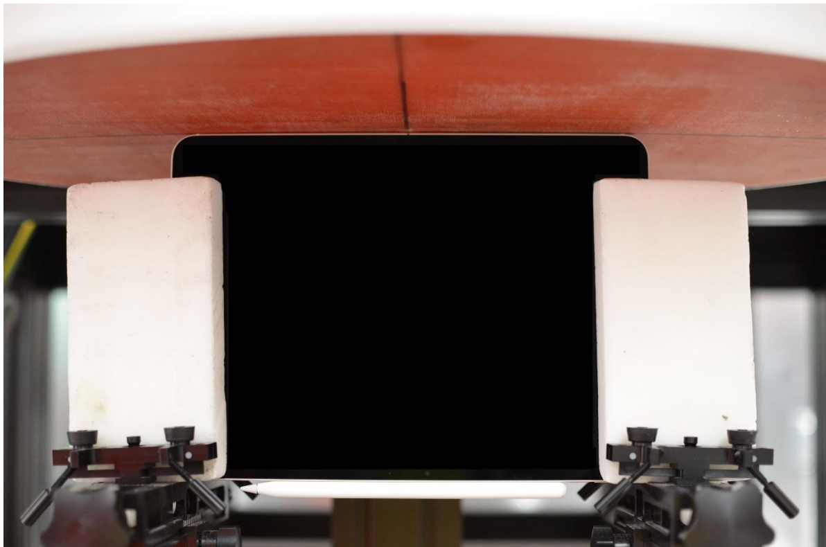
Wireless Power Transfer (wPT) Test Setup Photo 13: Body, Left Edge at 0.0 cm
