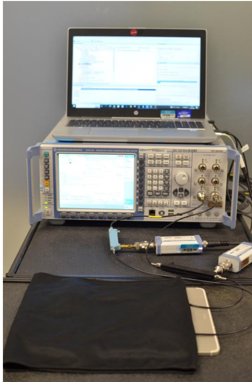
Test Setup Photo 5 – Conducted Test Setup (Figure 5-1d)
