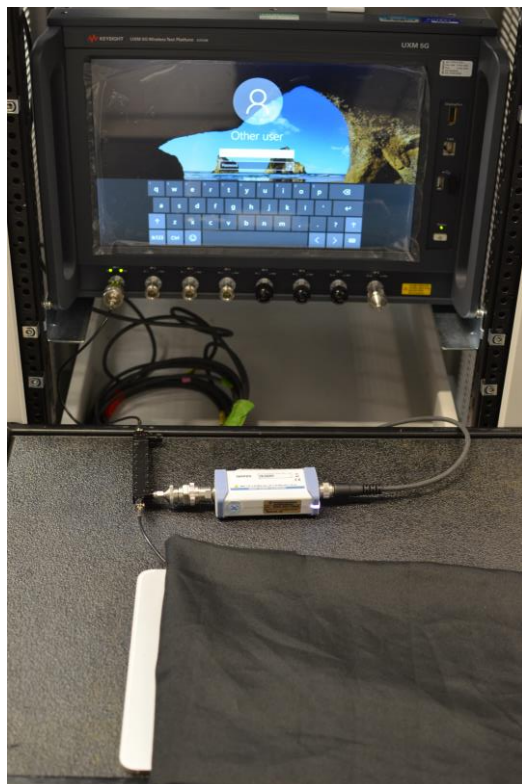
Test Setup Photo 2 – Conducted Test Setup (Figure 5-1a)
