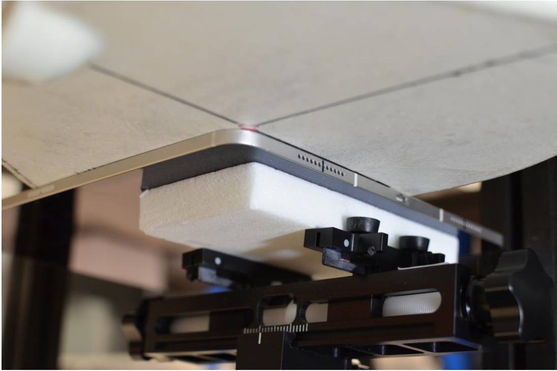
Test Setup Photo 7 – Body, Back Side at 0.0 cm – Antenna 2
