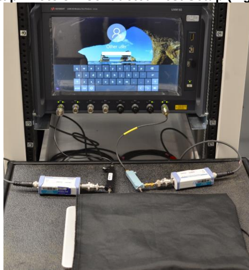
Test Setup Photo 4 – Conducted Test Setup (Figure 5-1c)
