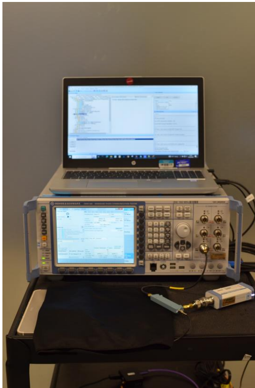
Test Setup Photo 1 – Conducted Test Setup (Figure 5-1a)
