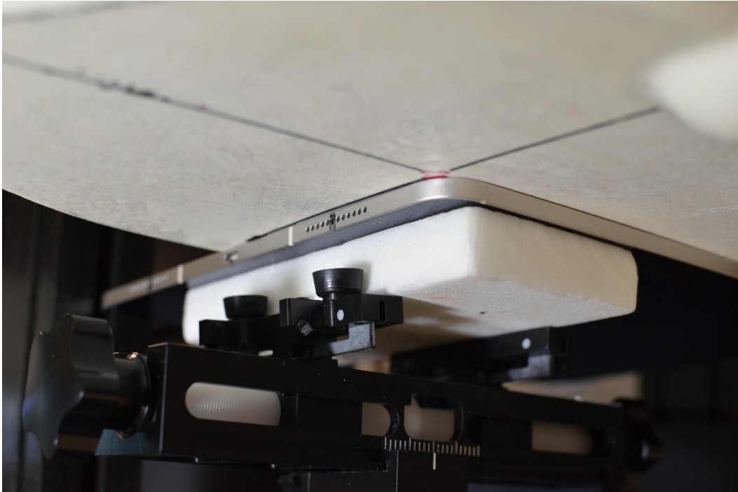
Test Setup Photo 9 – Body, Back Side at 0.0 cm – Antenna 1A
