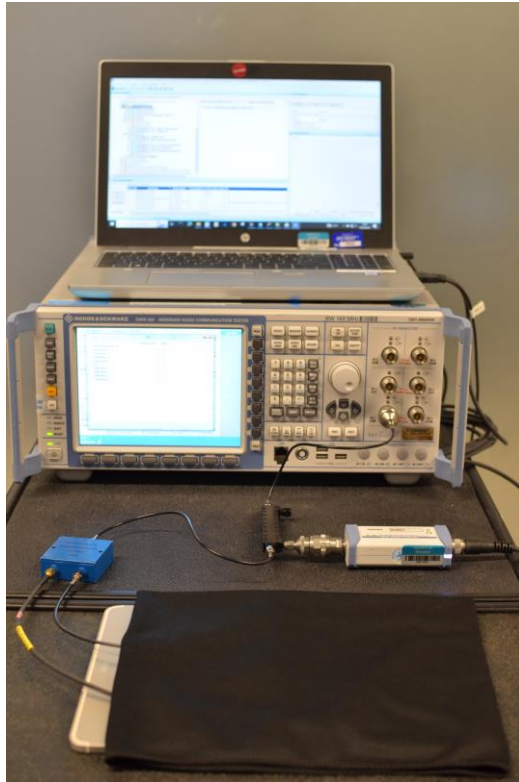
Test Setup Photo 3 – Conducted Test Setup (Figure 5-1b)
