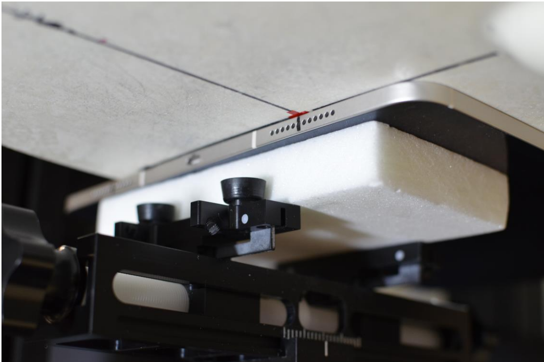
Test Setup Photo 8 – Body, Back Side at 0.0 cm – Antenna 1B
