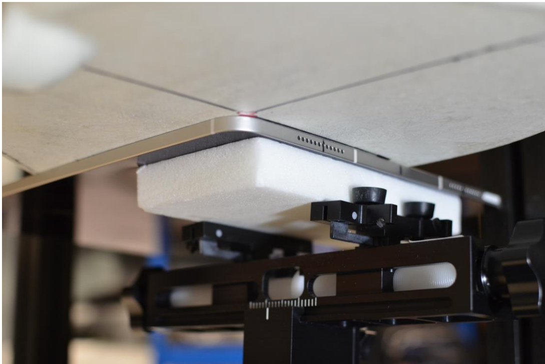
Test Setup Photo 6 – Body, Back Side at 0.0 cm – Antenna 4
