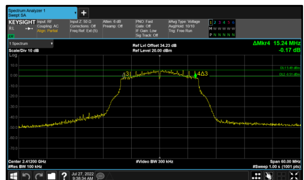
Figure 36 - 802.11g Maximum 6 dB EBW
