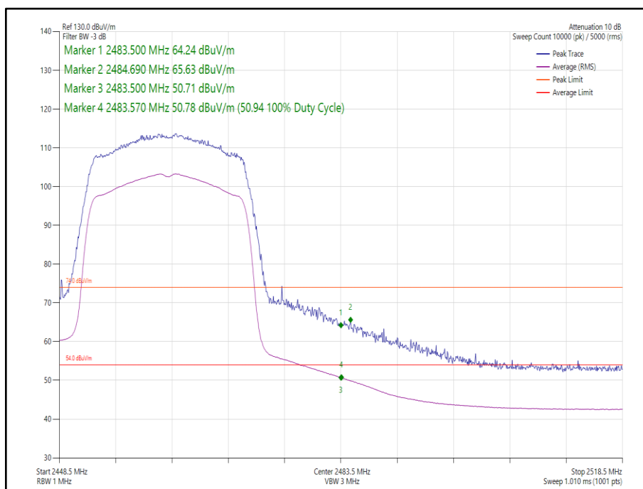
Figure 15 - 802.11ax HE20, Core 0, SU - 2462 MHz, Band Edge Frequency 2483.5 MHz
