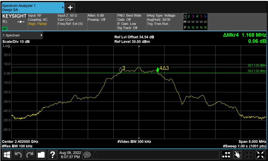
Figure 108 - BT Core 2 (C) 2402 MHz (CH37) 6 dB Bandwidth
