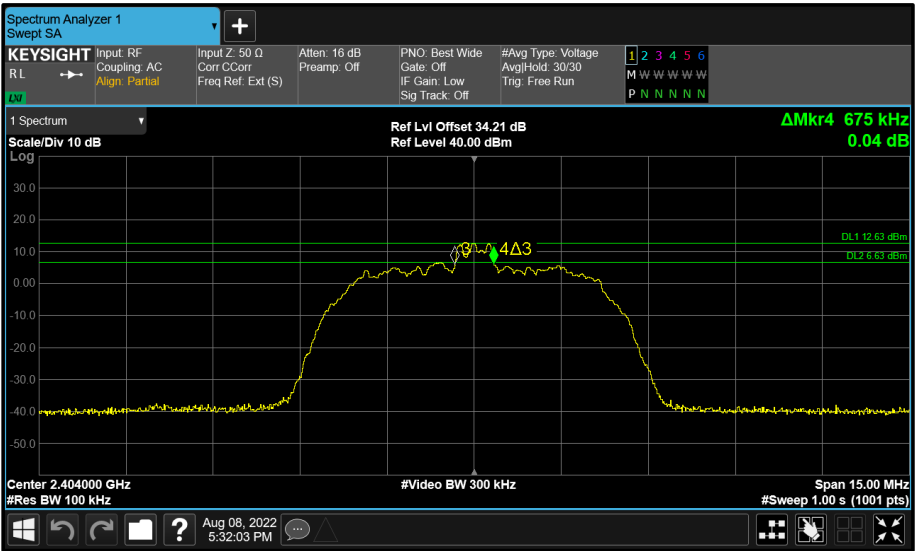
Figure 48 - BT Core 1 (B) 2404 MHz (CH2) 6 dB Bandwidth
