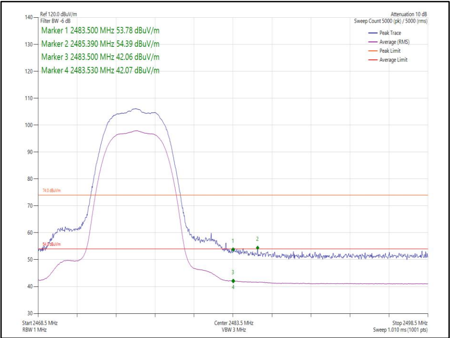
Figure 34 Core 1- Static - GFSK/8DH5 - 2476 MHz - Band Edge Frequency 2483.5 MHz
