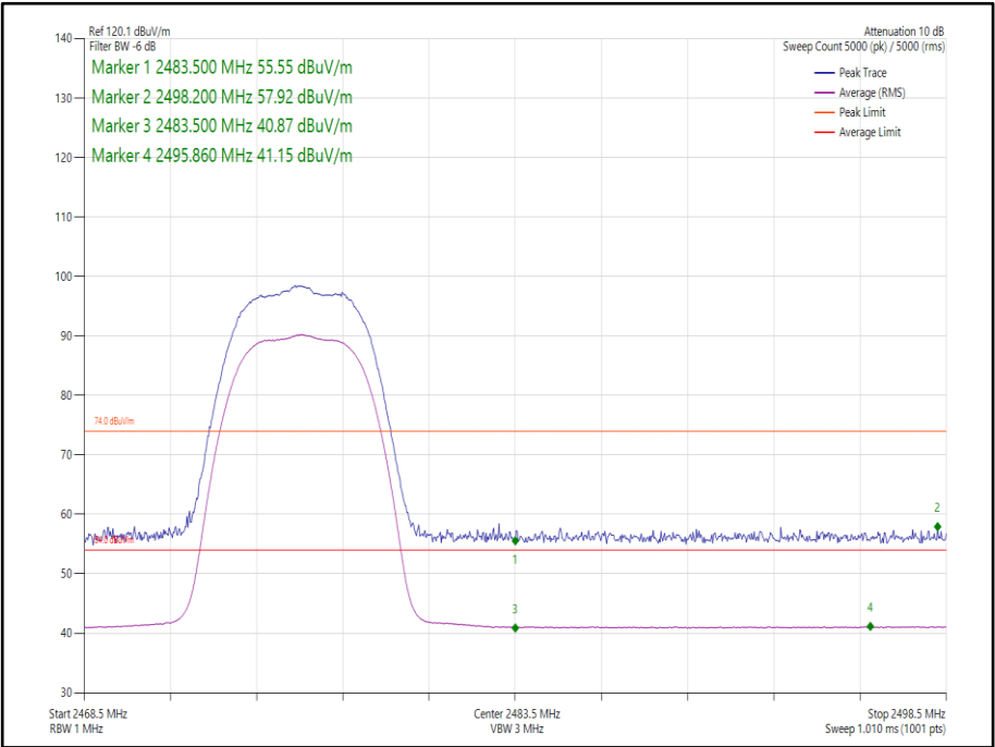
Figure 32 Core 1- Static - GFSK/8DH5 - 2476 MHz - Band Edge Frequency 2483.5 MHz
