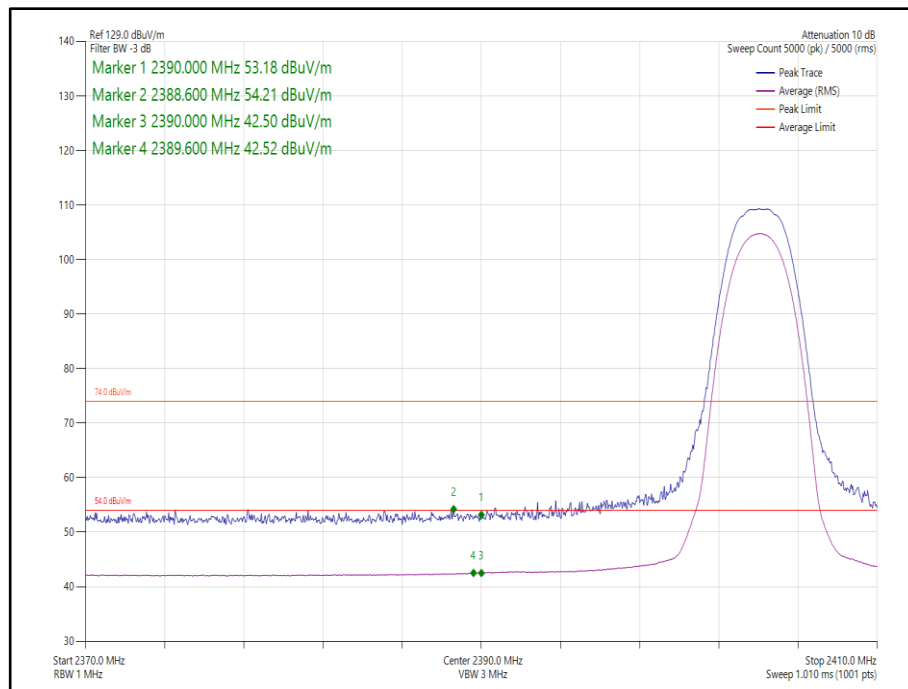
Figure 23 Core 1- Static - GFSK/4DH5 - 2404 MHz - Band Edge Frequency 2390.0 MHz
