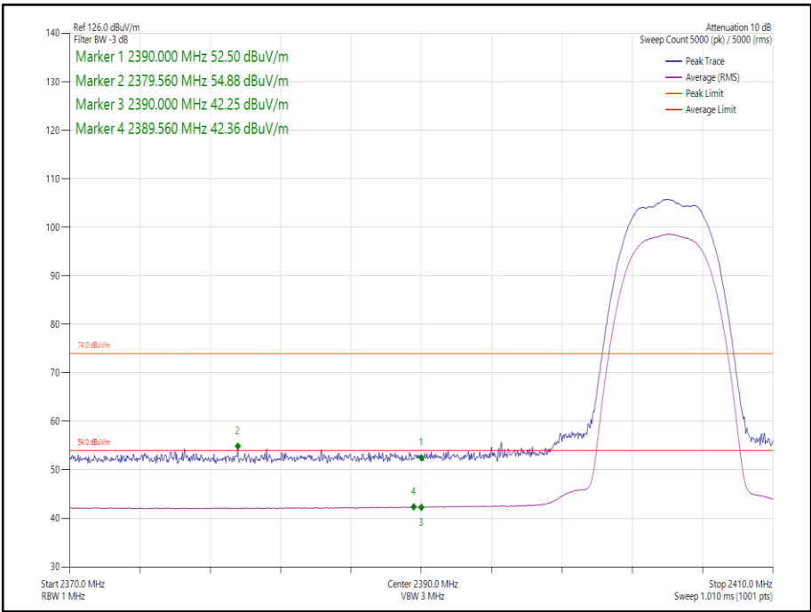
Figure 31 Core 1- Static - GFSK/8DH5 - 2404 MHz - Band Edge Frequency 2390.0 MHz
