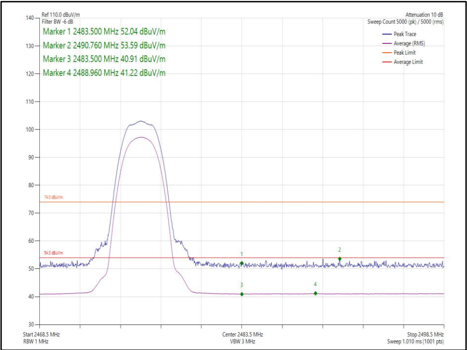
Figure 28 Core 0-1- Static - GFSK/4DH5 - 2476 MHz - Band Edge Frequency 2483.5 MHz
