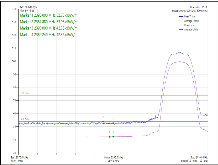
Figure 37 Core 0-1- Static - GFSK/8DH5 - 2404 MHz - Band Edge Frequency 2390.0 MHz
