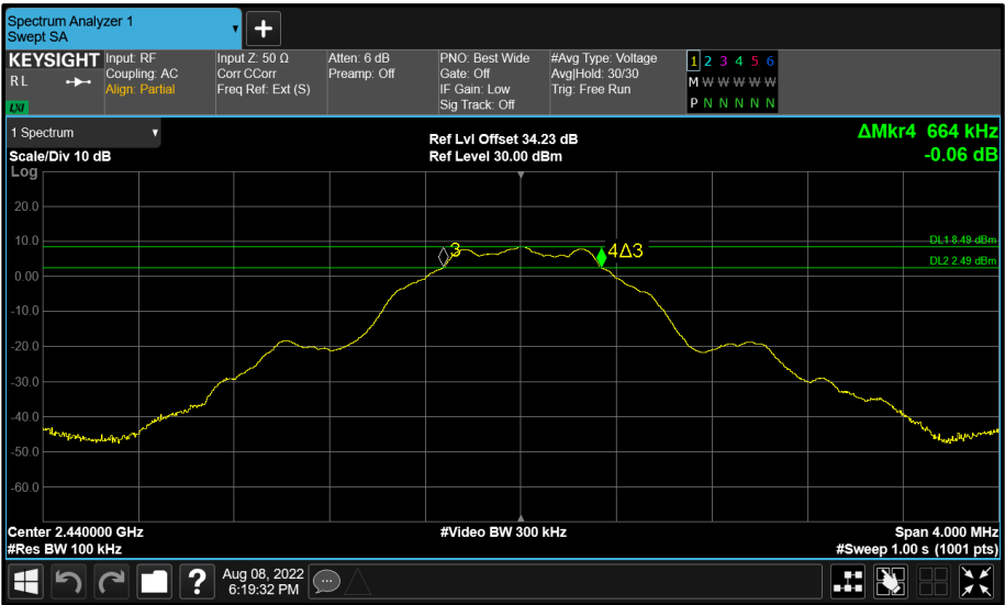
Figure 56 - BT Core 1 (B) 2440 MHz (CH17) 6 dB Bandwidth
