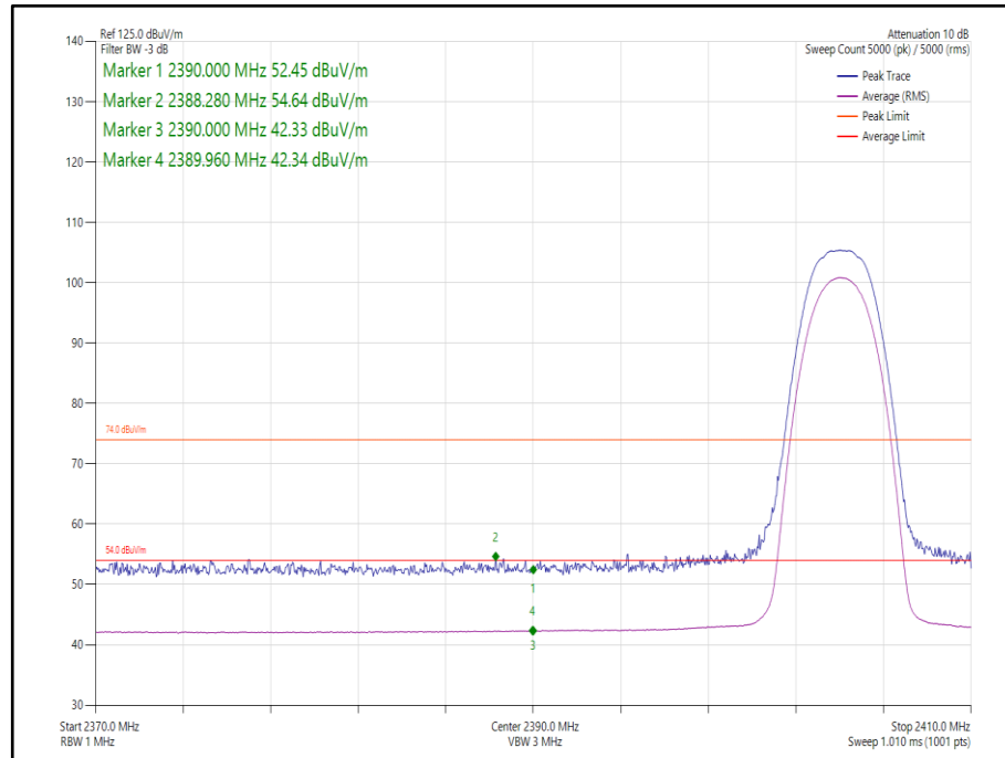
Figure 21 Core 1- Static - GFSK/4DH5 - 2404 MHz - Band Edge Frequency 2390.0 MHz
