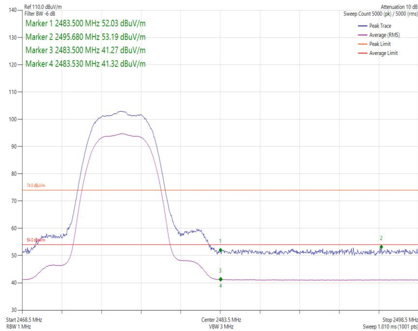
Figure 38 Core 0-1- Static - GFSK/8DH5 - 2476 MHz - Band Edge Frequency 2483.5 MHz
