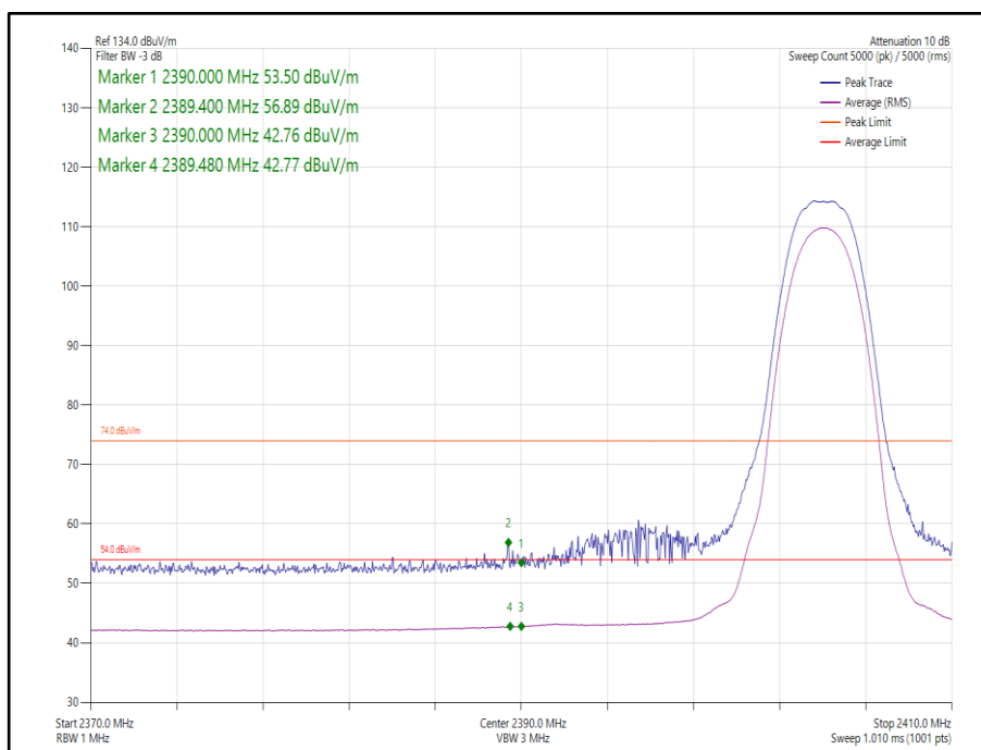
Figure 29 Core 0-1- Static - GFSK/4DH5 - 2404 MHz - Band Edge Frequency 2390.0 MHz
