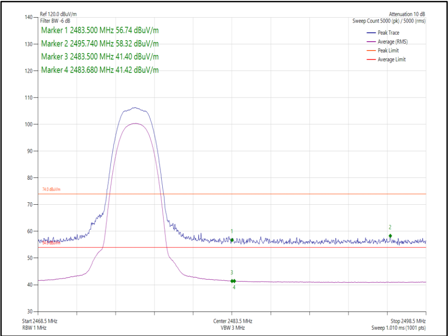
Figure 24 Core 1- Static - GFSK/4DH5 - 2476 MHz - Band Edge Frequency 2483.5 MHz
