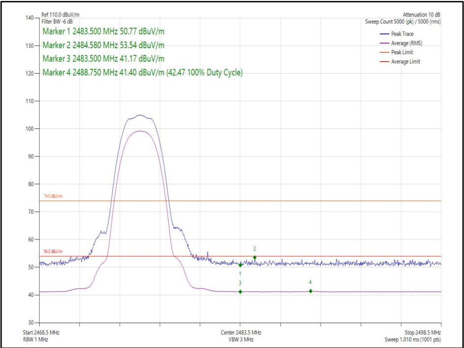
Figure 26 Core 2- Static - GFSK/4DH5 - 2476 MHz - Band Edge Frequency 2483.5 MHz
