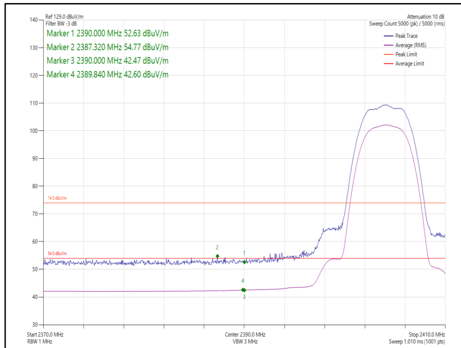
Figure 33 Core 1- Static - GFSK/8DH5 - 2404 MHz - Band Edge Frequency 2390.0 MHz
