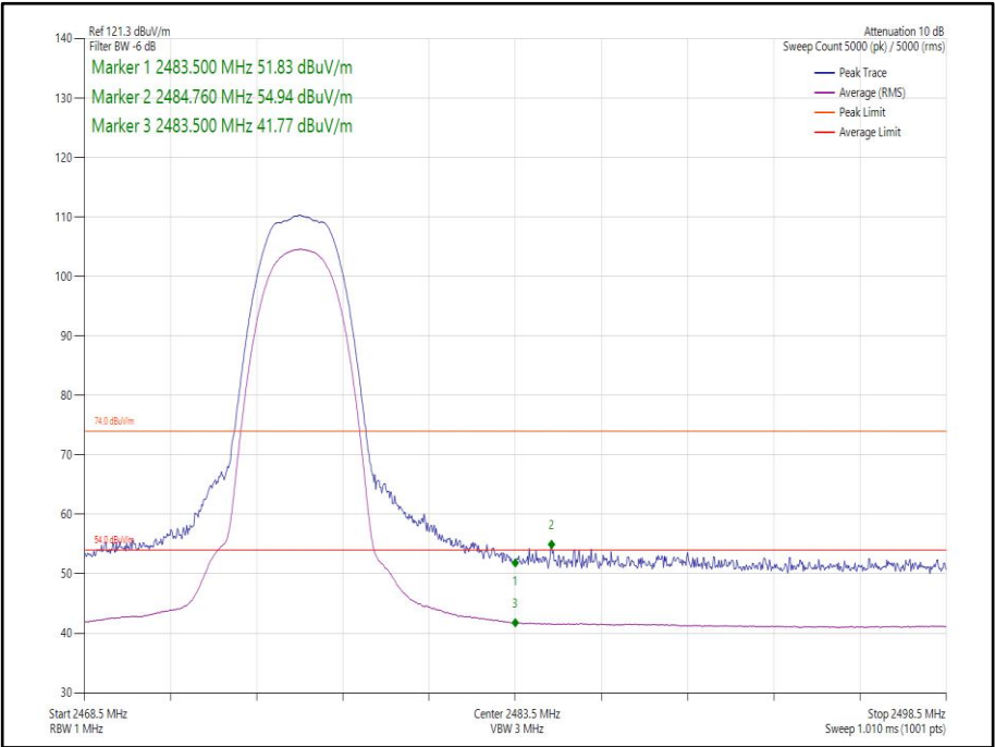
Figure 30 Core 0-1- Static - GFSK/4DH5 - 2476 MHz - Band Edge Frequency 2483.5 MHz
