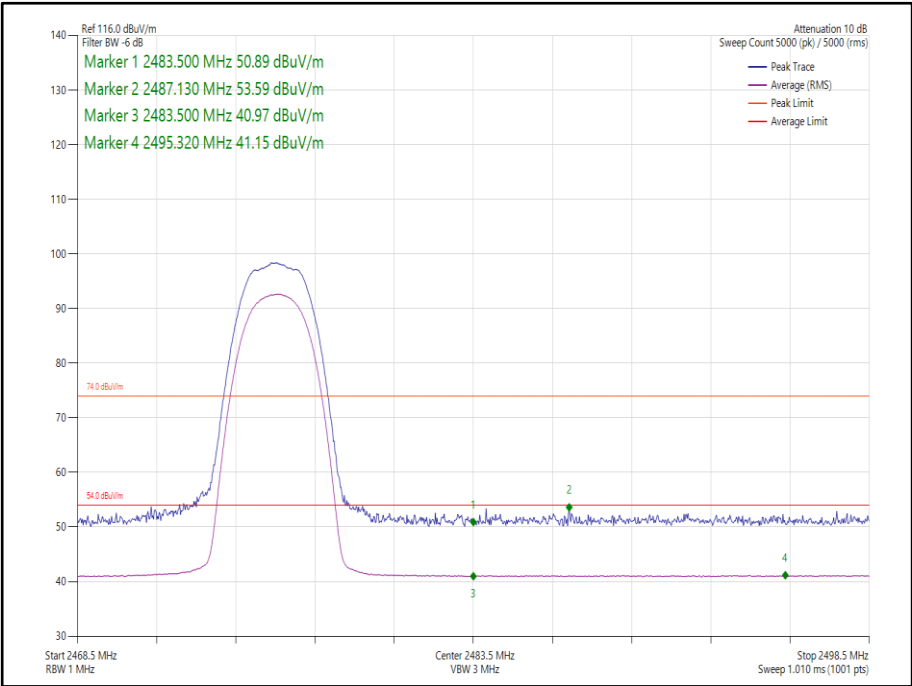
Figure 22 Core 1- Static - GFSK/4DH5 - 2476 MHz - Band Edge Frequency 2483.5 MHz
