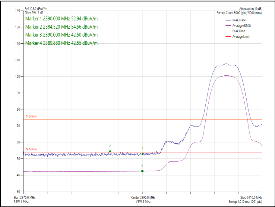
Figure 35 Core 2- Static - GFSK/4DH5 - 2404 MHz - Band Edge Frequency 2390.0 MHz
