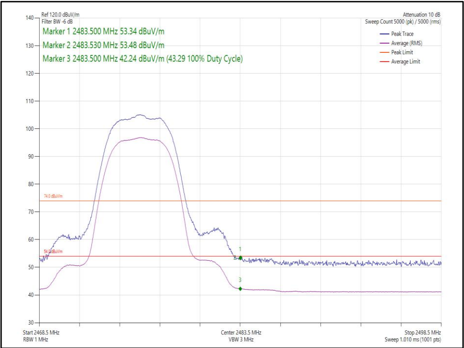
Figure 36 Core 2- Static - GFSK/4DH5 - 2476 MHz - Band Edge Frequency 2483.5 MHz
