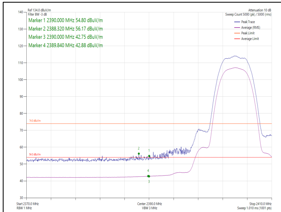
Figure 39 Core 0-1- Static - GFSK/8DH5 - 2404 MHz - Band Edge Frequency 2390.0 MHz
