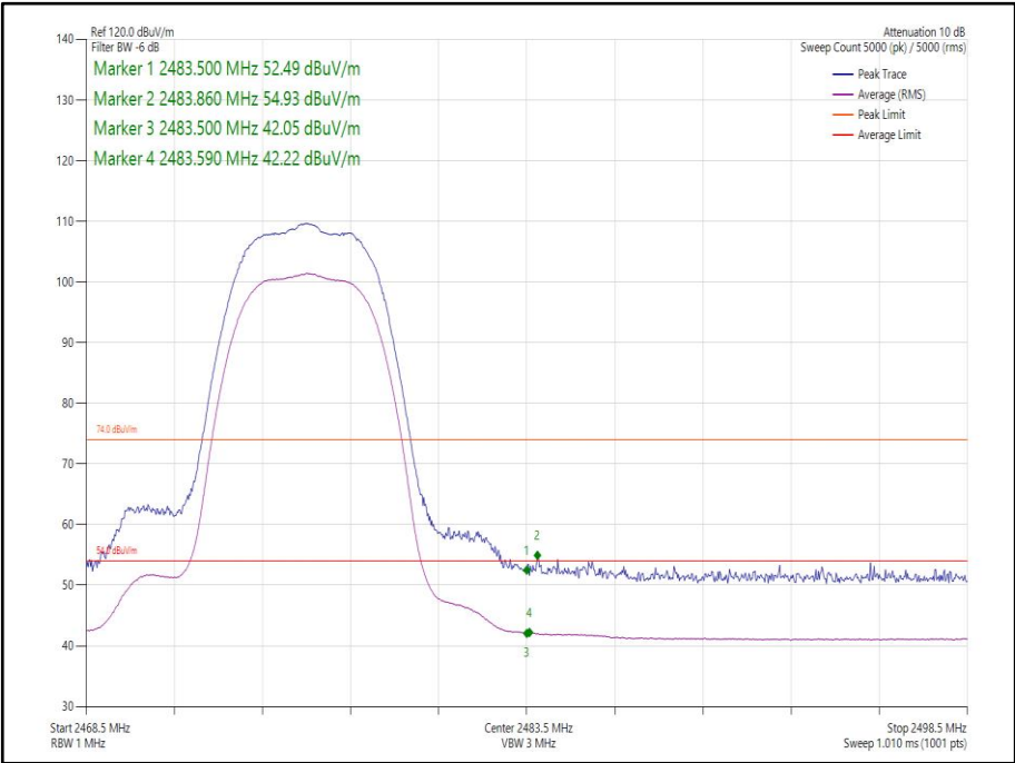
Figure 40 Core 0-1- Static - GFSK/8DH5 – 2476 MHz - Band Edge Frequency 2483.5 MHz
