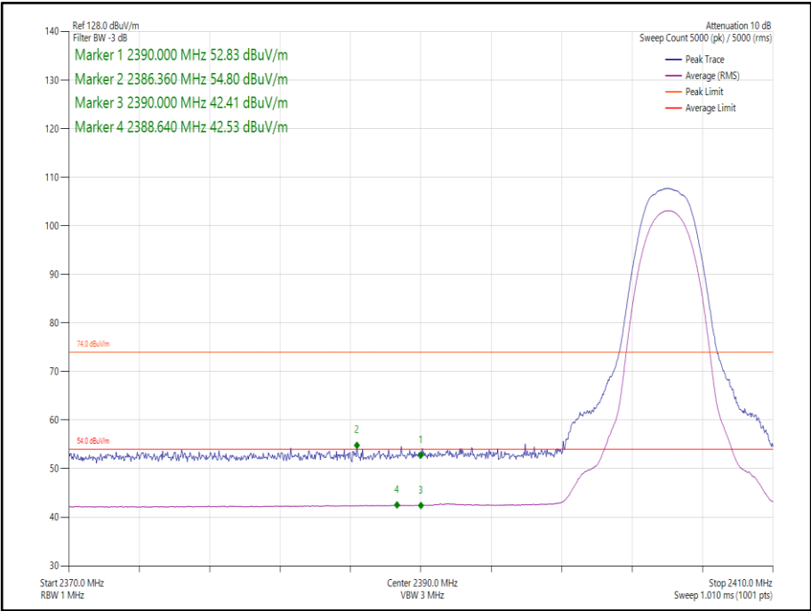
Figure 25 Core 2- Static - GFSK/4DH5 - 2404 MHz - Band Edge Frequency 2390.0 MHz
