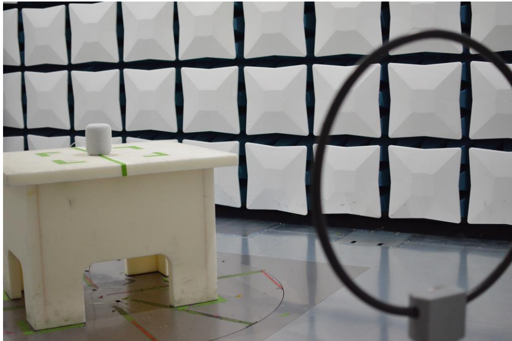
Figure 7: 9kHz-30MHz Test Setup (Front View)
