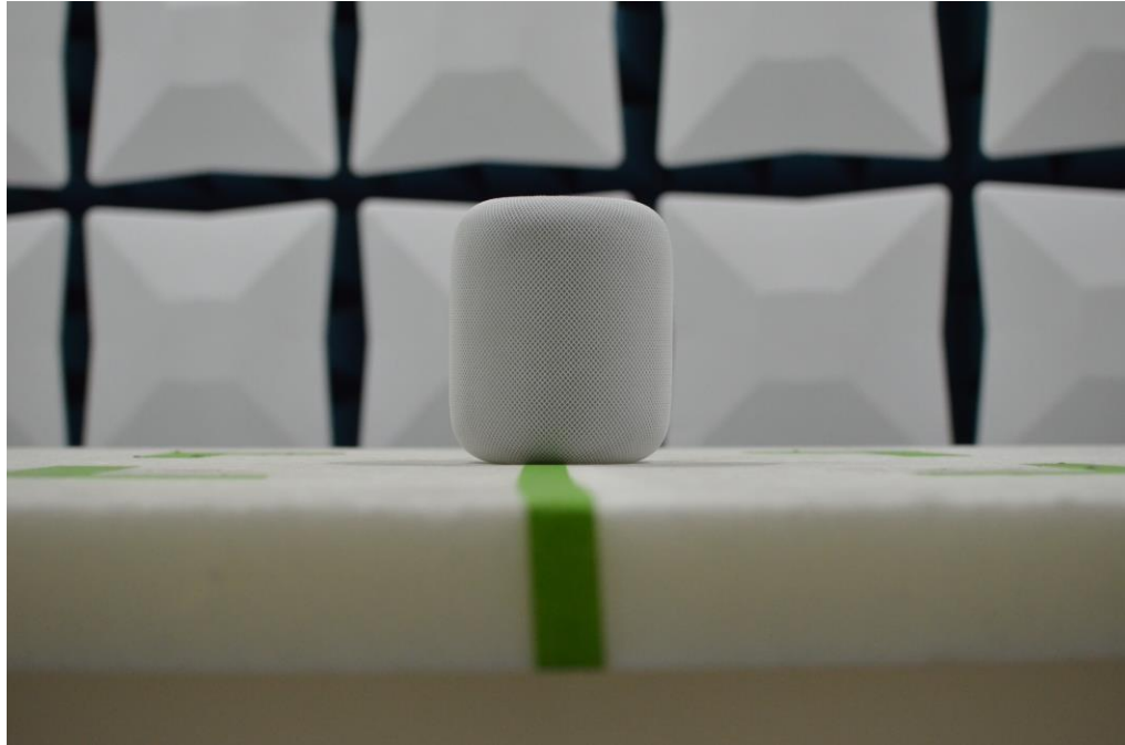
Figure 5: 30MHz-1GHz Test Setup (Front View)
