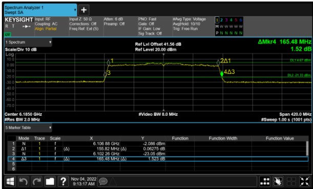
Figure 25 - 802.11ax HE160 SU Minimum 99% OBW
