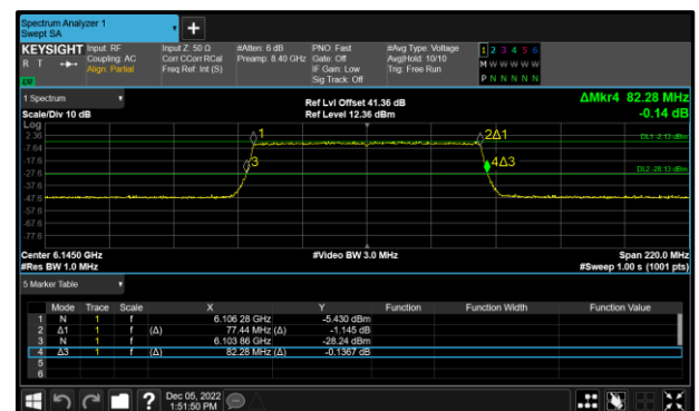
Figure 24 - 802.11ax HE80 SU Maximum 99% OBW
