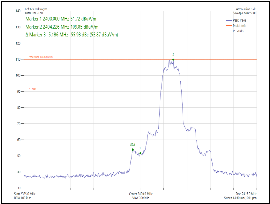
Figure 200 Core 0-1 - \pi/4 DQPSK/4-DH5 - 2404 MHz – Band Edge Frequency 2400.0 MHz
