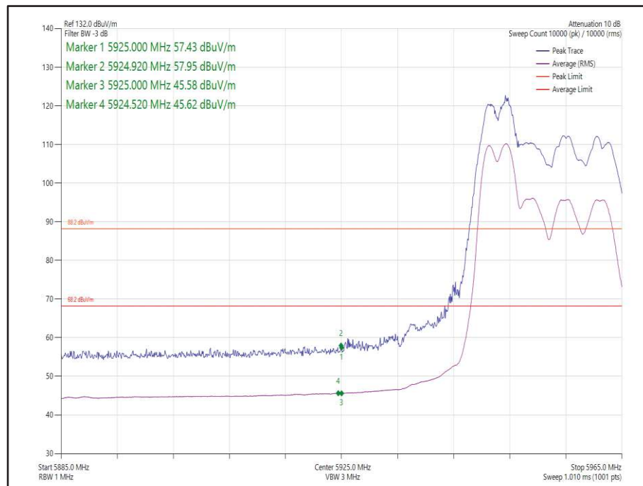
Figure 39 - 802.11ax HE20 SDM, Cores 0-1 52-37 - 5955 MHz Band Edge Frequency 5925 MHz
