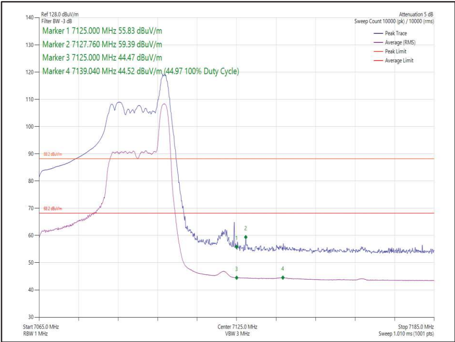
Figure 45 - 802.11ax HE40, Core 0, 26-17 - 7085 MHz Band Edge Frequency 7125 MHz
