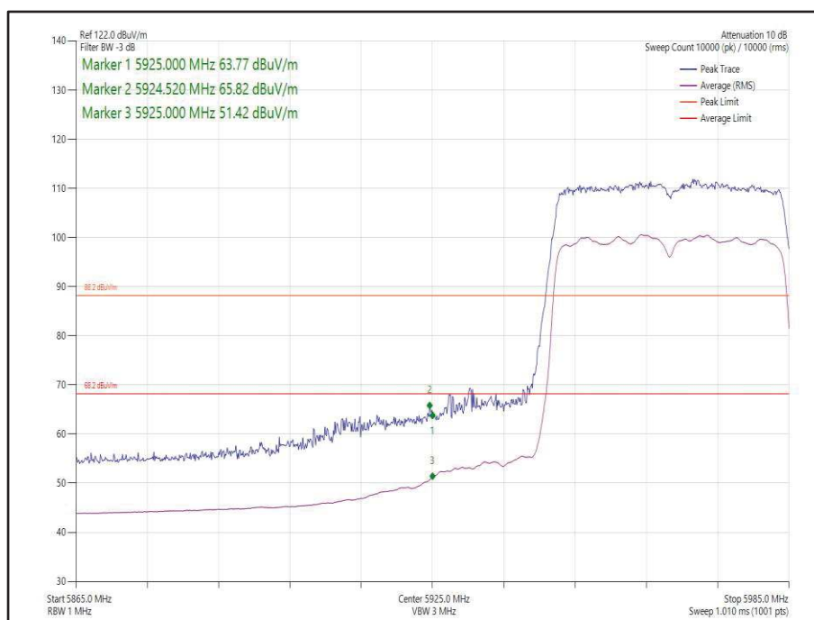
Figure 48 - 802.11ax HE40 SDM, Cores 0-1, SU - 5965 MHz Band Edge Frequency 5925 MHz
