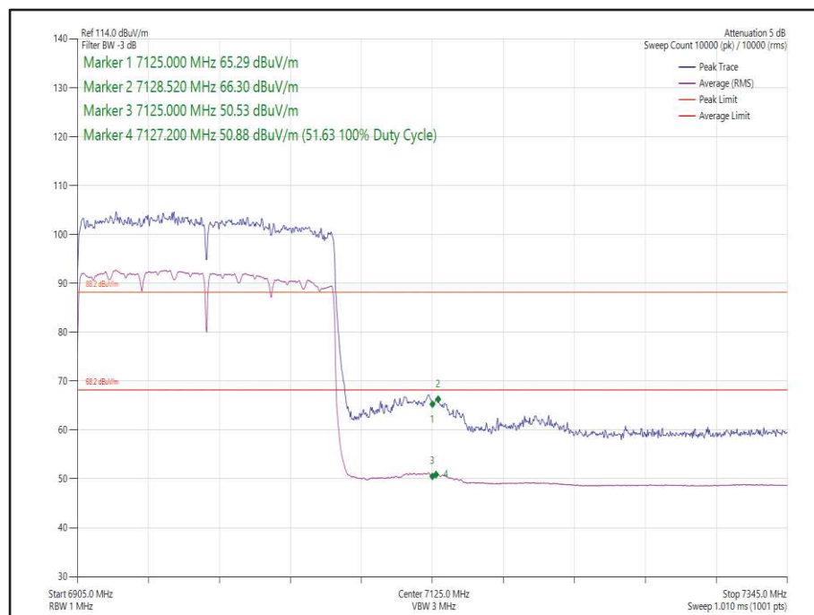
Figure 68 - 802.11ax HE160 Core 0 SU - 6985 MHz Band Edge Frequency 7125 MHz
