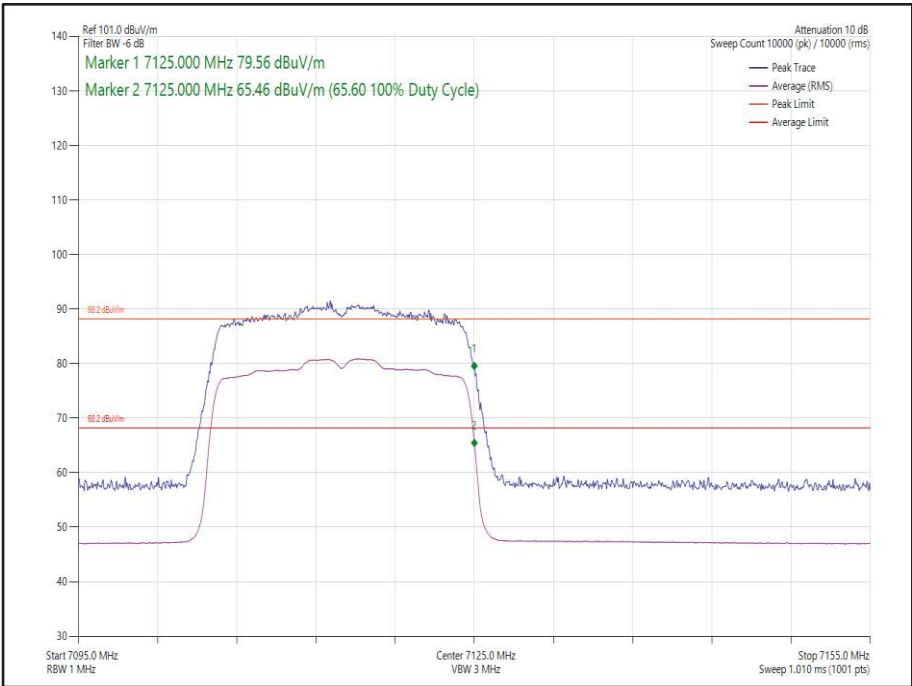
Figure 35- 802.11ax HE20, Core 0, SU - 7115 MHz, Band Edge Frequency 7125 MHz
