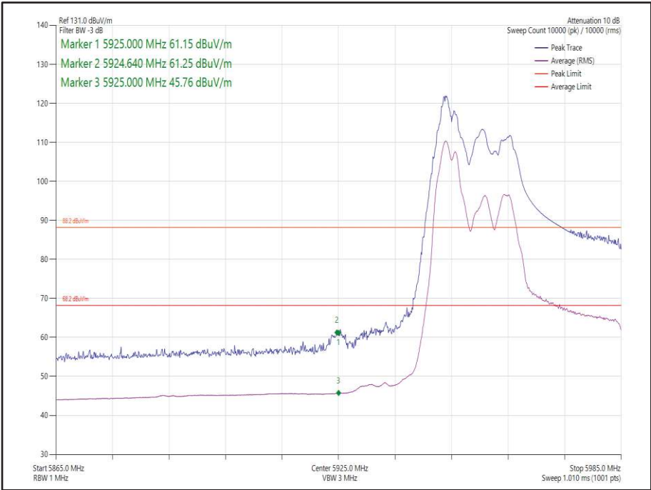
Figure 49 - 802.11ax HE40 SDM, Cores 0-1, 52-37 - 5965 MHz Band Edge Frequency 5925 MHz
