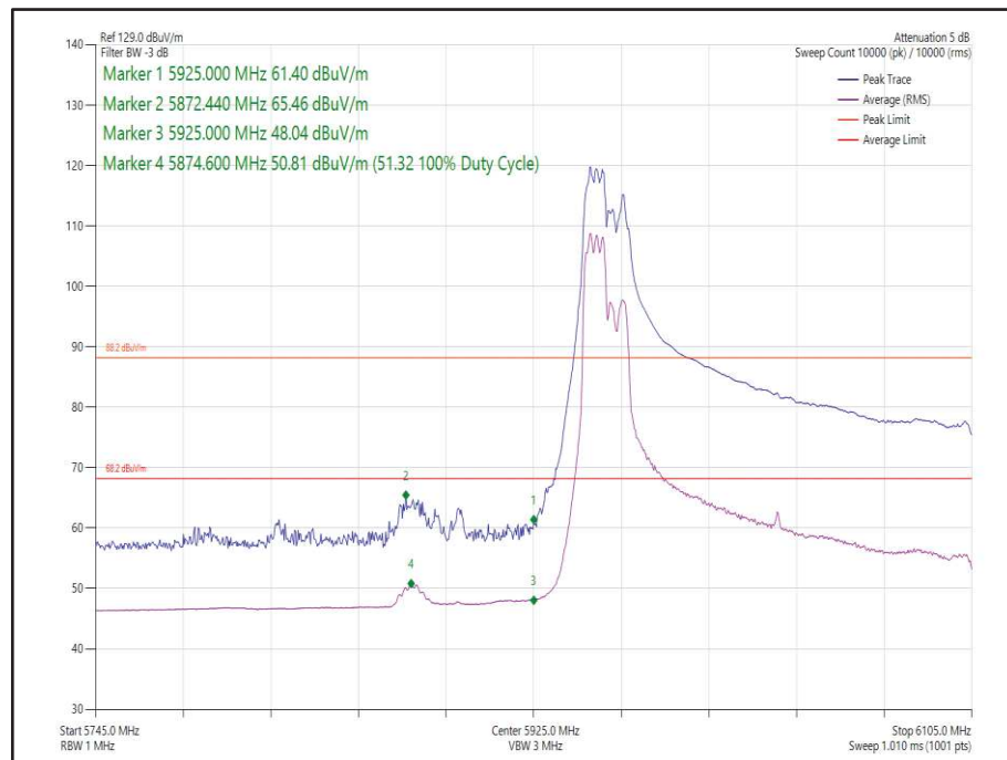
Figure 71 - 802.11ax HE160 CDD, Cores 0-1, 106-53 - 6025 MHz Band Edge Frequency 5925 MHz
