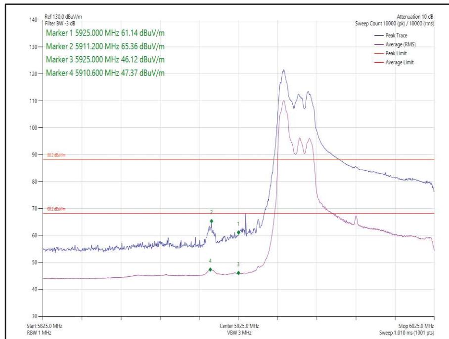
Figure 61 - 802.11ax HE80 SDM, Cores 0-1, 52-37 - 5985 MHz Band Edge Frequency 5925 MHz
