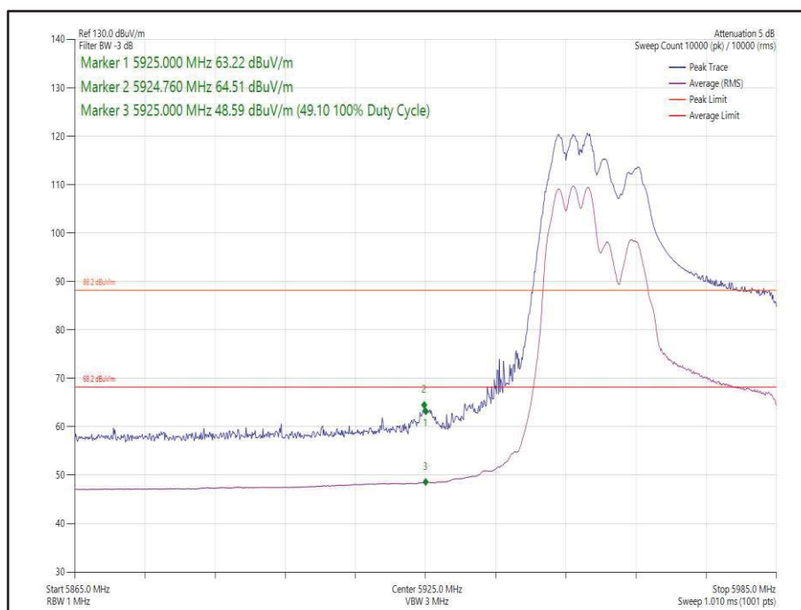
Figure 47 - 802.11ax HE40 CDD, Cores 0-1, 106-53 - 5965 MHz Band Edge Frequency 5925 MHz
