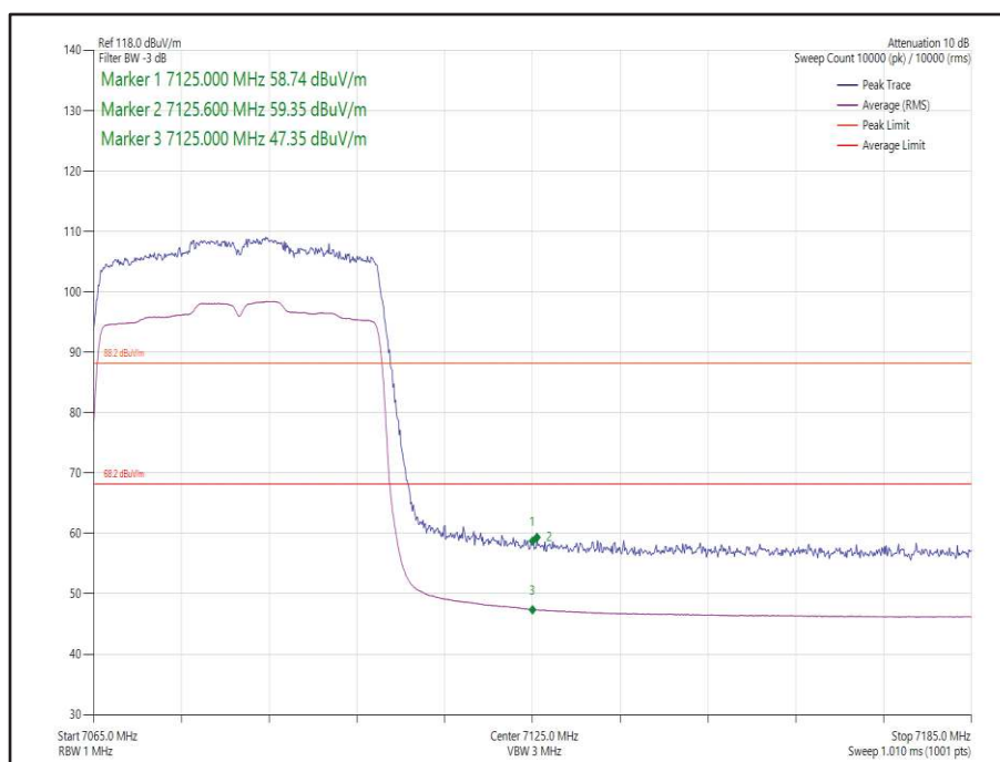
Figure 44 - 802.11ax HE40, Core 0, SU - 7085 MHz Band Edge Frequency 7125 MHz
