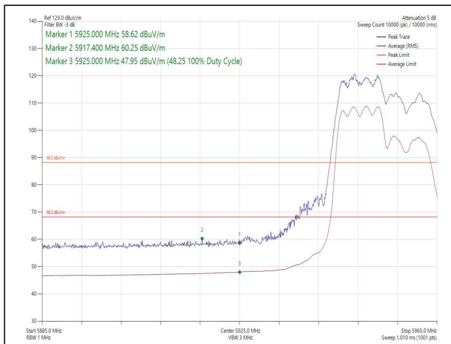
Figure 37 - 802.11ax HE20 CDD, Cores 0-1 106-53 - 5955 MHz Band Edge Frequency 5925 MHz
