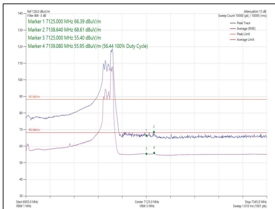
Figure 75 - 802.11ax HE160 CDD, Cores 0-1, 52-52 - 6985 MHz Band Edge Frequency 7125 MHz
