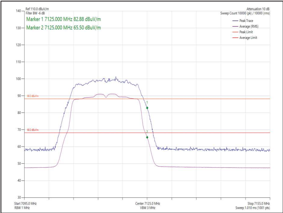
Figure 34 - 802.11a, Core 0 - 7115 MHz, Band Edge Frequency 7125 MHz
