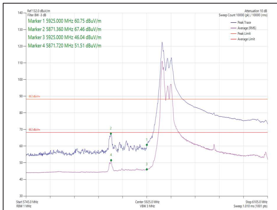
Figure 73 - 802.11ax HE160 SDM, Cores 0-1, 52-37 - 6025 MHz Band Edge Frequency 5925 MHz
