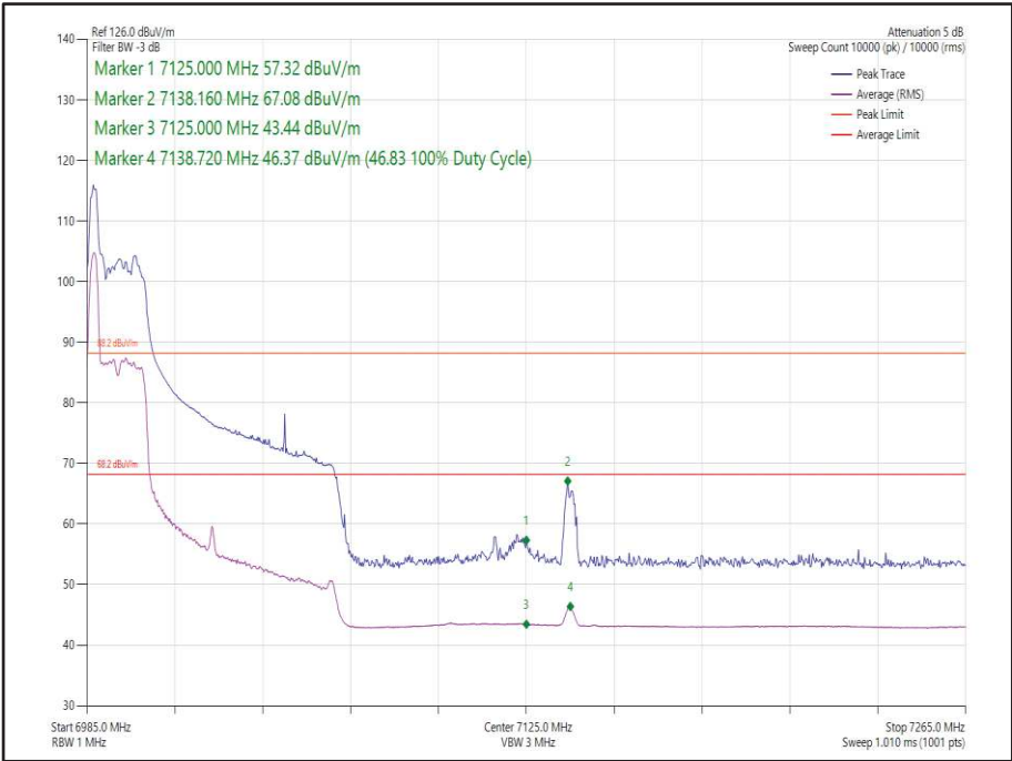
Figure 57 - 802.11ax HE80 Core 0 26-17 - 7025 MHz Band Edge Frequency 7125 MHz
