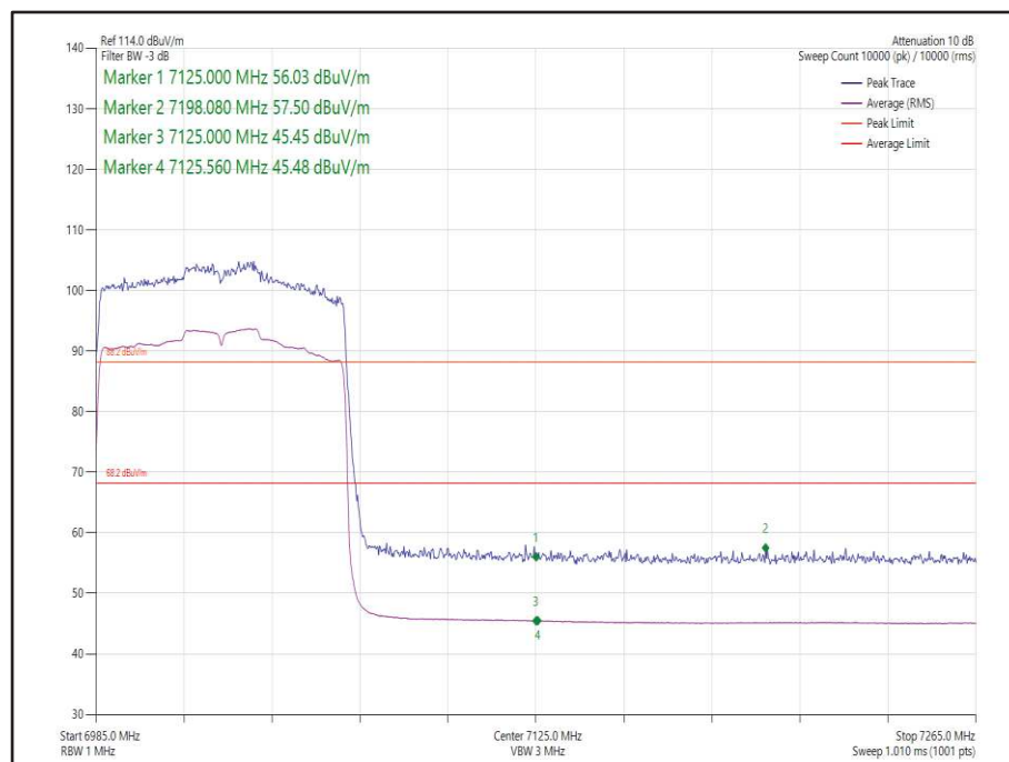
Figure 56 - 802.11ax HE80 Core 0 SU - 7025 MHz Band Edge Frequency 7125 MHz
