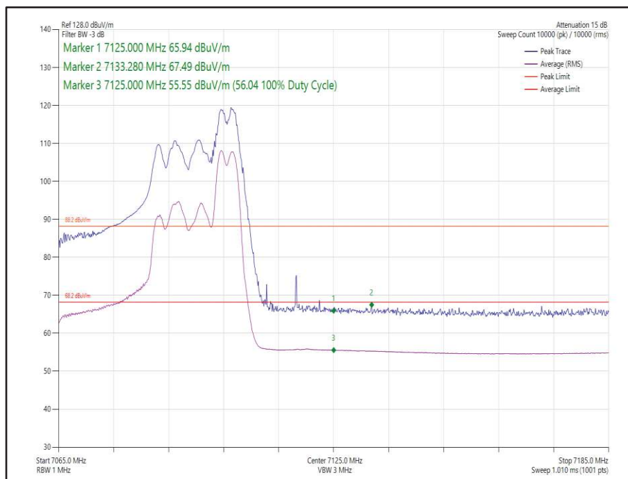
Figure 51 - 802.11ax HE40 CDD, Cores 0-1, 52-44 - 7085 MHz Band Edge Frequency 7125 MHz
