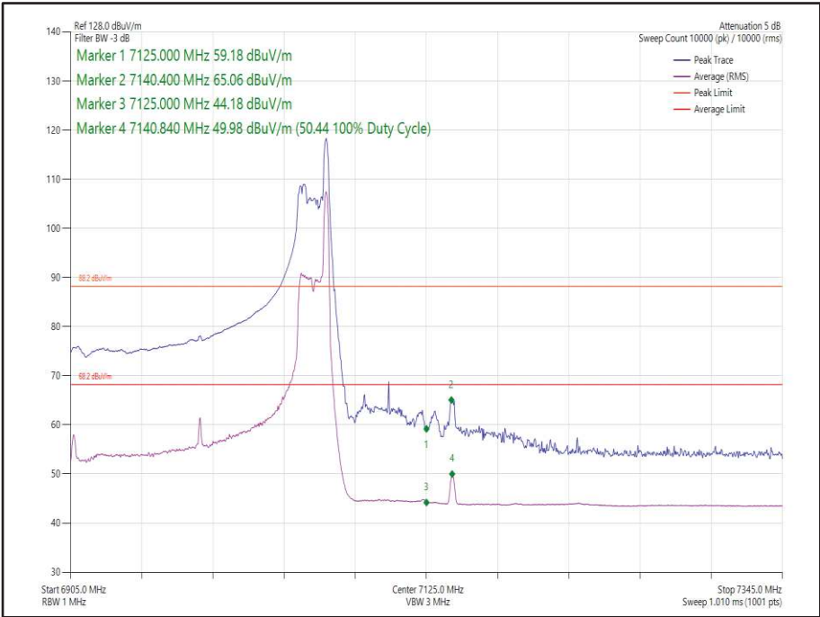
Figure 69 - 802.11ax HE160 Core 0 26-36 - 6985 MHz Band Edge Frequency 7125 MHz
