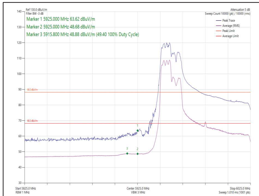
Figure 59 - 802.11ax HE80 CDD, Cores 0-1, 106-53 - 5985 MHz Band Edge Frequency 5925 MHz
