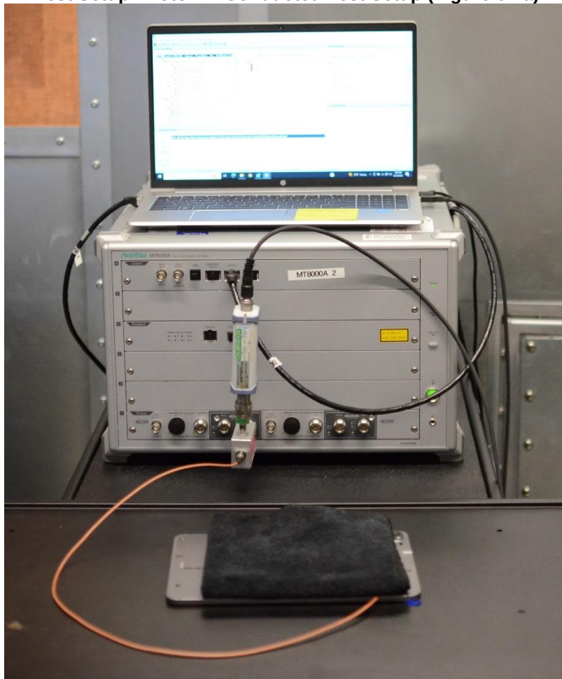
Test Setup Photo 2 – Conducted Test Setup (Figure 6-1a)
