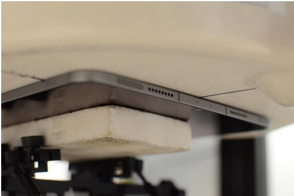
Test Setup Photo 8 – Body, Back Side at 0.0 cm – Antenna 4B
