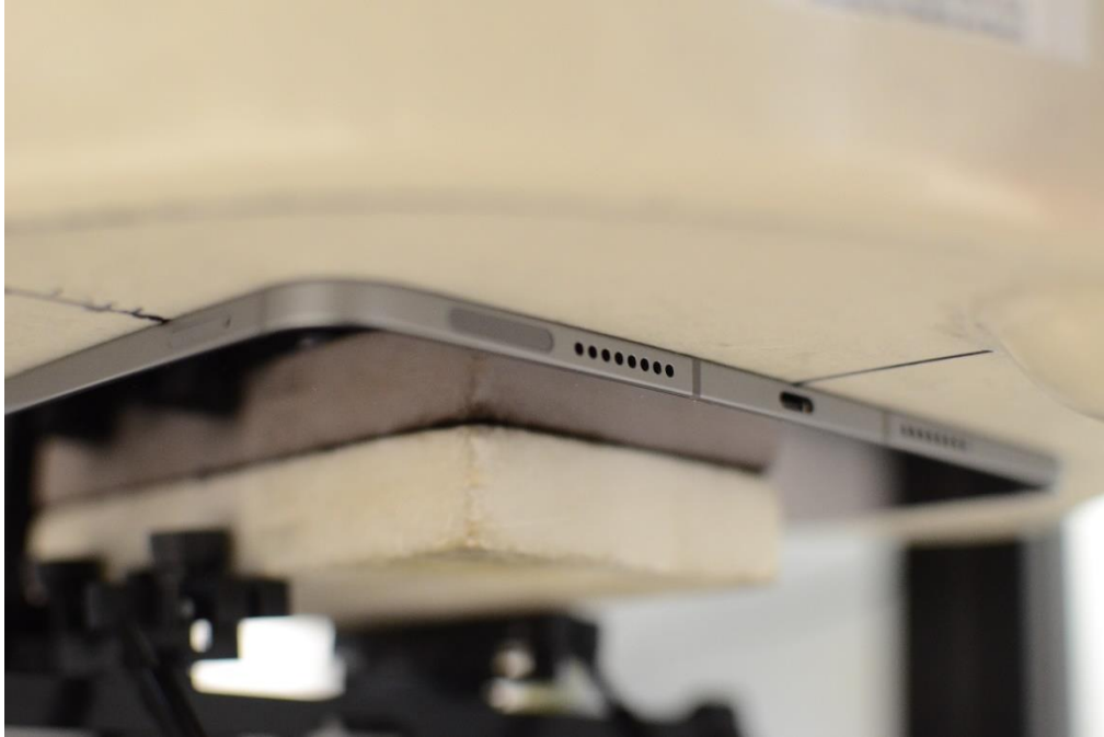
Test Setup Photo 7 – Body, Back Side at 0.0 cm – Antenna 1
