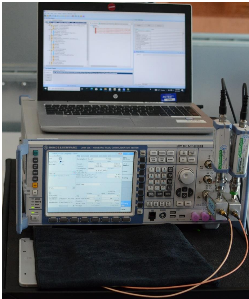
Test Setup Photo 6 – Conducted Test Setup (Figure 6-1c)
