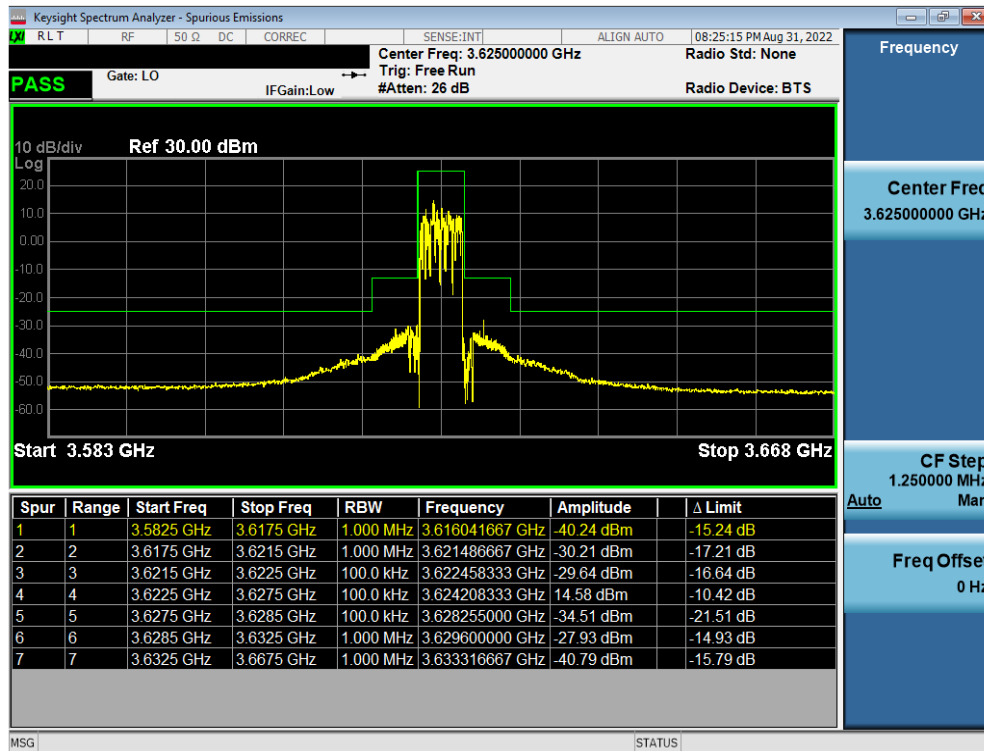
Plot 7-58. Channel Edge Plot (LTE Band 48 - 5MHz QPSK - Mid Channel)
