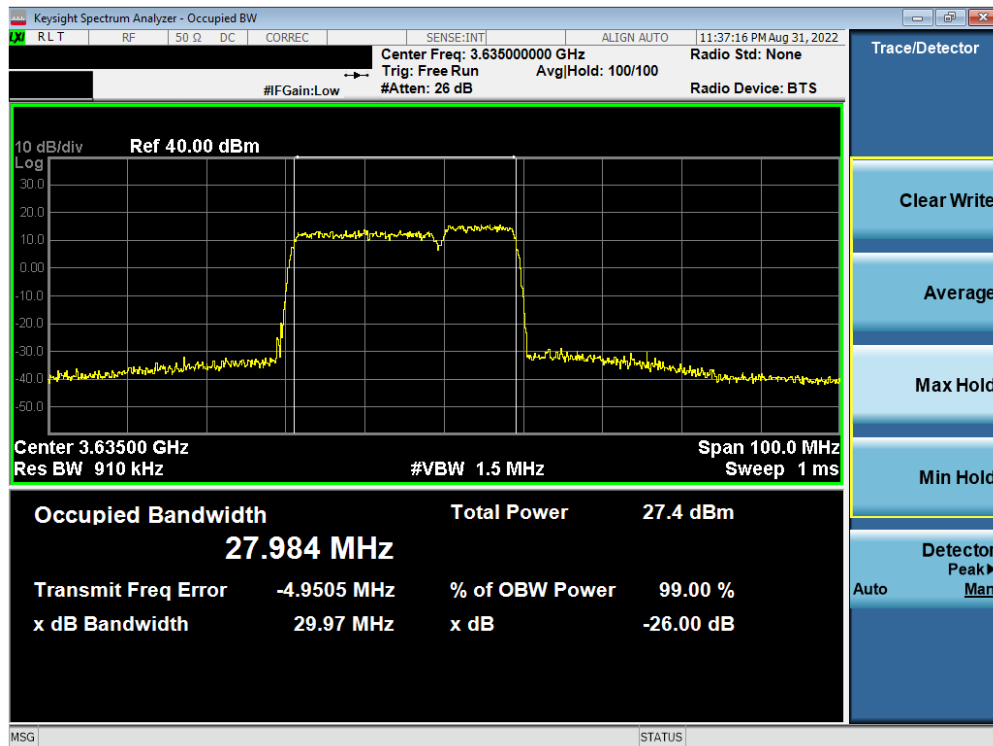
Plot 7-24. Occupied Bandwidth Plot (ULCA Band 48 - 20+10MHz 256-QAM - Full RB Configuration)
