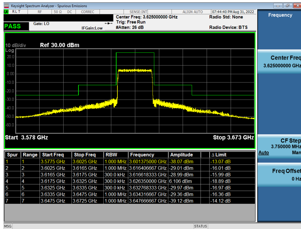
Plot 7-64. Channel Edge Plot (LTE Band 48 - 15MHz QPSK - Mid Channel)
