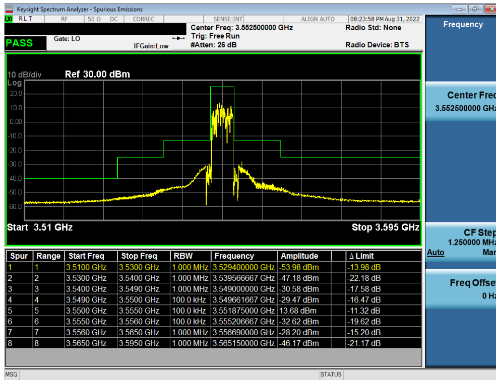
Plot 7-57. Channel Edge Plot (LTE Band 48 - 5MHz QPSK - Low Channel)
