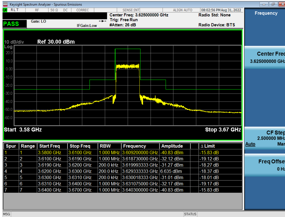
Plot 7-61. Channel Edge Plot (LTE Band 48 - 10MHz QPSK - Mid Channel)
