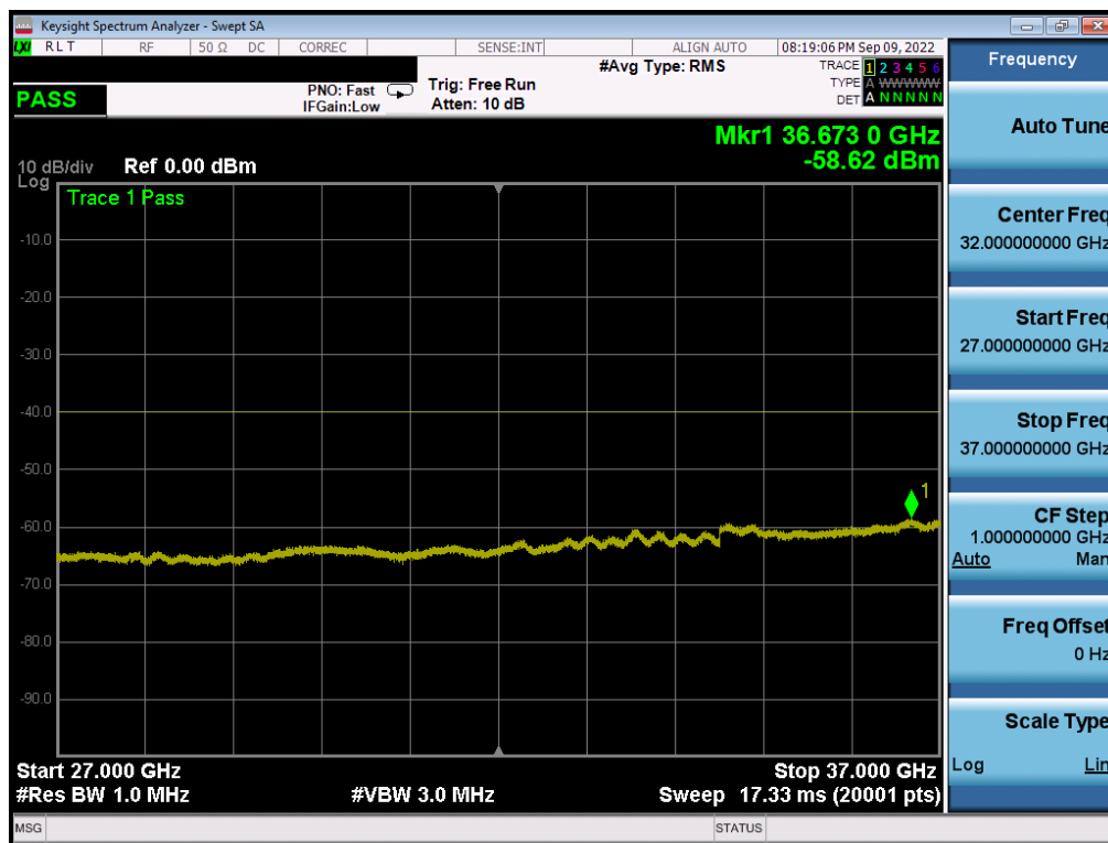
Plot 7-48. Conducted Spurious Plot (ULCA Band 48 - 20+20MHz QPSK - Low Channel)
