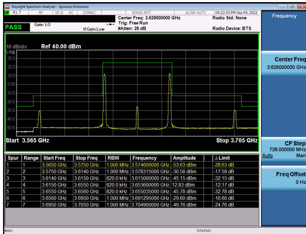
Plot 7-70. Channel Edge Plot (ULCA Band 48 – 20+20MHz QPSK - Mid Channel)
