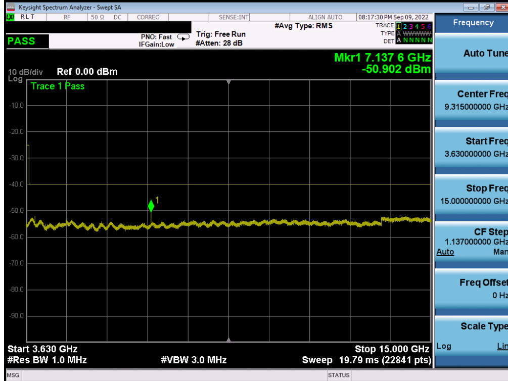
Plot 7-46. Conducted Spurious Plot (ULCA Band 48 - 20+20MHz QPSK - Low Channel)
