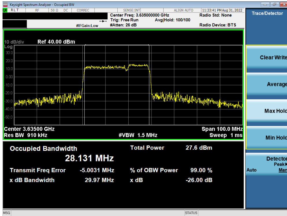
Plot 7-23. Occupied Bandwidth Plot (ULCA Band 48 - 20+10MHz 64-QAM - Full RB Configuration)
