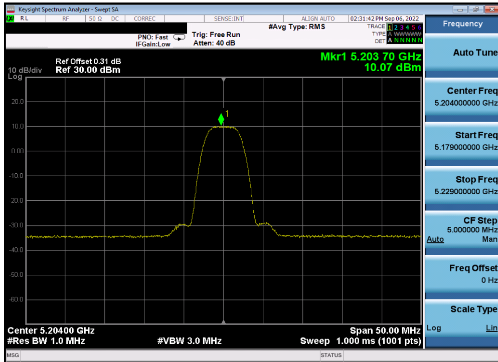
Plot 7-53. PSD Antenna 4a (HDR8, ePA, 5204MHz)
