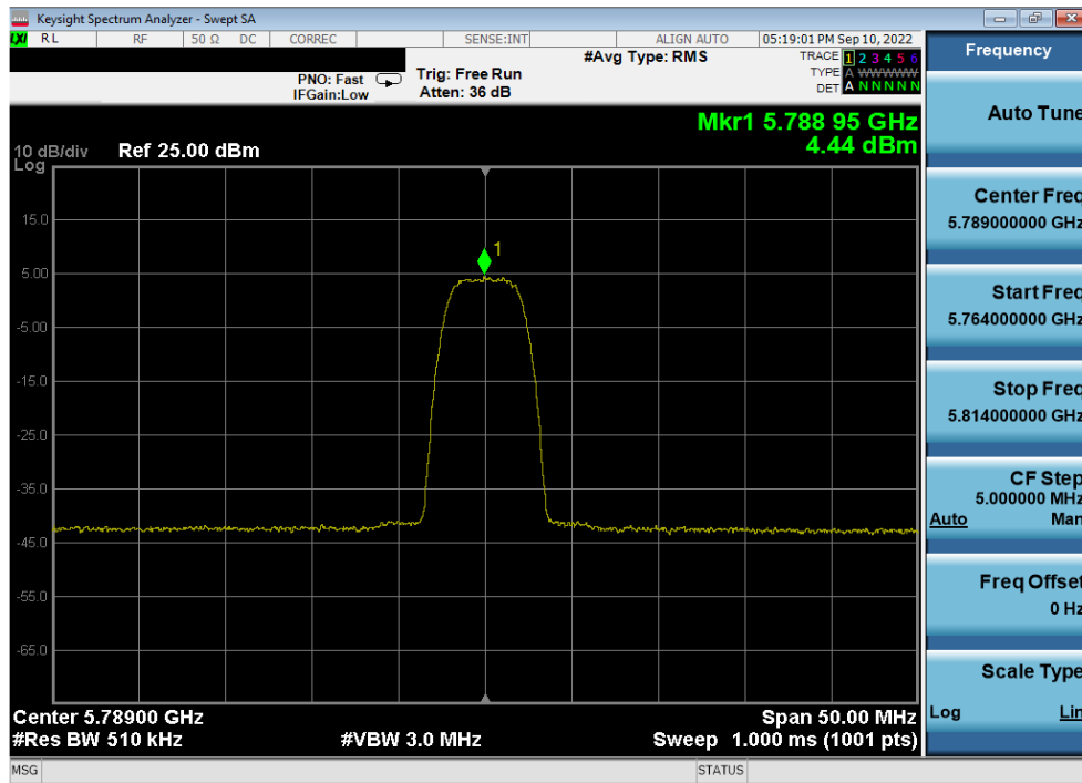
Plot 7-41. PSD Antenna 5b (HDR8, ePA, 5789MHz)
