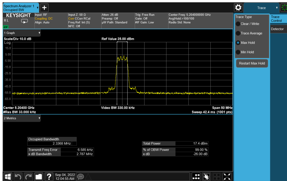
Plot 7-8. 26dB BW & 99% OBW Antenna 4a (HDR4, ePA, 5204MHz)
