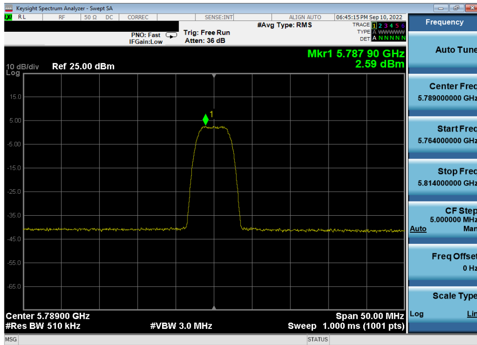
Plot 7-65. PSD Antenna 4a (HDR8, ePA, 5789MHz)
