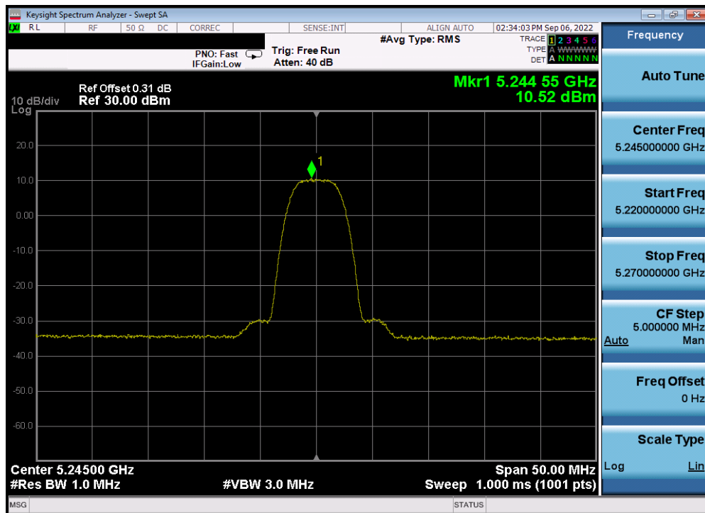
Plot 7-54. PSD Antenna 4a (HDR8, ePA, 5245MHz)
