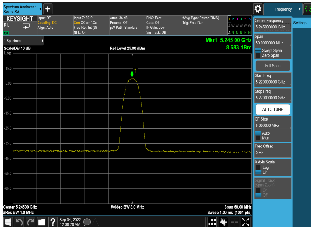
Plot 7-51. PSD Antenna 4a (HDR4, ePA, 5245MHz)
