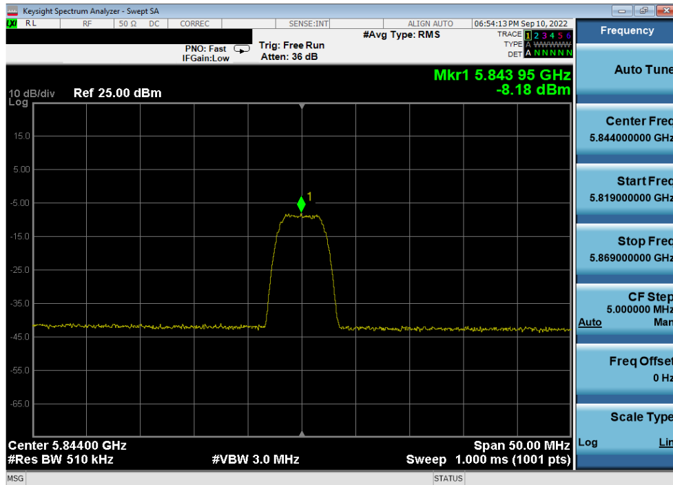
Plot 7-72. PSD Antenna 4a (HDR8, iPA, 5844MHz)
