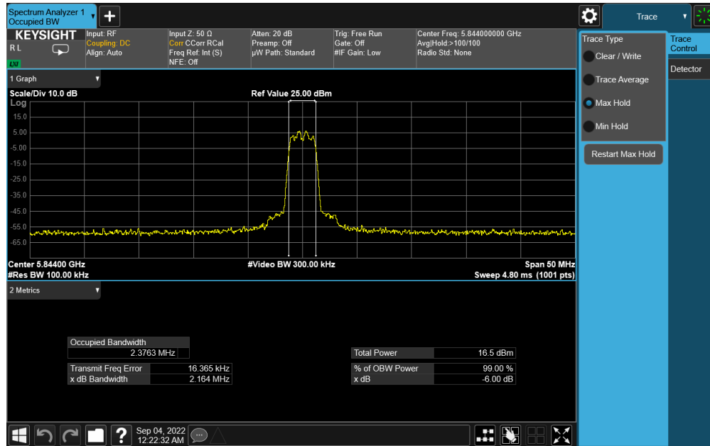
Plot 7-21. 6dB BW & 99% OBW Antenna 4a (HDR4, ePA, 5844MHz)
