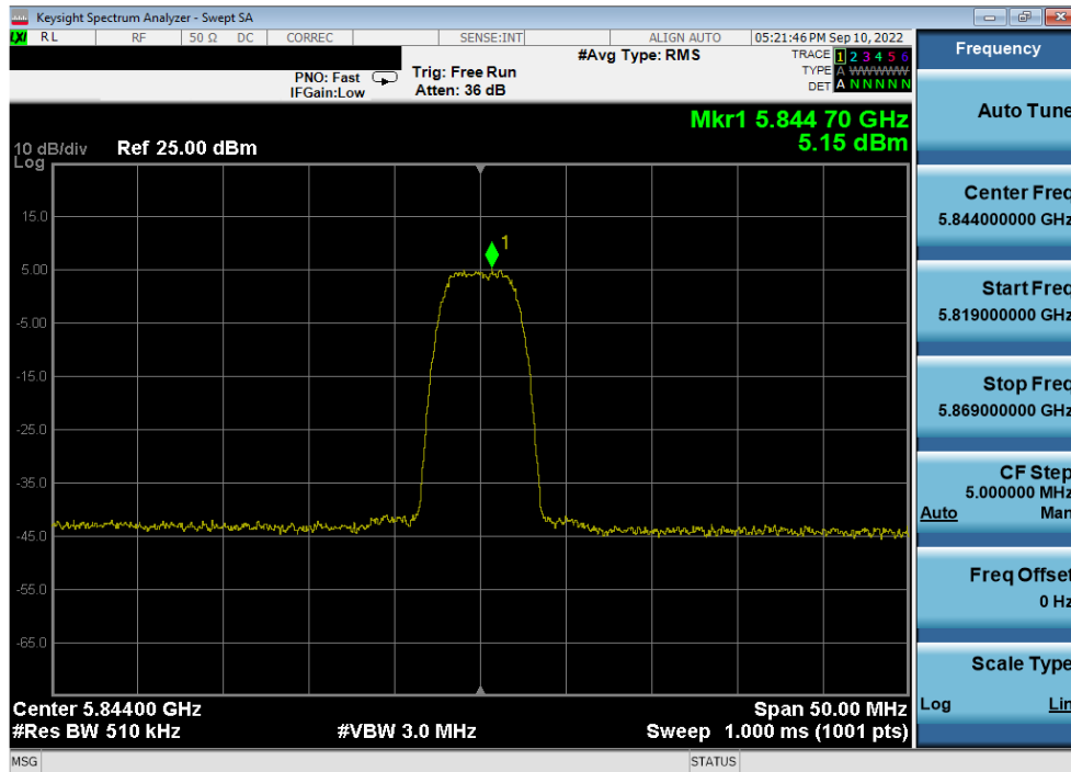
Plot 7-42. PSD Antenna 5b (HDR8, ePA, 5844MHz)
