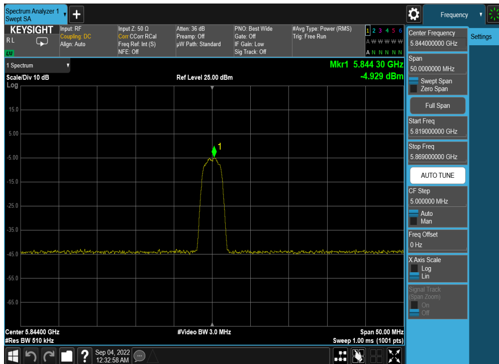
Plot 7-69. PSD Antenna 4a (HDR4, iPA, 5844MHz)
