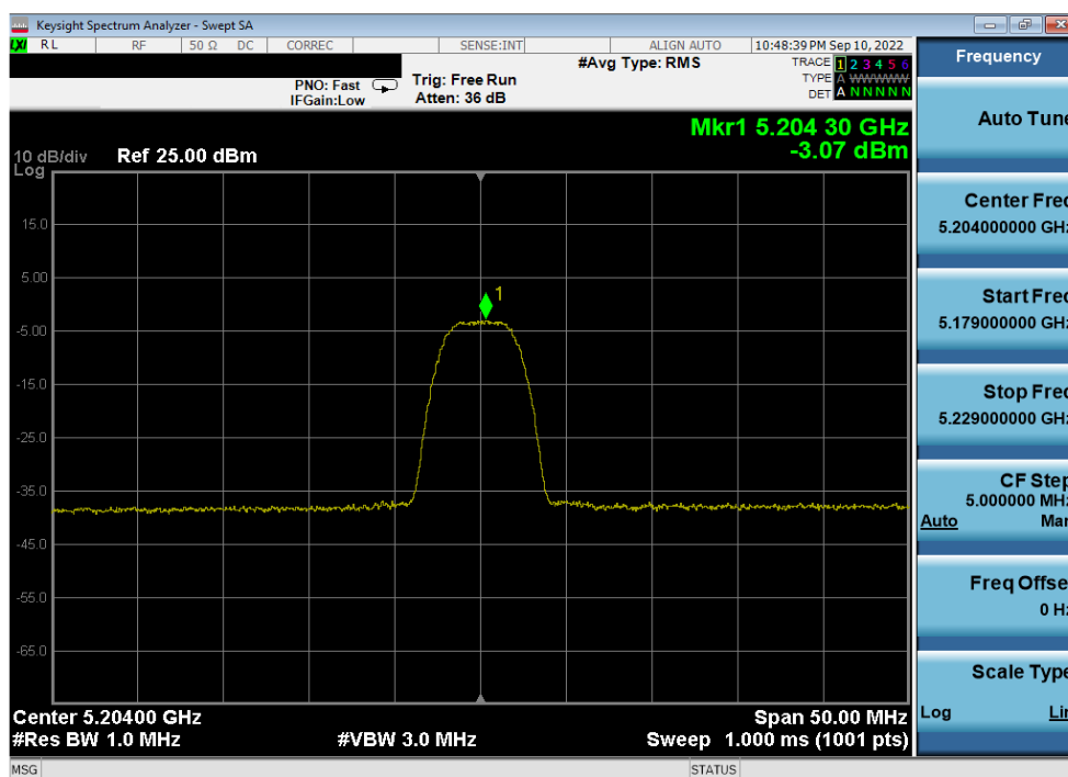
Plot 7-35. PSD Antenna 5b (HDR8, iPA, 5204MHz)
