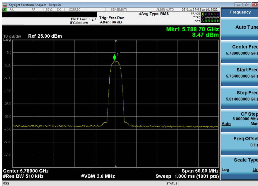
Plot 7-38. PSD Antenna 5b (HDR4, ePA, 5789MHz)
