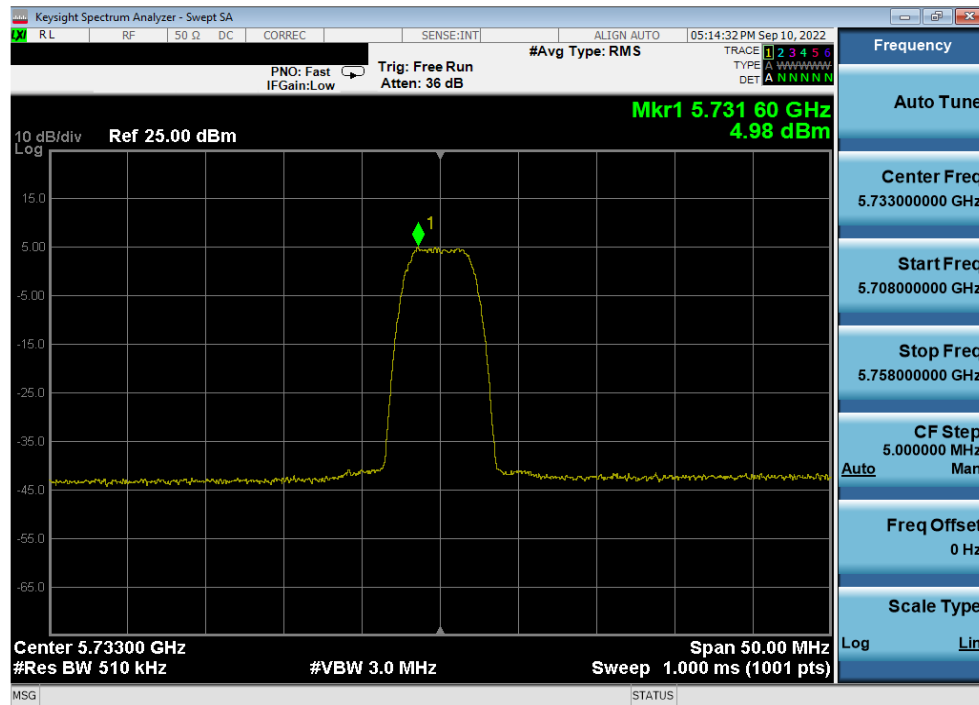
Plot 7-40. PSD Antenna 5b (HDR8, ePA, 5733MHz)
