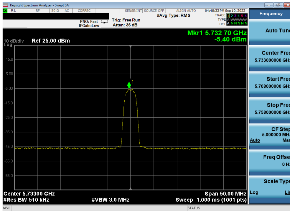
Plot 7-67. PSD Antenna 4a (HDR4, iPA, 5733MHz)
