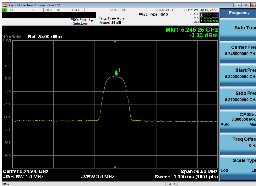
Plot 7-36. PSD Antenna 5b (HDR8, iPA, 5245MHz)
