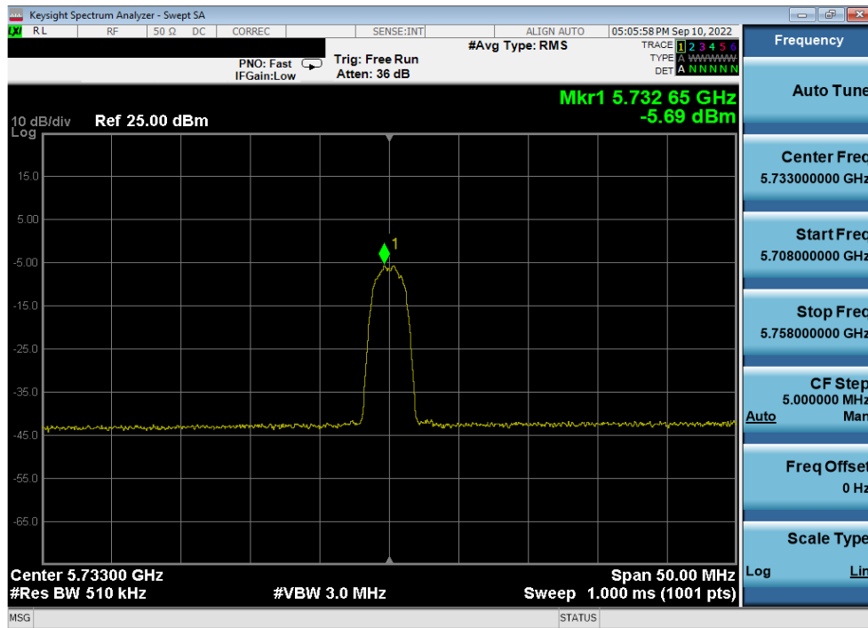
Plot 7-43. PSD Antenna 5b (HDR4, iPA, 5733MHz)
