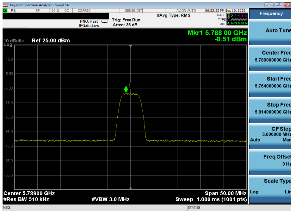
Plot 7-71. PSD Antenna 4a (HDR8, iPA, 5789MHz)
