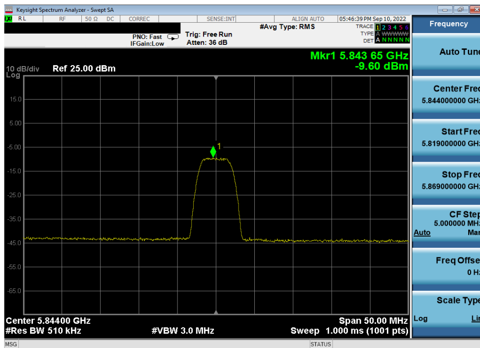
Plot 7-48. PSD Antenna 5b (HDR8, iPA, 5844MHz)
