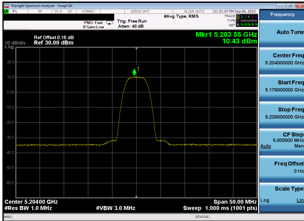
Plot 7-29. PSD Antenna 5b (HDR8, ePA, 5204MHz)
