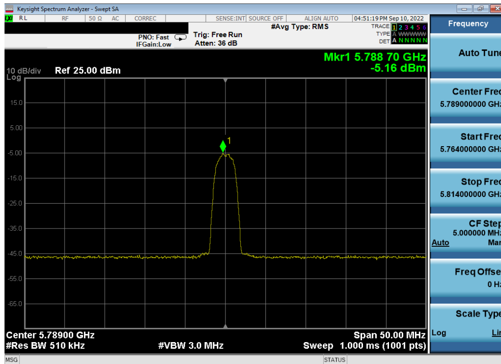
Plot 7-68. PSD Antenna 4a (HDR4, iPA, 5789MHz)
