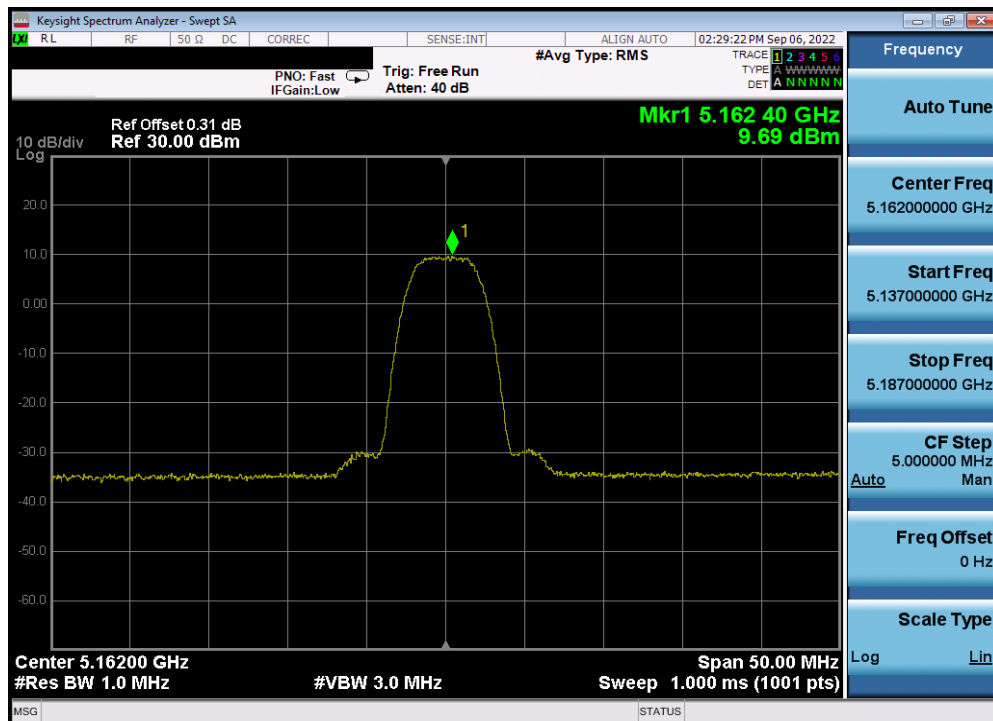
Plot 7-52. PSD Antenna 4a (HDR8, ePA, 5162MHz)
