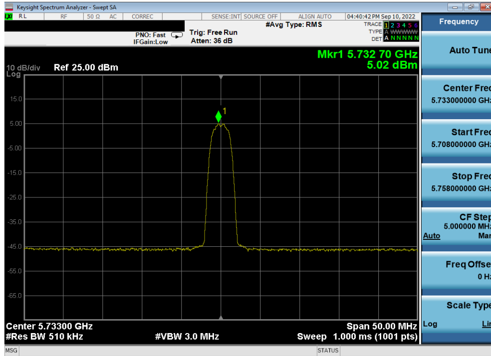
Plot 7-61. PSD Antenna 4a (HDR4,ePA, 5733MHz)
