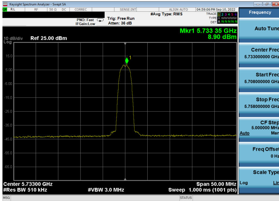
Plot 7-37. PSD Antenna 5b (HDR4, ePA, 5733MHz)
