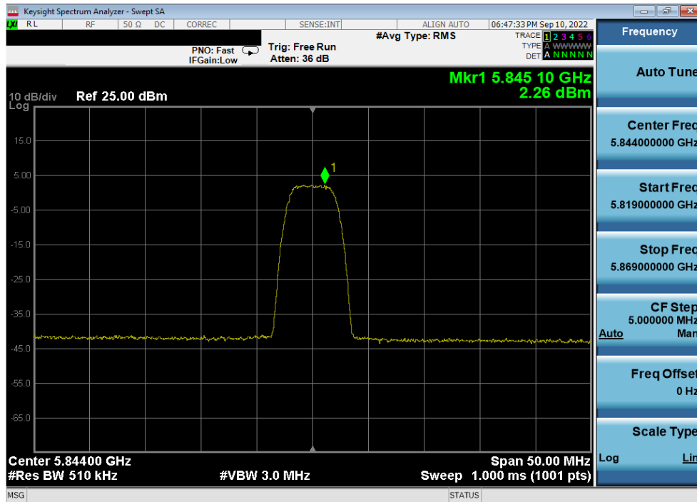
Plot 7-66. PSD Antenna 4a (HDR8, ePA, 5844MHz)
