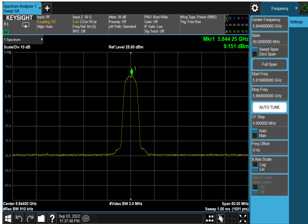
Plot 7-39. PSD Antenna 5b (HDR4, ePA, 5844MHz)
