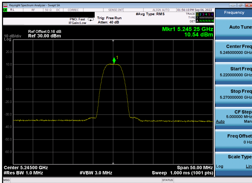
Plot 7-30. PSD Antenna 5b (HDR8, ePA, 5245MHz)
