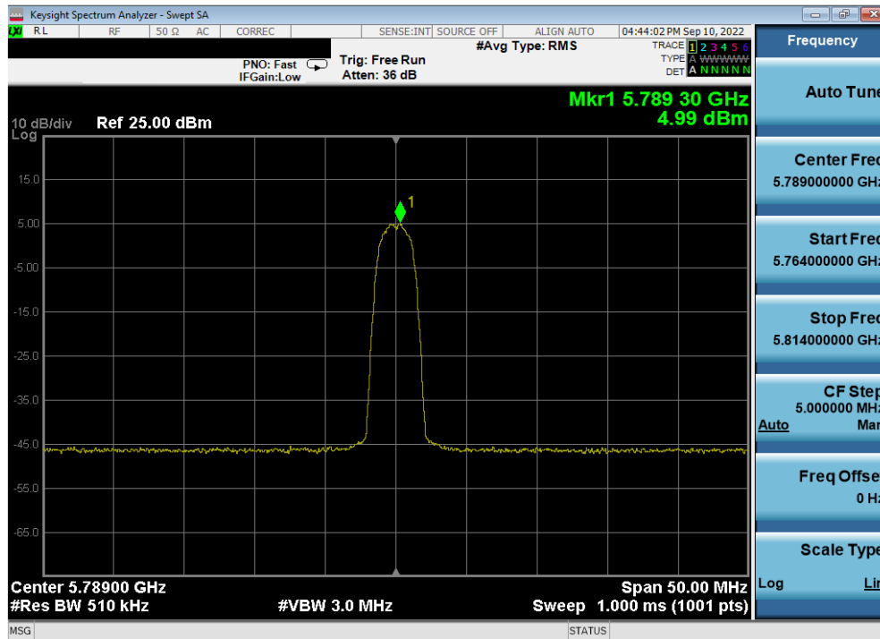
Plot 7-62. PSD Antenna 4a (HDR4, ePA, 5789MHz)
