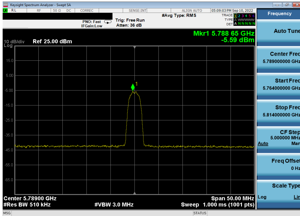
Plot 7-44. PSD Antenna 5b (HDR4, iPA, 5789MHz)
