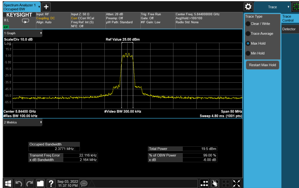
Plot 7-15. 6dB BW & 99% OBW Antenna 5b (HDR4, ePA, 5844MHz)
