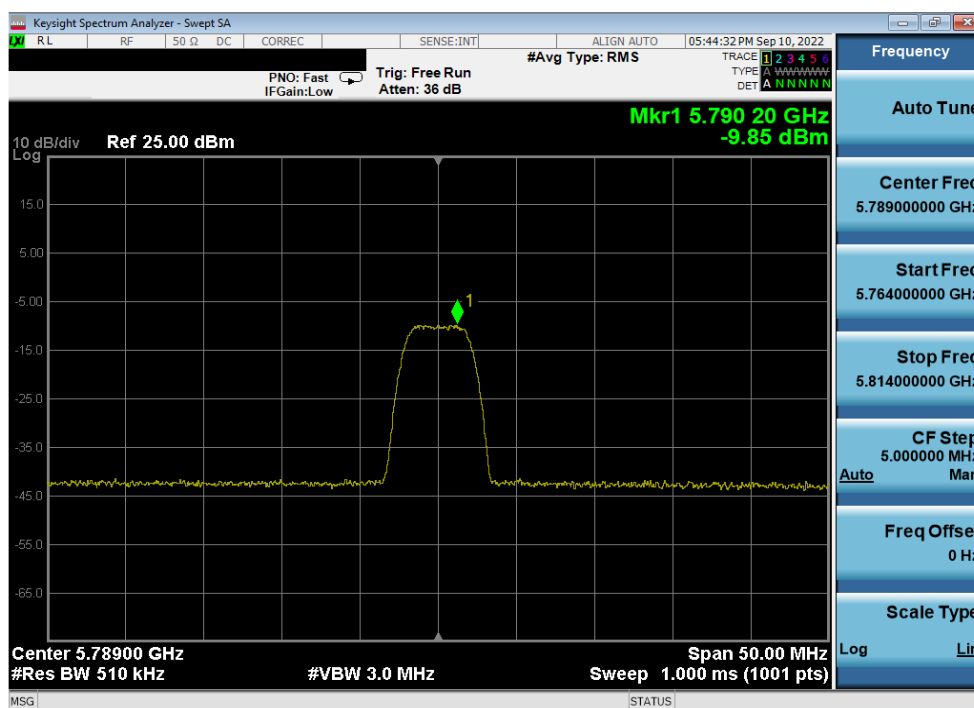
Plot 7-47. PSD Antenna 5b (HDR8, iPA, 5789MHz)
