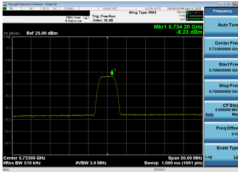
Plot 7-70. PSD Antenna 4a (HDR8, iPA, 5733MHz)
