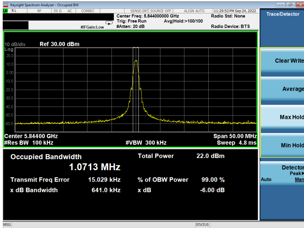
Plot 7-9. 6dB BW & 99% OBW Antenna 5b (BDR, ePA, 5844MHz)
