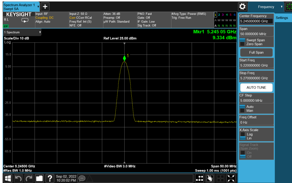
Plot 7-27. PSD Antenna 4a (BDR GFSK, ePA – 5245MHz)
