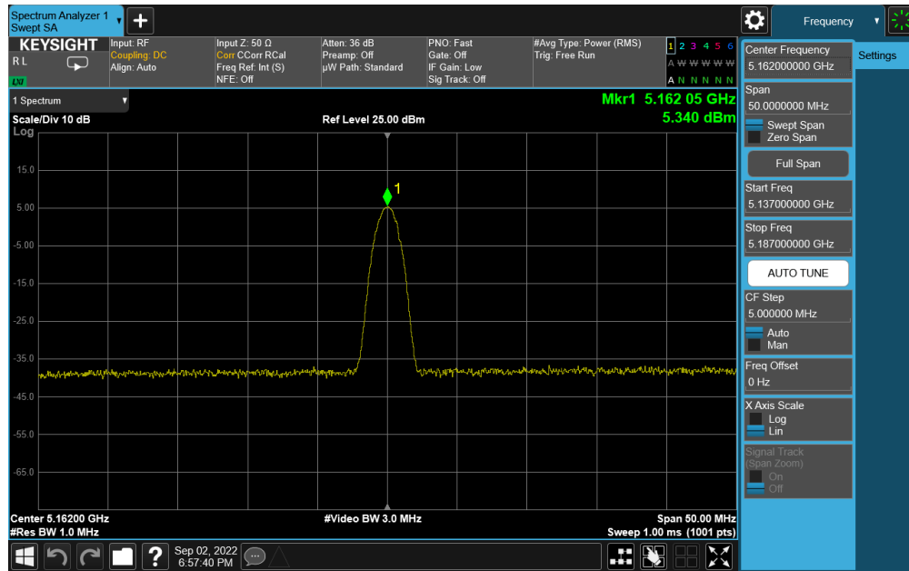
Plot 7-43. PSD TxBF Antenna 5b (BDR GFSK, iPA - 5162MHz)
