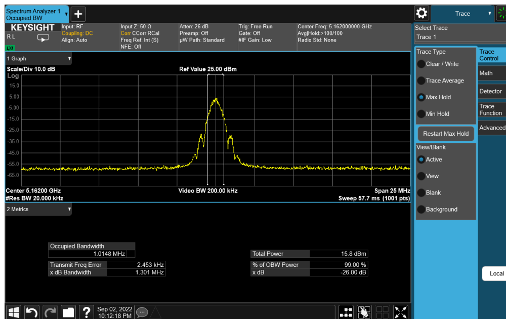
Plot 7-4. 26dB BW & 99% OBW Antenna 4a (BDR GFSK – 5162MHz)
