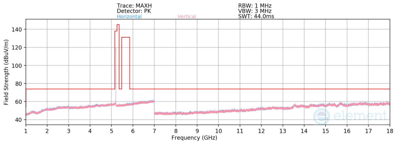
Plot 7-1. Radiated Spurious Emissions Above 1GHz TxBF (BT GFSK ePA – 5204MHz)
