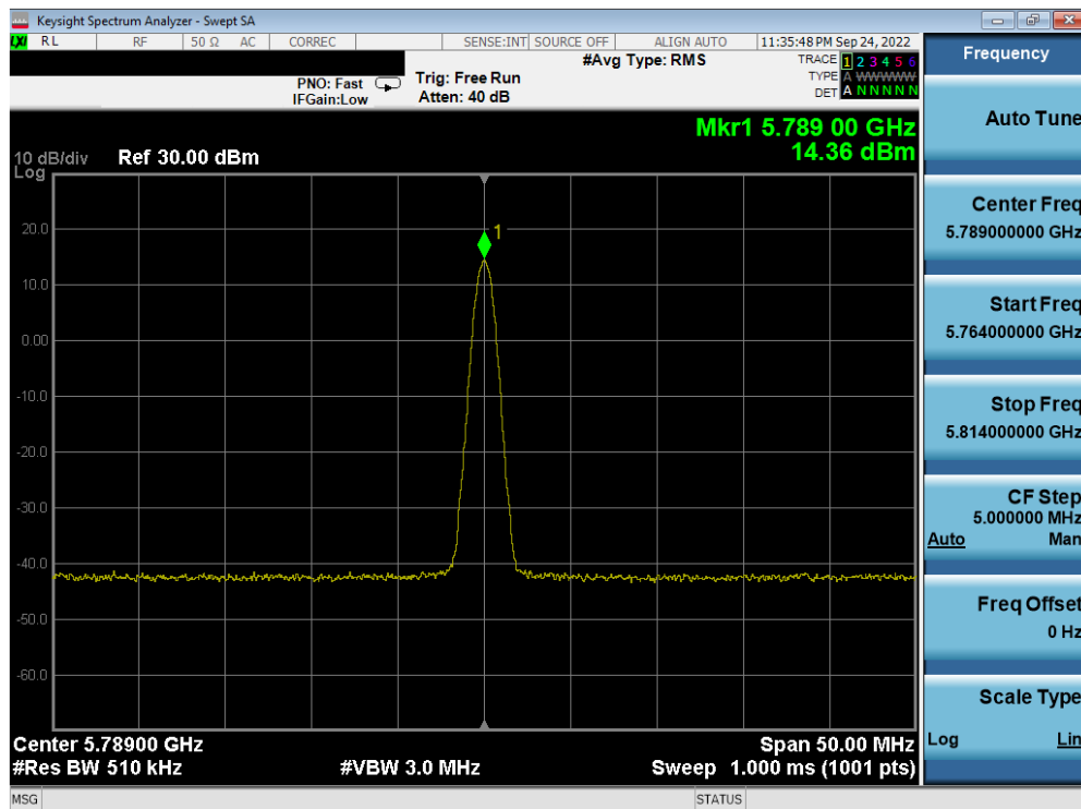
Plot 7-20. PSD Antenna 5b (BDR, ePA, 5789MHz)
