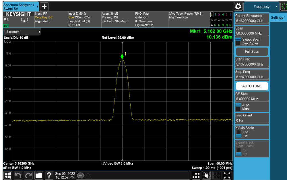
Plot 7-25. PSD Antenna 4a (BDR GFSK, ePA – 5162MHz)
