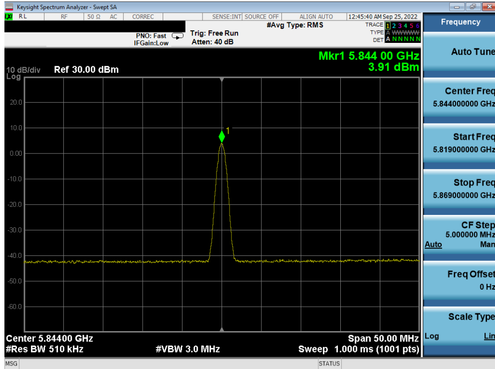
Plot 7-59. PSD TxBF Antenna 5b (BDR, iPA, 5844MHz)
