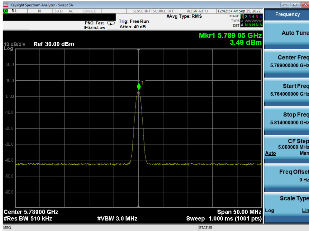
Plot 7-57. PSD TxBF Antenna 5b (BDR, iPA, 5789MHz)
