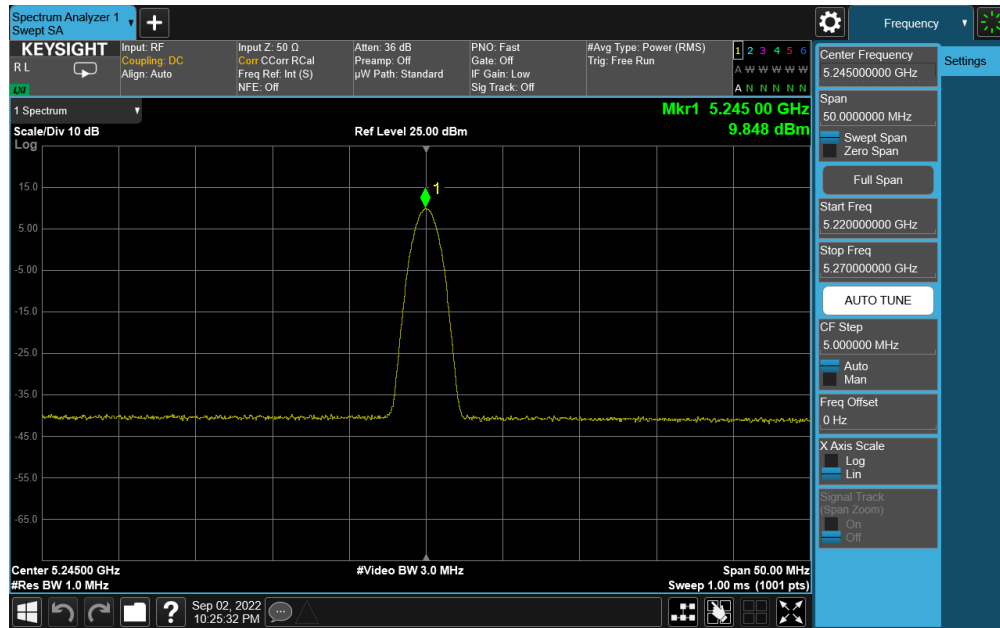
Plot 7-15. PSD Antenna 5b (BDR GFSK, ePA – 5245MHz)
