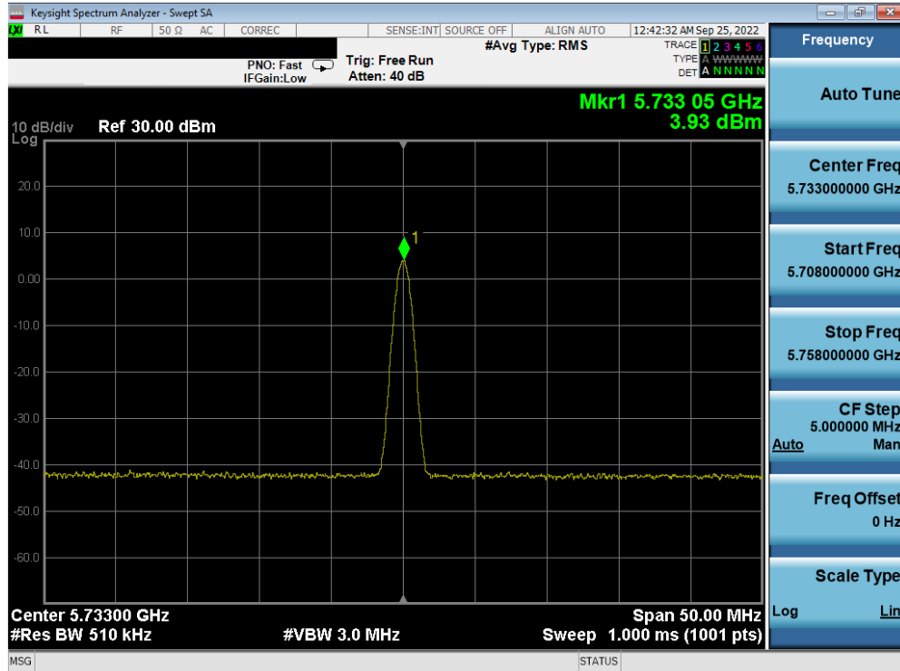
Plot 7-55. PSD TxBF Antenna 5b (BDR, iPA, 5733MHz)
