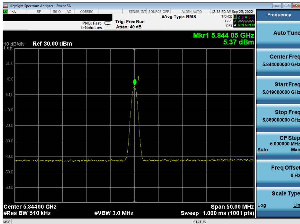
Plot 7-60. PSD TxBF Antenna 4a (BDR, iPA, 5844MHz)
