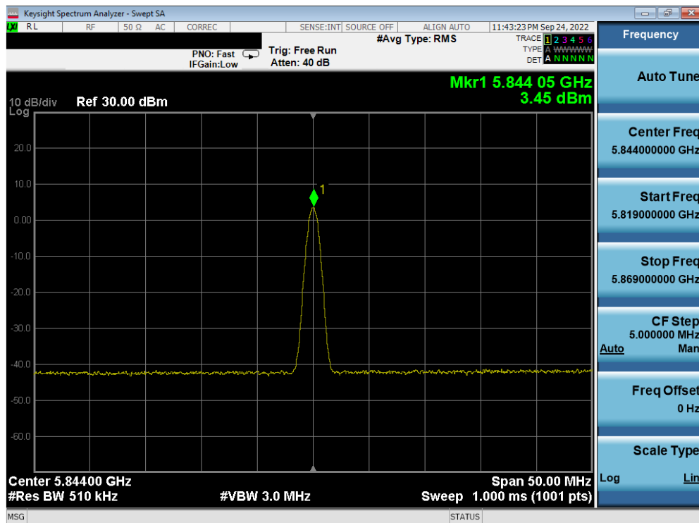
Plot 7-24. PSD Antenna 5b (BDR, iPA, 5844MHz)
