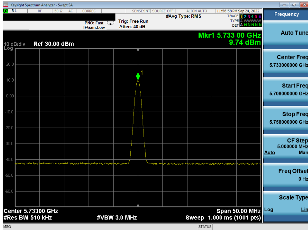
Plot 7-31. PSD Antenna 4a (BDR, ePA, 5733MHz)
