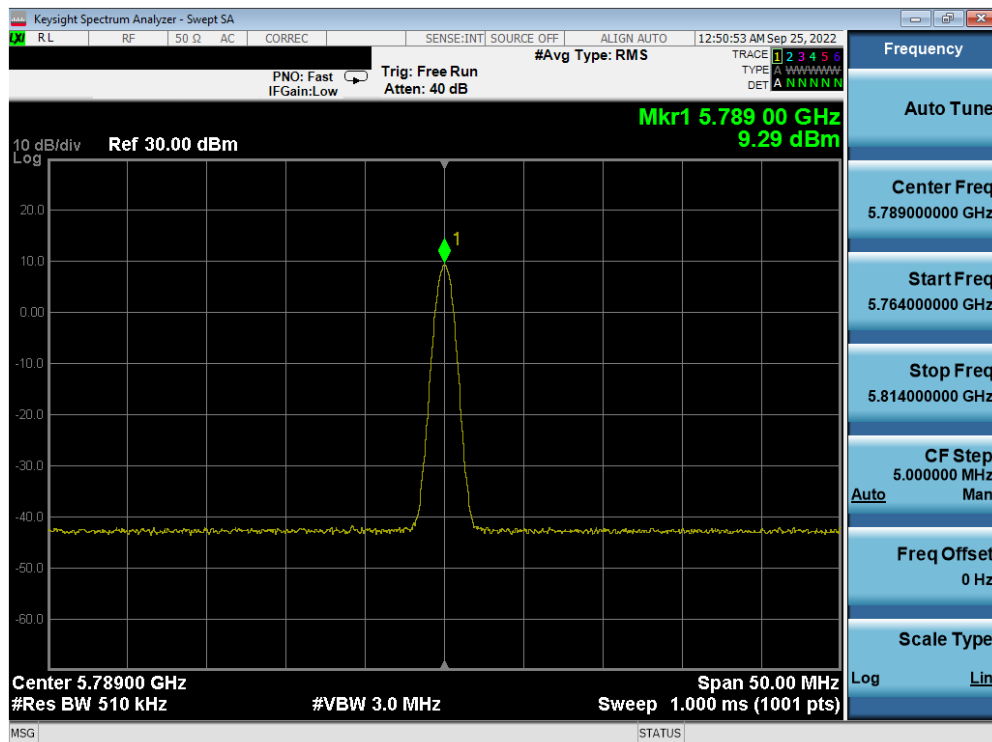
Plot 7-52. PSD TxBF Antenna 4a (BDR, ePA, 5789MHz)
