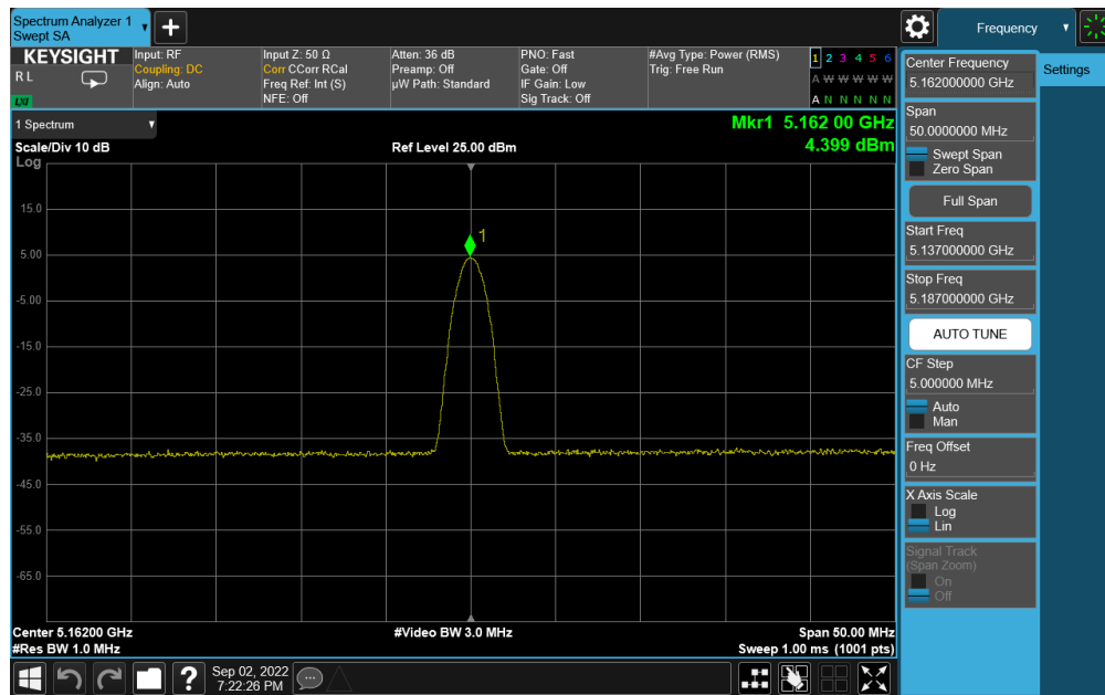
Plot 7-28. PSD Antenna 4a (BDR GFSK, iPA – 5162MHz)
