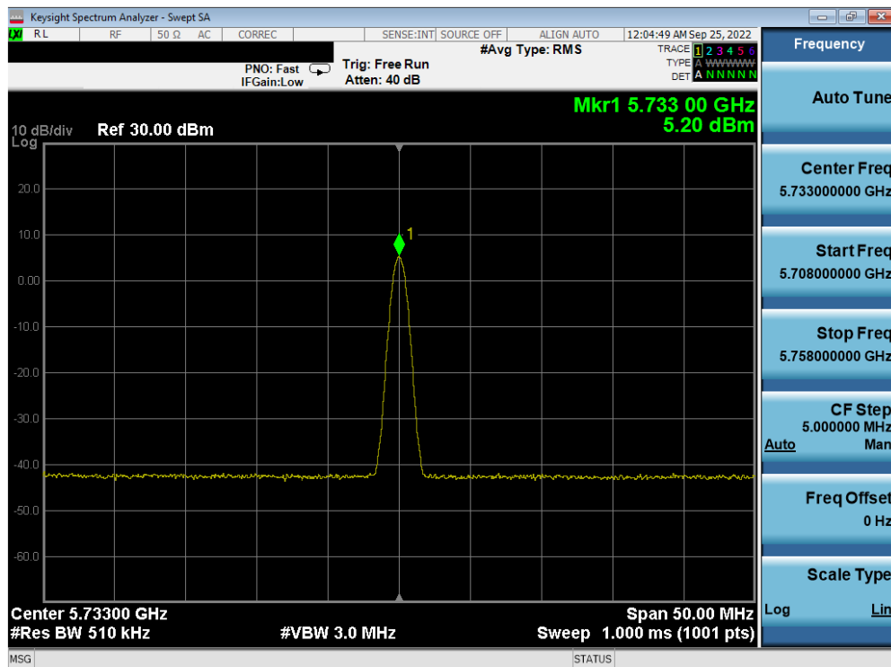
Plot 7-34. PSD Antenna 4a (BDR, iPA, 5733MHz)
