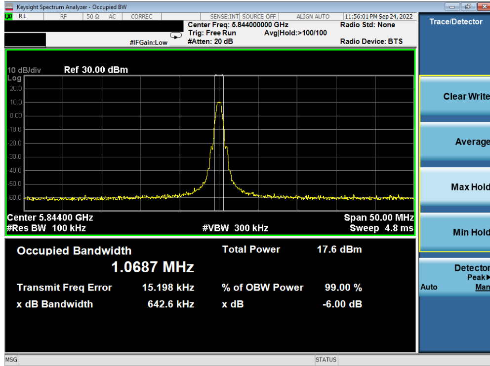
Plot 7-12. 6dB BW & 99% OBW Antenna 4a (BDR, ePA, 5844MHz)
