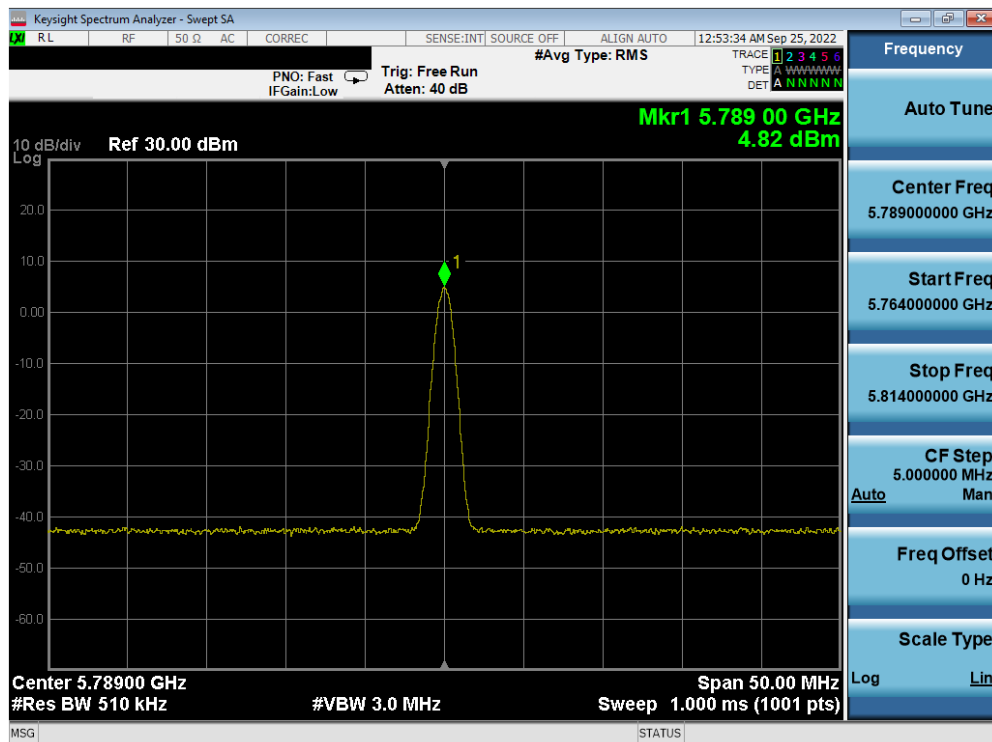
Plot 7-58. PSD TxBF Antenna 4a (BDR, iPA, 5789MHz)
