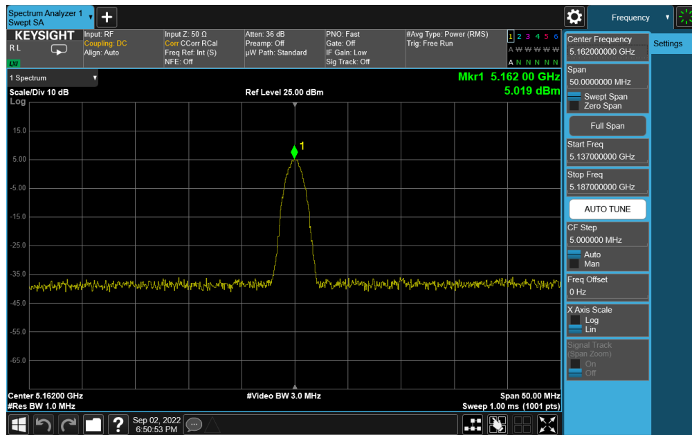
Plot 7-16. PSD Antenna 5b (BDR GFSK, iPA – 5162MHz)
