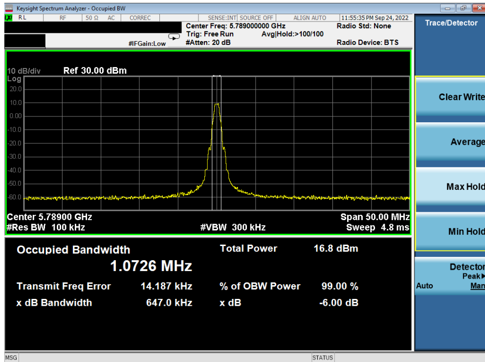
Plot 7-11. 6dB BW & 99% OBW Antenna 4a (BDR, ePA, 5789MHz)
