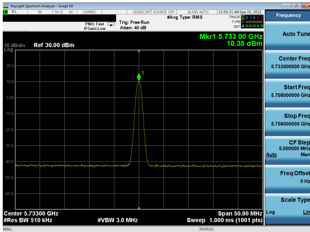
Plot 7-50. PSD TxBF Antenna 4a (BDR, ePA, 5733MHz)
