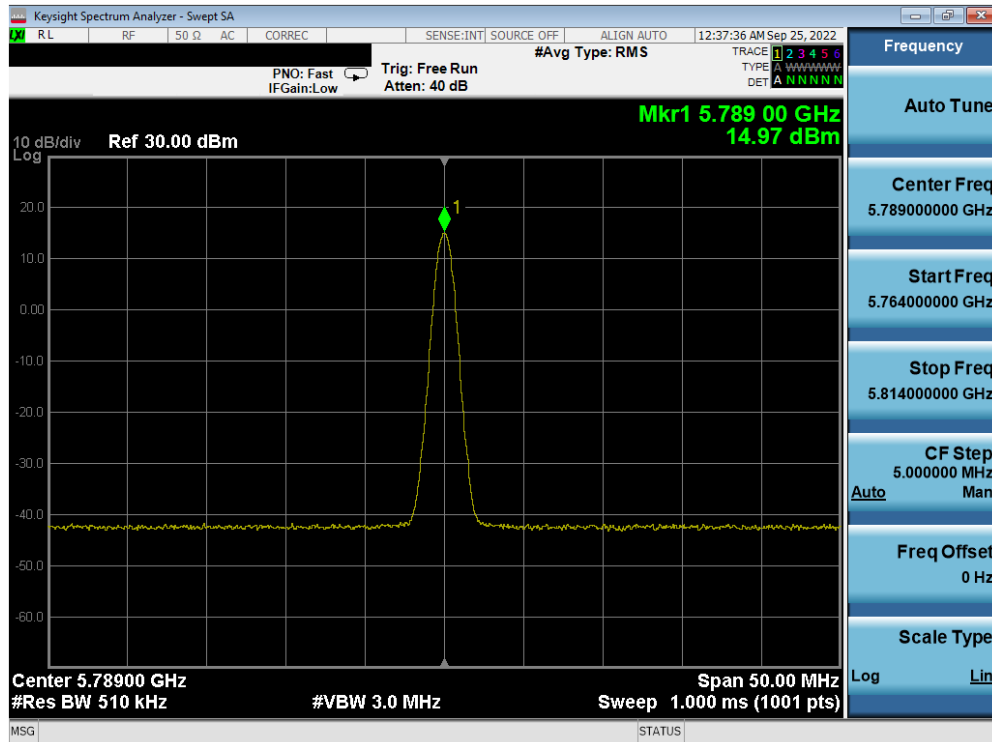
Plot 7-51. PSD TxBF Antenna 5b (BDR, ePA, 5789MHz)
