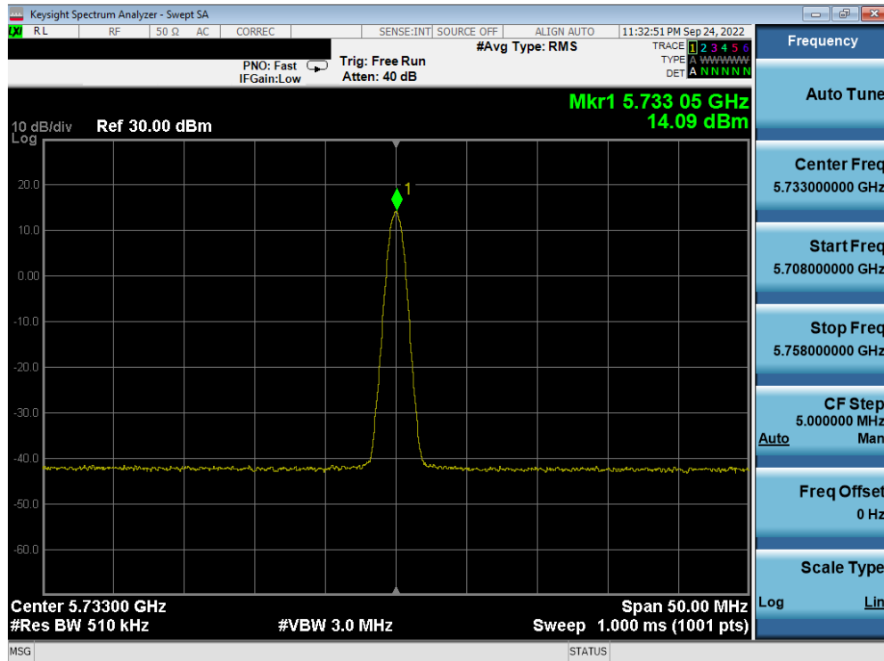
Plot 7-19. PSD Antenna 5b (BDR, ePA, 5733MHz)
