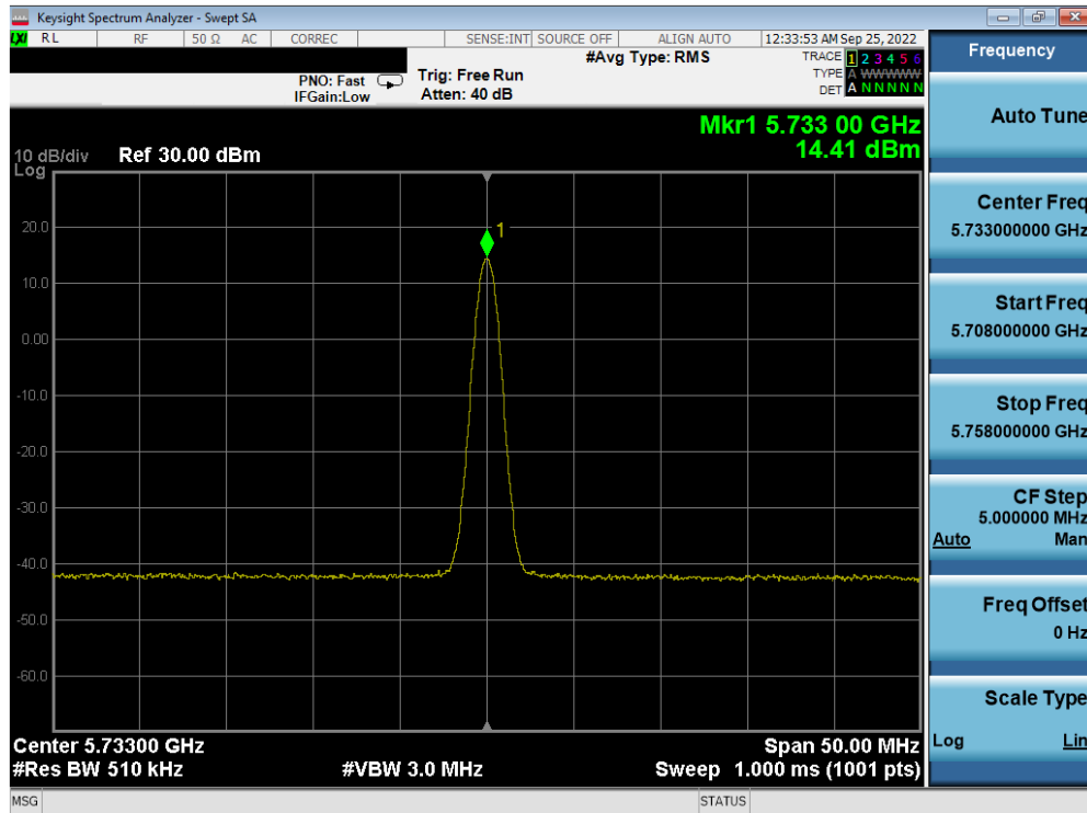
Plot 7-49. PSD TxBF Antenna 5b (BDR, ePA, 5733MHz)
