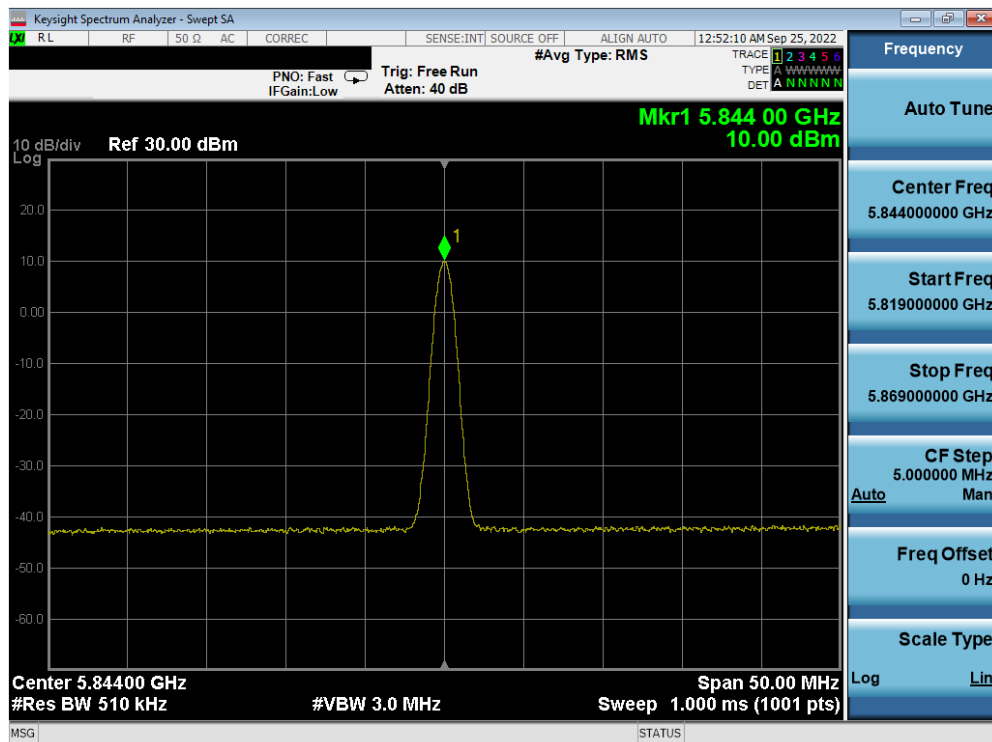
Plot 7-54. PSD TxBF Antenna 4a (BDR, ePA, 5844MHz)
