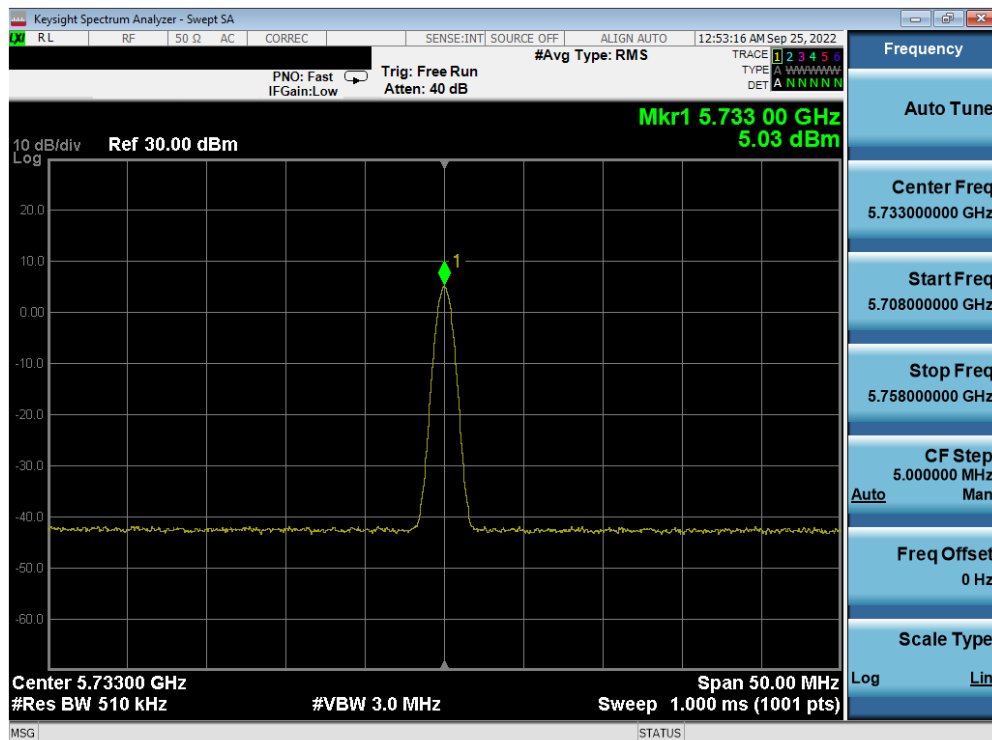
Plot 7-56. PSD TxBF Antenna 4a (BDR, iPA, 5733MHz)
