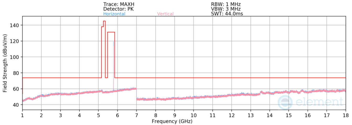
Plot 7-2. Radiated Spurious Emissions Above 1GHz TxBF (BT GFSK ePA – 5789MHz)
