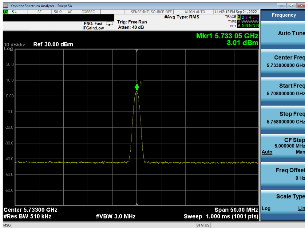
Plot 7-22. PSD Antenna 5b (BDR, iPA, 5733MHz)
