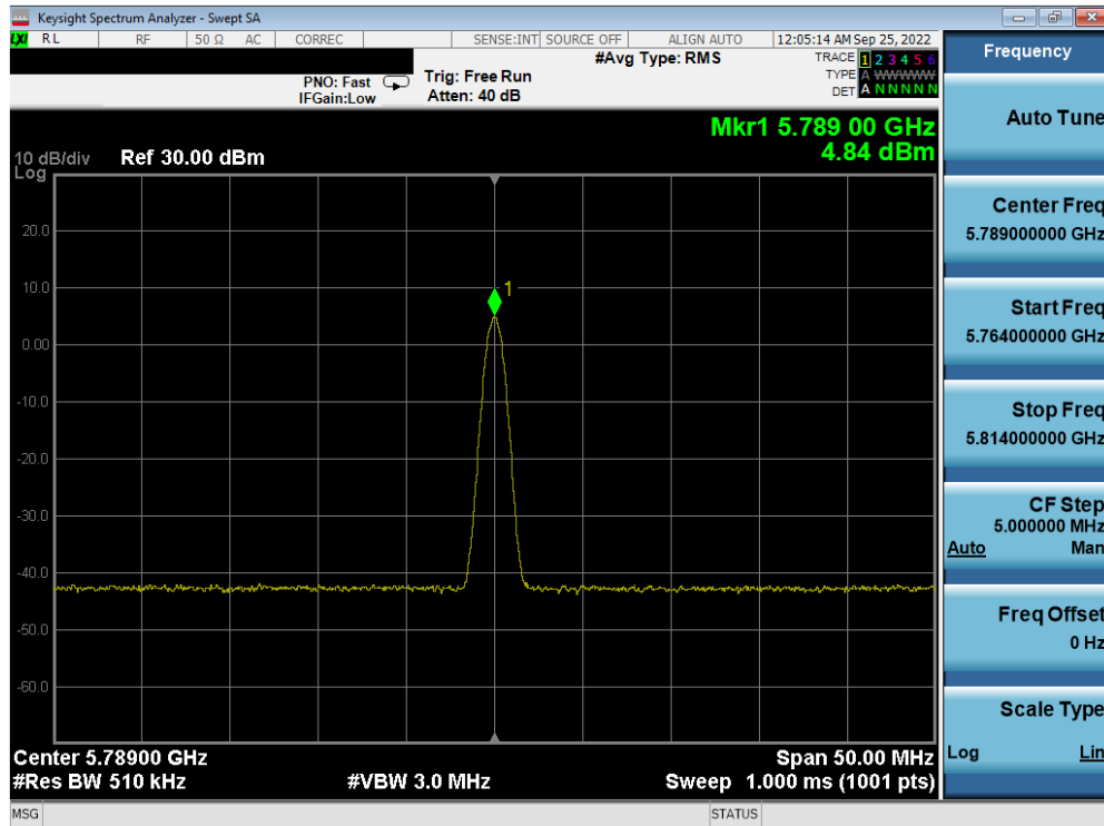
Plot 7-35. PSD Antenna 4a (BDR, iPA, 5789MHz)
