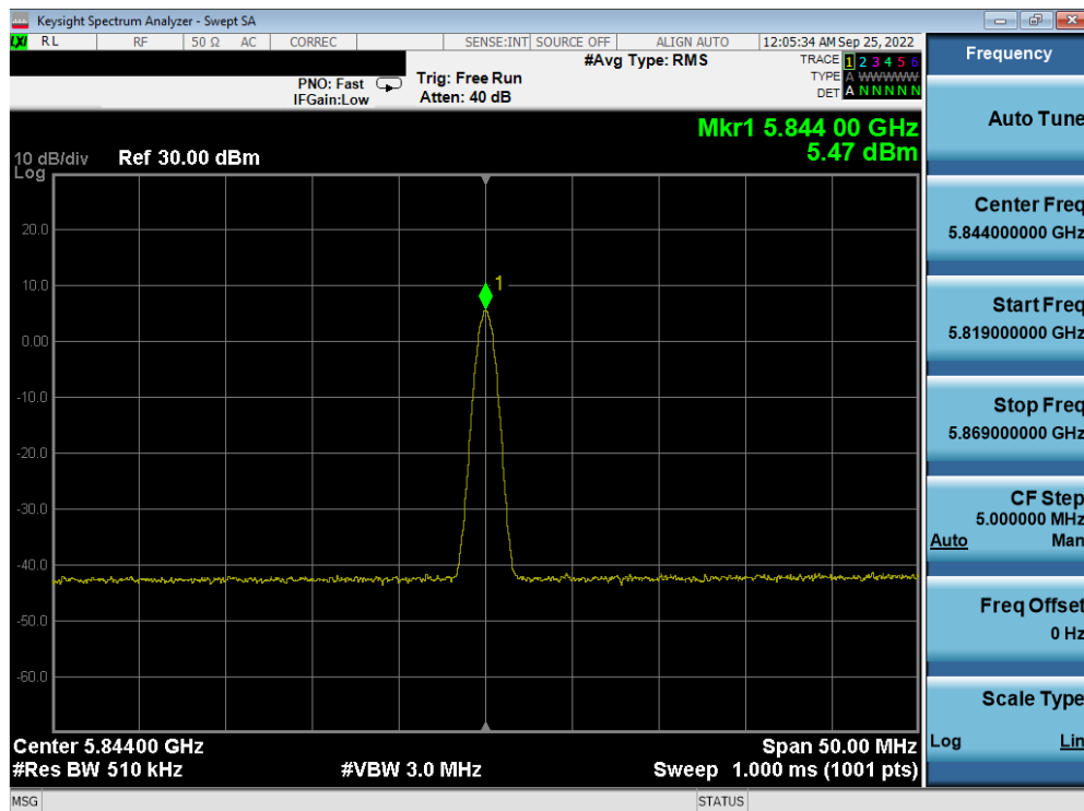
Plot 7-36. PSD Antenna 4a (BDR, iPA, 5844MHz)
