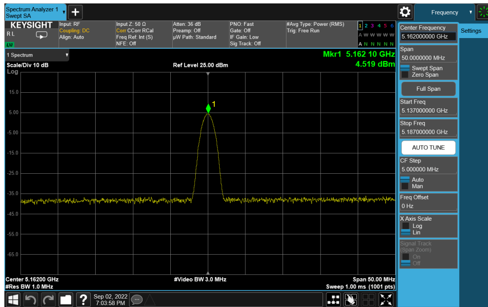
Plot 7-44. PSD TxBF Antenna 4a (BDR GFSK, iPA - 5162MHz)
