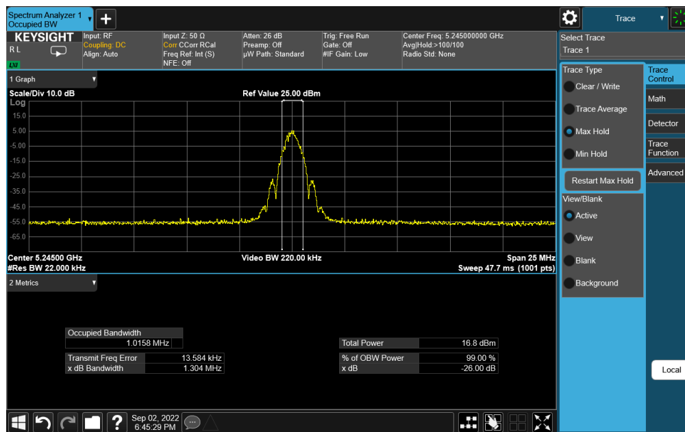
Plot 7-3. 26dB BW & 99% OBW Antenna 5b (BDR GFSK, ePA – 5245MHz)
