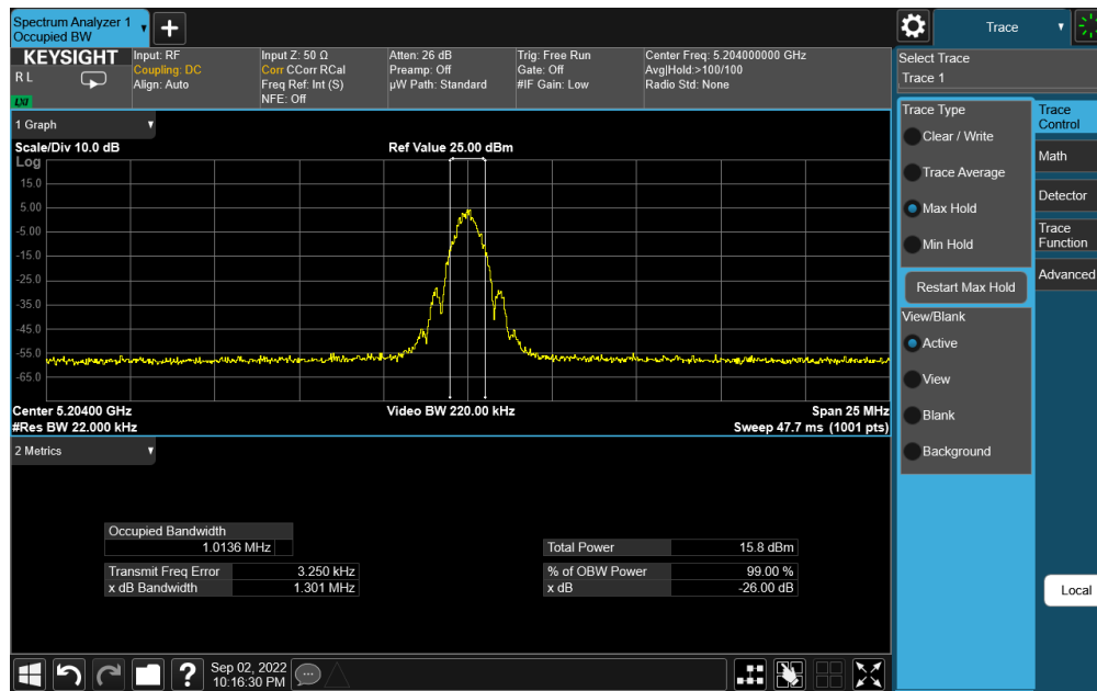
Plot 7-5. 26dB BW & 99% OBW Antenna 4a (BDR GFSK, ePA – 5204MHz)
