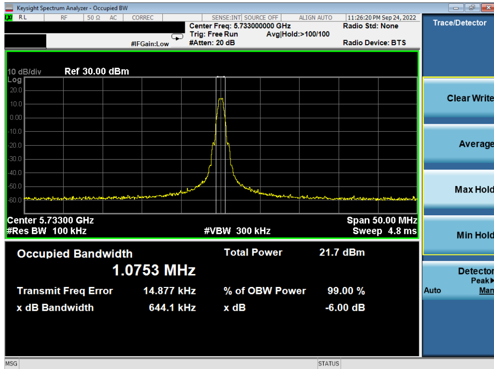
Plot 7-7. 6dB BW & 99% OBW Antenna 5b (BDR, ePA, 5733MHz)
