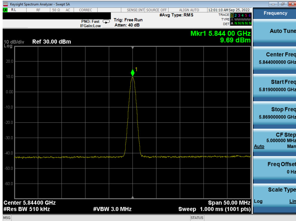
Plot 7-33. PSD Antenna 4a (BDR, ePA, 5844MHz)
