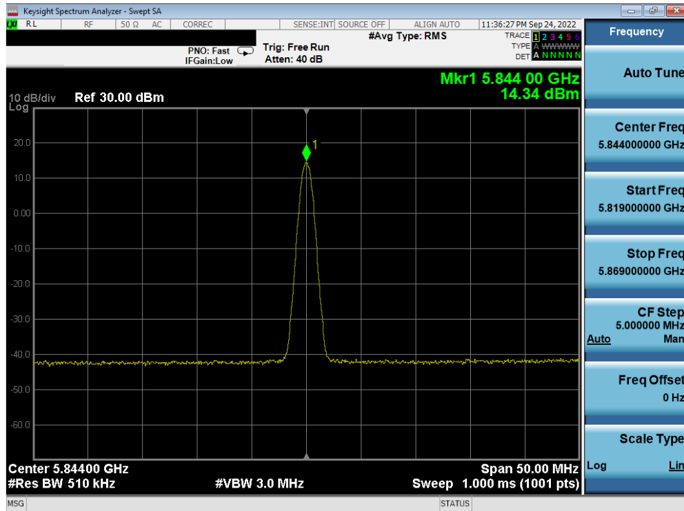
Plot 7-21. PSD Antenna 5b (BDR, ePA, 5844MHz)
