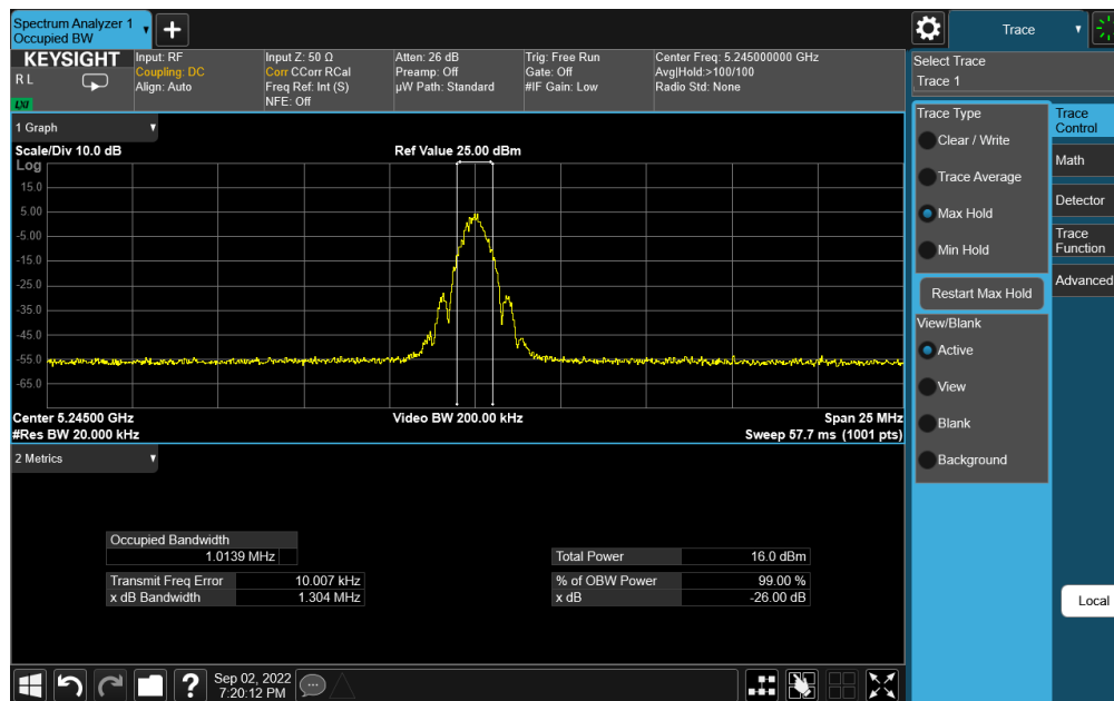
Plot 7-6. 26dB BW & 99% OBW Antenna 4a (BDR GFSK, ePA – 5245MHz)
