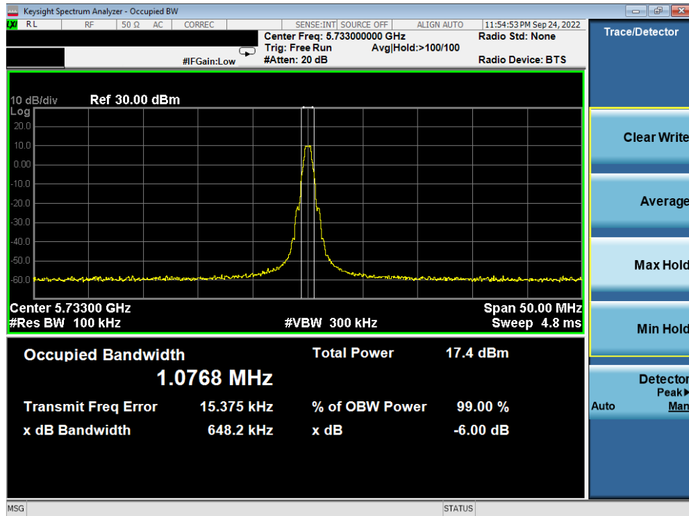
Plot 7-10. 6dB BW & 99% OBW Antenna 4a (BDR, ePA, 5733MHz)
