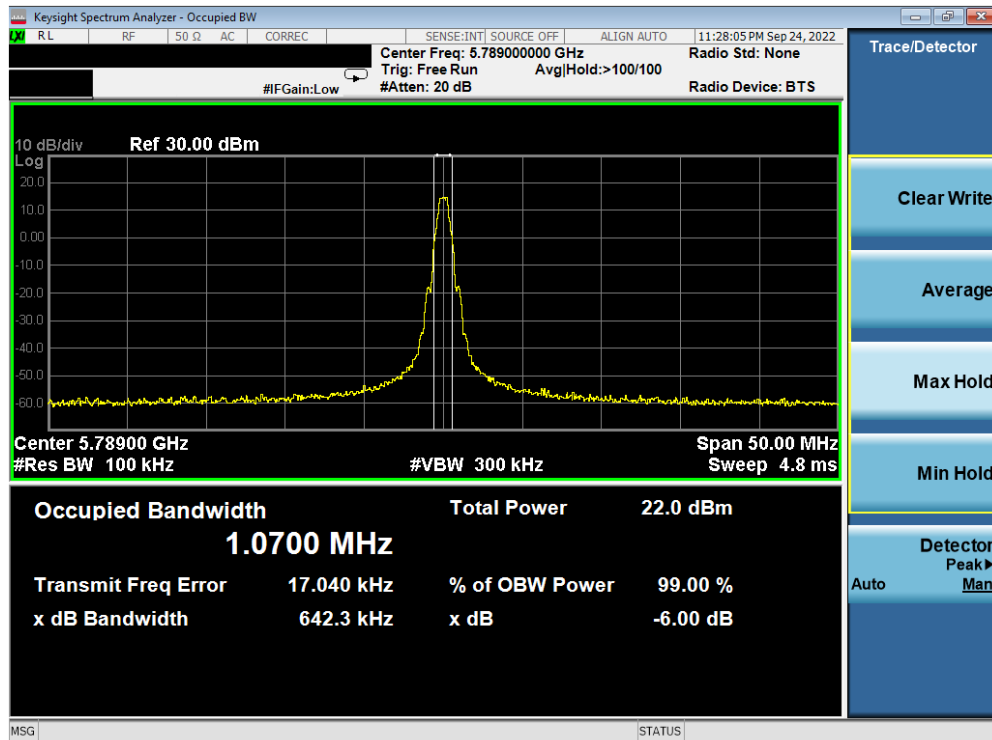
Plot 7-8. 6dB BW & 99% OBW Antenna 5b (BDR, ePA, 5789MHz)
