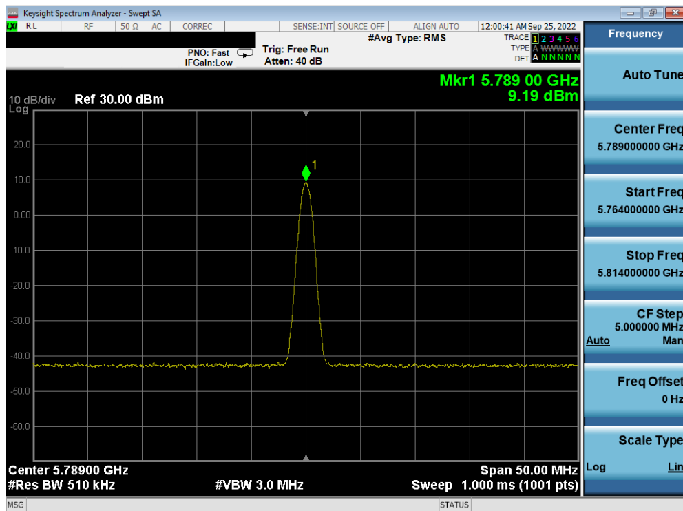
Plot 7-32. PSD Antenna 4a (BDR, ePA, 5789MHz)
