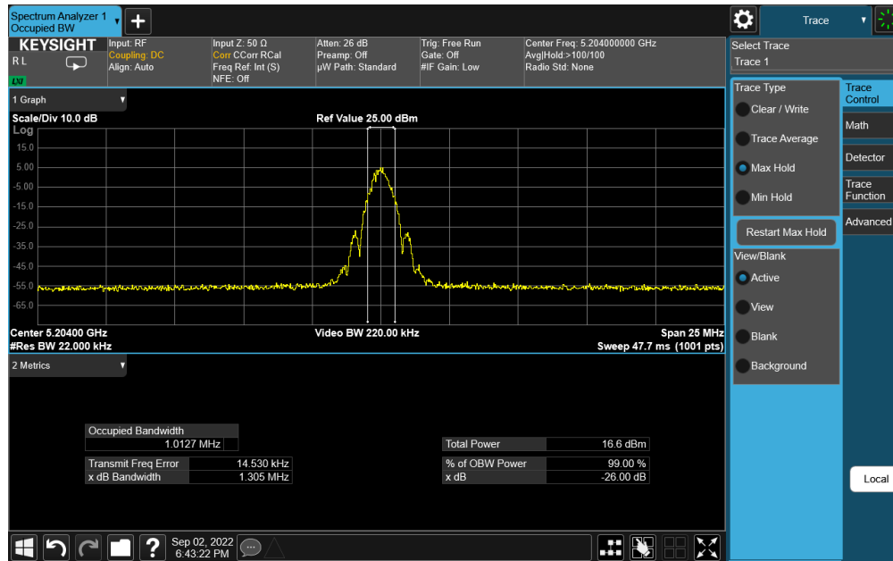
Plot 7-2. 26dB BW & 99% OBW Antenna 5b (BDR GFSK, ePA – 5204MHz)
