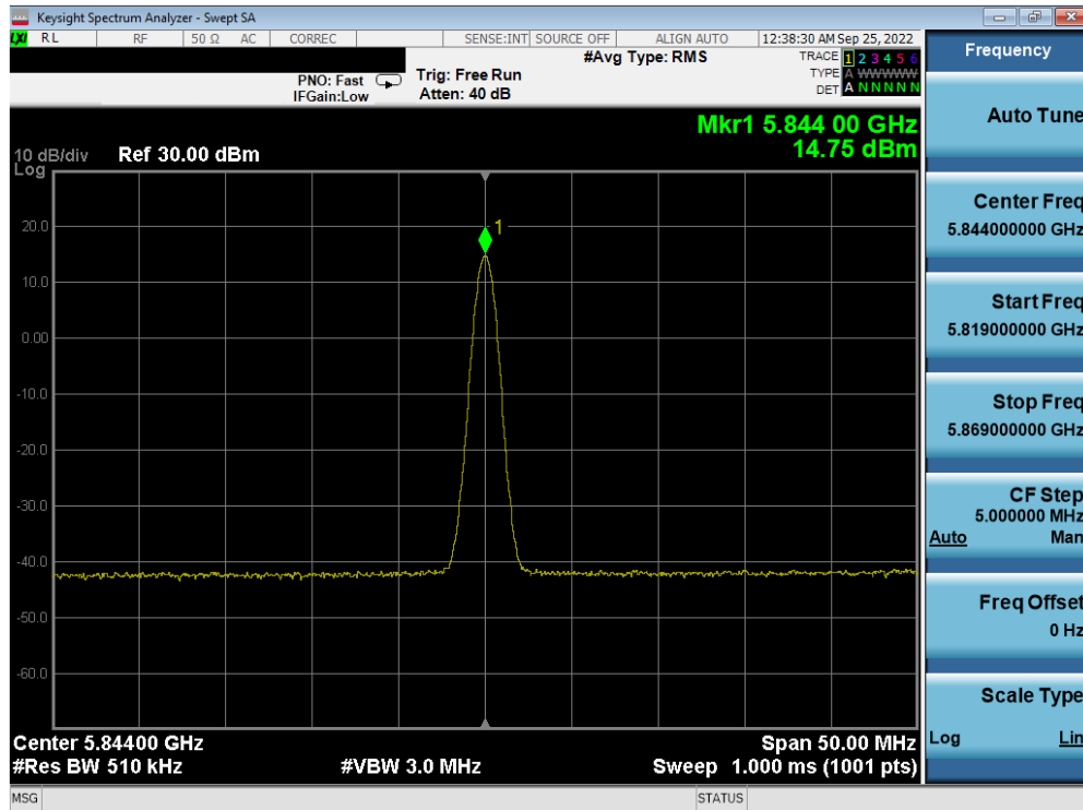
Plot 7-53. PSD TxBF Antenna 5b (BDR, ePA, 5844MHz)
