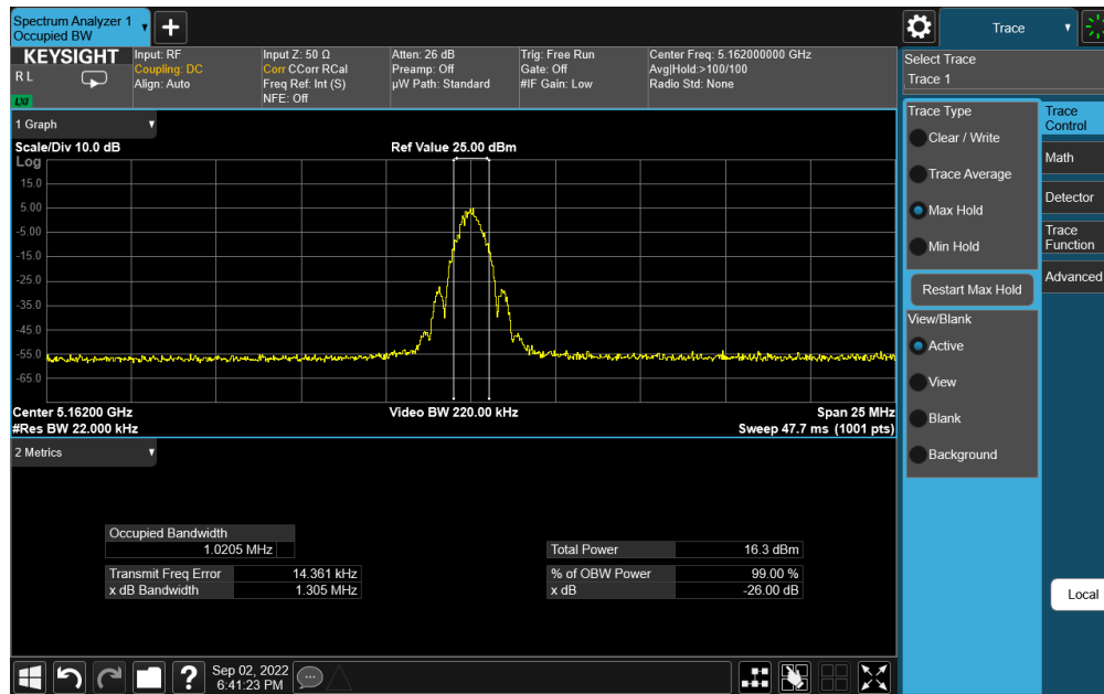
Plot 7-1. 26dB BW & 99% OBW Antenna 5b (BDR GFSK, ePA – 5162MHz)
