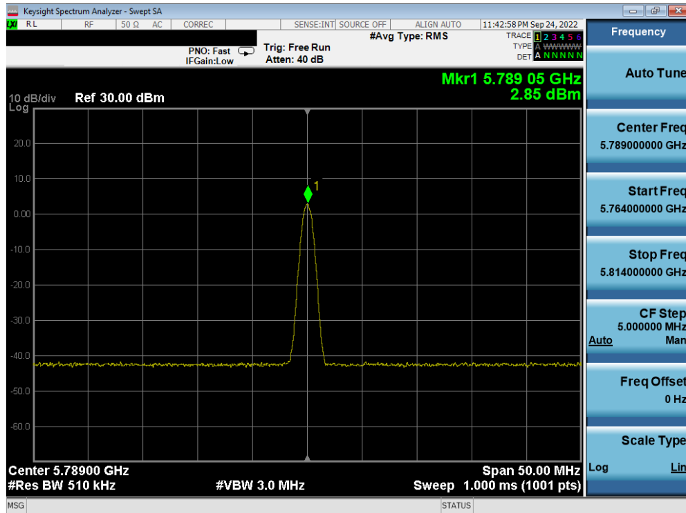
Plot 7-23. PSD Antenna 5b (BDR, iPA, 5789MHz)
