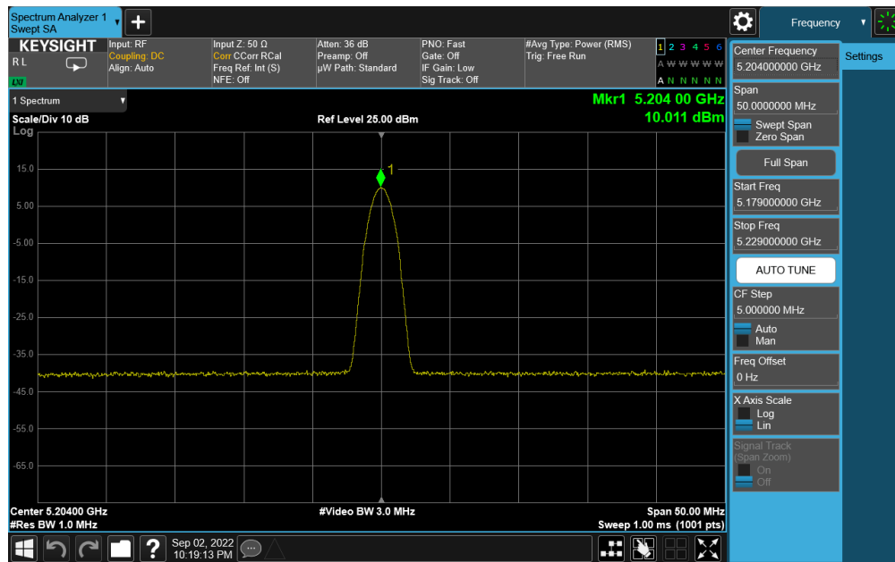
Plot 7-26. PSD Antenna 4a (BDR GFSK, ePA – 5204MHz)
