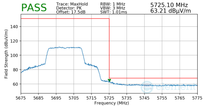
Plot 7-935. Antenna 4a (Pk, Ch.140, 802.11ax(SU), MCS2)
