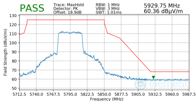
Plot 7-1003. Antenna 4a (Pk, Ch.159, 80.11ax(SU), MCS11)
