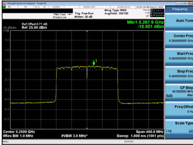
Plot 7-395. PSD CDD Antenna 5b (160MHz BW 802.11ax(SU) – Ch. 50, MCS2)
