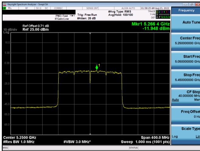
Plot 7-396. PSD CDD Antenna 4a (160MHz BW 802.11ax(SU) – Ch. 50, MCS2)
