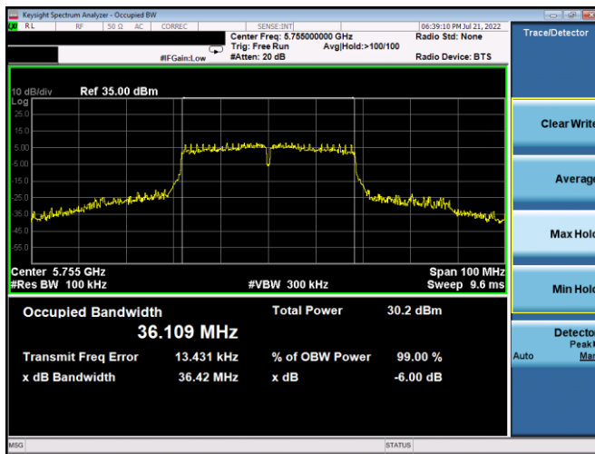
Plot 7-159. 6dB BW & 99% OBW Antenna 4a (40MHz BW 802.11n – Ch. 151, MCS4)
