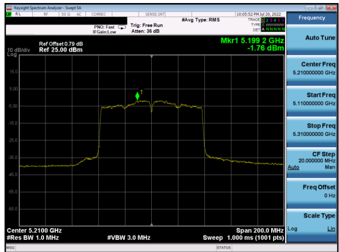
Plot 7-195. PSD Antenna 5b (80MHz BW 802.11ac – Ch. 42, MCS4)
