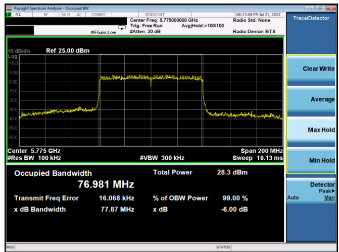
Plot 7-162. 6dB BW & 99% OBW Antenna 4a (80MHz BW 802.11ax(SU) – Ch. 155, MCS4)
