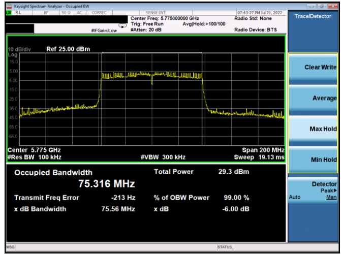
Plot 7-161. 6dB BW & 99% OBW Antenna 4a (80MHz BW 802.11ac – Ch. 155, MCS4)
