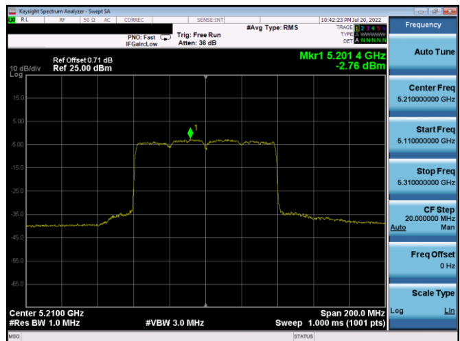
Plot 7-196. PSD Antenna 5b (80MHz BW 802.11ax(SU) – Ch. 42, MCS4)
