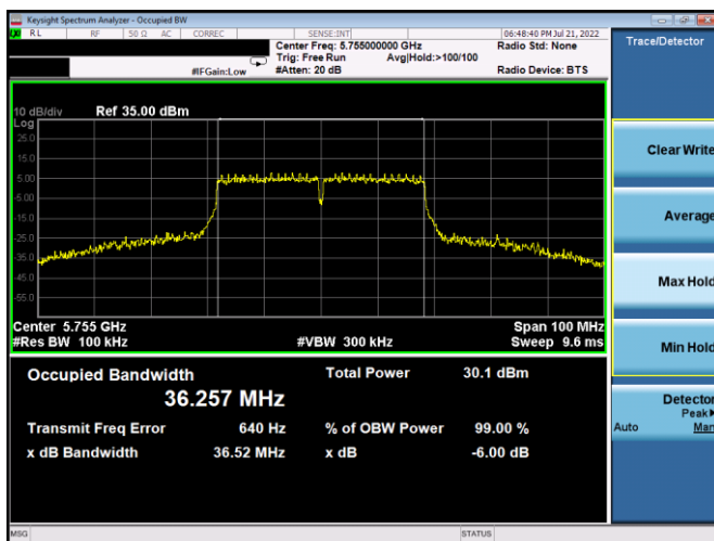
Plot 7-165. 6dB BW & 99% OBW Antenna 4a (40MHz BW 802.11n – Ch. 151, MCS9)
