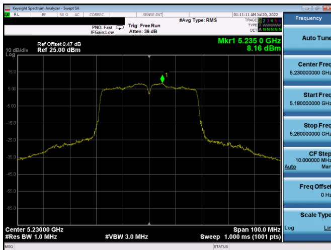
Plot 7-193. PSD Antenna 5b (40MHz BW 802.11n – Ch. 46, MCS4)
