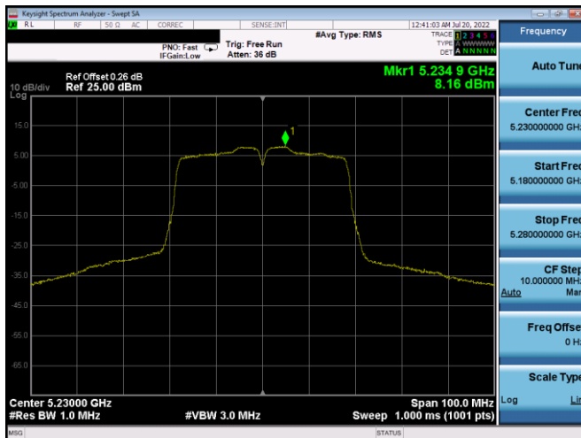
Plot 7-171. PSD Antenna 5b (40MHz BW 802.11n – Ch. 46, MCS2)
