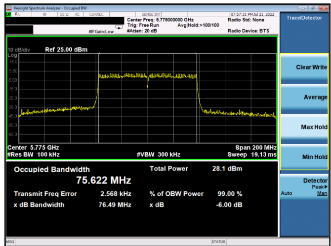
Plot 7-167. 6dB BW & 99% OBW Antenna 4a (80MHz BW 802.11ac – Ch. 155, MCS9)
