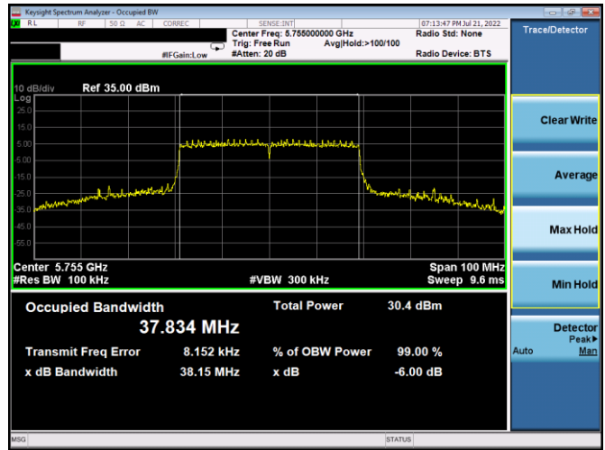
Plot 7-160. 6dB BW & 99% OBW Antenna 4a (40MHz BW 802.11ax (SU) – Ch. 151, MCS4)
