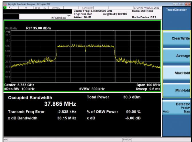
Plot 7-166. 6dB BW & 99% OBW Antenna 4a (40MHz BW 802.11ax(SU) – Ch. 151, MCS11)
