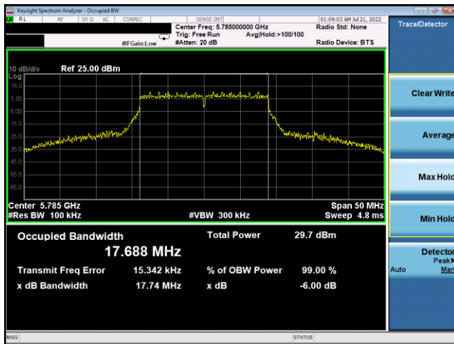
Plot 7-163. 6dB BW & 99% OBW Antenna 4a (20MHz BW 802.11n – Ch. 157, MCS7)
