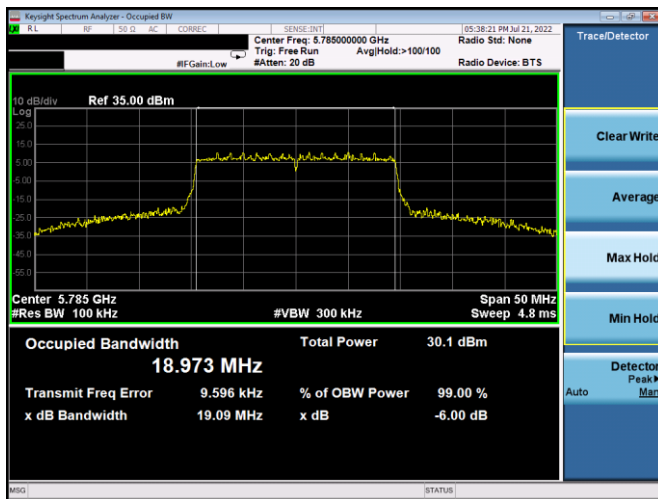
Plot 7-164. 6dB BW & 99% OBW Antenna 4a (20MHz BW 802.11ax(SU) – Ch. 157, MCS11)
