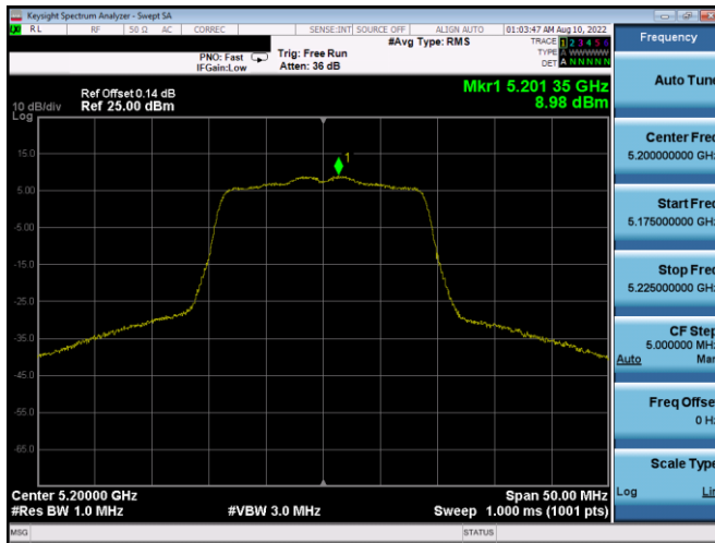
Plot 7-169. PSD Antenna 5b (20MHz BW 802.11n – Ch. 40, MCS2)
