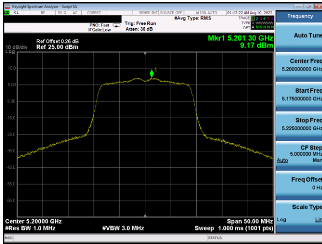
Plot 7-191. PSD Antenna 5b (20MHz BW 802.11n – Ch. 40, MCS4)
