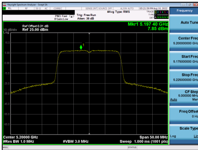
Plot 7-192. PSD Antenna 5b (20MHz BW 802.11ax(SU) – Ch. 40, MCS4)
