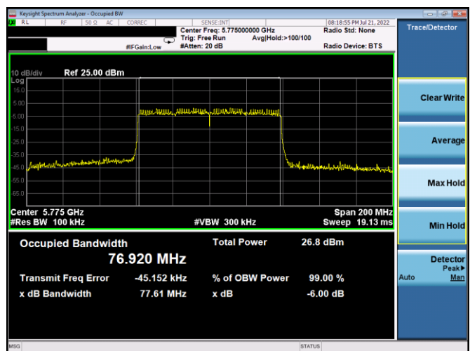
Plot 7-168. 6dB BW & 99% OBW Antenna 4a (80MHz BW 802.11ax(SU) – Ch. 155, MCS11)
