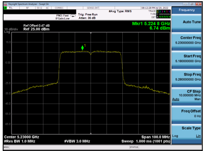
Plot 7-194. PSD Antenna 5b (40MHz BW 802.11ax(SU) – Ch. 46, MCS4)
