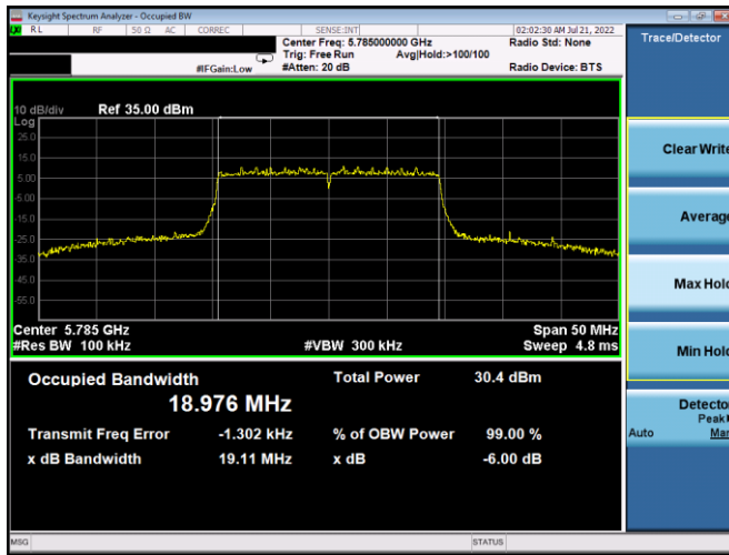
Plot 7-158. 6dB BW & 99% OBW Antenna 4a (20MHz BW 802.11ax(SU) – Ch. 157, MCS4)
