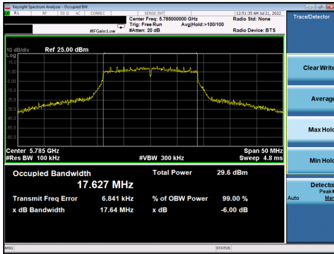
Plot 7-157. 6dB BW & 99% OBW Antenna 4a (20MHz BW 802.11n – Ch. 157, MCS4)
