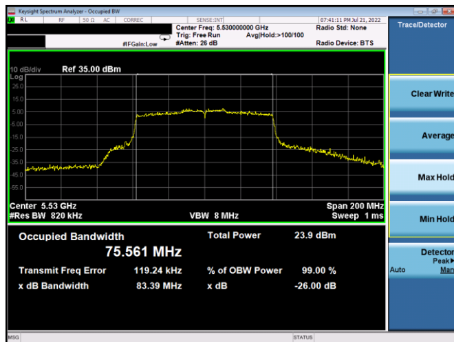
Plot 7-85. 26dB BW & 99% OBW Antenna 4a (80MHz BW 802.11ax(SU) – Ch. 106, MCS2)
