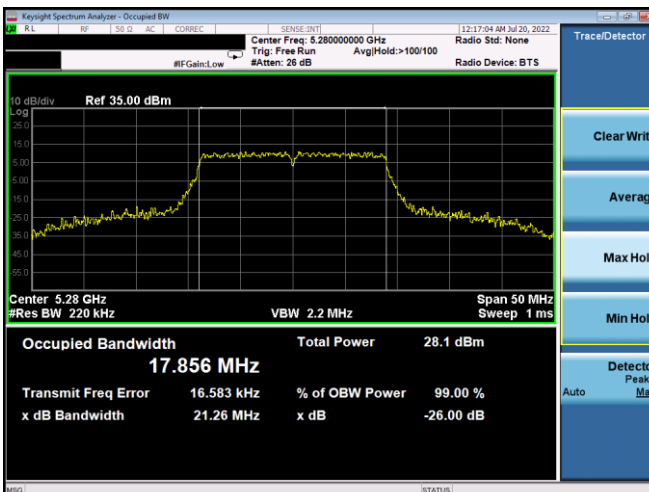
Plot 7-53. 26dB BW & 99% OBW Antenna 5b (20MHz BW 802.11n – Ch. 56, MCS7)
