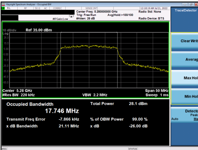
Plot 7-75. 26dB BW & 99% OBW Antenna 4a (20MHz BW 802.11n – Ch. 56, MCS2)
