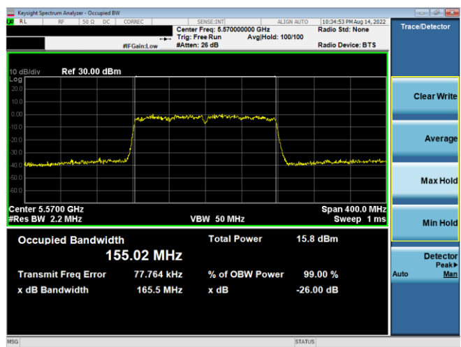
Plot 7-64. 26dB BW & 99% OBW Antenna 5b (160MHz BW 802.11ac – Ch. 114, MCS9)
