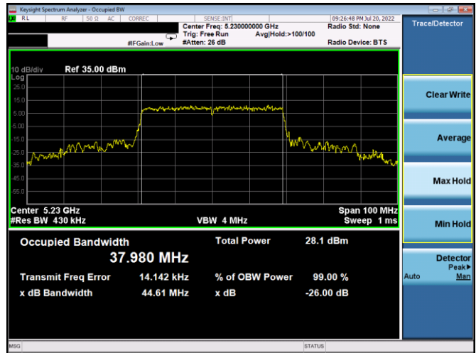
Plot 7-48. 26dB BW & 99% OBW Antenna 5b (40MHz BW 802.11ax(SU) - Ch. 46, MCS11)
