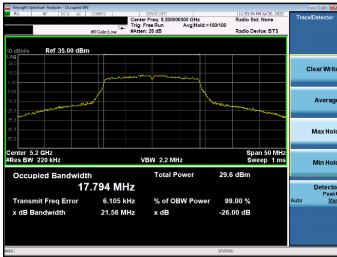
Plot 7-67. 26dB BW & 99% OBW Antenna 4a (20MHz BW 802.11n – Ch. 40, MCS2)
