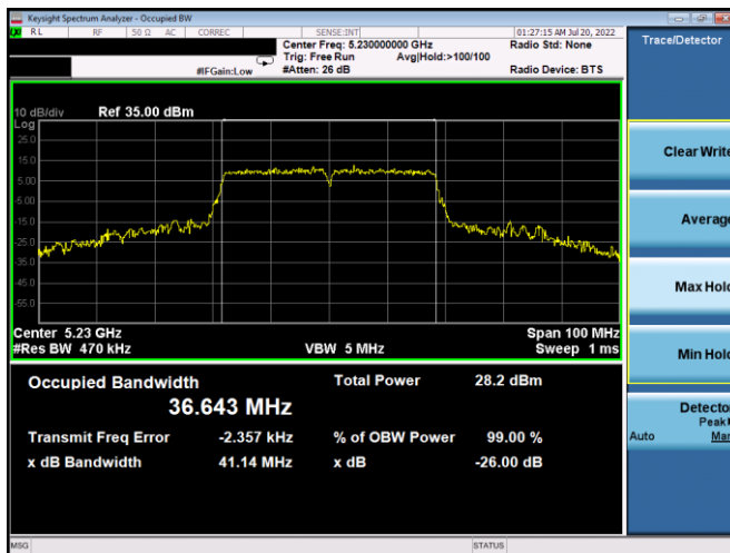
Plot 7-47. 26dB BW & 99% OBW Antenna 5b (40MHz BW 802.11n - Ch. 46, MCS7)
