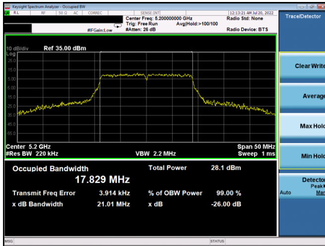
Plot 7-45. 26dB BW & 99% OBW Antenna 5b (20MHz BW 802.11n - Ch. 40, MCS7)
