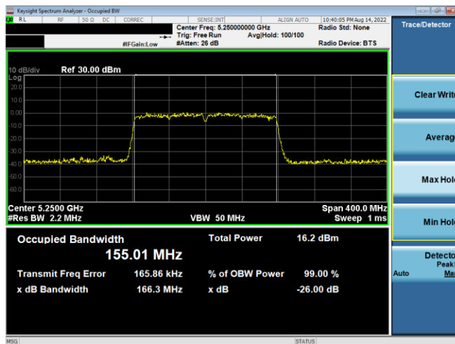
Plot 7-52. 26dB BW & 99% OBW Antenna 5b (160MHz BW 802.11ac – Ch. 50, MCS7)
