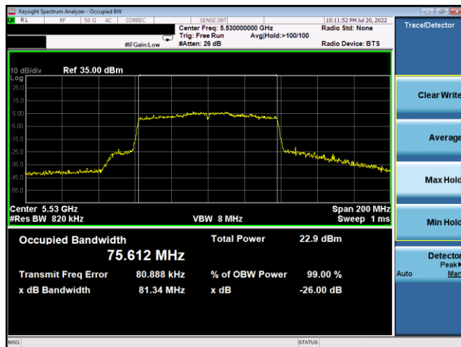
Plot 7-41. 26dB BW & 99% OBW Antenna 5b (80MHz BW 802.11ac – Ch. 106, MCS4)
