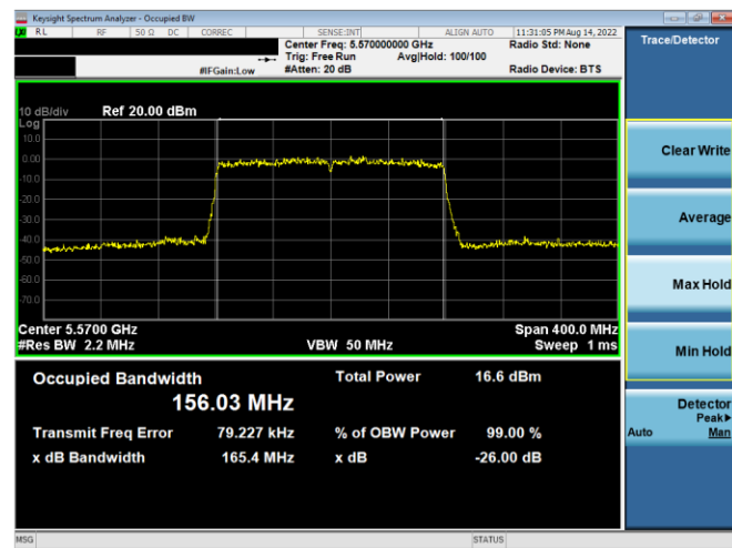
Plot 7-43. 26dB BW & 99% OBW Antenna 5b (160MHz BW 802.11ax – Ch. 114, MCS0)
