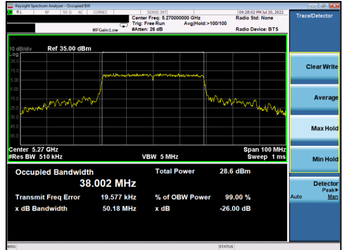
Plot 7-56. 26dB BW & 99% OBW Antenna 5b (40MHz BW 802.11ax(SU) – Ch. 54, MCS11)
