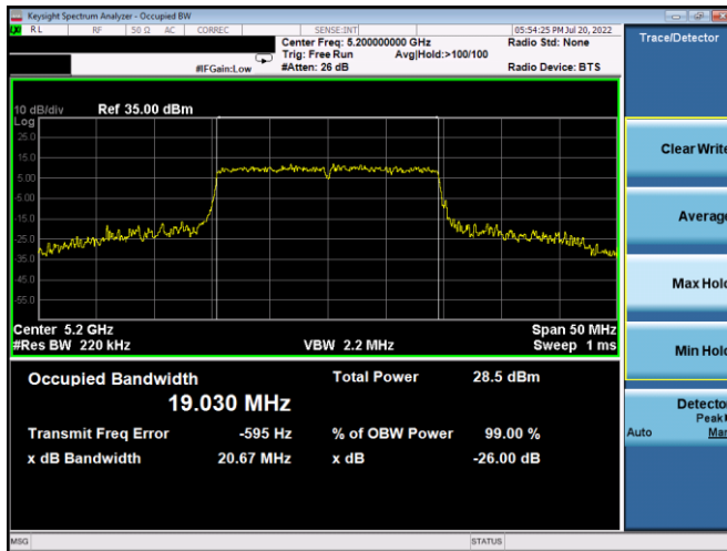
Plot 7-46. 26dB BW & 99% OBW Antenna 5b (20MHz BW 802.11ax(SU) - Ch. 40, MCS11)
