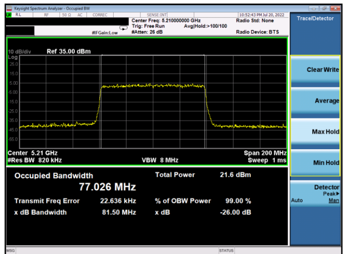
Plot 7-50. 26dB BW & 99% OBW Antenna 5b (80MHz BW 802.11ax(SU) - Ch. 42, MCS11)
