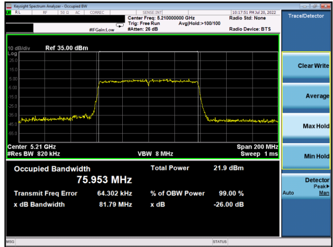
Plot 7-49. 26dB BW & 99% OBW Antenna 5b (80MHz BW 802.11ac - Ch. 42, MCS9)
