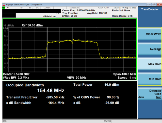
Plot 7-44. 26dB BW & 99% OBW Antenna 5b (160MHz BW 802.11ac – Ch. 114, MCS0)
