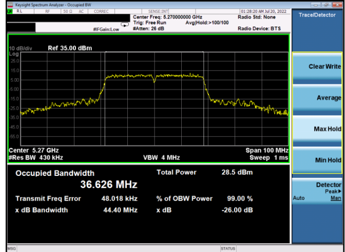
Plot 7-55. 26dB BW & 99% OBW Antenna 5b (40MHz BW 802.11n – Ch. 54, MCS7)
