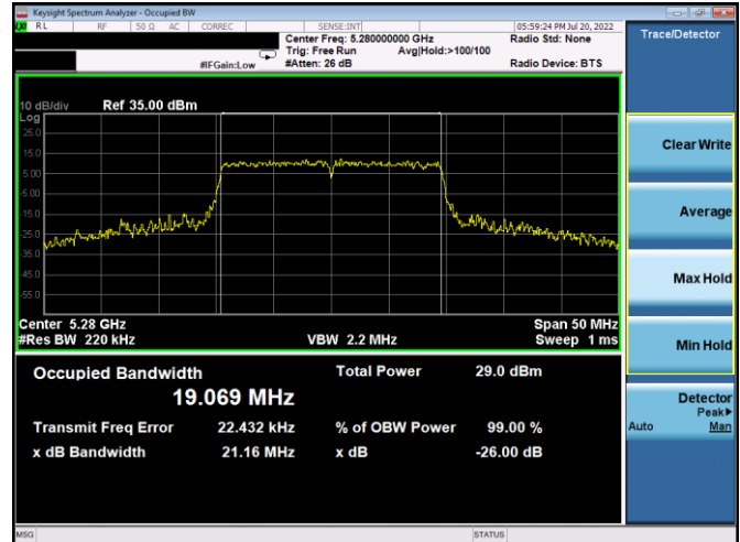
Plot 7-54. 26dB BW & 99% OBW Antenna 5b (20MHz BW 802.11ax(SU) – Ch. 56, MCS11)
