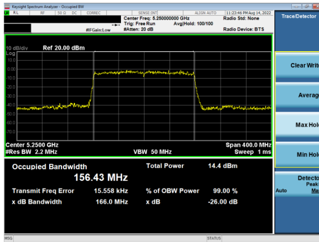
Plot 7-51. 26dB BW & 99% OBW Antenna 5b (160MHz BW 802.11ax – Ch. 50, MCS7)
