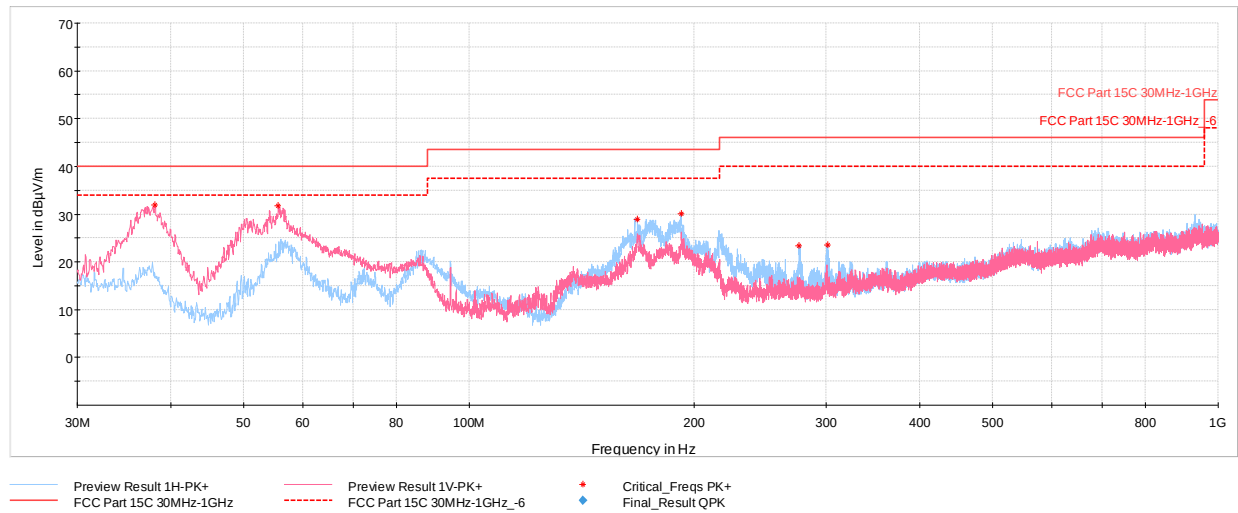
Plot 7-666. RSE below 1GHz SDM (RU26 – Ch.36), with AC/DC Adapter
