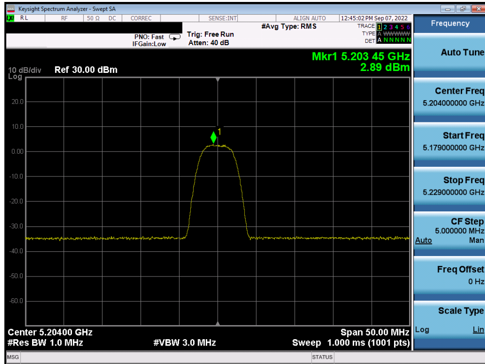
Plot 7-81. PSD TxBF Antenna WF5T (HDR8, ePA, 5204MHz)
