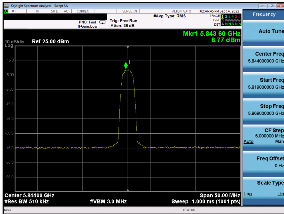
Plot 7-101. PSD TxBF Antenna WF5T (HDR4, ePA, 5844MHz)
