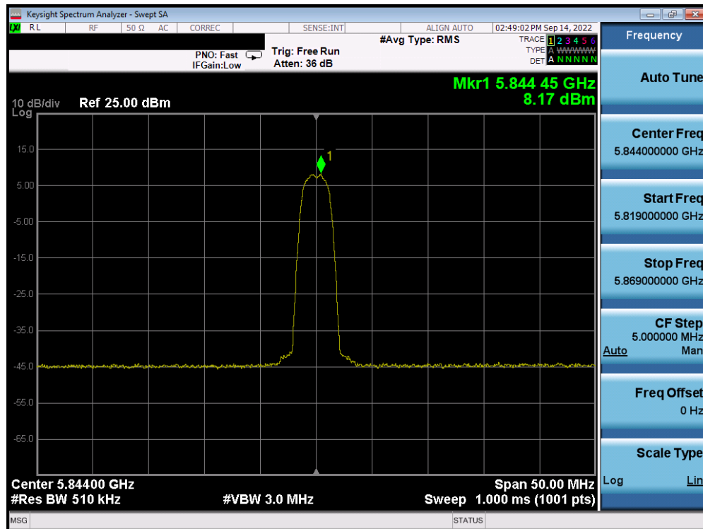
Plot 7-102. PSD TxBF Antenna WF5B (HDR4, ePA, 5844MHz)
