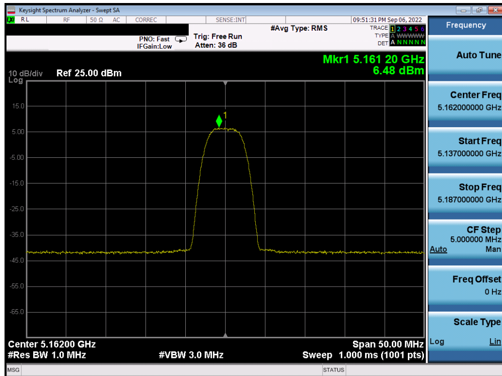
Plot 7-28. PSD Antenna WF5T (HDR8, ePA, 5162MHz)
