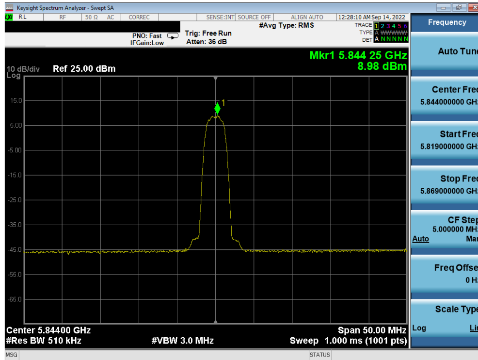
Plot 7-63. PSD Antenna WF5B (HDR4, ePA, 5844MHz)
