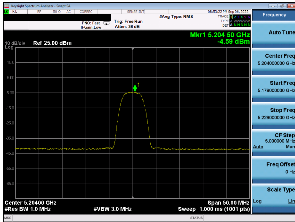
Plot 7-59. PSD Antenna WF5B (HDR8, iPA, 5204MHz)
