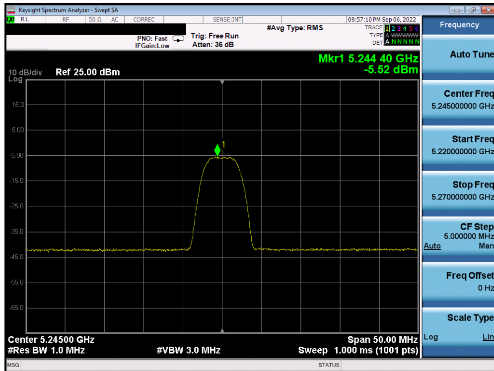
Plot 7-36. PSD Antenna WF5T (HDR8, iPA, 5245MHz)
