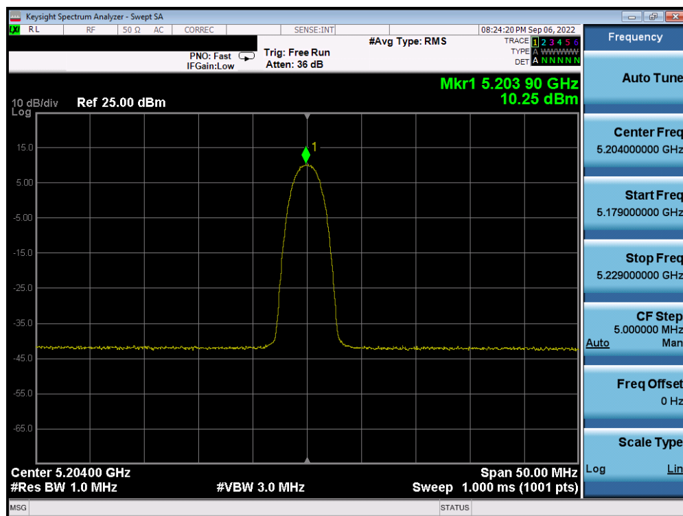
Plot 7-50. PSD Antenna WF5B (HDR4, ePA, 5204MHz)
