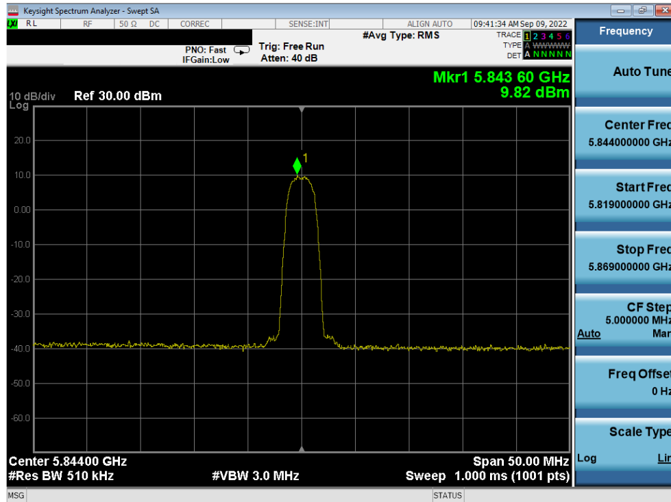
Plot 7-39. PSD Antenna WF5T (HDR4, ePA, 5844MHz)
