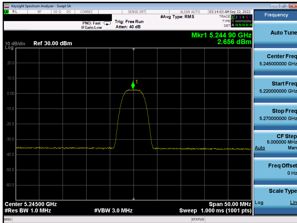
Plot 7-84. PSD TxBF Antenna WF5B (HDR8, ePA, 5245MHz)
