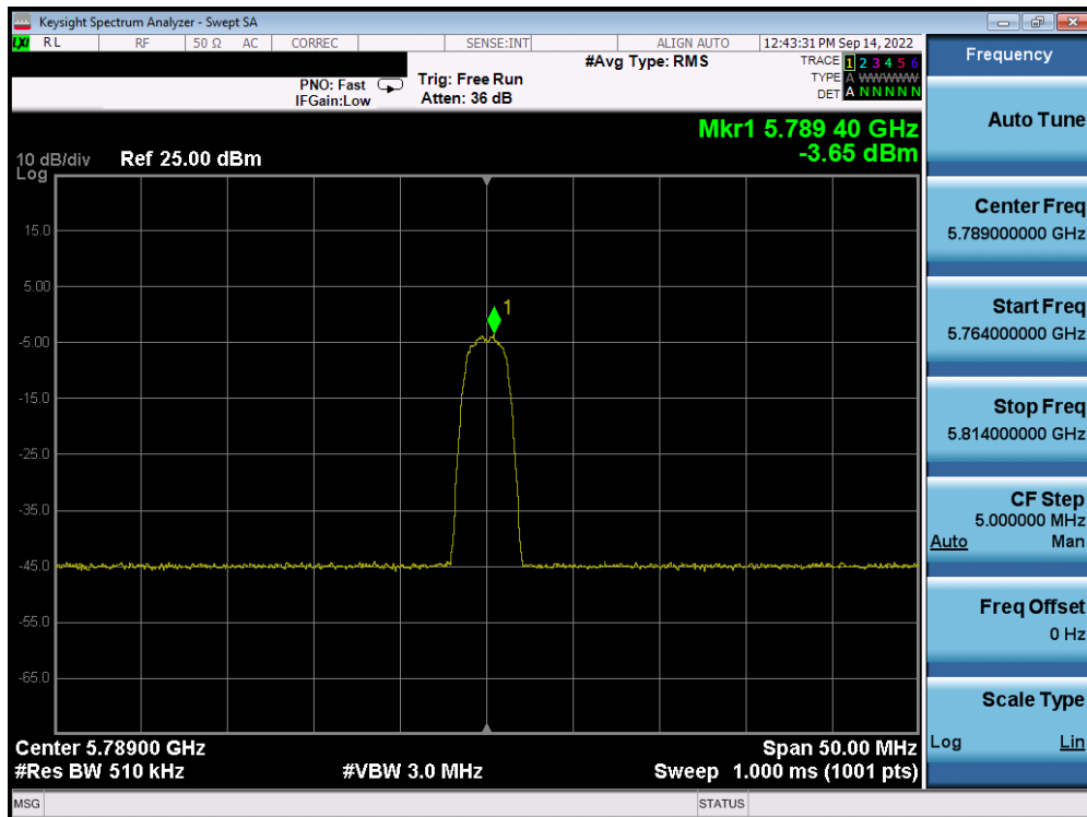
Plot 7-44. PSD Antenna WF5T (HDR4, iPA, 5789MHz)
