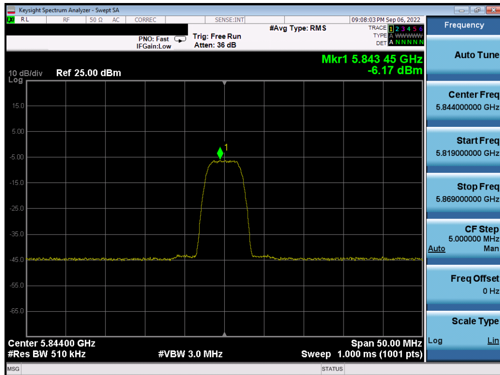
Plot 7-72. PSD Antenna WF5B (HDR8, iPA, 5844MHz)
