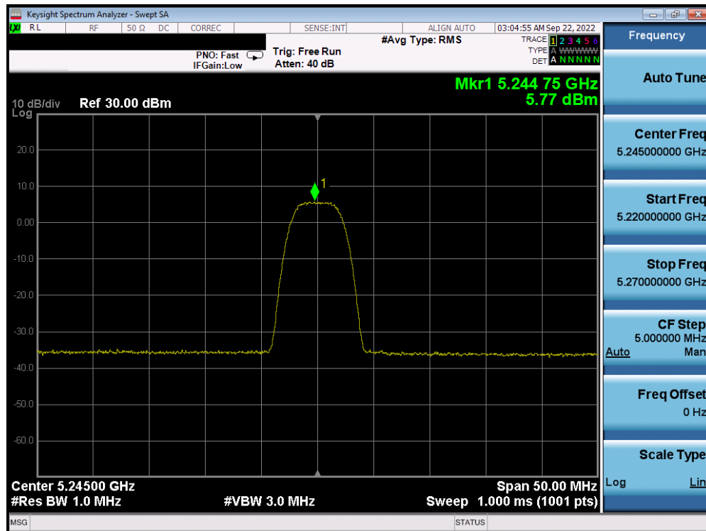
Plot 7-54. PSD Antenna WF5B (HDR8, ePA, 5245MHz)
