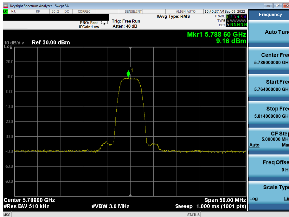
Plot 7-65. PSD Antenna WF5B (HDR8, ePA, 5789MHz)
