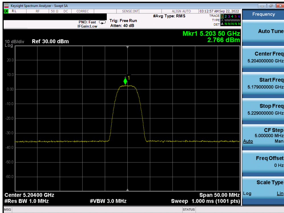
Plot 7-82. PSD TxBF Antenna WF5B (HDR8, ePA, 5204MHz)
