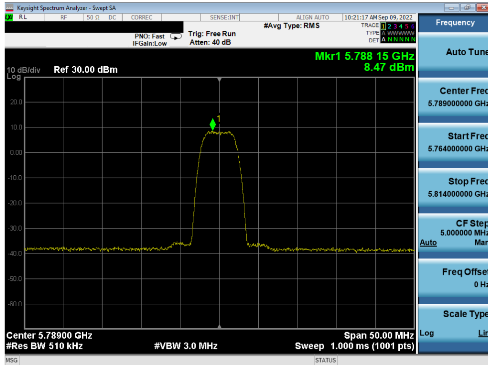
Plot 7-41. PSD Antenna WF5T (HDR8, ePA, 5789MHz)
