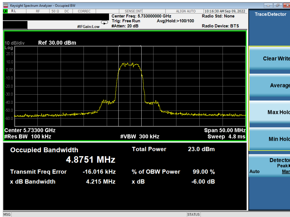
Plot 7-16. 6dB BW & 99% OBW Antenna WF5T (HDR8, ePA, 5733MHz)
