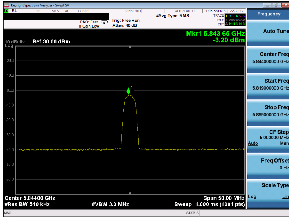
Plot 7-45. PSD Antenna WF5T (HDR4, iPA, 5844MHz)
