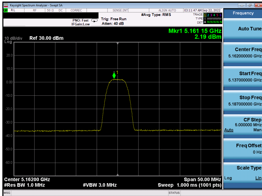
Plot 7-80. PSD TxBF Antenna WF5B (HDR8, ePA, 5162MHz)
