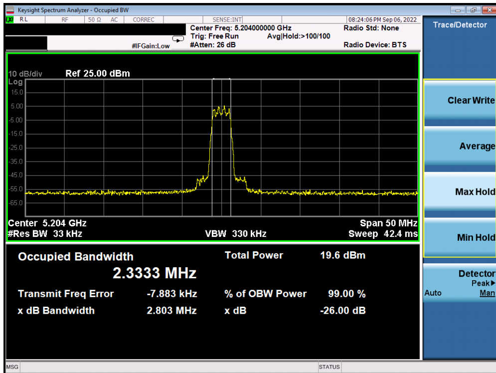
Plot 7-8. 26dB BW & 99% OBW Antenna WF5B (HDR4, ePA, 5204MHz)
