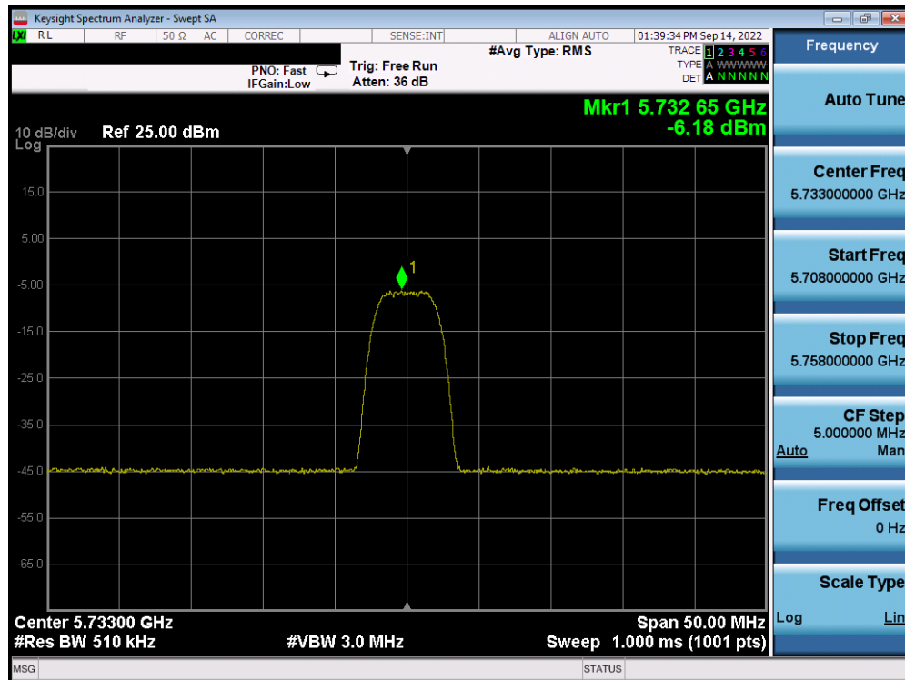
Plot 7-46. PSD Antenna WF5T (HDR8, iPA, 5733MHz)
