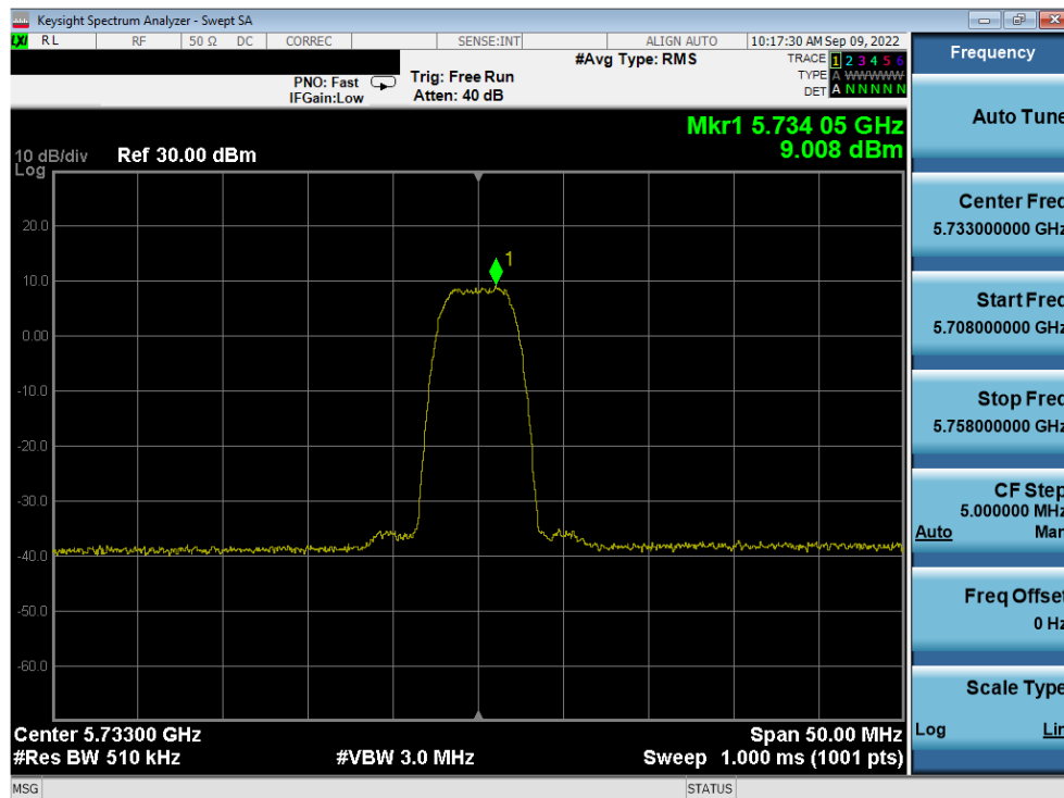
Plot 7-40. PSD Antenna WF5T (HDR8, ePA, 5733MHz)
