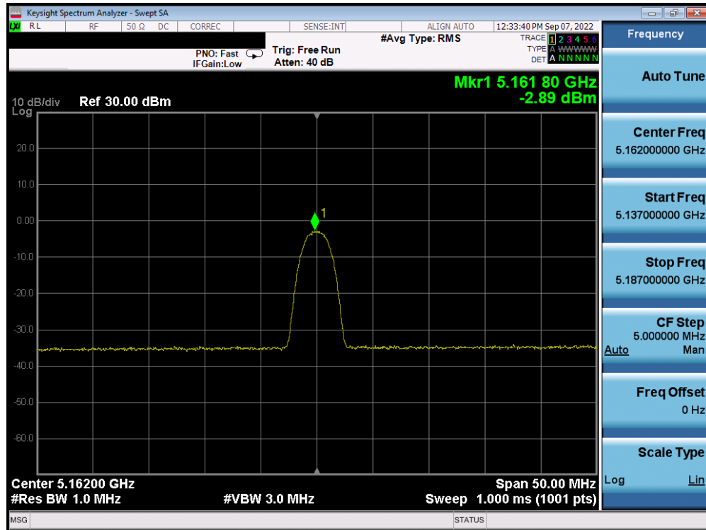
Plot 7-85. PSD TxBF Antenna WF5T (HDR4, iPA, 5162MHz)
