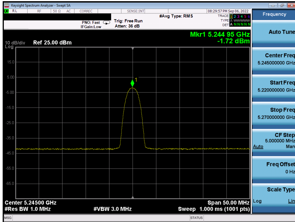
Plot 7-57. PSD Antenna WF5B (HDR4, iPA, 5245MHz)
