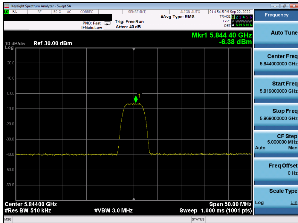
Plot 7-48. PSD Antenna WF5T (HDR8, iPA, 5844MHz)
