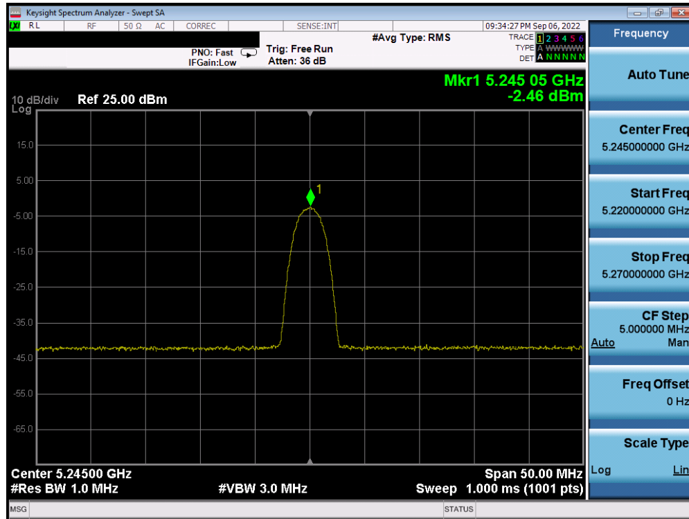
Plot 7-33. PSD Antenna WF5T (HDR4, iPA, 5245MHz)
