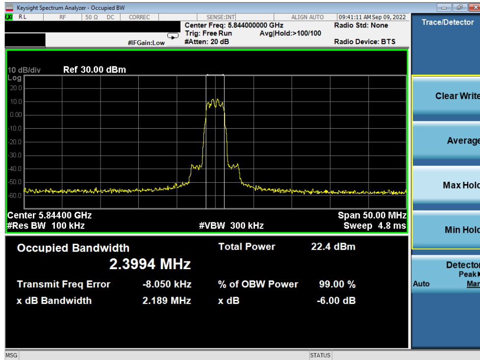
Plot 7-15. 6dB BW & 99% OBW Antenna WF5T (HDR4, ePA, 5844MHz)
