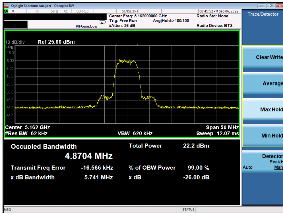
Plot 7-10. 26dB BW & 99% OBW Antenna WF5B (HDR8, ePA, 5162MHz)
