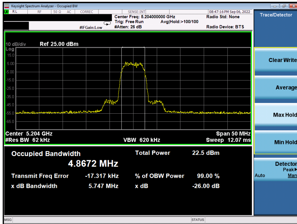
Plot 7-11. 26dB BW & 99% OBW Antenna WF5B (HDR8, ePA, 5204MHz)
