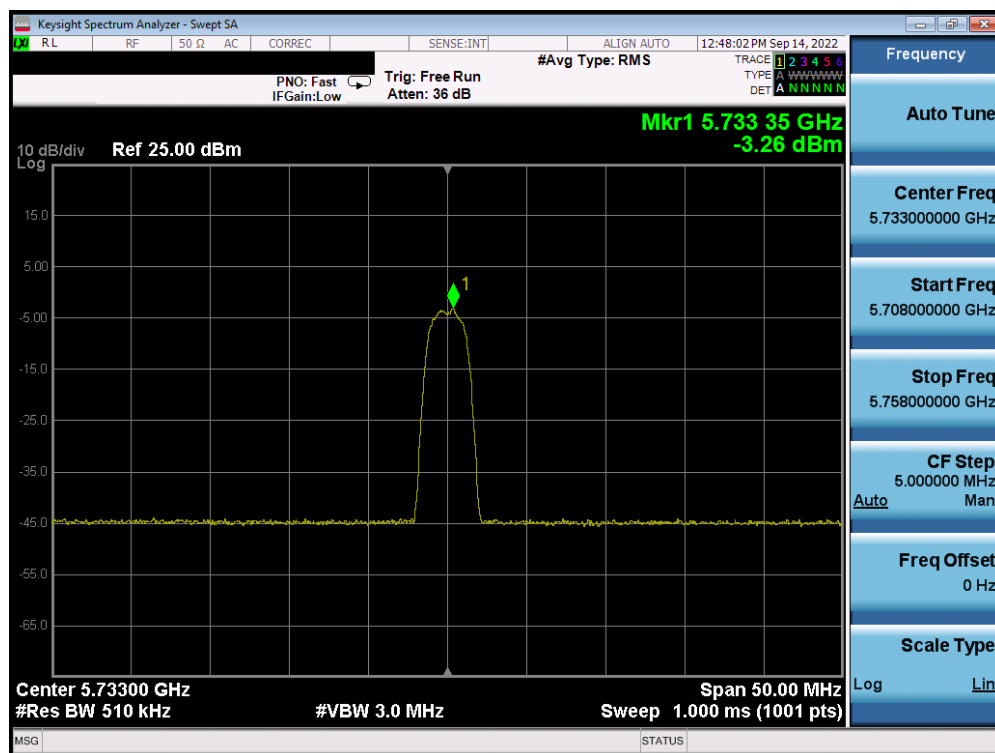
Plot 7-67. PSD Antenna WF5B (HDR4, iPA, 5733MHz)
