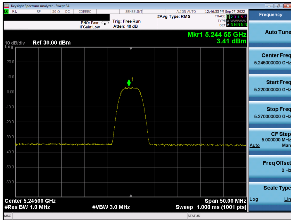
Plot 7-83. PSD TxBF Antenna WF5T (HDR8, ePA, 5245MHz)
