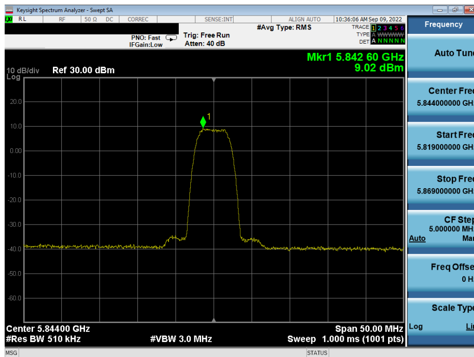
Plot 7-66. PSD Antenna WF5B (HDR8, ePA, 5844MHz)
