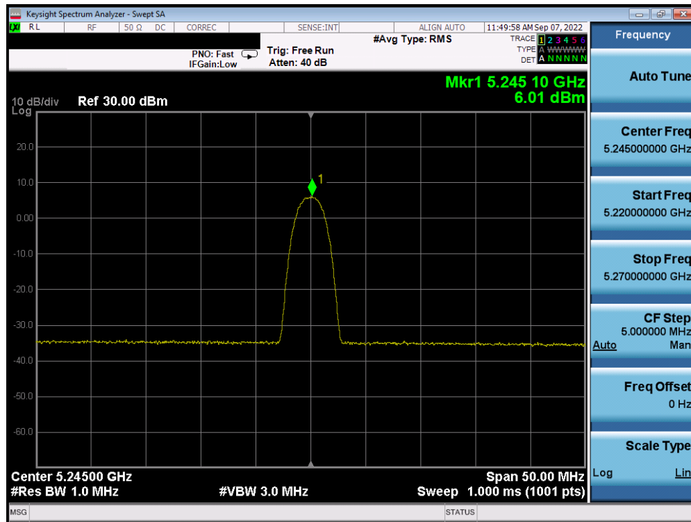
Plot 7-77. PSD TxBF Antenna WF5T (HDR4, ePA, 5245MHz)
