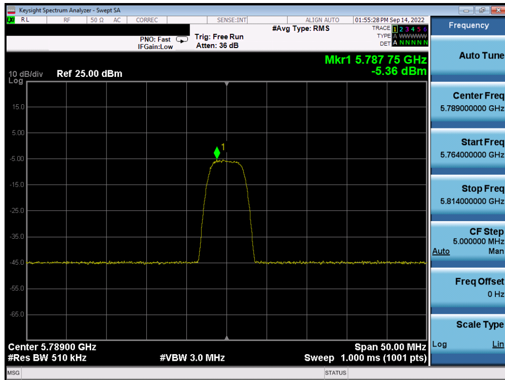
Plot 7-71. PSD Antenna WF5B (HDR8, iPA, 5789MHz)
