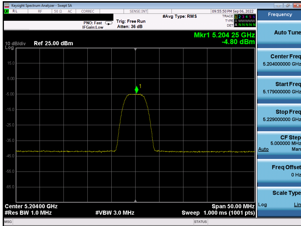
Plot 7-35. PSD Antenna WF5T (HDR8, iPA, 5204MHz)
