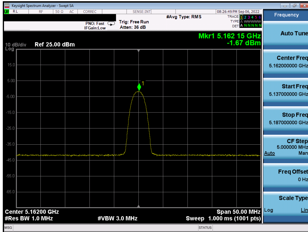
Plot 7-55. PSD Antenna WF5B (HDR4, iPA, 5162MHz)
