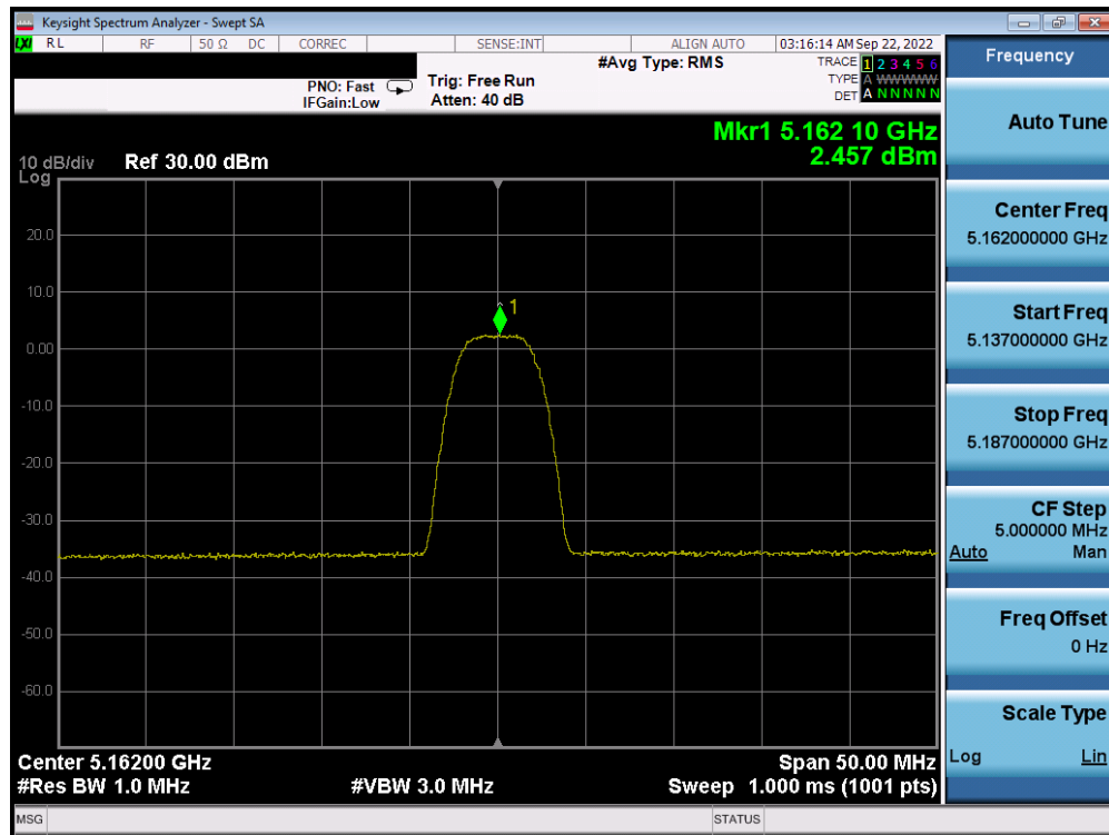
Plot 7-79. PSD TxBF Antenna WF5T (HDR8, ePA, 5162MHz)
