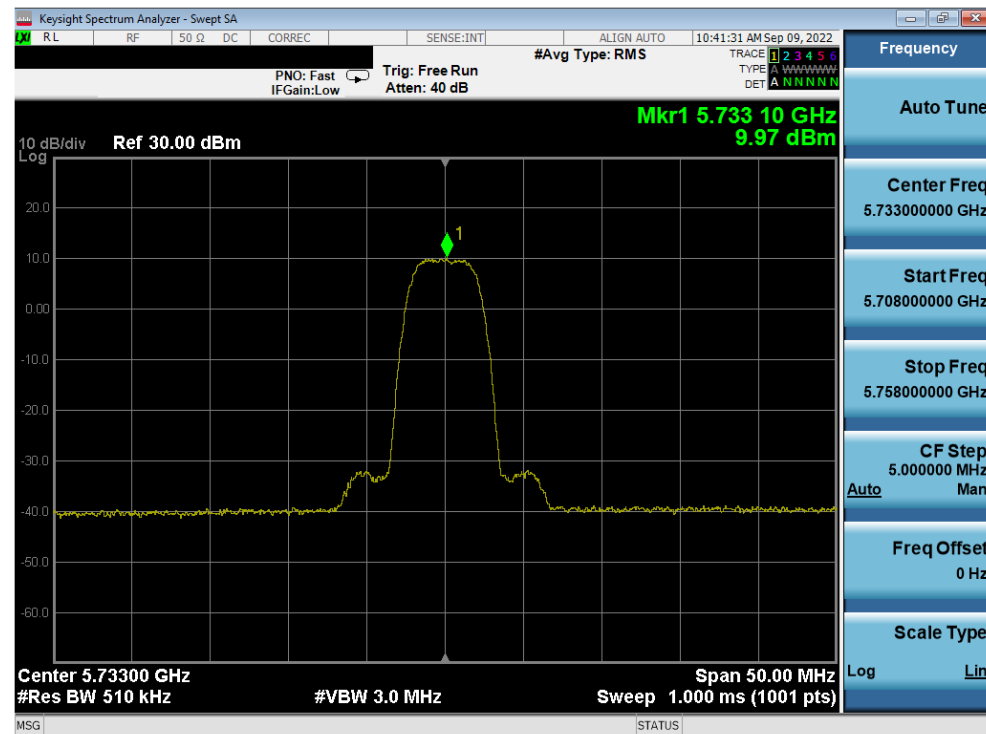
Plot 7-64. PSD Antenna WF5B (HDR8, ePA, 5733MHz)
