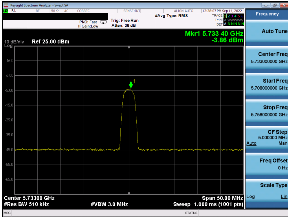
Plot 7-43. PSD Antenna WF5T (HDR4, iPA, 5733MHz)
