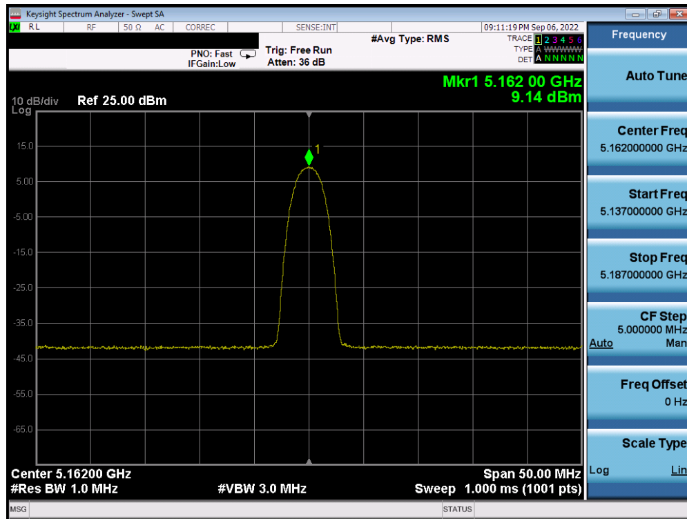
Plot 7-25. PSD Antenna WF5T (HDR4, ePA, 5162MHz)
