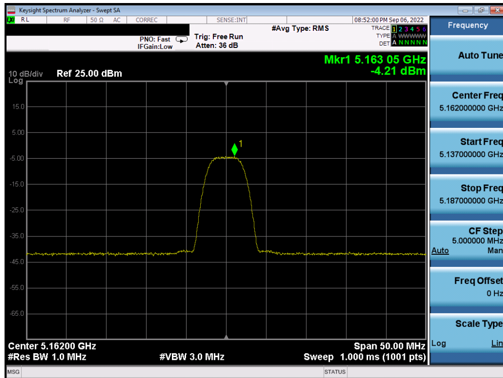
Plot 7-58. PSD Antenna WF5B (HDR8, iPA, 5162MHz)
