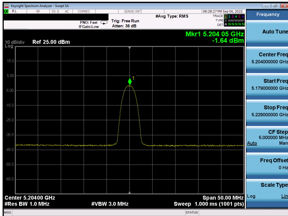
Plot 7-56. PSD Antenna WF5B (HDR4, iPA, 5204MHz)
