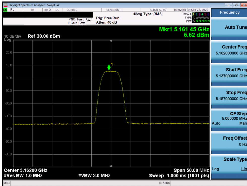
Plot 7-52. PSD Antenna WF5B (HDR8, ePA, 5162MHz)
