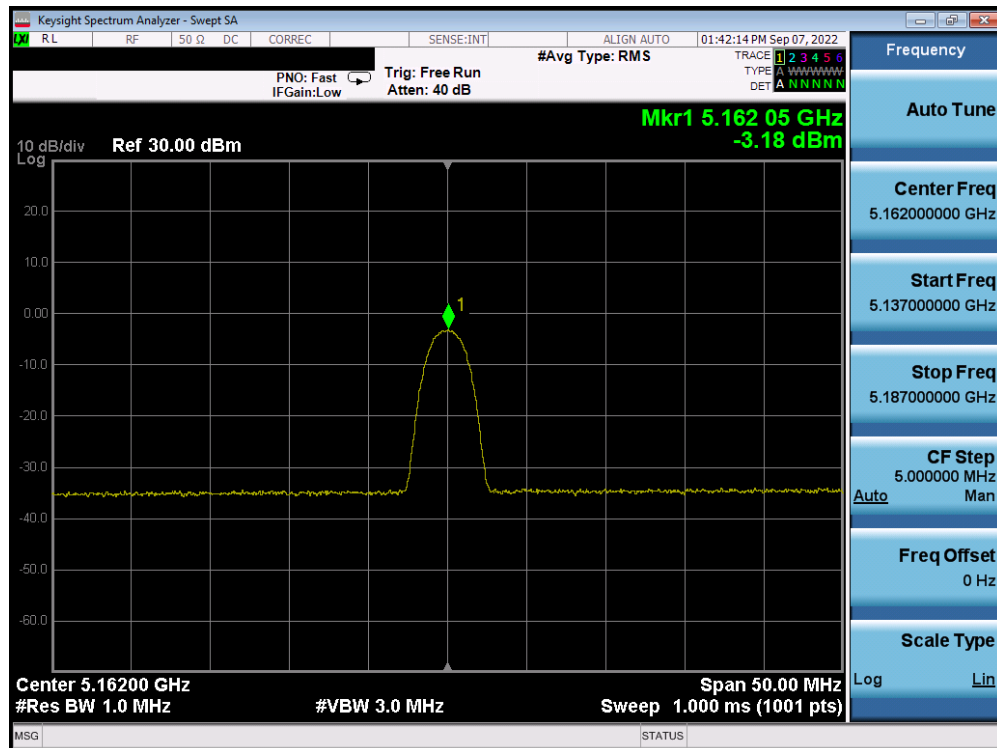
Plot 7-86. PSD TxBF Antenna WF5B (HDR4, iPA, 5162MHz)
