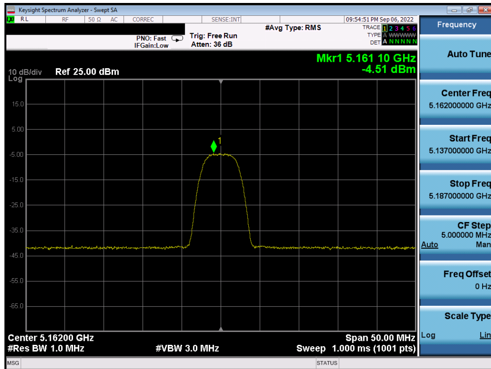
Plot 7-34. PSD Antenna WF5T (HDR8, iPA, 5162MHz)
