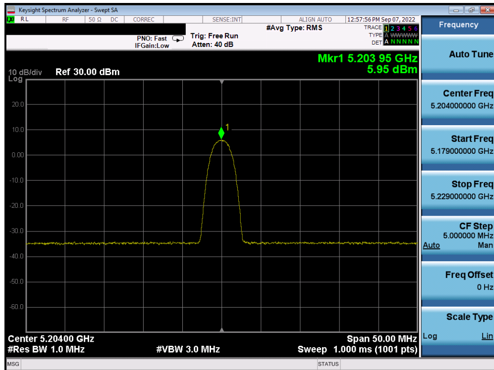
Plot 7-76. PSD TxBF Antenna WF5B (HDR4, ePA, 5204MHz)
