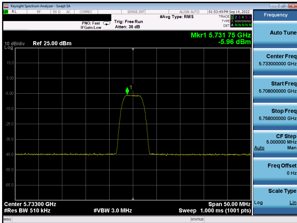
Plot 7-70. PSD Antenna WF5B (HDR8, iPA, 5733MHz)
