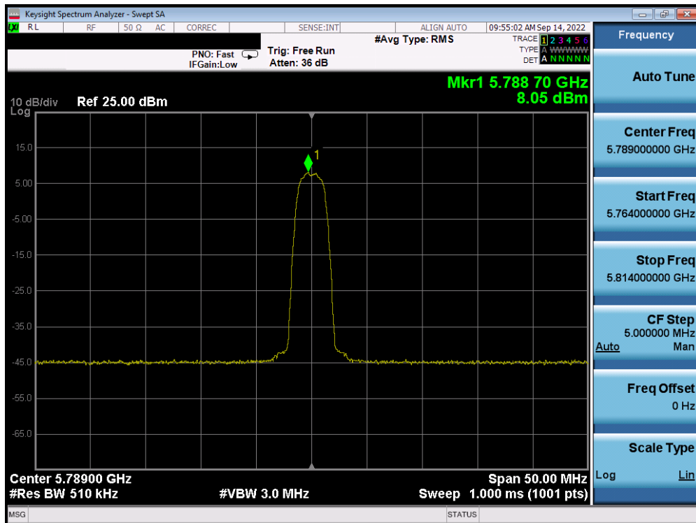
Plot 7-62. PSD Antenna WF5B (HDR4, ePA, 5789MHz)
