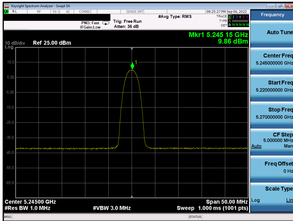
Plot 7-51. PSD Antenna WF5B (HDR4, ePA, 5245MHz)
