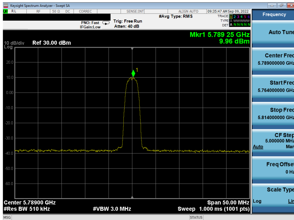
Plot 7-38. PSD Antenna WF5T (HDR4, ePA, 5789MHz)
