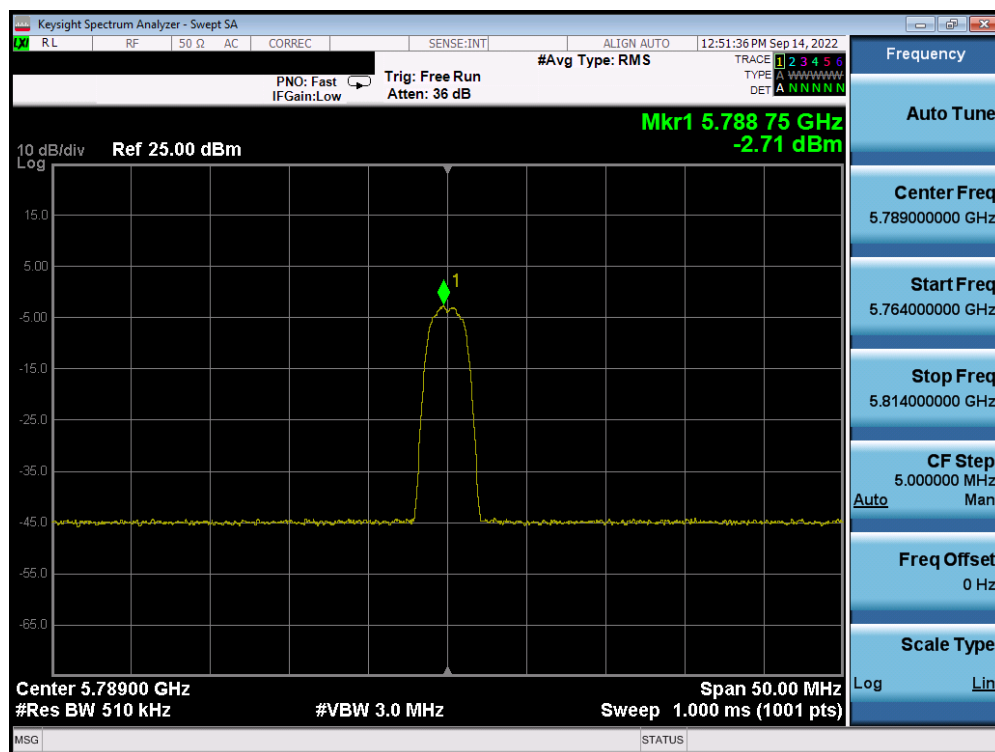
Plot 7-68. PSD Antenna WF5B (HDR4, iPA, 5789MHz)
