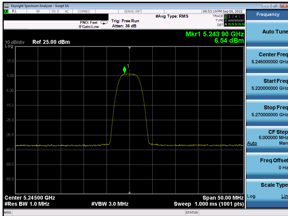
Plot 7-30. PSD Antenna WF5T (HDR8, ePA, 5245MHz)
