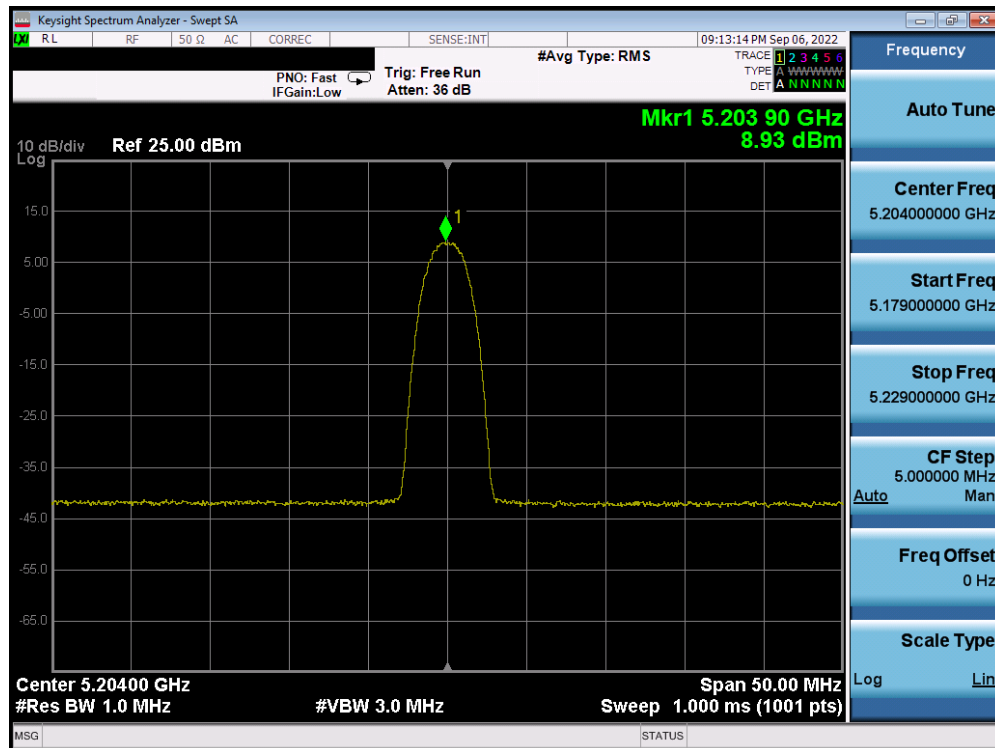
Plot 7-26. PSD Antenna WF5T (HDR4, ePA, 5204MHz)
