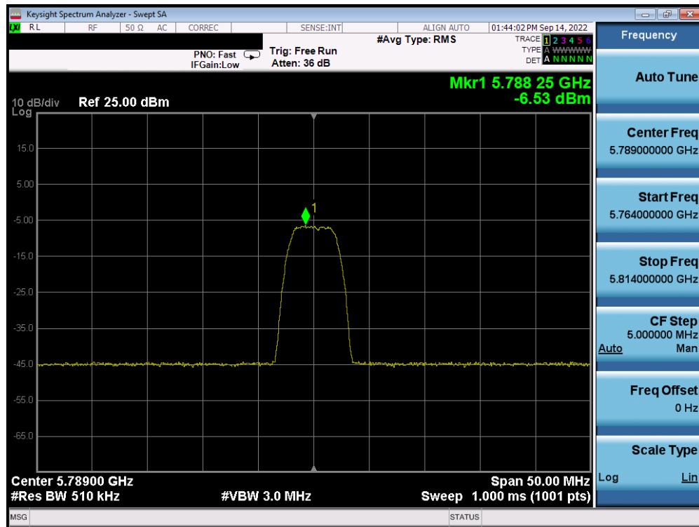
Plot 7-47. PSD Antenna WF5T (HDR8, iPA, 5789MHz)
