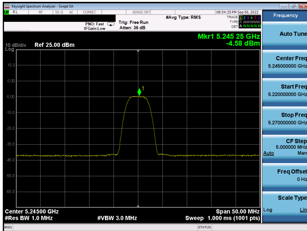
Plot 7-60. PSD Antenna WF5B (HDR8, iPA, 5245MHz)
