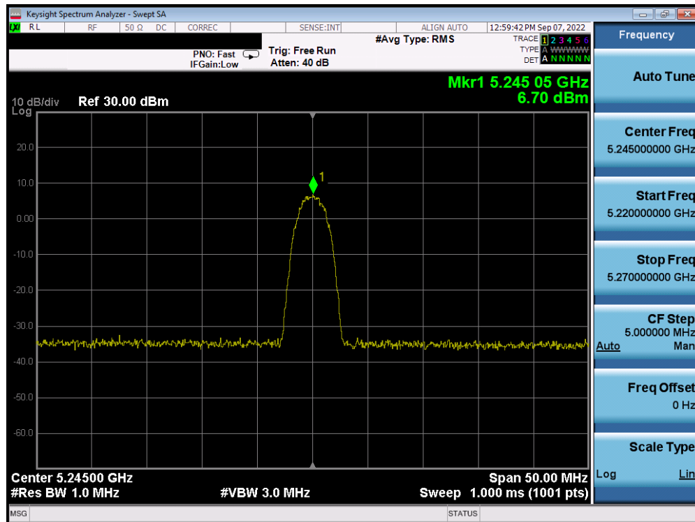
Plot 7-78. PSD TxBF Antenna WF5B (HDR4, ePA, 5245MHz)
