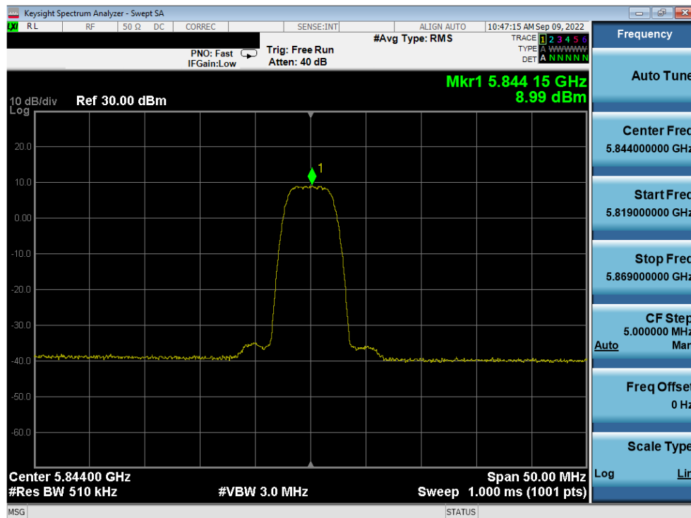
Plot 7-42. PSD Antenna WF5T (HDR8, ePA, 5844MHz)
