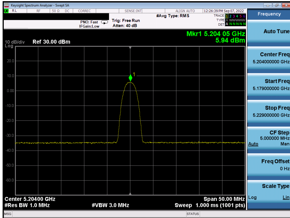
Plot 7-75. PSD TxBF Antenna WF5T (HDR4, ePA, 5204MHz)
