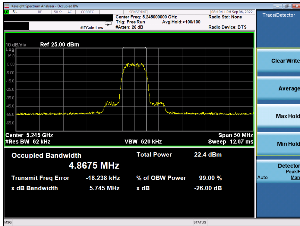
Plot 7-12. 26dB BW & 99% OBW Antenna WF5B (HDR8, ePA, 5245MHz)
