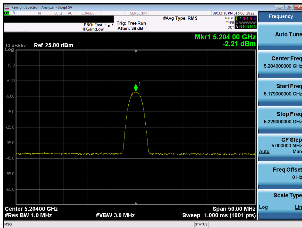
Plot 7-32. PSD Antenna WF5T (HDR4, iPA, 5204MHz)
