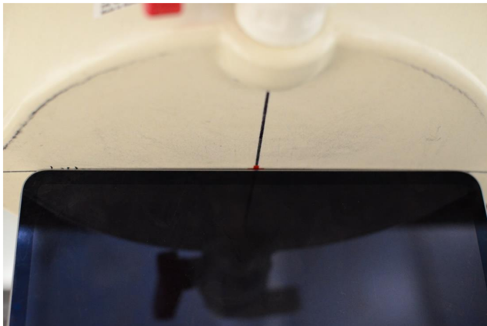
SAR Test Setup Photo 5: Body, Right Edge at 0mm
