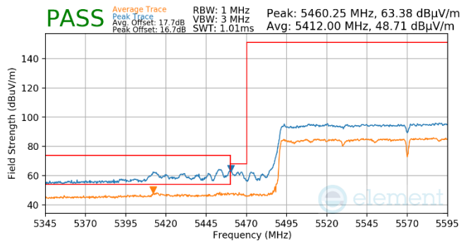
Plot 7-542. (FCC Only) Antenna WF5T (Pk & Avg, RU996x2, Index 68, Ch.114, MCS11)
