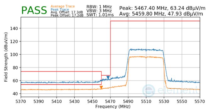
Plot 7-577. Antenna WF5B (Pk & Avg, RU484, Index 65, Ch.102, MCS11)
