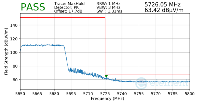
Plot 7-582. Antenna WF5B (Pk, RU484, Index 65, Ch.134, MCS11)
