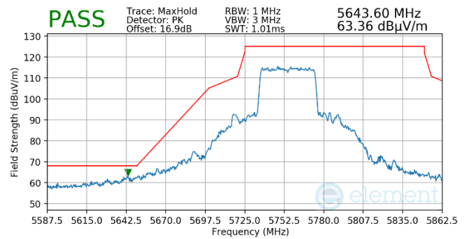
Plot 7-521. Antenna WF5T (Pk, RU484, Index 65, Ch.151, MCS11)
