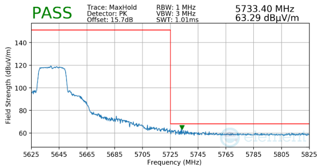
Plot 7-558. (FCC Only) Antenna WF5B (Pk, RU242, Index 61, Ch.128, MCS11)
