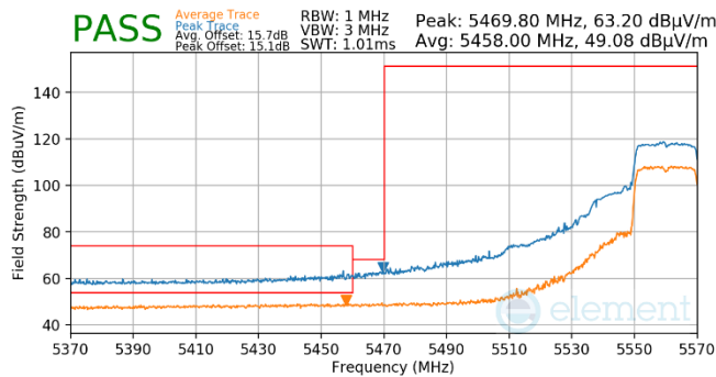
Plot 7-557. Antenna WF5B (Pk & Avg, RU242, Index 61, Ch.112, MCS11)
