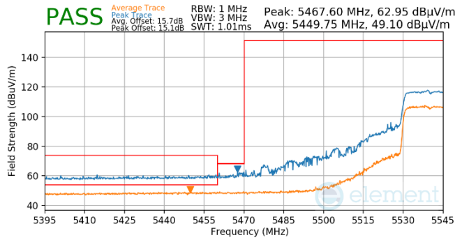
Plot 7-556. Antenna WF5B (Pk & Avg, RU242, Index 61, Ch.108, MCS11)
