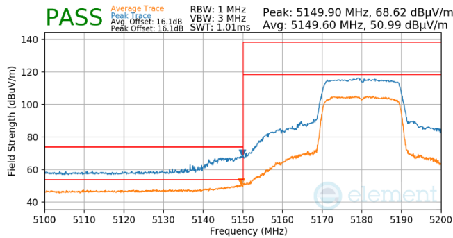
Plot 7-550. Antenna WF5B (Pk & Avg, RU242, Index 61, Ch.36, MCS11)
