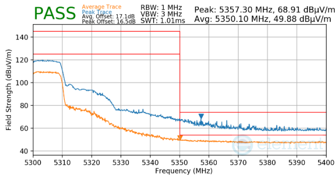
Plot 7-552. Antenna WF5B (Pk & Avg, RU242, Index 61, Ch.60, MCS11)
