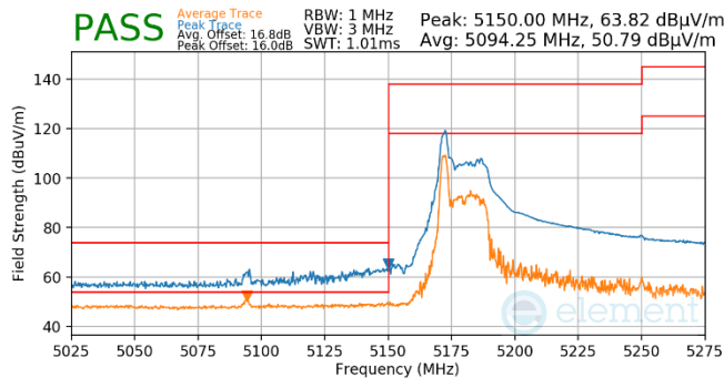
Plot 7-537. Antenna WF5T (Pk & Avg, RU26, Index 0, Ch.50, MCS11)
