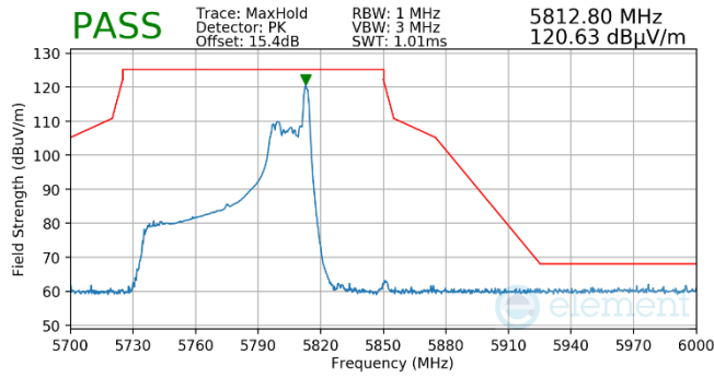
Plot 7-591. Antenna WF5B (Pk, RU26, Index 36, Ch.155, MCS11)
