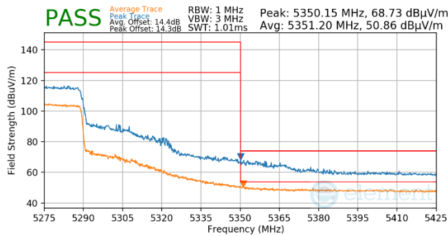
Plot 7-575. Antenna WF5B (Pk & Avg, RU484, Index 65, Ch.54, MCS11)
