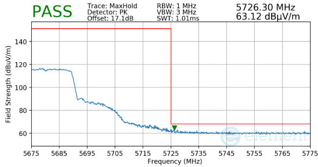
Plot 7-498. Antenna WF5T (Pk, RU242, Index 61, Ch.136, MCS11)
