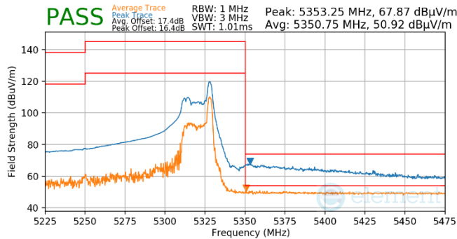
Plot 7-538. Antenna WF5T (Pk & Avg, RU26, Index 36, Ch.50, MCS11)
