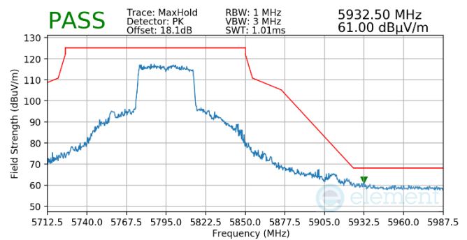
Plot 7-584. Antenna WF5B (Pk, RU484, Index 65, Ch.159, MCS11)
