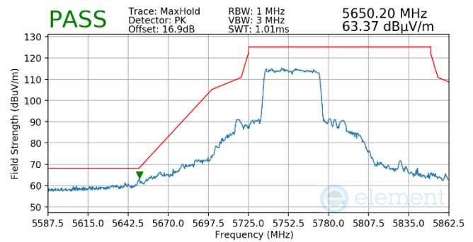
Plot 7-583. Antenna WF5B (Pk, RU484, Index 65, Ch.151, MCS11)
