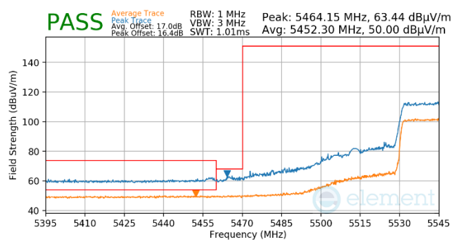
Plot 7-578. Antenna WF5B (Pk & Avg, RU484, Index 65, Ch.110, MCS11)
