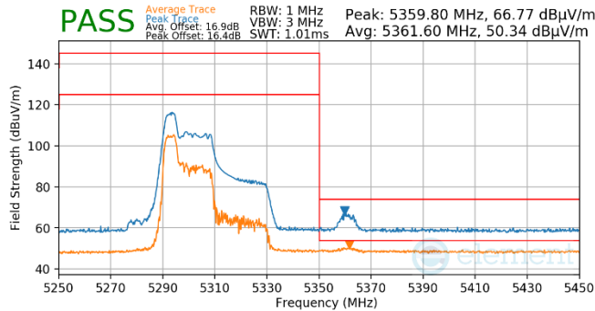
Plot 7-504. Antenna WF5T (Pk & Avg, RU52, Index 37, Ch.62, MCS11)
