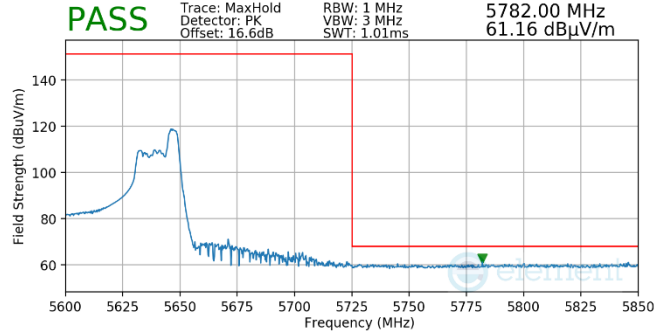
Plot 7-589. (FCC Only) Antenna WF5B (Pk, RU52, Index 52, Ch.122, MCS11)
