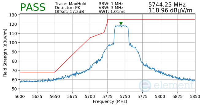
Plot 7-562. Antenna WF5B (Pk, RU242, Index 61, Ch.149, MCS11)
