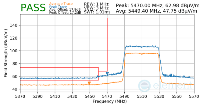
Plot 7-515. Antenna WF5T (Pk & Avg, RU484, Index 65, Ch.102, MCS11)
