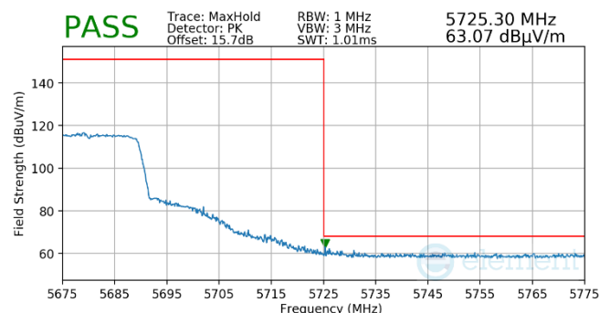
Plot 7-560. Antenna WF5B (Pk, RU242, Index 61, Ch.136, MCS11)
