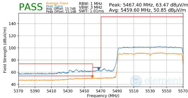
Plot 7-532. Antenna WF5T (Pk & Avg, RU996, Index 67, Ch.106, MCS11)
