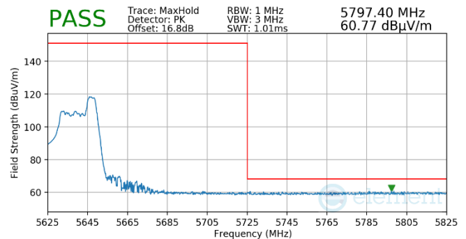
Plot 7-507. (FCC Only) Antenna WF5T (Pk, RU52, Index 44, Ch.126, MCS11)
