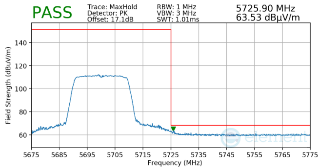
Plot 7-499. Antenna WF5T (Pk, RU242, Index 61, Ch.140, MCS11)
