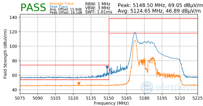
Plot 7-502. Antenna WF5T (Pk & Avg, RU26, Index 0, Ch.38, MCS11)
