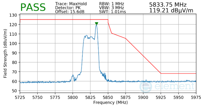
Plot 7-549. Antenna WF5B (Pk, RU26, Index 8, Ch.165, MCS11)
