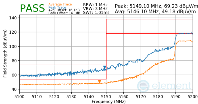
Plot 7-551. Antenna WF5B (Pk & Avg, RU242, Index 61, Ch.40, MCS11)
