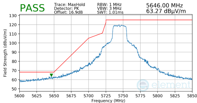
Plot 7-500. Antenna WF5T (Pk, RU242, Index 61, Ch.149, MCS11)
