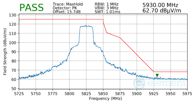
Plot 7-563. Antenna WF5B (Pk, RU242, Index 61, Ch.165, MCS11)
