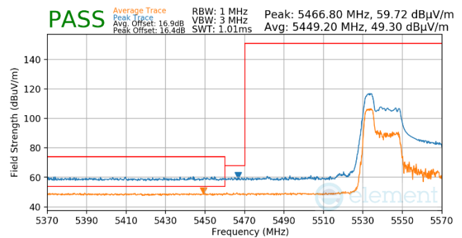
Plot 7-506. Antenna WF5T (Pk & Avg, RU52, Index 37, Ch.110, MCS11)
