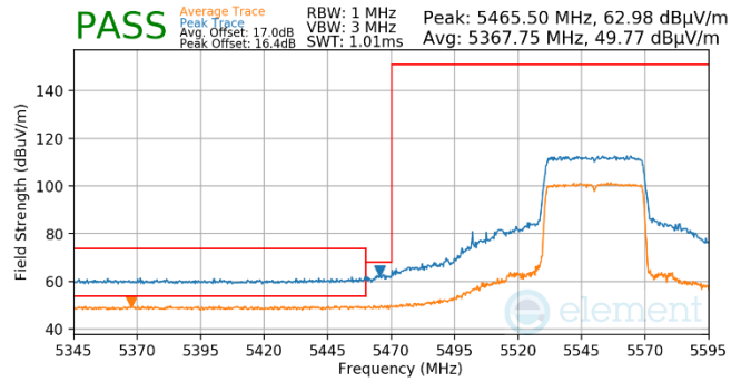
Plot 7-516. Antenna WF5T (Pk & Avg, RU484, Index 65, Ch.110, MCS11)
