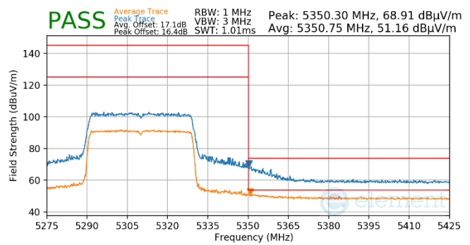
Plot 7-576. Antenna WF5B (Pk & Avg, RU484, Index 65, Ch.62, MCS11)
