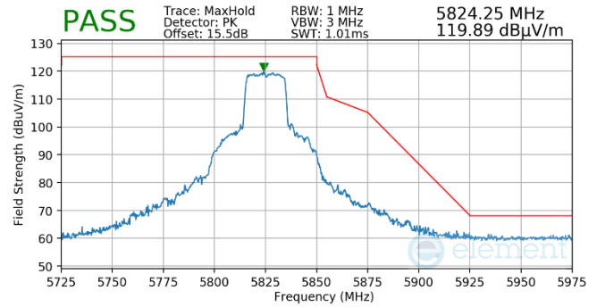
Plot 7-501. Antenna WF5T (Pk, RU242, Index 61, Ch.165, MCS11)
