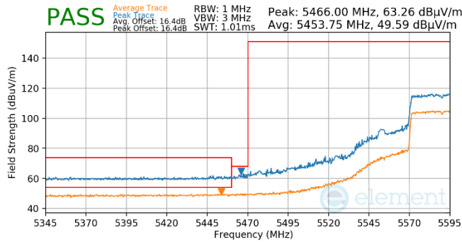
Plot 7-579. (FCC Only) Antenna WF5B (Pk & Avg, RU484, Index 65, Ch.118, MCS11)
