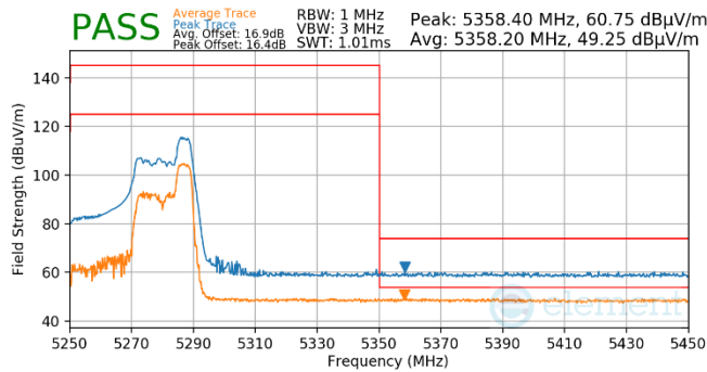
Plot 7-503. Antenna WF5T (Pk & Avg, RU52, Index 44, Ch.54, MCS11)
