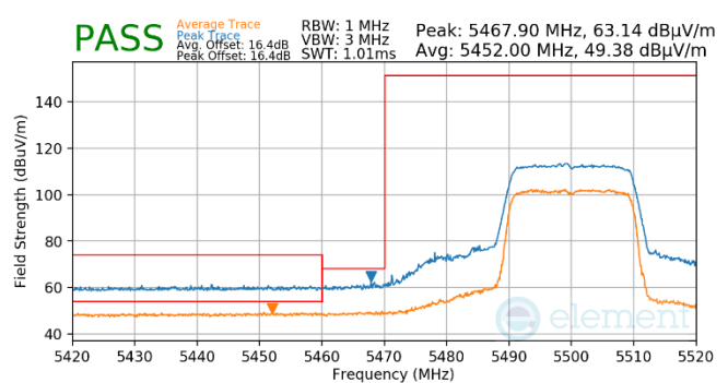
Plot 7-554. Antenna WF5B (Pk & Avg, RU242, Index 61, Ch.100, MCS11)
