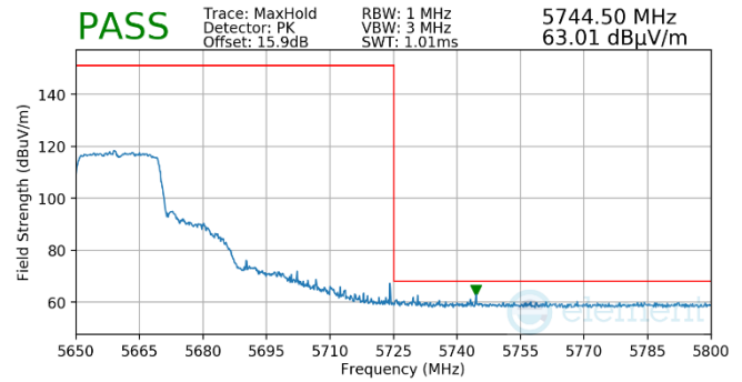
Plot 7-559. Antenna WF5B (Pk, RU242, Index 61, Ch.132, MCS11)
