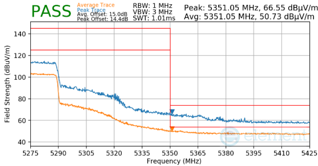
Plot 7-513. Antenna WF5T (Pk & Avg, RU484, Index 65, Ch.54, MCS11)
