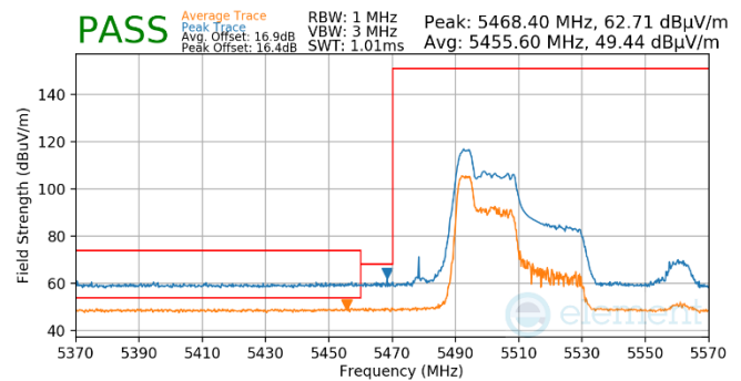
Plot 7-505. Antenna WF5T (Pk & Avg, RU52, Index 37, Ch.102, MCS11)
