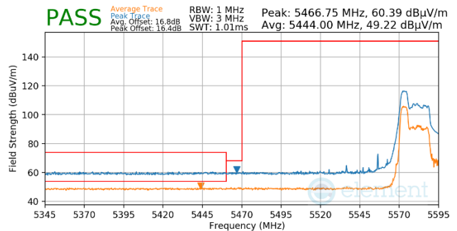
Plot 7-588. (FCC Only) Antenna WF5B (Pk & Avg, RU52, Index 37, Ch.122, MCS11)
