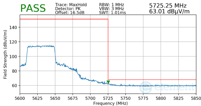
Plot 7-519. (FCC Only) Antenna WF5T (Pk, RU484, Index 65, Ch.126, MCS11)
