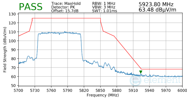
Plot 7-536. Antenna WF5T (Pk, RU996, Index 67, Ch.155, MCS11)
