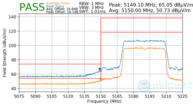
Plot 7-511. Antenna WF5T (Pk & Avg, RU484, Index 65, Ch.38, MCS11)
