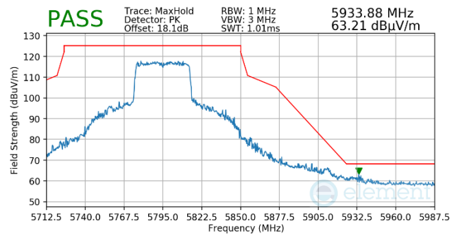
Plot 7-522. Antenna WF5T (Pk, RU484, Index 65, Ch.159, MCS11)
