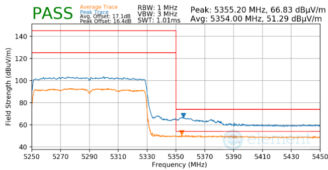
Plot 7-531. Antenna WF5T (Pk & Avg, RU996, Index 67, Ch.58, MCS11)
