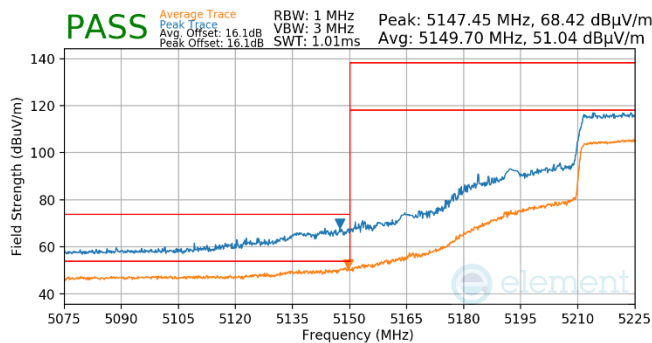
Plot 7-574. Antenna WF5B (Pk & Avg, RU484, Index 65, Ch.46, MCS11)
