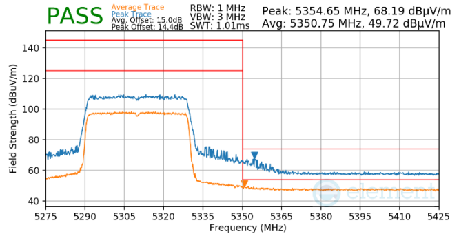
Plot 7-514. Antenna WF5T (Pk & Avg, RU484, Index 65, Ch.62, MCS11)
