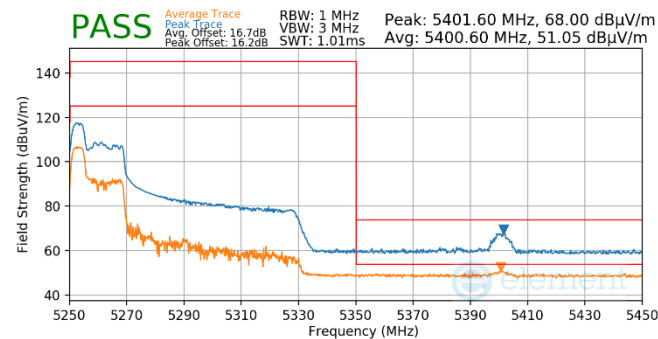
Plot 7-586. Antenna WF5B (Pk & Avg, RU52, Index 37, Ch.58, MCS11)
