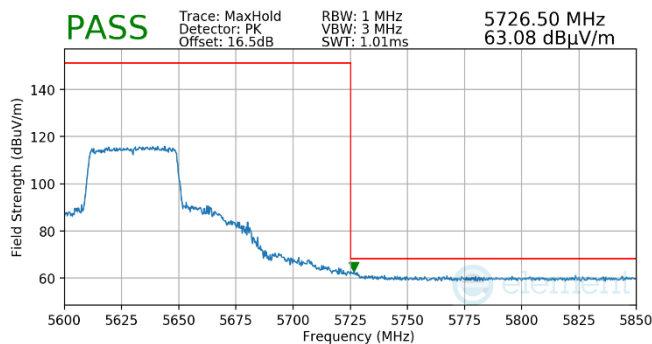
Plot 7-581. (FCC Only) Antenna WF5B (Pk, RU484, Index 65, Ch.126, MCS11)
