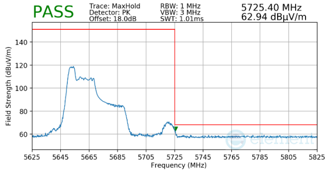
Plot 7-570. Antenna WF5B (Pk, RU52, Index 37, Ch.134, MCS11)
