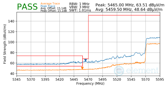
Plot 7-533. (FCC Only) Antenna WF5T (Pk & Avg, RU996, Index 67, Ch.122, MCS11)
