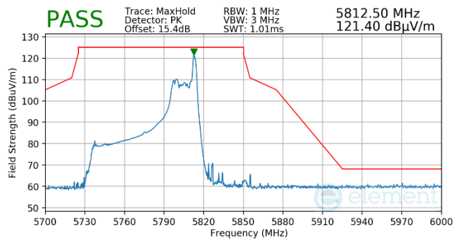
Plot 7-529. Antenna WF5T (Pk, RU26, Index 36, Ch.155, MCS11)
