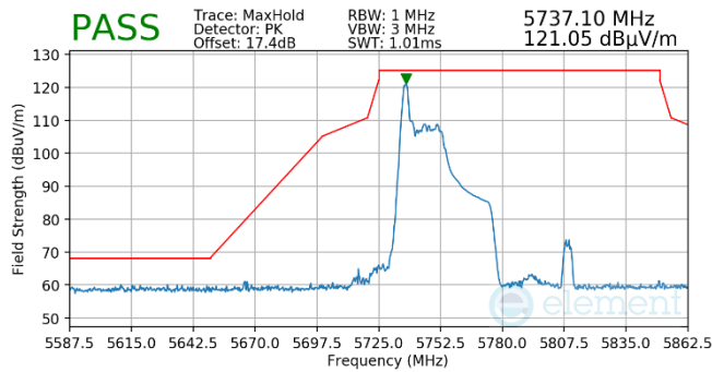
Plot 7-571. Antenna WF5B (Pk, RU26, Index 0, Ch.151, MCS11)
