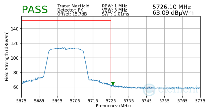
Plot 7-561. Antenna WF5B (Pk, RU242, Index 61, Ch.140, MCS11)
