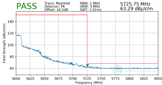
Plot 7-580. (FCC Only) Antenna WF5B (Pk, RU484, Index 65, Ch.118, MCS11)
