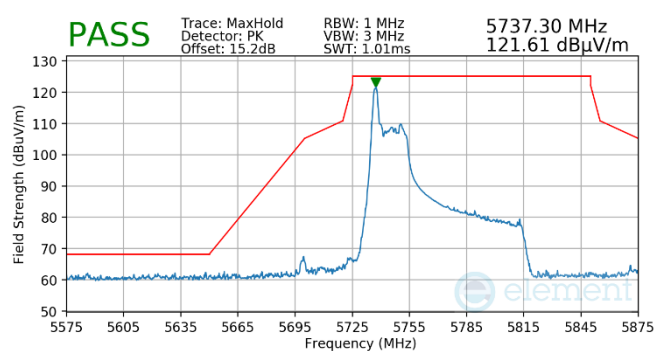
Plot 7-590. Antenna WF5B (Pk, RU26, Index 0, Ch.155, MCS11)
