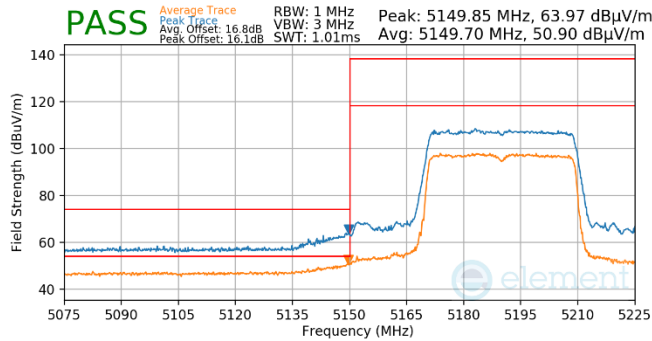
Plot 7-573. Antenna WF5B (Pk & Avg, RU484, Index 65, Ch.38, MCS11)
