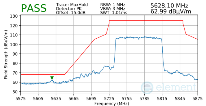
Plot 7-535. Antenna WF5T (Pk, RU996, Index 67, Ch.155, MCS11)
