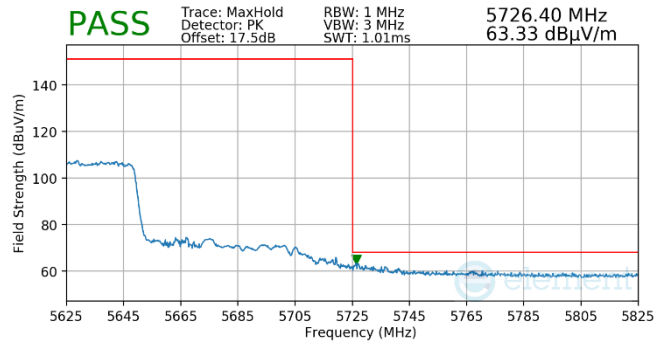
Plot 7-534. (FCC Only) Antenna WF5T (Pk, RU996, Index 67, Ch.122, MCS11)
