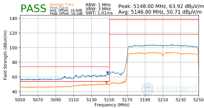
Plot 7-530. Antenna WF5T (Pk & Avg, RU996, Index 67, Ch.42, MCS11)
