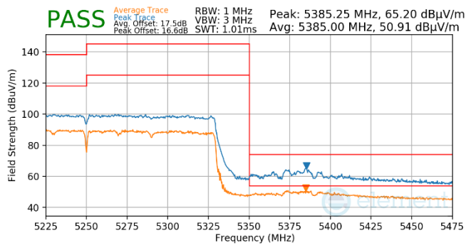
Plot 7-541. Antenna WF5T (Pk & Avg, RU996x2, Index 68, Ch.50, MCS11)
