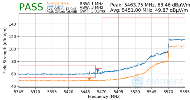
Plot 7-517. (FCC Only) Antenna WF5T (Pk & Avg, RU484, Index 65, Ch.118, MCS11)
