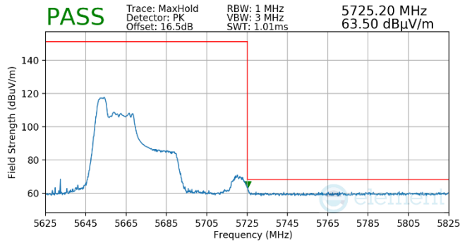
Plot 7-508. Antenna WF5T (Pk, RU52, Index 37, Ch.134, MCS11)
