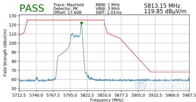
Plot 7-510. Antenna WF5T (Pk, RU26, Index 17, Ch.159, MCS11)
