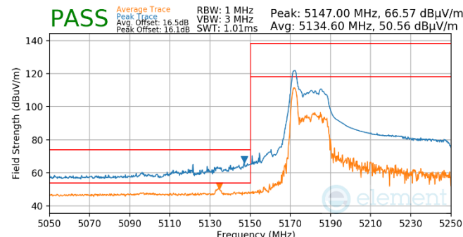
Plot 7-585. Antenna WF5B (Pk & Avg, RU26, Index 0, Ch.42, MCS11)
