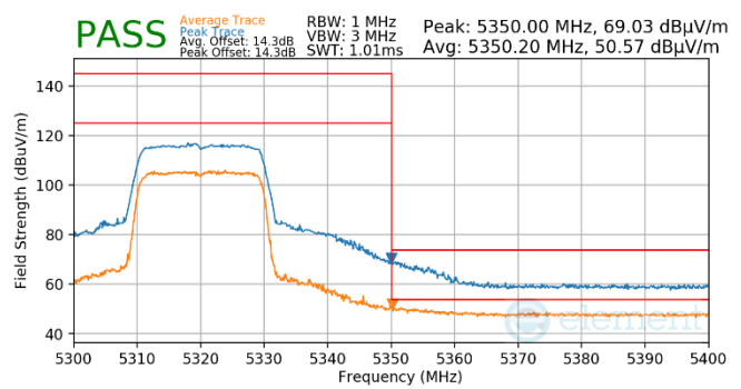
Plot 7-553. Antenna WF5B (Pk & Avg, RU242, Index 61, Ch.64, MCS11)
