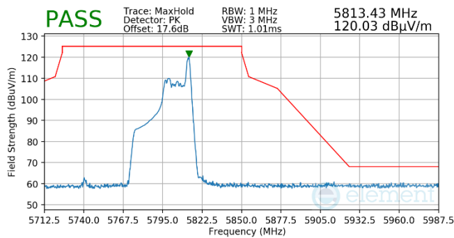
Plot 7-572. Antenna WF5B (Pk, RU26, Index 17, Ch.159, MCS11)
