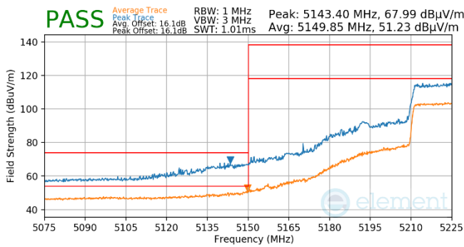
Plot 7-512. Antenna WF5T (Pk & Avg, RU484, Index 65, Ch.46, MCS11)
