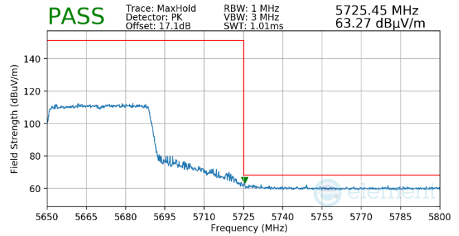
Plot 7-520. Antenna WF5T (Pk, RU484, Index 65, Ch.134, MCS11)
