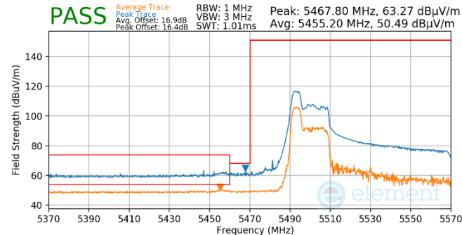
Plot 7-587. Antenna WF5B (Pk & Avg, RU52, Index 37, Ch.106, MCS11)
