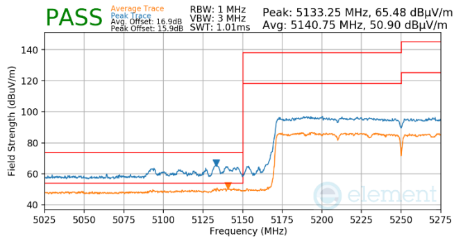
Plot 7-540. Antenna WF5T (Pk & Avg, RU996x2, Index 68, Ch.50, MCS11)
