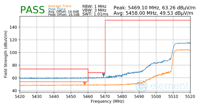
Plot 7-555. Antenna WF5B (Pk & Avg, RU242, Index 61, Ch.104, MCS11)
