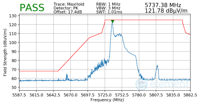
Plot 7-509. Antenna WF5T (Pk, RU26, Index 0, Ch.151, MCS11)
