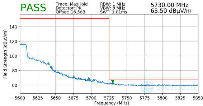
Plot 7-518. (FCC Only) Antenna WF5T (Pk, RU484, Index 65, Ch.118, MCS11)
