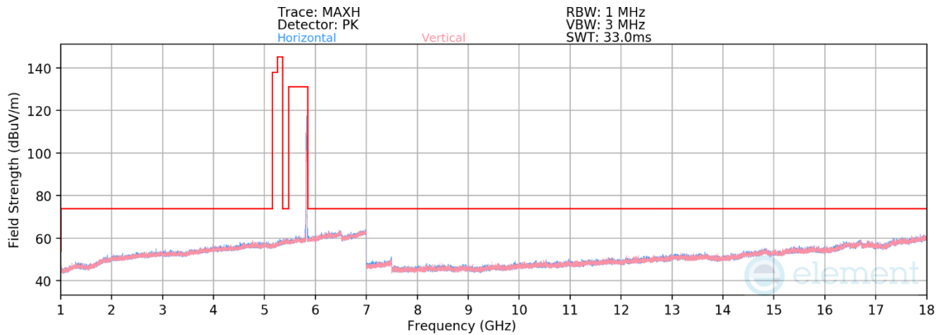
Plot 7-432. RSE above 1GHz Antenna WF5B (11ax – Ch.165 – RU26)
