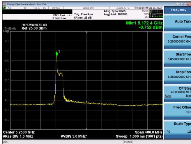
Plot 7-392. ISED PSD Antenna WF5B (20MHz BW 11ax Index 0 - RU26 - Ch.50(L))
