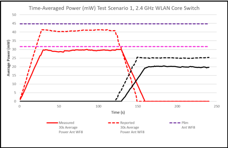
Figure G-2 30s Average Power vs. Time, 2.4 GHz
