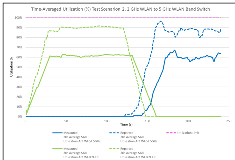
Figure G-5 30s Average Utilization vs. Time during Band Switch
