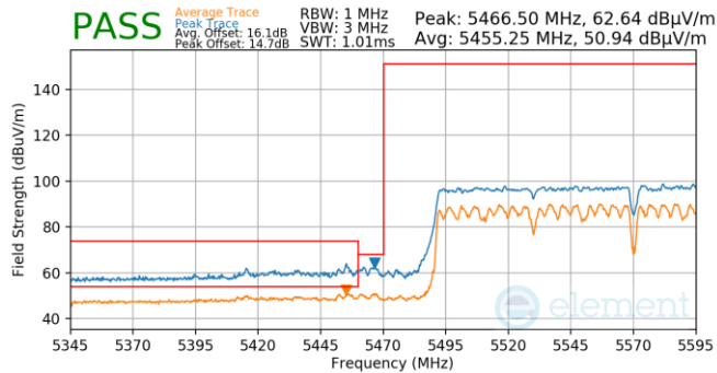
Plot 7-1262. (FCC Only) CDD (Pk & Avg, Ch.114, 802.ac, MCS9)
