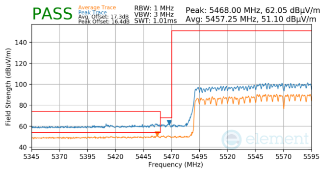
CDD Plot 7-1270. (FCC Only) CDD (Pk & Avg, Ch.114, 802. ax(SU), MCS4)
