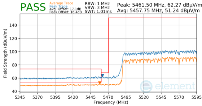
Plot 7-1269. (FCC Only) CDD (Pk & Avg, Ch.114, 802.11 ax(SU), MCS2)
