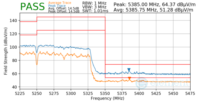
Plot 7-1258. CDD (Pk & Avg, Ch.50, 802.ac, MCS4)
