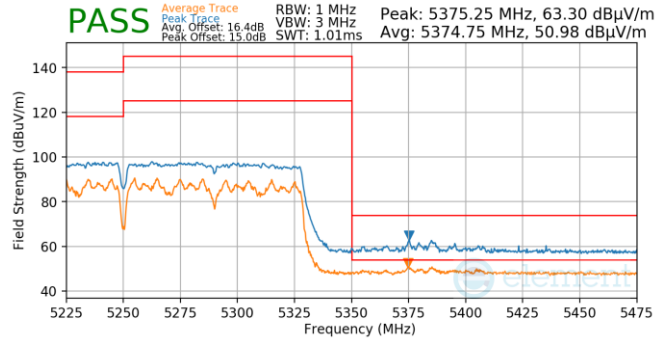
Plot 7-1259. CDD (Pk & Avg, Ch.50, 802.ac, MCS9)
