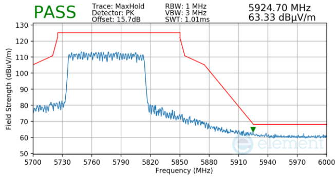
Plot 7-1251. CDD (Pk, Ch.155, 802.11ax(SU), MCS2)
