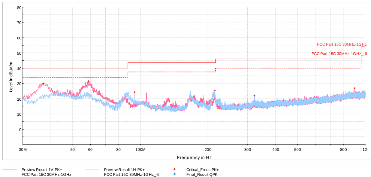
Plot 7-1272. Radiated Spurious Emissions below 1GHz CDD, 802.11n, Ch.40 with AC/DC Adapter
