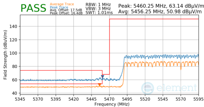
Plot 7-1271. (FCC Only) CDD (Pk & Avg, Ch.114, 802. ax(SU), MCS11)
