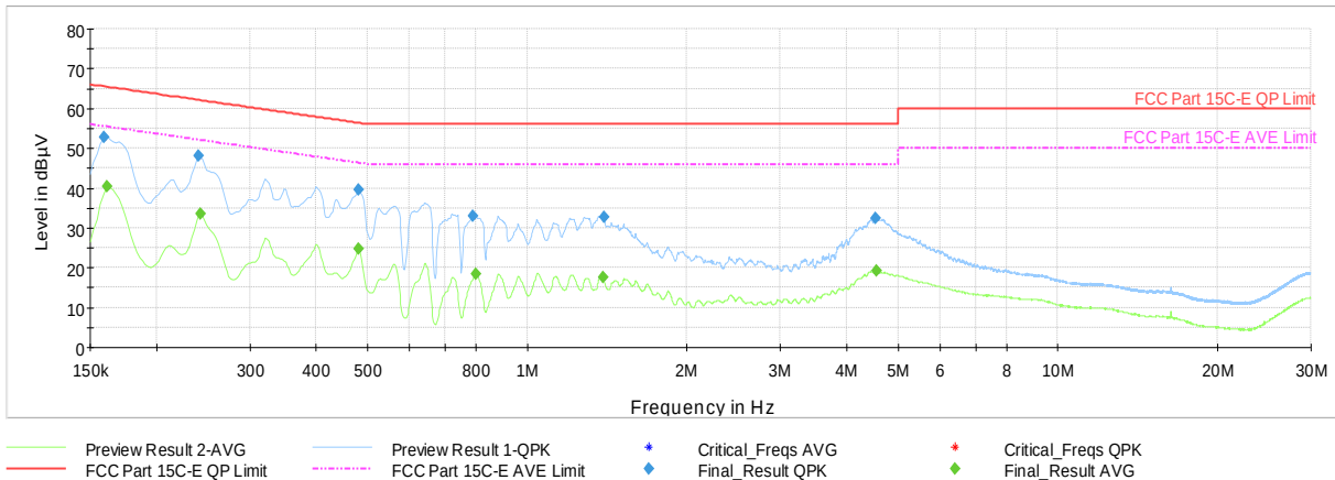
Plot 7-1275. AC Line Conducted Plot with 802.11n CDD- Ch.40 (N), with AC/DC adapter
