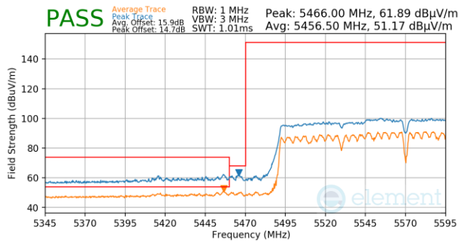
Plot 7-1261. (FCC Only) CDD (Pk & Avg, Ch.114, 802.ac, MCS4)
