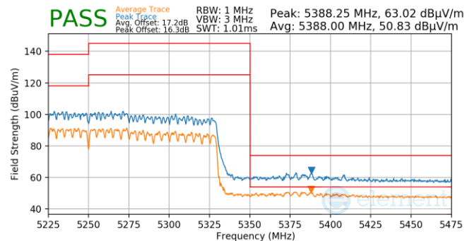
Plot 7-1267. CDD (Pk & Avg, Ch.50, 802. ax(SU), MCS4)
