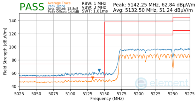
Plot 7-1256. CDD (Pk & Avg, Ch.50, 802.ac, MCS9)
