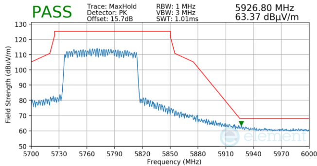
Plot 7-1253. CDD (Pk, Ch.155, 802.11ax(SU), MCS11)
