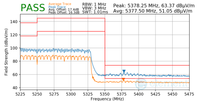
Plot 7-1268. CDD (Pk & Avg, Ch.50, 802. ax(SU), MCS11)
