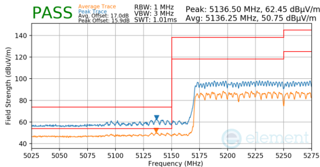
Plot 7-1265. CDD (Pk & Avg, Ch.50, 802. ax(SU), MCS11)
