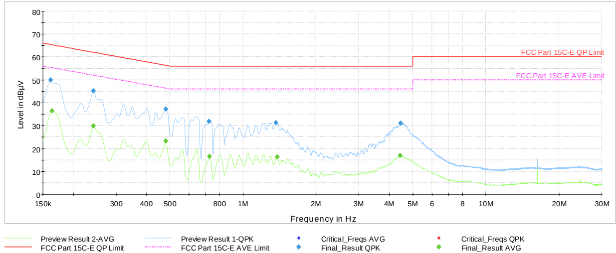
Plot 7-1276. AC Line Conducted Plot with 802.11ax(SU) CDD– Ch.40 (L1), with AC/DC adapter
