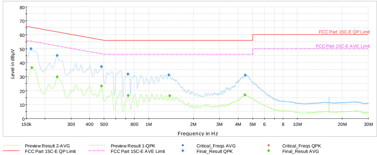
Plot 7-1274. AC Line Conducted Plot with 802.11n CDD- Ch.40 (L1), with AC/DC adapter
