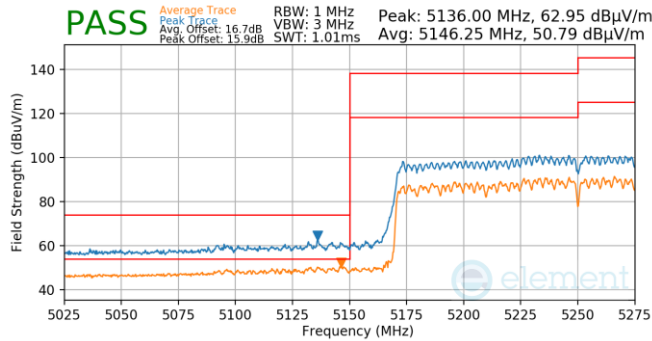
Plot 7-1263. CDD (Pk & Avg, Ch.50, 802.11ax(SU), MCS2)
