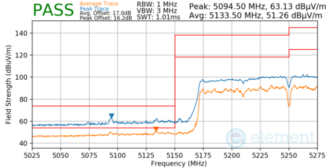
Plot 7-1254. CDD (Pk & Avg, Ch.50, 802.11ac, MCS2)
