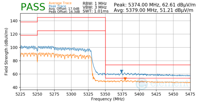
Plot 7-1266. CDD (Pk & Avg, Ch.50, 802.11ax(SU), MCS2)
