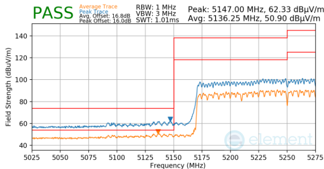
Plot 7-1264. CDD (Pk & Avg, Ch.50, 802. ax(SU), MCS4)
