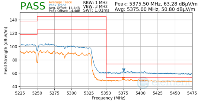
Plot 7-1257. CDD (Pk & Avg, Ch.50, 802.11ac, MCS2)
