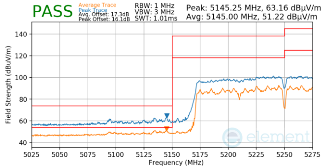
Plot 7-1255. CDD (Pk & Avg, Ch.50, 802.ac, MCS4)
