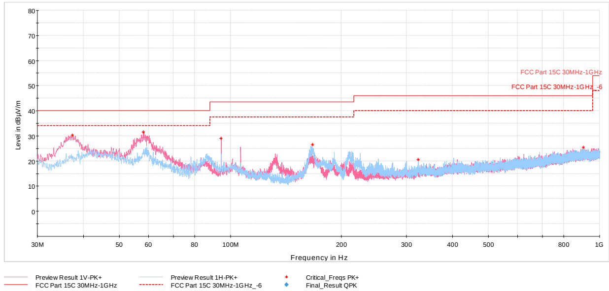
Plot 7-1273. Radiated Spurious Emissions below 1GHz CDD, 802.11ax (SU), Ch.40 with AC/DC Adapter
