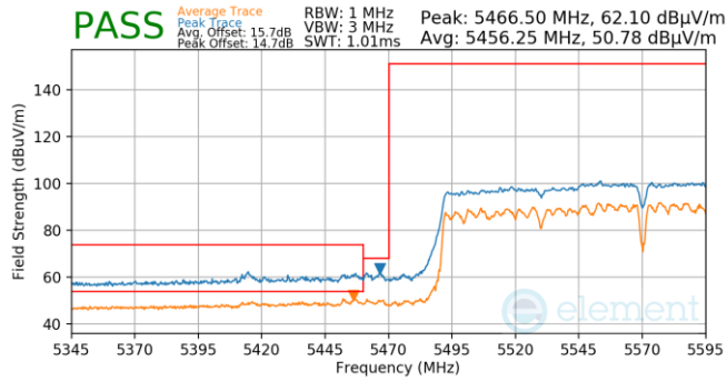
Plot 7-1260. (FCC only) CDD (Pk & Avg, Ch.114, 802.ac, MCS2)
