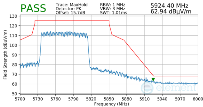
Plot 7-1252. CDD (Pk, Ch.155, 802.11ax(SU), MCS4)
