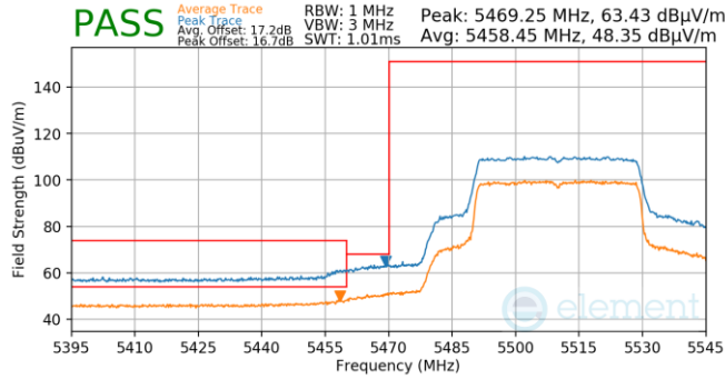
Plot 7-1001. Antenna WF5B (Pk & Avg, Ch.102, 802.11ax(SU), MCS2)
