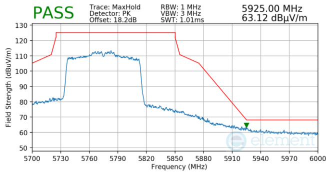
Plot 7-1043. Antenna WF5B (Pk, Ch.155, 802.11ac, MCS2)
