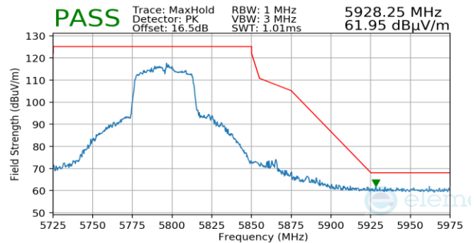
Plot 7-987. Antenna WF5B (Pk, Ch.159, 802.11n, MCS4)
