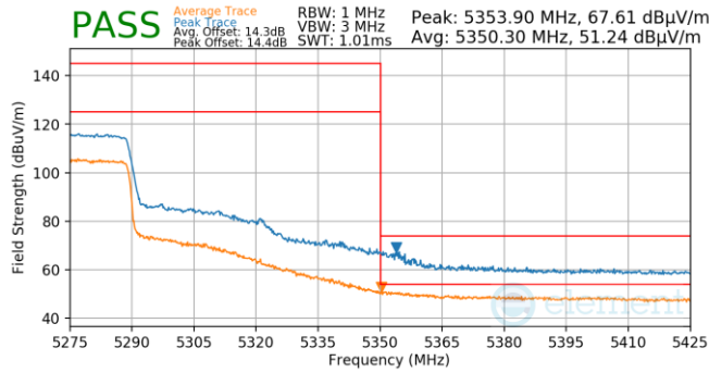
Plot 7-995. Antenna WF5B (Pk & Avg, Ch.54, 802.11ax(SU), MCS2)
