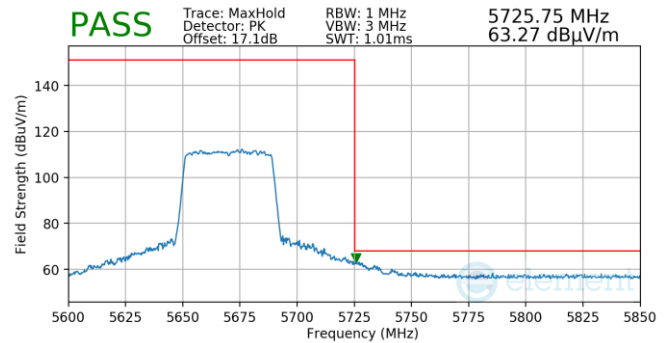
Plot 7-1018. Antenna WF5B (Pk, Ch.134, 802.11ax(SU), MCS11)
