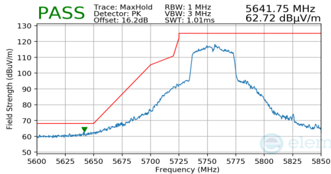
Plot 7-984. Antenna WF5B (Pk, Ch.151, 802.11n, MCS4)
