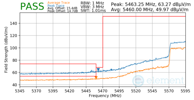
Plot 7-1035. (FCC Only) Antenna WF5B (Pk & Avg, Ch.122, 802.11ac, MCS4)
