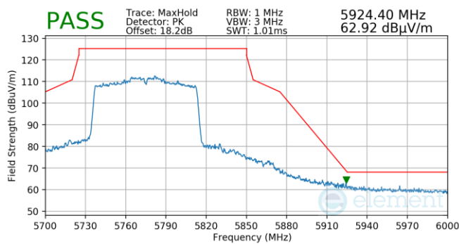
Plot 7-1044. Antenna WF5B (Pk, Ch.155, 802.11ac, MCS4)
