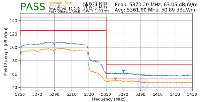
Plot 7-1029. Antenna WF5B (Pk & Avg, Ch.58, 802.11ac, MCS4)
