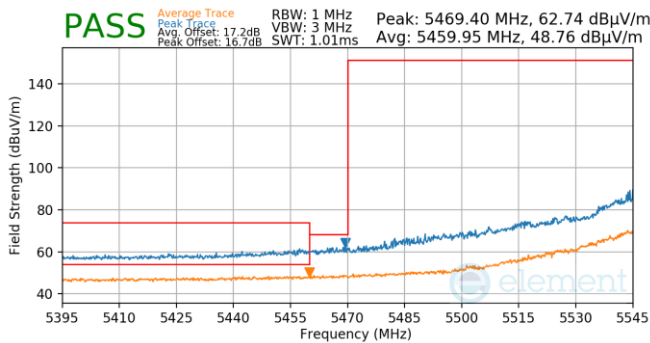
Plot 7-1008. (FCC Only) Antenna WF5B (Pk & Avg, Ch.118, 802.11ax(SU), MCS4)
