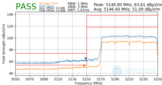
Plot 7-1027. Antenna WF5B (Pk & Avg, Ch.42, 802.11ac, MCS9)
