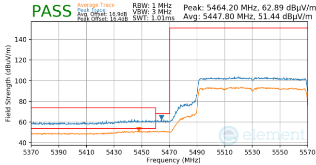
Plot 7-1052. Antenna WF5B (Pk & Avg, Ch.106, 802.11ax(SU), MCS2)
