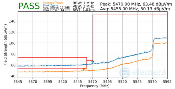
Plot 7-1034. (FCC Only) Antenna WF5B (Pk & Avg, Ch.122, 802.11ac, MCS2)
