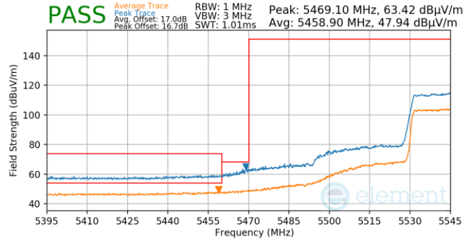
Plot 7-1004. Antenna WF5B (Pk & Avg, Ch.110, 802.11ax(SU), MCS2)
