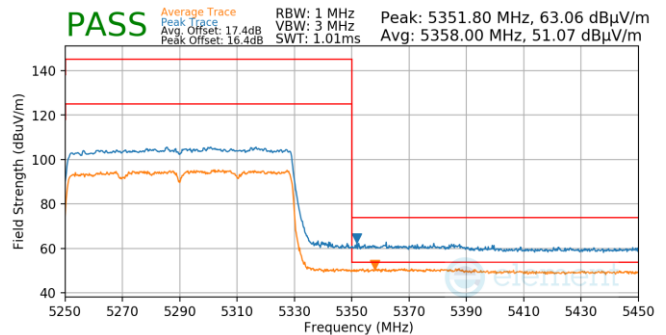
Plot 7-1051. Antenna WF5B (Pk & Avg, Ch.58, 802.11ax(SU), MCS11)
