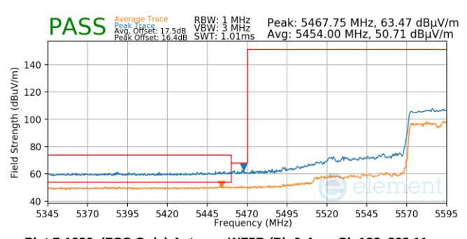
Plot 7-1036. (FCC Only) Antenna WF5B (Pk & Avg, Ch.122, 802.11ac, MCS9)
