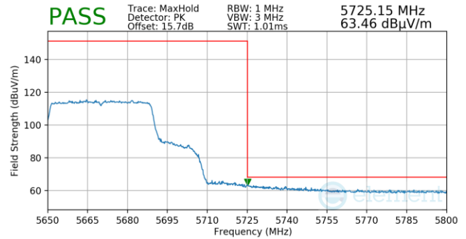
Plot 7-1016. Antenna WF5B (Pk, Ch.134, 802.11ax(SU), MCS2)
