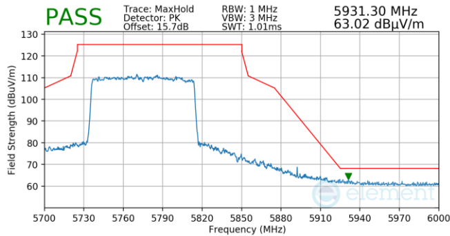
Plot 7-1066. Antenna WF5B (Pk, Ch.155, 802.11ax(SU), MCS11)
