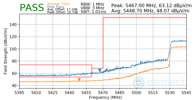
Plot 7-1005. Antenna WF5B (Pk & Avg, Ch.110, 802.11ax(SU), MCS4)
