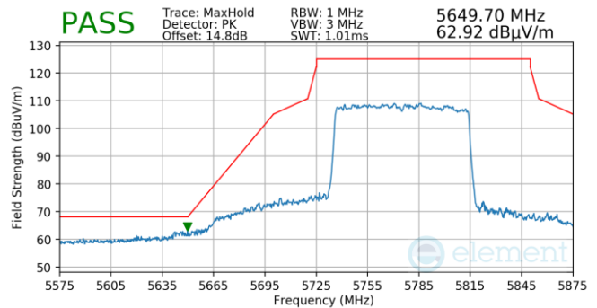
Plot 7-1063. Antenna WF5B (Pk, Ch.155, 802.11ax(SU), MCS11)
