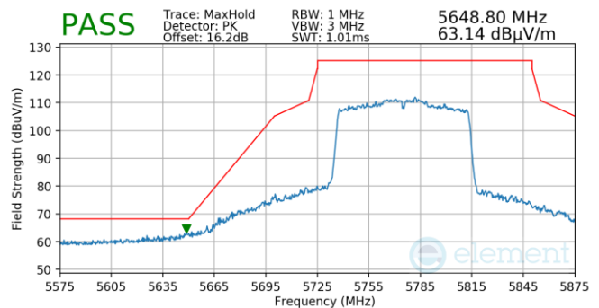
Plot 7-1041. Antenna WF5B (Pk, Ch.155, 802.11ac, MCS4)
