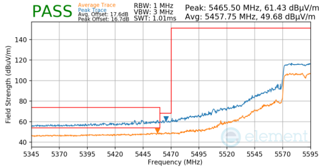
Plot 7-976. (FCC Only) Antenna WF5B (Pk, Ch.118, 802.11n, MCS7)
