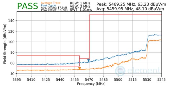
Plot 7-1006. Antenna WF5B (Pk & Avg, Ch.110, 802.11ax(SU), MCS11)
