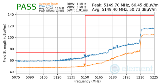
Plot 7-993. Antenna WF5B (Pk & Avg, Ch.46, 802.11ax(SU), MCS4)
