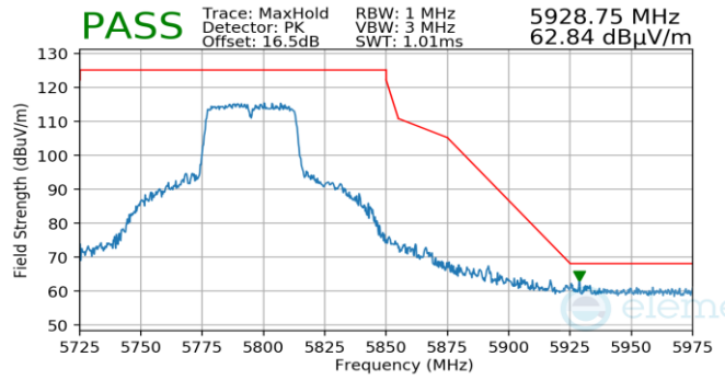
Plot 7-988. Antenna WF5B (Pk, Ch.159, 802.11n, MCS7)
