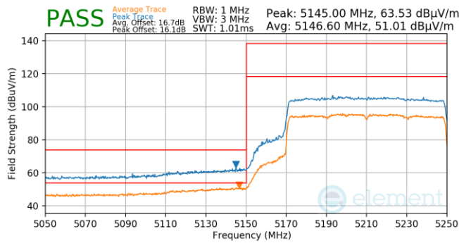
Plot 7-1046. Antenna WF5B (Pk & Avg, Ch.42, 802.11ax(SU), MCS2)
