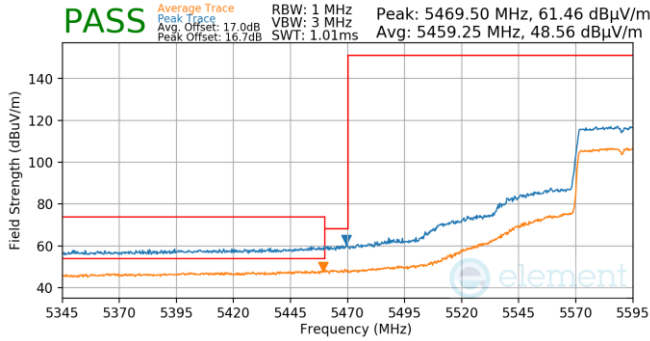
Plot 7-1007. (FCC Only) Antenna WF5B (Pk & Avg, Ch.118, 802.11ax(SU), MCS2)
