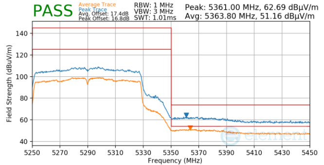
Plot 7-1028. Antenna WF5B (Pk & Avg, Ch.58, 802.11ac, MCS2)
