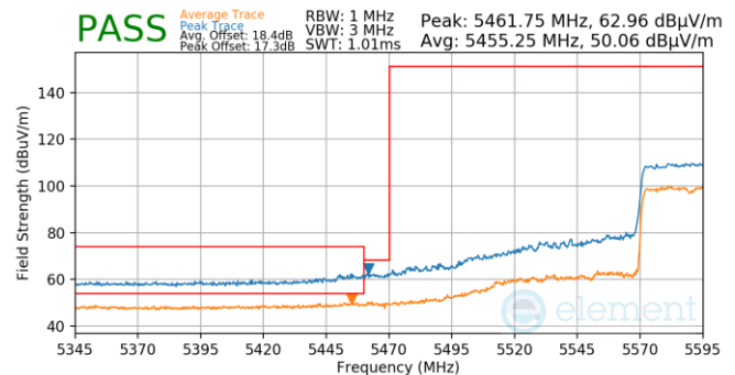
Plot 7-1057. (FCC Only) Antenna WF5B (Pk & Avg, Ch.122, 802.11ax(SU), MCS11)
