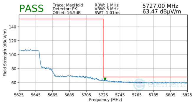
Plot 7-1059. (FCC Only) Antenna WF5B (Pk, Ch.122, 802.11ax(SU), MCS4)
