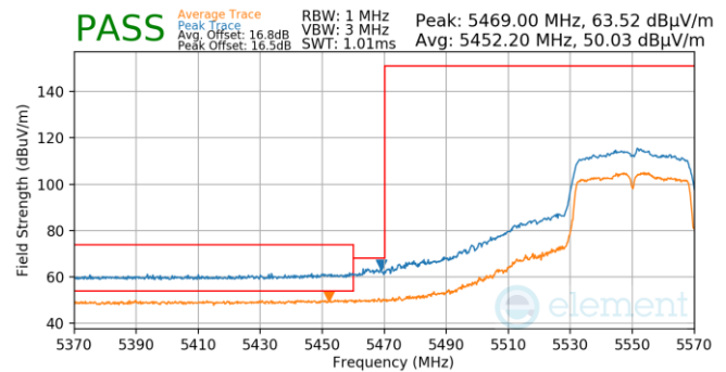
Plot 7-974. Antenna WF5B (Pk & Avg, Ch.110, 802.11n, MCS4)
