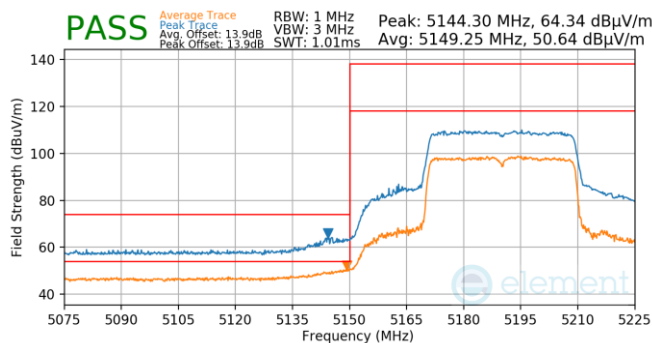
Plot 7-990. Antenna WF5B (Pk & Avg, Ch.38, 802.11ax(SU), MCS4)
