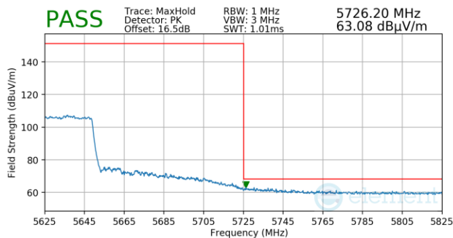
Plot 7-1060. (FCC Only) Antenna WF5B (Pk, Ch.122, 802.11ax(SU), MCS11)
