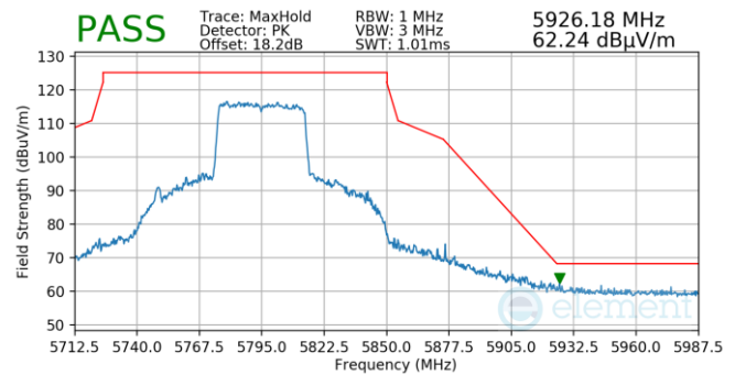
Plot 7-1023. Antenna WF5B (Pk, Ch.159, 802.11ax(SU), MCS4)
