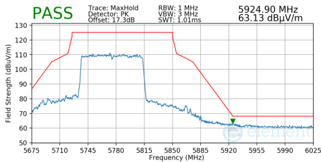
Plot 7-1045. Antenna WF5B (Pk, Ch.155, 802.11ac, MCS9)
