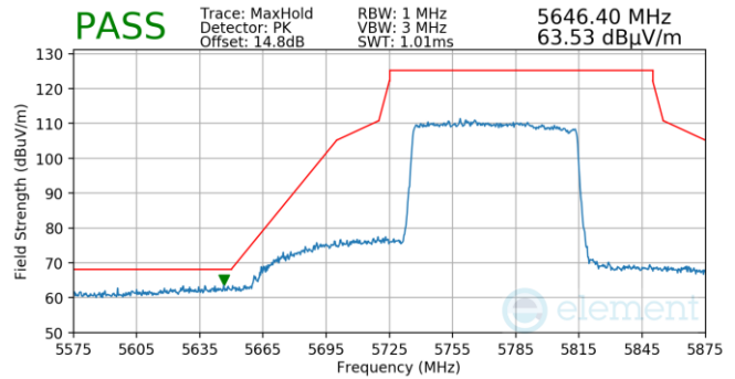
Plot 7-1061. Antenna WF5B (Pk, Ch.155, 802.11ax(SU), MCS2)
