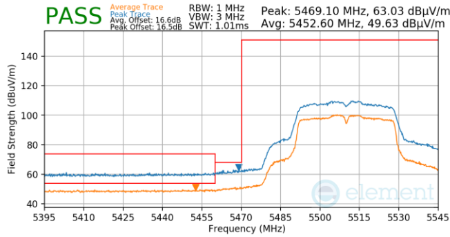
Plot 7-970. Antenna WF5B (Pk & Avg, Ch.102, 802.11n, MCS2)
