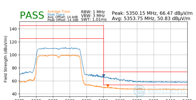
Plot 7-1000. Antenna WF5B (Pk & Avg, Ch.62, 802.11ax(SU), MCS11)
