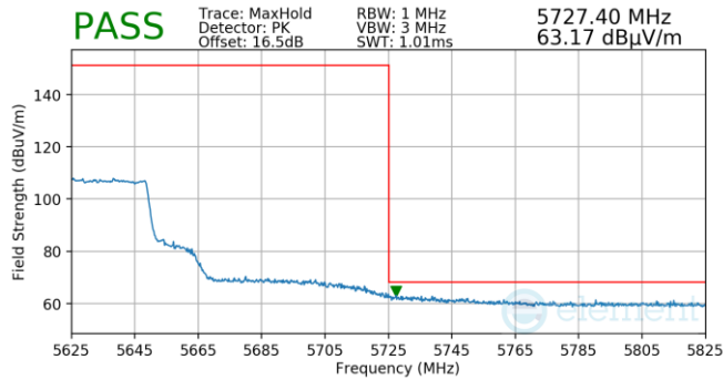
Plot 7-1058. (FCC Only) Antenna WF5B (Pk, Ch.122, 802.11ax(SU), MCS2)
