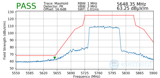
Plot 7-1042. Antenna WF5B (Pk, Ch.155, 802.11ac, MCS9)
