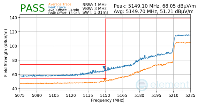
Plot 7-994. Antenna WF5B (Pk & Avg, Ch.46, 802.11ax(SU), MCS11)
