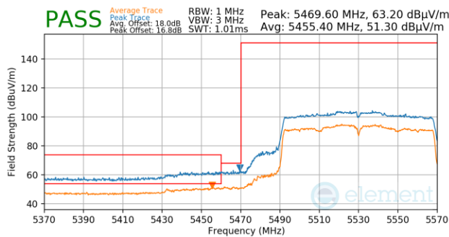
Plot 7-1032. Antenna WF5B (Pk & Avg, Ch.106, 802.11ac, MCS4)
