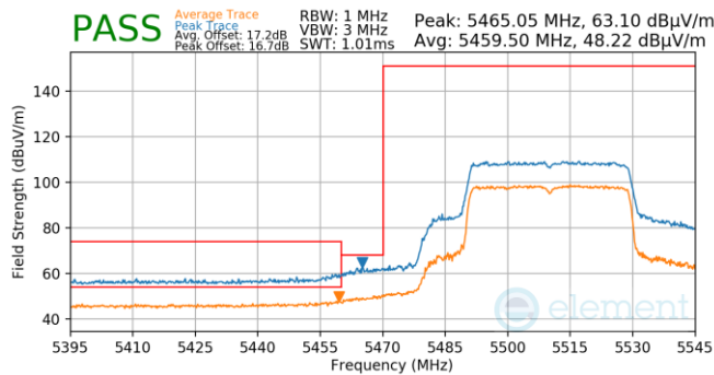
Plot 7-1002. Antenna WF5B (Pk & Avg, Ch.102, 802.11ax(SU), MCS4)
