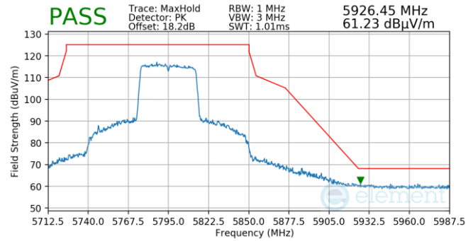
Plot 7-1022. Antenna WF5B (Pk, Ch.159, 802.11ax(SU), MCS2)
