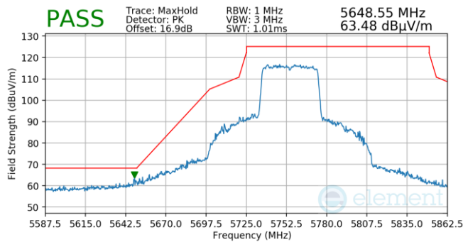
Plot 7-1020. Antenna WF5B (Pk, Ch.151, 802.11ax(SU), MCS4)
