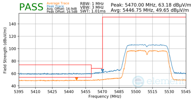
Plot 7-972. Antenna WF5B (Pk & Avg, Ch.102, 802.11n, MCS7)
