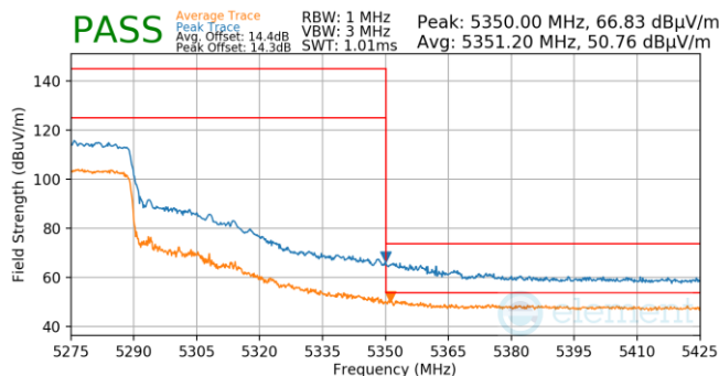
Plot 7-997. Antenna WF5B (Pk & Avg, Ch.54, 802.11ax(SU), MCS11)
