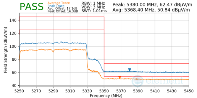
Plot 7-1050. Antenna WF5B (Pk & Avg, Ch.58, 802.11ax(SU), MCS4)
