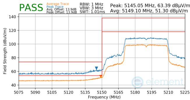
Plot 7-989. Antenna WF5B (Pk & Avg, Ch.38, 802.11ax(SU), MCS2)
