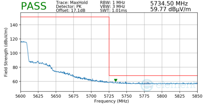
Plot 7-1010. (FCC Only) Antenna WF5B (Pk, Ch.118, 802.11ax(SU), MCS2)
