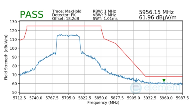
Plot 7-1024. Antenna WF5B (Pk, Ch.159, 802.11ax(SU), MCS11)
