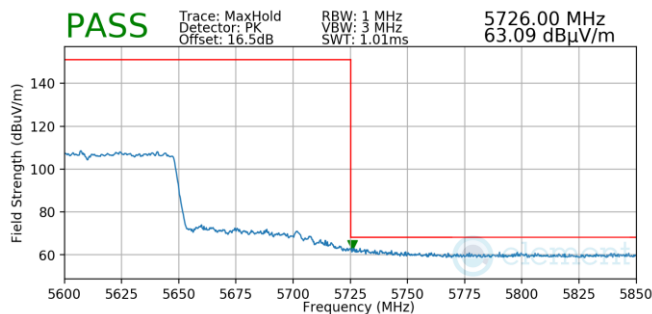
Plot 7-1039. (FCC Only) Antenna WF5B (Pk, Ch.122, 802.11ac, MCS9)
