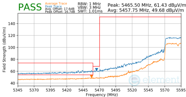
Plot 7-1009. (FCC Only) Antenna WF5B (Pk & Avg, Ch.118, 802.11ax(SU), MCS11)
