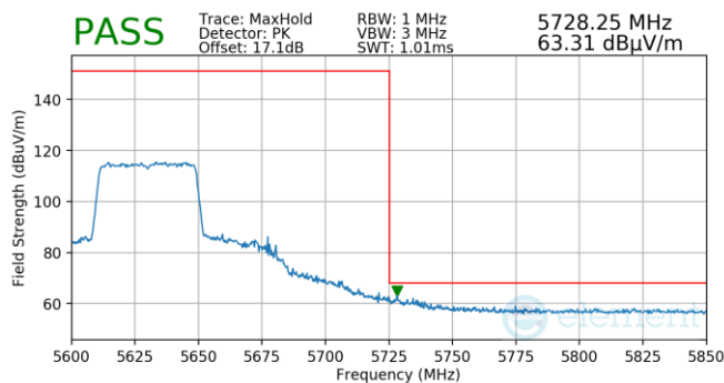
Plot 7-1014. (FCC Only) Antenna WF5B (Pk, Ch.126, 802.11ax(SU), MCS4)
