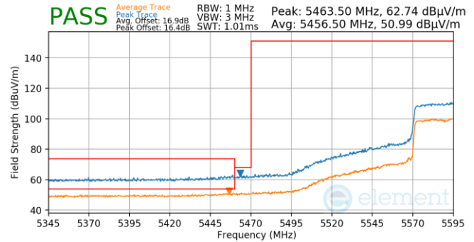
Plot 7-1055. (FCC Only) Antenna WF5B (Pk & Avg, Ch.122, 802.11ax(SU), MCS2)
