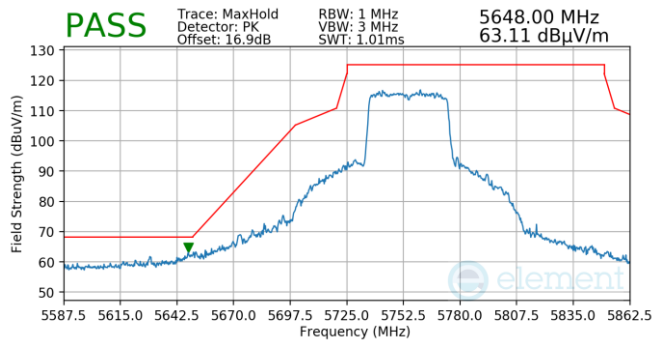
Plot 7-1021. Antenna WF5B (Pk, Ch.151, 802.11ax(SU), MCS11)
