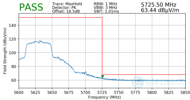
Plot 7-978. (FCC Only) Antenna WF5B (Pk, Ch.126, 802.11n, MCS4)
