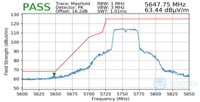
Plot 7-985. Antenna WF5B (Pk, Ch.151, 802.11n, MCS7)
