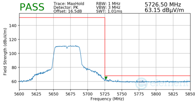
Plot 7-982. Antenna WF5B (Pk, Ch.134, 802.11n, MCS7)
