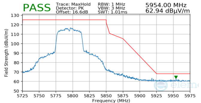
Plot 7-986. Antenna WF5B (Pk, Ch.159, 802.11n, MCS2)
