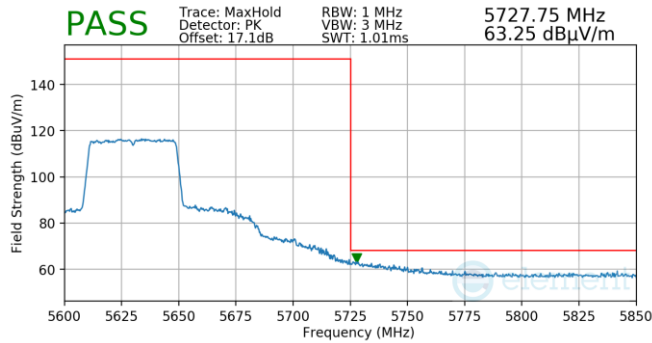
Plot 7-1013. (FCC Only) Antenna WF5B (Pk, Ch.126, 802.11ax(SU), MCS2)
