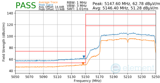
Plot 7-1025. Antenna WF5B (Pk & Avg, Ch.42, 802.11ac, MCS2)
