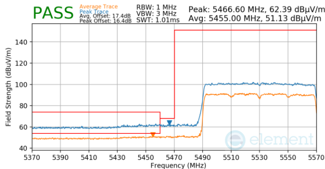
Plot 7-1054. Antenna WF5B (Pk & Avg, Ch.106, 802.11ax(SU), MCS11)
