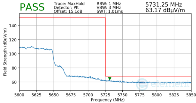
Plot 7-1037. (FCC Only) Antenna WF5B (Pk, Ch.122, 802.11ac, MCS2)
