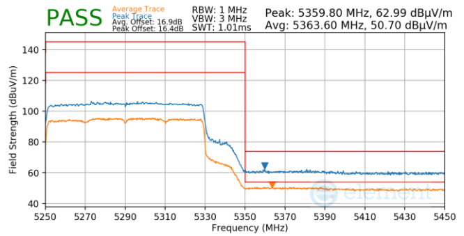
Plot 7-1049. Antenna WF5B (Pk & Avg, Ch.58, 802.11ax(SU), MCS2)
