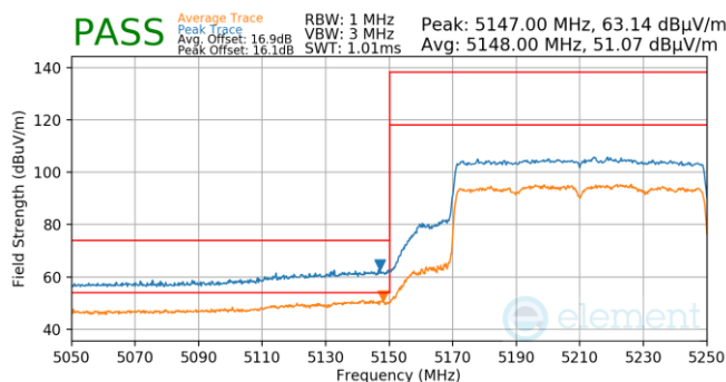
Plot 7-1047. Antenna WF5B (Pk & Avg, Ch.42, 802.11ax(SU), MCS4)
