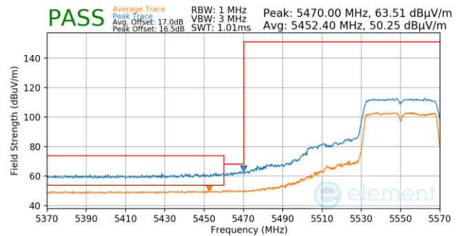
Plot 7-975. Antenna WF5B (Pk & Avg, Ch.110, 802.11n, MCS7)
