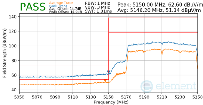
Plot 7-1026. Antenna WF5B (Pk & Avg, Ch.42, 802.11ac, MCS4)
