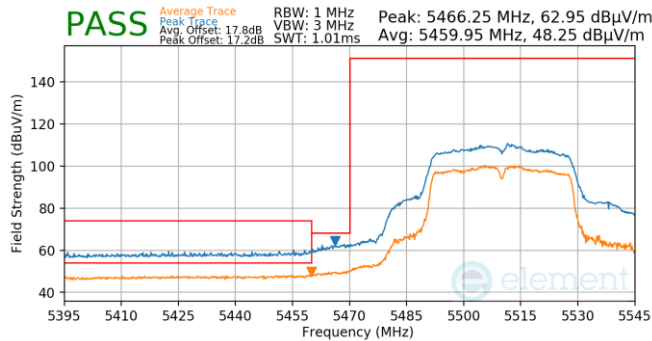
Plot 7-971. Antenna WF5B (Pk & Avg, Ch.102, 802.11n, MCS4)
