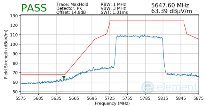
Plot 7-1062. Antenna WF5B (Pk, Ch.155, 802.11ax(SU), MCS4)
