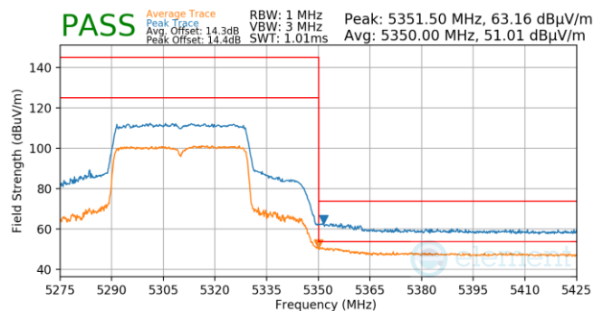
Plot 7-999. Antenna WF5B (Pk & Avg, Ch.62, 802.11ax(SU), MCS4)
