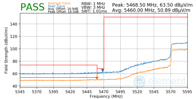
Plot 7-1056. (FCC Only) Antenna WF5B (Pk & Avg, Ch.122, 802.11ax(SU), MCS4)
