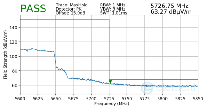
Plot 7-1038. (FCC Only) Antenna WF5B (Pk, Ch.122, 802.11ac, MCS4)
