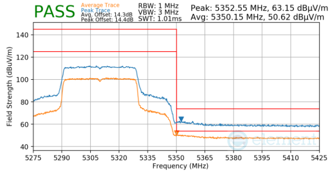
Plot 7-998. Antenna WF5B (Pk & Avg, Ch.62, 802.11ax(SU), MCS2)
