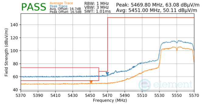
Plot 7-973. Antenna WF5B (Pk & Avg, Ch.110, 802.11n, MCS2)
