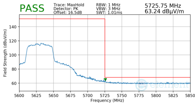
Plot 7-977. (FCC Only) Antenna WF5B (Pk, Ch.126, 802.11n, MCS2)
