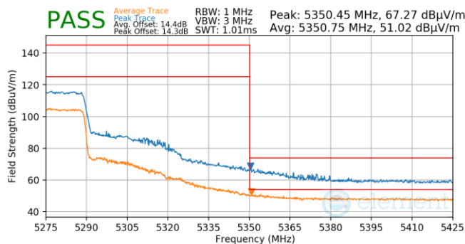
Plot 7-996. Antenna WF5B (Pk & Avg, Ch.54, 802.11ax(SU), MCS4)
