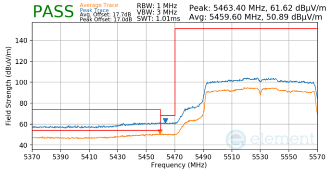
Plot 7-1031. Antenna WF5B (Pk & Avg, Ch.106, 802.11ac, MCS2)
