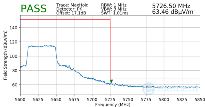
Plot 7-1015. (FCC Only) Antenna WF5B (Pk, Ch.126, 802.11ax(SU), MCS11)
