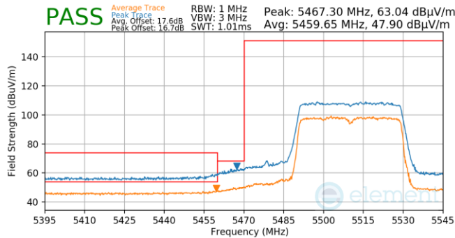
Plot 7-1003. Antenna WF5B (Pk & Avg, Ch.102, 802.11ax(SU), MCS11)
