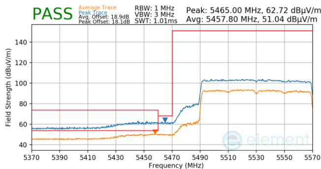
Plot 7-1053. Antenna WF5B (Pk & Avg, Ch.106, 802.11ax(SU), MCS4)
