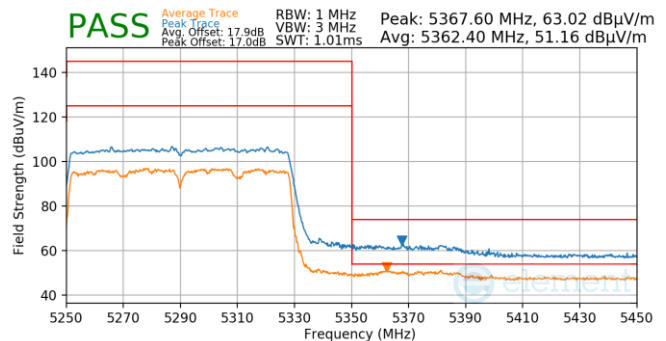
Plot 7-1030. Antenna WF5B (Pk & Avg, Ch.58, 802.11ac, MCS9)
