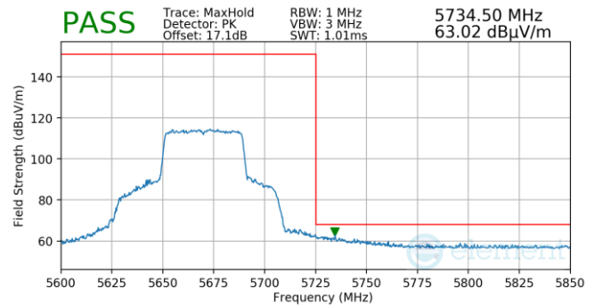
Plot 7-1017. Antenna WF5B (Pk, Ch.134, 802.11ax(SU), MCS4)
