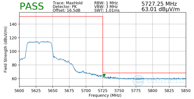
Plot 7-979. (FCC Only) Antenna WF5B (Pk, Ch.126, 802.11n, MCS7)
