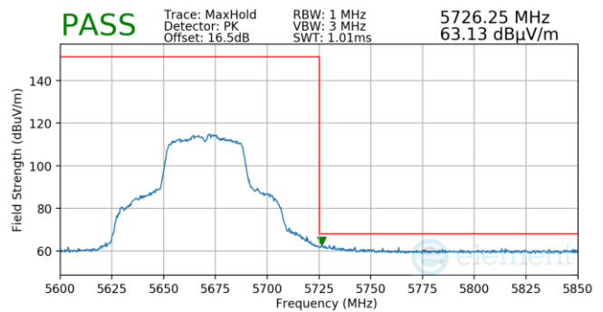
Plot 7-980. Antenna WF5B (Pk, Ch.134, 802.11n, MCS2)
