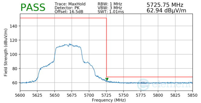
Plot 7-981. Antenna WF5B (Pk, Ch.134, 802.11n, MCS4)
