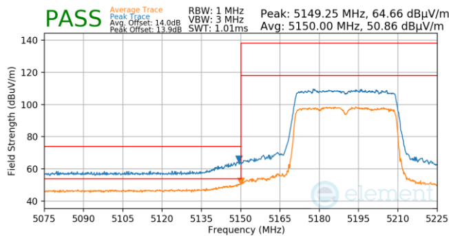
Plot 7-991. Antenna WF5B (Pk & Avg, Ch.38, 802.11ax(SU), MCS11)
