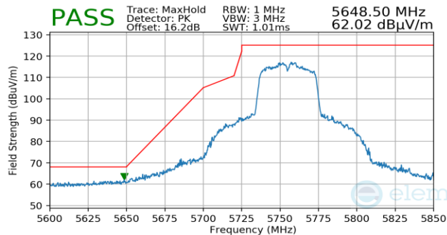
Plot 7-983. Antenna WF5B (Pk, Ch.151, 802.11n, MCS2)
