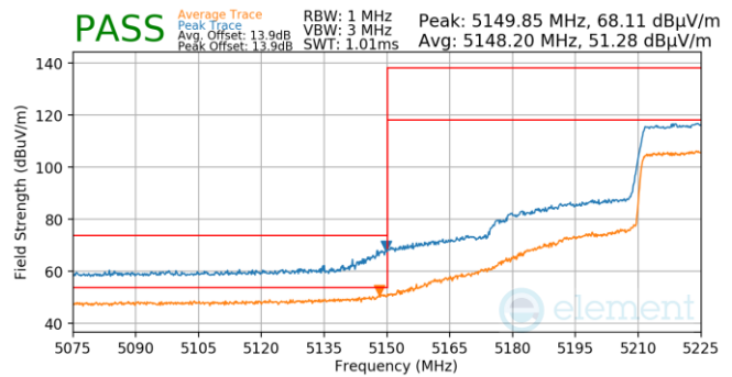
Plot 7-992. Antenna WF5B (Pk & Avg, Ch.46, 802.11ax(SU), MCS2)
