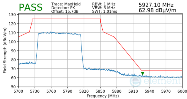
Plot 7-1065. Antenna WF5B (Pk, Ch.155, 802.11ax(SU), MCS4)
