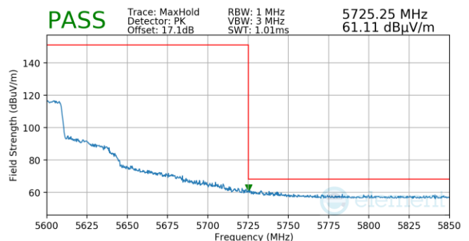
Plot 7-1011. (FCC Only) Antenna WF5B (Pk, Ch.118, 802.11ax(SU), MCS4)
