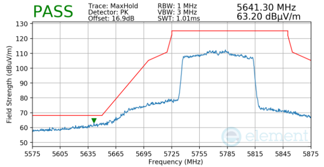
Plot 7-1040. Antenna WF5B (Pk, Ch.155, 802.11ac, MCS2)
