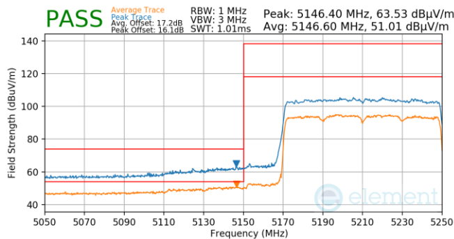
Plot 7-1048. Antenna WF5B (Pk & Avg, Ch.42, 802.11ax(SU), MCS11)
