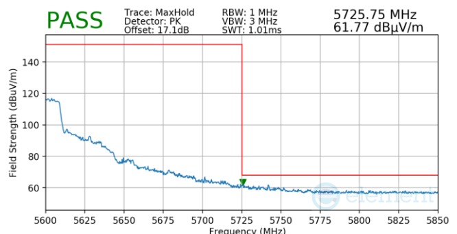
Plot 7-1012. (FCC Only) Antenna WF5B (Pk, Ch.118, 802.11ax(SU), MCS11)
