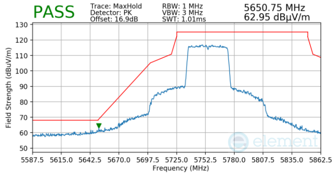
Plot 7-1019. Antenna WF5B (Pk, Ch.151, 802.11ax(SU), MCS2)
