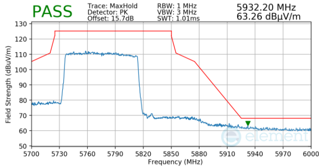
Plot 7-1064. Antenna WF5B (Pk, Ch.155, 802.11ax(SU), MCS2)
