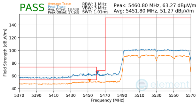
Plot 7-1033. Antenna WF5B (Pk & Avg, Ch.106, 802.11ac, MCS9)
