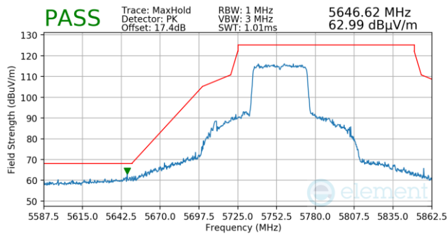
Plot 7-823. Antenna WF5T (Pk, Ch.151, 802.11ax(SU), MCS4)
