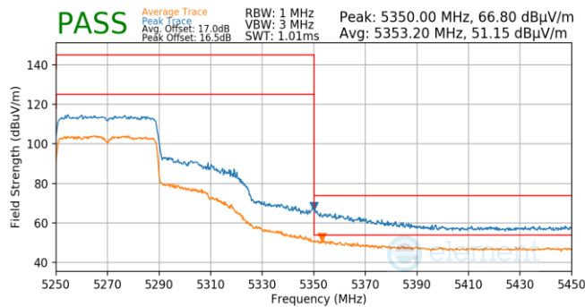
Plot 7-799. Antenna WF5T (Pk & Avg, Ch.54, 802.11ax(SU), MCS4)
