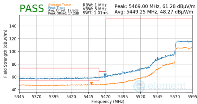
Plot 7-811. (FCC Only) Antenna WF5T (Pk & Avg, Ch.118, 802.11ax(SU), MCS4)
