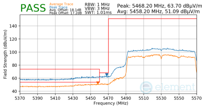
Plot 7-835. Antenna WF5T (Pk & Avg, Ch.106, 802.11ac, MCS4)
