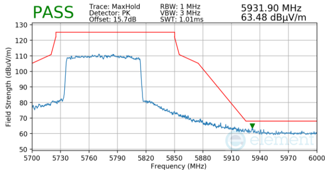
Plot 7-869. Antenna WF5T (Pk, Ch.155, 802.11ax(SU), MCS11)
