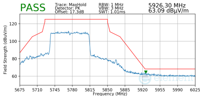
Plot 7-848. Antenna WF5T (Pk, Ch.155, 802.11ac, MCS9)
