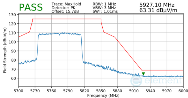
Plot 7-868. Antenna WF5T (Pk, Ch.155, 802.11ax(SU), MCS4)
