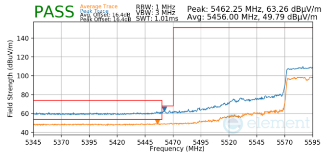
Plot 7-839. (FCC Only) Antenna WF5T (Pk & Avg, Ch.122, 802.11ac, MCS9)
