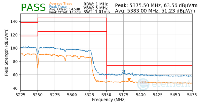
Plot 7-874. Antenna WF5T (Pk & Avg, Ch.50, 802.ac, MCS4)
