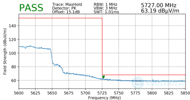
Plot 7-841. (FCC Only) Antenna WF5T (Pk, Ch.122, 802.11ac, MCS4)
