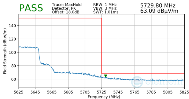
Plot 7-862. (FCC Only) Antenna WF5T (Pk, Ch.122, 802.11ax(SU), MCS4)
