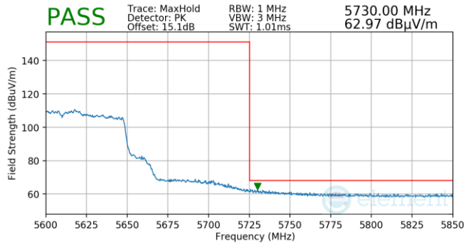
Plot 7-840. (FCC Only) Antenna WF5T (Pk, Ch.122, 802.11ac, MCS2)
