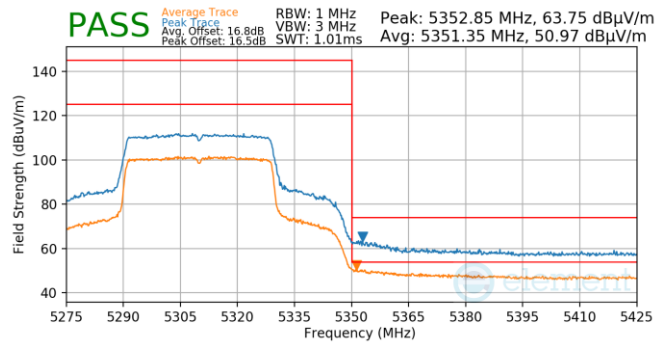
Plot 7-801. Antenna WF5T (Pk & Avg, Ch.62, 802.11ax(SU), MCS2)
