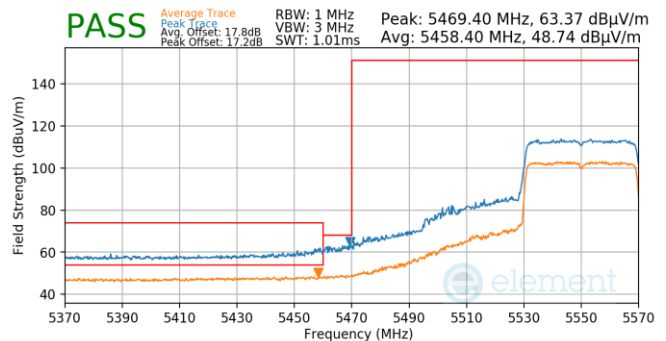
Plot 7-808. Antenna WF5T (Pk & Avg, Ch.110, 802.11ax(SU), MCS4)
