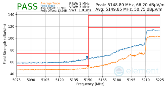
Plot 7-797. Antenna WF5T (Pk & Avg, Ch.46, 802.11ax(SU), MCS11)
