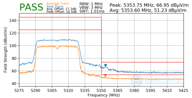
Plot 7-803. Antenna WF5T (Pk & Avg, Ch.62, 802.11ax(SU), MCS11)
