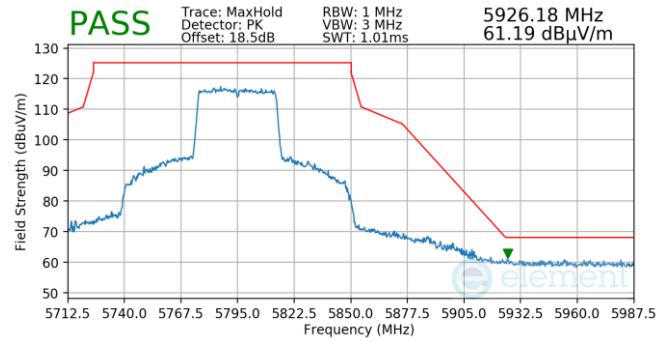
Plot 7-825. Antenna WF5T (Pk, Ch.159, 802.11ax(SU), MCS2)
