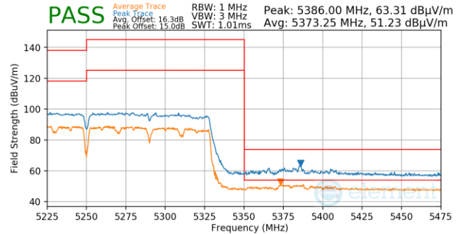
Plot 7-873. Antenna WF5T (Pk & Avg, Ch.50, 802.11ac, MCS2)
