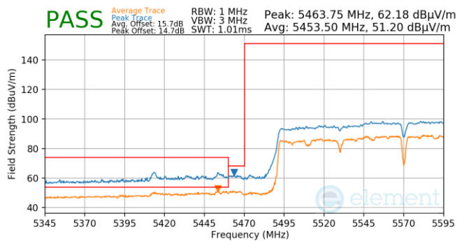
Plot 7-877. (FCC Only) Antenna WF5T (Pk & Avg, Ch.114, 802.ac, MCS4)
