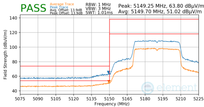
Plot 7-792. Antenna WF5T (Pk & Avg, Ch.38, 802.11ax(SU), MCS2)
