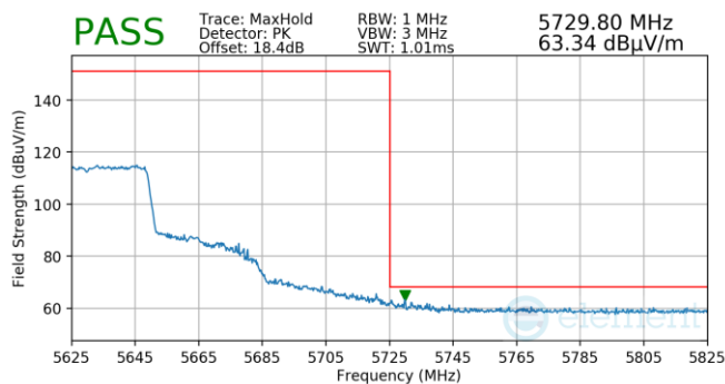
Plot 7-817. (FCC Only) Antenna WF5T (Pk, Ch.126, 802.11ax(SU), MCS4)
