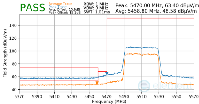
Plot 7-806. Antenna WF5T (Pk & Avg, Ch.102, 802.11ax(SU), MCS11)
