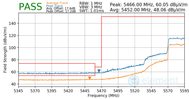
Plot 7-810. (FCC Only) Antenna WF5T (Pk & Avg, Ch.118, 802.11ax(SU), MCS2)
