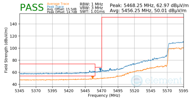
Plot 7-838. (FCC Only) Antenna WF5T (Pk & Avg, Ch.122, 802.11ac, MCS4)
