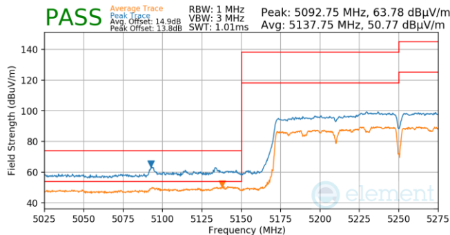
Plot 7-871. Antenna WF5T (Pk & Avg, Ch.50, 802.ac, MCS4)
