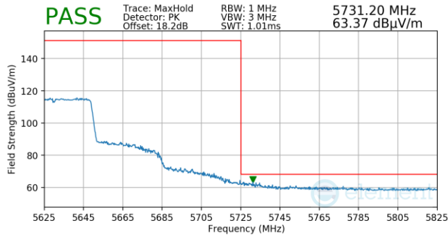
Plot 7-816. (FCC Only) Antenna WF5T (Pk, Ch.126, 802.11ax(SU), MCS2)
