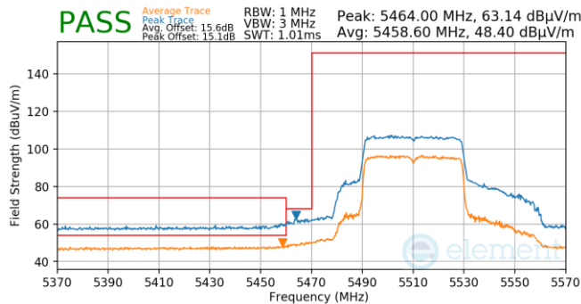
Plot 7-805. Antenna WF5T (Pk & Avg, Ch.102, 802.11ax(SU), MCS4)
