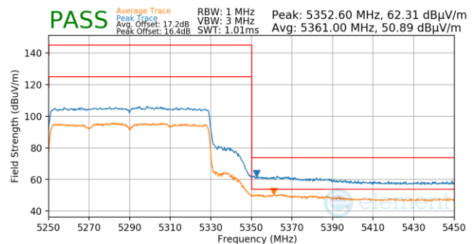
Plot 7-853. Antenna WF5T (Pk & Avg, Ch.58, 802.11ax(SU), MCS4)
