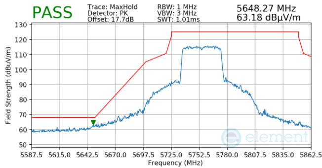
Plot 7-824. Antenna WF5T (Pk, Ch.151, 802.11ax(SU), MCS11)
