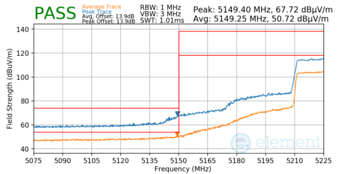
Plot 7-795. Antenna WF5T (Pk & Avg, Ch.46, 802.11ax(SU), MCS2)
