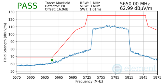
Plot 7-843. Antenna WF5T (Pk, Ch.155, 802.11ac, MCS2)
