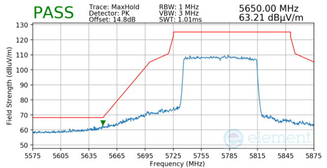
Plot 7-865. Antenna WF5T (Pk, Ch.155, 802.11ax(SU), MCS4)
