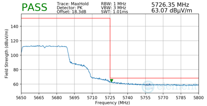
Plot 7-819. Antenna WF5T (Pk, Ch.134, 802.11ax(SU), MCS2)
