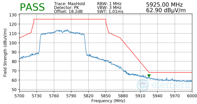
Plot 7-846. Antenna WF5T (Pk, Ch.155, 802.11ac, MCS2)
