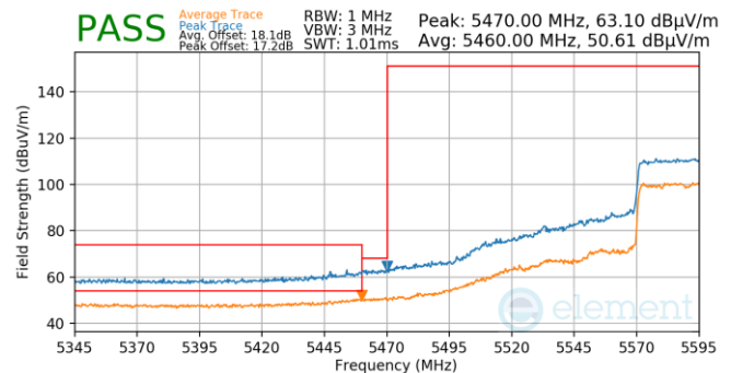
Plot 7-859. (FCC Only) Antenna WF5T (Pk & Avg, Ch.122, 802.11ax(SU), MCS4)
