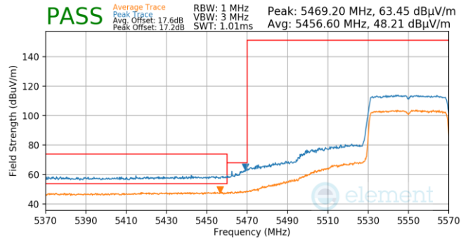
Plot 7-807. Antenna WF5T (Pk & Avg, Ch.110, 802.11ax(SU), MCS2)
