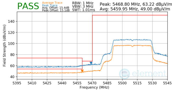
Plot 7-804. Antenna WF5T (Pk & Avg, Ch.102, 802.11ax(SU), MCS2)
