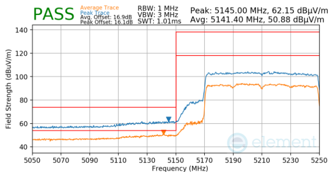
Plot 7-850. Antenna WF5T (Pk & Avg, Ch.42, 802.11ax(SU), MCS4)
