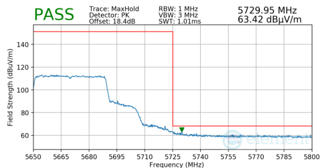
Plot 7-820. Antenna WF5T (Pk, Ch.134, 802.11ax(SU), MCS4)
