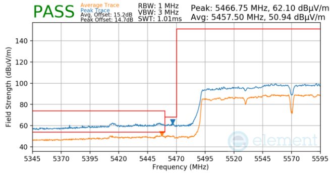
Plot 7-876. (FCC Only) Antenna WF5T (Pk & Avg, Ch.114, 802.ac, MCS2)
