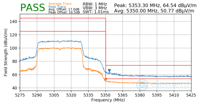
Plot 7-802. Antenna WF5T (Pk & Avg, Ch.62, 802.11ax(SU), MCS4)
