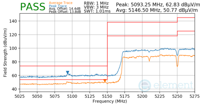
Plot 7-870. Antenna WF5T (Pk & Avg, Ch.50, 802.11ac, MCS2)
