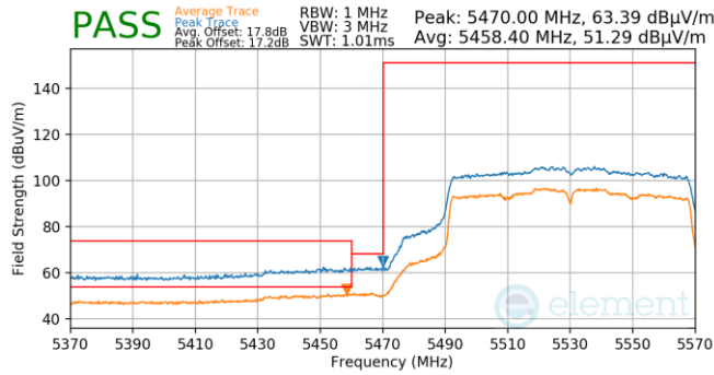
Plot 7-834. Antenna WF5T (Pk & Avg, Ch.106, 802.11ac, MCS2)
