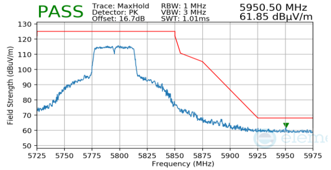
Plot 7-791. Antenna WF5T (Pk, Ch.159, 802.11n, MCS7)
