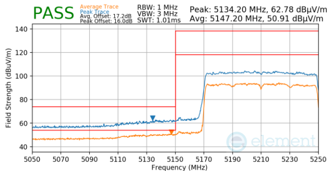
Plot 7-851. Antenna WF5T (Pk & Avg, Ch.42, 802.11ax(SU), MCS11)
