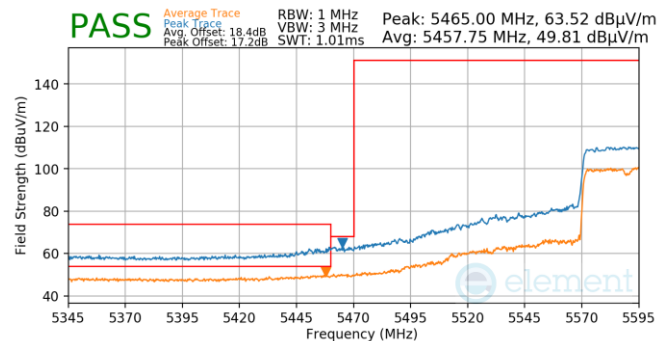
Plot 7-860. (FCC Only) Antenna WF5T (Pk & Avg, Ch.122, 802.11ax(SU), MCS11)
