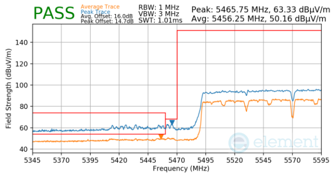
Plot 7-878. (FCC Only) Antenna WF5T (Pk & Avg, Ch.114, 802.ac, MCS9)
