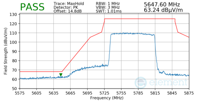
Plot 7-864. Antenna WF5T (Pk, Ch.155, 802.11ax(SU), MCS2)
