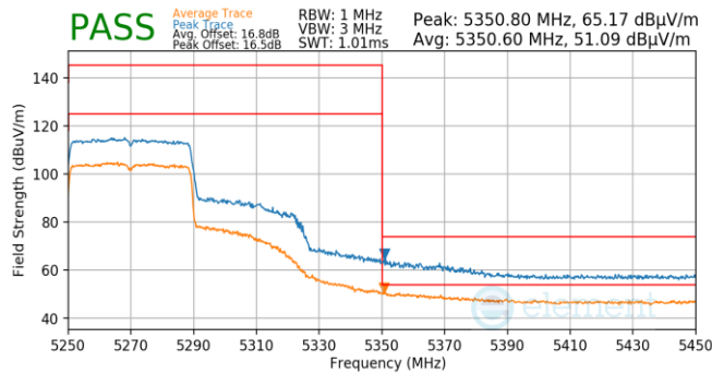
Plot 7-798. Antenna WF5T (Pk & Avg, Ch.54, 802.11ax(SU), MCS2)
