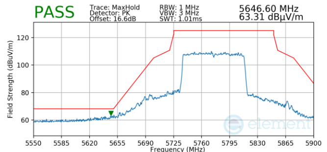
Plot 7-845. Antenna WF5T (Pk, Ch.155, 802.11ac, MCS9)
