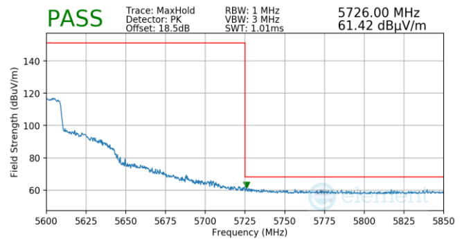
Plot 7-814. (FCC Only) Antenna WF5T (Pk, Ch.118, 802.11ax(SU), MCS4)
