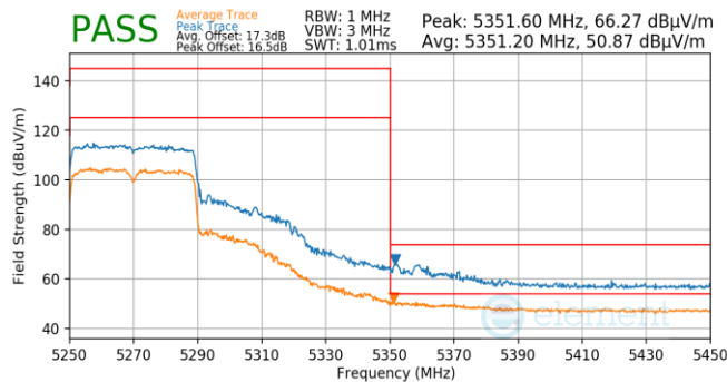
Plot 7-800. Antenna WF5T (Pk & Avg, Ch.54, 802.11ax(SU), MCS11)
