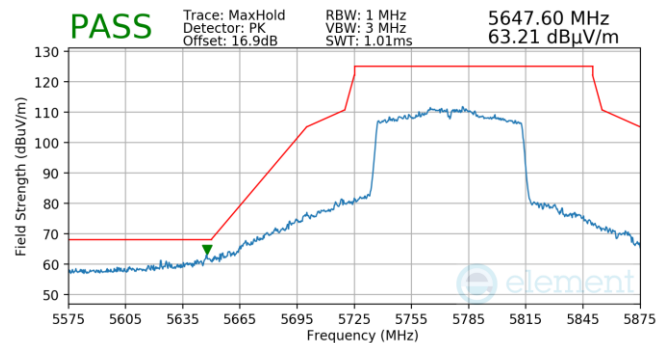
Plot 7-844. Antenna WF5T (Pk, Ch.155, 802.11ac, MCS4)
