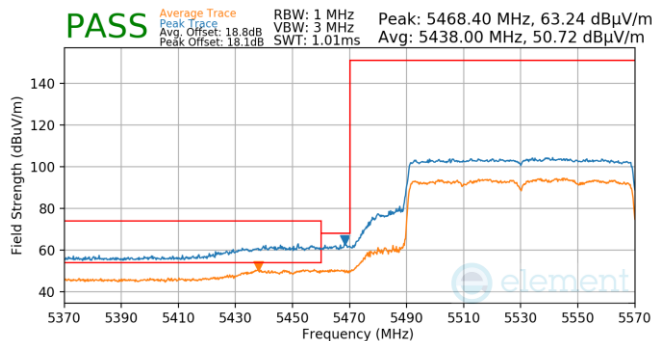
Plot 7-856. Antenna WF5T (Pk & Avg, Ch.106, 802.11ax(SU), MCS4)
