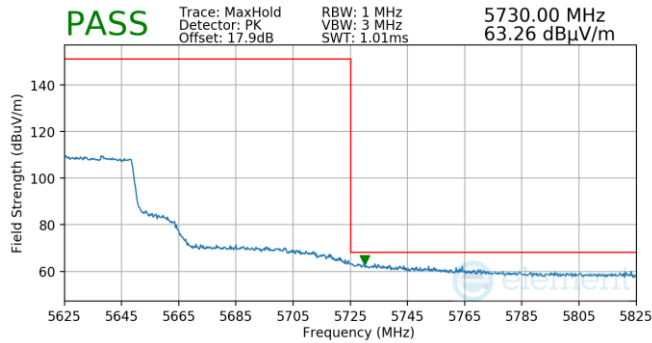
Plot 7-861. (FCC Only) Antenna WF5T (Pk, Ch.122, 802.11ax(SU), MCS2)
