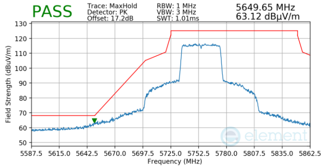
Plot 7-822. Antenna WF5T (Pk, Ch.151, 802.11ax(SU), MCS2)
