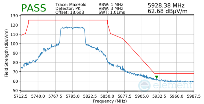
Plot 7-826. Antenna WF5T (Pk, Ch.159, 802.11ax(SU), MCS4)
