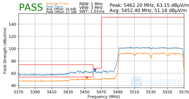
Plot 7-836. Antenna WF5T (Pk & Avg, Ch.106, 802.11ac, MCS9)
