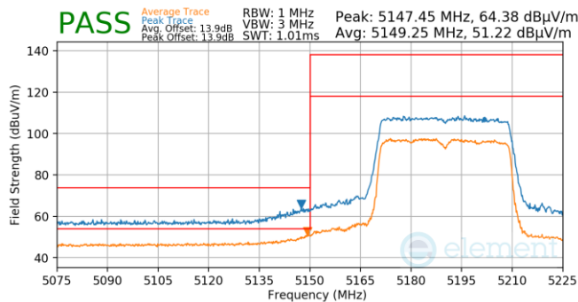
Plot 7-794. Antenna WF5T (Pk & Avg, Ch.38, 802.11ax(SU), MCS11)
