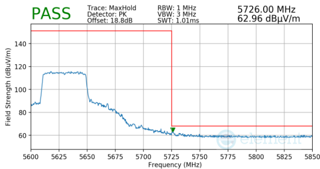
Plot 7-818. (FCC Only) Antenna WF5T (Pk, Ch.126, 802.11ax(SU), MCS11)
