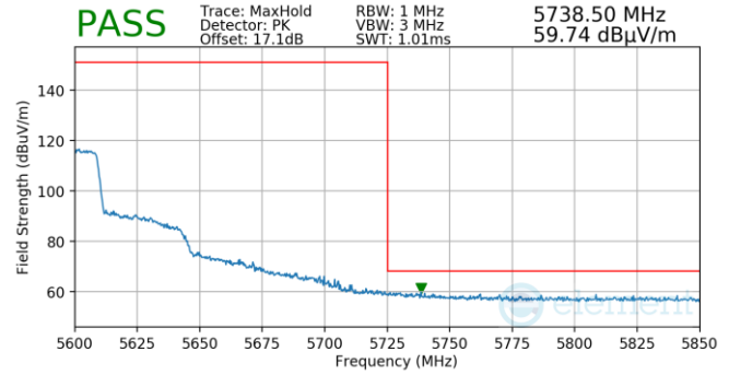
Plot 7-813. (FCC Only) Antenna WF5T (Pk, Ch.118, 802.11ax(SU), MCS2)
