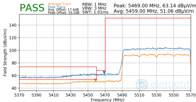
Plot 7-857. Antenna WF5T (Pk & Avg, Ch.106, 802.11ax(SU), MCS11)
