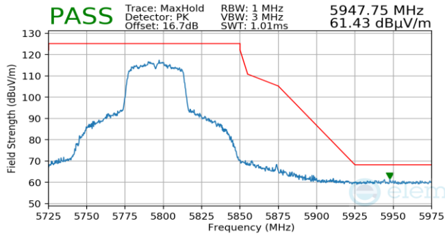
Plot 7-789. Antenna WF5T (Pk, Ch.159, 802.11n, MCS2)
