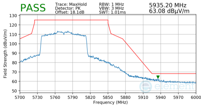
Plot 7-847. Antenna WF5T (Pk, Ch.155, 802.11ac, MCS4)
