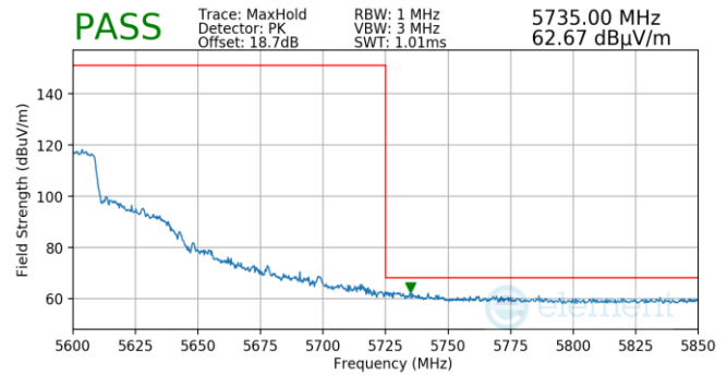
Plot 7-815. (FCC Only) Antenna WF5T (Pk, Ch.118, 802.11ax(SU), MCS11)
