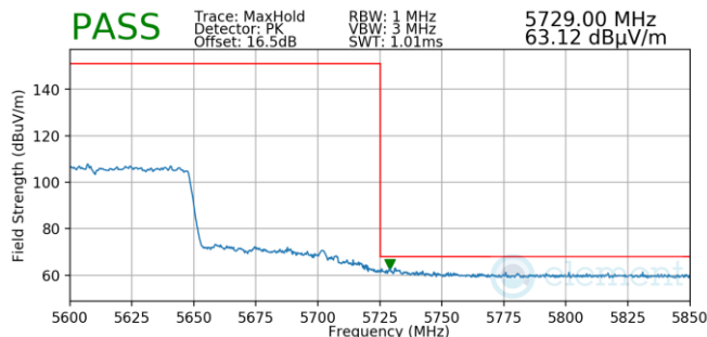
Plot 7-842. (FCC Only) Antenna WF5T (Pk, Ch.122, 802.11ac, MCS9)
