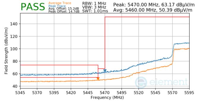
Plot 7-837. (FCC Only) Antenna WF5T (Pk & Avg, Ch.122, 802.11ac, MCS2)
