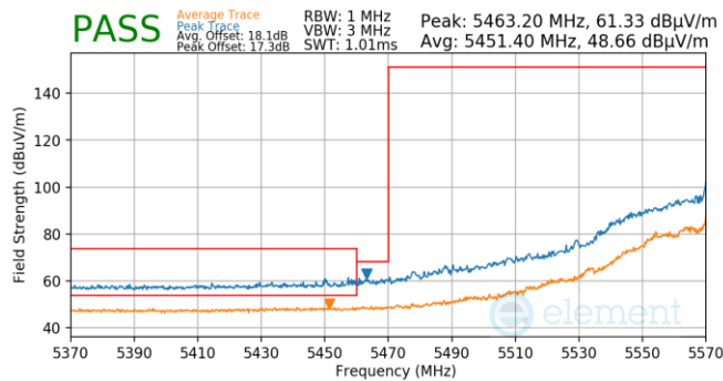
Plot 7-812. (FCC Only) Antenna WF5T (Pk & Avg, Ch.118, 802.11ax(SU), MCS11)
