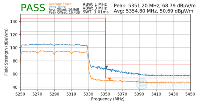
Plot 7-854. Antenna WF5T (Pk & Avg, Ch.58, 802.11ax(SU), MCS11)
