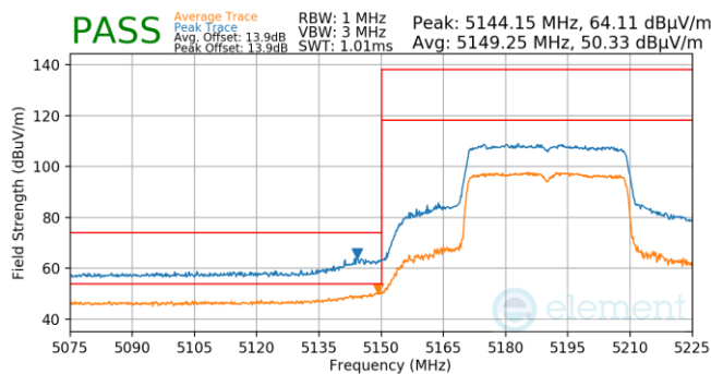
Plot 7-793. Antenna WF5T (Pk & Avg, Ch.38, 802.11ax(SU), MCS4)
