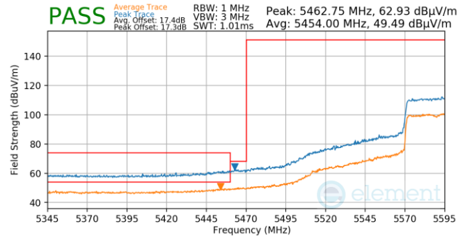
Plot 7-858. (FCC Only) Antenna WF5T (Pk & Avg, Ch.122, 802.11ax(SU), MCS2)
