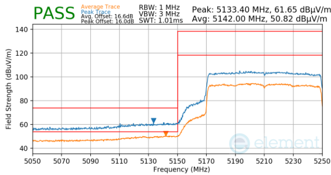
Plot 7-849. Antenna WF5T (Pk & Avg, Ch.42, 802.11ax(SU), MCS2)
