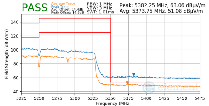
Plot 7-875. Antenna WF5T (Pk & Avg, Ch.50, 802.ac, MCS9)
