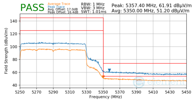
Plot 7-852. Antenna WF5T (Pk & Avg, Ch.58, 802.11ax(SU), MCS2)
