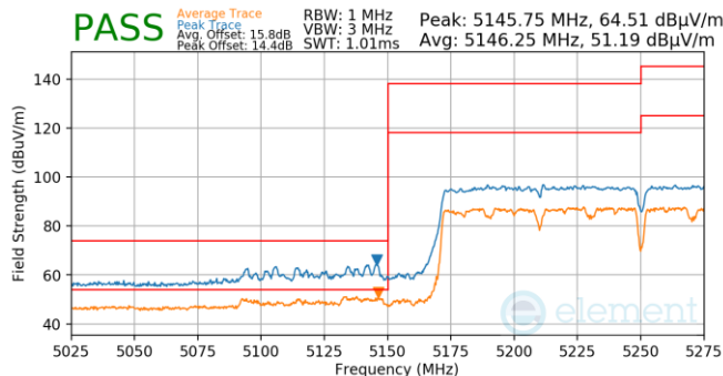
Plot 7-872. Antenna WF5T (Pk & Avg, Ch.50, 802.ac, MCS9)
