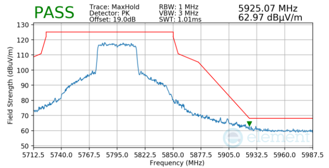
Plot 7-827. Antenna WF5T (Pk, Ch.159, 802.11ax(SU), MCS11)
