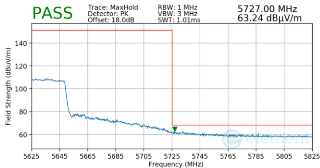
Plot 7-863. (FCC Only) Antenna WF5T (Pk, Ch.122, 802.11ax(SU), MCS11)
