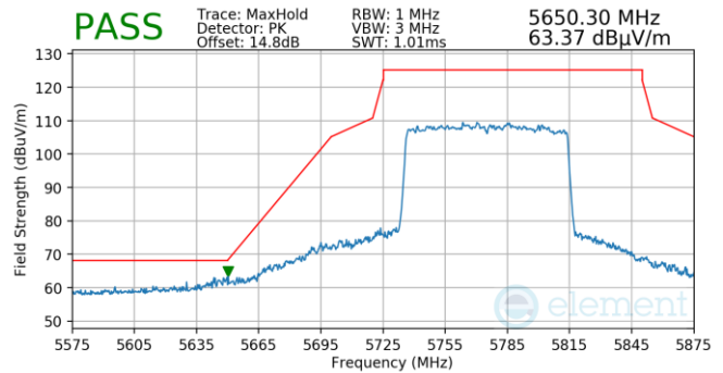
Plot 7-866. Antenna WF5T (Pk, Ch.155, 802.11ax(SU), MCS11)
