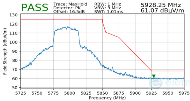
Plot 7-790. Antenna WF5T (Pk, Ch.159, 802.11n, MCS4)
