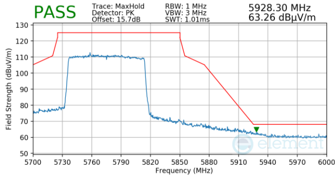
Plot 7-867. Antenna WF5T (Pk, Ch.155, 802.11ax(SU), MCS2)
