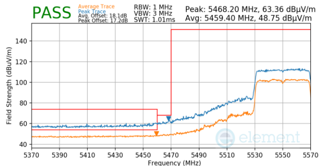
Plot 7-809. Antenna WF5T (Pk & Avg, Ch.110, 802.11ax(SU), MCS11)
