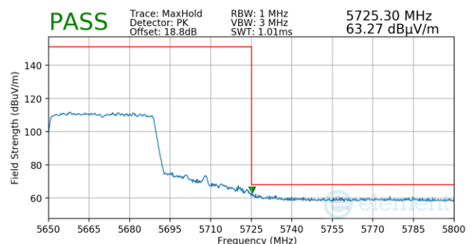
Plot 7-821. Antenna WF5T (Pk, Ch.134, 802.11ax(SU), MCS11)
