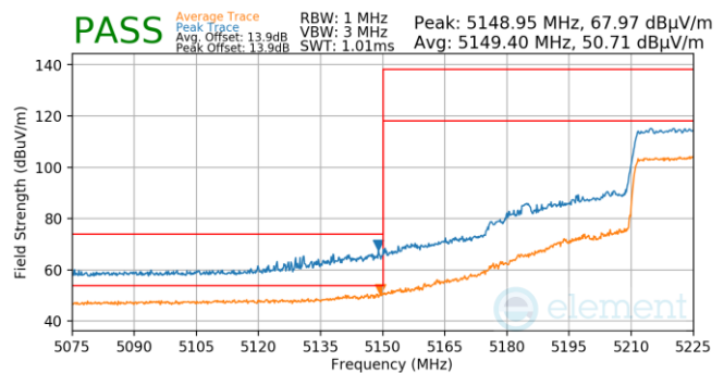
Plot 7-796. Antenna WF5T (Pk & Avg, Ch.46, 802.11ax(SU), MCS4)
