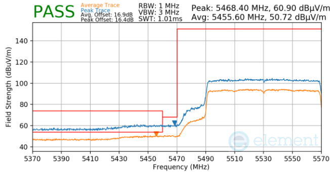
Plot 7-855. Antenna WF5T (Pk & Avg, Ch.106, 802.11ax(SU), MCS2)
