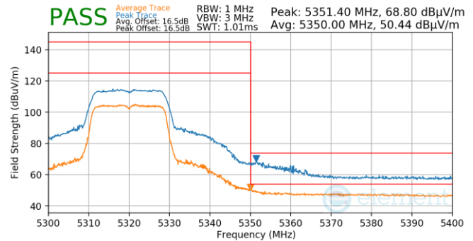
Plot 7-700. Antenna WF5T (Pk & Avg, Ch.64, 802.11n, MCS7)
