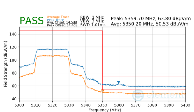
Plot 7-730. Antenna WF5T (Pk & Avg, Ch.64, 802.11ax(SU), MCS2)
