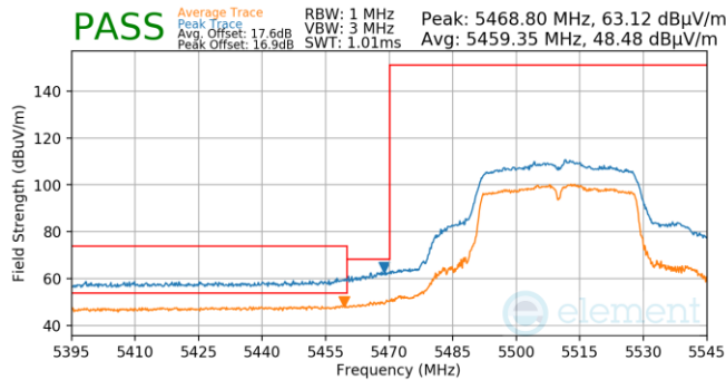
Plot 7-772. Antenna WF5T (Pk & Avg, Ch.102, 802.11n, MCS4)
