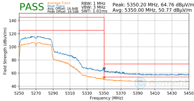
Plot 7-765. Antenna WF5T (Pk & Avg, Ch.54, 802.11n, MCS2)
