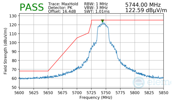
Plot 7-716. Antenna WF5T (Pk, Ch.149, 802.11n, MCS4)
