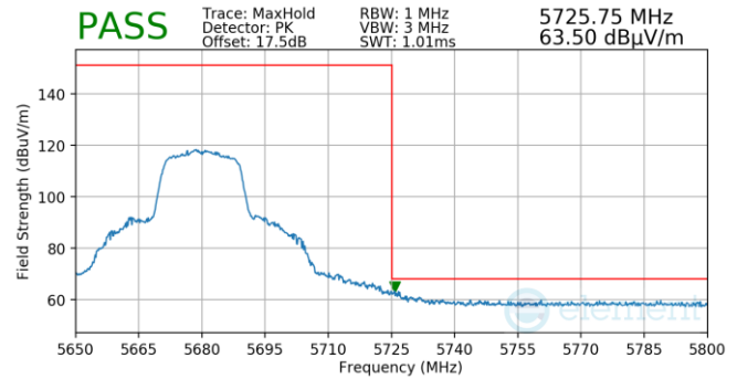
Plot 7-710. Antenna WF5T (Pk, Ch.136, 802.11n, MCS4)
