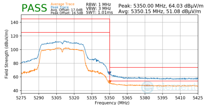
Plot 7-769. Antenna WF5T (Pk & Avg, Ch.62, 802.11n, MCS4)
