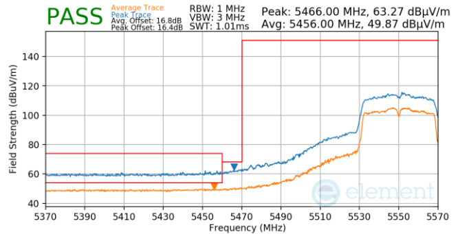
Plot 7-775. Antenna WF5T (Pk & Avg, Ch.110, 802.11n, MCS4)
