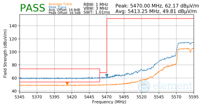
Plot 7-779. (FCC Only) Antenna WF5T (Pk & Avg, Ch.118, 802.11n, MCS7)
