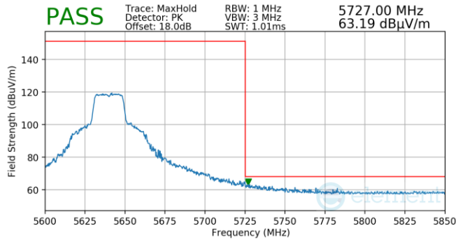
Plot 7-743. *(FCC Only) Antenna WF5T (Pk, Ch.128, 802.11ax(SU), MCS11)
