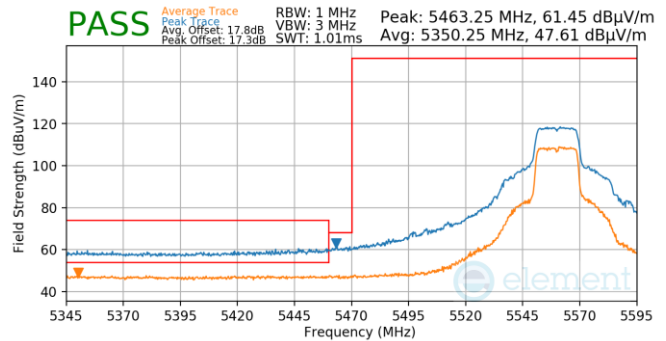
Plot 7-742. Antenna WF5T (Pk & Avg, Ch.112, 802.11ax(SU), MCS11)
