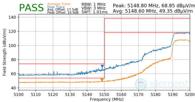
Plot 7-726. Antenna WF5T (Pk & Avg, Ch.40, 802.11ax(SU), MCS11)
