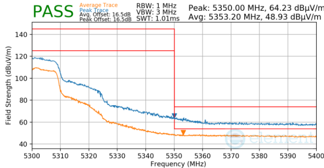
Plot 7-696. Antenna WF5T (Pk & Avg, Ch.60, 802.11n, MCS4)
