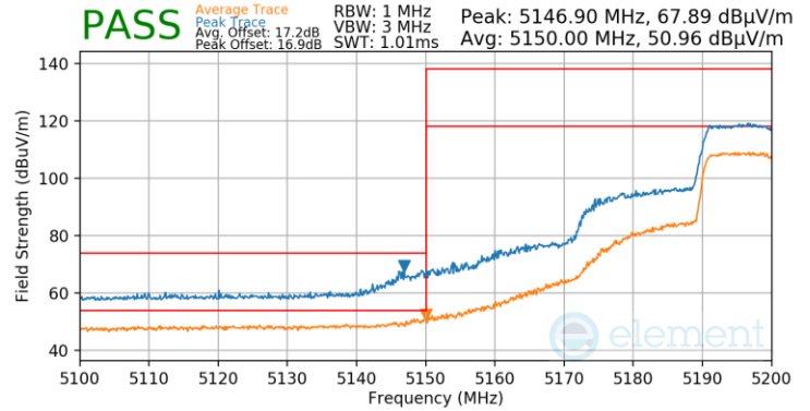
Plot 7-724. Antenna WF5T (Pk & Avg, Ch.40, 802.11ax(SU), MCS2)
