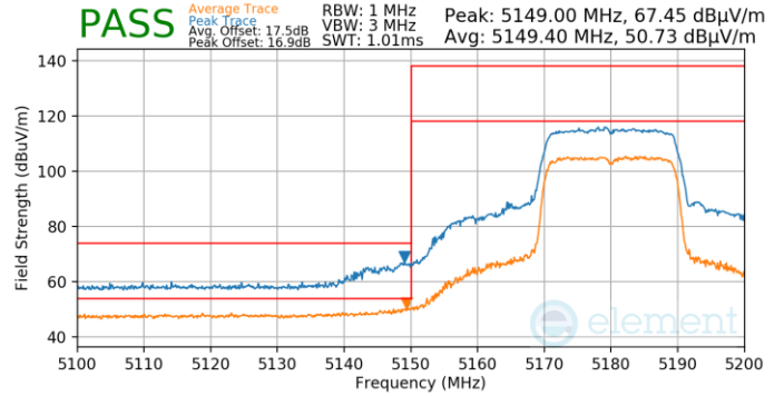
Plot 7-723. Antenna WF5T (Pk & Avg, Ch.36, 802.11ax(SU), MCS11)
