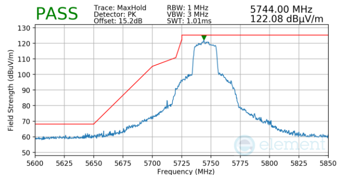
Plot 7-754. Antenna WF5T (Pk, Ch.149, 802.11ax(SU), MCS4)
