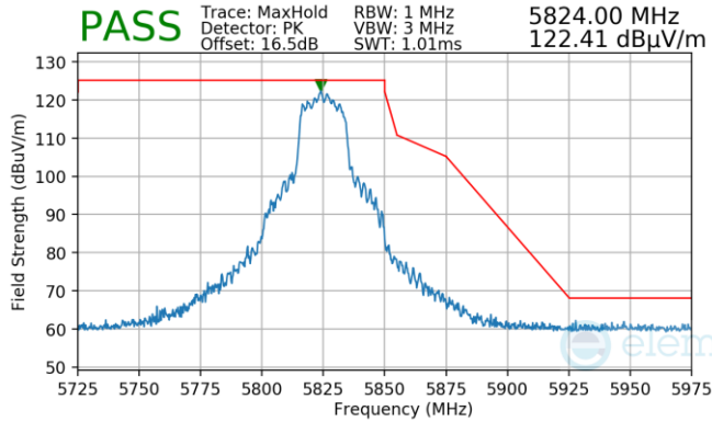
Plot 7-719. Antenna WF5T (Pk, Ch.165, 802.11n, MCS4)
