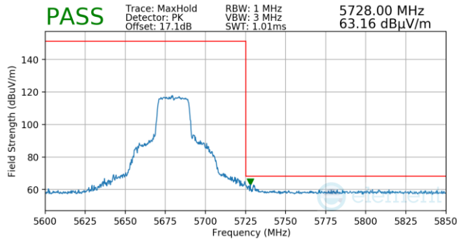
Plot 7-749. Antenna WF5T (Pk, Ch.136, 802.11ax(SU), MCS11)
