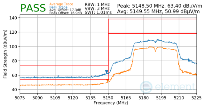
Plot 7-760. Antenna WF5T (Pk & Avg, Ch.38, 802.11n, MCS4)
