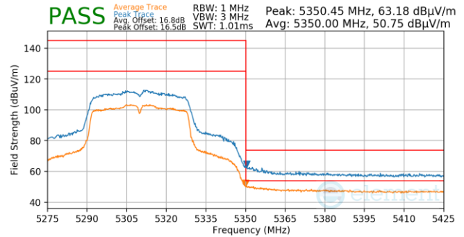
Plot 7-768. Antenna WF5T (Pk & Avg, Ch.62, 802.11n, MCS2)
