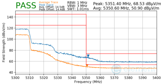
Plot 7-727. Antenna WF5T (Pk & Avg, Ch.60, 802.11ax(SU), MCS2)
