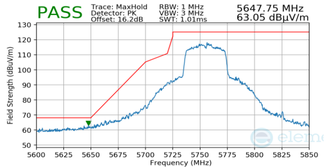
Plot 7-787. Antenna WF5T (Pk, Ch.151, 802.11n, MCS4)
