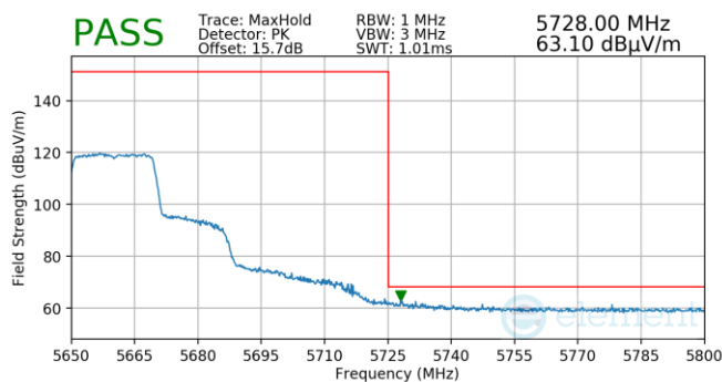
Plot 7-744. Antenna WF5T (Pk, Ch.132, 802.11ax(SU), MCS2)
