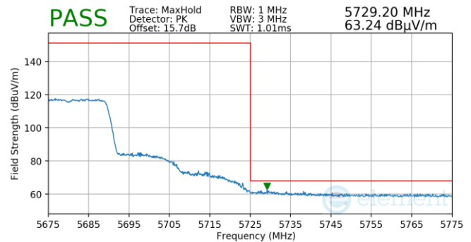
Plot 7-747. Antenna WF5T (Pk, Ch.136, 802.11ax(SU), MCS2)
