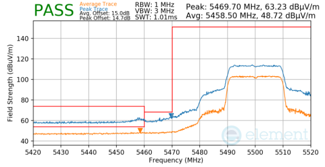
Plot 7-734. Antenna WF5T (Pk & Avg, Ch.100, 802.11ax(SU), MCS4)
