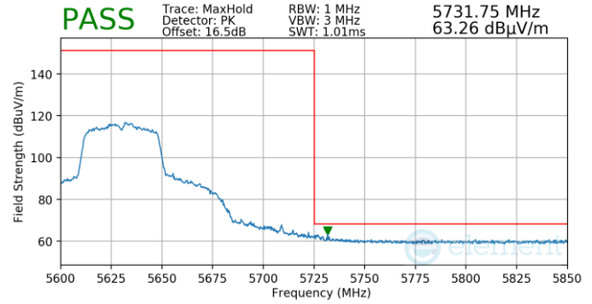
Plot 7-780. (FCC Only) Antenna WF5T (Pk, Ch.126, 802.11n, MCS2)
