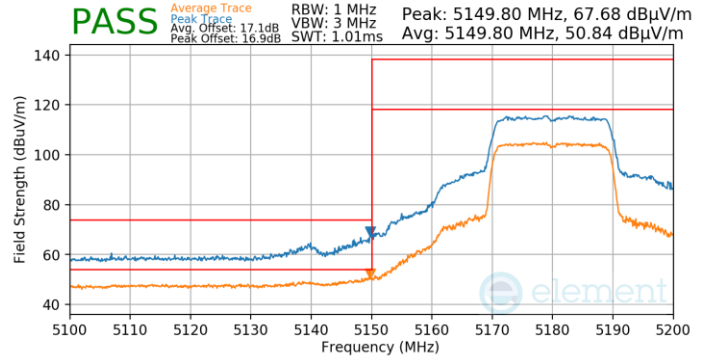
Plot 7-722. Antenna WF5T (Pk & Avg, Ch.36, 802.11ax(SU), MCS4)
