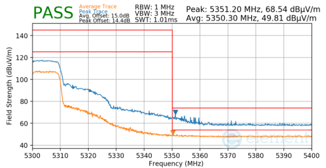
Plot 7-729. Antenna WF5T (Pk & Avg, Ch.60, 802.11ax(SU), MCS11)
