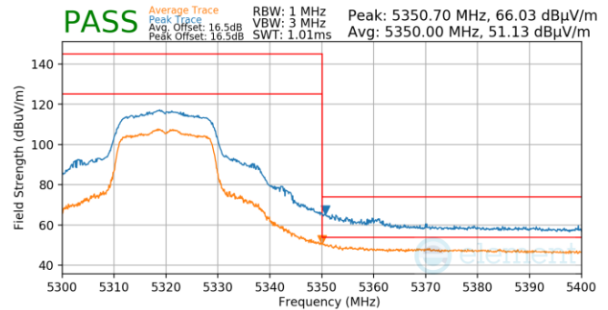
Plot 7-699. Antenna WF5T (Pk & Avg, Ch.64, 802.11n, MCS4)
