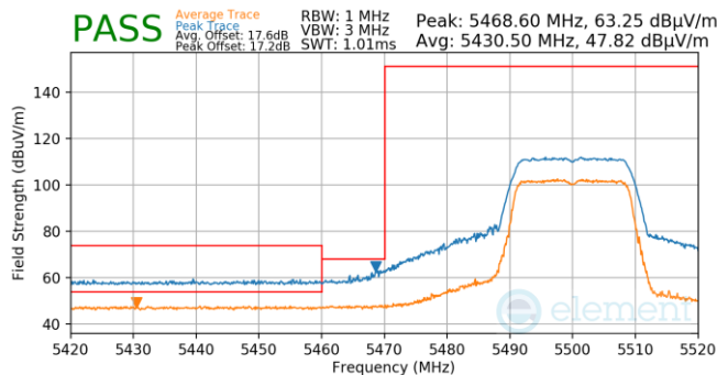
Plot 7-703. Antenna WF5T (Pk & Avg, Ch.100, 802.11n, MCS7)
