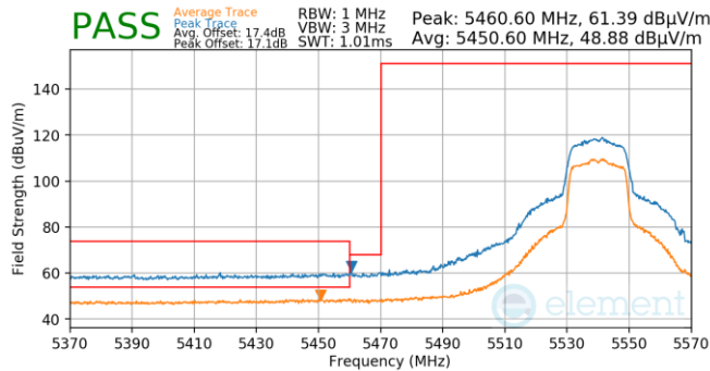
Plot 7-739. Antenna WF5T (Pk & Avg, Ch.108, 802.11ax(SU), MCS2)
