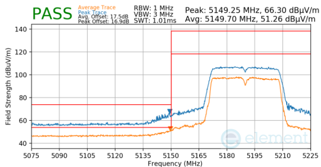
Plot 7-761. Antenna WF5T (Pk & Avg, Ch.38, 802.11n, MCS7)
