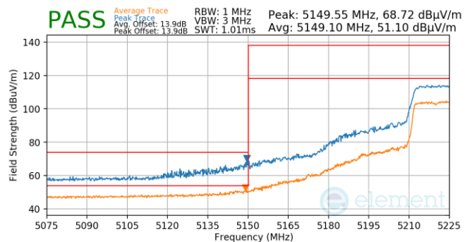
Plot 7-764. Antenna WF5T (Pk & Avg, Ch.46, 802.11n, MCS7)
