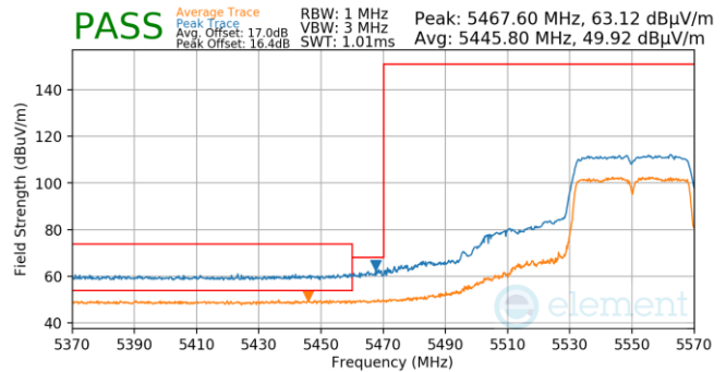
Plot 7-776. Antenna WF5T (Pk & Avg, Ch.110, 802.11n, MCS7)
