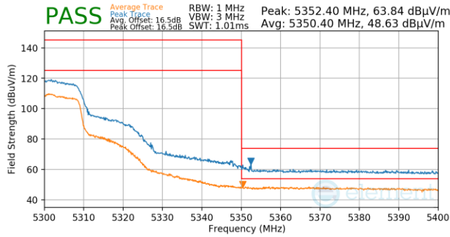
Plot 7-695. Antenna WF5T (Pk & Avg, Ch.60, 802.11n, MCS2)
