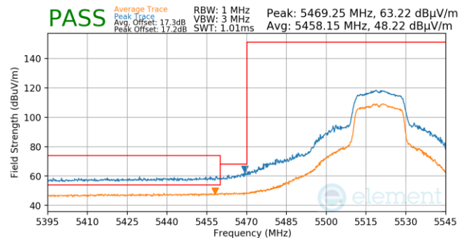
Plot 7-705. Antenna WF5T (Pk & Avg, Ch.104, 802.11n, MCS4)
