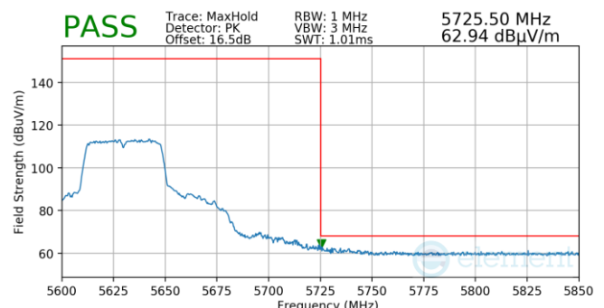
Plot 7-782. (FCC Only) Antenna WF5T (Pk, Ch.126, 802.11n, MCS7)
