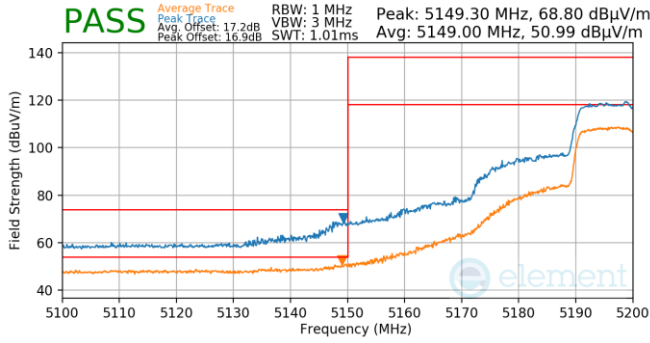
Plot 7-725. Antenna WF5T (Pk & Avg, Ch.40, 802.11ax(SU), MCS4)
