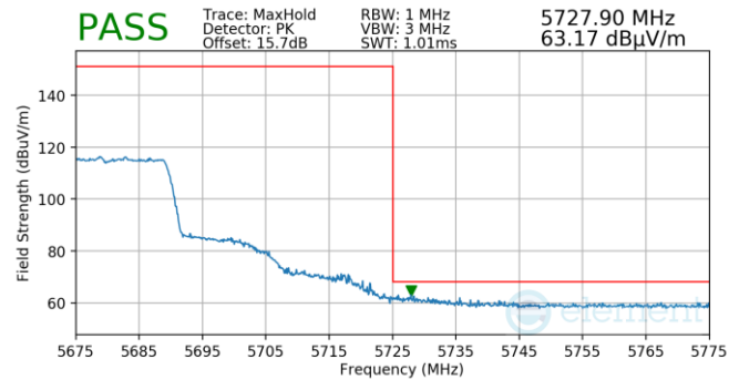
Plot 7-748. Antenna WF5T (Pk, Ch.136, 802.11ax(SU), MCS4)
