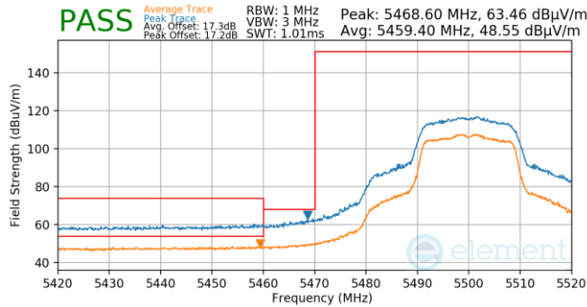
Plot 7-701. Antenna WF5T (Pk & Avg, Ch.100, 802.11n, MCS2)
