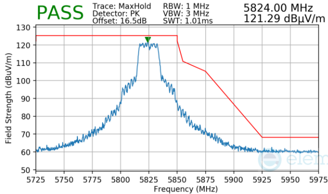
Plot 7-720. Antenna WF5T (Pk, Ch.165, 802.11n, MCS7)
