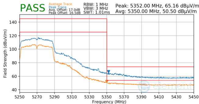
Plot 7-766. Antenna WF5T (Pk & Avg, Ch.54, 802.11n, MCS4)
