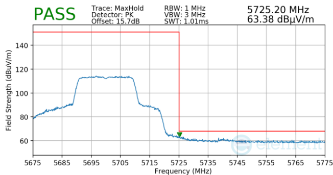
Plot 7-750. Antenna WF5T (Pk, Ch.140, 802.11ax(SU), MCS2)
