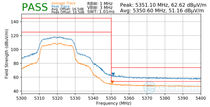
Plot 7-698. Antenna WF5T (Pk & Avg, Ch.64, 802.11n, MCS2)
