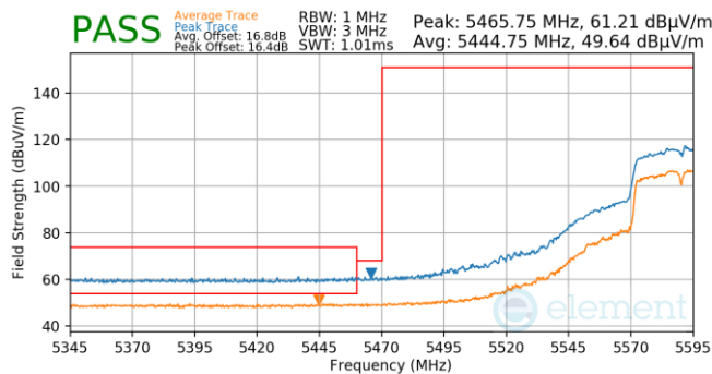
Plot 7-778. (FCC Only) Antenna WF5T (Pk & Avg, Ch.118, 802.11n, MCS4)
