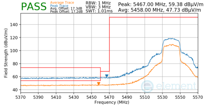
Plot 7-740. Antenna WF5T (Pk & Avg, Ch.108, 802.11ax(SU), MCS4)
