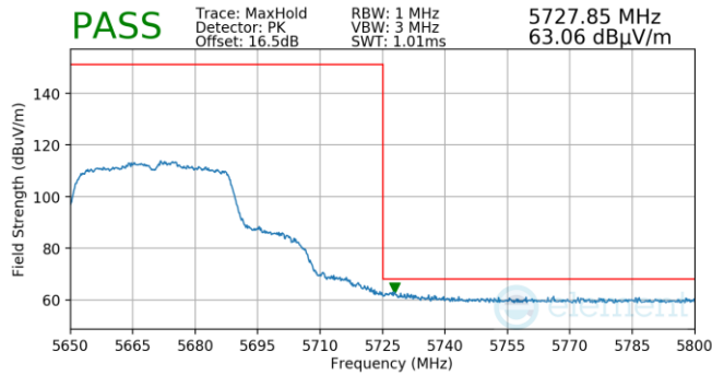
Plot 7-783. Antenna WF5T (Pk, Ch.134, 802.11n, MCS2)
