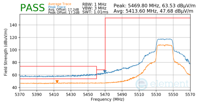
Plot 7-741. Antenna WF5T (Pk & Avg, Ch.108, 802.11ax(SU), MCS11)
