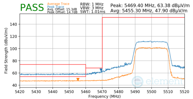
Plot 7-735. Antenna WF5T (Pk & Avg, Ch.100, 802.11ax(SU), MCS11)
