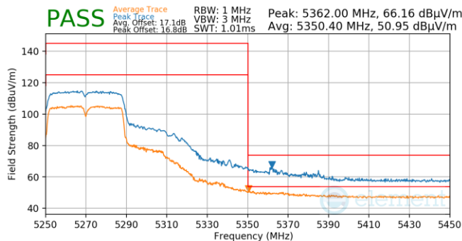
Plot 7-767. Antenna WF5T (Pk & Avg, Ch.54, 802.11n, MCS7)
