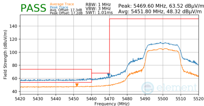
Plot 7-702. Antenna WF5T (Pk & Avg, Ch.100, 802.11n, MCS4)
