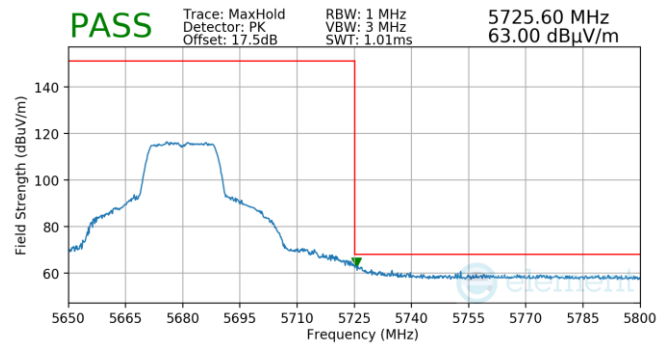
Plot 7-711. Antenna WF5T (Pk, Ch.136, 802.11n, MCS7)
