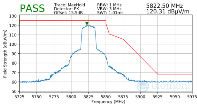
Plot 7-756. Antenna WF5T (Pk, Ch.165, 802.11ax(SU), MCS2)
