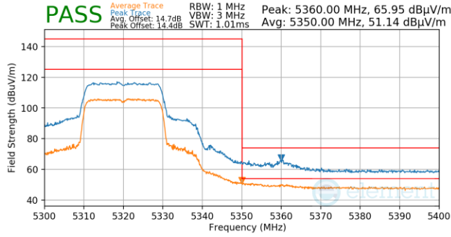
Plot 7-731. Antenna WF5T (Pk & Avg, Ch.64, 802.11ax(SU), MCS4)
