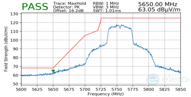
Plot 7-786. Antenna WF5T (Pk, Ch.151, 802.11n, MCS2)
