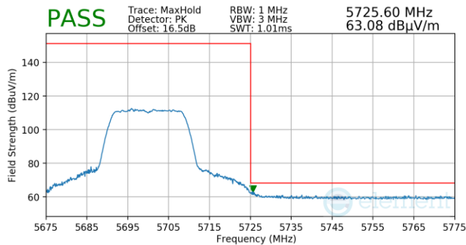
Plot 7-714. Antenna WF5T (Pk, Ch.140, 802.11n, MCS7)
