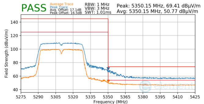
Plot 7-770. Antenna WF5T (Pk & Avg, Ch.62, 802.11n, MCS7)
