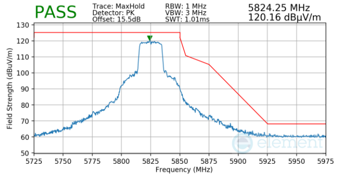
Plot 7-758. Antenna WF5T (Pk, Ch.165, 802.11ax(SU), MCS11)
