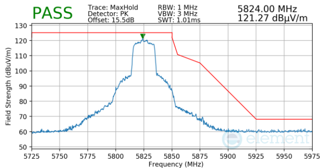
Plot 7-757. Antenna WF5T (Pk, Ch.165, 802.11ax(SU), MCS4)
