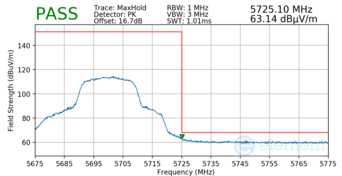
Plot 7-712. Antenna WF5T (Pk, Ch.140, 802.11n, MCS2)
