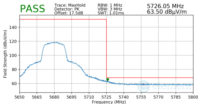
Plot 7-709. Antenna WF5T (Pk, Ch.136, 802.11n, MCS2)
