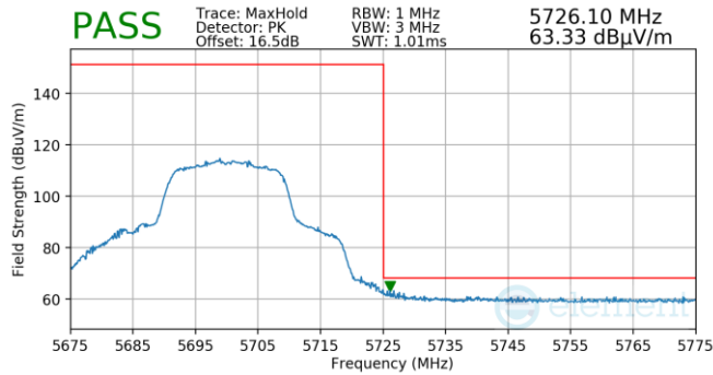
Plot 7-713. Antenna WF5T (Pk, Ch.140, 802.11n, MCS4)
