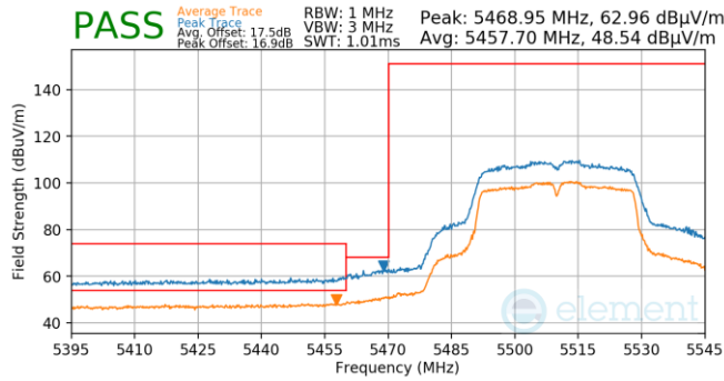
Plot 7-771. Antenna WF5T (Pk & Avg, Ch.102, 802.11n, MCS2)
