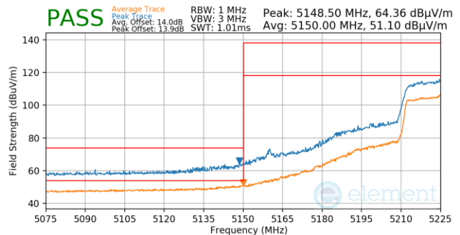
Plot 7-763. Antenna WF5T (Pk & Avg, Ch.46, 802.11n, MCS4)
