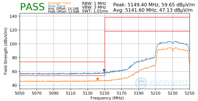
Plot 7-762. Antenna WF5T (Pk & Avg, Ch.46, 802.11n, MCS2)
