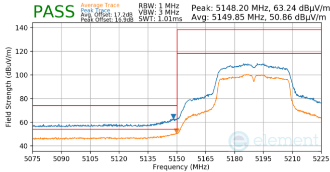
Plot 7-759. Antenna WF5T (Pk & Avg, Ch.38, 802.11n, MCS2)
