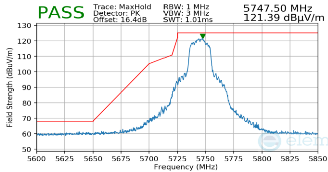
Plot 7-715. Antenna WF5T (Pk, Ch.149, 802.11n, MCS2)
