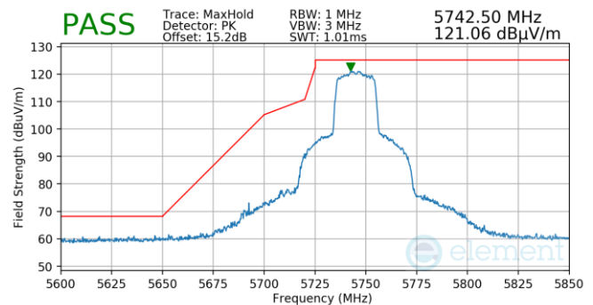
Plot 7-753. Antenna WF5T (Pk, Ch.149, 802.11ax(SU), MCS2)
