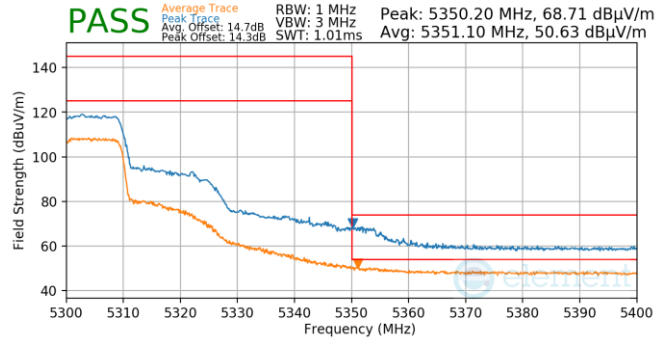
Plot 7-728. Antenna WF5T (Pk & Avg, Ch.60, 802.11ax(SU), MCS4)
