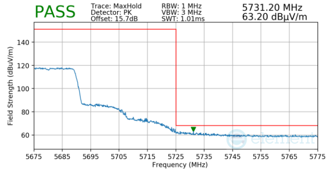
Plot 7-746. Antenna WF5T (Pk, Ch.132, 802.11ax(SU), MCS11)
