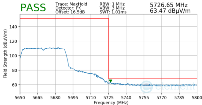
Plot 7-785. Antenna WF5T (Pk, Ch.134, 802.11n, MCS7)
