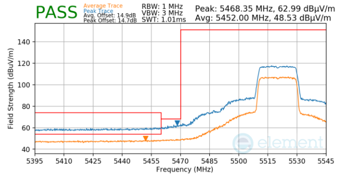
Plot 7-736. Antenna WF5T (Pk & Avg, Ch.104, 802.11ax(SU), MCS2)
