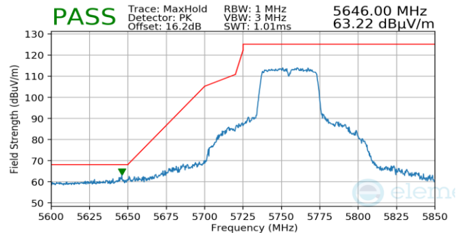
Plot 7-788. Antenna WF5T (Pk, Ch.151, 802.11n, MCS7)
