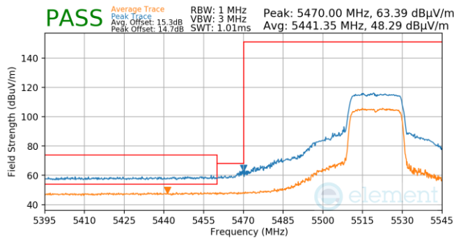
Plot 7-738. Antenna WF5T (Pk & Avg, Ch.104, 802.11ax(SU), MCS11)
