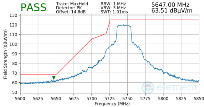
Plot 7-755. Antenna WF5T (Pk, Ch.149, 802.11ax(SU), MCS11)
