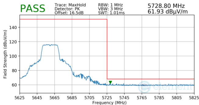
Plot 7-708. Antenna WF5T (Pk, Ch.132, 802.11n, MCS7)
