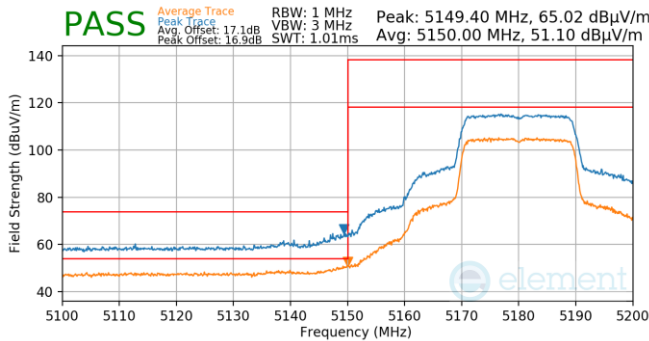
Plot 7-721. Antenna WF5T (Pk & Avg, Ch.36, 802.11ax(SU), MCS2)
