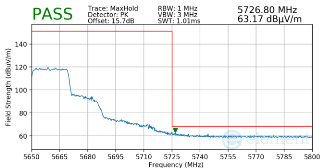
Plot 7-745. Antenna WF5T (Pk, Ch.132, 802.11ax(SU), MCS4)
