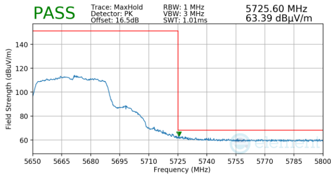
Plot 7-784. Antenna WF5T (Pk, Ch.134, 802.11n, MCS4)
