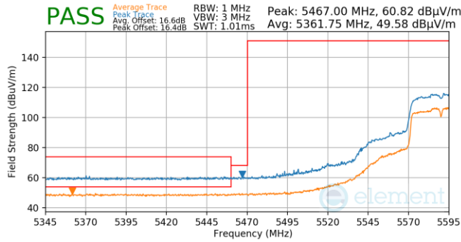
Plot 7-777. (FCC Only) Antenna WF5T (Pk & Avg, Ch.118, 802.11n, MCS2)
