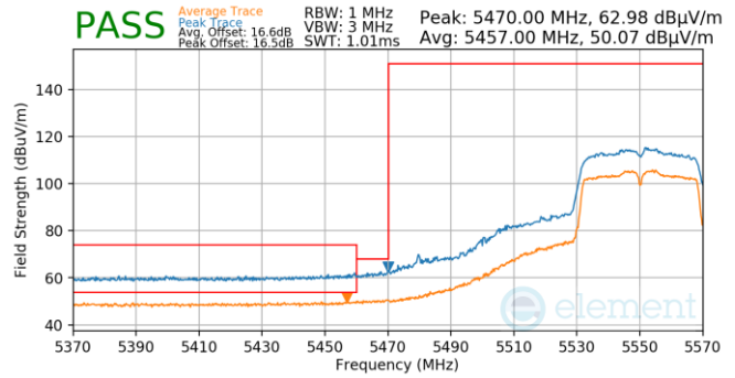
Plot 7-774. Antenna WF5T (Pk & Avg, Ch.110, 802.11n, MCS2)
