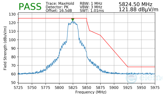
Plot 7-718. Antenna WF5T (Pk, Ch.165, 802.11n, MCS2)
