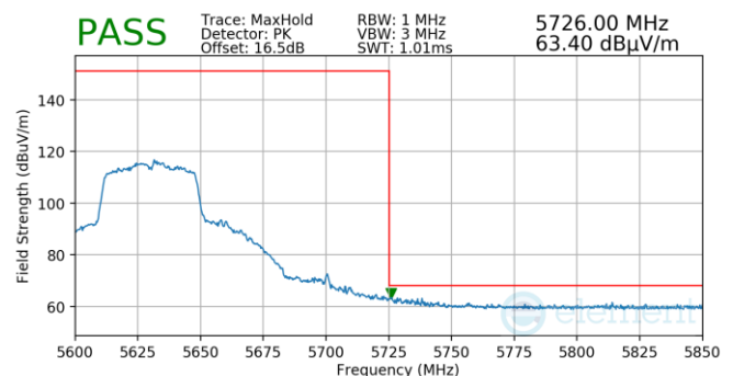
Plot 7-781. (FCC Only) Antenna WF5T (Pk, Ch.126, 802.11n, MCS4)
