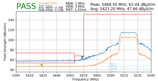
Plot 7-706. Antenna WF5T (Pk & Avg, Ch.104, 802.11n, MCS7)
