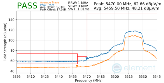
Plot 7-704. Antenna WF5T (Pk & Avg, Ch.104, 802.11n, MCS2)
