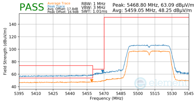
Plot 7-773. Antenna WF5T (Pk & Avg, Ch.102, 802.11n, MCS7)
