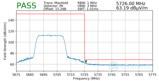
Plot 7-752. Antenna WF5T (Pk, Ch.140, 802.11ax(SU), MCS11)
