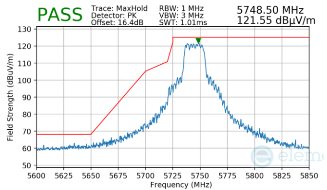
Plot 7-717. Antenna WF5T (Pk, Ch.149, 802.11n, MCS7)
