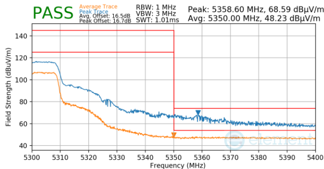
Plot 7-697. Antenna WF5T (Pk & Avg, Ch.60, 802.11n, MCS7)
