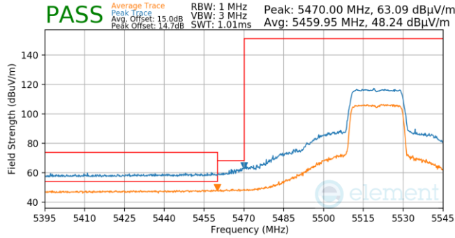
Plot 7-737. Antenna WF5T (Pk & Avg, Ch.104, 802.11ax(SU), MCS4)
