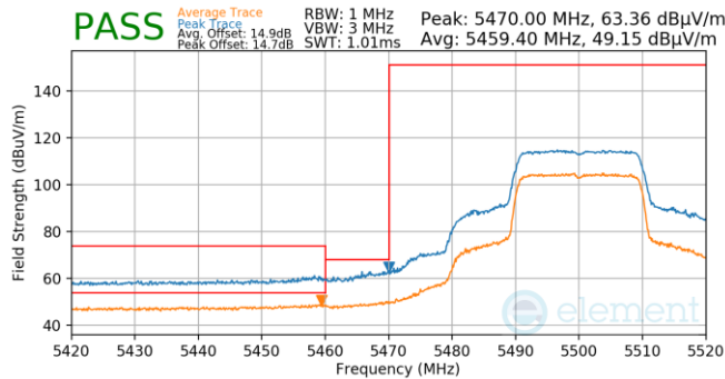
Plot 7-733. Antenna WF5T (Pk & Avg, Ch.100, 802.11ax(SU), MCS2)
