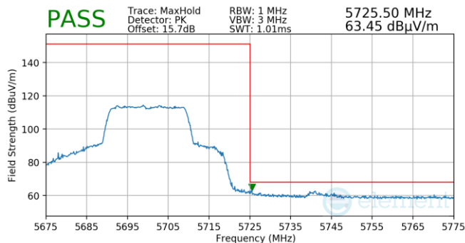
Plot 7-751. Antenna WF5T (Pk, Ch.140, 802.11ax(SU), MCS4)
