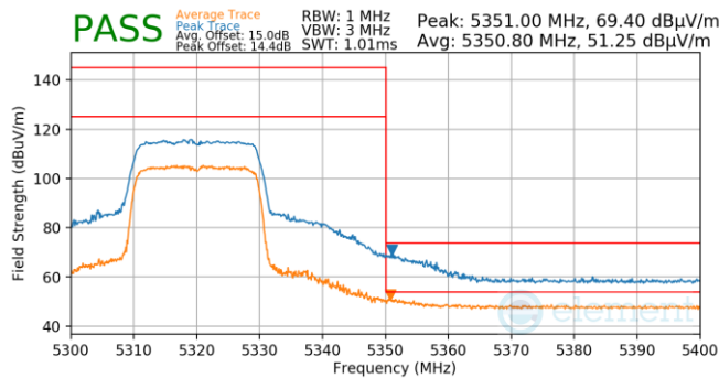
Plot 7-732. Antenna WF5T (Pk & Avg, Ch.64, 802.11ax(SU), MCS11)
