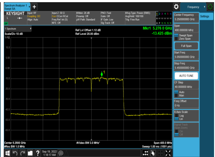
Plot 7-600. PSD CDD Antenna WF5B (160MHz BW 802.11ax(SU) – Ch. 50, MCS11)
