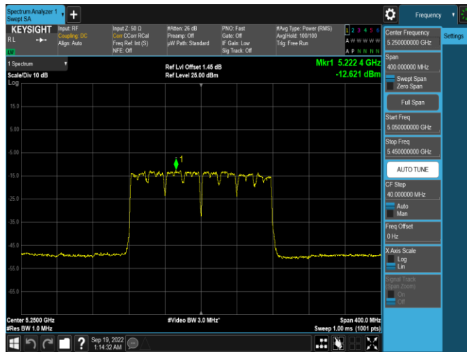
Plot 7-597. PSD CDD Antenna WF5T (160MHz BW 802.11ac – Ch. 50, MCS9)
