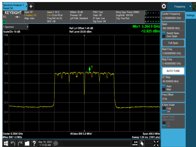
Plot 7-598. PSD CDD Antenna WF5B (160MHz BW 802.11ac – Ch. 50, MCS9)
