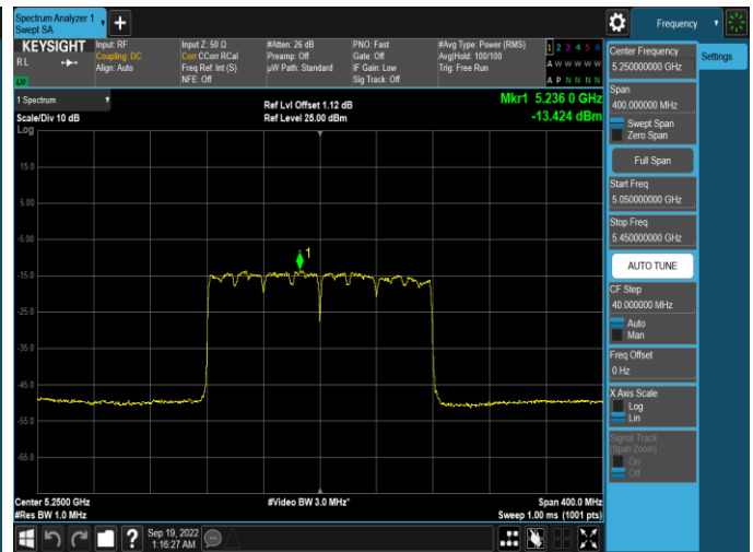
Plot 7-599. PSD CDD Antenna WF5T (160MHz BW 802.11ax(SU) – Ch. 50, MCS11)
