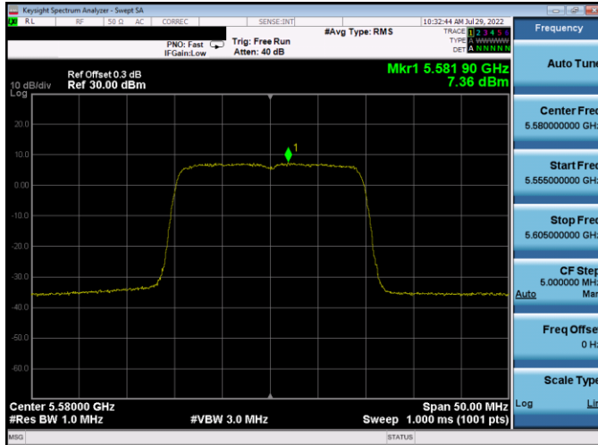
Plot 7-459. PSD CDD Antenna WF5T (20MHz BW 802.11ax(SU) – Ch. 116, MCS4)
