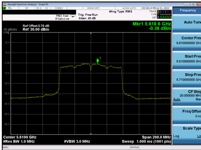
Plot 7-422. PSD CDD Antenna WF5B (80MHz BW 802.11ac - Ch. 122, MCS2)
