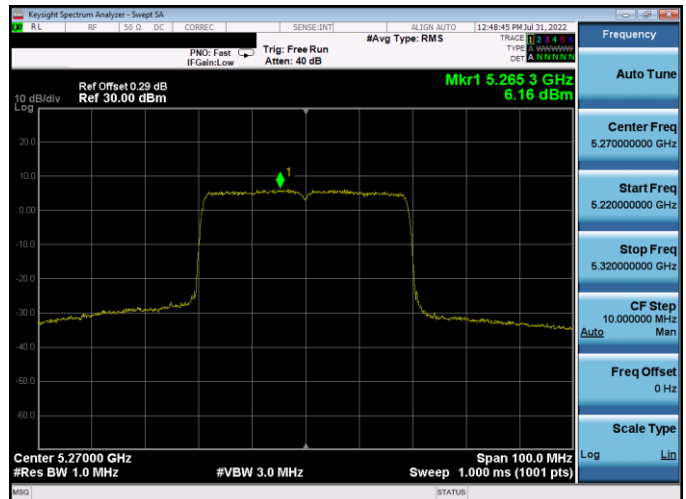
Plot 7-407. PSD CDD Antenna WF5T (40MHz BW 802.11ax(SU) – Ch. 54, MCS2)
