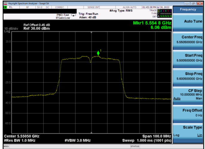
Plot 7-418. PSD SDM Antenna WF5B (40MHz BW 802.11n – Ch. 110, MCS10)
