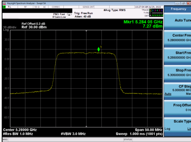
Plot 7-447. PSD CDD Antenna WF5T (20MHz BW 802.11ax(SU) – Ch. 56, MCS4)
