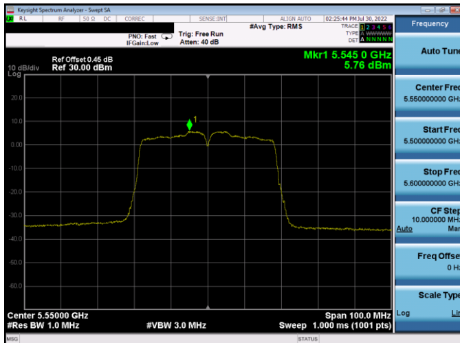
Plot 7-417. PSD SDM Antenna WF5T (40MHz BW 802.11n – Ch. 110, MCS10)
