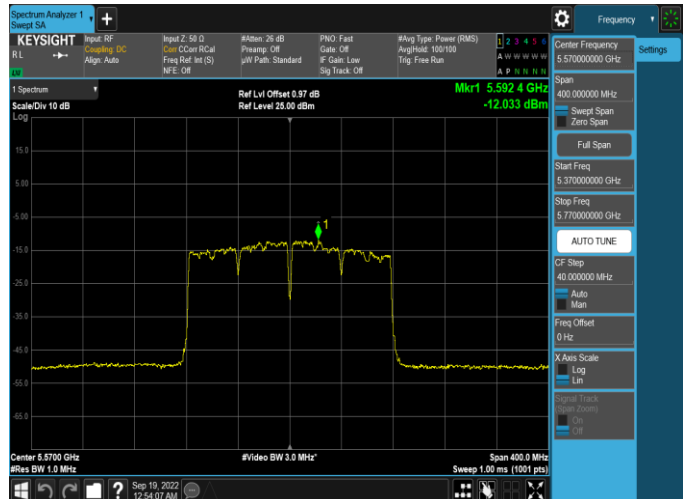
Plot 7-426. PSD CDD Antenna WF5B (160MHz BW 802.11ac - Ch. 114, MCS2)
