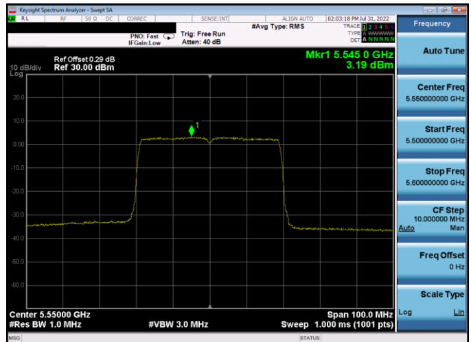
Plot 7-420. PSD SDM Antenna WF5B (40MHz BW 802.11ax(SU) – Ch. 110, MCS2)
