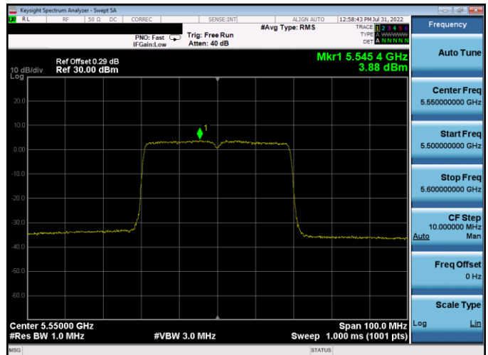
Plot 7-419. PSD SDM Antenna WF5T (40MHz BW 802.11ax(SU) – Ch. 110, MCS2)
