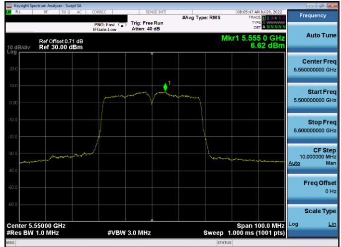
Plot 7-462. PSD CDD Antenna WF5B (40MHz BW 802.11n – Ch. 110, MCS12)
