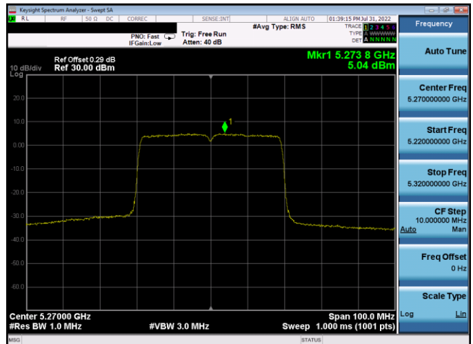
Plot 7-408. PSD CDD Antenna WF5B (40MHz BW 802.11ax(SU) – Ch. 54, MCS2)
