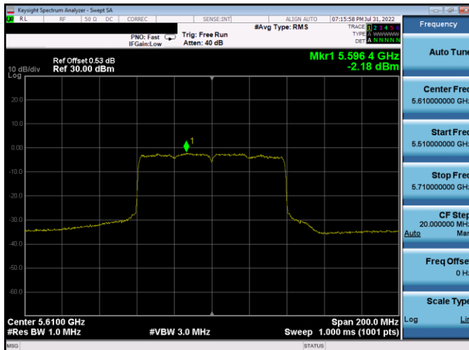
Plot 7-423. PSD CDD Antenna WF5T (80MHz BW 802.11ax(SU) - Ch. 122, MCS2)
