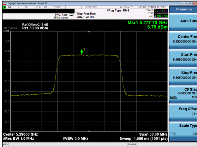
Plot 7-403. PSD CDD Antenna WF5T (20MHz BW 802.11ax(SU) – Ch. 56, MCS2)
