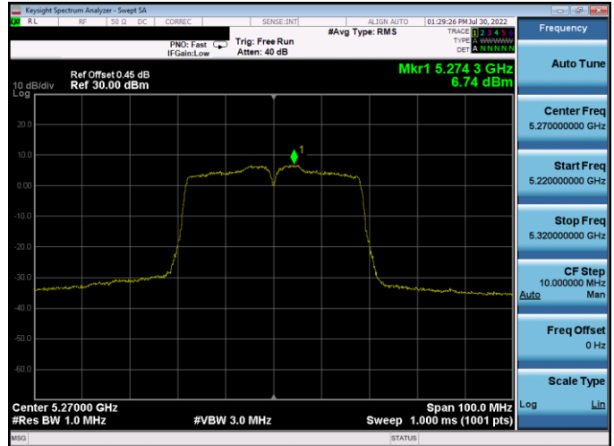
Plot 7-406. PSD CDD Antenna WF5B (40MHz BW 802.11n – Ch. 54, MCS10)
