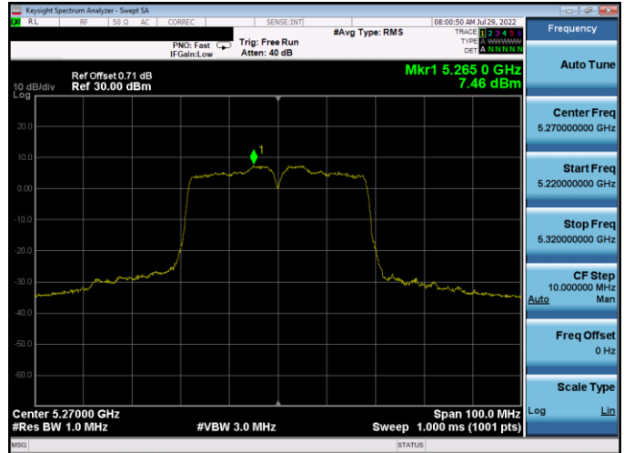
Plot 7-450. PSD CDD Antenna WF5B (40MHz BW 802.11n – Ch. 54, MCS12)
