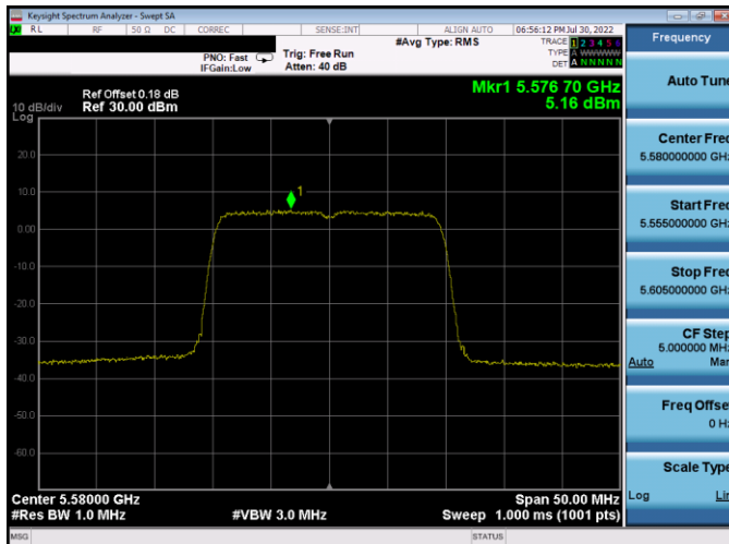
Plot 7-416. PSD SDM Antenna WF5B (20MHz BW 802.11ax(SU) – Ch. 116, MCS2)
