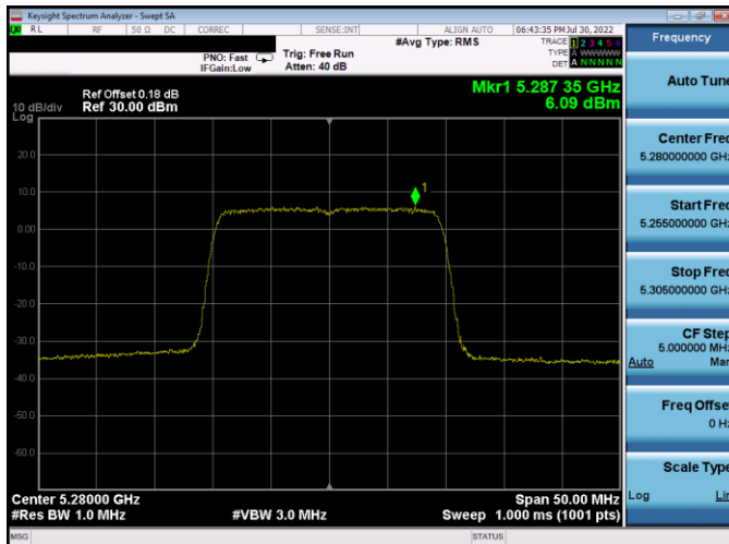
Plot 7-404. PSD CDD Antenna WF5B (20MHz BW 802.11ax(SU) – Ch. 56, MCS2)
