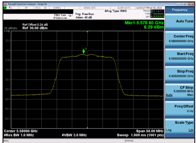
Plot 7-414. PSD SDM Antenna WF5B (20MHz BW 802.11n - Ch. 116, MCS10)
