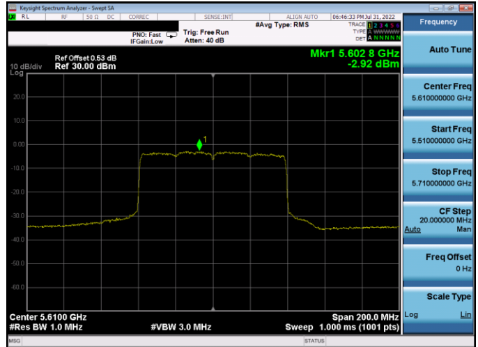
Plot 7-424. PSD CDD Antenna WF5B (80MHz BW 802.11ax(SU) - Ch. 122, MCS2)
