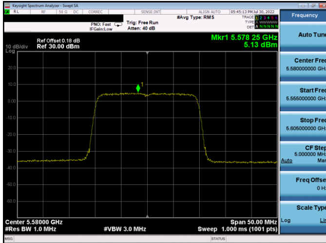
Plot 7-415. PSD SDM Antenna WF5T (20MHz BW 802.11ax(SU) – Ch. 116, MCS2)
