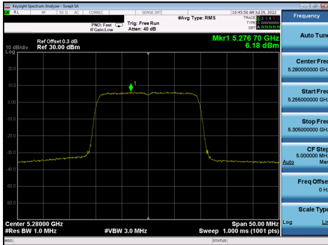
Plot 7-448. PSD CDD Antenna WF5B (20MHz BW 802.11ax(SU) – Ch. 56, MCS4)
