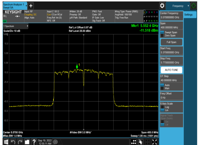
Plot 7-425. PSD CDD Antenna WF5T (160MHz BW 802.11ac - Ch. 114, MCS2)
