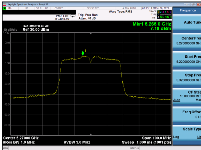
Plot 7-405. PSD CDD Antenna WF5T (40MHz BW 802.11n – Ch. 54, MCS10)
