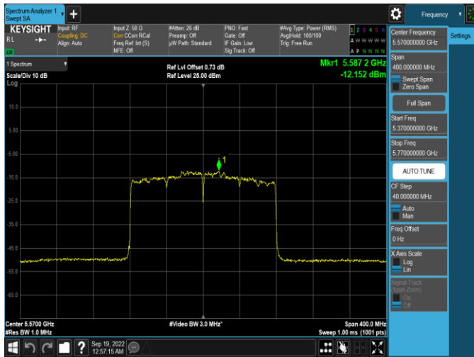
Plot 7-428. PSD CDD Antenna WF5B (160MHz BW 802.11ax(SU) – Ch. 114, MCS2)
