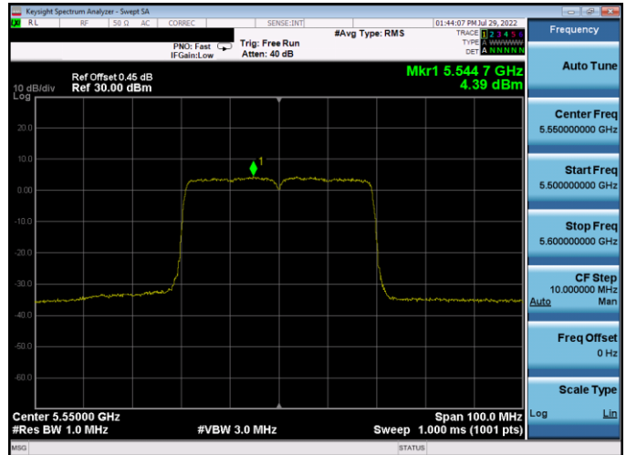
Plot 7-464. PSD CDD Antenna WF5B (40MHz BW 802.11ax(SU) – Ch. 110, MCS4)
