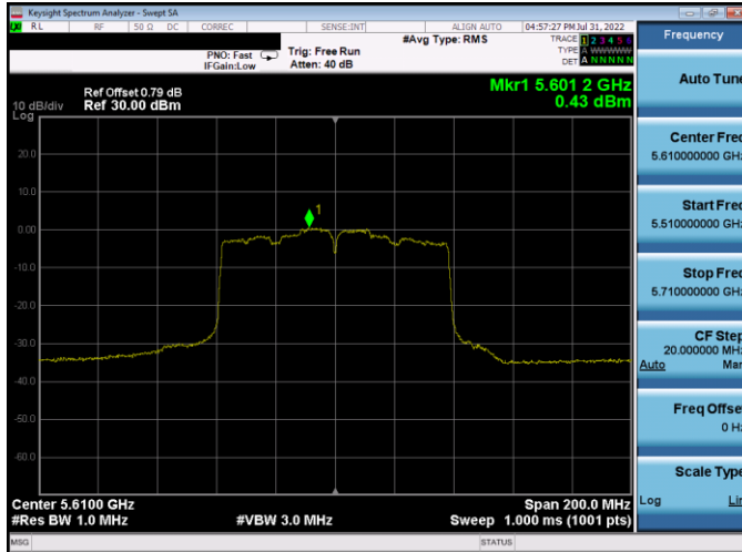
Plot 7-421. PSD CDD Antenna WF5T (80MHz BW 802.11ac - Ch. 122, MCS2)
