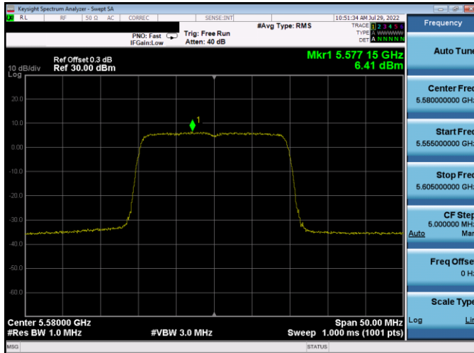
Plot 7-460. PSD CDD Antenna WF5B (20MHz BW 802.11ax(SU) – Ch. 116, MCS4)
