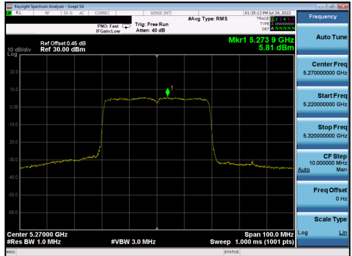
Plot 7-452. PSD CDD Antenna WF5B (40MHz BW 802.11ax(SU) – Ch. 54, MCS4)
