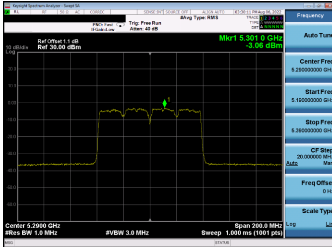
Plot 7-333. PSD Antenna WF5B (80MHz BW 802.11ac - Ch. 58, MCS9)
