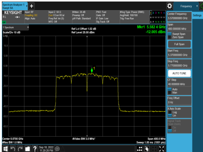
Plot 7-319. PSD Antenna WF5B (160MHz BW 802.11ac – Ch. 114, MC4)
