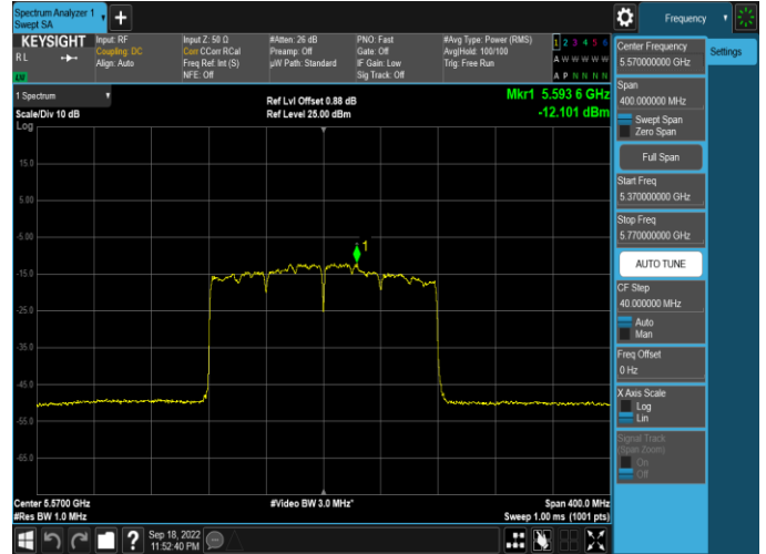
Plot 7-320. PSD Antenna WF5B (160MHz BW 802.11ax(SU) – Ch. 114, MCS4)
