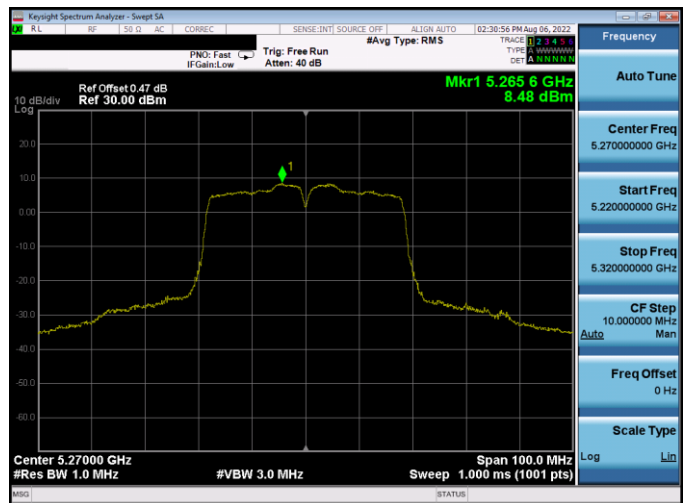
Plot 7-309. PSD Antenna WF5B (40MHz BW 802.11n – Ch. 54, MCS4)
