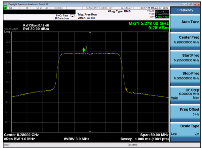
Plot 7-286. PSD Antenna WF5B (20MHz BW 802.11ax(SU) - Ch. 56, MCS2)
