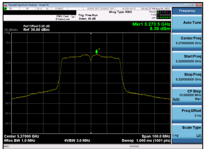
Plot 7-287. PSD Antenna WF5B (40MHz BW 802.11n - Ch. 54, MCS2)
