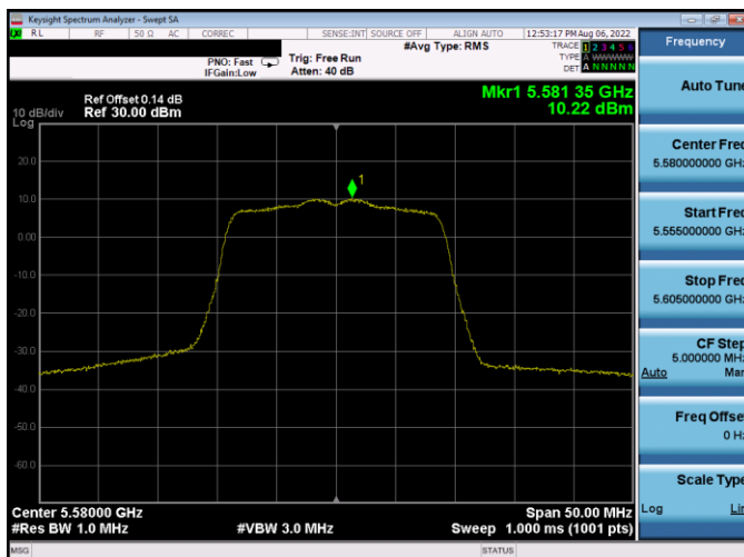
Plot 7-291. PSD Antenna WF5B (20MHz BW 802.11n - Ch. 116, MCS2)
