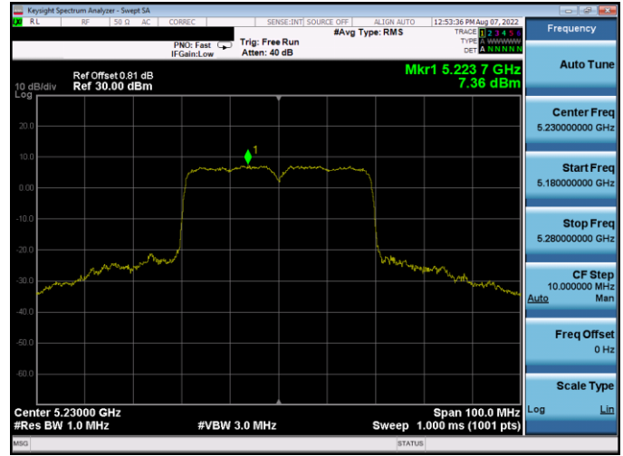
Plot 7-324. PSD Antenna WF5B (40MHz BW 802.11ax(SU) – Ch. 46, MCS11)
