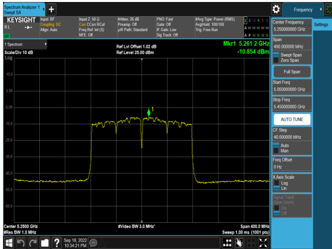
Plot 7-305. PSD Antenna WF5B (160MHz BW 802.11ac – Ch. 50, MCS4)
