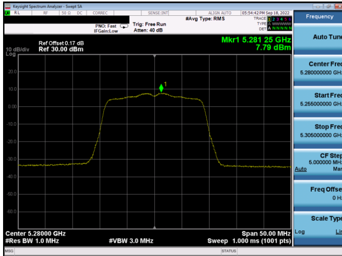
Plot 7-285. PSD Antenna WF5B (20MHz BW 802.11n - Ch. 56, MCS2)
