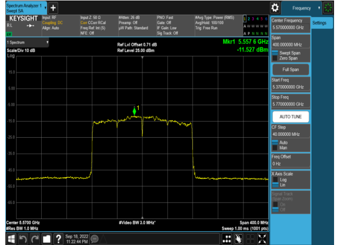
Plot 7-298. PSD Antenna WF5B (160MHz BW 802.11ax(SU) – Ch. 114, MCS2)
