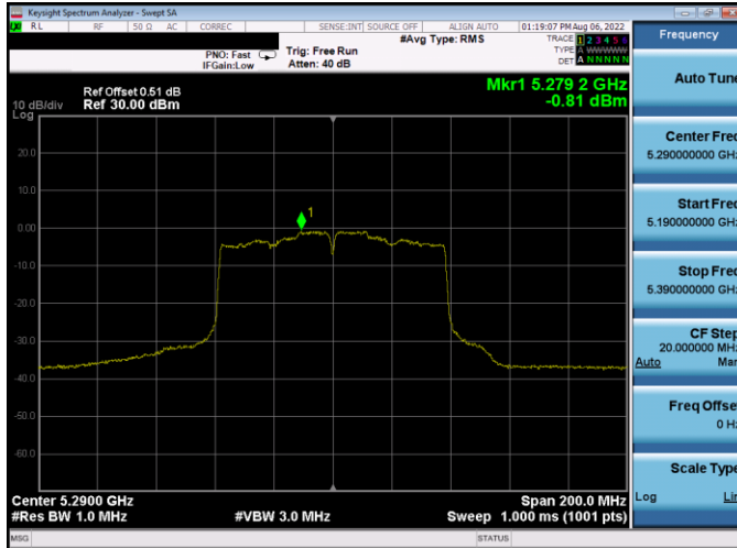
Plot 7-289. PSD Antenna WF5B (80MHz BW 802.11ac - Ch. 58, MCS2)
