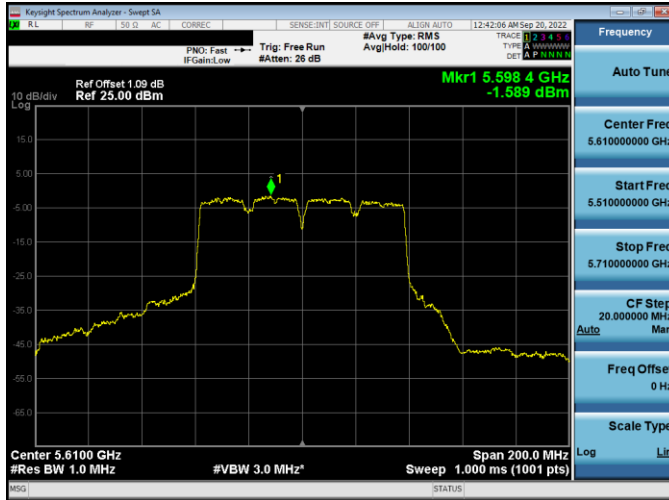
Plot 7-295. PSD Antenna WF5B (80MHz BW 802.11ac – Ch. 122, MCS2)
