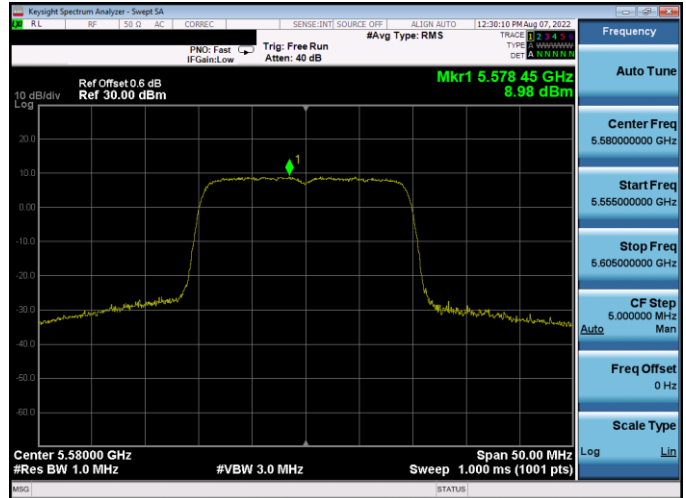
Plot 7-336. PSD Antenna WF5B (20MHz BW 802.11ax(SU) - Ch. 116, MCS11)
