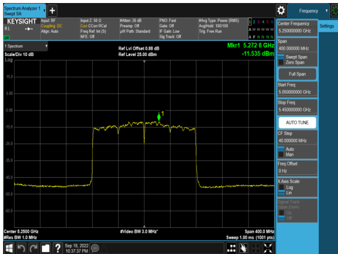
Plot 7-306. PSD Antenna WF5B (160MHz BW 802.11ax(SU) – Ch. 50, MCS4)
