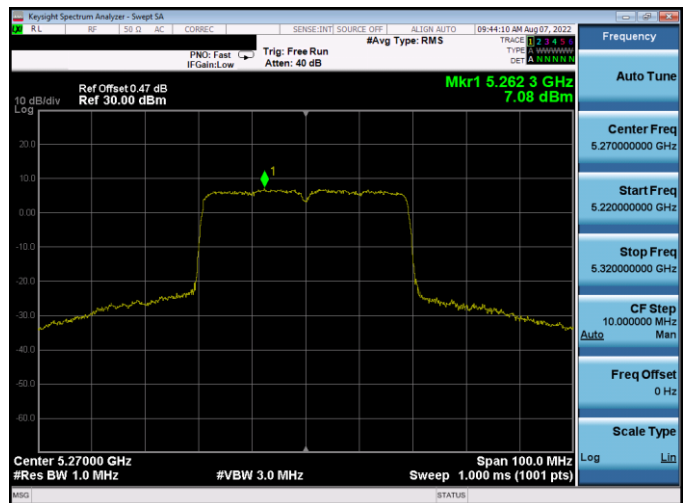
Plot 7-310. PSD Antenna WF5B (40MHz BW 802.11ax(SU) – Ch. 54, MCS4)
