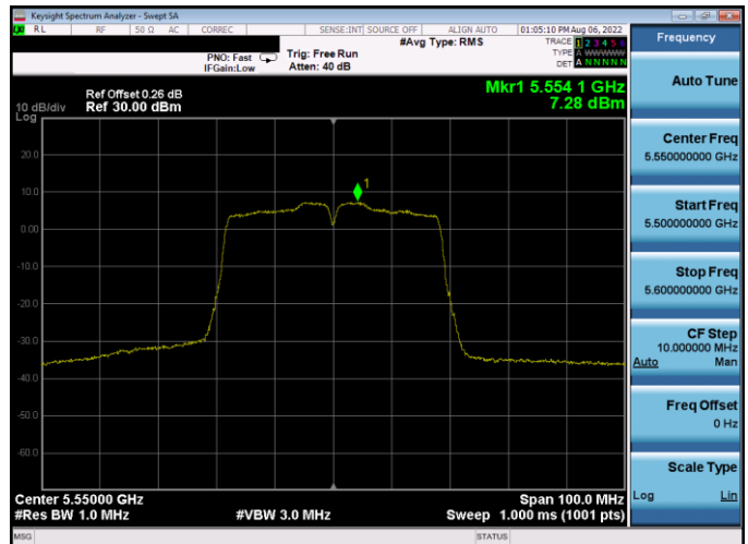
Plot 7-293. PSD Antenna WF5B (40MHz BW 802.11n - Ch. 110, MCS2)
