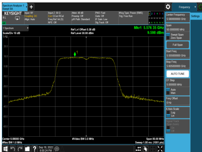
Plot 7-335. PSD Antenna WF5B (20MHz BW 802.11n - Ch. 116, MCS7)
