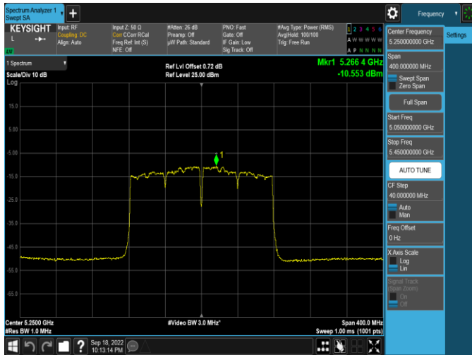
Plot 7-283. PSD Antenna WF5B (160MHz BW 802.11ac - Ch. 50, MCS2)
