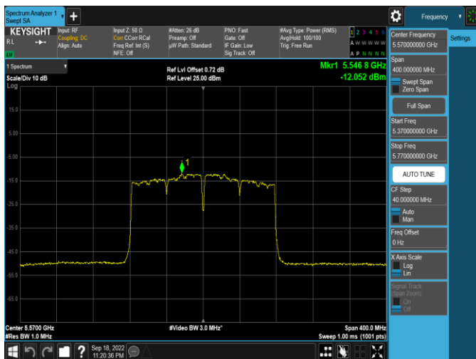
Plot 7-297. PSD Antenna WF5B (160MHz BW 802.11ac – Ch. 114, MCS2)
