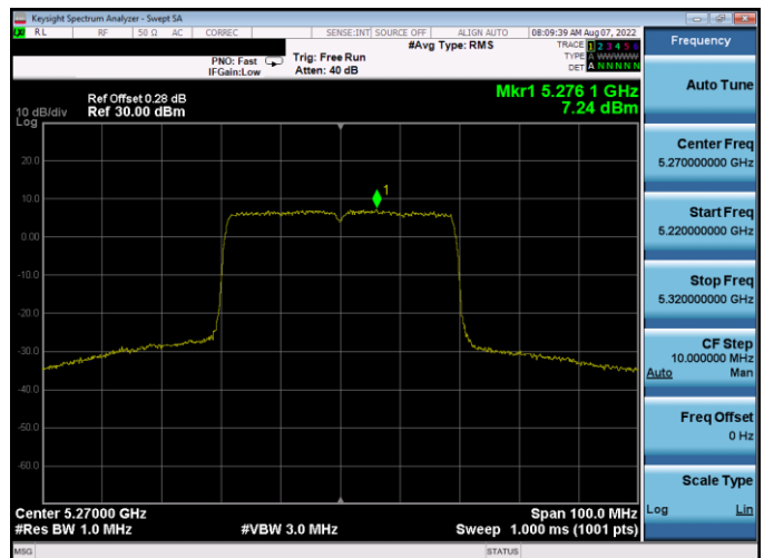
Plot 7-288. PSD Antenna WF5B (40MHz BW 802.11ax(SU) - Ch. 54, MCS2)
