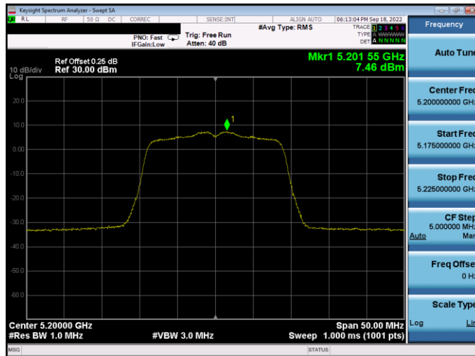
Plot 7-277. PSD Antenna WF5B (20MHz BW 802.11n - Ch. 40, MCS2)
