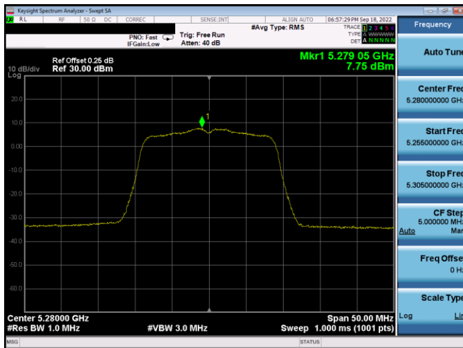
Plot 7-307. PSD Antenna WF5B (20MHz BW 802.11n – Ch. 56, MCS4)
