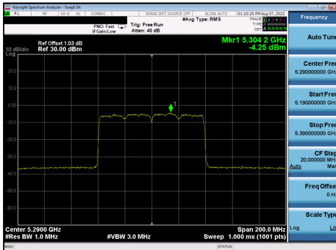
Plot 7-334. PSD Antenna WF5B (80MHz BW 802.11ax(SU) - Ch. 58, MCS11)
