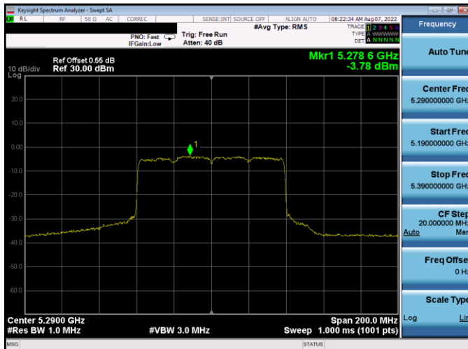
Plot 7-290. PSD Antenna WF5B (80MHz BW 802.11ax(SU) - Ch. 58, MCS2)
