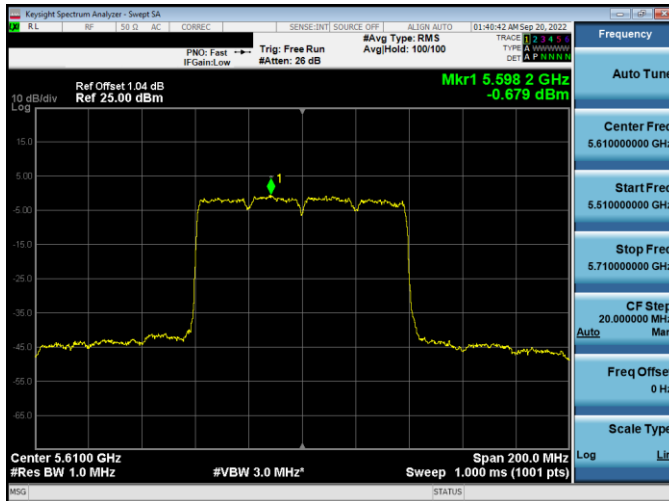
Plot 7-318. PSD Antenna WF5B (80MHz BW 802.11ax(SU) – Ch. 122, MCS4)
