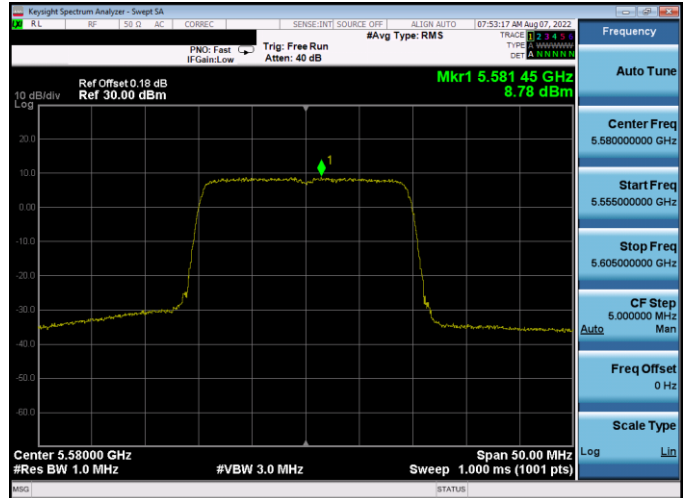
Plot 7-292. PSD Antenna WF5B (20MHz BW 802.11ax(SU) - Ch. 116, MCS2)
