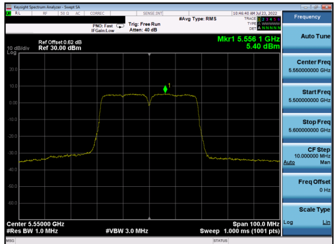
Plot 7-337. PSD Antenna WF5B (40MHz BW 802.11n - Ch. 110, MCS7)
