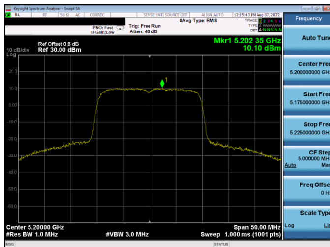
Plot 7-322. PSD Antenna WF5B (20MHz BW 802.11ax(SU) – Ch. 40, MCS11)
