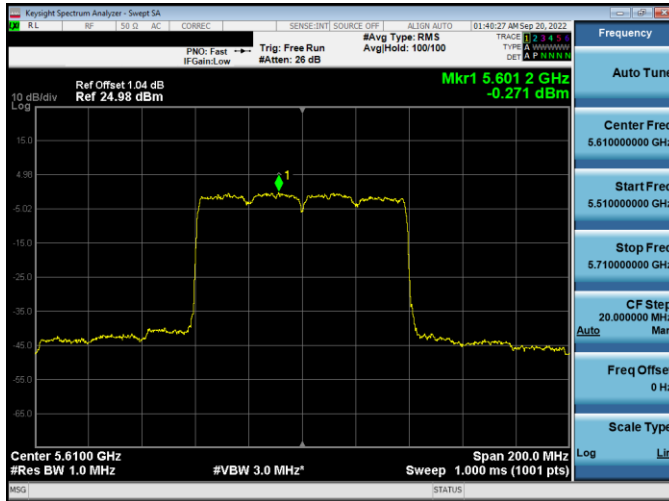
Plot 7-296. PSD Antenna WF5B (80MHz BW 802.11ax(SU) – Ch. 122, MCS2)
