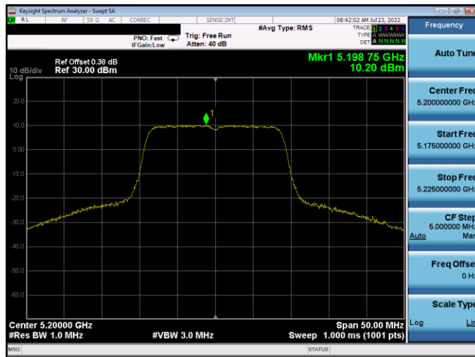
Plot 7-321. PSD Antenna WF5B (20MHz BW 802.11n – Ch. 40, MCS7)
