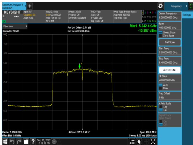
Plot 7-284. PSD Antenna WF5B (160MHz BW 802.11ax(SU) - Ch. 50, MCS2)
