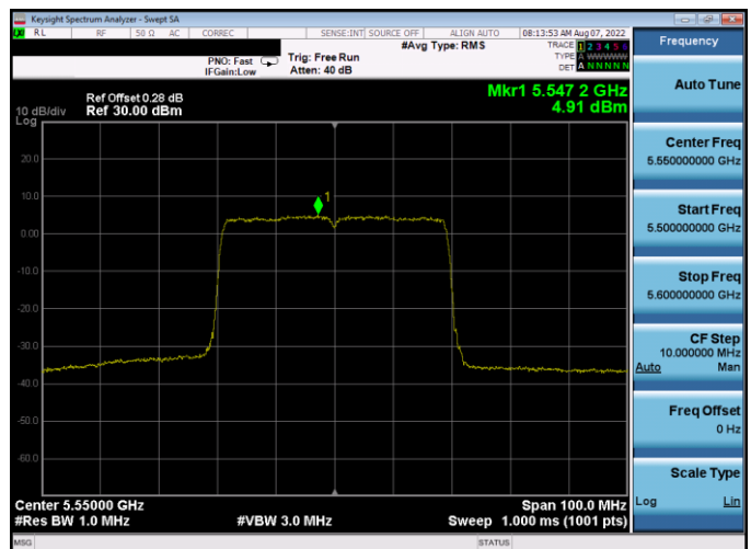
Plot 7-294. PSD Antenna WF5B (40MHz BW 802.11ax(SU) - Ch. 110, MCS2)
