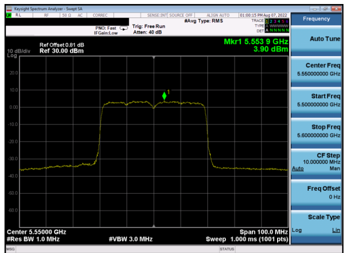
Plot 7-338. PSD Antenna WF5B (40MHz BW 802.11ax(SU) - Ch. 110, MCS11)
