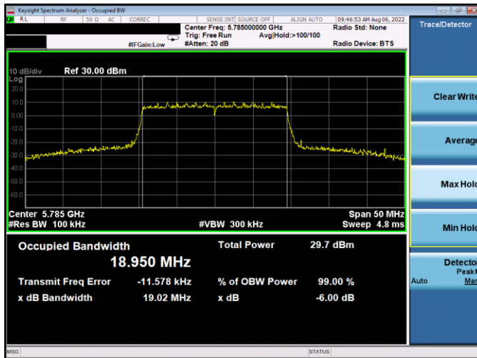
Plot 7-140. 6dB BW & 99% OBW Antenna WF5T (20MHz BW 802.11ax(SU) – Ch. 157, MCS4)
