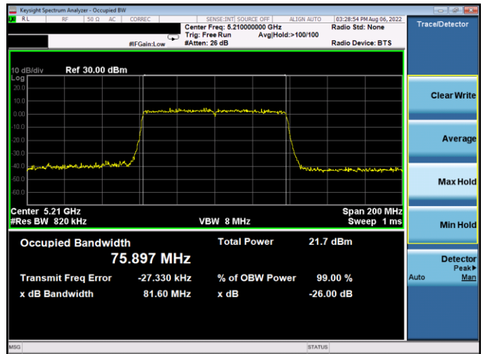
Plot 7-115. 26dB BW & 99% OBW Antenna WF5B (80MHz BW 802.11ac - Ch. 42, MCS9)
