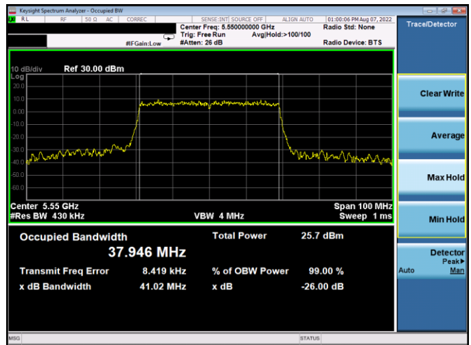
Plot 7-128. 26dB BW & 99% OBW Antenna WF5B (40MHz BW 802.11ax(SU) – Ch. 110, MCS11)
