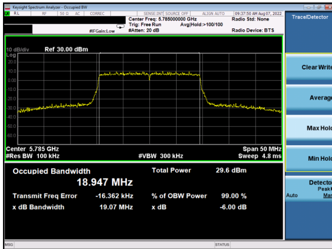
Plot 7-158. 6dB BW & 99% OBW Antenna WF5B (20MHz BW 802.11ax(SU) – Ch. 157, MCS4)
