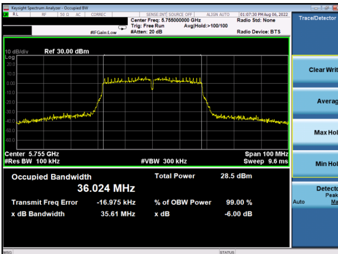
Plot 7-153. 6dB BW & 99% OBW Antenna WF5B (40MHz BW 802.11n - Ch. 151, MCS2)
