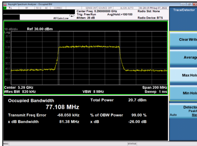
Plot 7-124. 26dB BW & 99% OBW Antenna WF5B (80MHz BW 802.11ax(SU) – Ch. 58, MCS11)
