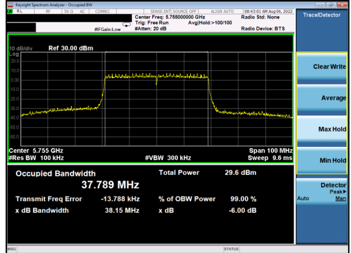
Plot 7-136. 6dB BW & 99% OBW Antenna WF5T (40MHz BW 802.11ax(SU) – Ch. 151, MCS2)
