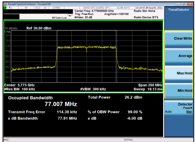
Plot 7-144. 6dB BW & 99% OBW Antenna WF5T (80MHz BW 802.11ax(SU) – Ch. 155, MCS4)
