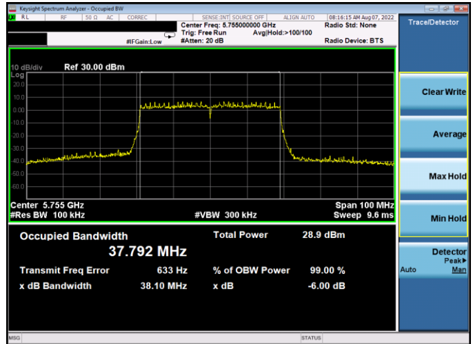
Plot 7-154. 6dB BW & 99% OBW Antenna WF5B (40MHz BW 802.11ax(SU) - Ch. 151, MCS2)
