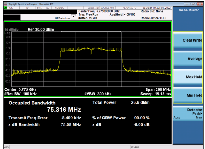
Plot 7-155. 6dB BW & 99% OBW Antenna WF5B (80MHz BW 802.11ac - Ch. 155, MCS2)
