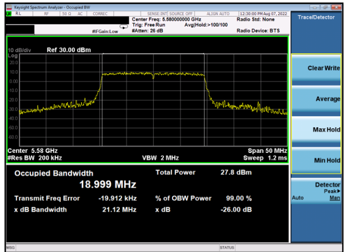
Plot 7-126. 26dB BW & 99% OBW Antenna WF5B (20MHz BW 802.11ax(SU) – Ch. 116, MCS11)
