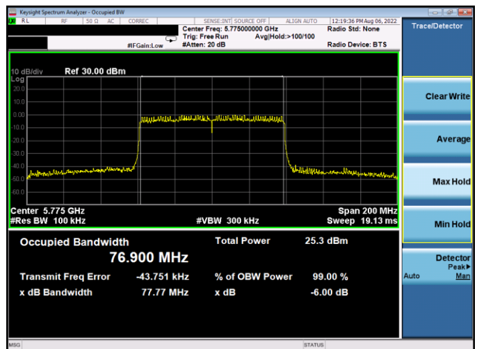
Plot 7-150. 6dB BW & 99% OBW Antenna WF5T (80MHz BW 802.11ax(SU) – Ch. 155, MCS11)
