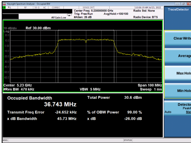
Plot 7-113. 26dB BW & 99% OBW Antenna WF5B (40MHz BW 802.11n - Ch. 46, MCS7)
