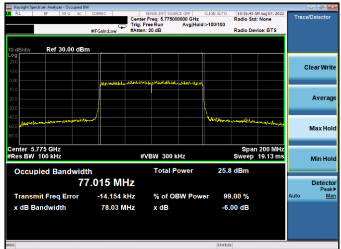
Plot 7-162. 6dB BW & 99% OBW Antenna WF5B (80MHz BW 802.11ax(SU) – Ch. 155, MCS4)
