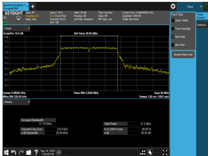
Plot 7-125. 26dB BW & 99% OBW Antenna WF5B (20MHz BW 802.11n – Ch. 116, MCS7)
