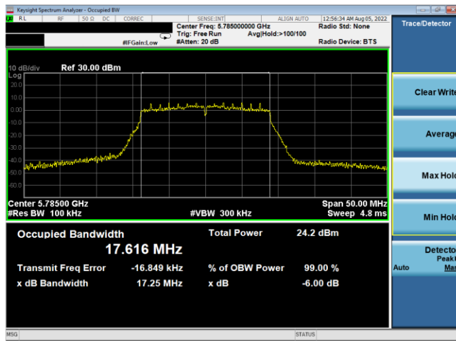
Plot 7-151. 6dB BW & 99% OBW Antenna WF5B (20MHz BW 802.11n - Ch. 157, MCS2)
