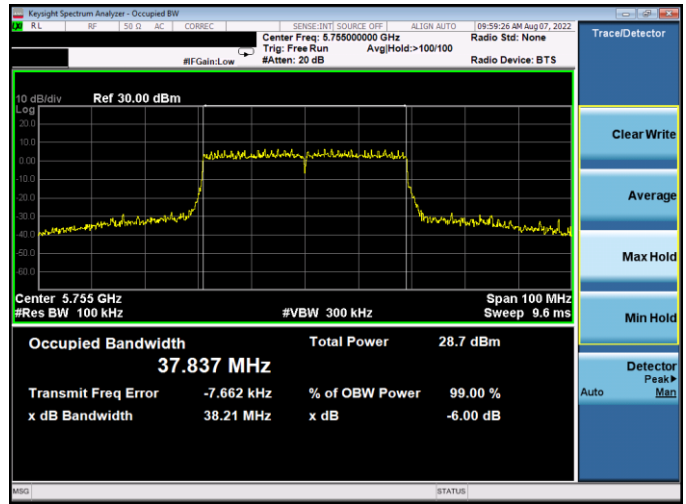
Plot 7-160. 6dB BW & 99% OBW Antenna WF5B (40MHz BW 802.11ax(SU) – Ch. 151, MCS4)
