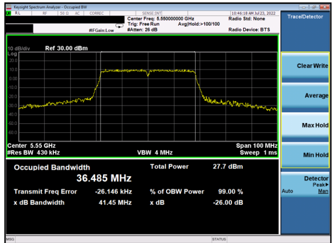
Plot 7-127. 26dB BW & 99% OBW Antenna WF5B (40MHz BW 802.11n – Ch. 110, MCS7)
