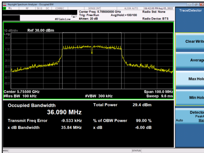
Plot 7-141. 6dB BW & 99% OBW Antenna WF5T (40MHz BW 802.11n – Ch. 151, MCS4)
