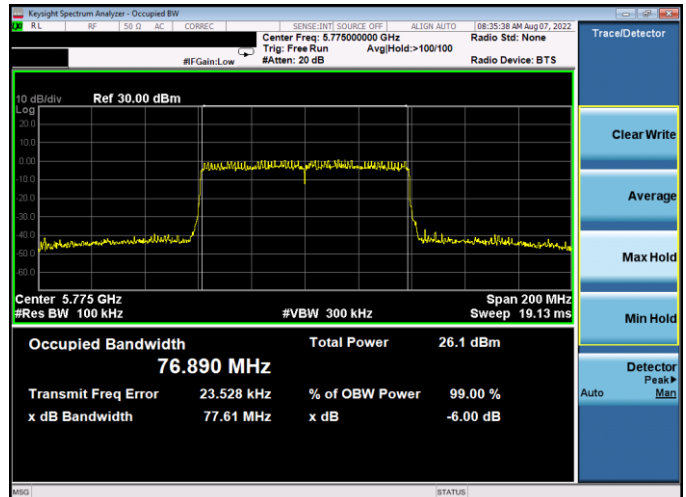
Plot 7-156. 6dB BW & 99% OBW Antenna WF5B (80MHz BW 802.11ax(SU) - Ch. 155, MCS2)
