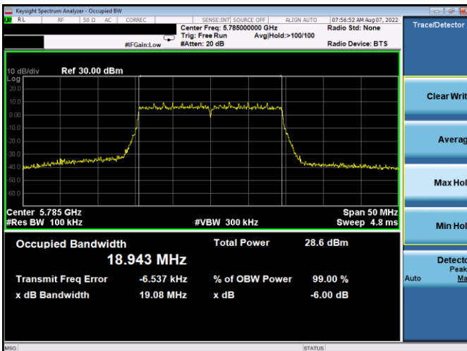
Plot 7-152. 6dB BW & 99% OBW Antenna WF5B (20MHz BW 802.11ax(SU) - Ch. 157, MCS2)
