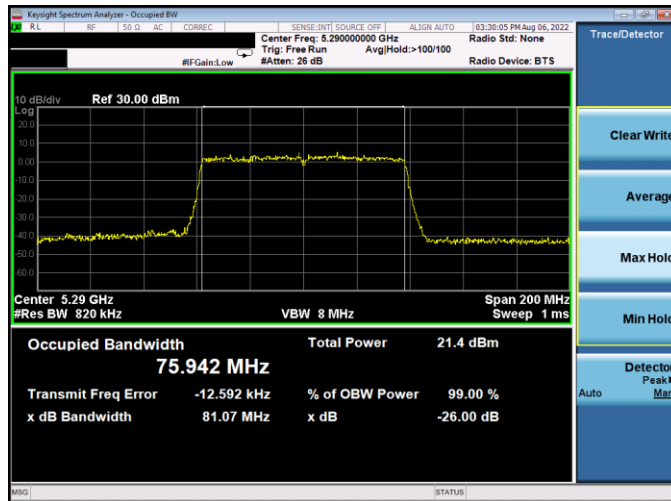
Plot 7-123. 26dB BW & 99% OBW Antenna WF5B (80MHz BW 802.11ac – Ch. 58, MCS9)
