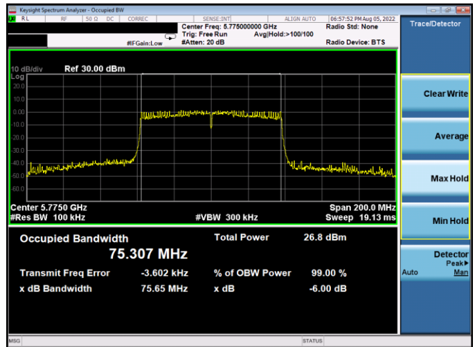
Plot 7-143. 6dB BW & 99% OBW Antenna WF5T (80MHz BW 802.11ac – Ch. 155, MCS4)
