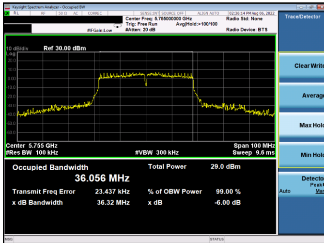
Plot 7-159. 6dB BW & 99% OBW Antenna WF5B (40MHz BW 802.11n – Ch. 151, MCS4)
