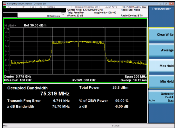
Plot 7-161. 6dB BW & 99% OBW Antenna WF5B (80MHz BW 802.11ac – Ch. 155, MCS4)
