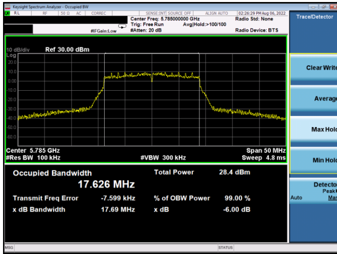
Plot 7-157. 6dB BW & 99% OBW Antenna WF5B (20MHz BW 802.11n – Ch. 157, MCS4)
