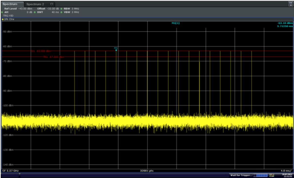
Figure 7-4. 5570MHz – Radar Pulse Type 0 (160MHz)
