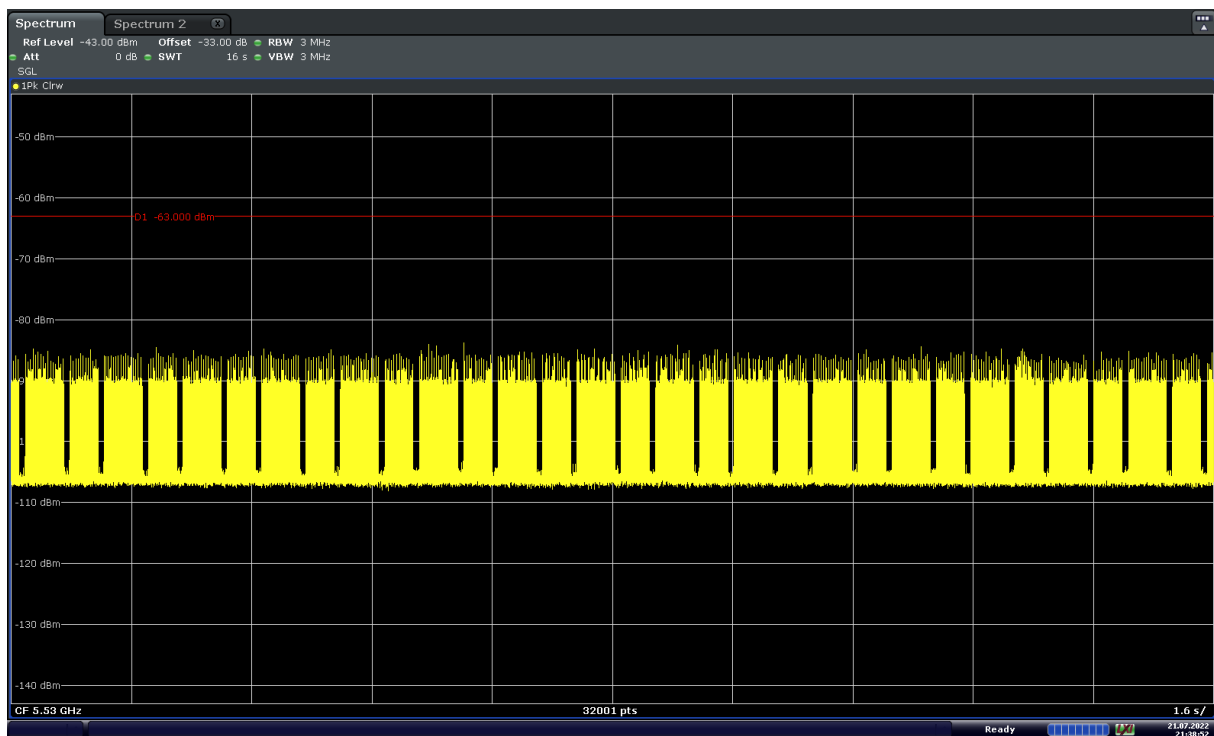
Figure 9-7. 5530MHz - Channel Loading - Mode 3 (80MHz)
