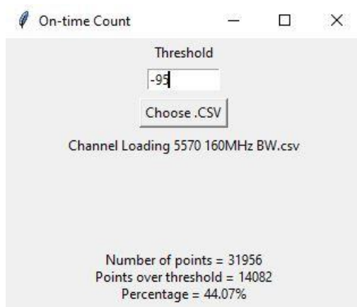
Figure 9-4. 5570MHz - Channel Loading Calculation - Mode 1 (160MHz)
